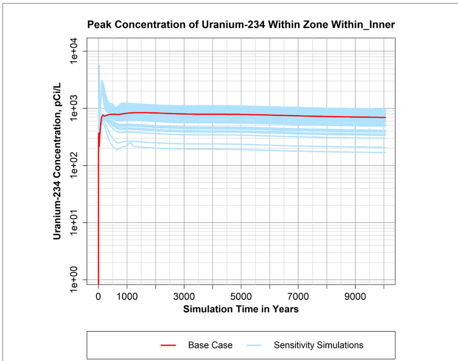
Figure B-40. Peak simulated concentration of Uranium-234 over time within the "Within_Inner" zone defined within the P2R Model version 8.3 domain.
