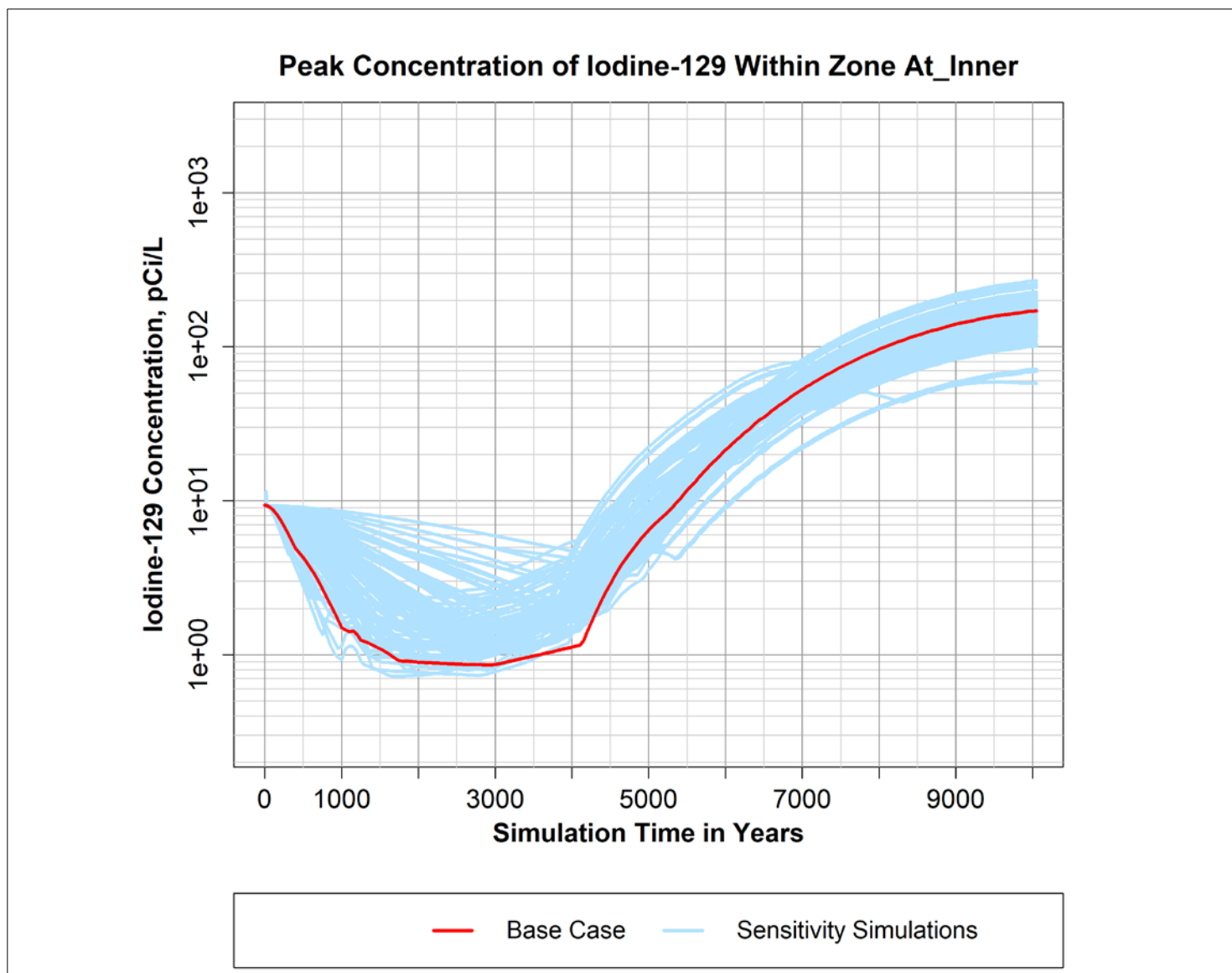
Figure B-4. Peak simulated concentration of Iodine-129 over time within the "At_Inner" zone defined within the P2R Model version 8.3 domain.
