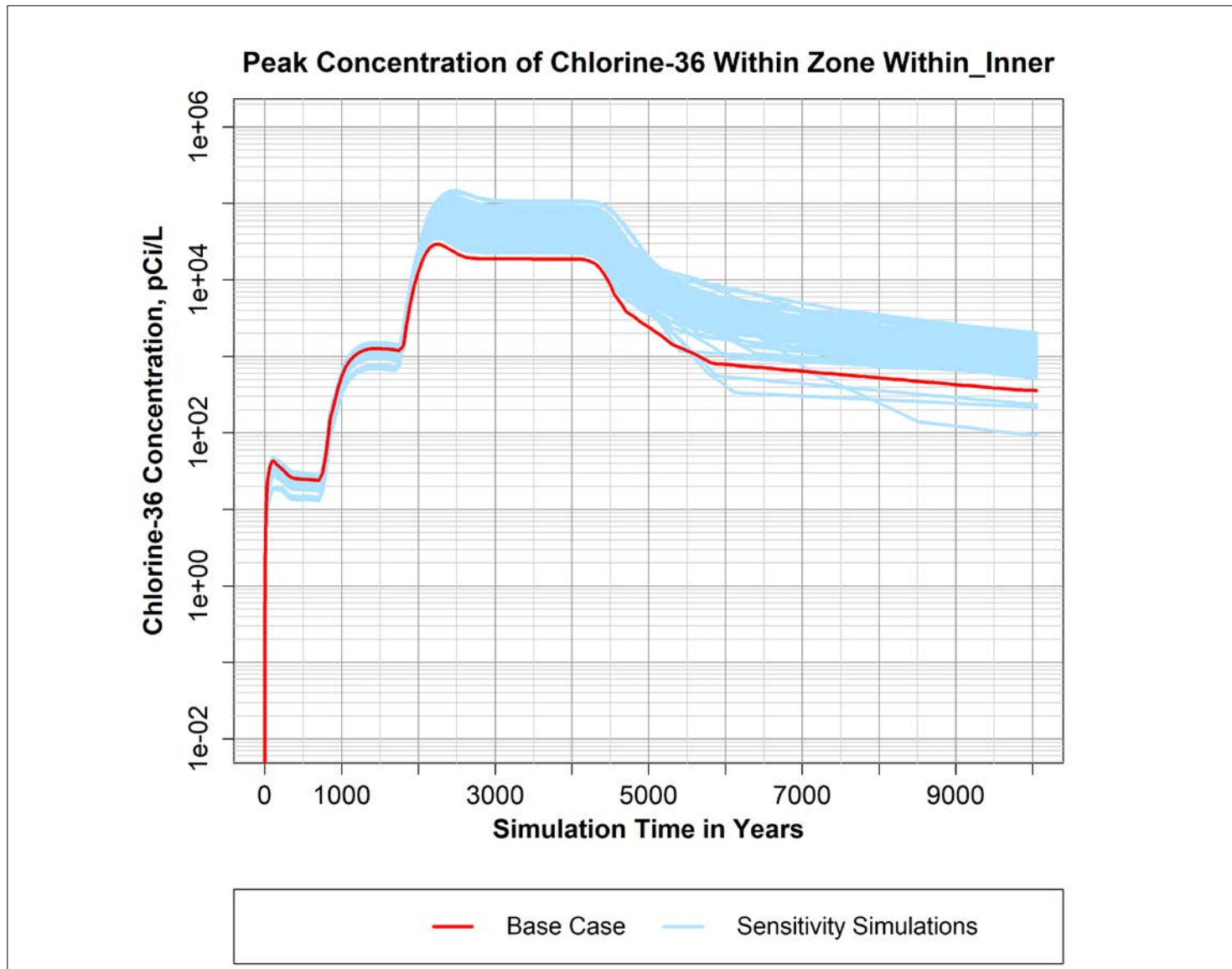
Figure B-30. Peak simulated concentration of Chlorine-36 over time within the "Within_Inner" zone defined within the P2R Model version 8.3 domain.
