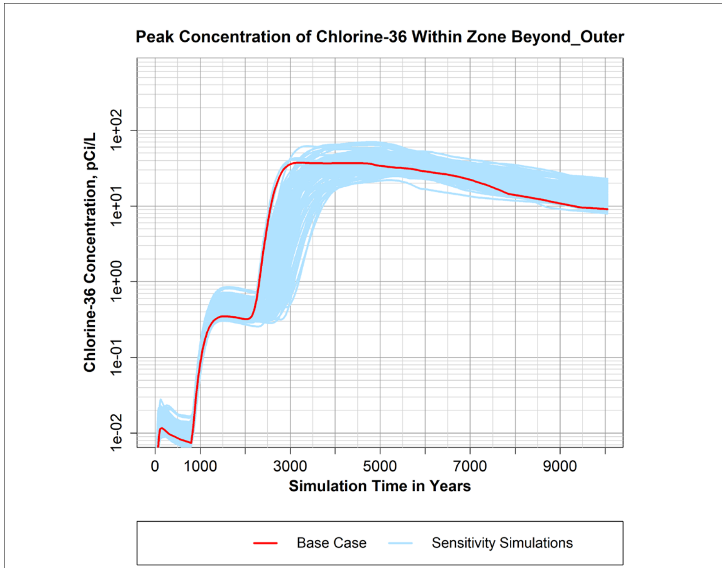
Figure B-26. Peak simulated concentration of Chlorine-36 over time within the "Beyond_Outer" zone defined within the P2R Model version 8.3 domain.
