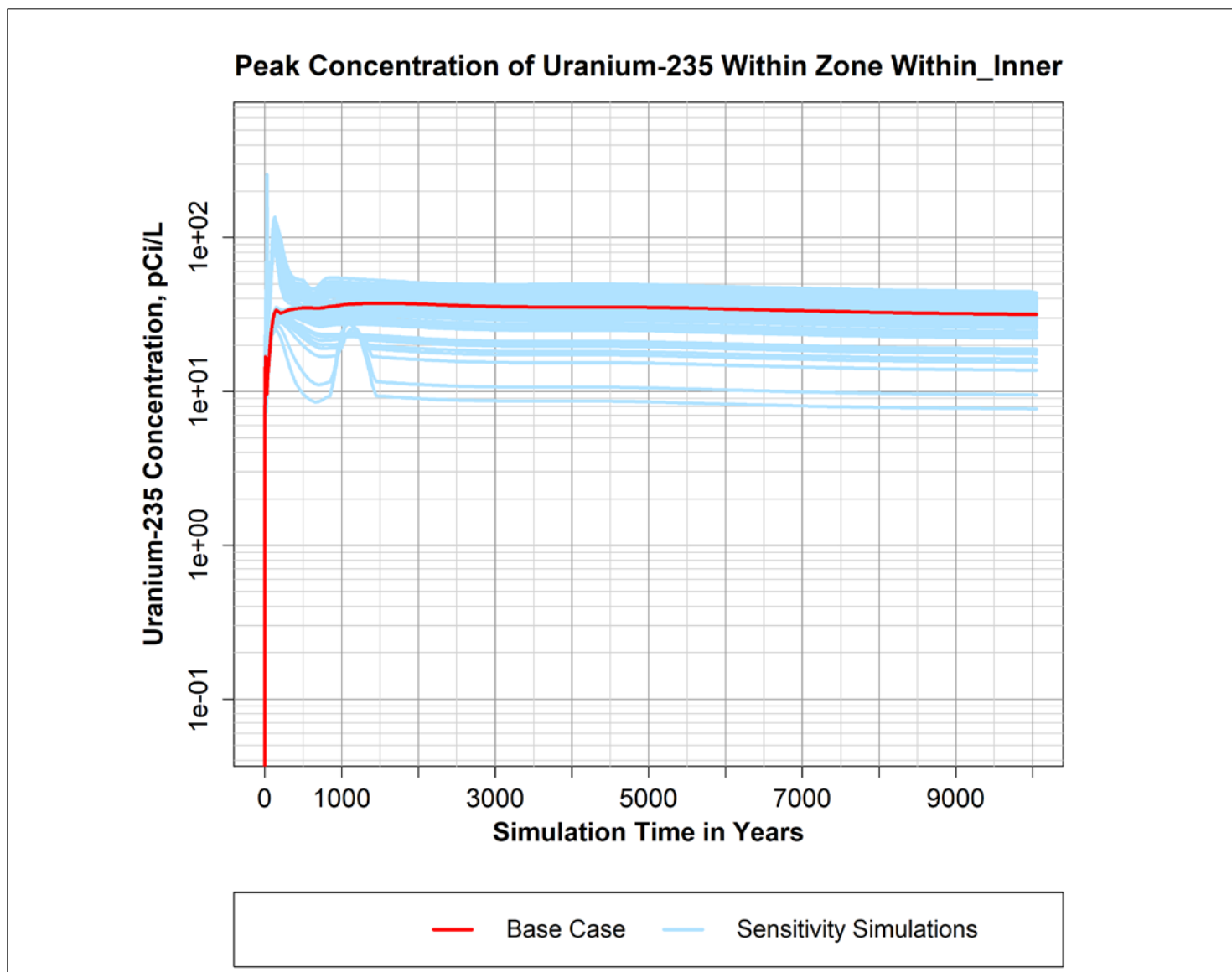
Figure B-45. Peak simulated concentration of Uranium-235 over time within the "Within_Inner" zone defined within the P2R Model version 8.3 domain.
