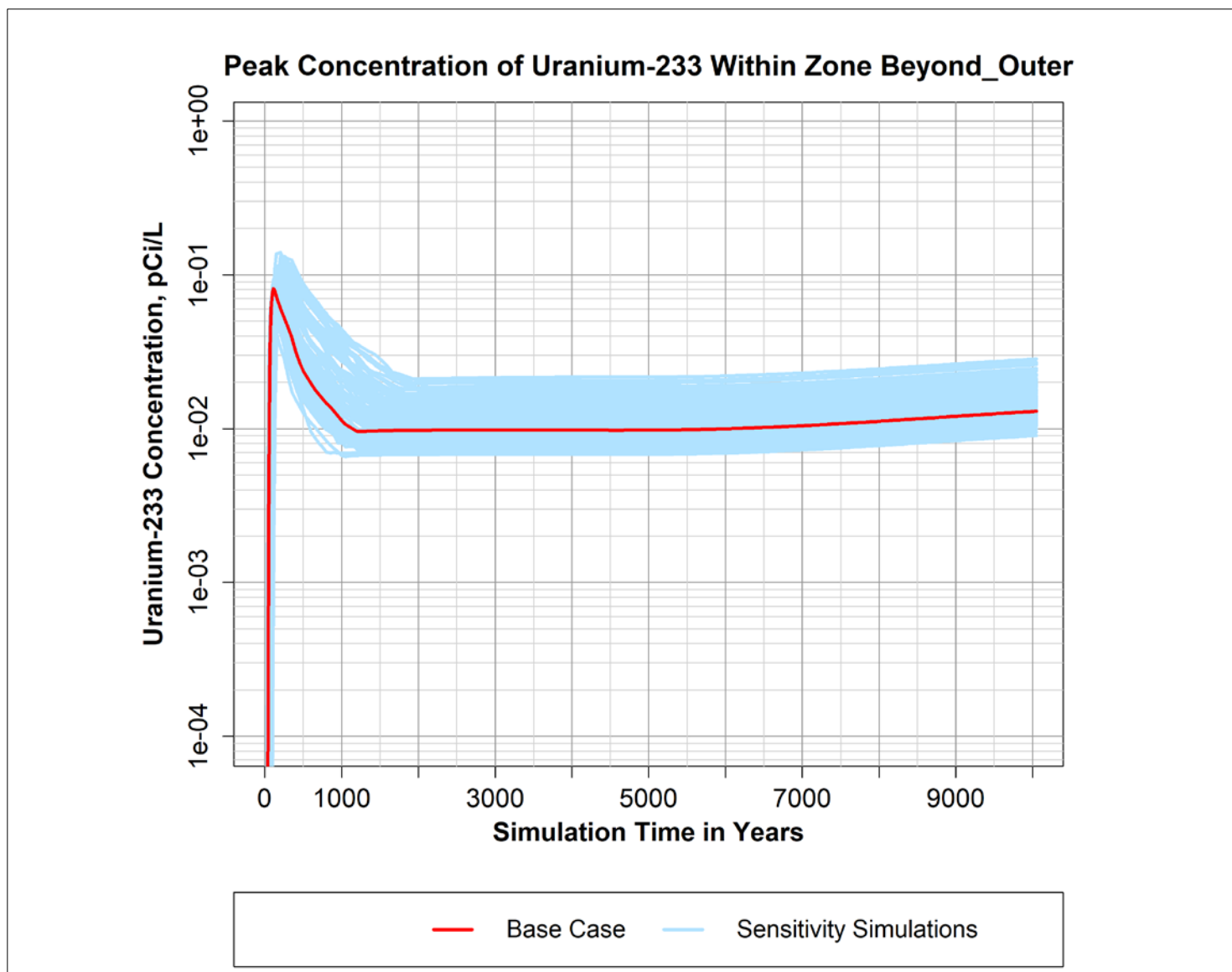
Figure B-31. Peak simulated concentration of Uranium-233 over time within the "Beyond_Outer" zone defined within the P2R Model version 8.3 domain.
