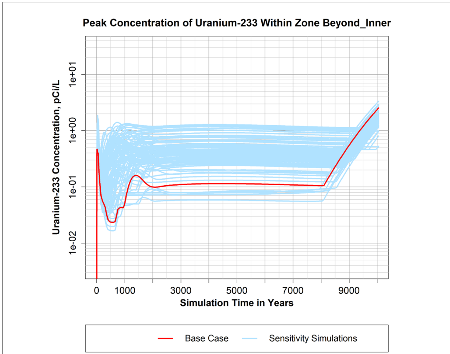
Figure B-33. Peak simulated concentration of Uranium-233 over time within the "Beyond_Inner" zone defined within the P2R Model version 8.3 domain.
