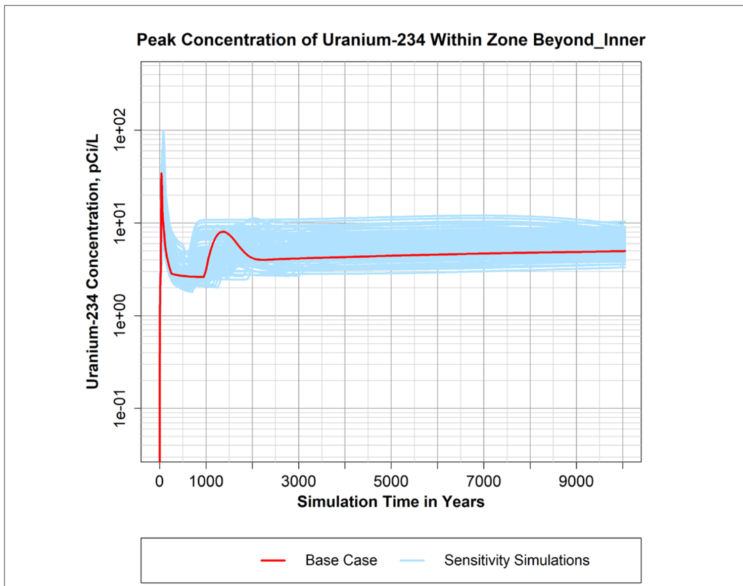
Figure B-38. Peak simulated concentration of Uranium-234 over time within the "Beyond_Inner" zone defined within the P2R Model version 8.3 domain.
