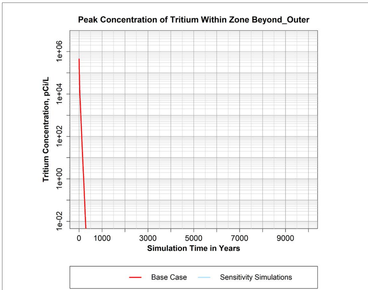
Figure B-11. Peak simulated concentration of Tritium over time within the "Beyond_Outer" zone defined within the P2R Model version 8.3 domain.
