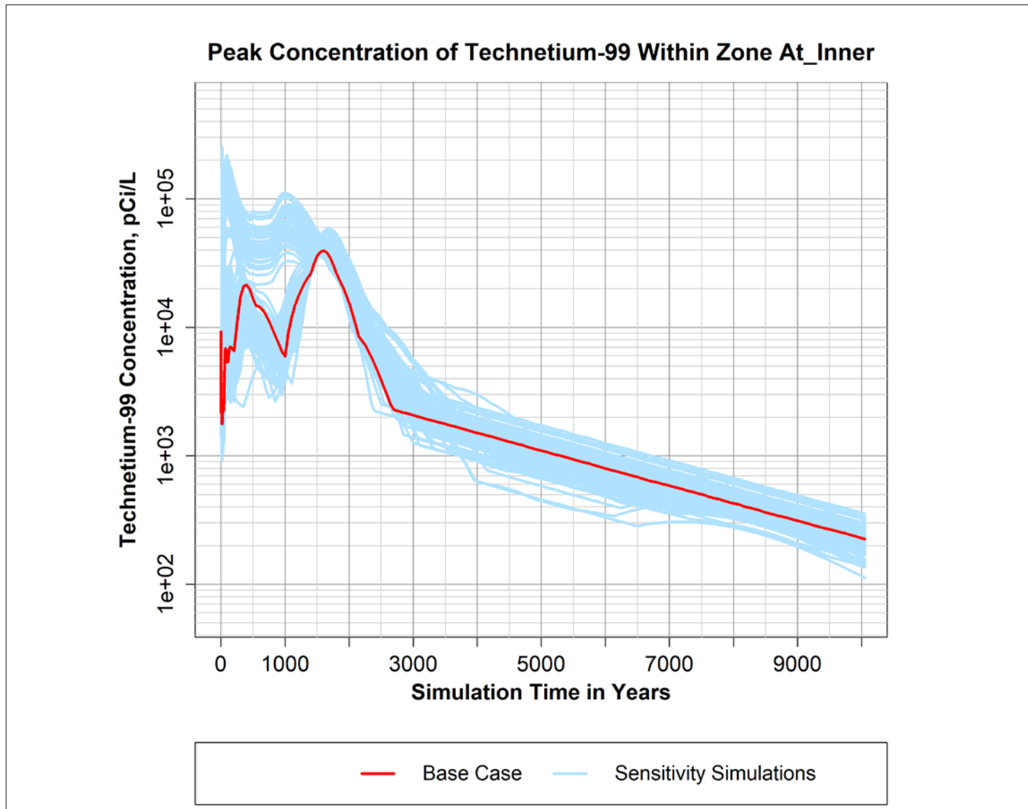
Figure B-9. Peak simulated concentration of Technetium-99 over time within the "At_Inner" zone defined within the P2R Model version 8.3 domain.
