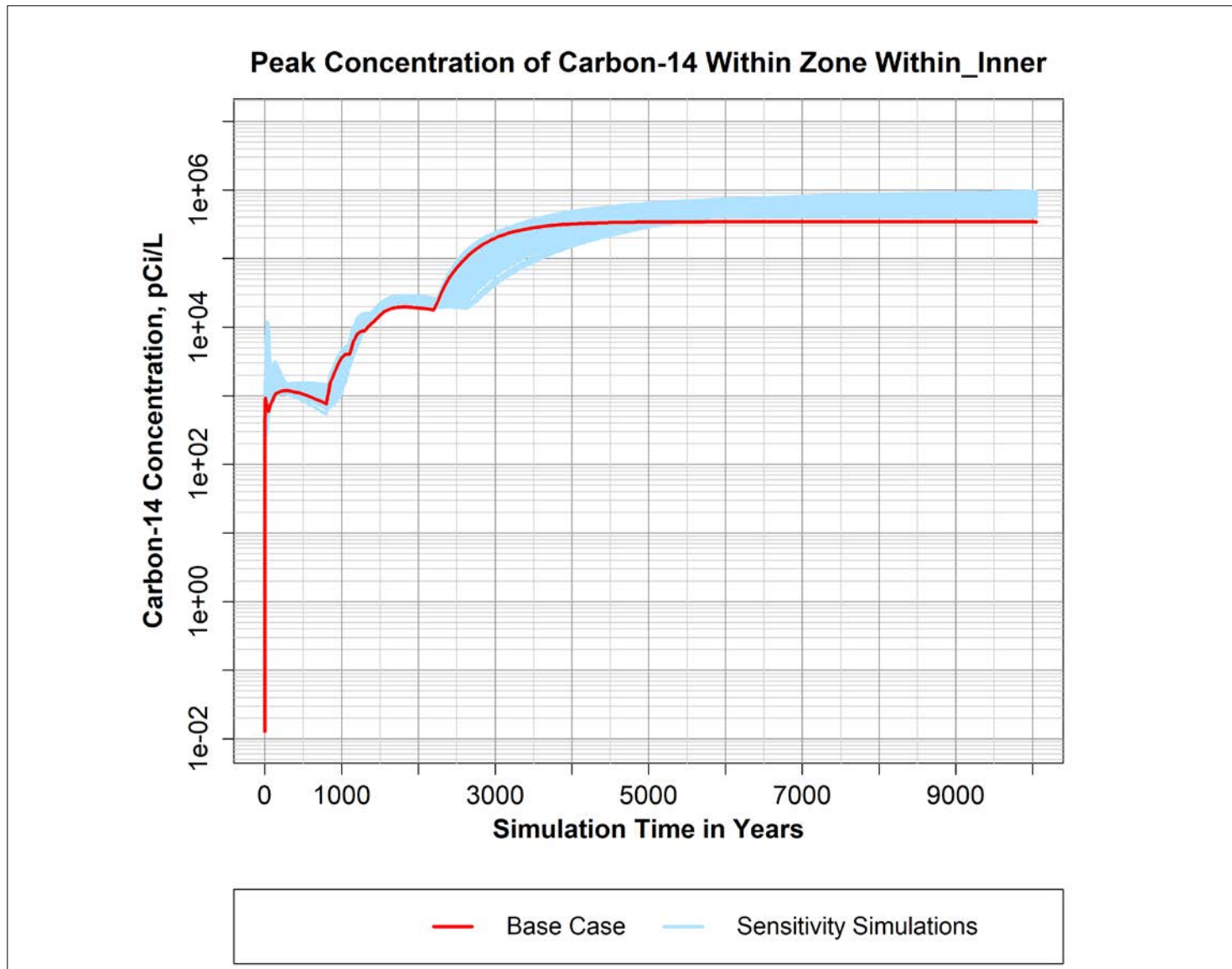
Figure B-25. Peak simulated concentration of Carbon-14 over time within the "Within_Inner" zone defined within the P2R Model version 8.3 domain.
