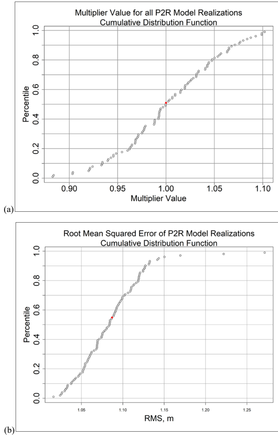
Figure 2-1. Example ECDFs for (a) Recharge Multiplier and (b) Root Mean Squared Error with each of the Variant Simulations Represented as a Separate Point on the Plot; the Calibrated Simulation Shown as a Red Dot
