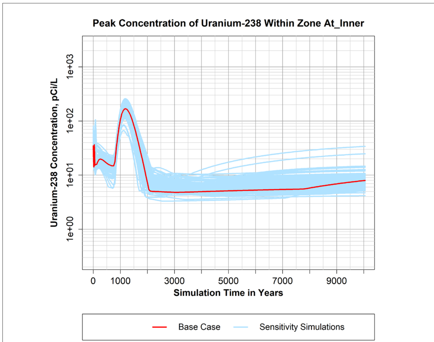
Figure B-19. Peak simulated concentration of Uranium-238 over time within the "At_Inner" zone defined within the P2R Model version 8.3 domain.
