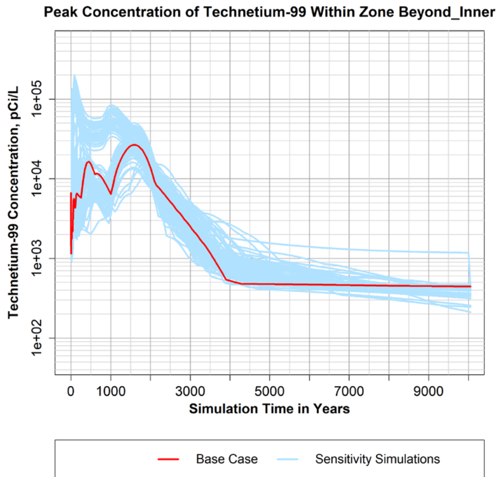
Figure 6-2. Simulated Maximum Concentrations of Technetium-99 over Time within the “Beyond_Inner” zone from the P2R Model Version 8.3 for the CA Base Case (red) overlying the NSMC Variant Simulation Results (blue)
