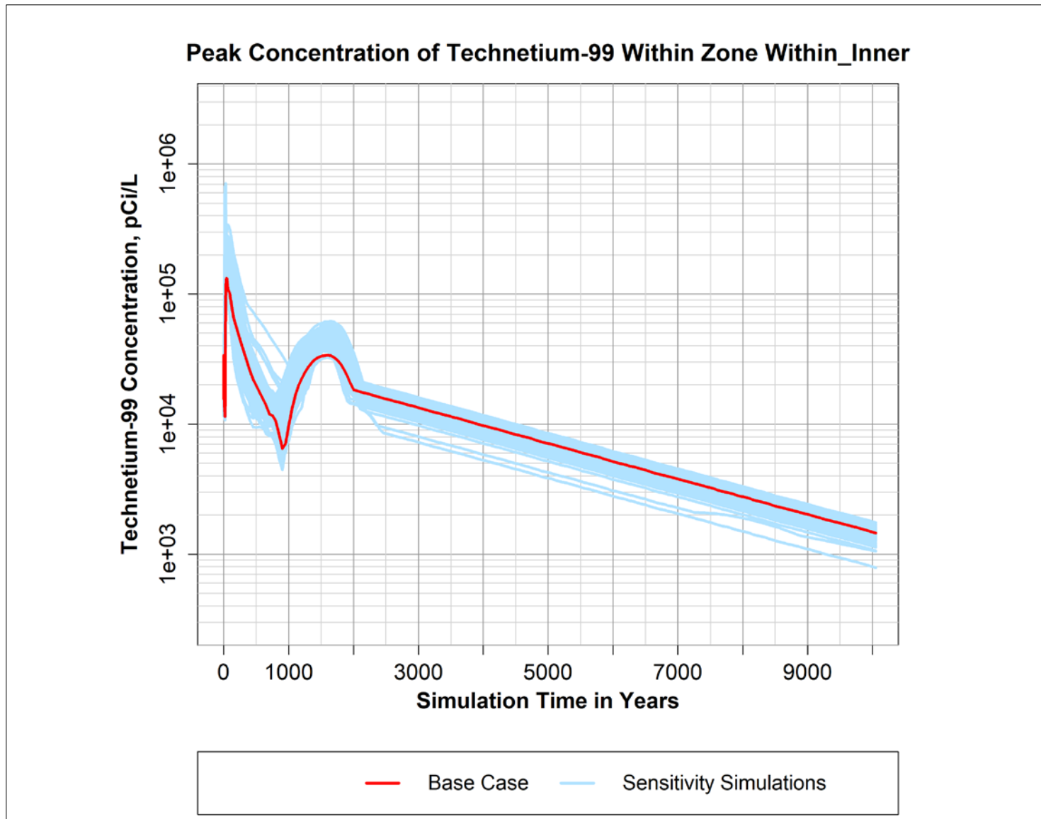
Figure B-10. Peak simulated concentration of Technetium-99 over time within the "Within_Inner" zone defined within the P2R Model version 8.3 domain.
