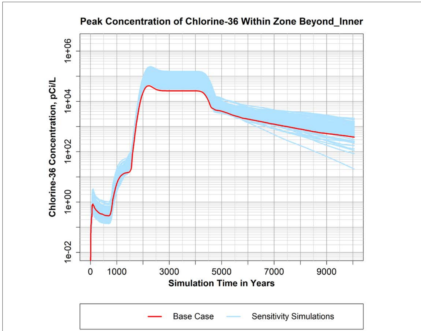
Figure B-28. Peak simulated concentration of Chlorine-36 over time within the "Beyond_Inner" zone defined within the P2R Model version 8.3 domain.
