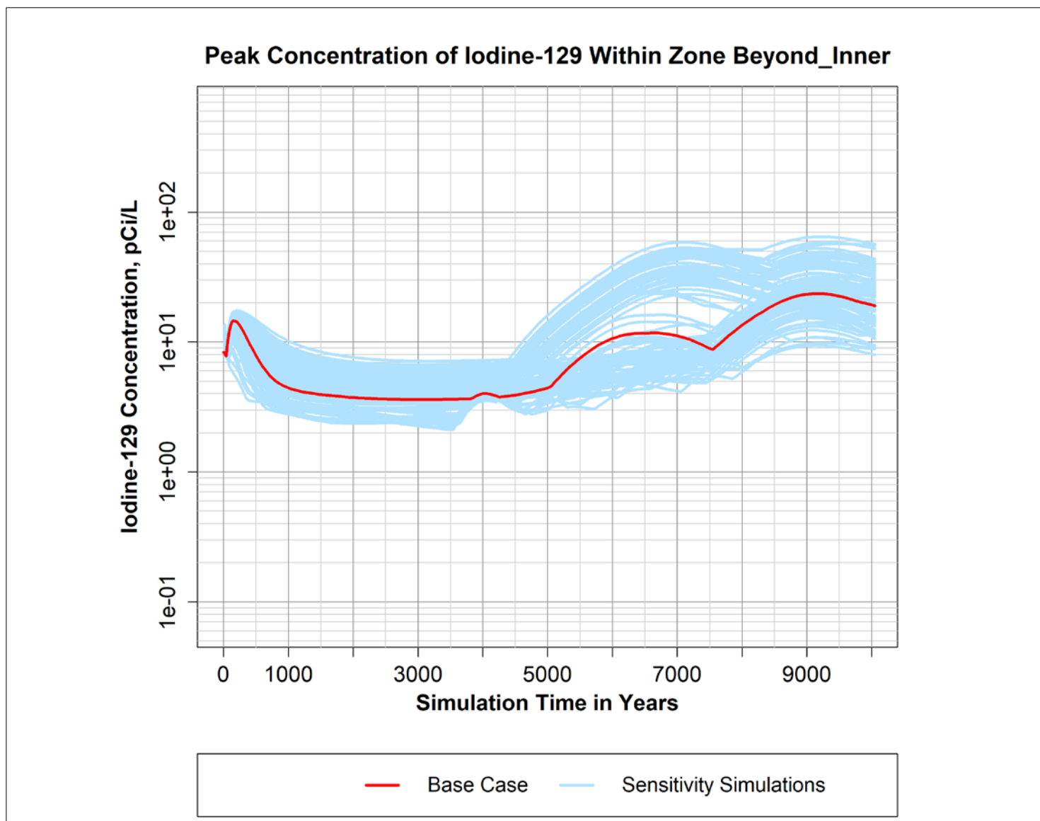
Figure B-3. Peak simulated concentration of Iodine-129 over time within the "Beyond_Inner" zone defined within the P2R Model version 8.3 domain.
