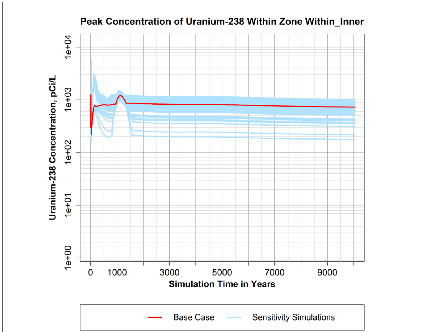
Figure B-20. Peak simulated concentration of Uranium-238 over time within the "Within_Inner" zone defined within the P2R Model version 8.3 domain.
