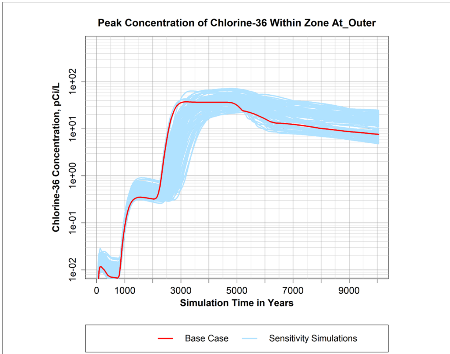
Figure B-27. Peak simulated concentration of Chlorine-36 over time within the "At_Outer" zone defined within the P2R Model version 8.3 domain.
