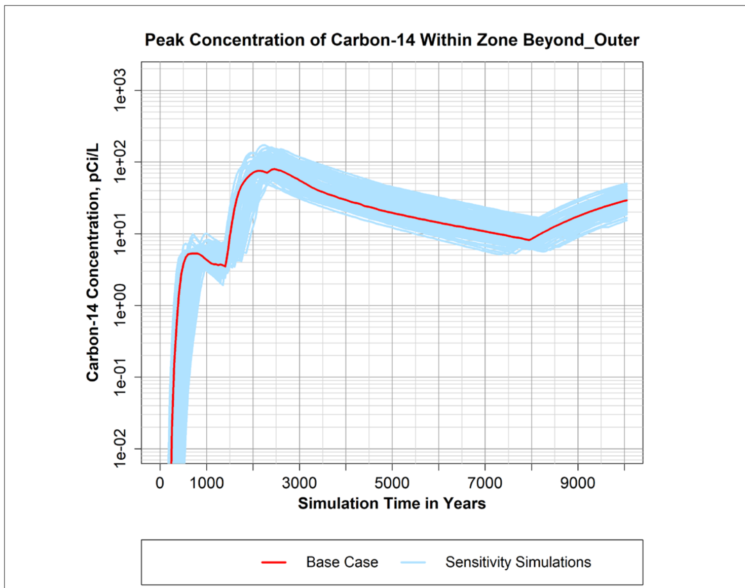
Figure B-21. Peak simulated concentration of Carbon-14 over time within the "Beyond_Outer" zone defined within the P2R Model version 8.3 domain.
