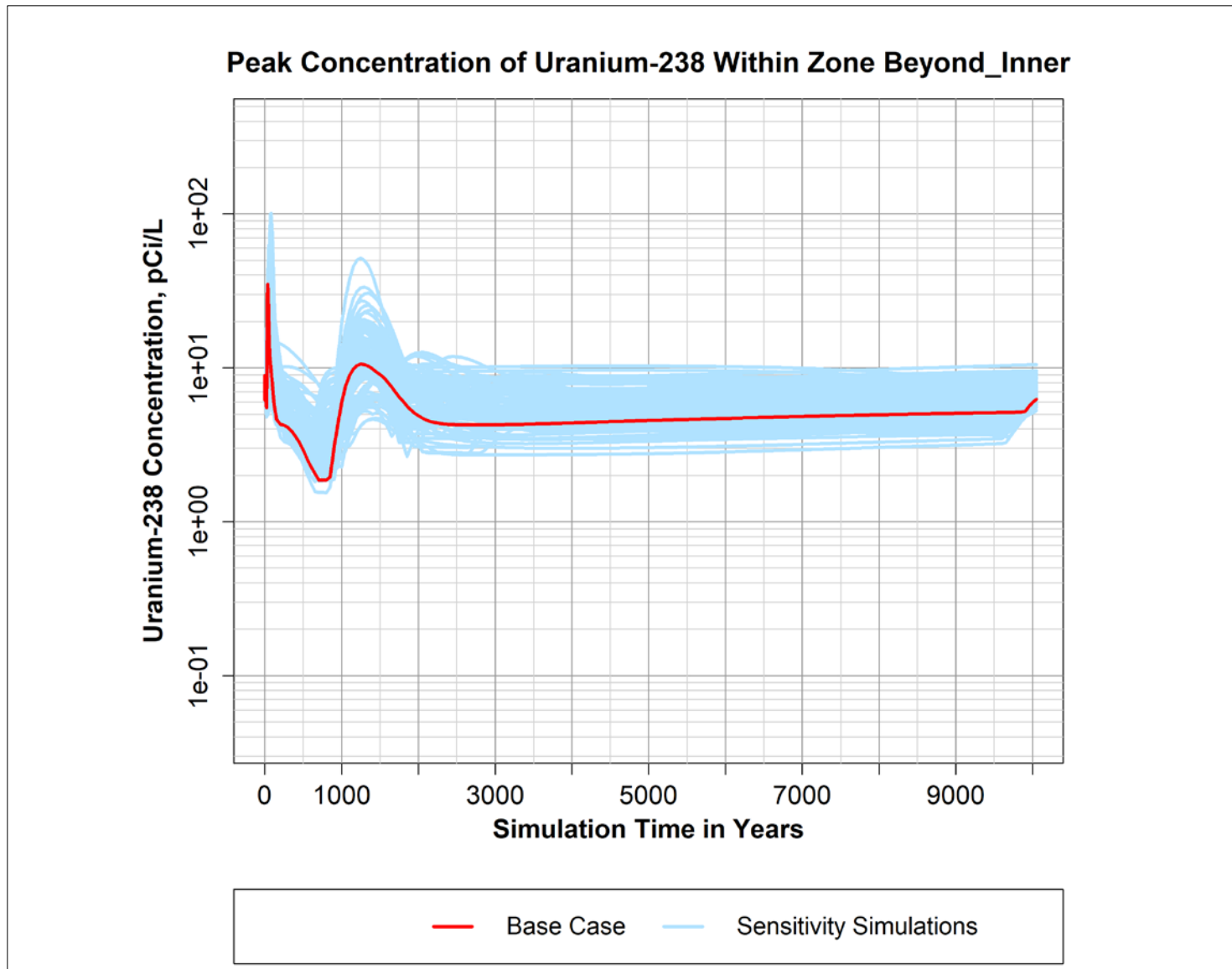
Figure B-18. Peak simulated concentration of Uranium-238 over time within the "Beyond_Inner" zone defined within the P2R Model version 8.3 domain.
