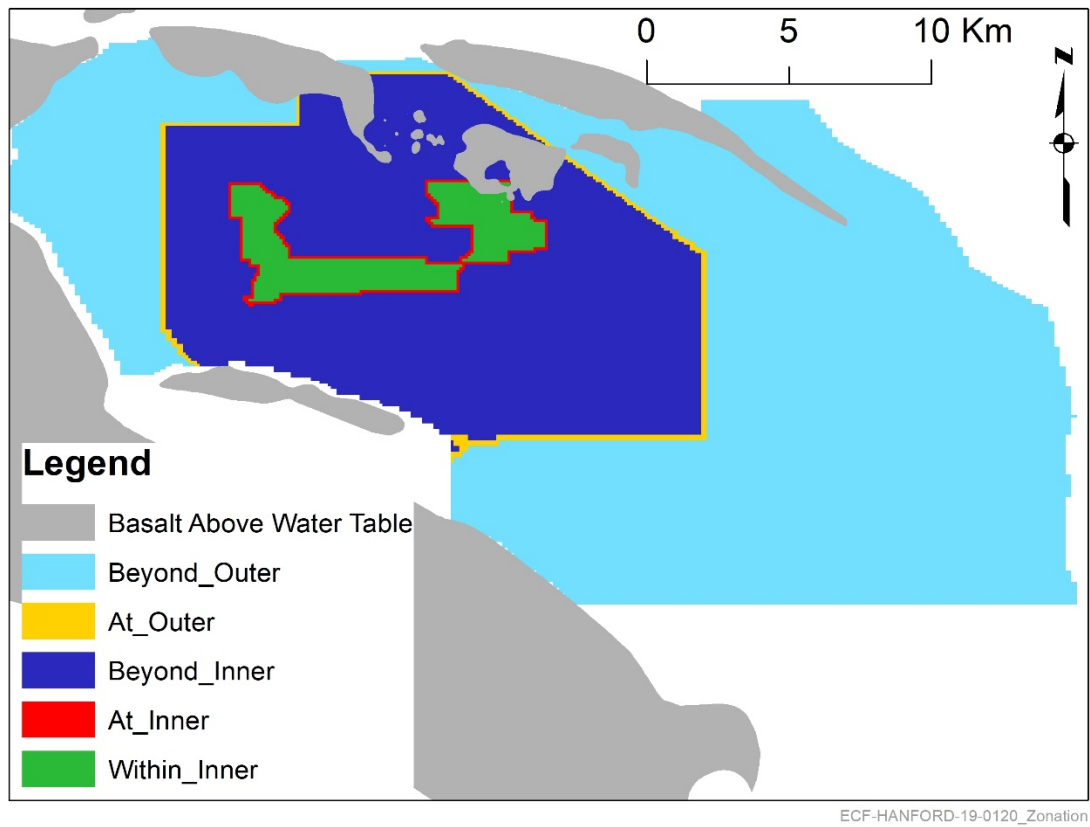
Figure 6-1. P2R Version 8.3 Peak Concentration Summary Zonation Extents
