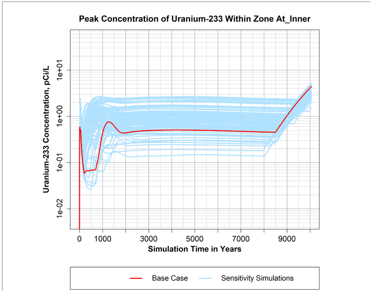
Figure B-34. Peak simulated concentration of Uranium-233 over time within the "At_Inner" zone defined within the P2R Model version 8.3 domain.
