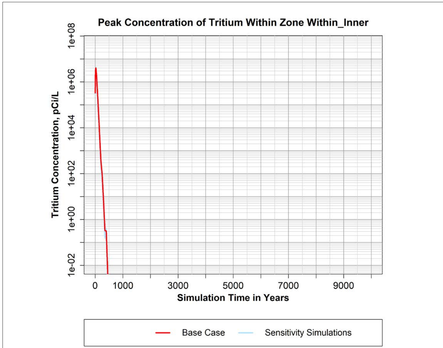
Figure B-15. Peak simulated concentration of Tritium over time within the "Within_Inner" zone defined within the P2R Model version 8.3 domain.
