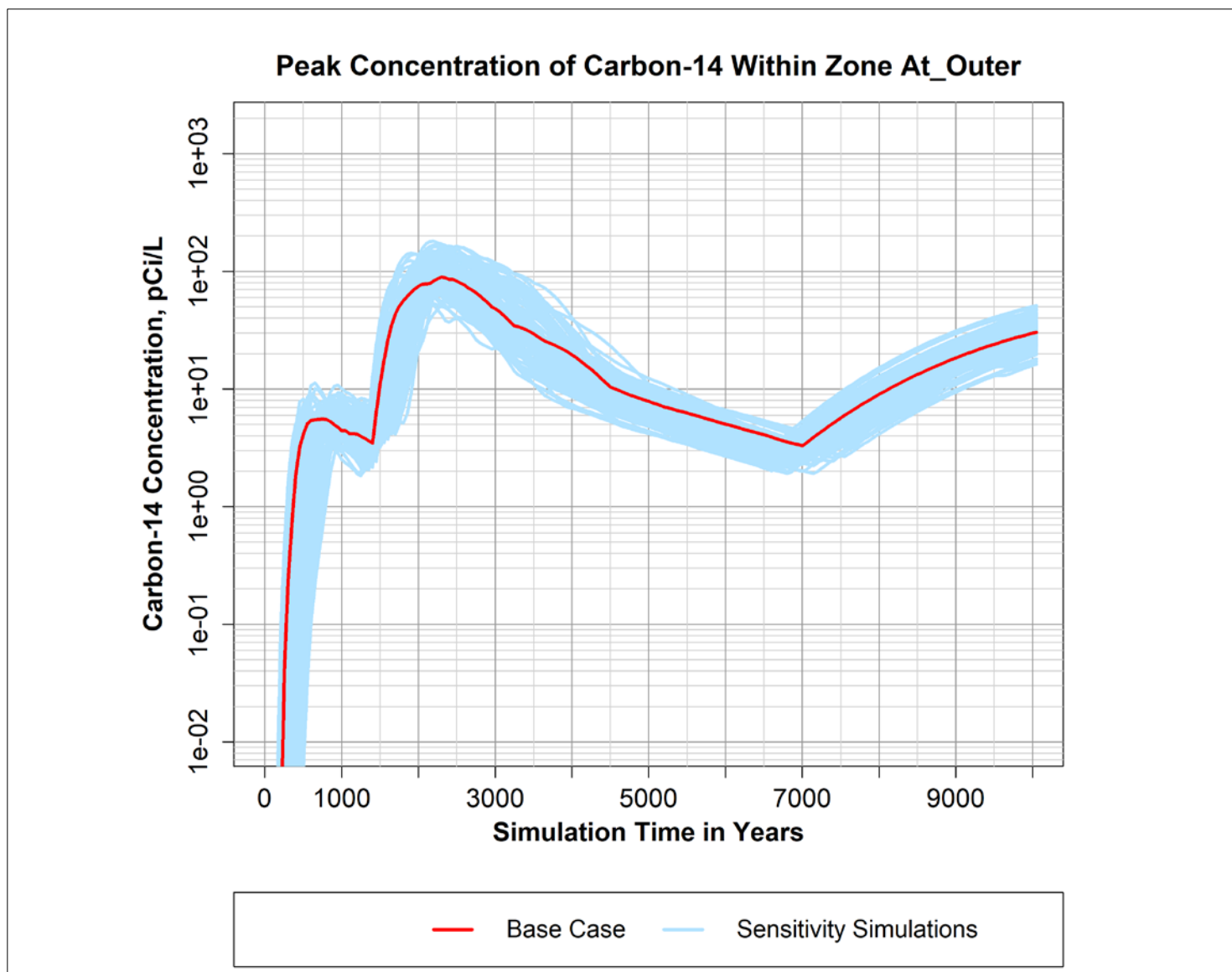
Figure B-22. Peak simulated concentration of Carbon-14 over time within the "At_Outer" zone defined within the P2R Model version 8.3 domain.
