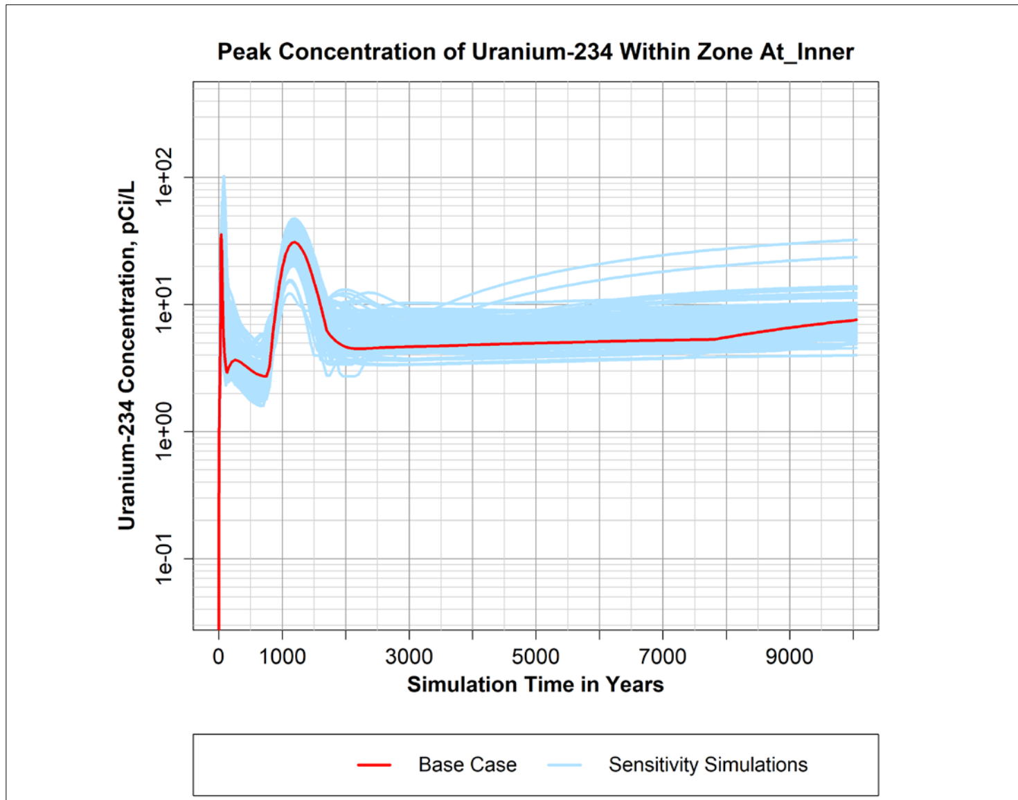
Figure B-39. Peak simulated concentration of Uranium-234 over time within the "At_Inner" zone defined within the P2R Model version 8.3 domain.
