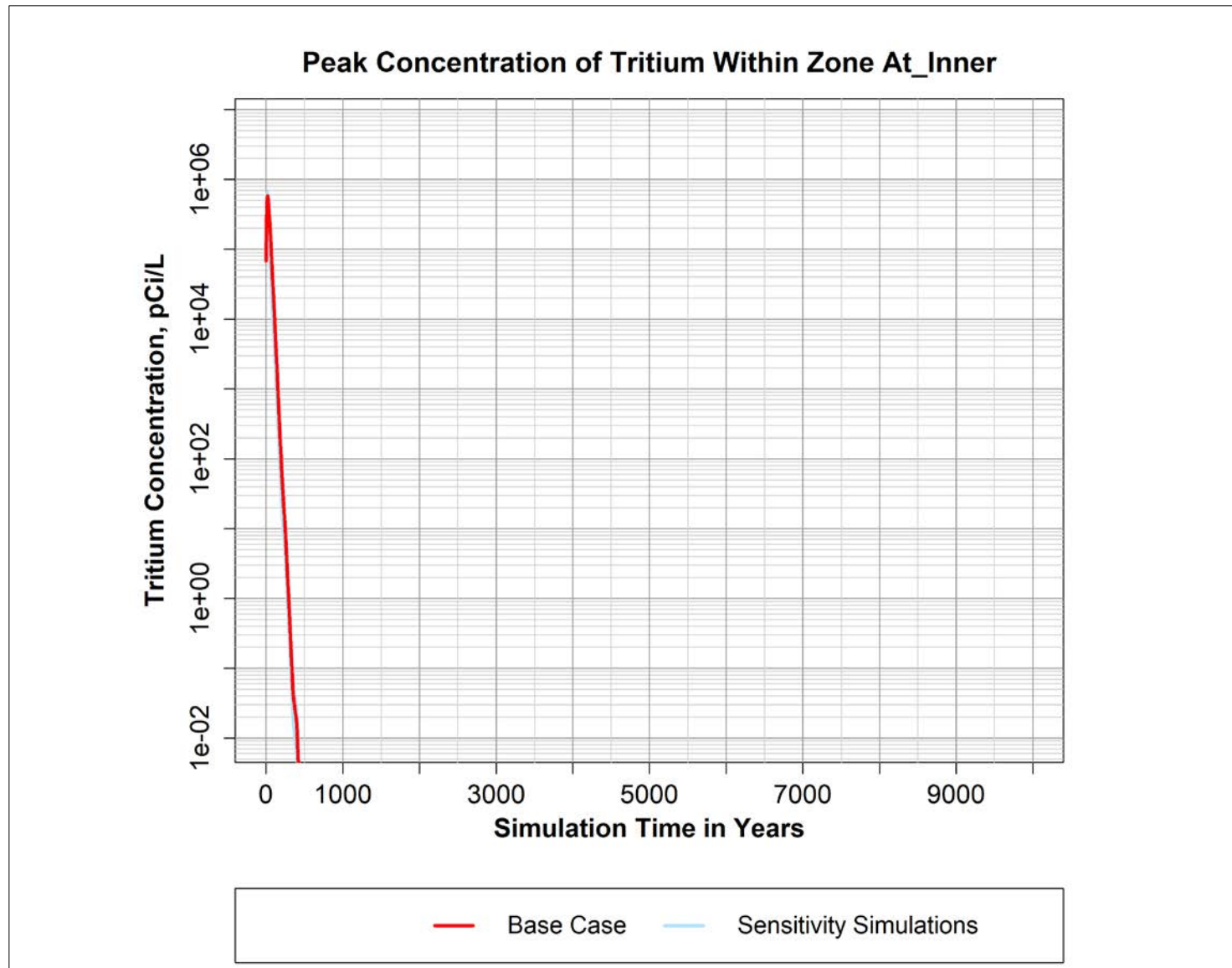
Figure B-14. Peak simulated concentration of Tritium over time within the "At_Inner" zone defined within the P2R Model version 8.3 domain.
