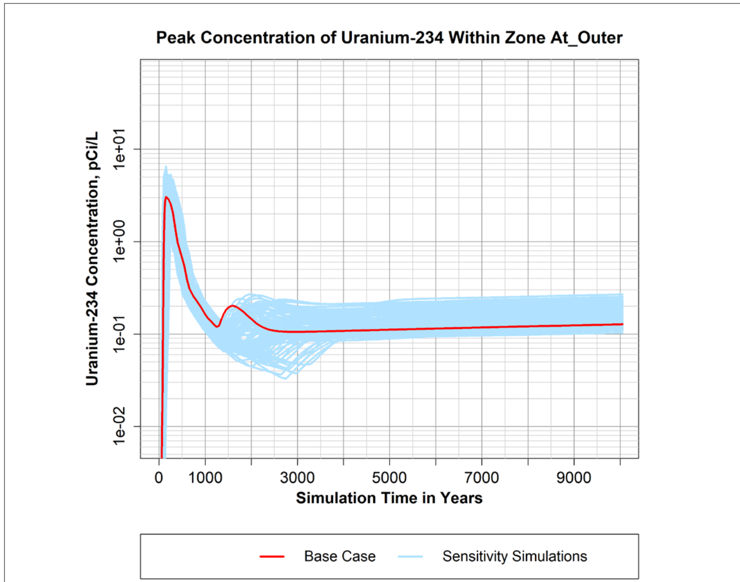
Figure B-37. Peak simulated concentration of Uranium-234 over time within the "At_Outer" zone defined within the P2R Model version 8.3 domain.
