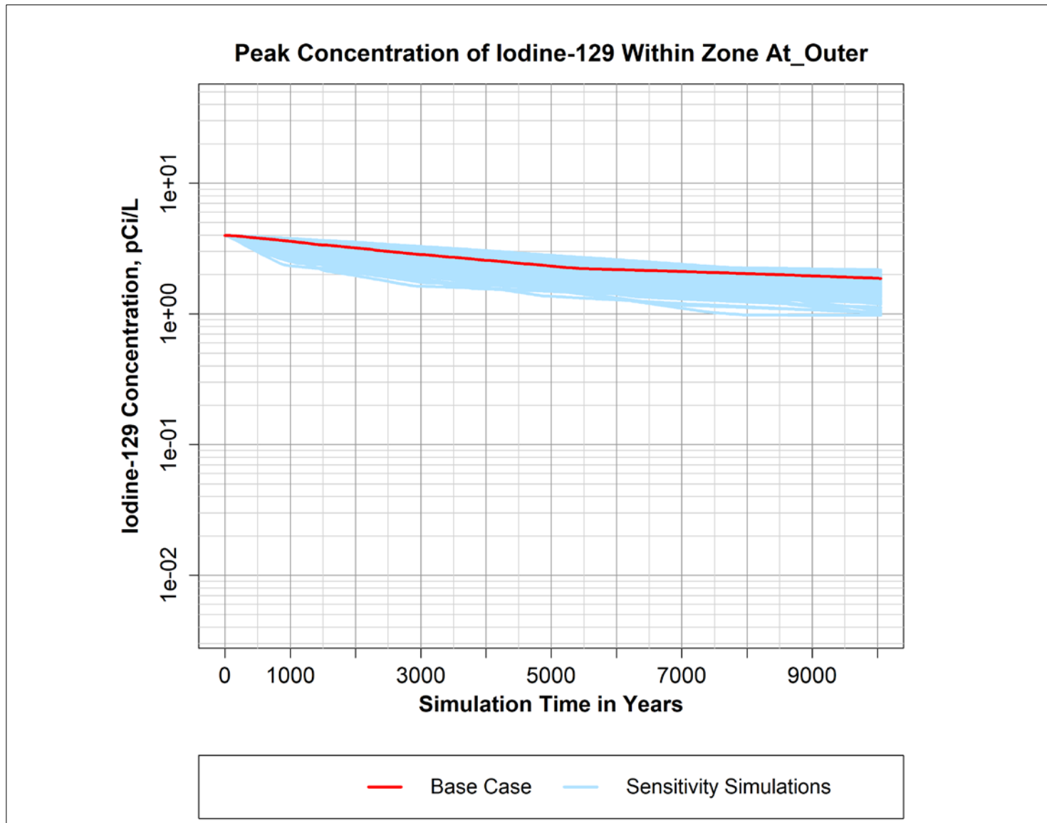
Figure B-2. Peak simulated concentration of Iodine-129 over time within the "At_Outer" zone defined within the P2R Model version 8.3 domain.
