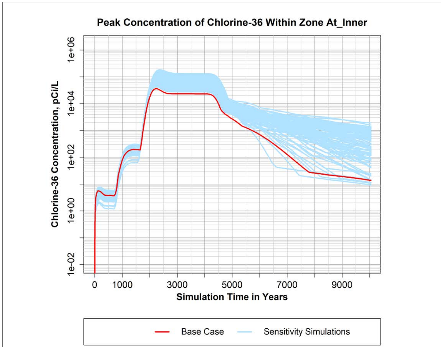
Figure B-29. Peak simulated concentration of Chlorine-36 over time within the "At_Inner" zone defined within the P2R Model version 8.3 domain.
