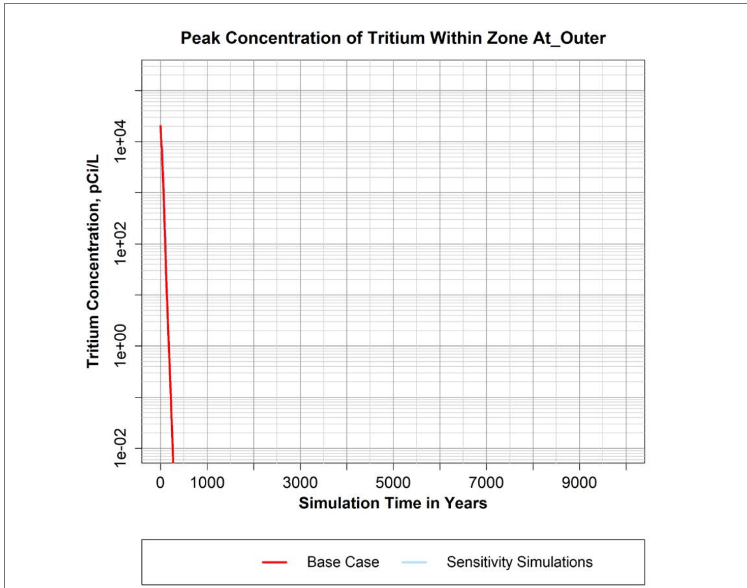
Figure B-12. Peak simulated concentration of Tritium over time within the "At_Outer" zone defined within the P2R Model version 8.3 domain.
