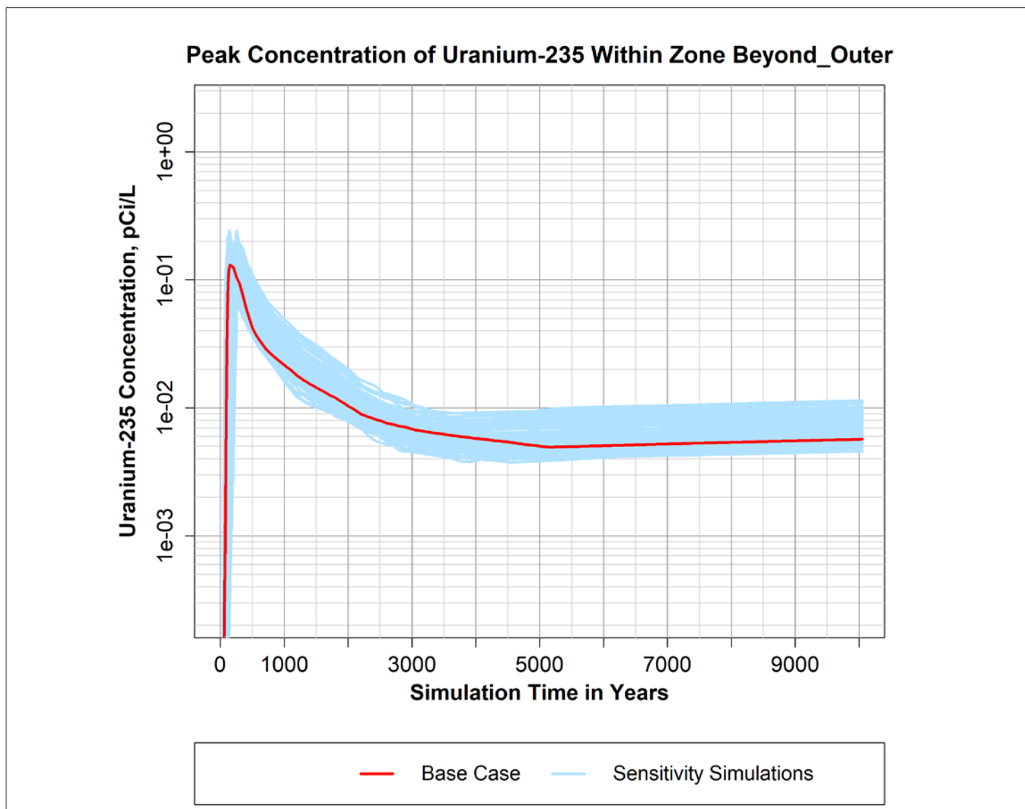
Figure B-41. Peak simulated concentration of Uranium-235 over time within the "Beyond_Outer" zone defined within the P2R Model version 8.3 domain.
