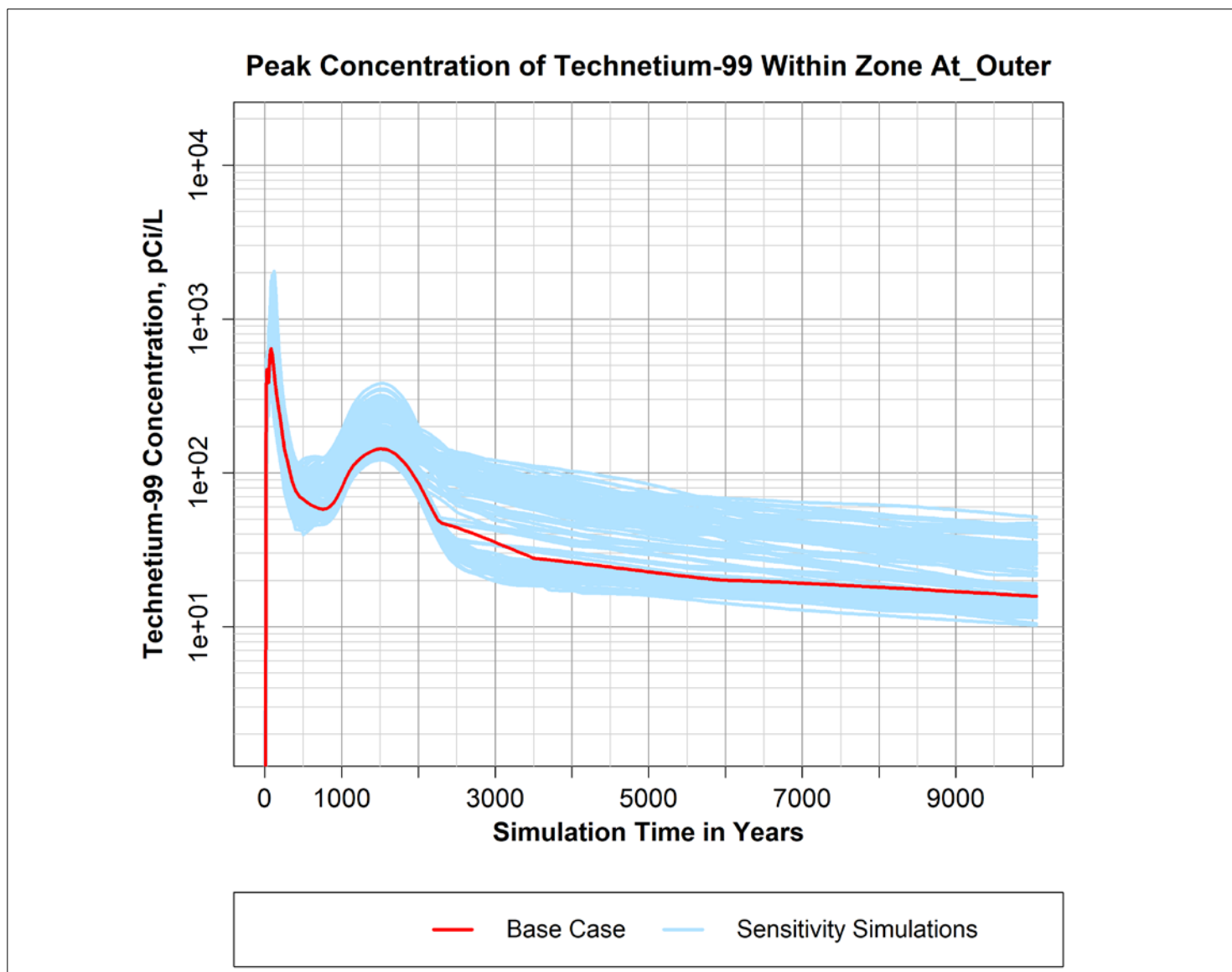
Figure B-7. Peak simulated concentration of Technetium-99 over time within the "At_Outer" zone defined within the P2R Model version 8.3 domain.
