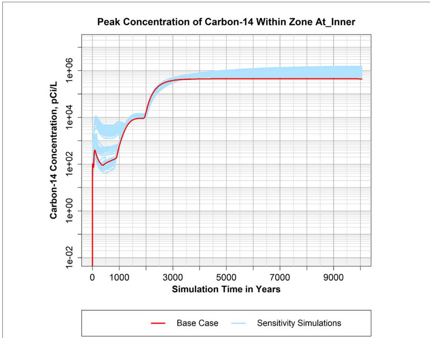
Figure B-24. Peak simulated concentration of Carbon-14 over time within the "At_Inner" zone defined within the P2R Model version 8.3 domain.
