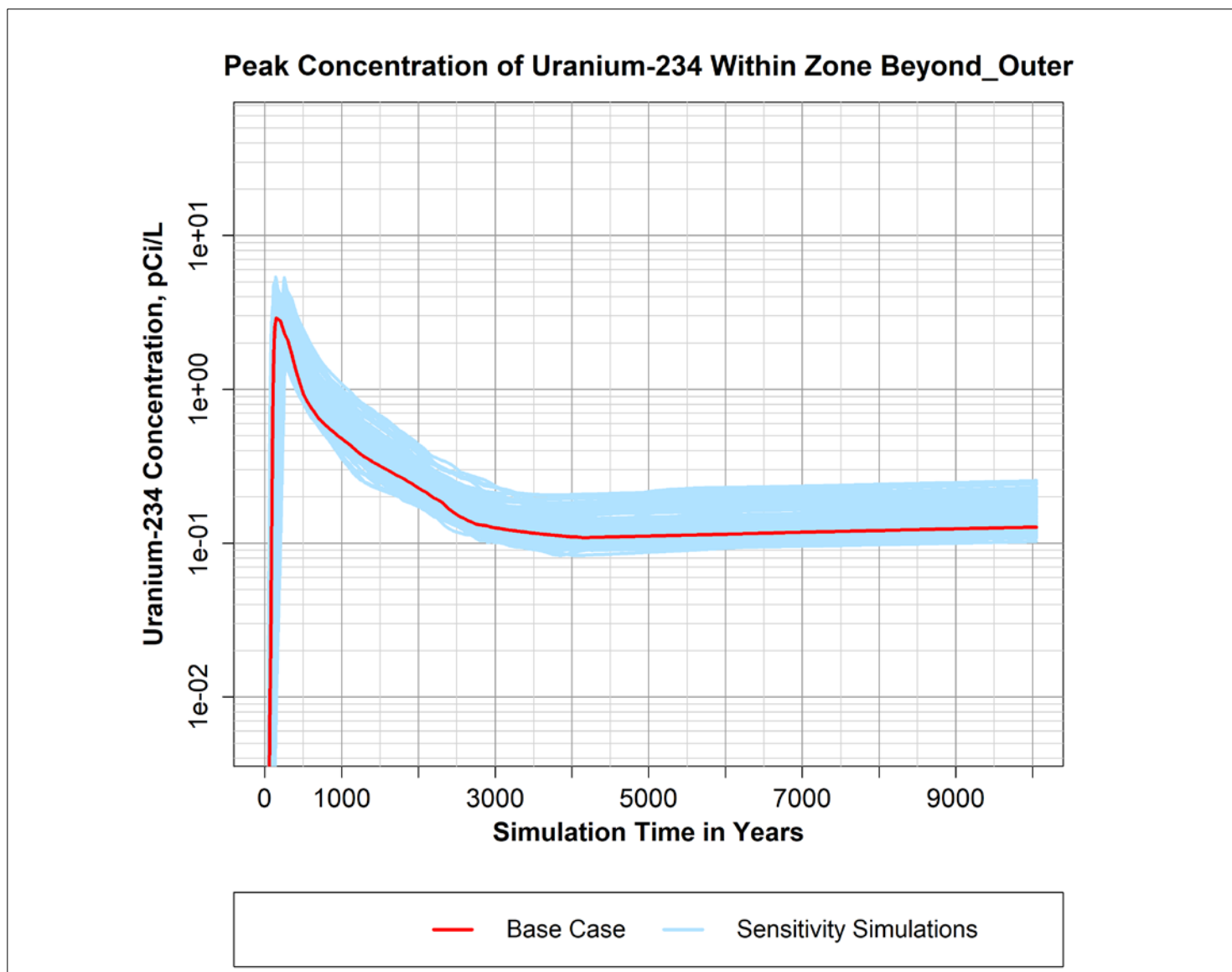
Figure B-36. Peak simulated concentration of Uranium-234 over time within the "Beyond_Outer" zone defined within the P2R Model version 8.3 domain.
