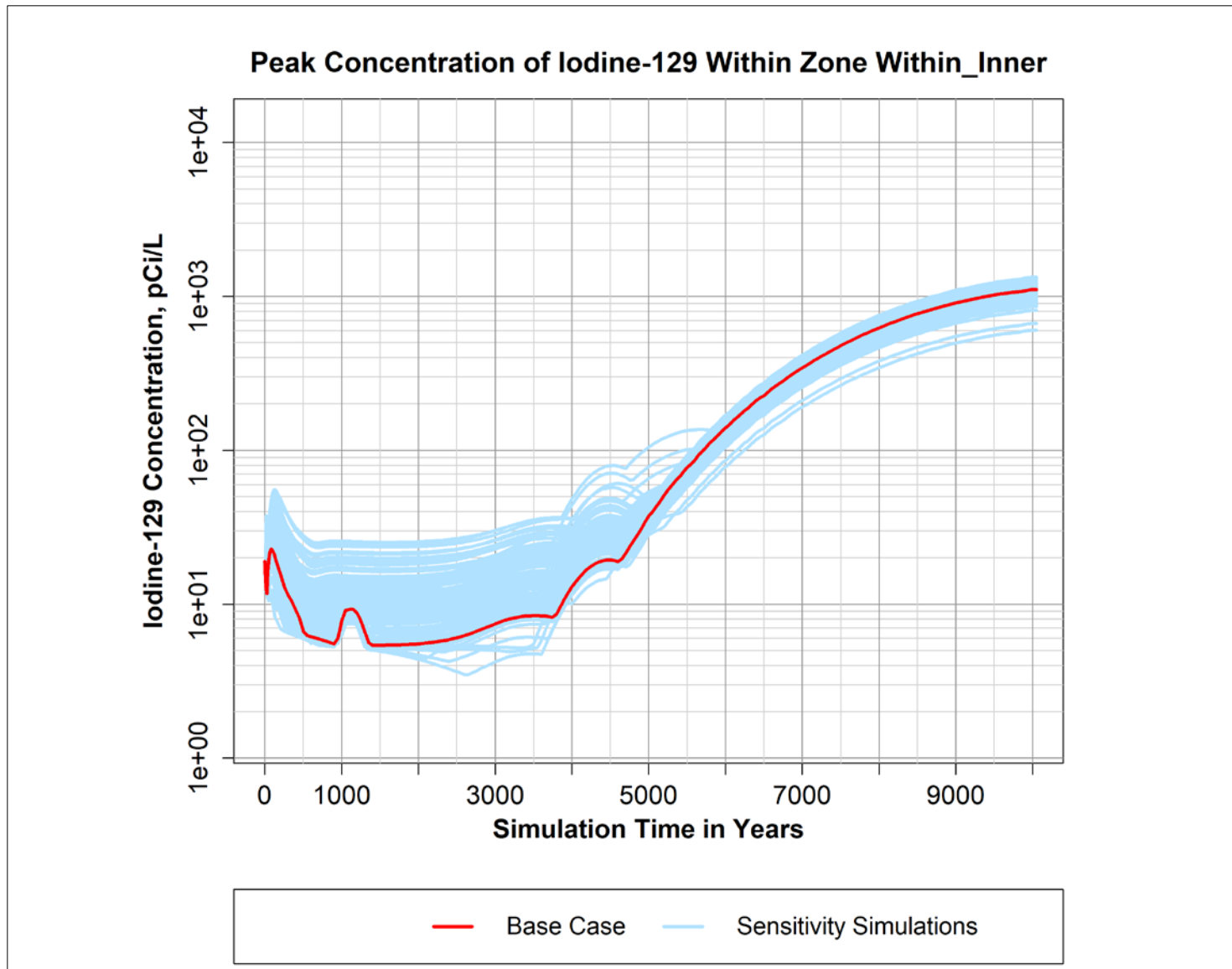
Figure B-5. Peak simulated concentration of Iodine-129 over time within the "Within_Inner" zone defined within the P2R Model version 8.3 domain.
