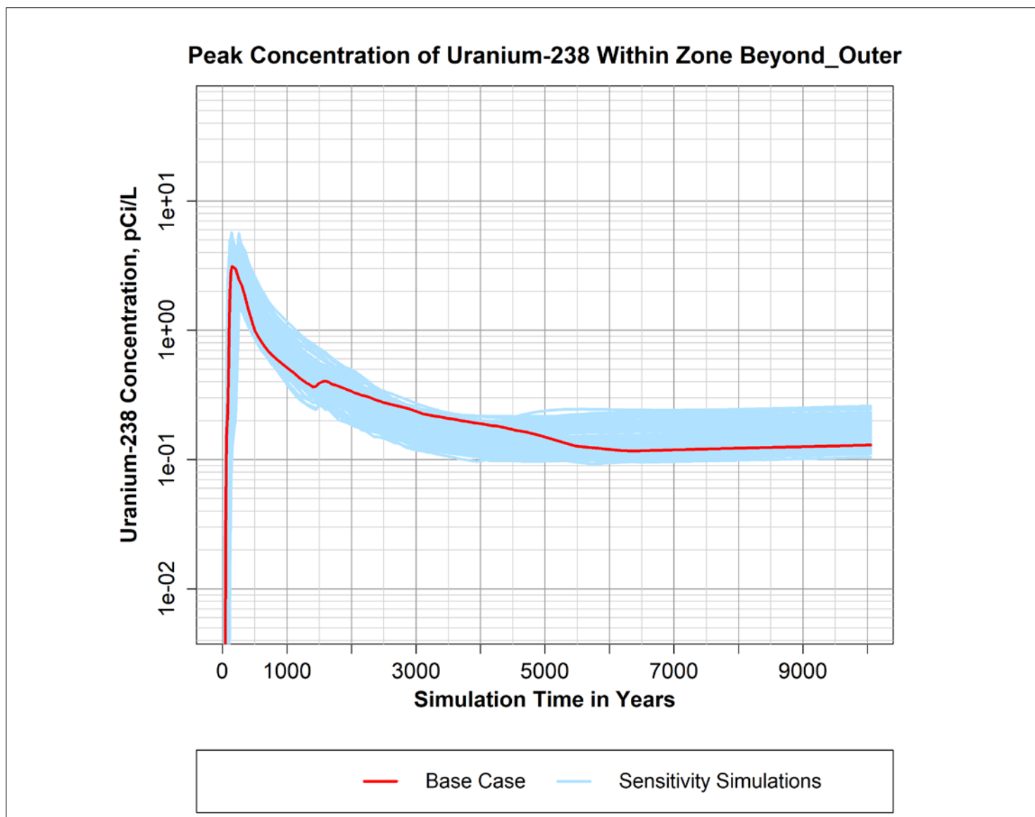
Figure B-16. Peak simulated concentration of Uranium-238 over time within the "Beyond_Outer" zone defined within the P2R Model version 8.3 domain.
