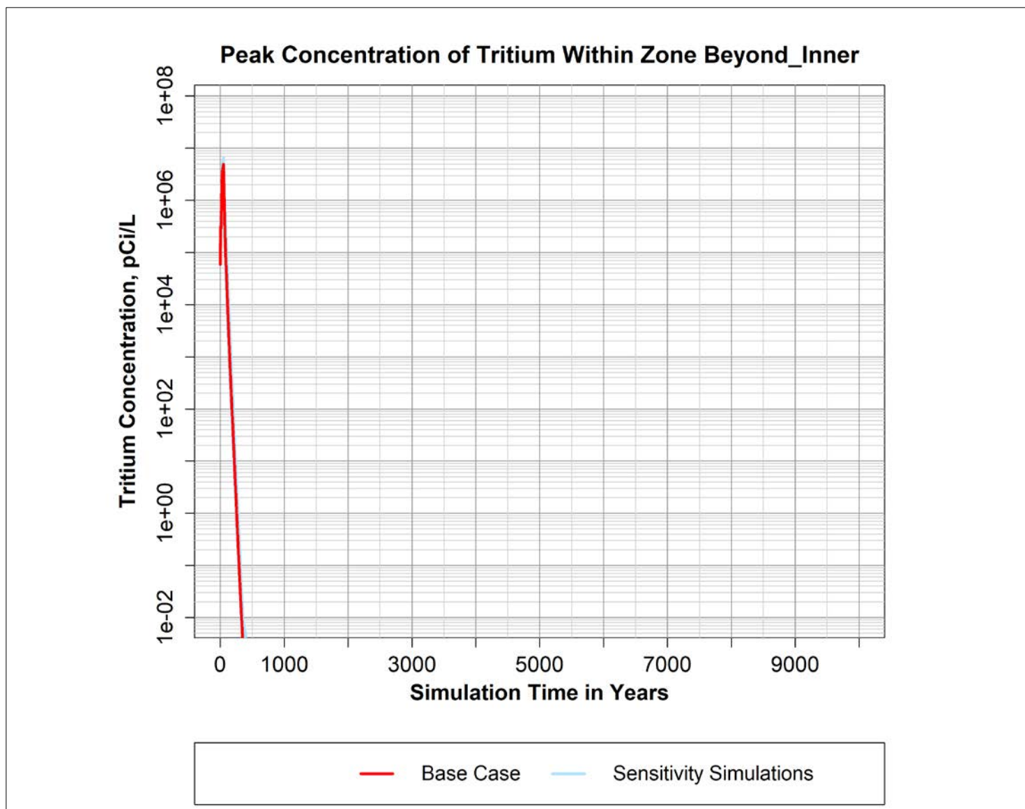
Figure B-13. Peak simulated concentration of Tritium over time within the "Beyond_Inner" zone defined within the P2R Model version 8.3 domain.
