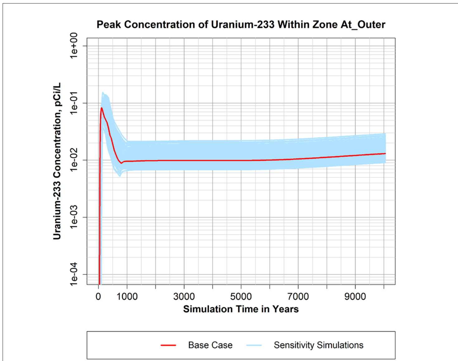
Figure B-32. Peak simulated concentration of Uranium-233 over time within the "At_Outer" zone defined within the P2R Model version 8.3 domain.
