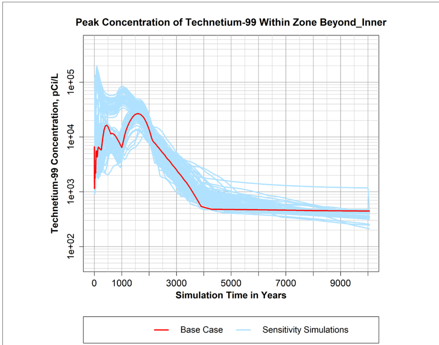
Figure B-8. Peak simulated concentration of Technetium-99 over time within the "Beyond_Inner" zone defined within the P2R Model version 8.3 domain.
