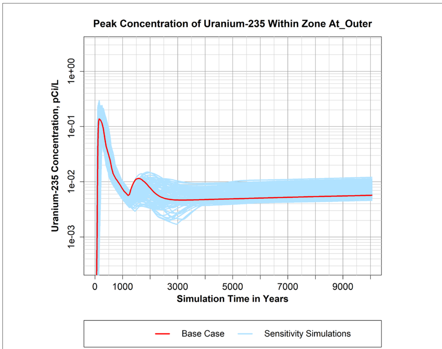
Figure B-42. Peak simulated concentration of Uranium-235 over time within the "At_Outer" zone defined within the P2R Model version 8.3 domain.
