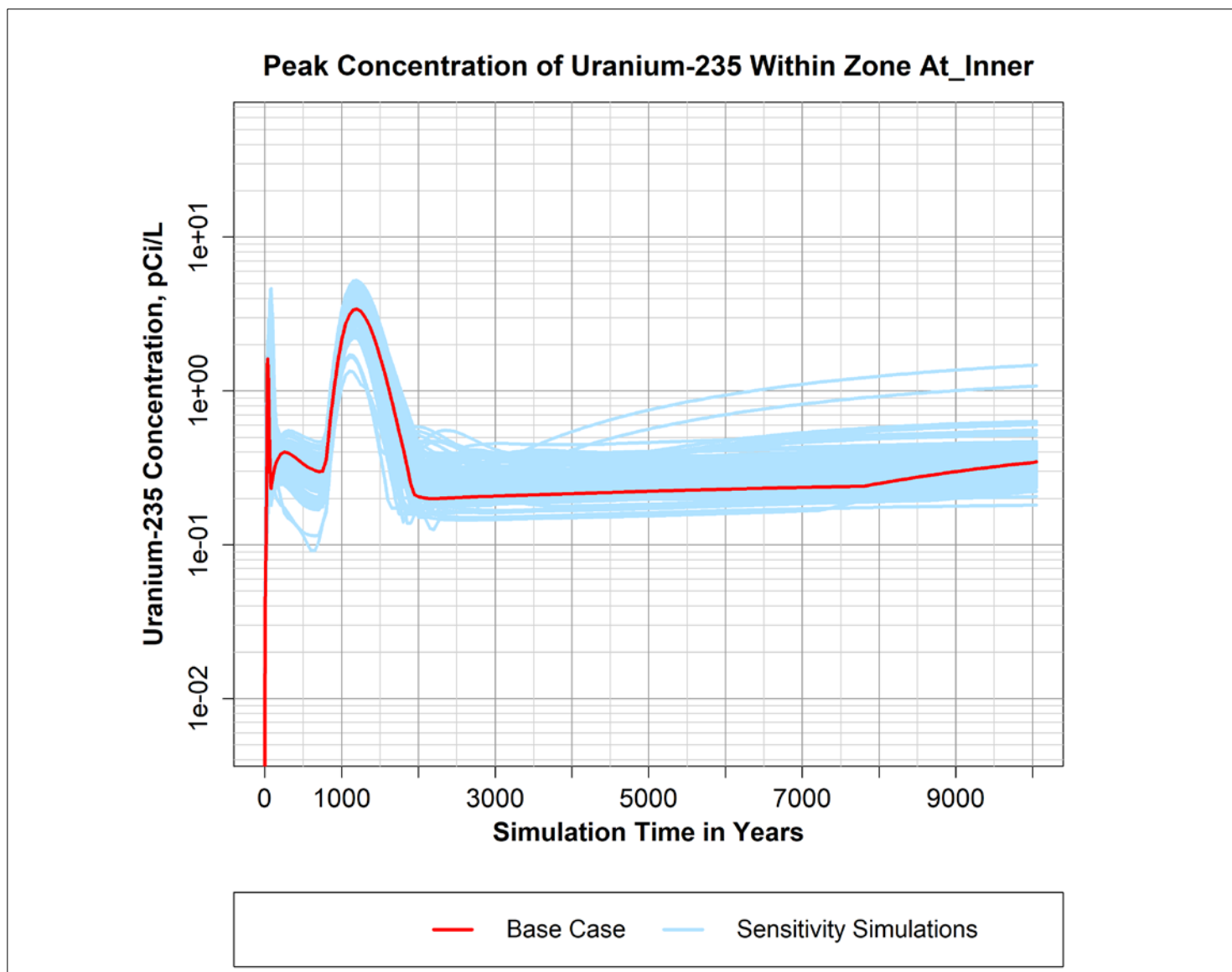
Figure B-44. Peak simulated concentration of Uranium-235 over time within the "At_Inner" zone defined within the P2R Model version 8.3 domain.
