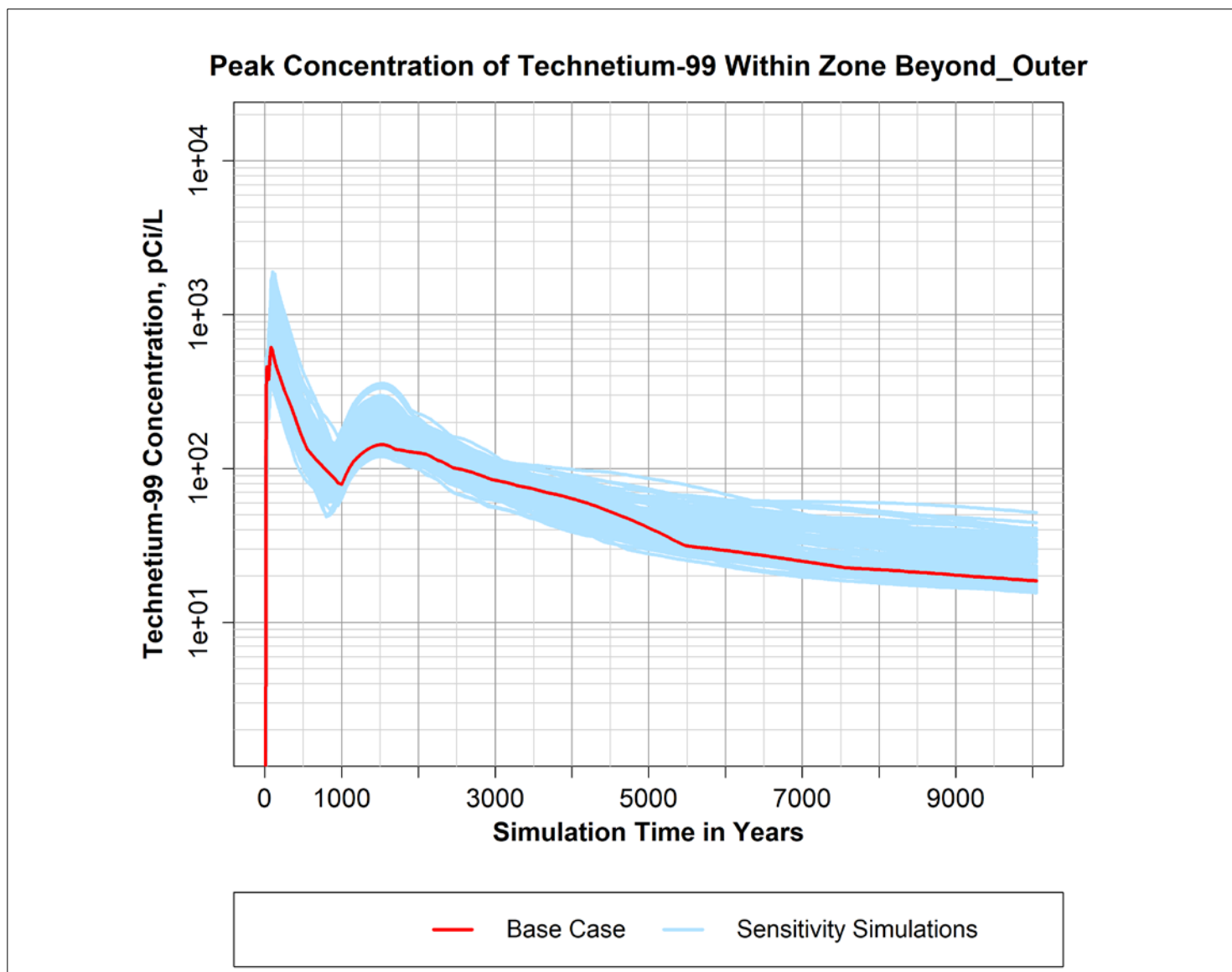
Figure B-6. Peak simulated concentration of Technetium-99 over time within the "Beyond_Outer" zone defined within the P2R Model version 8.3 domain.
