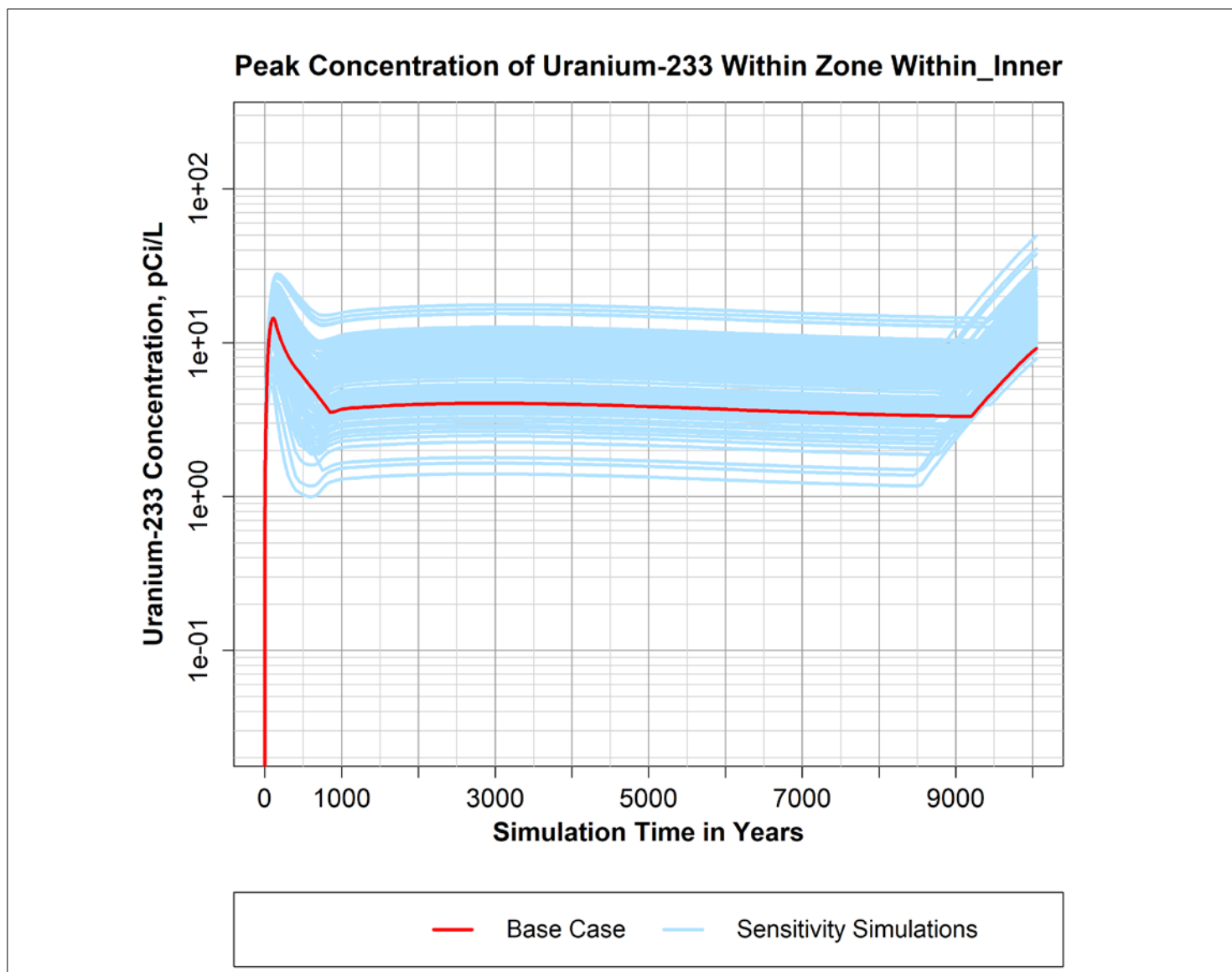
Figure B-35. Peak simulated concentration of Uranium-233 over time within the "Within_Inner" zone defined within the P2R Model version 8.3 domain.
