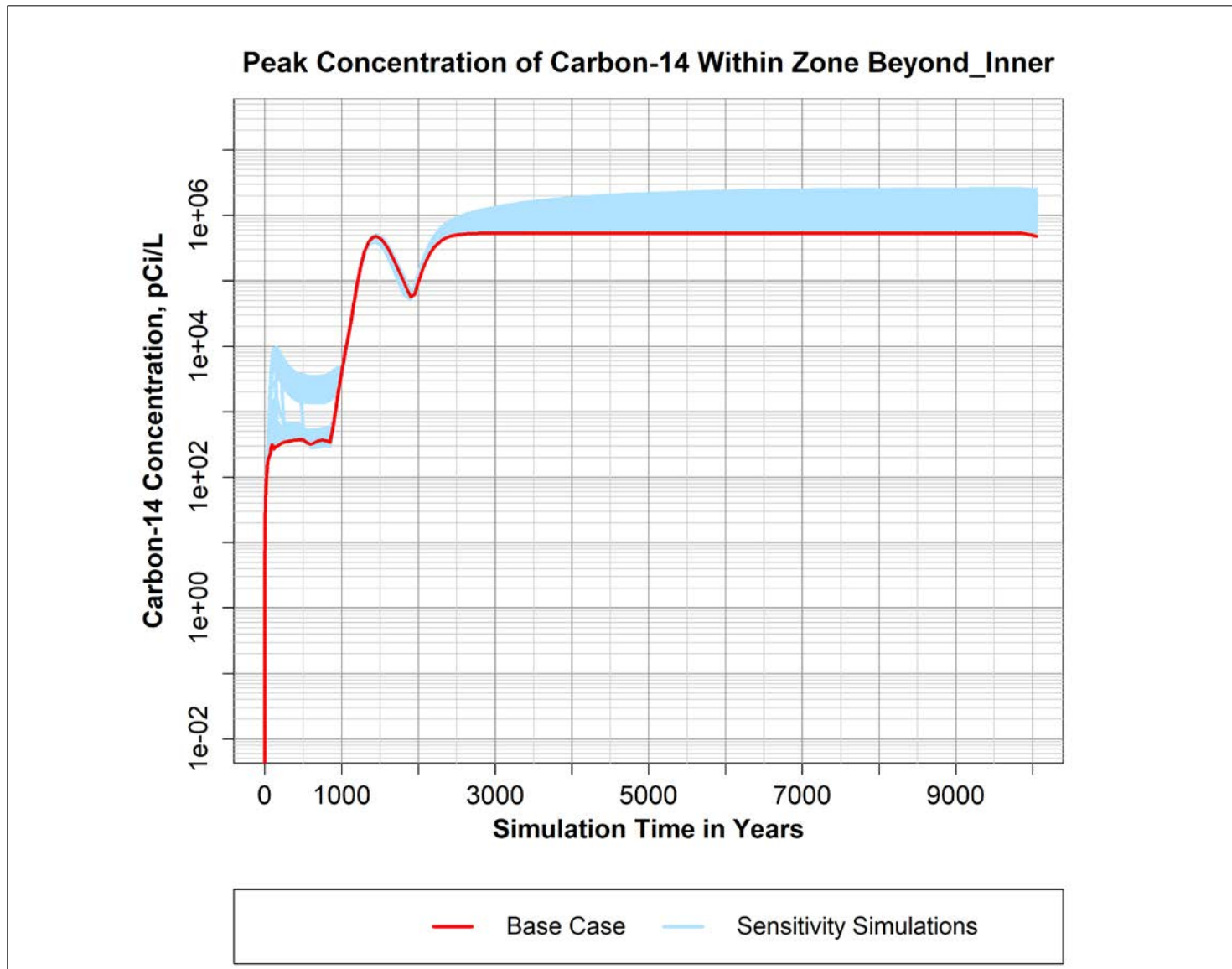
Figure B-23. Peak simulated concentration of Carbon-14 over time within the "Beyond_Inner" zone defined within the P2R Model version 8.3 domain.
