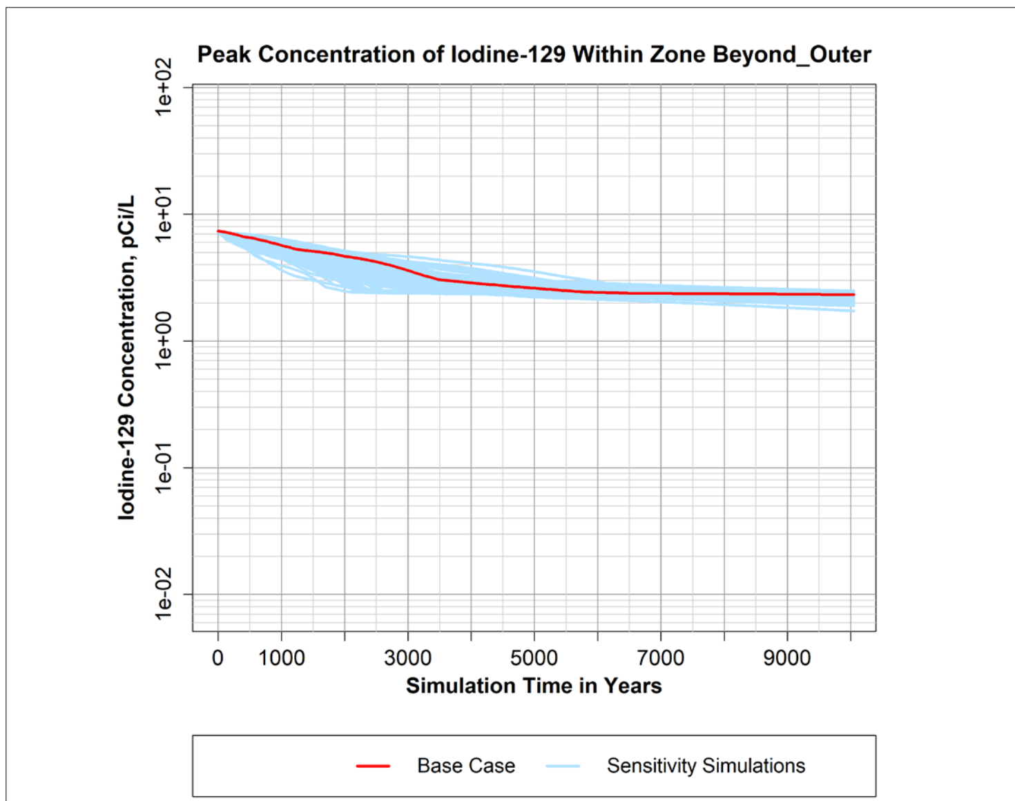
Figure B-1. Peak simulated concentration of Iodine-129 over time within the "Beyond_Outer" zone defined within the P2R Model version 8.3 domain.
