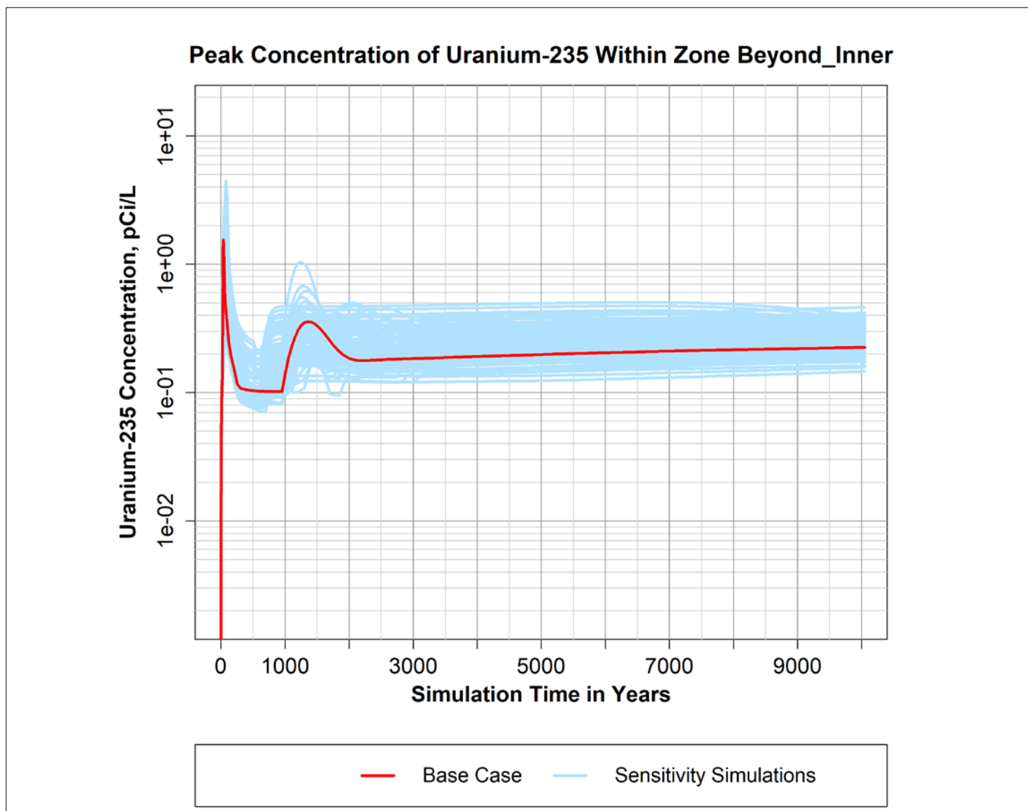
Figure B-43. Peak simulated concentration of Uranium-235 over time within the "Beyond_Inner" zone defined within the P2R Model version 8.3 domain.
