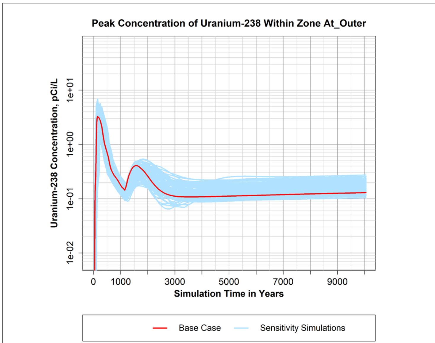
Figure B-17. Peak simulated concentration of Uranium-238 over time within the "At_Outer" zone defined within the P2R Model version 8.3 domain.
