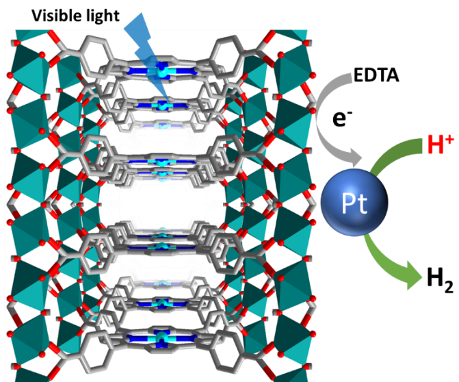
Figure 8. The structure of Al-PMOF featuring Zn-porphyrin sites as photosensitizers for hydrogen evolution.
