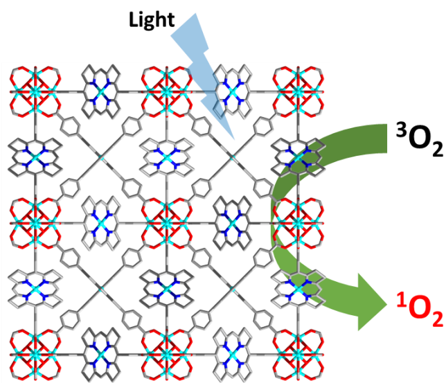
Figure 16. The structure of DBP-UiO featuring \text{Hf}_6 nodes and porphyrin linkers for the light induced generation of singlet oxygen.
