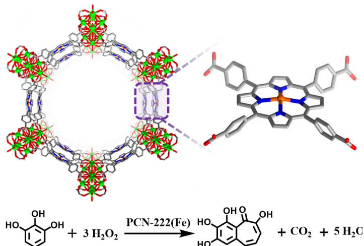
Figure 4. The structure of PCN-222/MOF-545 featuring iron porphyrin sites for catalyzing the oxidation of pyrogallol.
