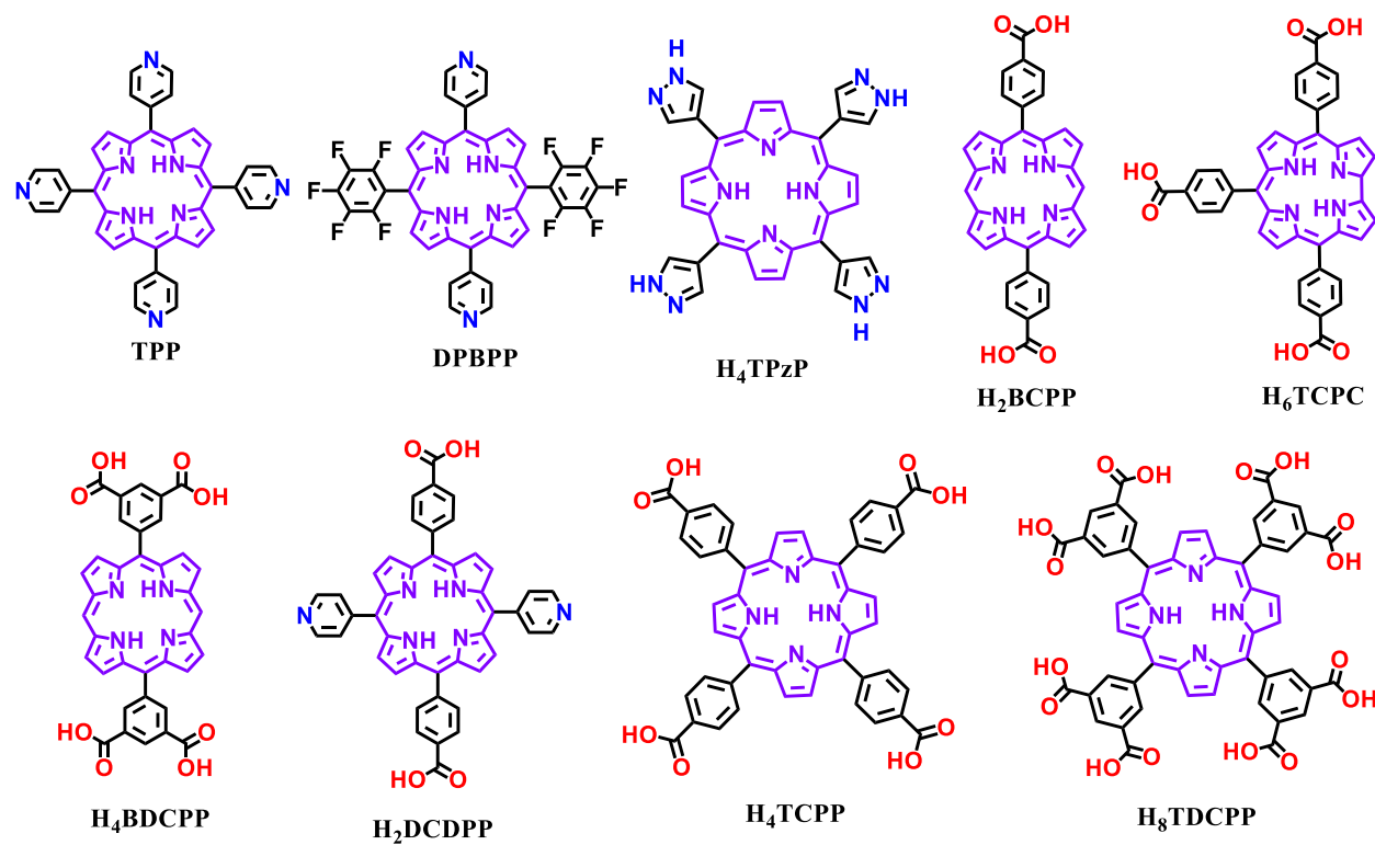
Figure 2. Representative molecular structures of porphyrin-based organic linkers for the synthesis of MOFs.
