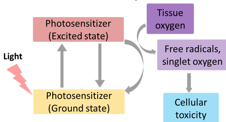
Figure 15. A schematic representation of PDT.
