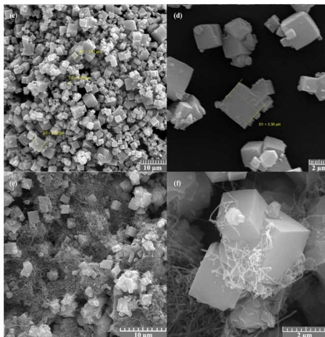
Figure 10. SEM images of PCN-224(Co) (top) and PCN-224(Co)/MWCNT (bottom). Adapted with permission from ref. 183. Copyright 2018 Springer Nature.
