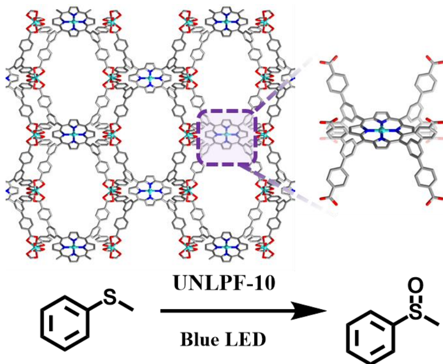
Figure 9. Structure of UNLPF-10 featuring In-porphyrin sites for the photocatalytic oxidation of thioanisole.
