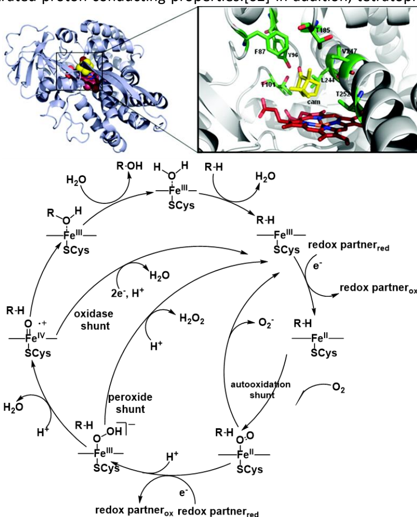
Figure 3. Active site (top) and representative catalytic oxidation mechanism (bottom) of cytochrome P450. Adapted with permission from Ref. 67. Copyright 2012 American Chemical Society.
