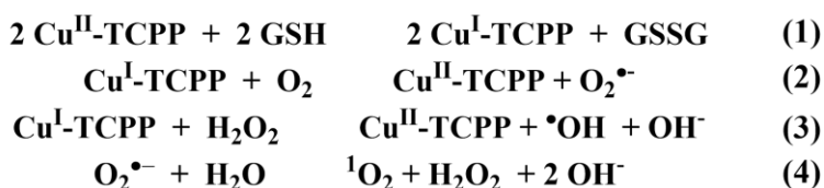
Figure 17. A proposed mechanism for the production of ^1\text{O}_2 from Cu-TCPP in the absence of externally applied light. Here GSH is glutathione and GSSG is the oxidized form of glutathione.
