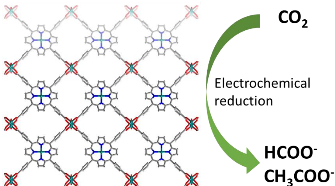
Figure 11. Structure of Cu 2 (CuTCPP) featuring Cu 2 nodes and Cu-porphyrin sites for the electrochemical reduction of CO 2 to formate and acetate.
