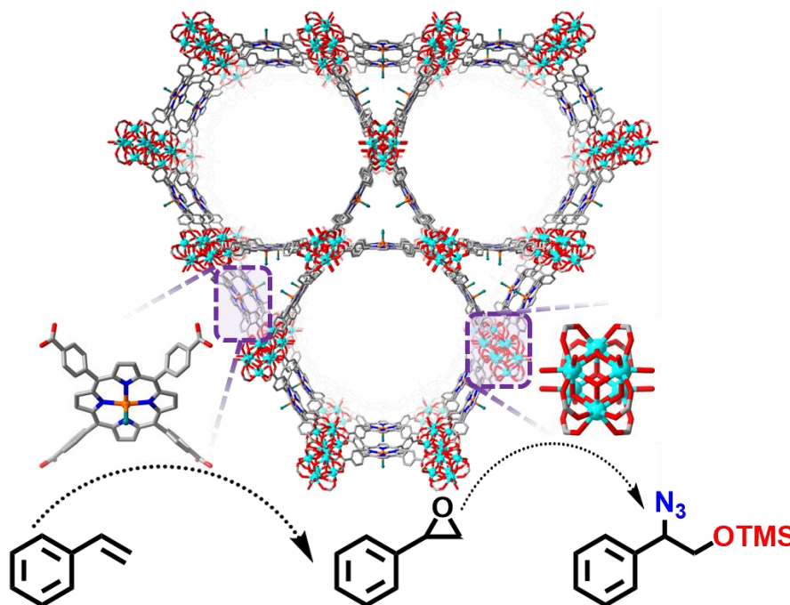
Figure 6. The structure of Hf-PCN-222(Fe) featuring Fe-porphyrin and Hf 6 sites for the tandem transformation of styrene.
