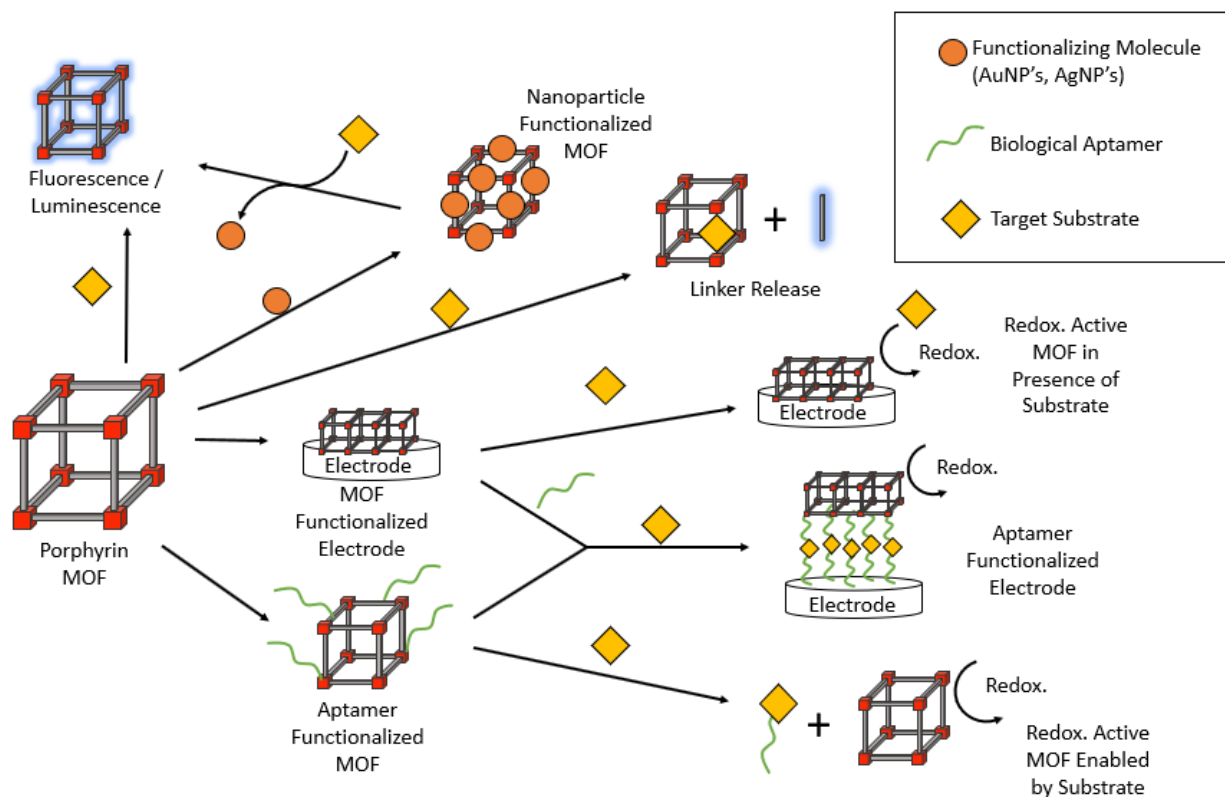
Figure 12. A summary of various kinds of sensing mechanisms enabled by porphyrin-based MOFs.
