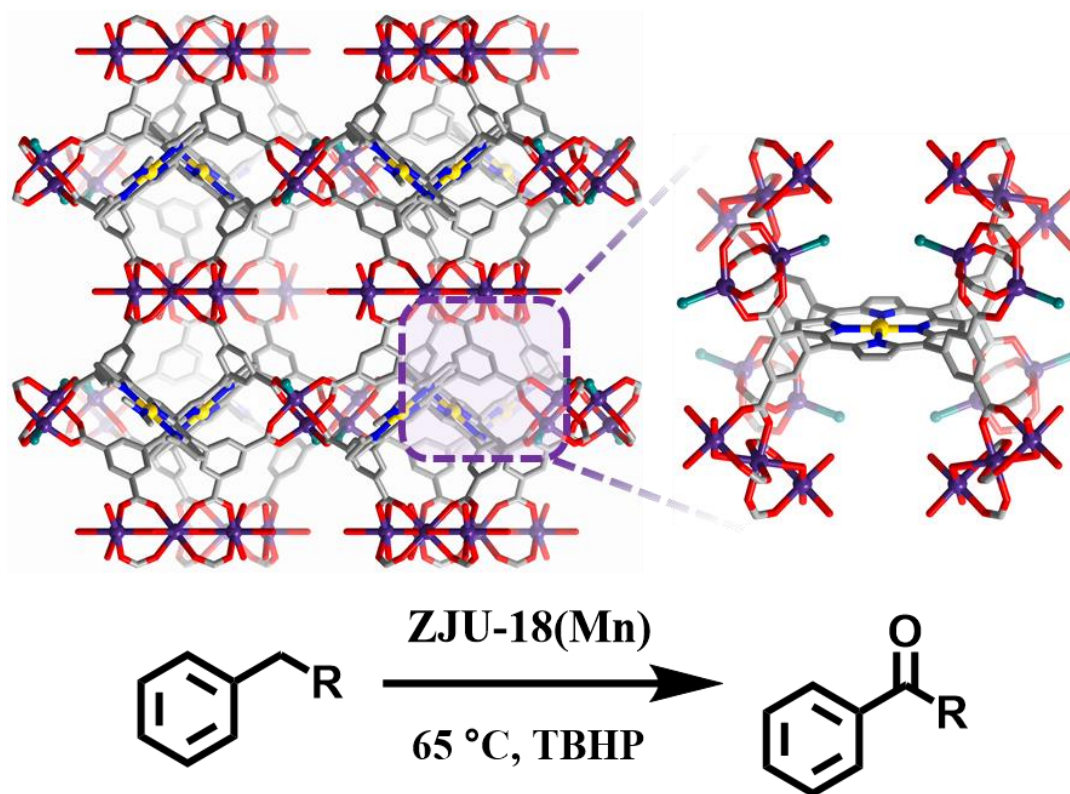
Figure 7. Structure of ZJU-18 featuring Mn-nodes and Mn-porphyrin linker sites for the catalytic oxidation of alkylbenzene to ketones.
