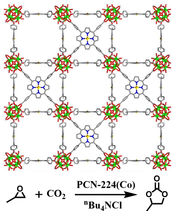
Figure 5. The structure of PCN-224 featuring cobalt porphyrin sites for catalyzing CO 2 insertion into epoxide.
