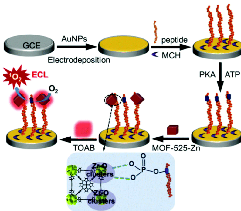
Figure 14. Schematic illustration of the electrochemiluminescence kinase activity assay using MOF-525 featuring Zn-porphyrin sites. Reproduced with permission from ref. 239. Copyright 2016 Royal Society of Chemistry.
