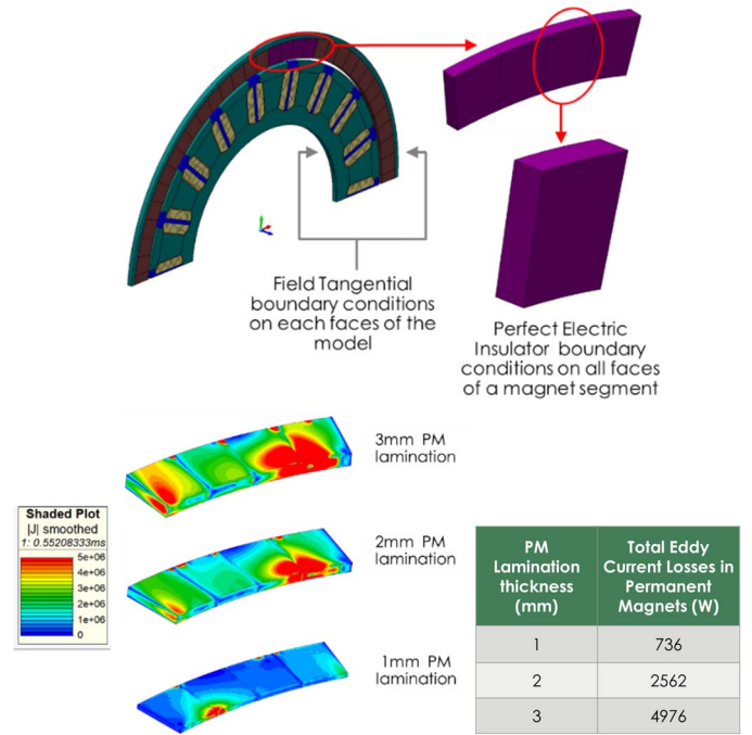
Fig. 10. Calculation of PM Eddy Current Loss.
