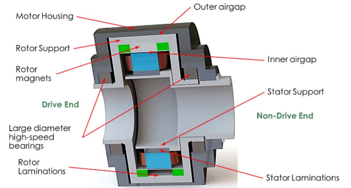
Fig. 14. Mechanical assembly.
