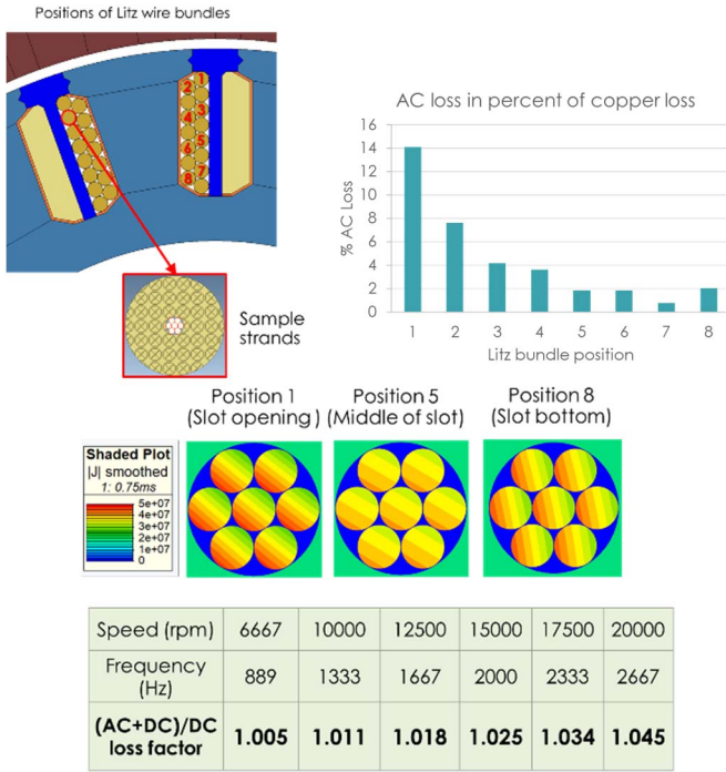
Fig. 9. AC Loss Calculation.
