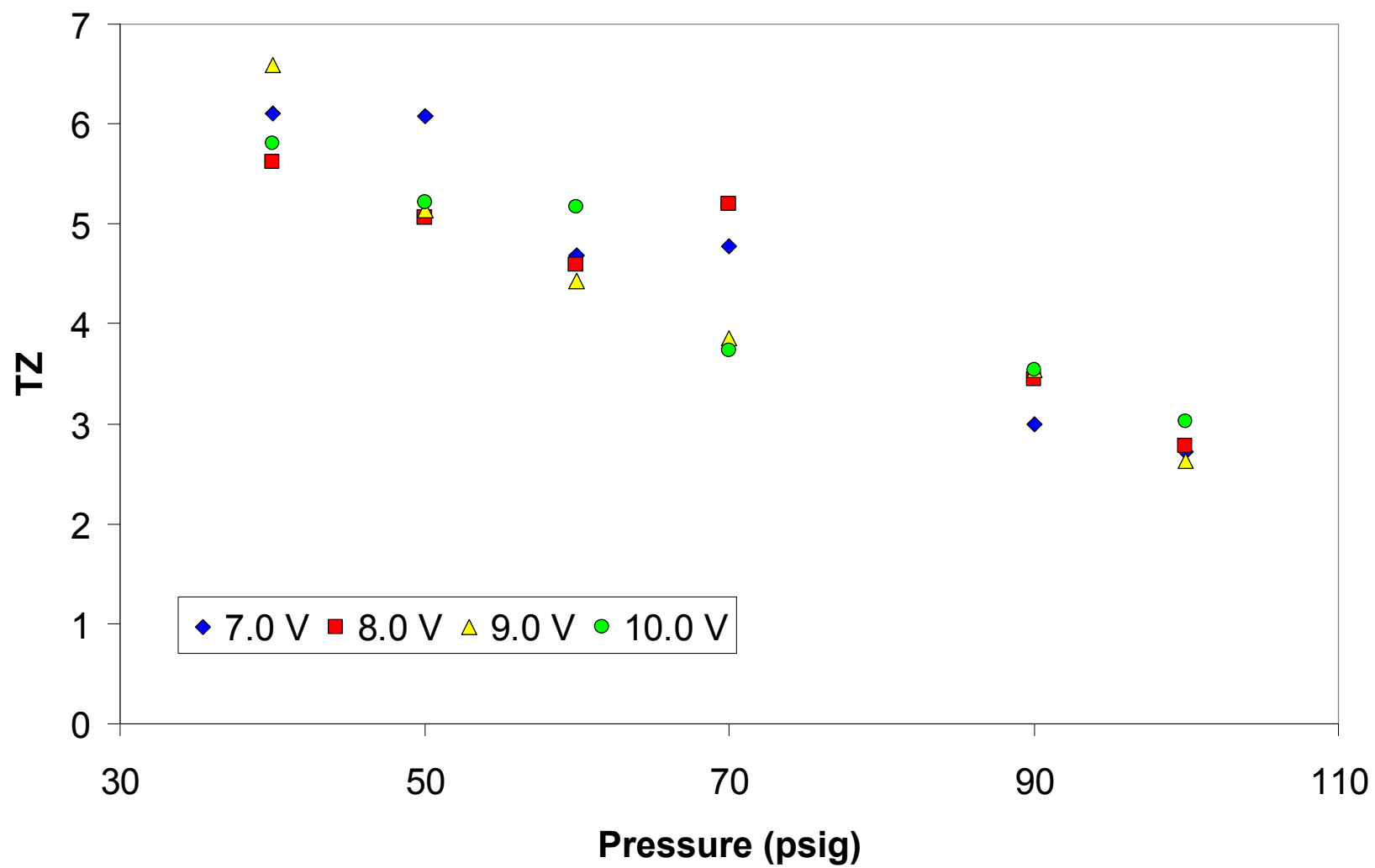
Figure 6.9. Plot of C8-C12 TZ vs. inlet pressure for various applied valve voltages.
