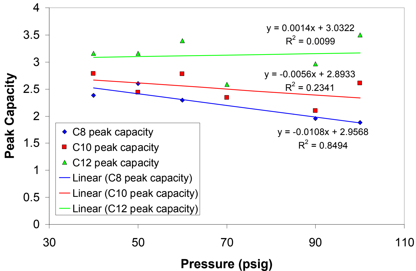
Figure 6.8. Plot of 9.0 V applied voltage maximum peak capacity vs inlet pressure for three n-alkanes.
