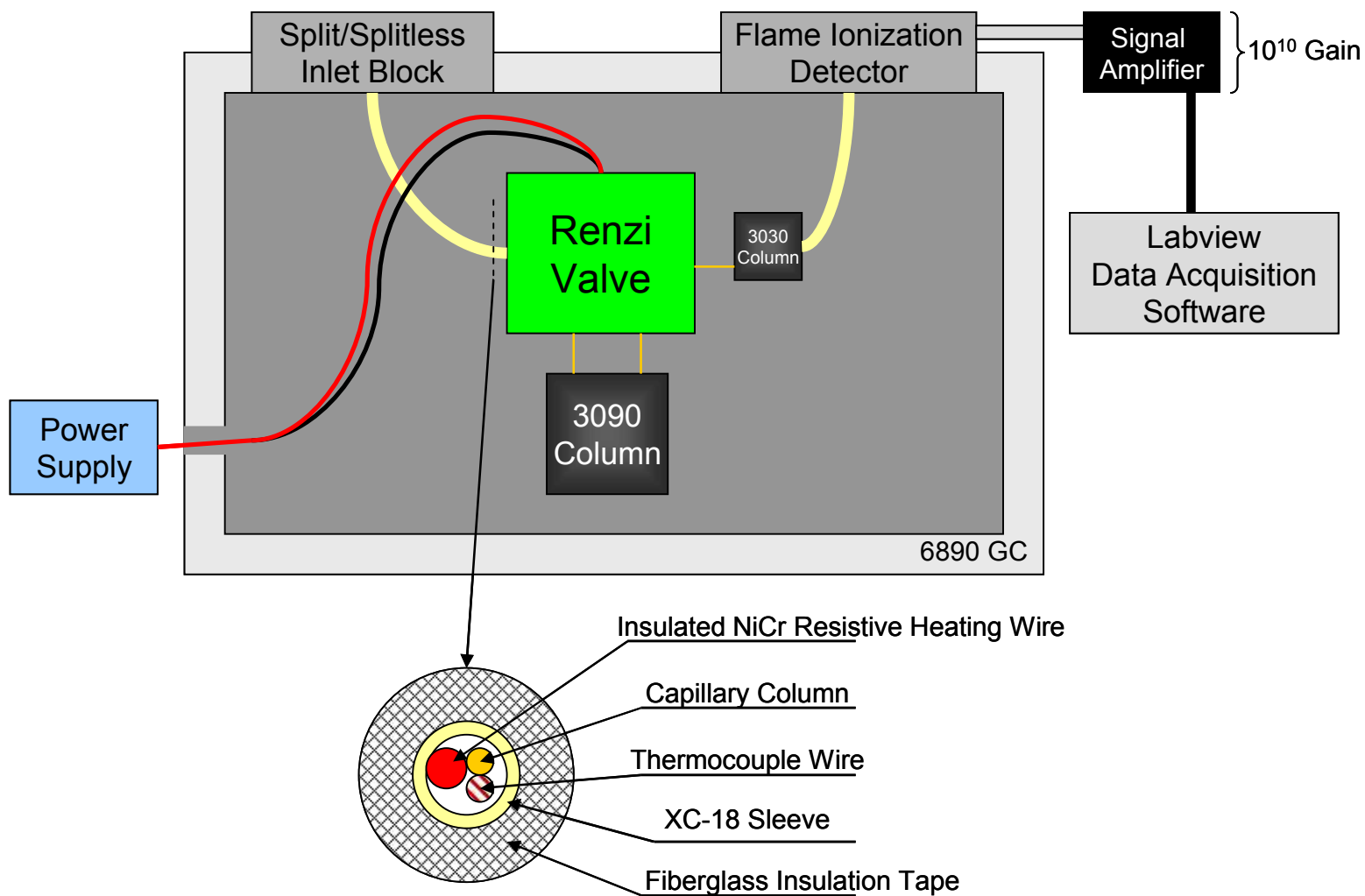
Figure 6.1. Instrument Schematic
