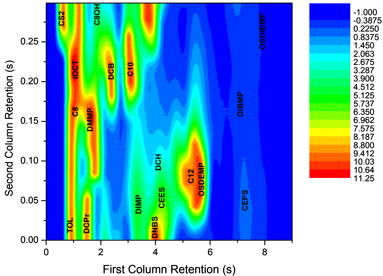
Figure 6.7. 18 component separation using the Renzi valve modulator.
