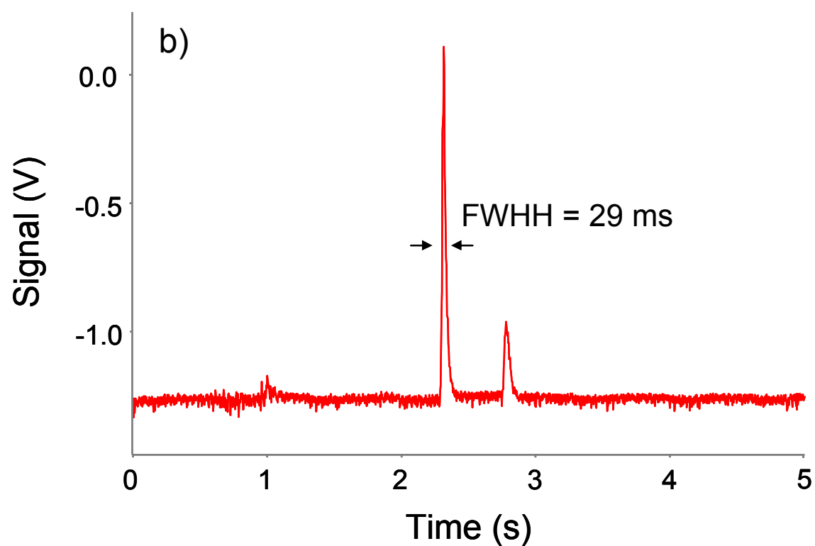
Figure 6.4. Representative depiction of methane modulation. The inlet pressure and applied valve voltage are: a) 15 psig and 10.0 V; b) 40 psig and 4.0 V.
