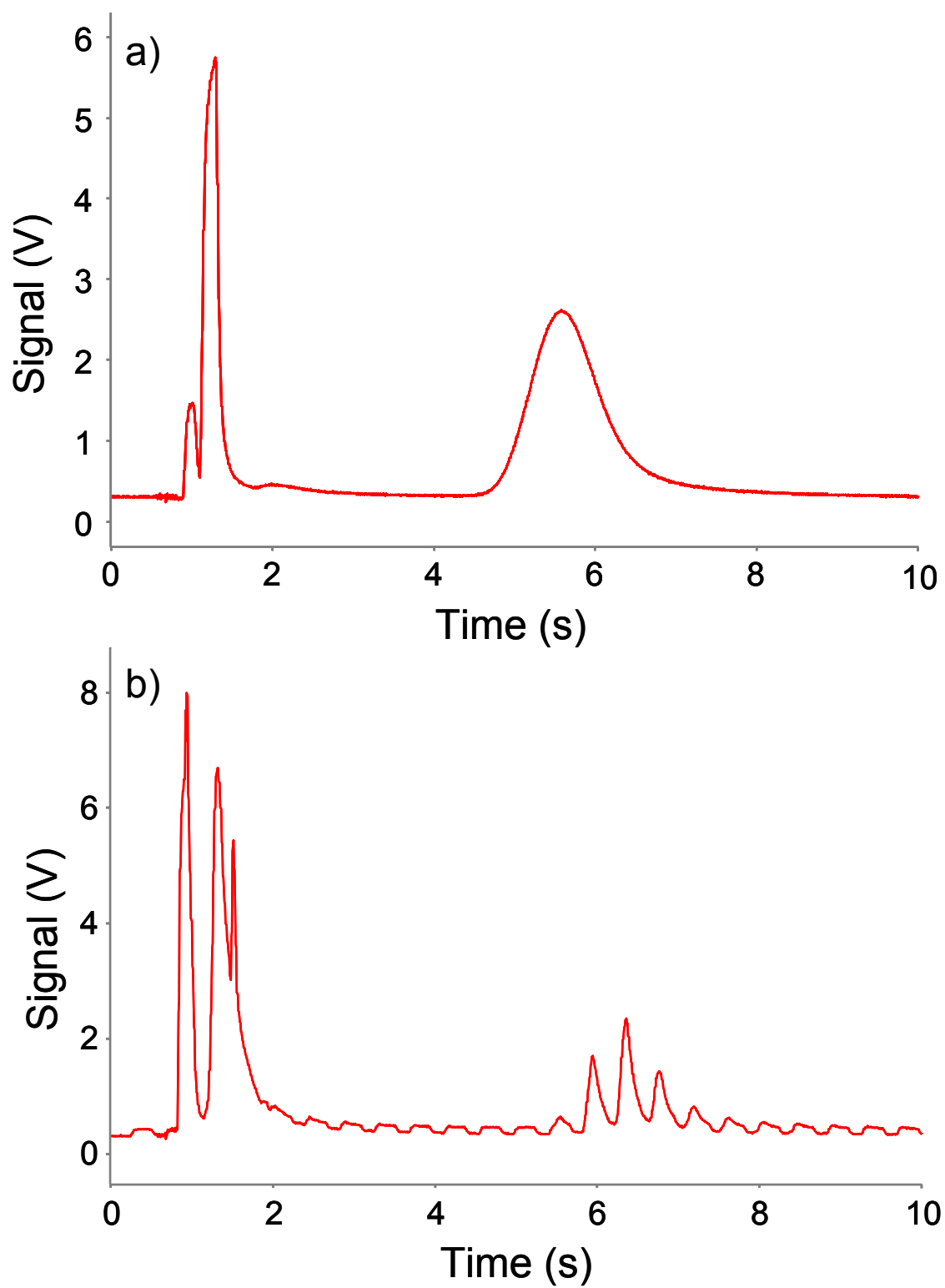
Figure 6.6. Dodecane sample a) unmodulated and b) modulated with 6.0 V valve voltage.
