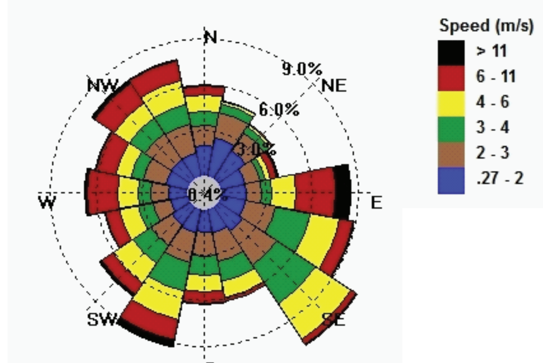
2011 Annual Windrose from Tower A36
