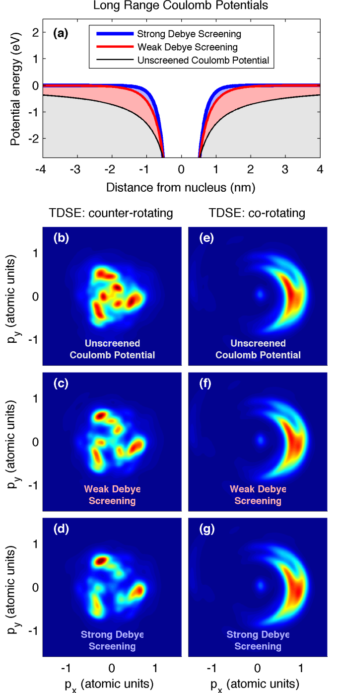
FIG. 4. (color online) Time-dependent Schrödinger equation (TDSE) simulations investigating the effects of the Coulomb potential. (a) The electron-nuclear potentials used in the TDSE calculations. (b-d) For the counter-rotating case, the low-energy structures disappear as the screening factor for the Coulomb potential is increased, confirming that the low-energy structures are due to strong electron-ion rescattering. (e-g) In the co-rotating case no change as the screening factor is varied, indicating the absence of rescattering.
