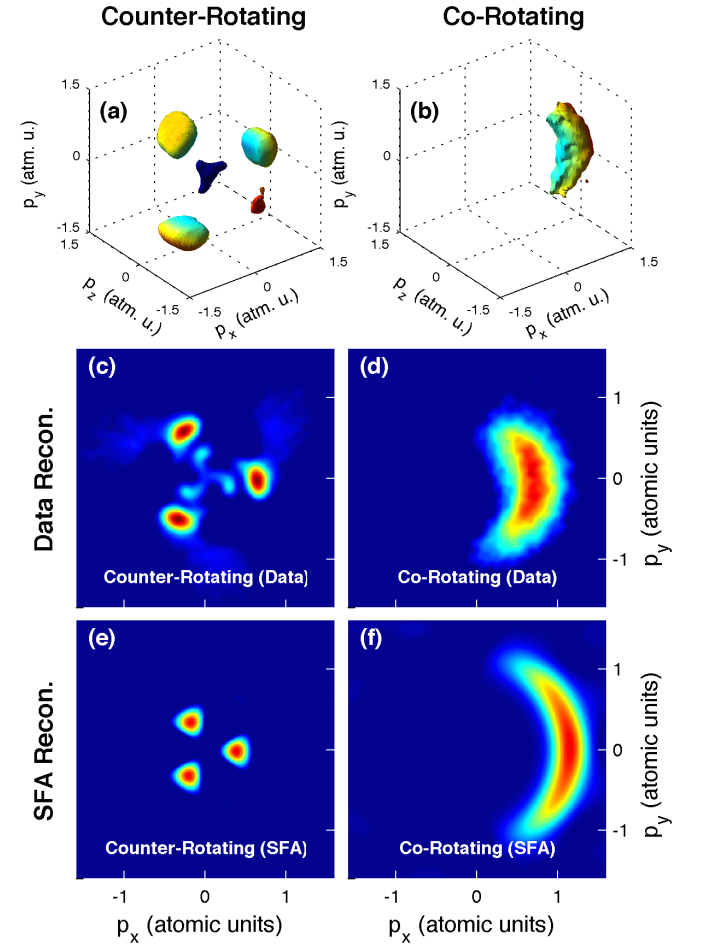
FIG. 3. (color online) (a,b) The experimental 3D photoelectron distribution for both counter- and co-rotating fields. (c-f) 2D projections of the 3D photoelectron distribution are compared to 2D SFA calculations. While the co-rotating data (d) is adequately reproduced by the SFA calculations (f), the counter-rotating case (c) exhibits low-energy structures that do not appear in the SFA model (e).
