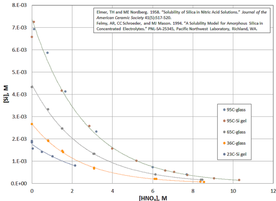
Figure 12. Solubility of Silica in Nitric Acid (Elmer and Nordberg 1958; Felmy et al. 1994)
