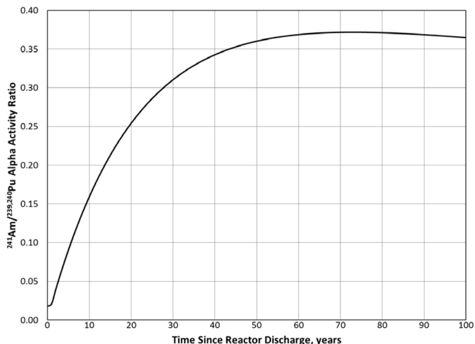
Figure 26. Americium-241/Pu-239,240 Alpha Activity Ratio for Weapons-Grade Plutonium as a Function of Time from Reactor Discharge
