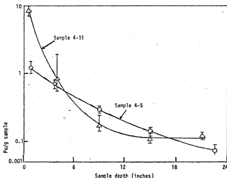
Figure 29. Plutonium Concentrations for Samples 4-5 and 4-11 of 216-Z-9 as Functions of Depth (Figure 5 of Swanson 1973)
