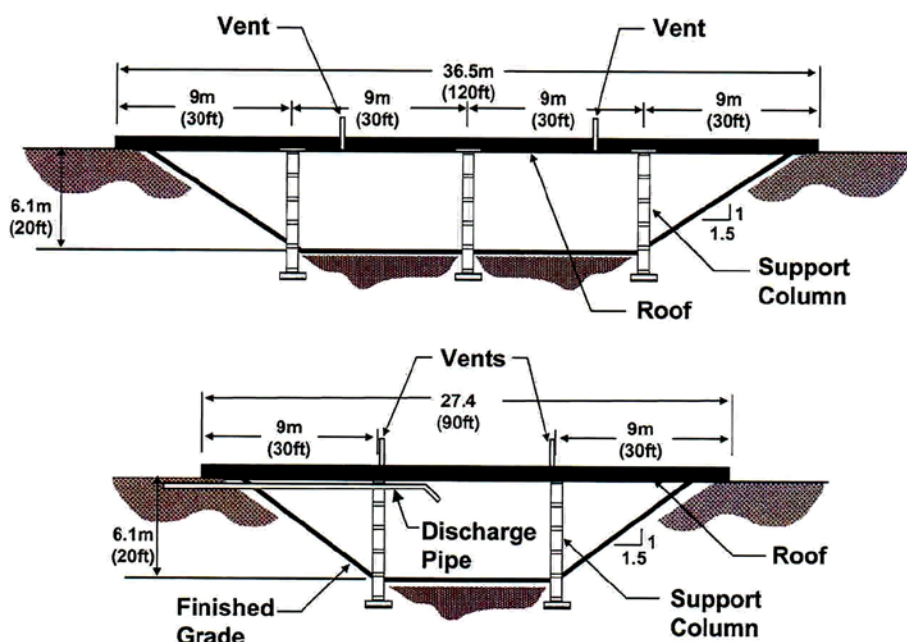
Figure 15. As-Constructed 216-Z-9 Crib during Time of Service (Figure 2-3 of Winkel 2018)
