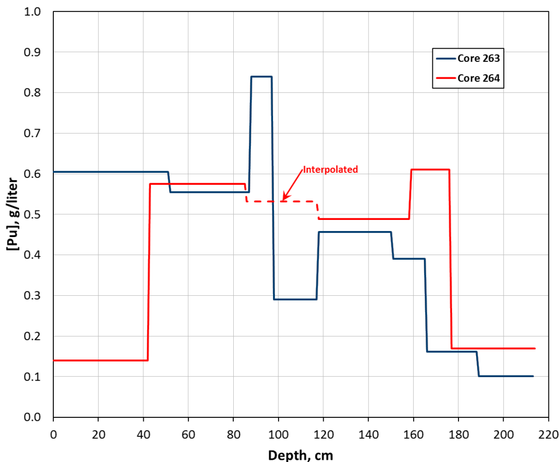
Figure 14. Plutonium Concentration Profiles in Tank 241-Z-361 from Cores 263 and 264
