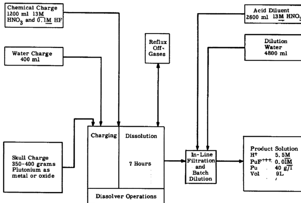
Figure 10. Skull and Oxide Dissolution Flowsheet (Figure 9 of Judson et al. 1956a)
