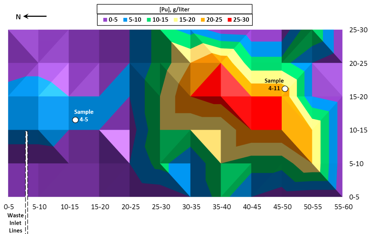
Figure 28. Plutonium Concentration Profile in Top Inch of Z-9 (based on pages N-17 and B-4 of Smith 1973)
