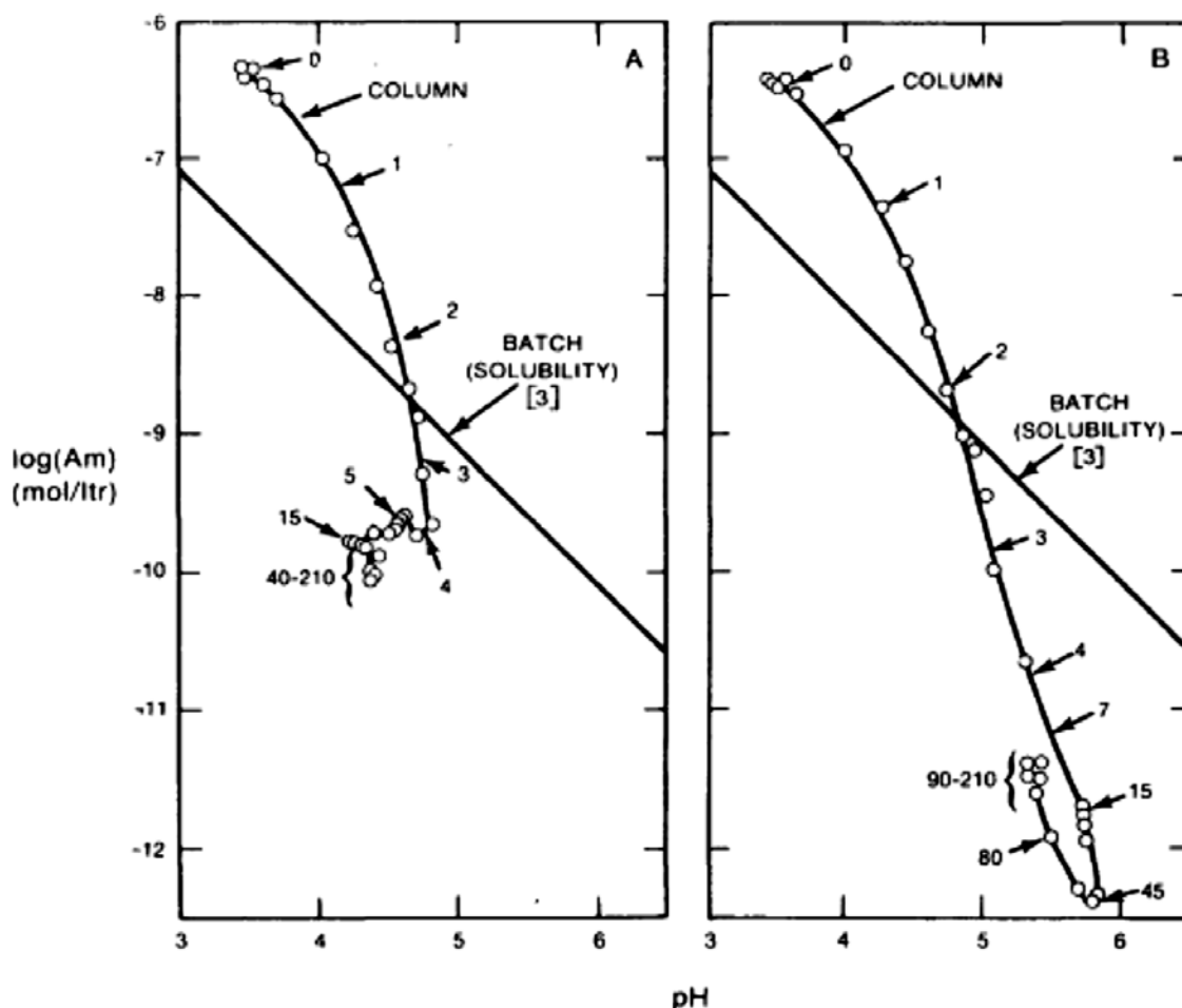
Figure 32. Saturated Column Americium Leaching from 216-Z-1A Sediments Using A: 0.01 M \text{CaCl}_2 and B: Simulated Groundwater. Numbers show throughput column pore volumes. (Figure 1 of Delegard et al. 1981)
