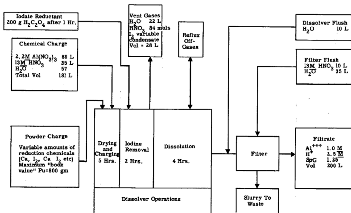
Figure 8. Scrap Dissolution for Reduction Misfire Charges (Figure 7 of Judson et al. 1956a)
