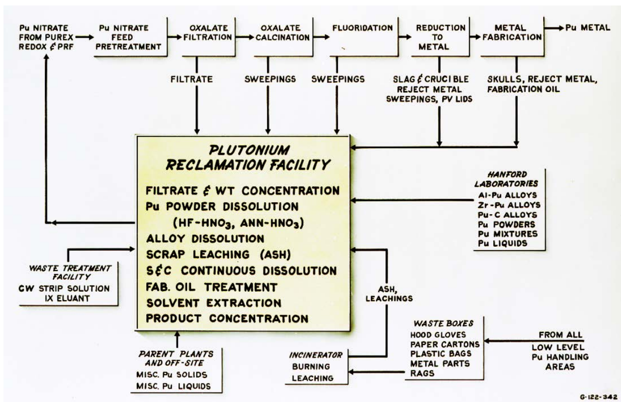
Figure 5. Plutonium Scrap Recovery Sources for the PRF (from Figure 1 of Bruns 1967 from Hanford drawing 38336-4CN)
