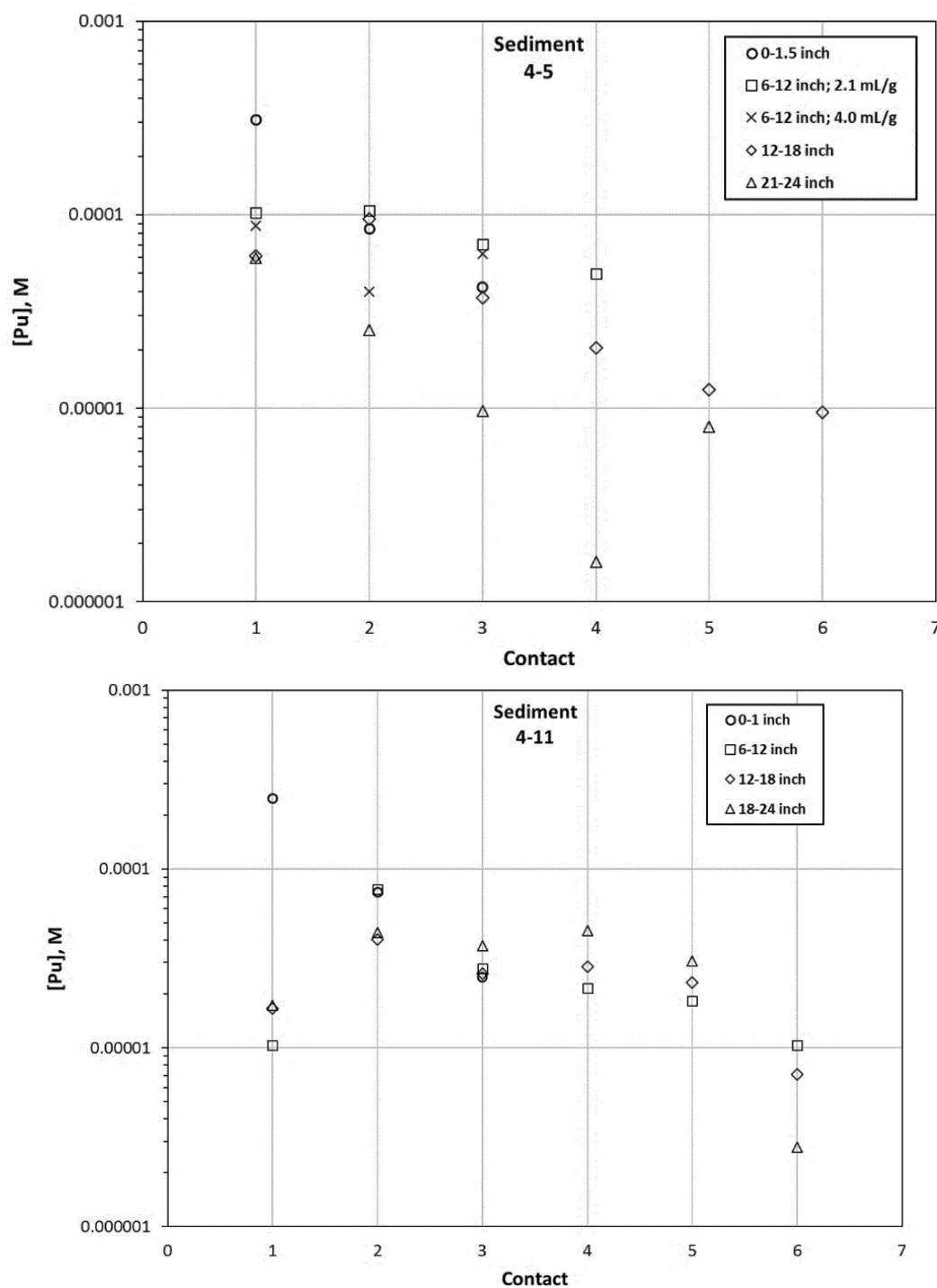
Figure 31. Pu Solution Concentrations in Multiple Leach Contacts with 4-5 and 4-11 Z-9 Sediment (based on data from Swanson 1973)
