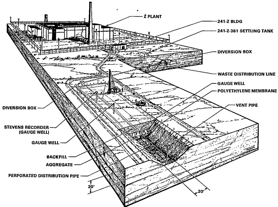
Figure 21. The 216-Z-12 Crib (Figure 6 in Kasper 1982)
