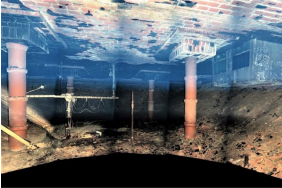
Figure 17. View to the North Interior of the Z-9 Crib When Mining Was Underway (Figure 2-4 of Winkel 2018; note operations cubicle in ceiling to the right)
