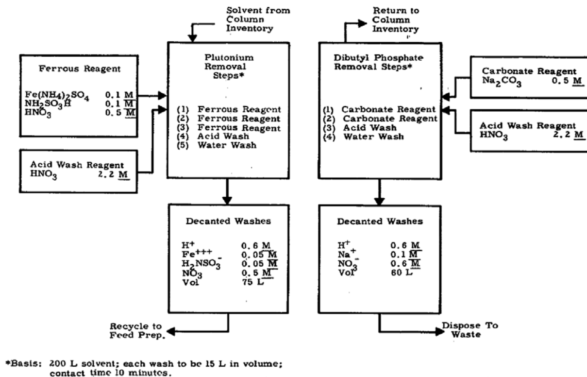
Figure 13. Solvent Treatment for Plutonium and DBP Removal (Figure 28 of Judson et al. 1956b)
