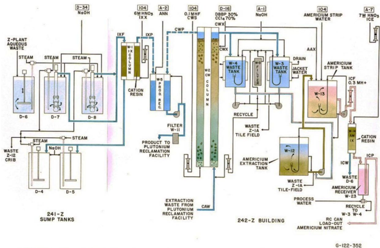
Figure 6. Waste Treatment and Americium Recovery Flowsheet for the 242-Z Building
