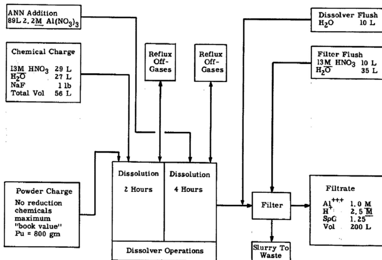
Figure 9. Pu Oxide Scrap Dissolution Flowsheet (Figure 8 of Judson et al. 1956a)
