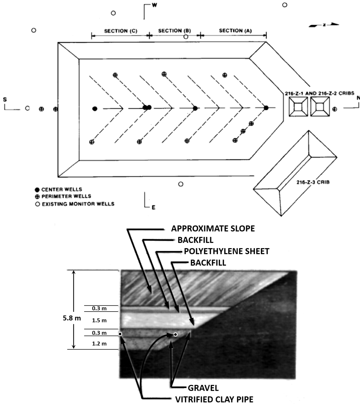
Figure 20. Plan View (above) of 216-Z-1, Z-2, Z-3, and Z-1A Cribs and Section View (below) of 216-Z-1A (Kasper et al. 1979, Kasper 1982)
