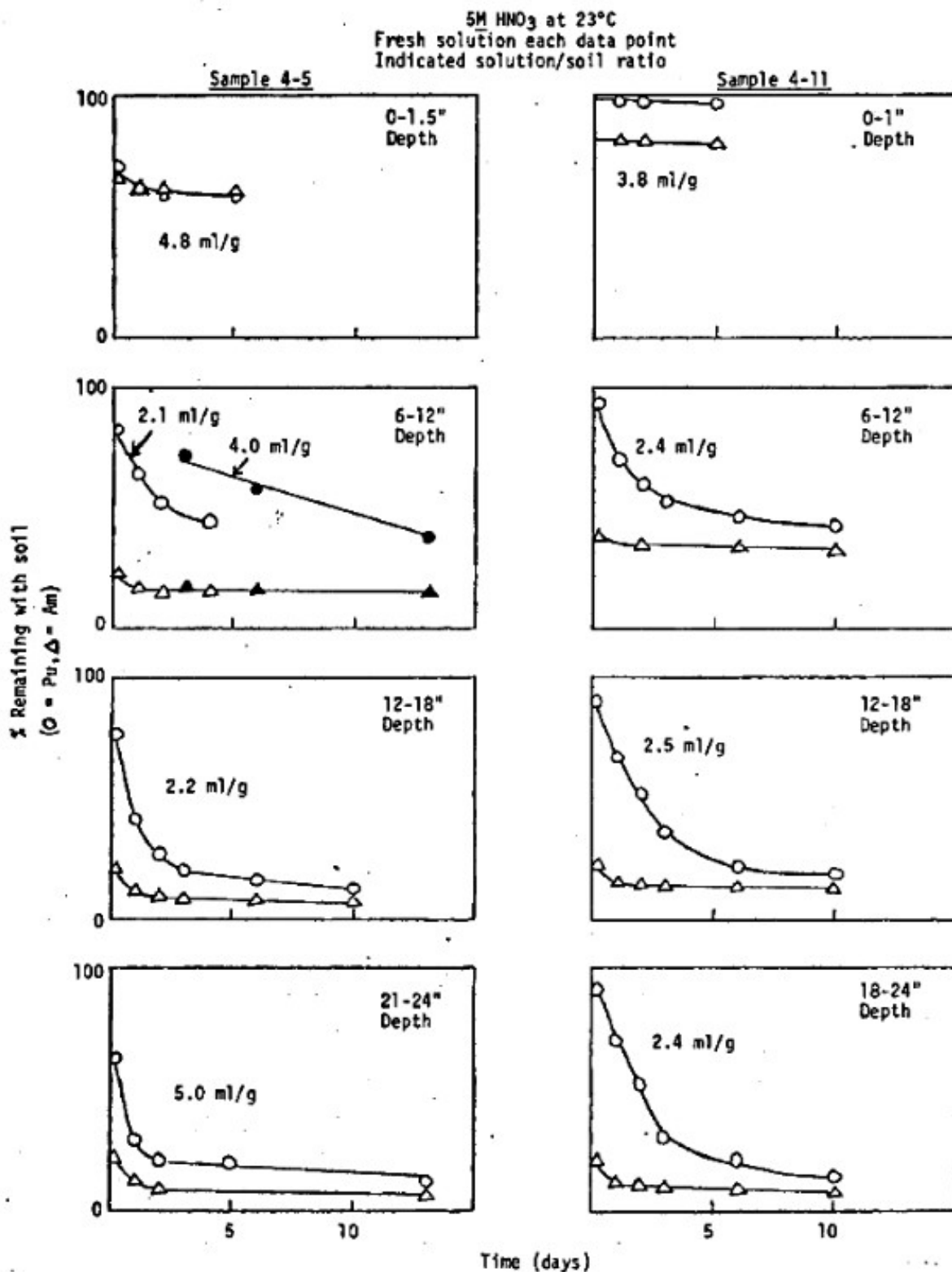
Figure 30. Z-9 Sediment Leaching Behavior Using 5 M HNO 3 (Figure 1 of Swanson 1973)
