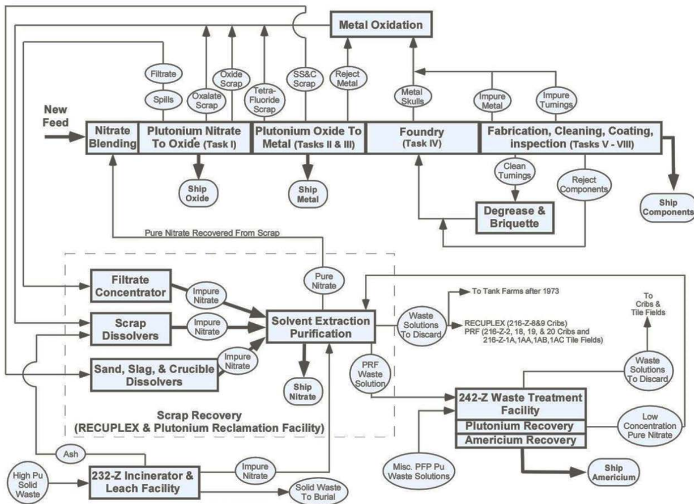
Figure 2. Plutonium Processing Cycle at the PFP (Hoyt and Teal 2004)
