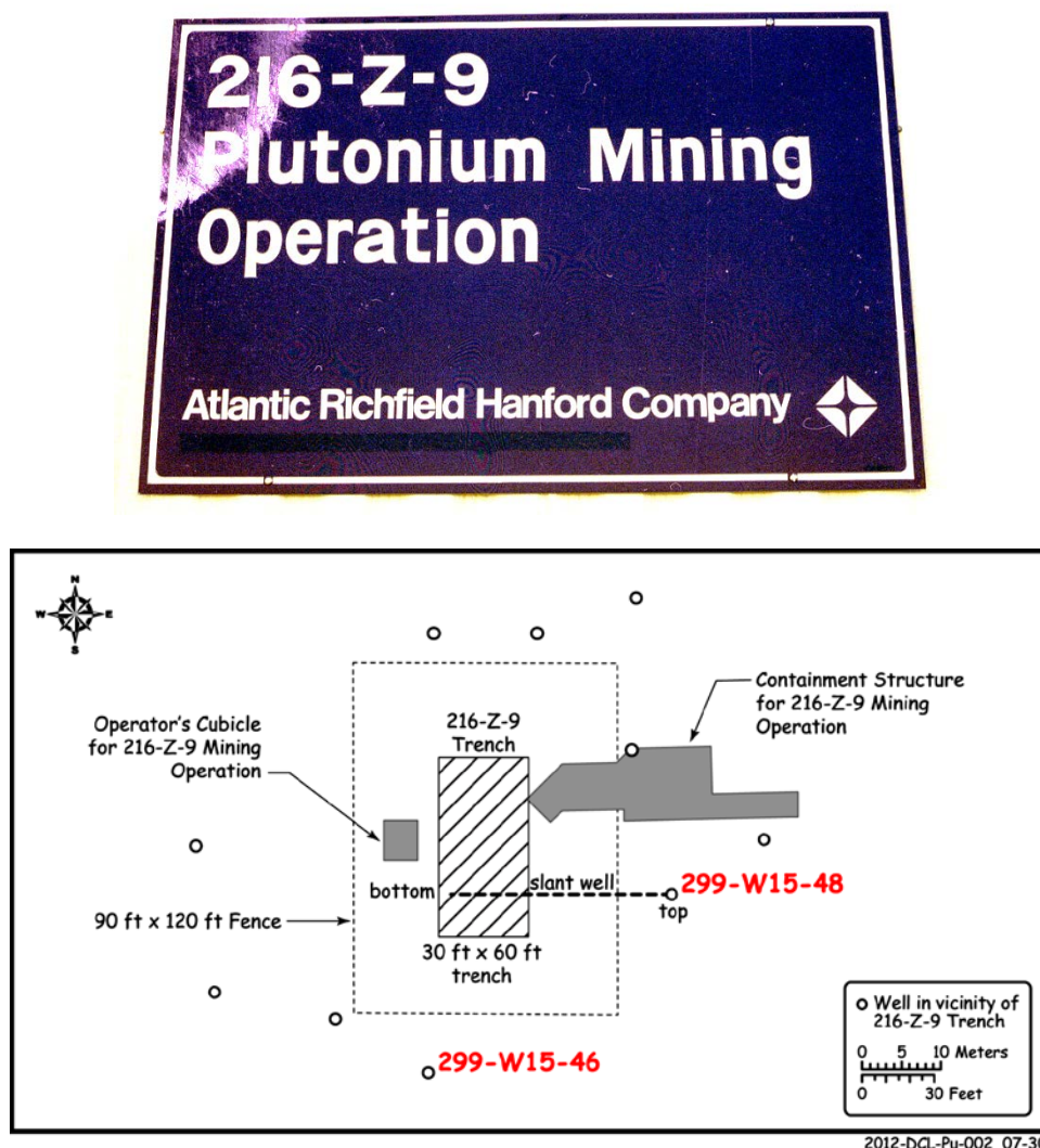
Figure 16. Support Buildings for 216-Z-9 Plutonium Mining. Top: Sign on support building (image 72698-29CN from Hanford Site photo archive). Bottom: Support building (216-Z-9A) and operations cubicle layout (Figure 3.4 of Cantrell and Felmy 2012)
