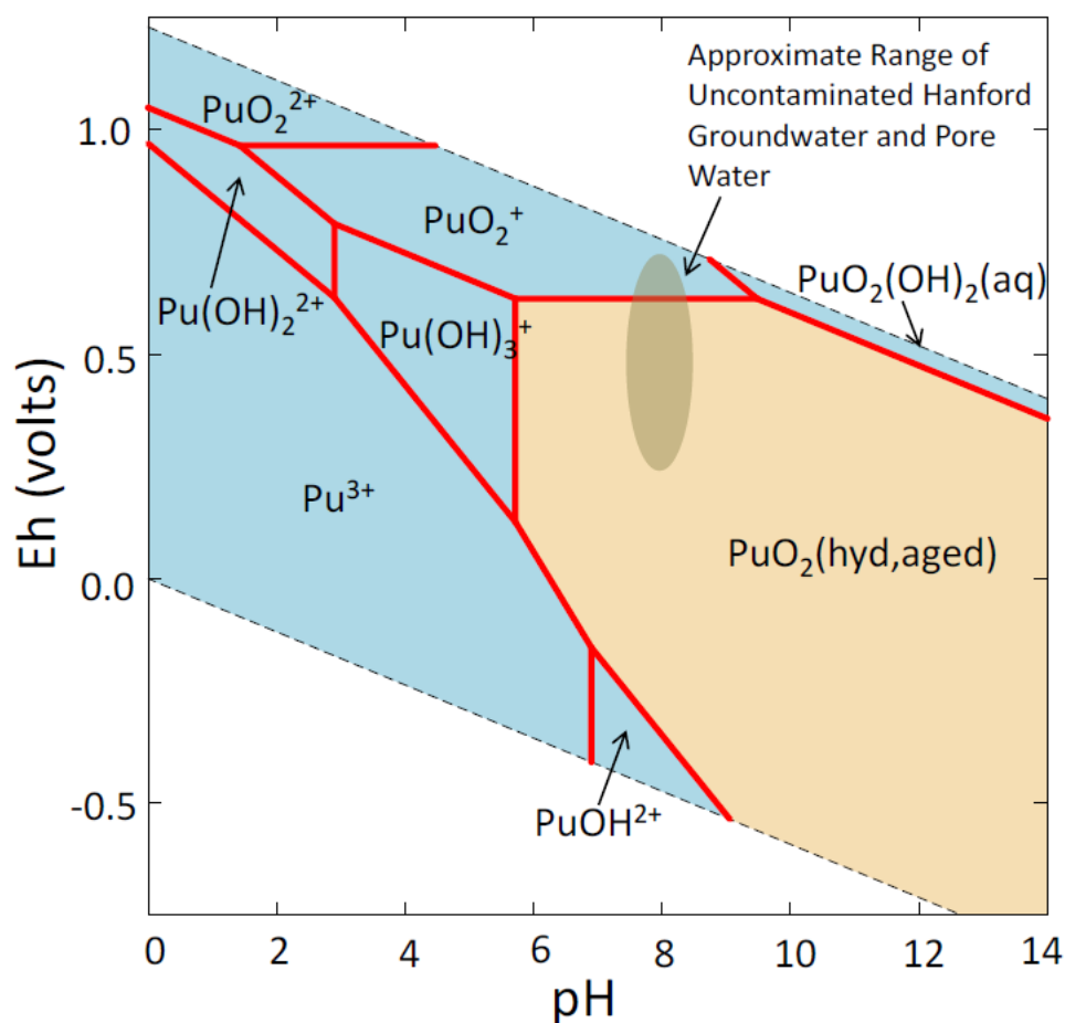
Figure 23. Eh pH Diagram for Plutonium at a Concentration of 10^{-10} M (1,500 pCi/L, the maximum contaminant level, MCL) in Pure Water (298.15 K, 0.1 MPa) (Figure 4.2 in Cantrell and Felmy, 2012)
