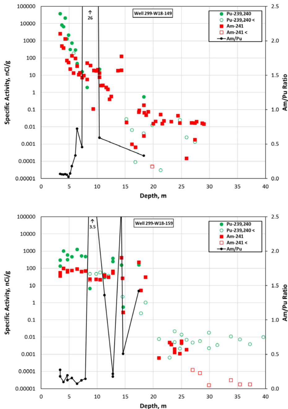
Figure 25. Plutonium and Americium Concentrations and Americium/Plutonium Concentration Ratios in Two Centerline Wells in 216-Z-1A as Functions of Depth (data from Appendix B of Price et al. 1979)
