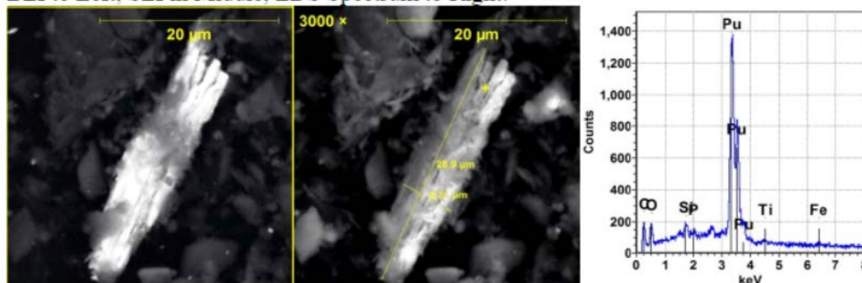
Figure 11. Plutonium-Rich “Petrified Wood” Plutonium Particle from the Z-9 Crib (McCoskey and Cooke 2013)
