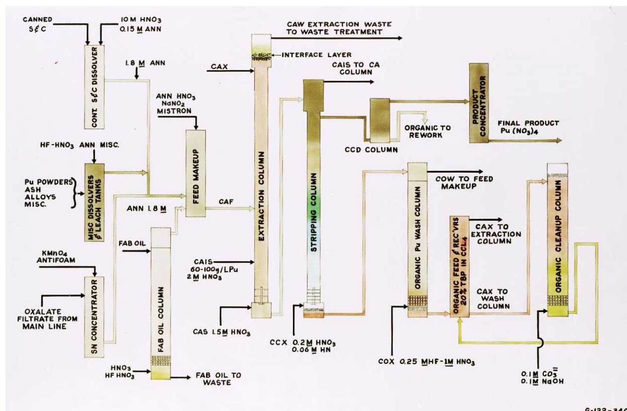
Figure 4. PRF Flowsheet (from Figure 2 of Bruns 1967 from Hanford drawing 38336-3CN)
