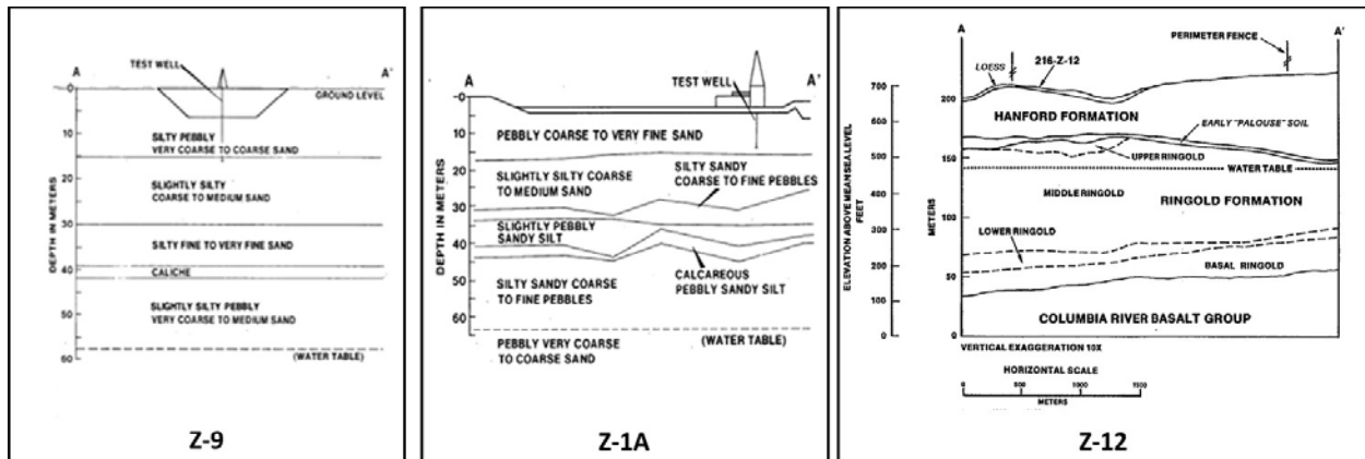
Figure 22. Stratigraphy and Granulometry of Sediments beneath the 216-Z-9, 216-Z-1A, and 216-Z-12. Top: stratigraphy (Figure 2 of Parker and Singleton 1995; see also page C-6 of Lindsey 1996). Bottom: granulometry (from Figures 1, Z-9, and 2, Z-1A, of Price and Ames 1975 and Figure 12, Z-12, of Kasper 1982; descriptions seemingly related to US Geological Survey terms 1 )
