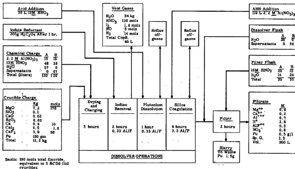
Figure 7. SS&C Dissolution Flowsheet in RECUPLEX (Figure 5 of Judson et al. 1956a)
