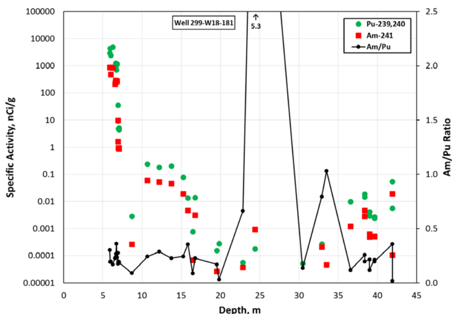
Figure 27. Plutonium and Americium Concentrations and Americium/Plutonium Concentration Ratios in Centerline Well in 216-Z-12 as Functions of Depth (data from Appendix C of Kasper 1982)
