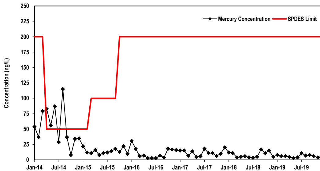
Figure 3-4. Maximum Concentrations of Mercury Discharged from the BNL Sewage Treatment Plant, 2014–2019.
