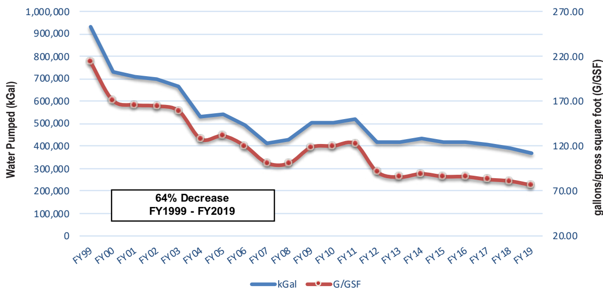
Figure 2-2. Annual Potable Water Use, 1999-2019.
