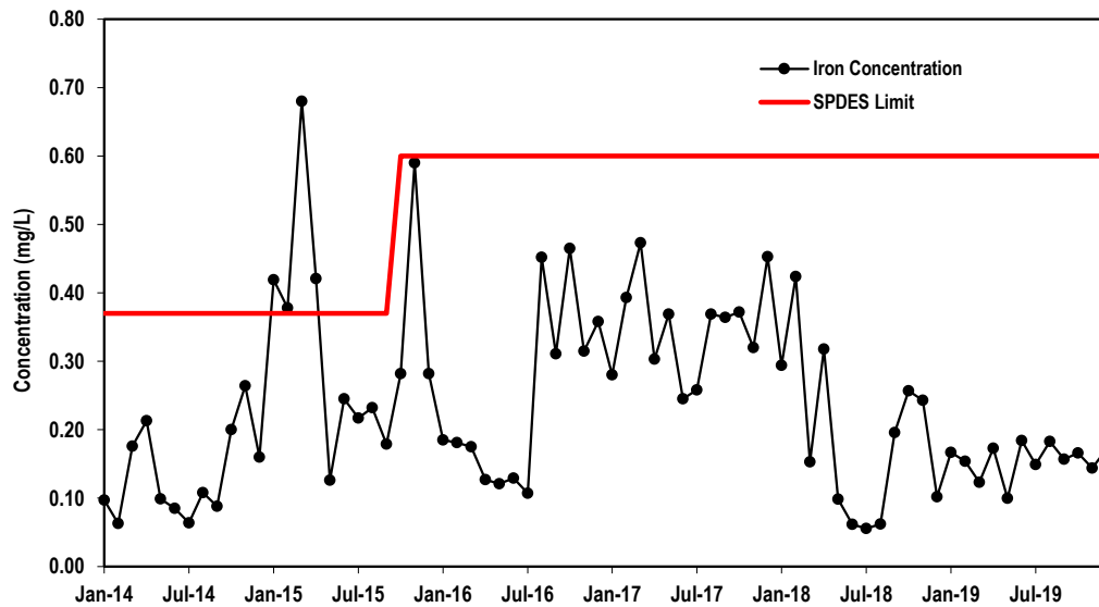
Figure 3-2. Maximum Concentrations of Iron Discharged from the BNL Sewage Treatment Plant, 2014–2019.
