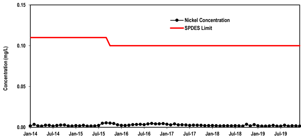
Figure 3-5. Maximum Concentrations of Nickel Discharged from the BNL Sewage Treatment Plant, 2014–2019.
