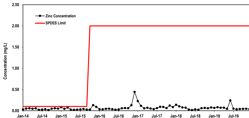
Figure 3-7. Maximum Concentrations of Zinc Discharged from the BNL Sewage Treatment Plant, 2014–2019.
