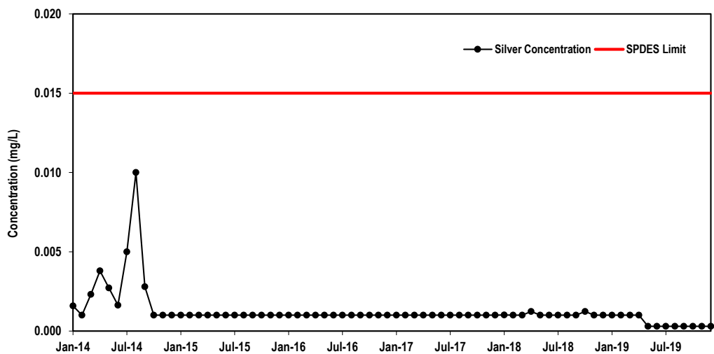
Figure 3-6. Maximum Concentrations of Silver Discharged from the BNL Sewage Treatment Plant, 2014–2019.
