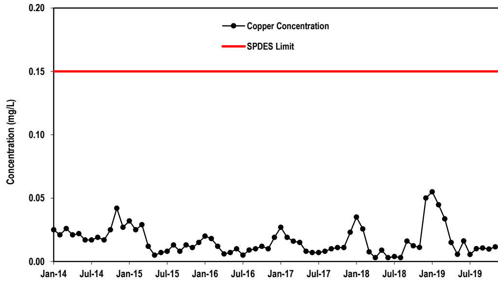
Figure 3-1. Maximum Concentrations of Copper Discharged from the BNL Sewage Treatment Plant, 2014–2019.
