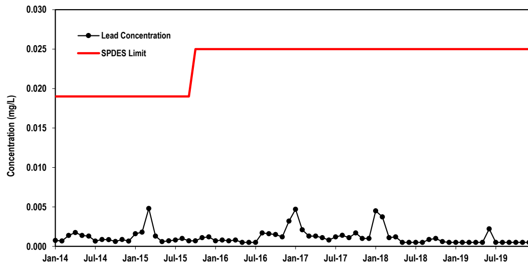
Figure 3-3. Maximum Concentrations of Lead Discharged from the BNL Sewage Treatment Plant, 2014–2019.
