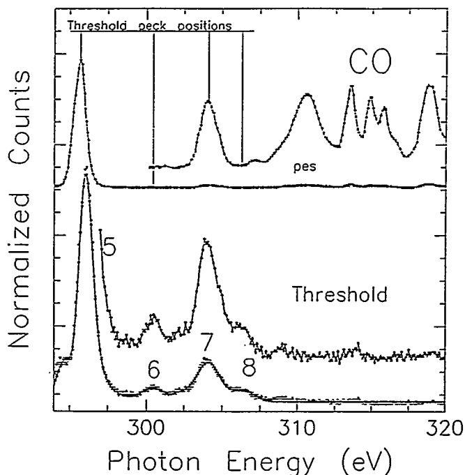
Figure 1. ZKE scan of CO above the C1s threshold. The solid line is a least-squares fit to the spectrum. Included for comparison is the PES spectrum of Gelius et al. 1
