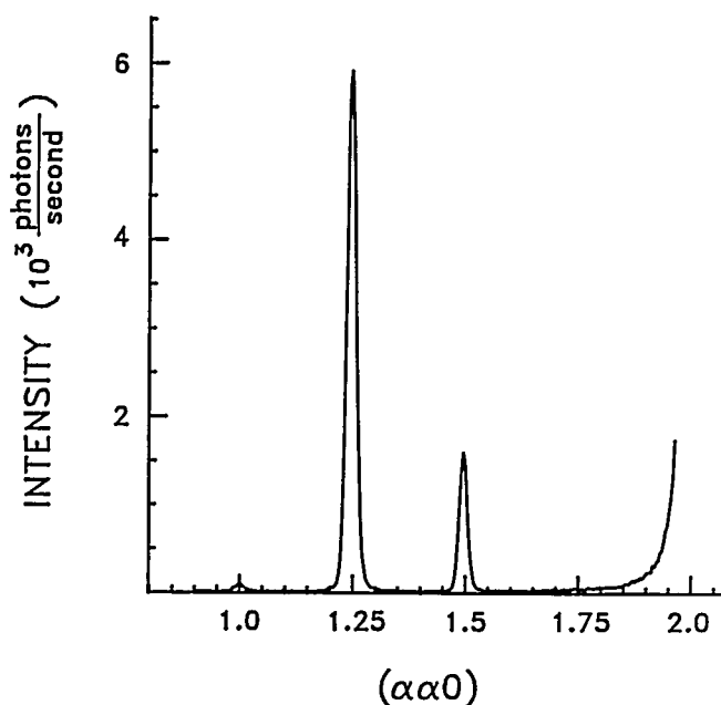
Fig. 2: Data along the (110) azimuth from a GaAs (001) surface prepared at 500 C in 100 torr of flowing H 2 .
