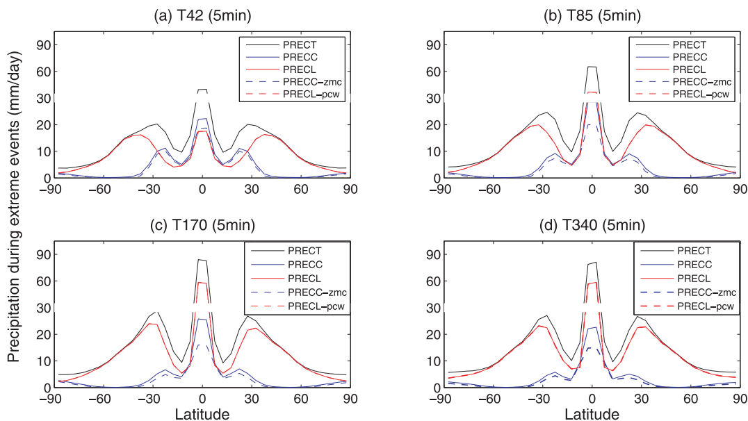
Fig. 2. Different components of the time-averaged, zonal-averaged daily precipitation extremes ( \text{mm day}^{-1} ) during 95% percentile extreme events from simulations at four different spatial resolutions and a fixed 5-min timestep. The dashed red line falls under the solid red line.
