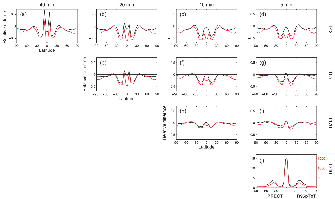
Fig. 1. The relative difference of time-averaged, zonal-averaged daily total precipitation (PRECT) in black and precipitation extremes ( R95pTOT ) in red, with respect to results from a T340 reference simulation run with a 5 min physics time step. The relative difference is calculated by (T_{xx} - T340)/T340 . Panel j shows the absolute amounts of daily precipitation ( \text{mm day}^{-1} ; black axis) and R95pTOT precipitation extreme ( \text{mm year}^{-1} ; red axis) in the T340 reference case.
