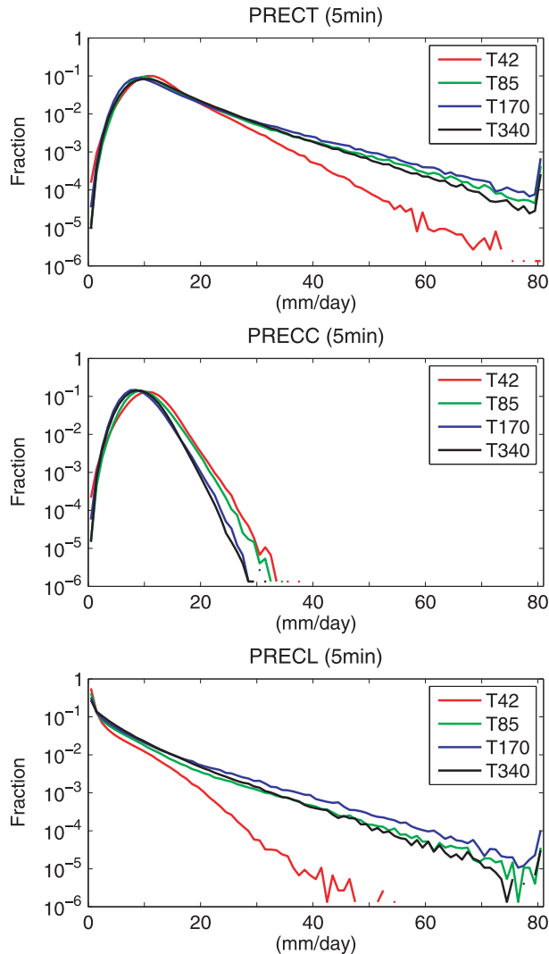
Fig. 3. Probability distributions of daily precipitation in the equatorial zone from 5° S to 5° N aggregated in 1 mm day -1 bins from 0 to 80 mm day -1 . Precipitation larger than 80 mm day -1 is treated as one bin. Distributions of total precipitation (PRECT), convective precipitation (PRECC) and large-scale precipitation (PRECL) are shown for simulations at four horizontal resolutions and a fixed 5-min timestep.
