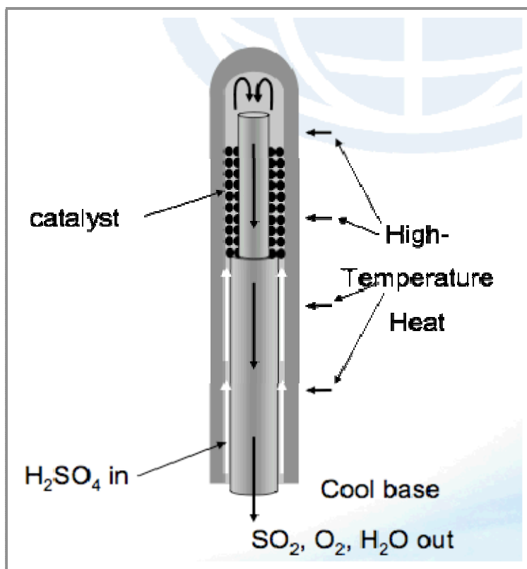
Figure 4.1.1 Bayonet decomposition reactor designed by Sandia National Laboratories
