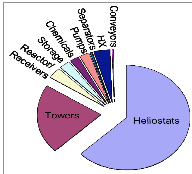
Figure 4.6.5 Estimated capital cost distribution for the mixed metal oxide realization of the Sodium Manganese cycle
