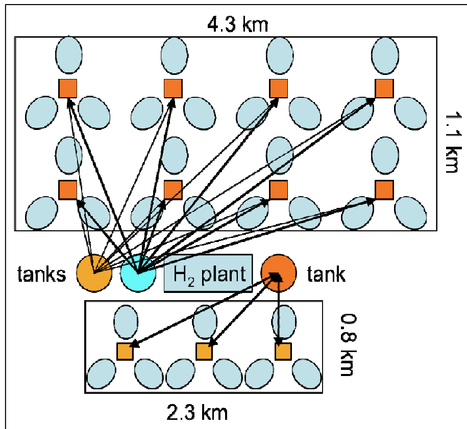
Figure 4.6.4 System layout with a single chemical plant for the Mx-Sodium Manganese cycle
