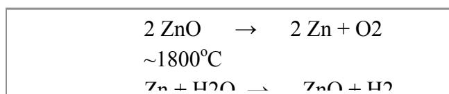
Figure 4.4.1 Zinc Oxide cycle chemistry
