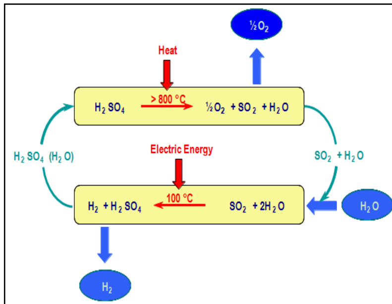
Figure 4.2.1 The Hybrid Sulfur cycle
