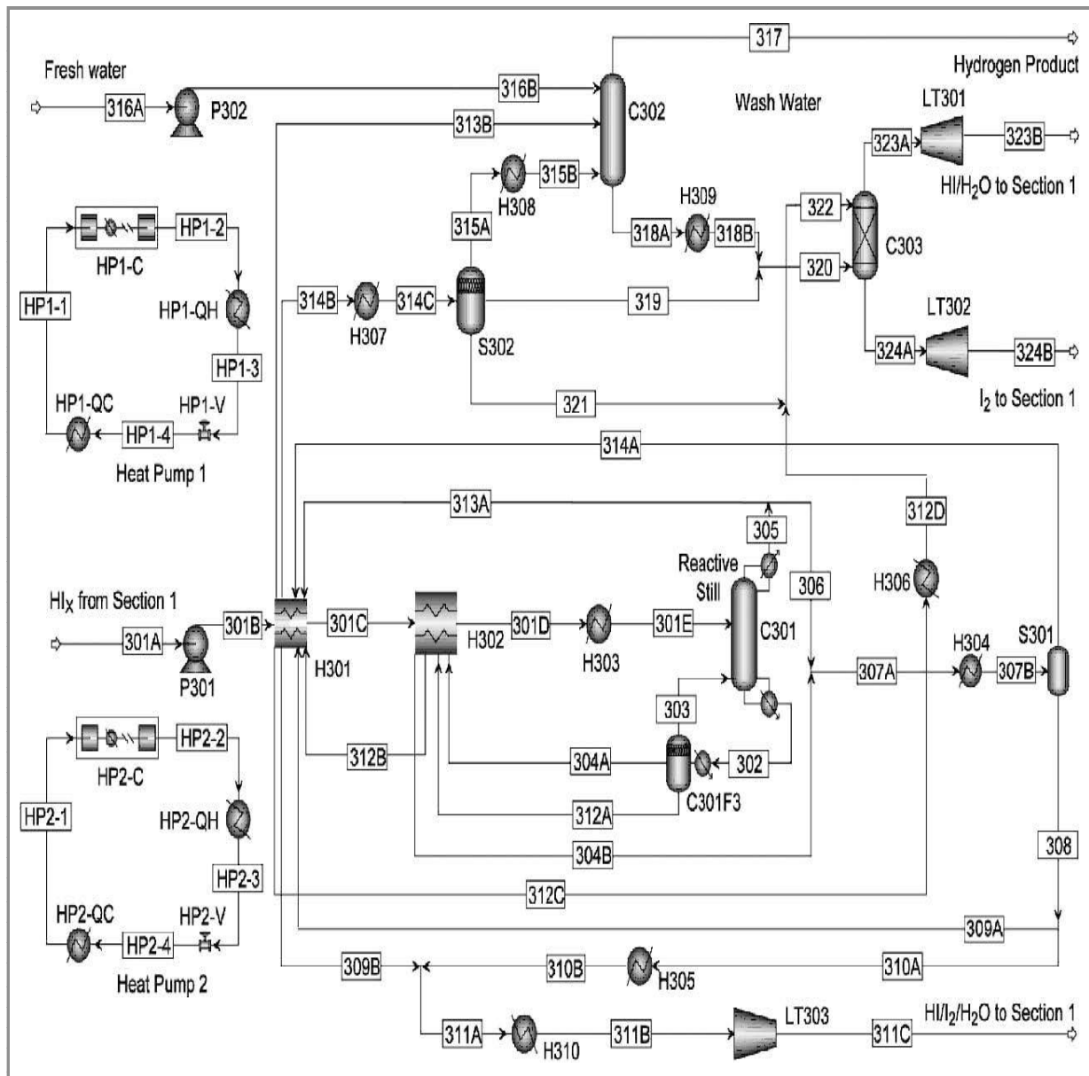
Figure 4.1.6 HI decomposition flow sheet (section 3)
