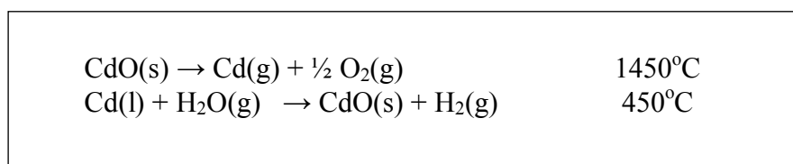
Figure 4.5.1 Chemical steps of the Cadmium Oxide cycle
