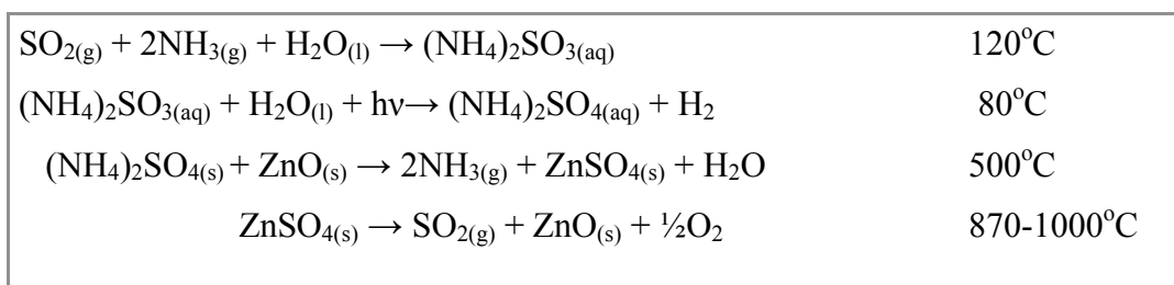
Figure 4.3.2 Process chemistry for Photolytic Sulfur Ammonia
