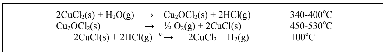
Figure 4.9.1 Hybrid Copper Chloride chemistry
