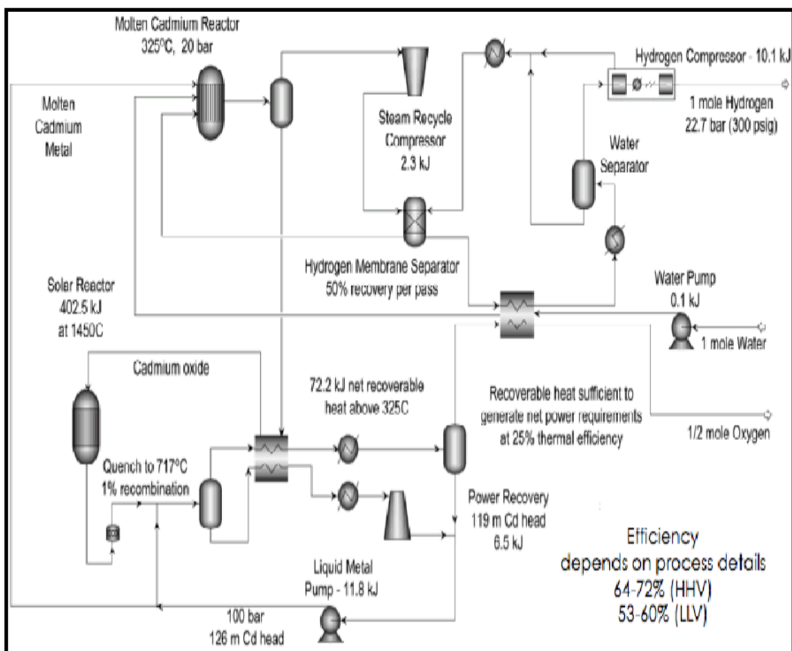
Figure 4.5.5 CdO cycle flowsheet, AIChE Meeting, Salt Lake City, November 7, 2007
