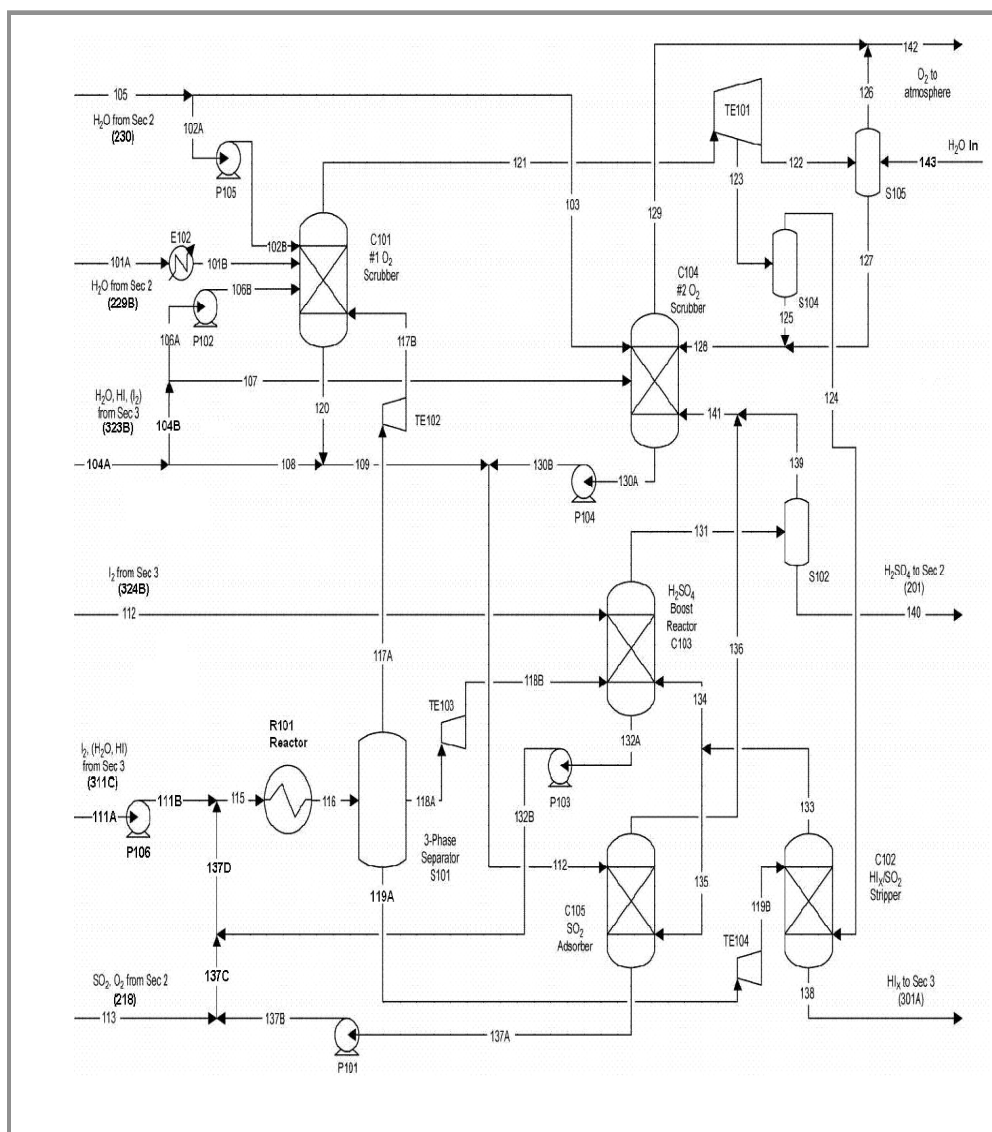
Figure 4.1.4 Bunsen reaction flowsheet (section 1)
