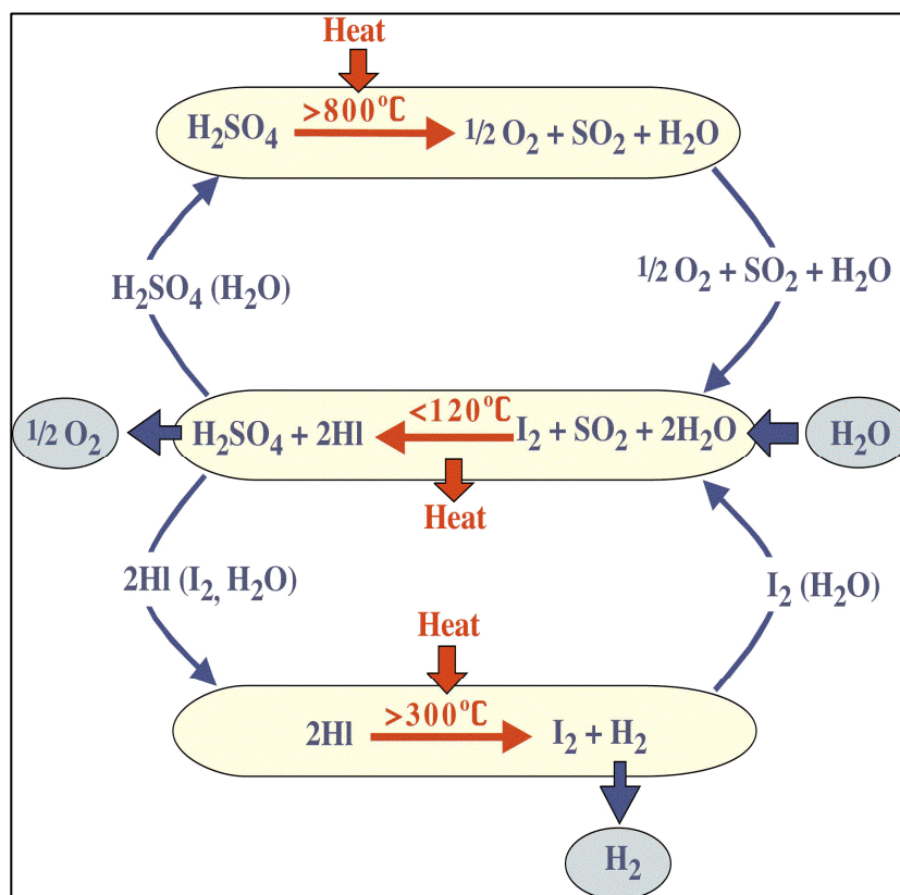
Figure 4.1.1 Sulfur Iodine three-step cycle
