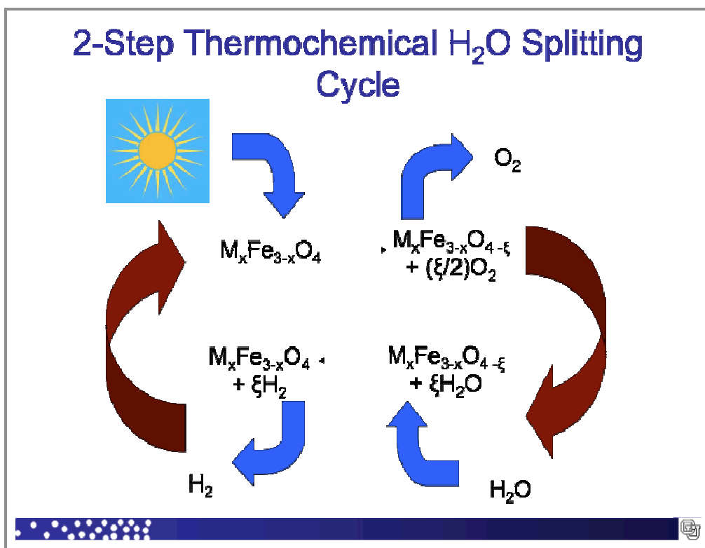
Figure 4.8.1 Schematic chemistry of a water-splitting ferrite cycle
