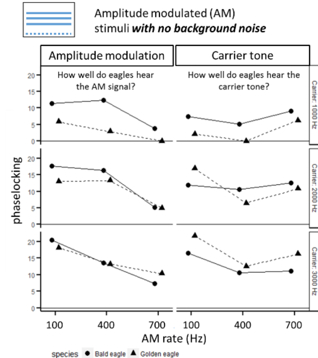
Figure K3. The stimuli with amplitude modulation (AM) are played with a chord consisting of three tones: a middle “carrier” tone, a higher sideband tone, and a lower sideband tone. The sideband tones are the same frequency distance from the carrier and produce an AM equal to that distance. For example a three tone set composed of a 2000 Hz carrier with 1600 Hz and 2400 Hz sideband tones ( \pm 400 Hz) yields an AM rate of 400 Hz. The auditory system of the eagle phaselocks to the three tones and also to the AM rate. Above, we show how Golden and Bald Eagles phaselock to the AM rate and to the carrier tone. We show data from the nine combinations we tested: three different carrier tones (3 rows: 1000, 2000, 3000 Hz) and with three different AM rates for each (x-axis: 100, 400, 700 Hz). Golden and Bald Eagles perform similarly for each of these combinations, although Golden Eagles appear to have more trouble hearing the AM component and the carrier tone with a 1000 Hz carrier. They also seem to be better than Bald Eagles at processing the 3000 Hz carrier. These data are all from treatments without background noise.
