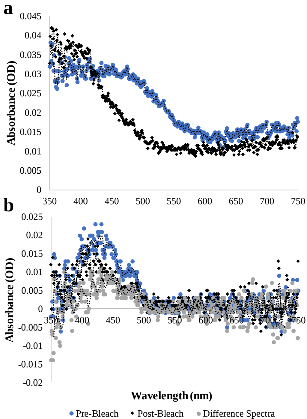
Figure L11. Pre- and Post-bleach absorbance spectra of the SWS single cone from the Golden ( a ) and Bald ( b ) Eagle. Grey spectrum shows the difference between the pre- and post-bleach spectra. Moving averages are shown with black dashed lines.
