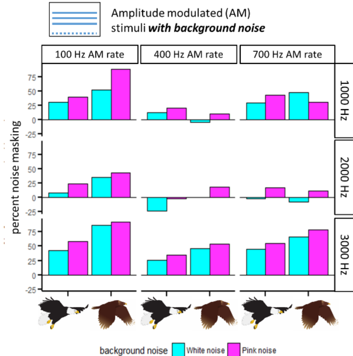
Figure K4. Most amplitude modulated (AM) stimuli are masked by background noise, and the responses of Golden and Bald Eagles are similar. The data above show the average effect of noise on the eagle's ability to hear all four components of the AM stimulus (carrier tone, high and low sideband tones, and the AM rate). The low effect of noise on several of the AM stimuli is promising, especially for 400 Hz AM with a 2000 Hz carrier, where phaselocking is strong (Figure K3) and noise masking is low. These are good candidates for stimuli to use in the field.
