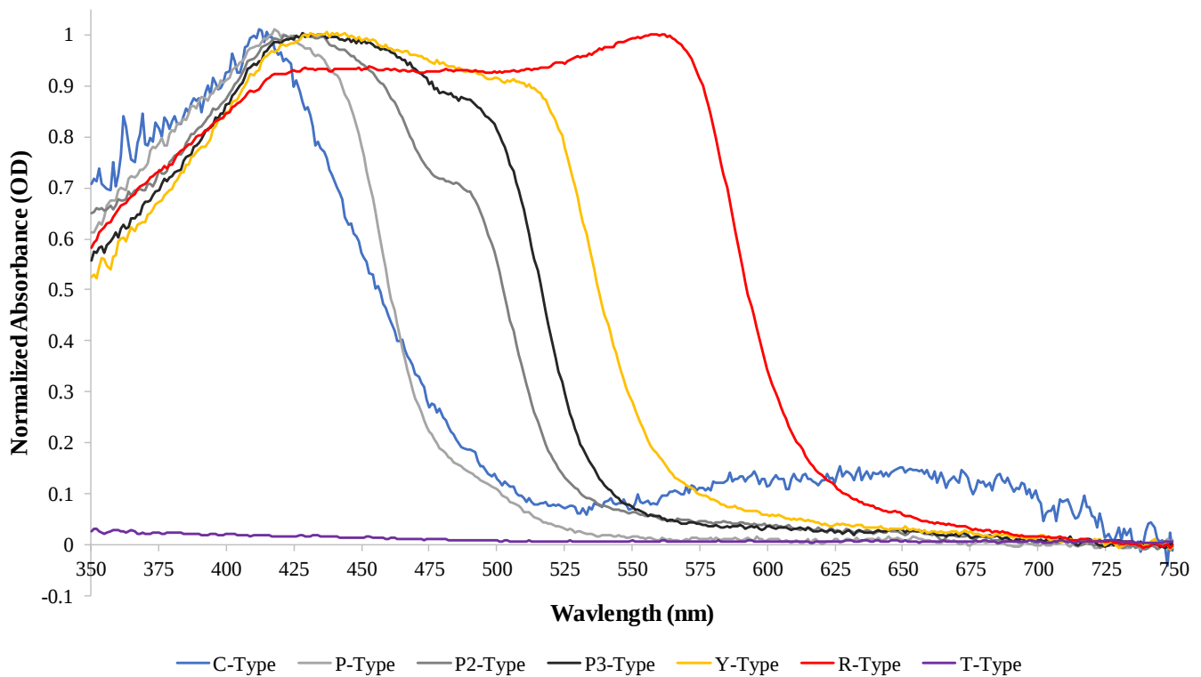
Figure L17. The average normalized oil droplet absorbance spectra from the Bald Eagle. The T-Type oil droplet (purple line) was not normalized for ease of viewing.
