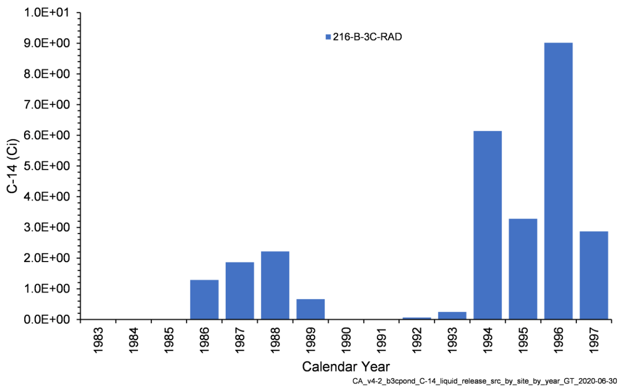
Figure 4-20. Annual C-14 Activity Released from Liquid Waste Sites in the B-3C Pond Model
