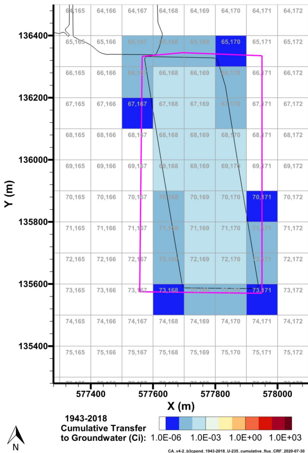
Figure 7-35. Cumulative U-235 Activity Discharged to Groundwater from the B-3C Pond Model from 1943–2018 per P2R Grid Cell
