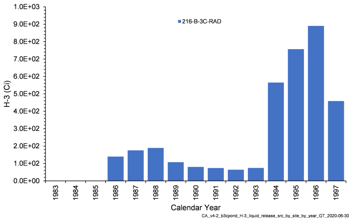
Figure 4-21. Annual H-3 Activity Released from Liquid Waste Sites in the B-3C Pond Model
