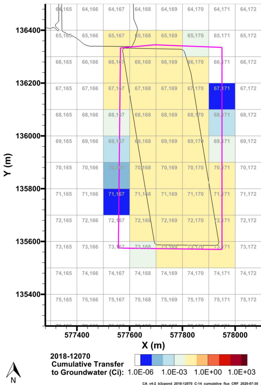
Figure 7-2. Cumulative C-14 Activity Discharged to Groundwater from the B-3C Pond Model from 2018–12070 per P2R Grid Cell
