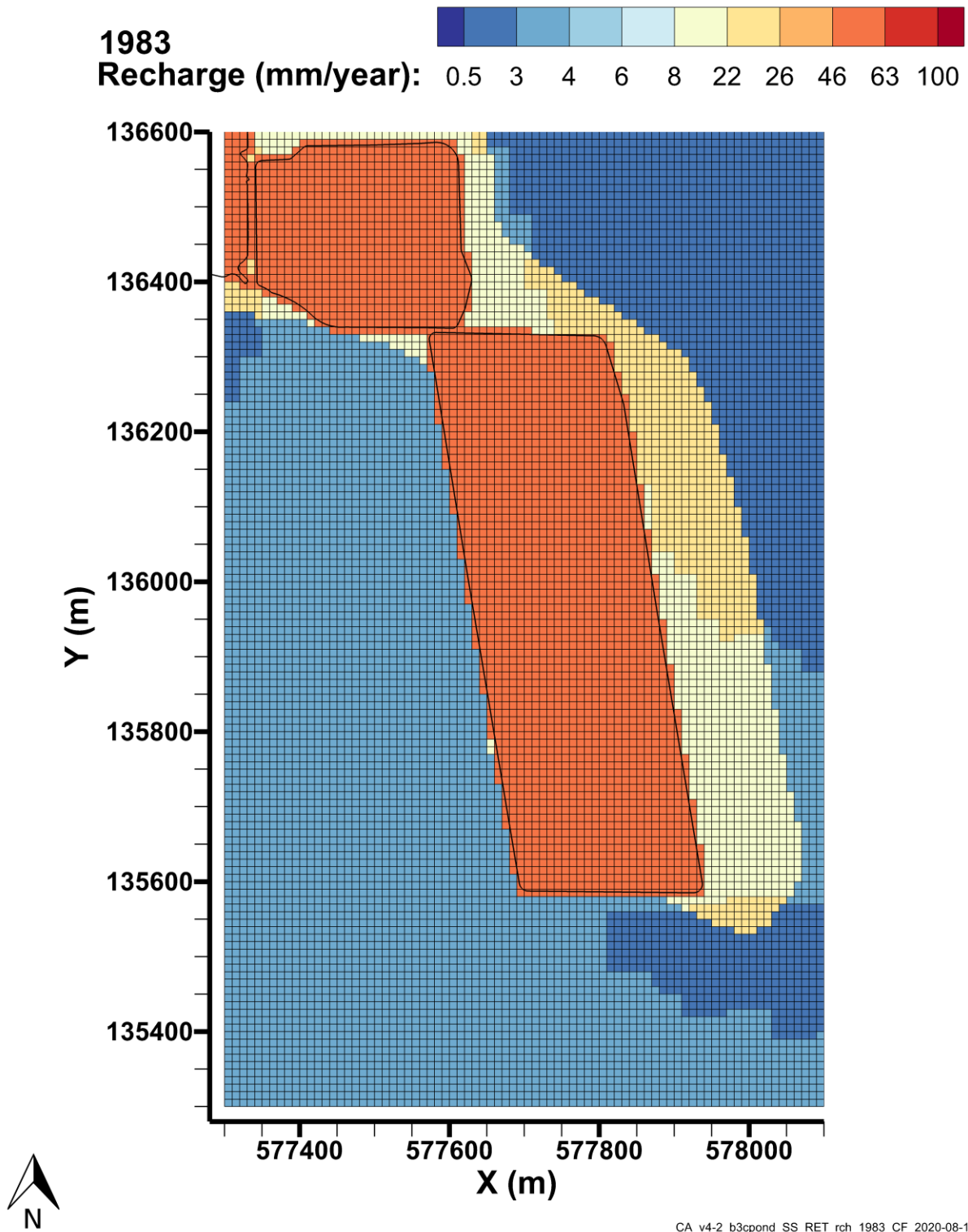
Figure 4-35. Transient Recharge Estimates for the B-3C Pond Model, 1983
