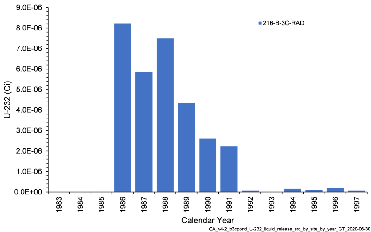
Figure 4-26. Annual U-232 Activity Released from Liquid Waste Sites in the B-3C Pond Model
