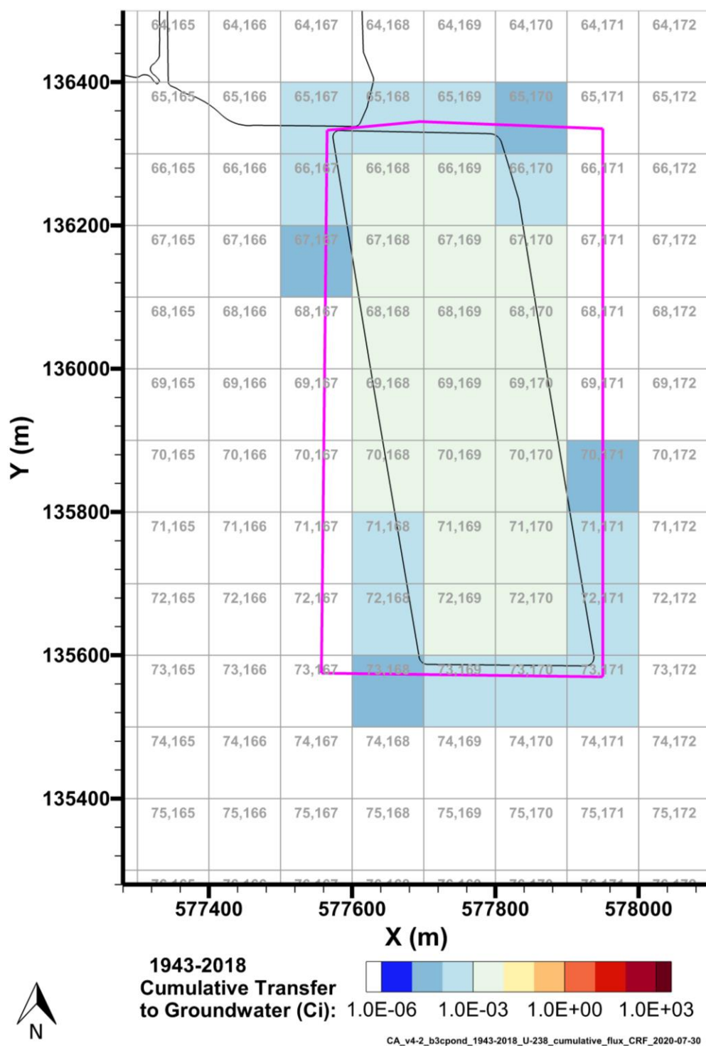
Figure 7-43. Cumulative U-238 Activity Discharged to Groundwater from the B-3C Pond Model from 1943–2018 per P2R Grid Cell
