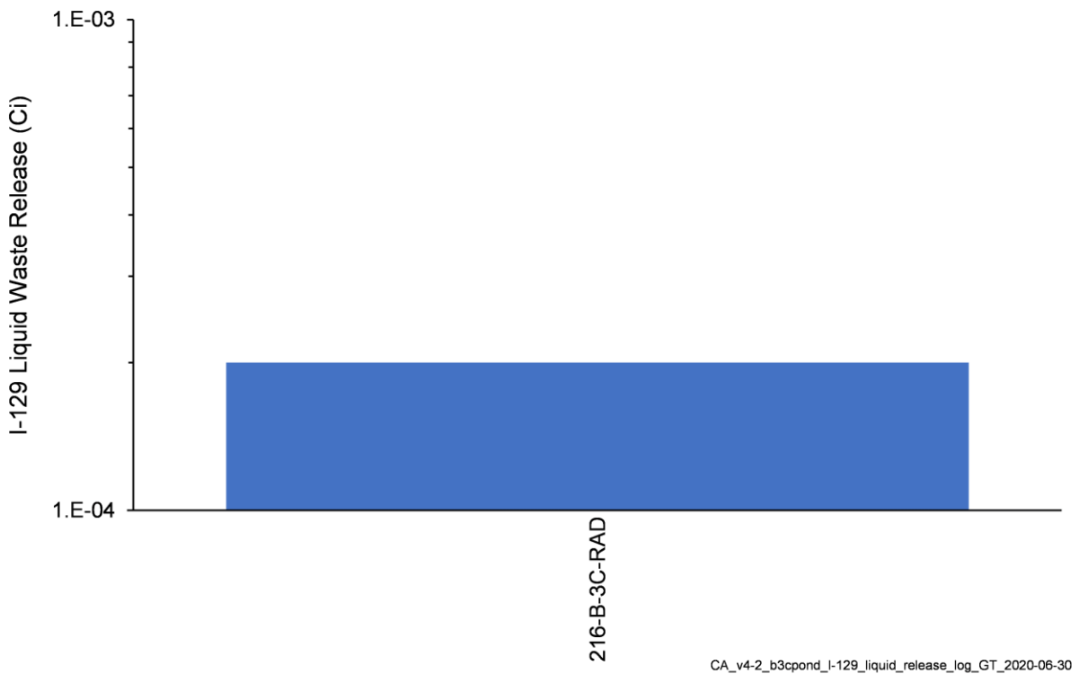
Figure 4-10. Total I-129 Activity Released from Liquid Waste Sites in the B-3C Pond Model
