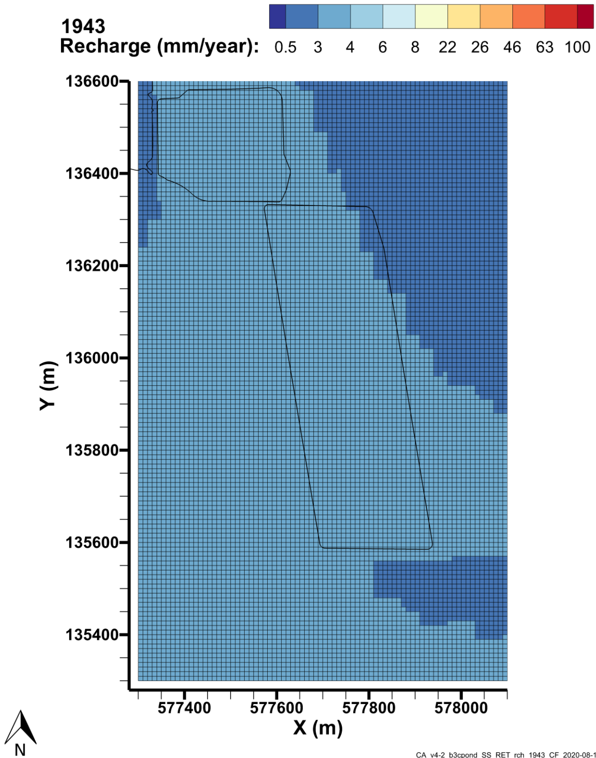
Figure 4-34. Transient Recharge Estimates for the B-3C Pond Model, 1943
