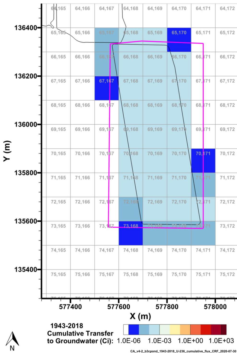
Figure 7-39. Cumulative U-236 Activity Discharged to Groundwater from the B-3C Pond Model from 1943–2018 per P2R Grid Cell
