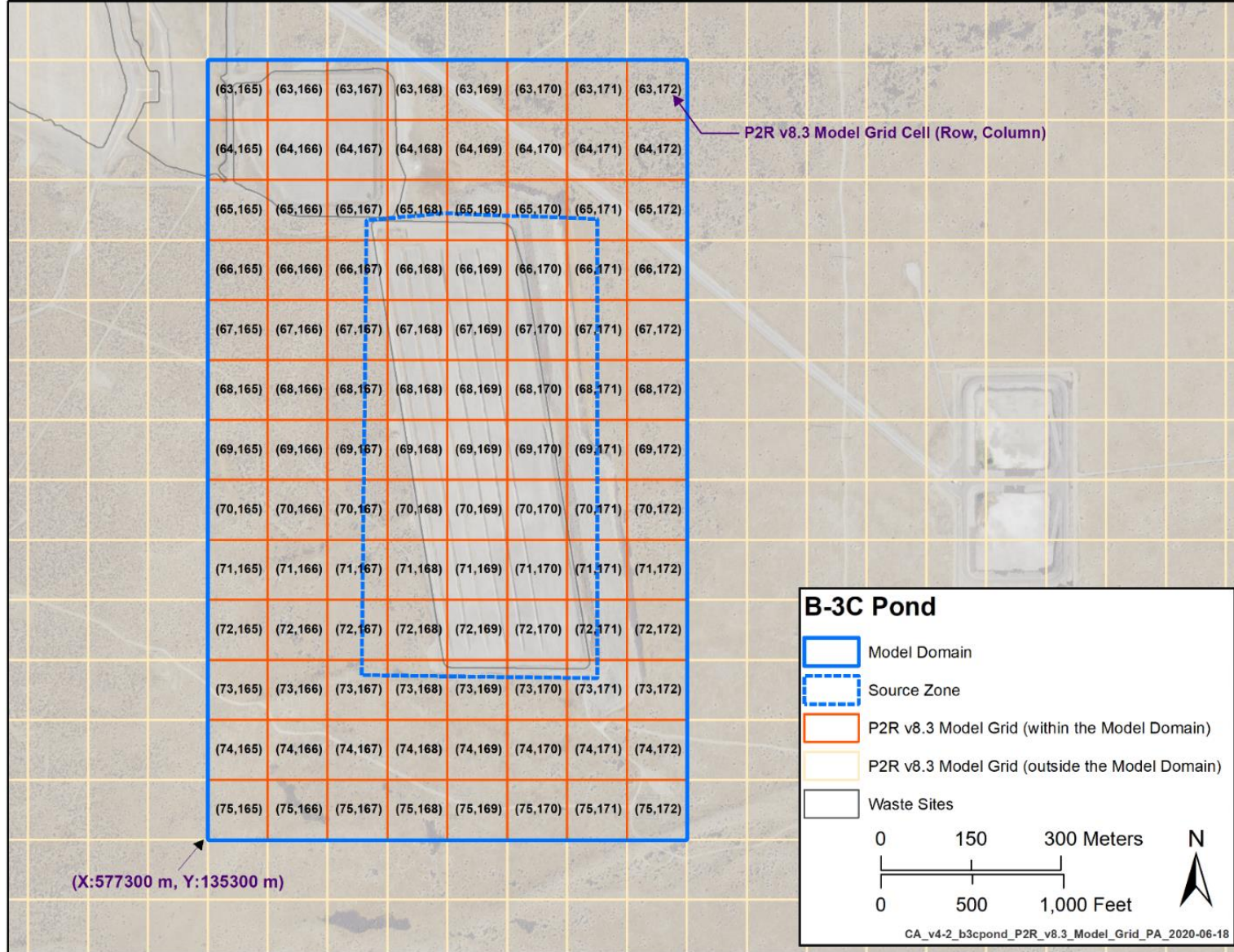
Figure 4-2. Plan View of the P2R Grid Cells in the B-3C Pond Model
