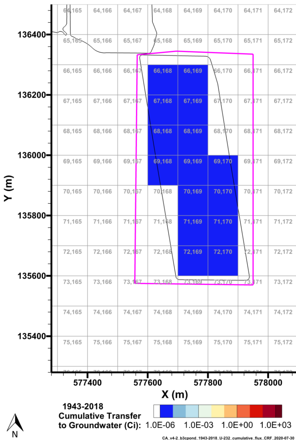
Figure 7-26. Cumulative U-232 Activity Discharged to Groundwater from the B-3C Pond Model from 1943–2018 per P2R Grid Cell
