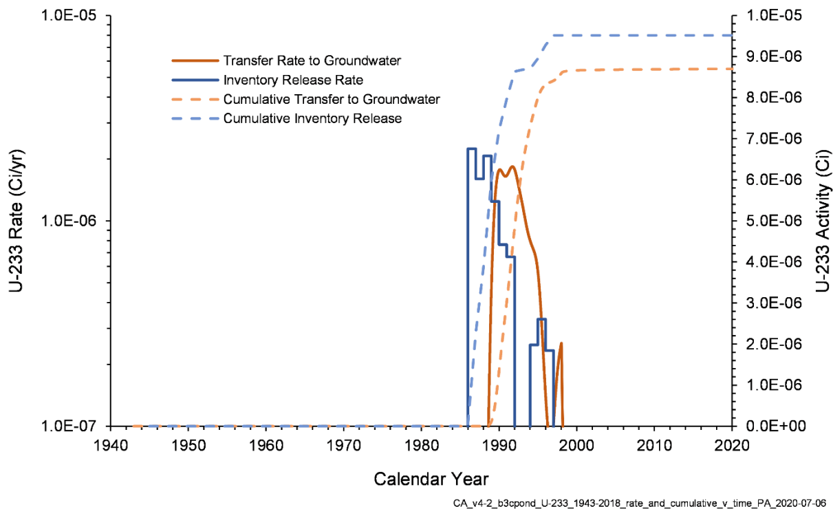
Figure 7-29. U-233 Inventory Release from Waste Sites and Transfer to Groundwater for the B-3C Pond Model from 1943–2018
