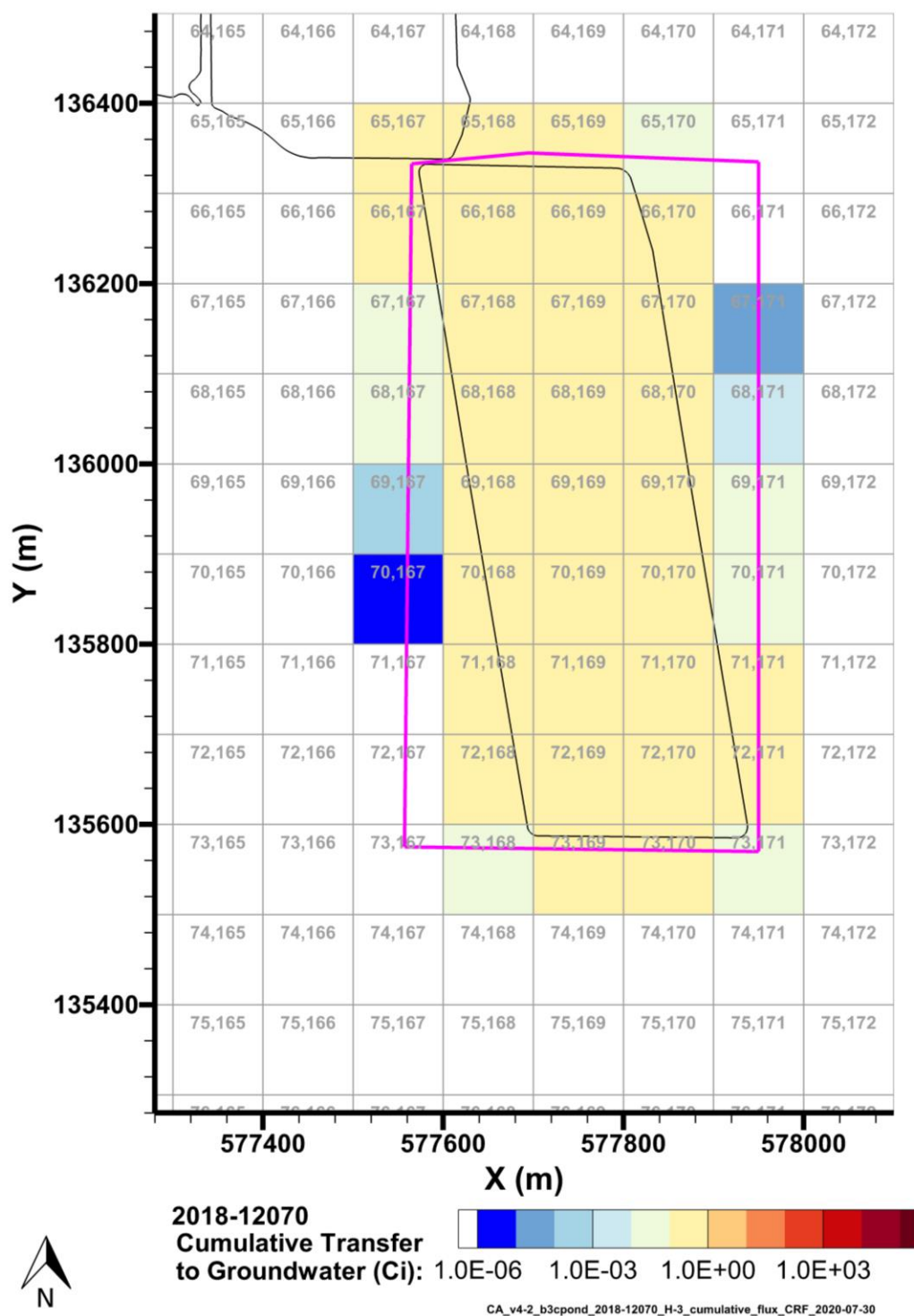
Figure 7-6. Cumulative H-3 Activity Discharged to Groundwater from the B-3C Pond Model from 2018–12070 per P2R Grid Cell
