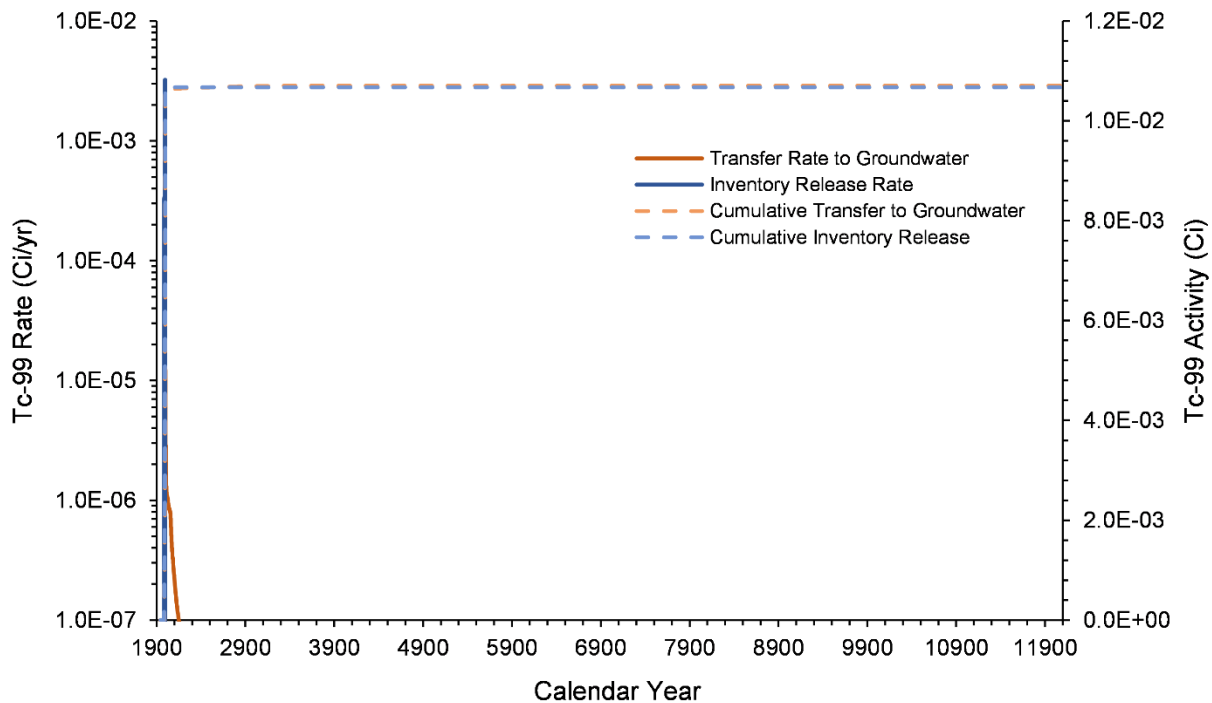
Figure 7-25. Tc-99 Inventory Release from Waste Sites and Transfer to Groundwater for the B-3C Pond Model from 1943–12070
