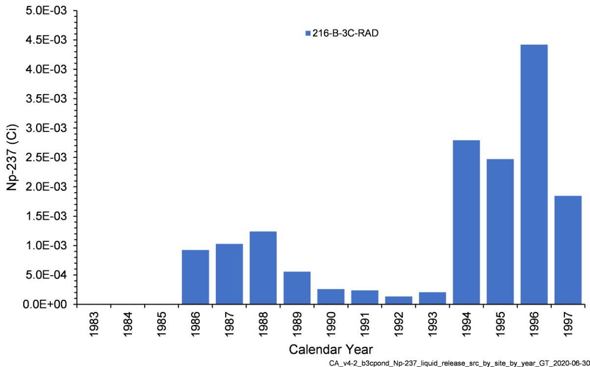
Figure 4-23. Annual Np-237 Activity Released from Liquid Waste Sites in the B-3C Pond Model
