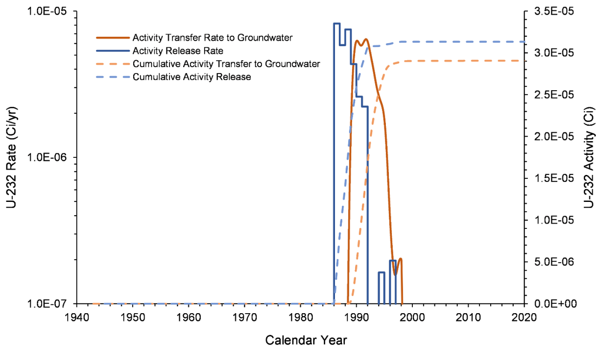
Figure 7-27. U-232 Inventory Release from Waste Sites and Transfer to Groundwater for the B-3C Pond Model from 1943–2018
