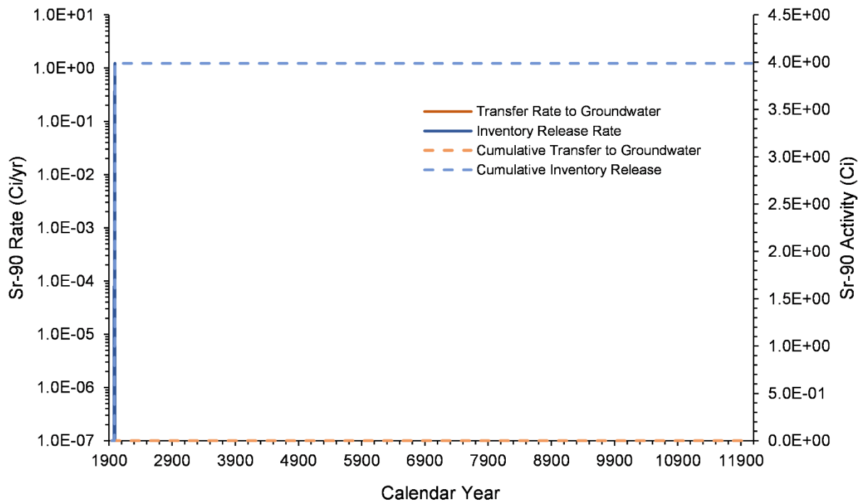
Figure 7-21. Sr-90 Inventory Release from Waste Sites and Transfer to Groundwater for the B-3C Pond Model from 1943–12070
