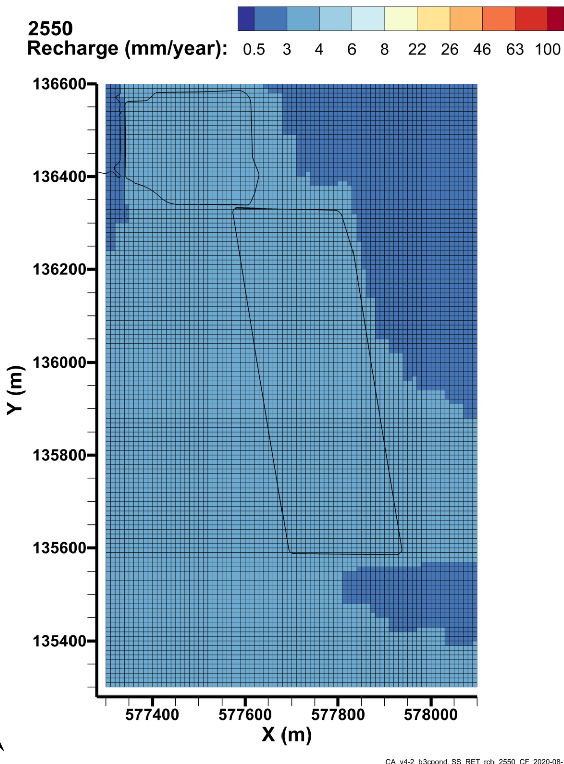
Figure 4-37. Transient Recharge Estimates for the B-3C Pond Model, 2550
