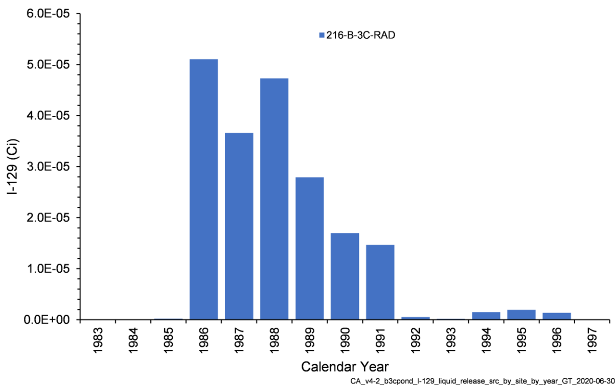
Figure 4-22. Annual I-129 Activity Released from Liquid Waste Sites in the B-3C Pond Model
