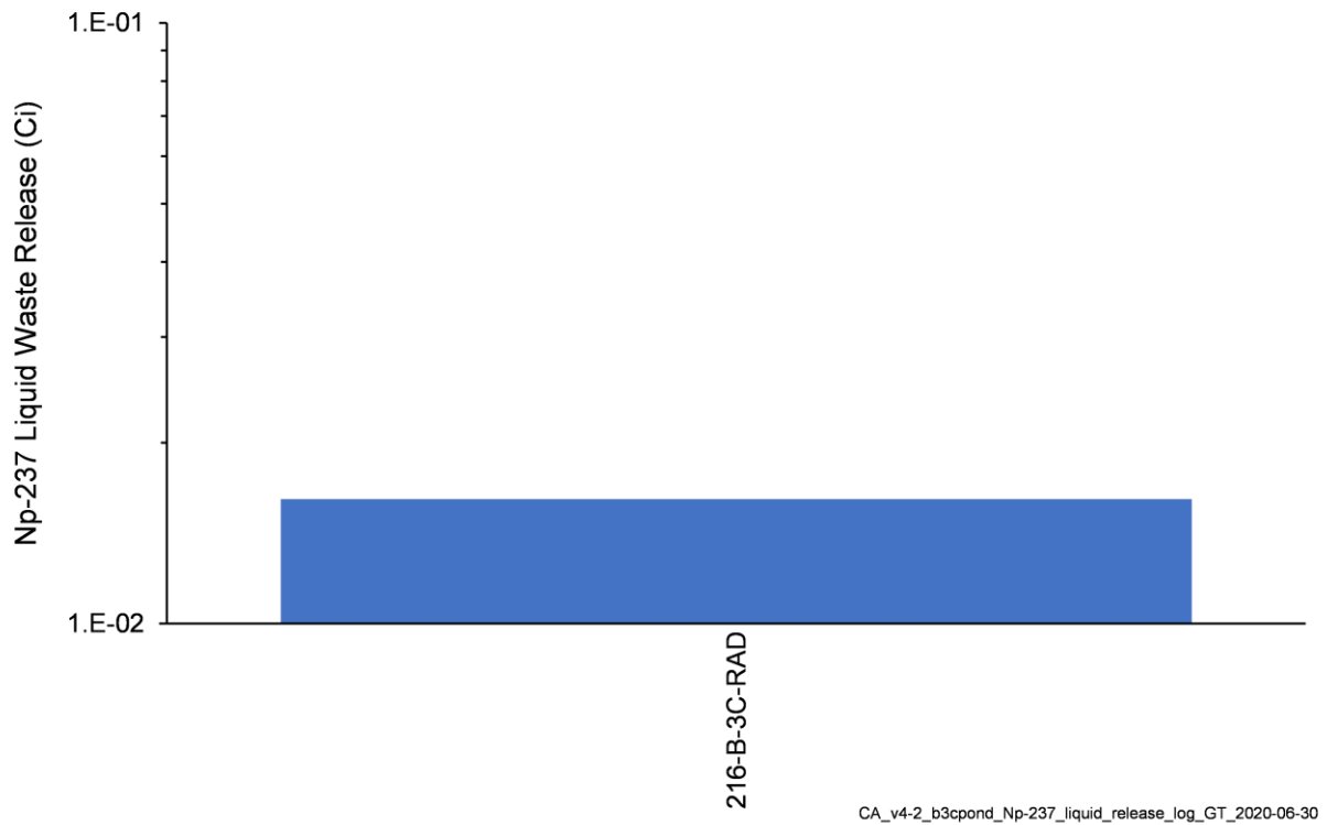
Figure 4-11. Total Np-237 Activity Released from Liquid Waste Sites in the B-3C Pond Model
