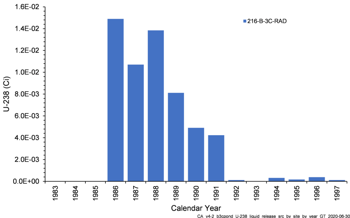
Figure 4-31. Annual U-238 Activity Released from Liquid Waste Sites in the B-3C Pond Model
