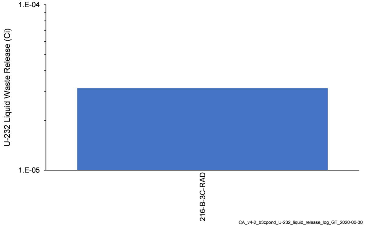
Figure 4-14. Total U-232 Activity Released from Liquid Waste Sites in the B-3C Pond Model
