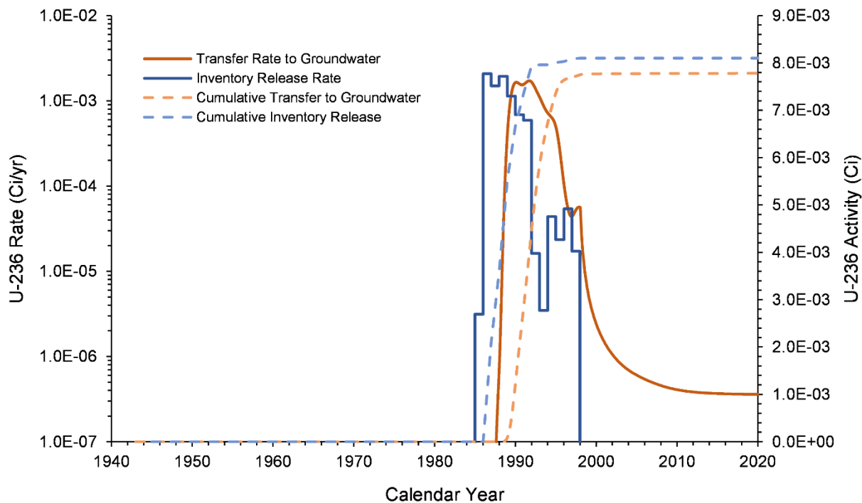
Figure 7-41. U-236 Inventory Release from Waste Sites and Transfer to Groundwater for the B-3C Pond Model from 1943–2018
