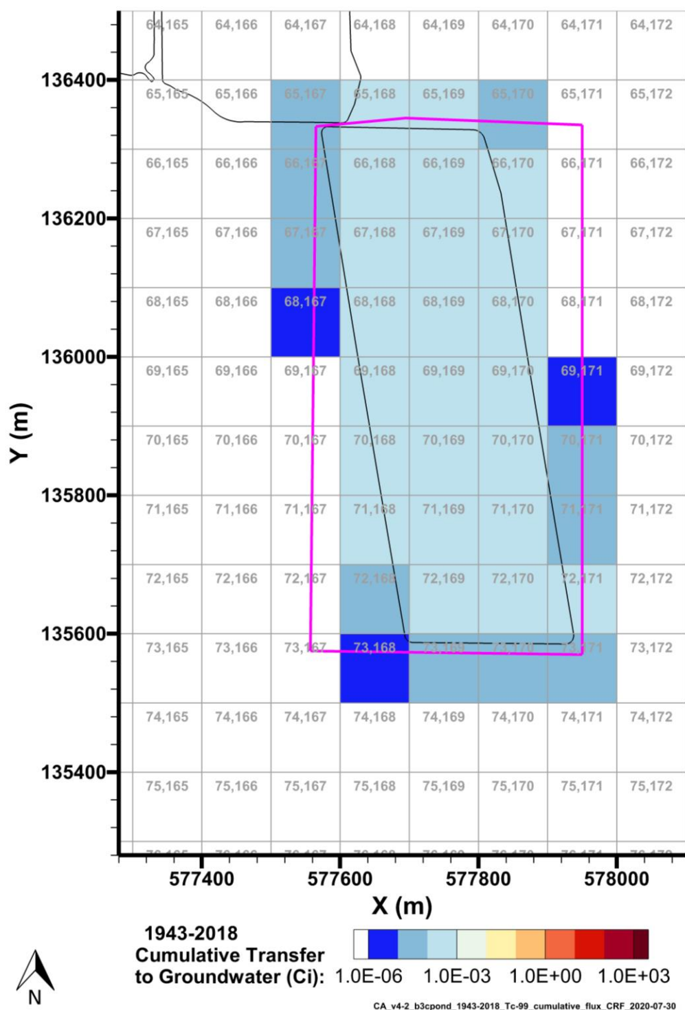
Figure 7-22. Cumulative Tc-99 Activity Discharged to Groundwater from the B-3C Pond Model from 1943–2018 per P2R Grid Cell
