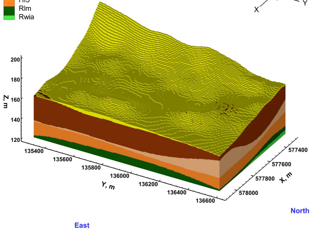
Figure 4-3. Model Hydrostratigraphy Three-Dimensional View Showing the North and East Faces
