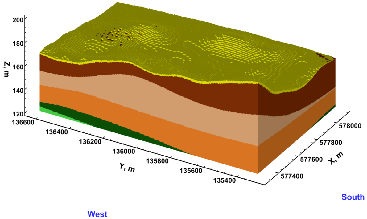
Figure 4-5. Model Hydrostratigraphy Three-Dimensional View Showing the South and West Faces
