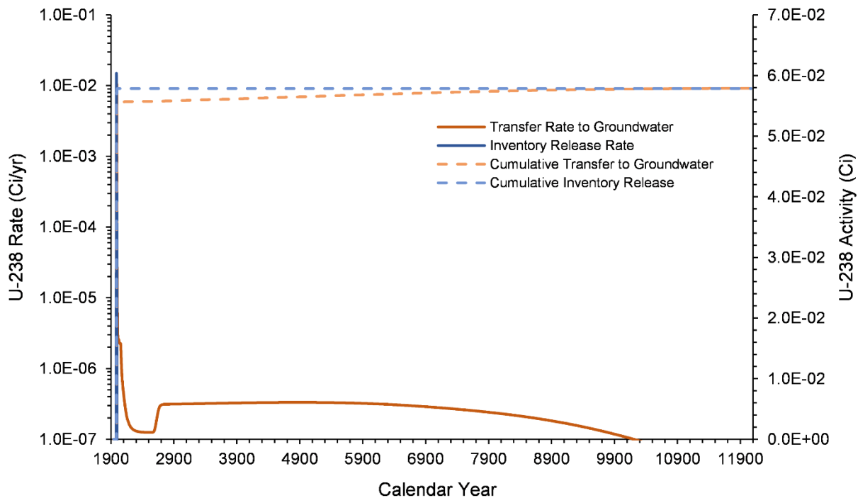
Figure 7-46. U-238 Inventory Release from Waste Sites and Transfer to Groundwater for the B-3C Pond Model from 1943–12070
