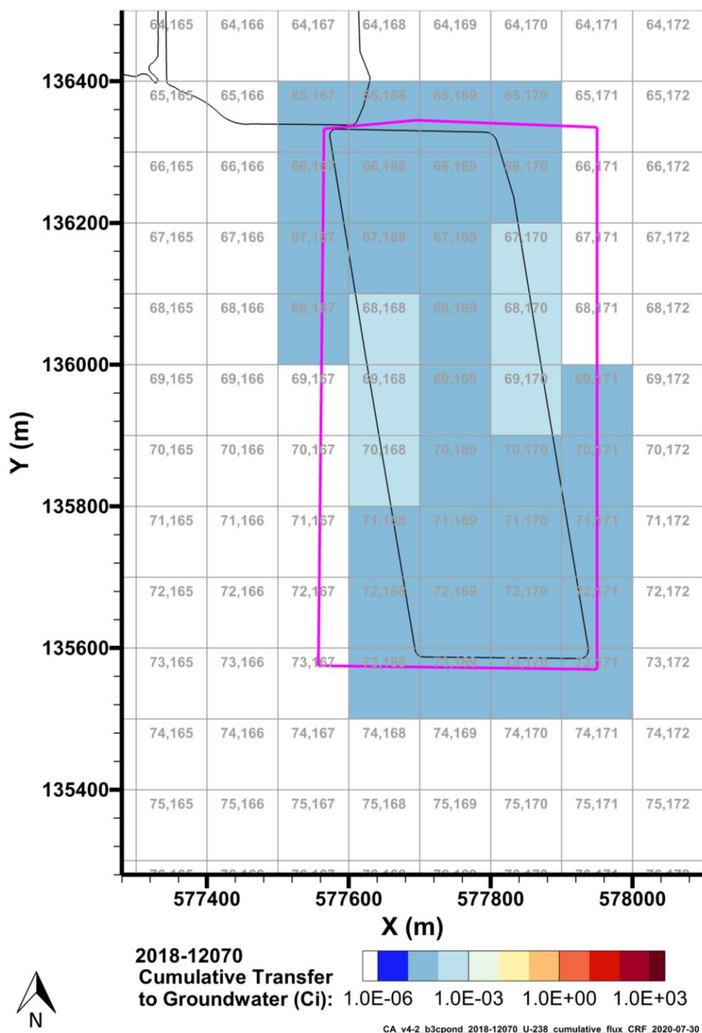
Figure 7-44. Cumulative U-238 Activity Discharged to Groundwater from the B-3C Pond Model from 2018–12070 per P2R Grid Cell
