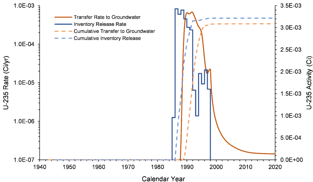
Figure 7-37. U-235 Inventory Release from Waste Sites and Transfer to Groundwater for the B-3C Pond Model from 1943–2018
