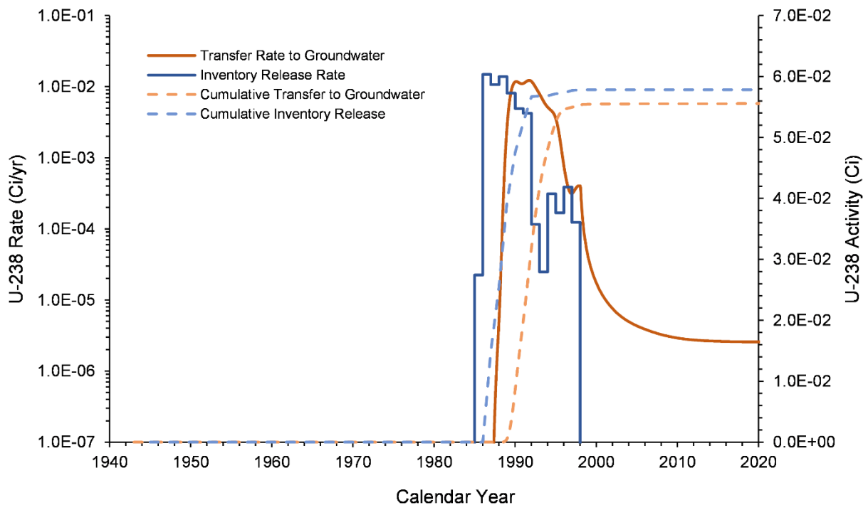
Figure 7-45. U-238 Inventory Release from Waste Sites and Transfer to Groundwater for the B-3C Pond Model from 1943–2018
