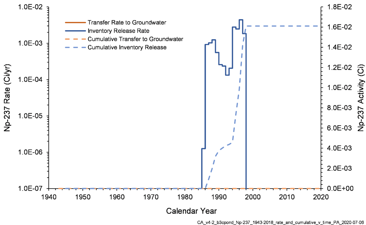
Figure 7-18. Np-237 Inventory Release from Waste Sites and Transfer to Groundwater for the B-3C Pond Model from 1943–2018
