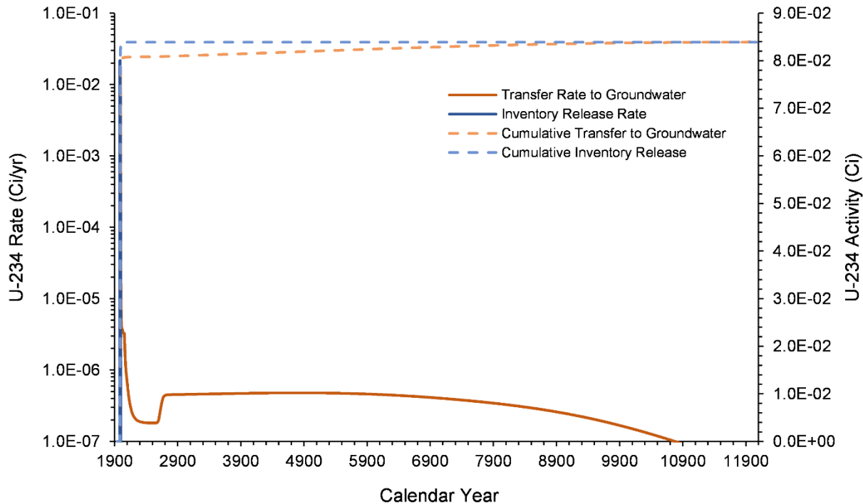
Figure 7-34. U-234 Inventory Release from Waste Sites and Transfer to Groundwater for the B-3C Pond Model from 1943–12070
