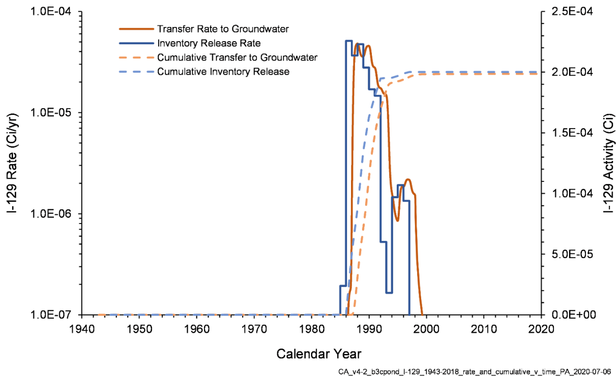
Figure 7-16. I-129 Inventory Release from Waste Sites and Transfer to Groundwater for the B-3C Pond Model from 1943–2018
