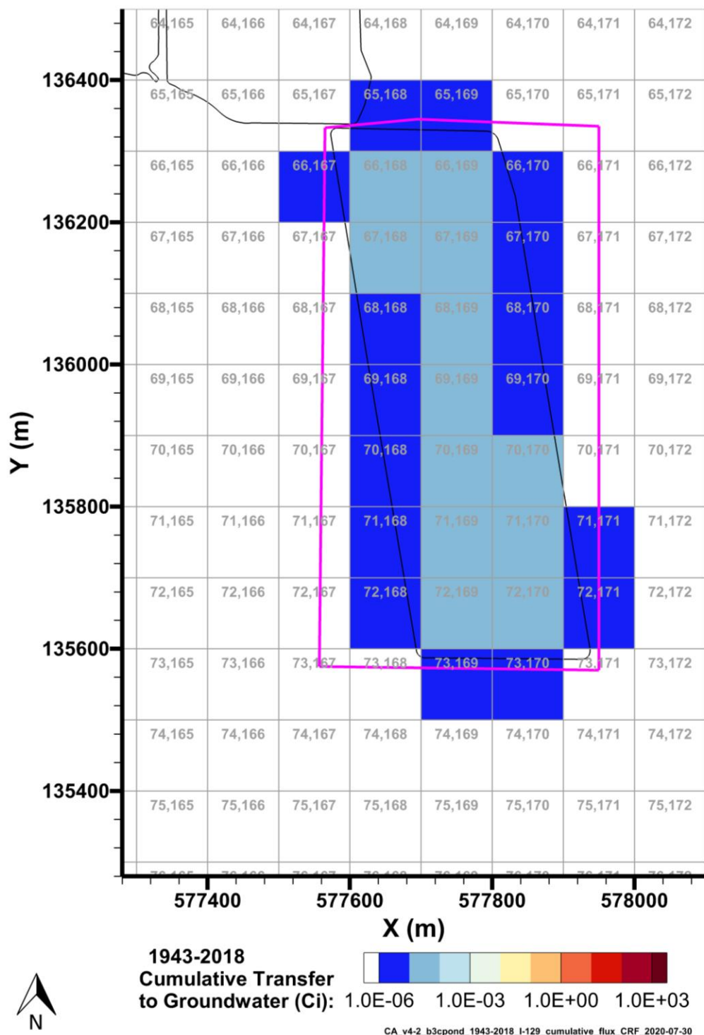
Figure 7-15. Cumulative I-129 Activity Discharged to Groundwater from the B-3C Pond Model from 1943–2018 per P2R Grid Cell
