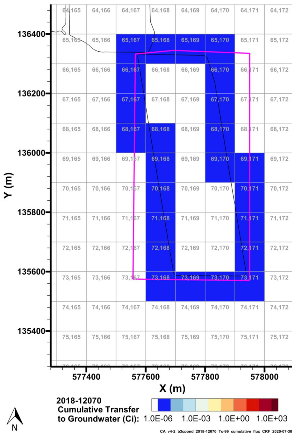
Figure 7-23. Cumulative Tc-99 Activity Discharged to Groundwater from the B-3C Pond Model from 2018–12070 per P2R Grid Cell
