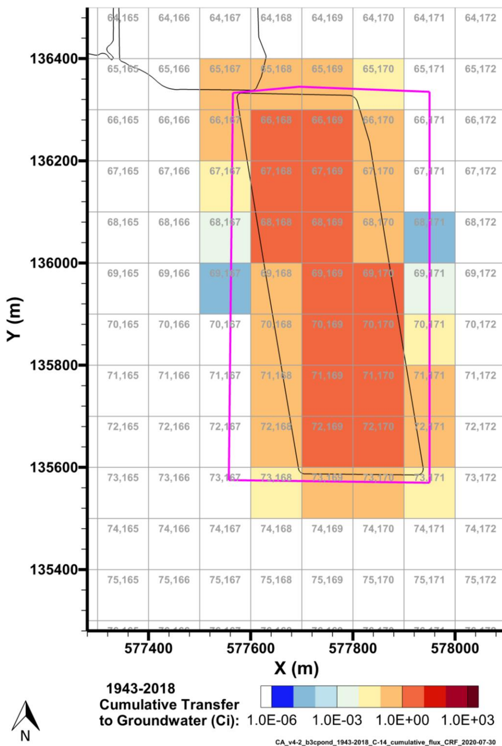
Figure 7-1. Cumulative C-14 Activity Discharged to Groundwater from the B-3C Pond Model from 1943–2018 per P2R Grid Cell
