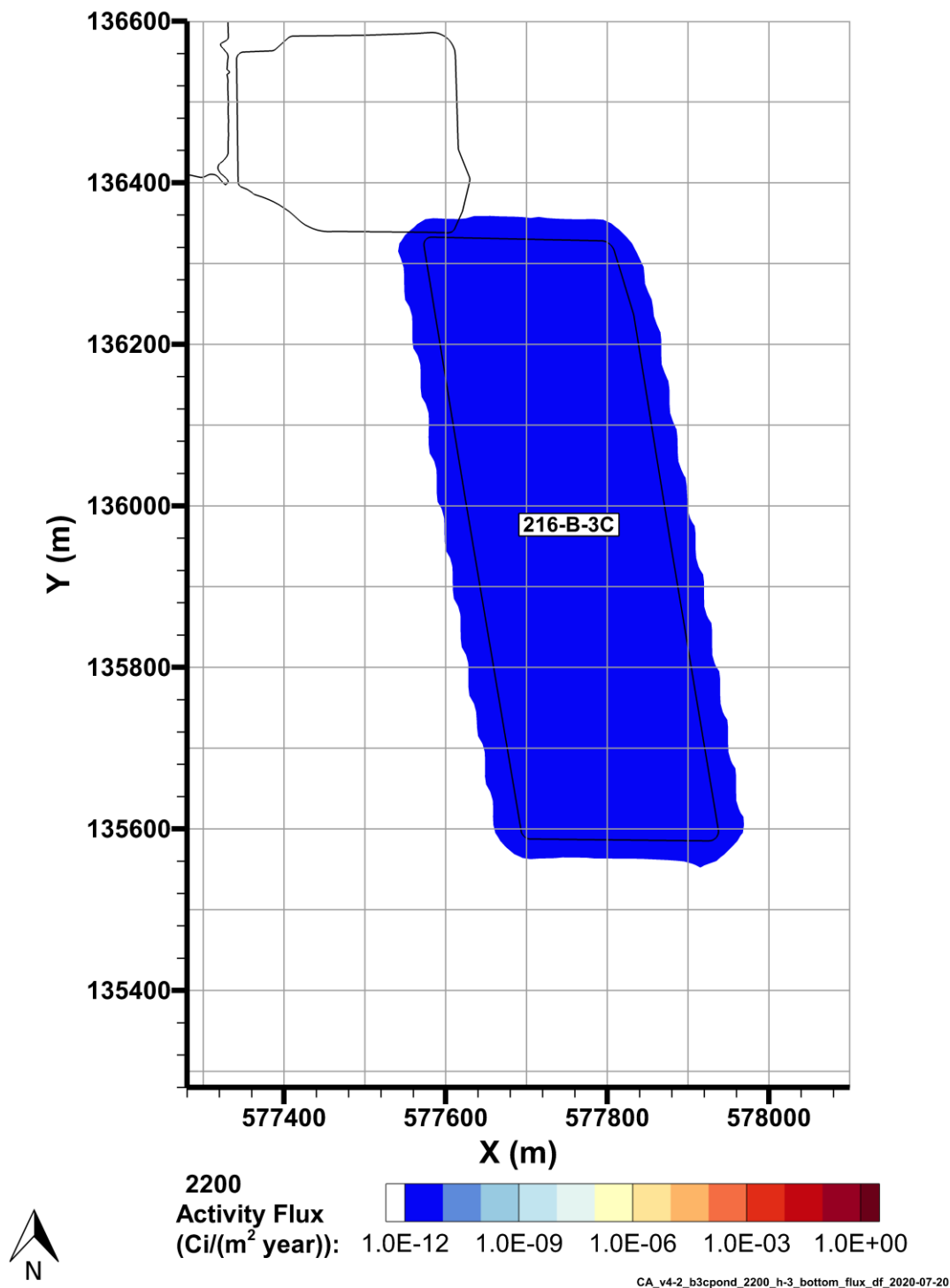
Figure 7-13. H-3 Flux to Groundwater, 2200
