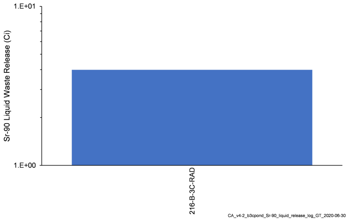
Figure 4-12. Total Sr-90 Activity Released from Liquid Waste Sites in the B-3C Pond Model
