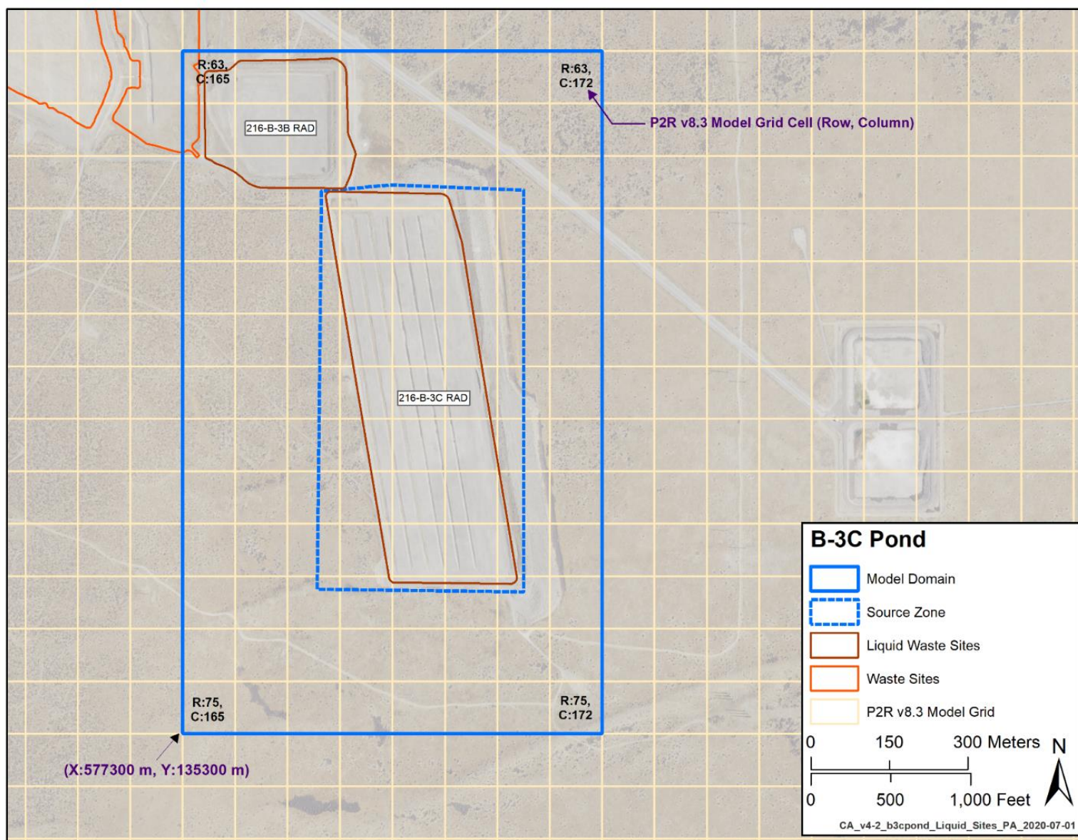
Figure 4-7. Waste Sites in the B-3C Pond Model with Liquid Source Inventory
