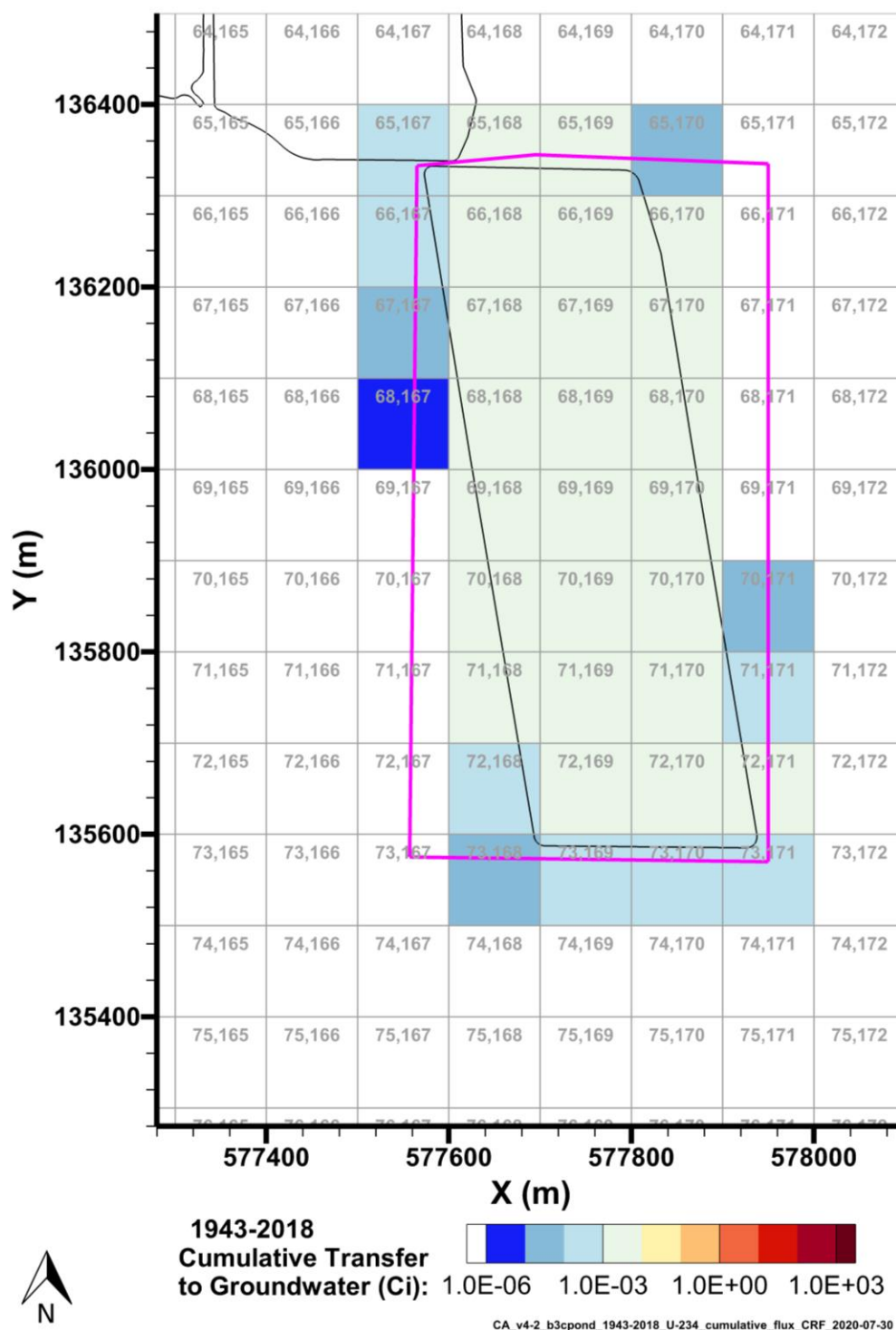
Figure 7-31. Cumulative U-234 Activity Discharged to Groundwater from the B-3C Pond Model from 1943–2018 per P2R Grid Cell
