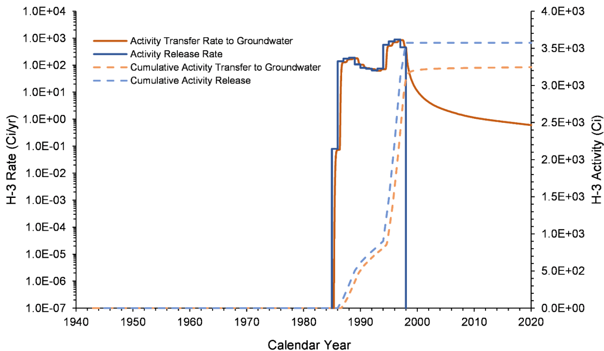
Figure 7-7. H-3 Inventory Release from Waste Sites and Transfer to Groundwater for the B-3C Pond Model from 1943–2018
