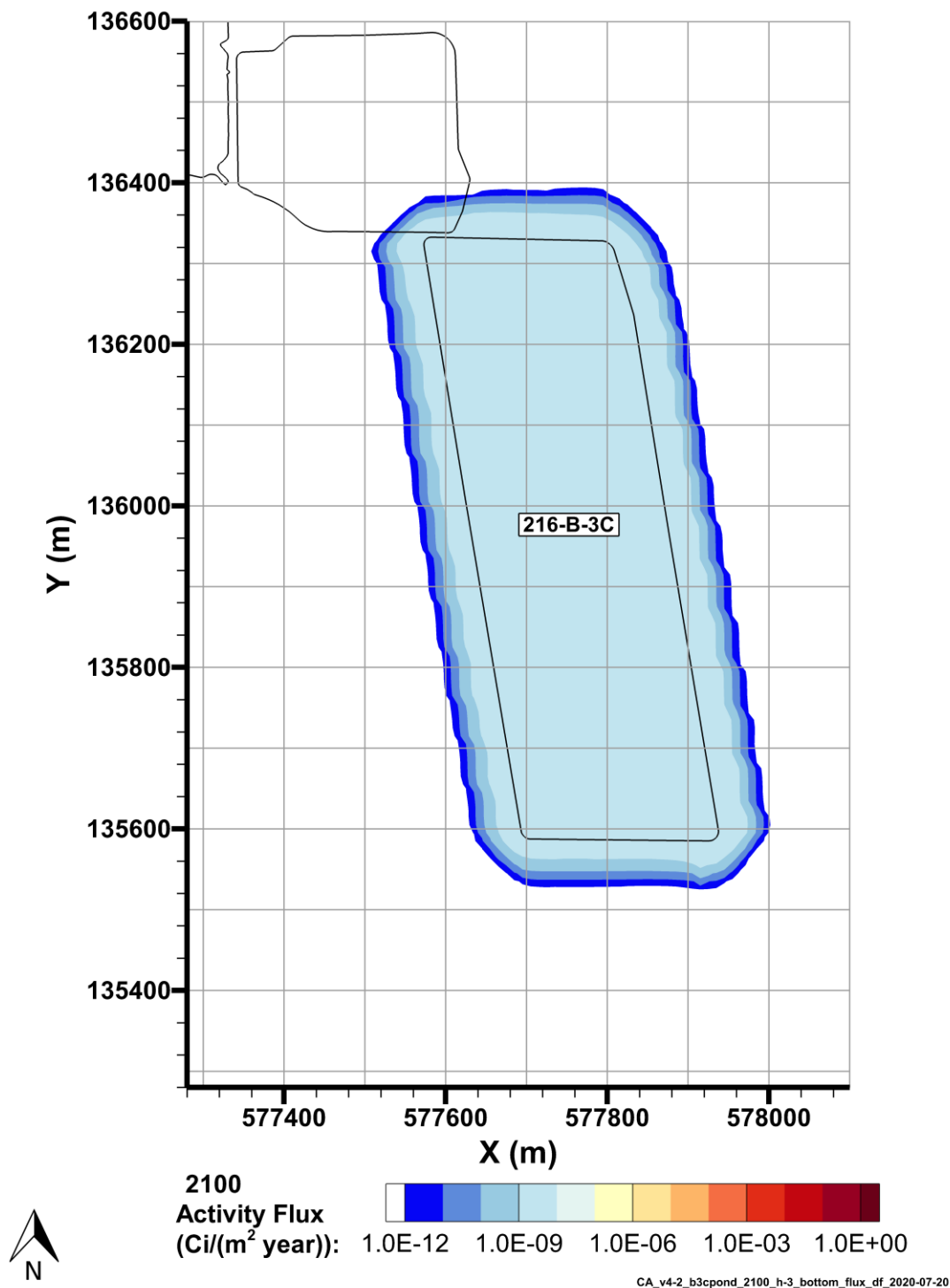
Figure 7-12. H-3 Flux to Groundwater, 2100
