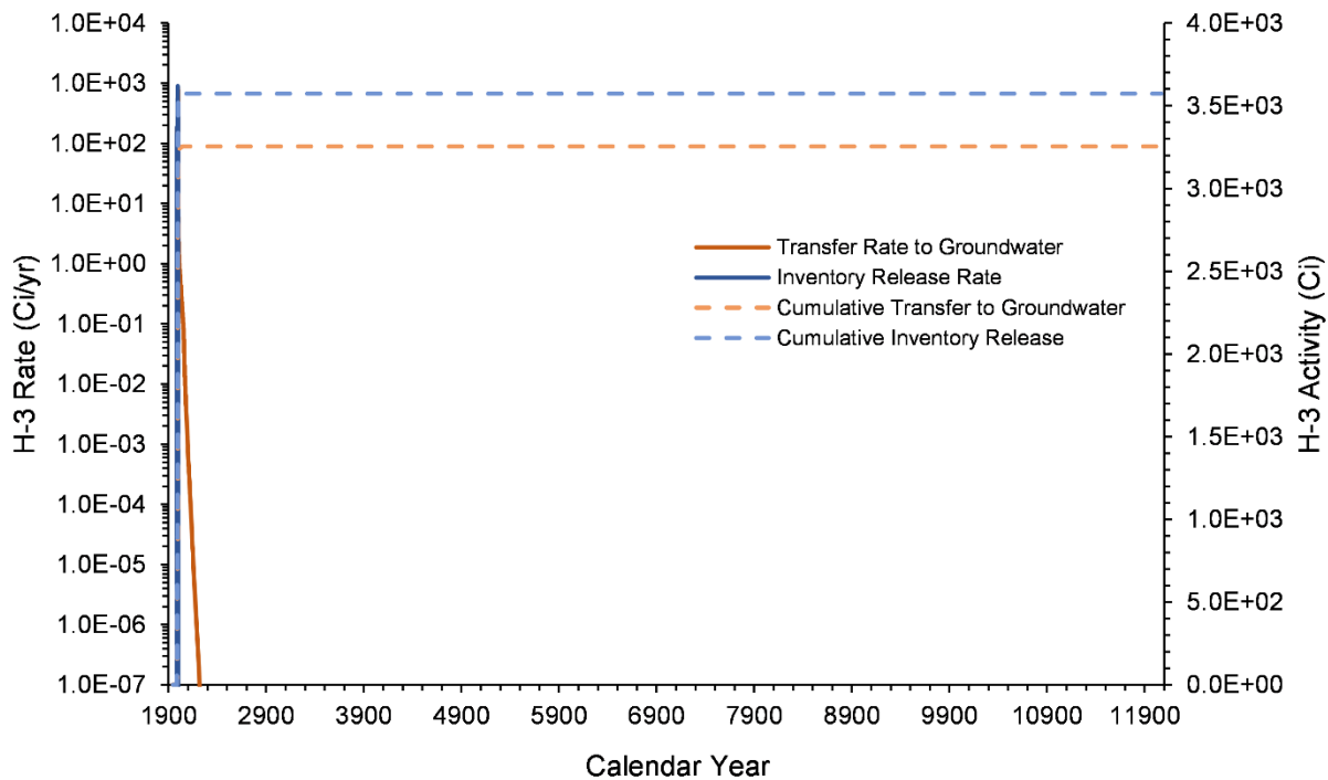
Figure 7-8. H-3 Inventory Release from Waste Sites and Transfer to Groundwater for the B-3C Pond Model from 1943–12070
