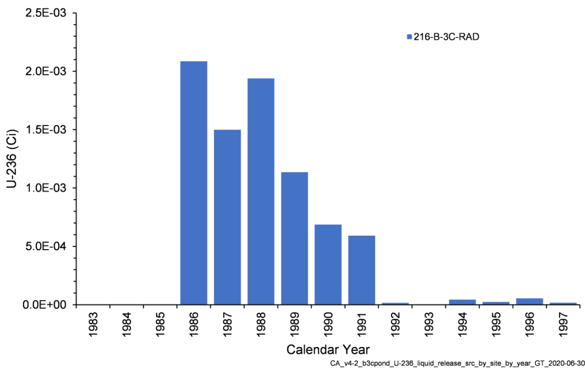
Figure 4-30. Annual U-236 Activity Released from Liquid Waste Sites in the B-3C Pond Model
