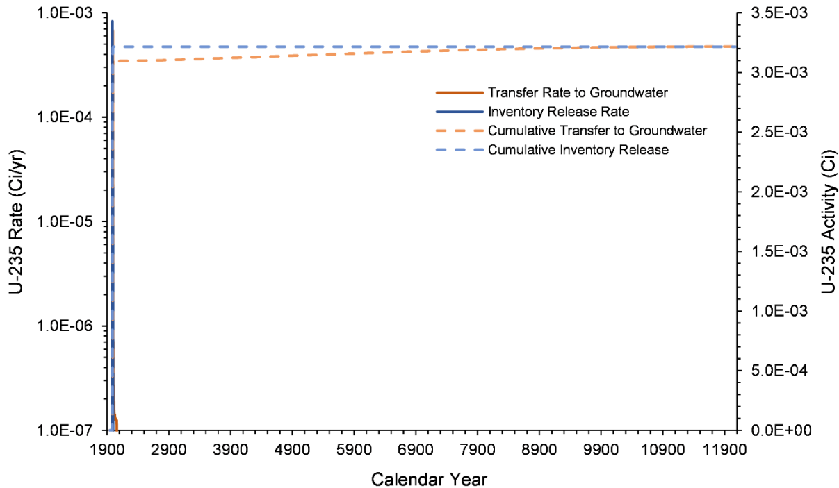
Figure 7-38. U-235 Inventory Release from Waste Sites and Transfer to Groundwater for the B-3C Pond Model from 1943–12070
