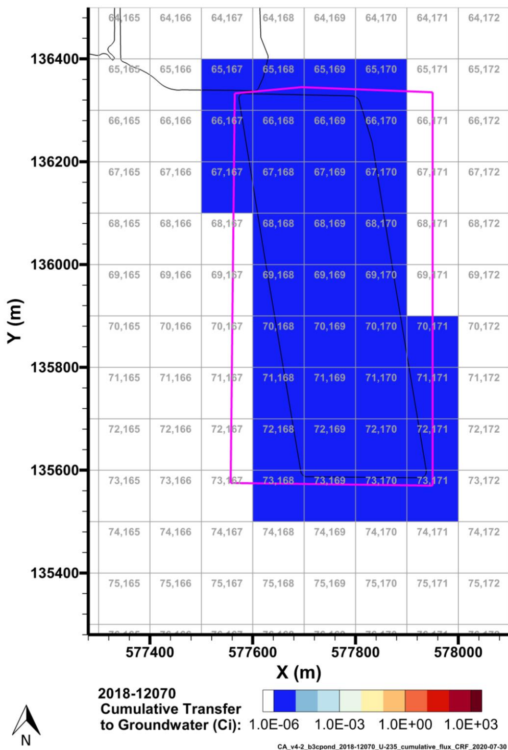
Figure 7-36. Cumulative U-235 Activity Discharged to Groundwater from the B-3C Pond Model from 2018–12070 per P2R Grid Cell
