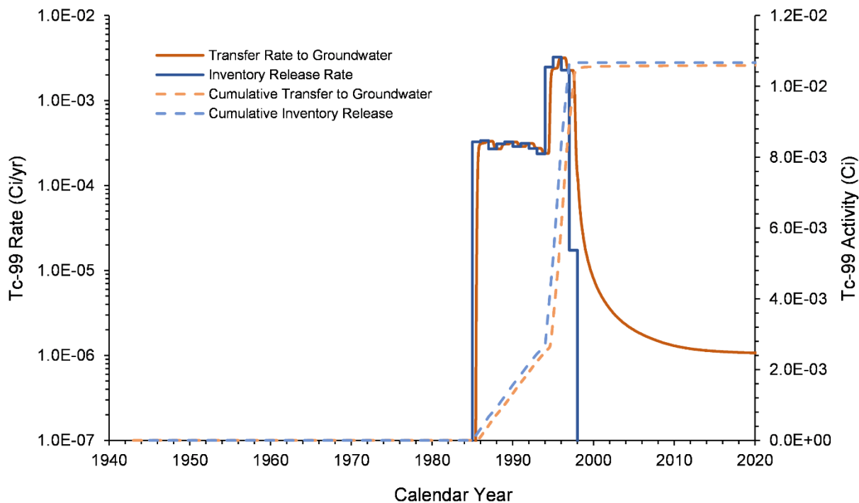
Figure 7-24. Tc-99 Inventory Release from Waste Sites and Transfer to Groundwater for the B-3C Pond Model from 1943–2018
