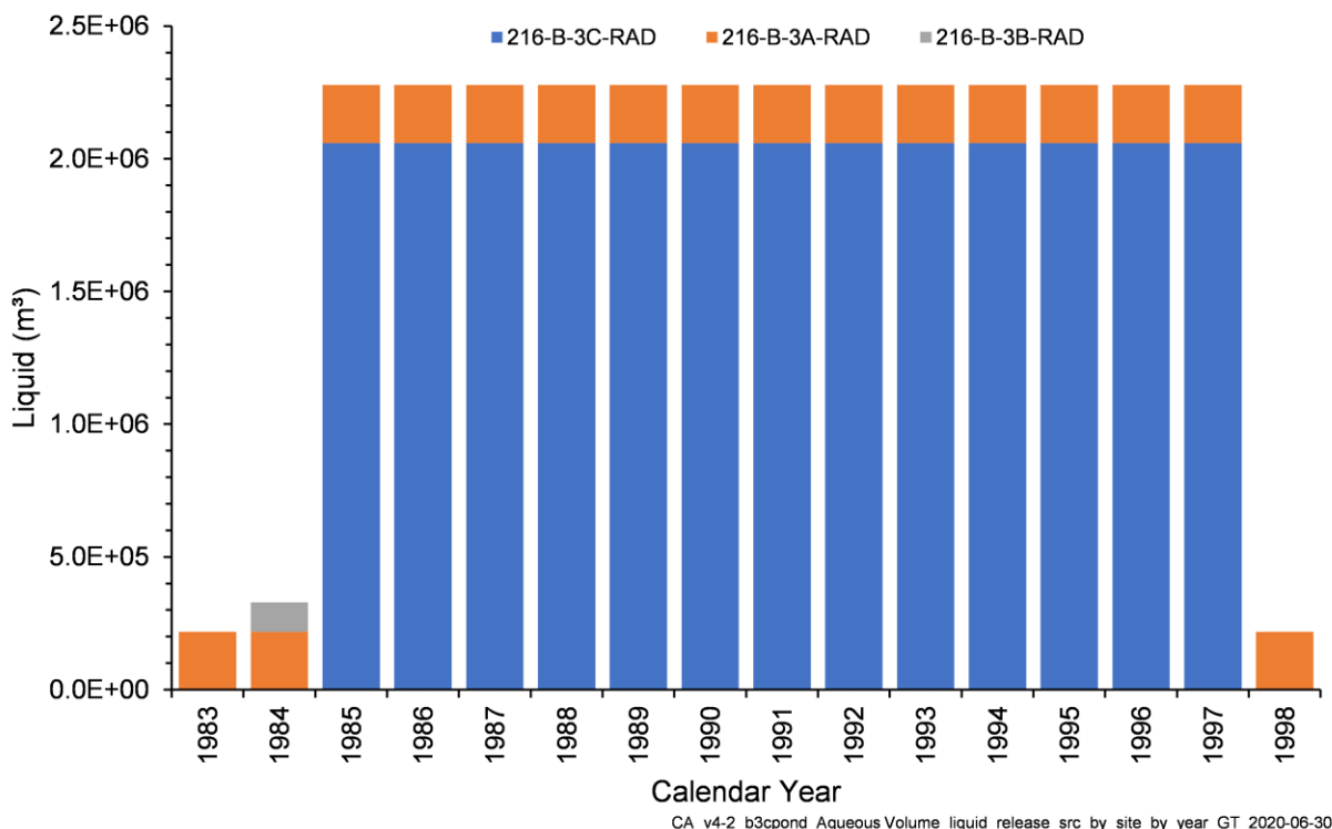
Figure 4-33. Total Volume of Water Released by Year from Liquid Waste Sites in the B-3C Pond Model
