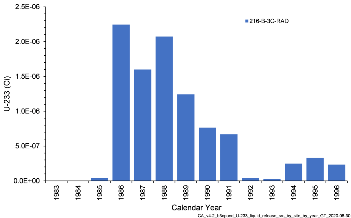
Figure 4-27. Annual U-233 Activity Released from Liquid Waste Sites in the B-3C Pond Model
