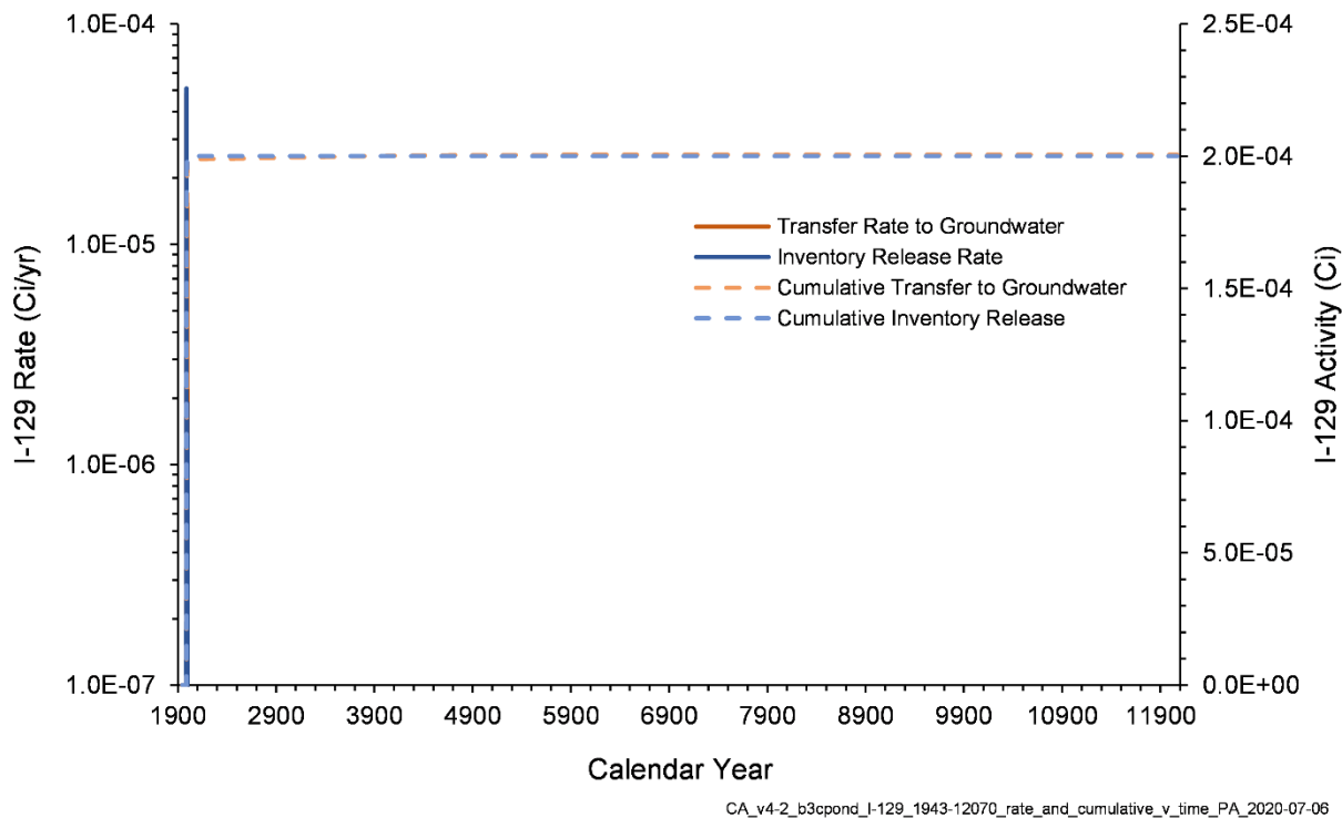
Figure 7-17. I-129 Inventory Release from Waste Sites and Transfer to Groundwater for the B-3C Pond Model from 1943–12070
