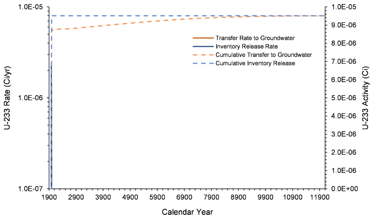
Figure 7-30. U-233 Inventory Release from Waste Sites and Transfer to Groundwater for the B-3C Pond Model from 1943–12070
