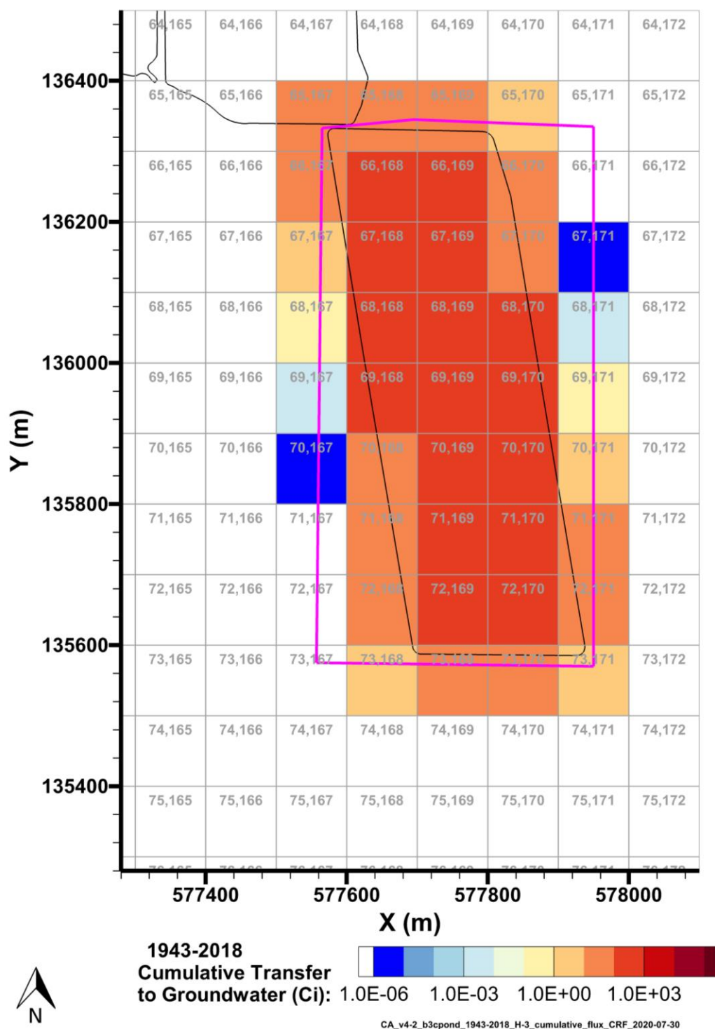
Figure 7-5. Cumulative H-3 Activity Discharged to Groundwater from the B-3C Pond Model from 1943–2018 per P2R Grid Cell
