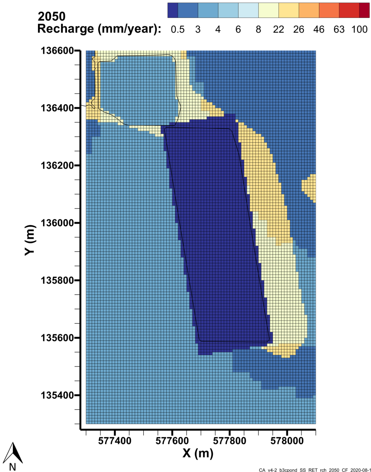
Figure 4-36. Transient Recharge Estimates for the B-3C Pond Model, 2050
