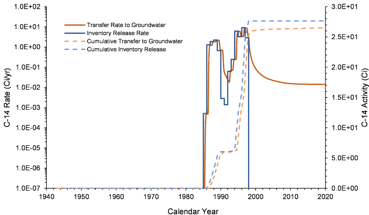
Figure 7-3. C-14 Inventory Release from Waste Sites and Transfer to Groundwater for the B-3C Pond Model from 1943–2018
