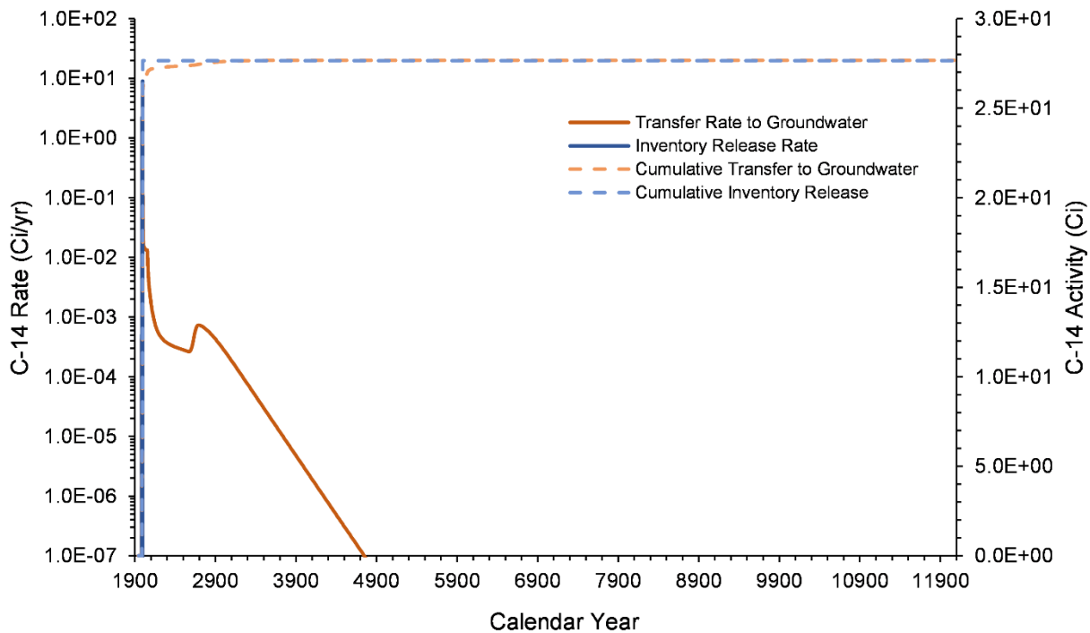
Figure 7-4. C-14 Inventory Release from Waste Sites and Transfer to Groundwater for the B-3C Pond Model from 1943–12070
