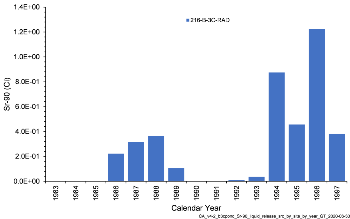
Figure 4-24. Annual Sr-90 Activity Released from Liquid Waste Sites in the B-3C Pond Model
