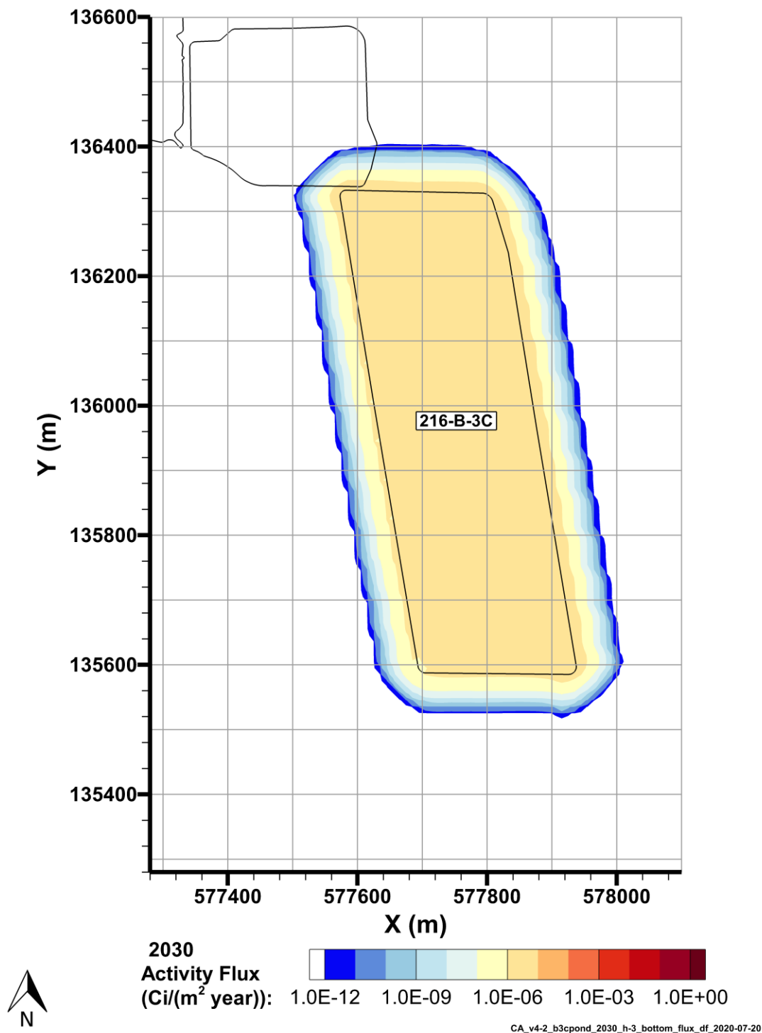
Figure 7-11. H-3 Flux to Groundwater, 2030
