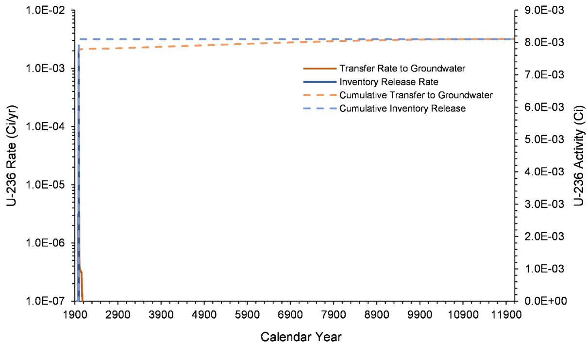
Figure 7-42. U-236 Inventory Release from Waste Sites and Transfer to Groundwater for the B-3C Pond Model from 1943–12070
