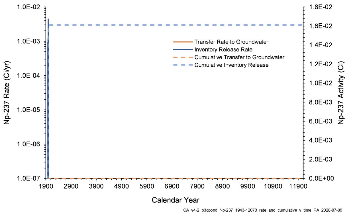
Figure 7-19. Np-237 Inventory Release from Waste Sites and Transfer to Groundwater for the B-3C Pond Model from 1943–12070
