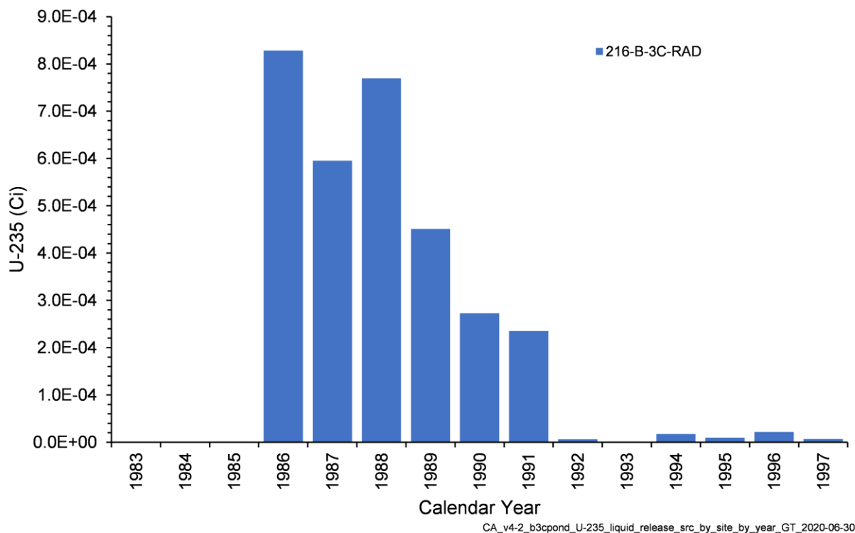
Figure 4-29. Annual U-235 Activity Released from Liquid Waste Sites in the B-3C Pond Model
