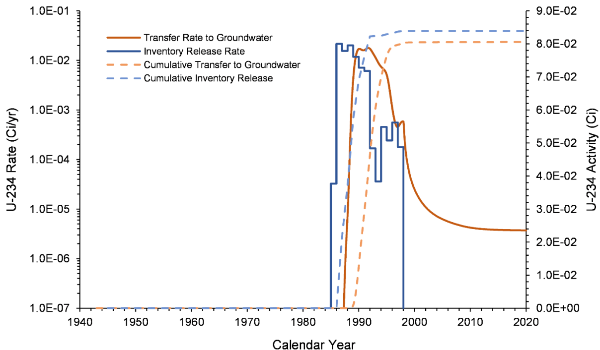
Figure 7-33. U-234 Inventory Release from Waste Sites and Transfer to Groundwater for the B-3C Pond Model from 1943–2018
