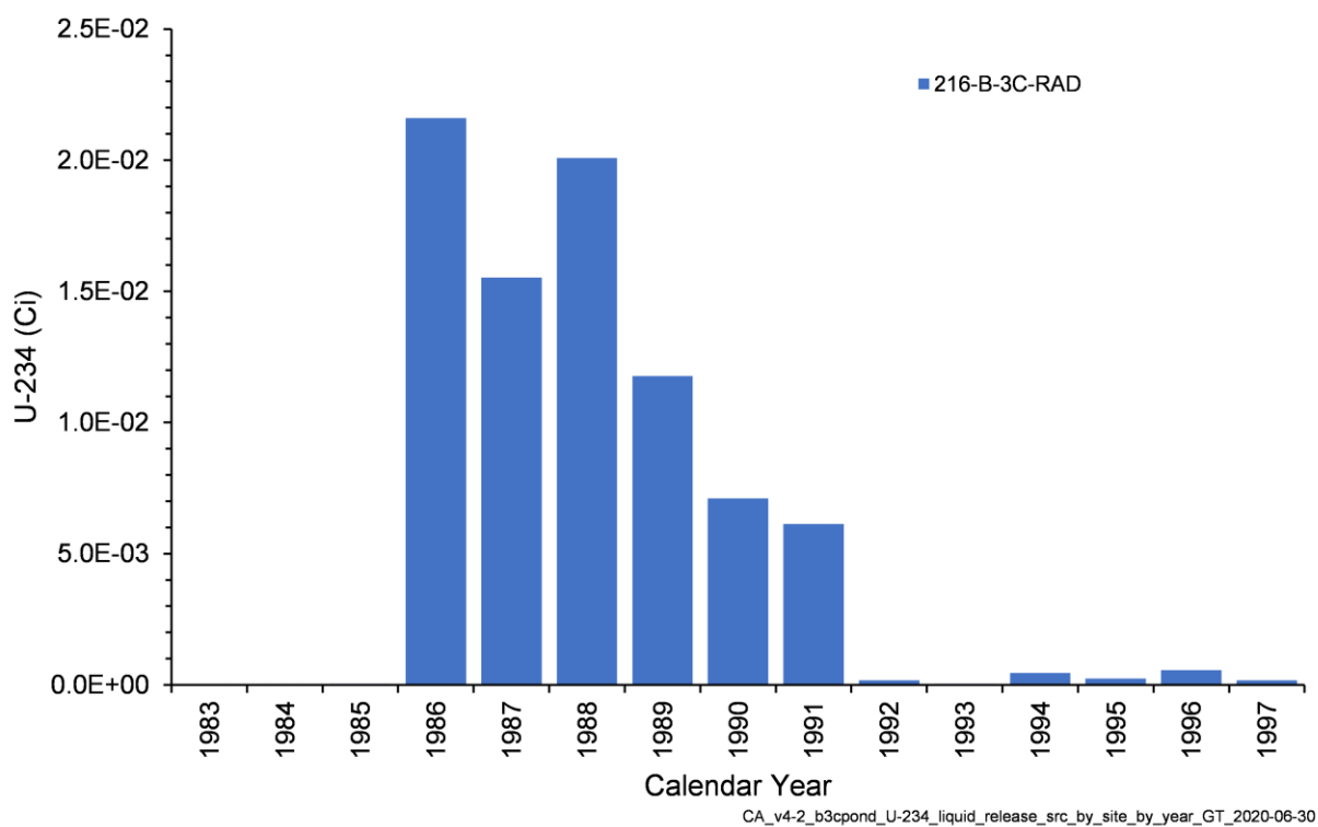
Figure 4-28. Annual U-234 Activity Released from Liquid Waste Sites in the B-3C Pond Model
