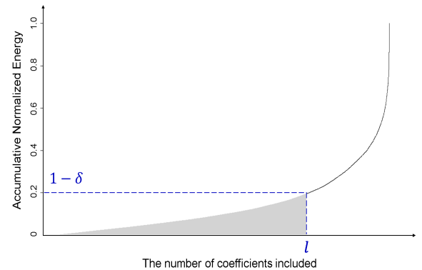
FIGURE 1. Pictorial explanation for determining a cut-off value of l .
