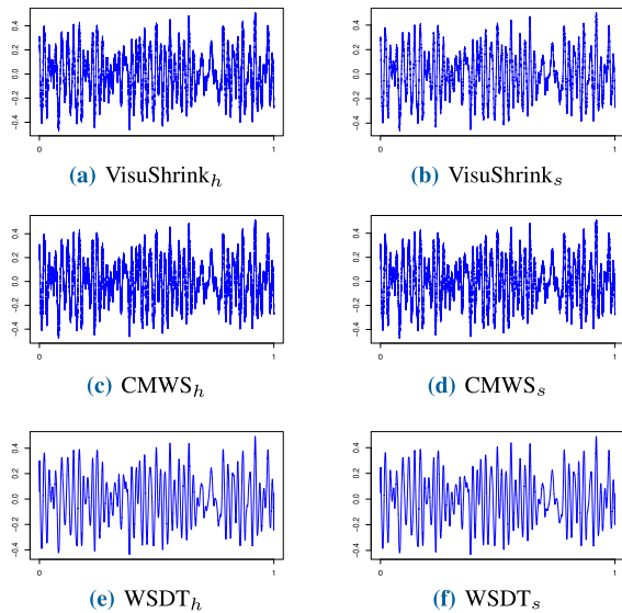
FIGURE 9. Reconstruction of the Sound 1 signal.
