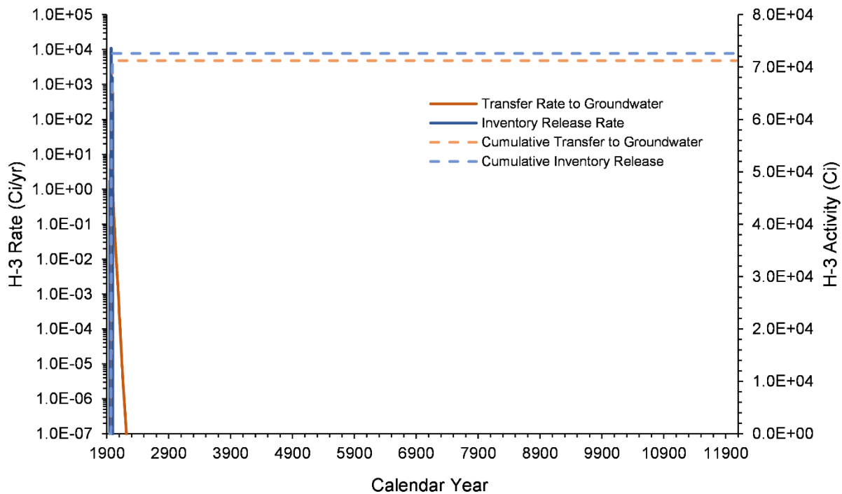
Figure 7-8. H-3 Inventory Release from Waste Sites and Transfer to Groundwater for the B-3 Pond Model from 1943–12070
