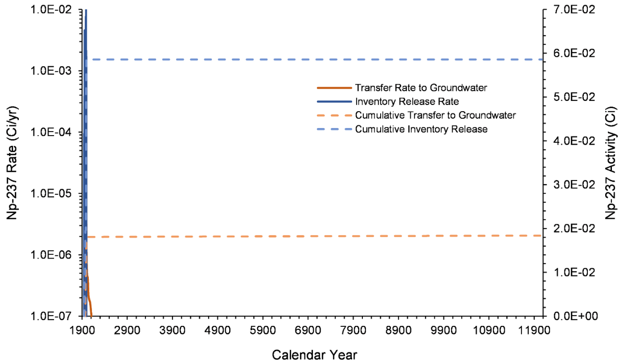
Figure 7-22. Np-237 Inventory Release from Waste Sites and Transfer to Groundwater for the B-3 Pond Model from 1943–12070
