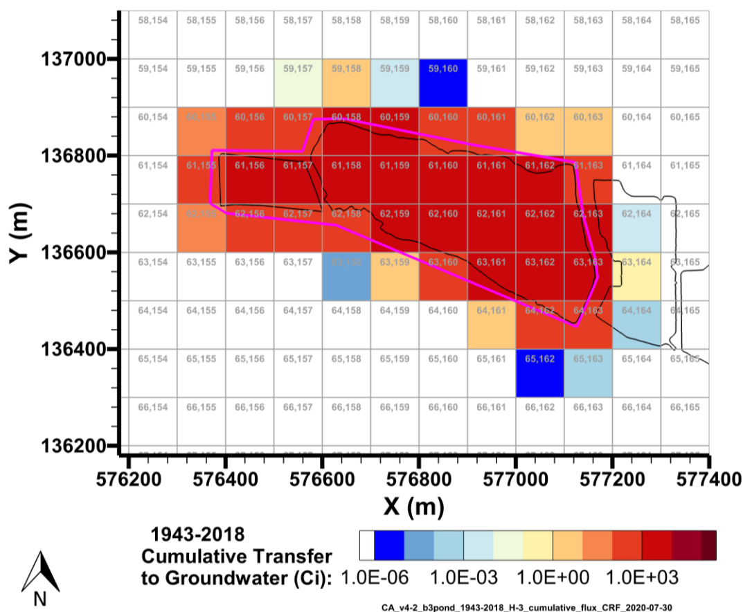
Figure 7-5. Cumulative H-3 Activity Discharged to Groundwater from the B-3 Pond Model from 1943–2018 per P2R Grid Cell
