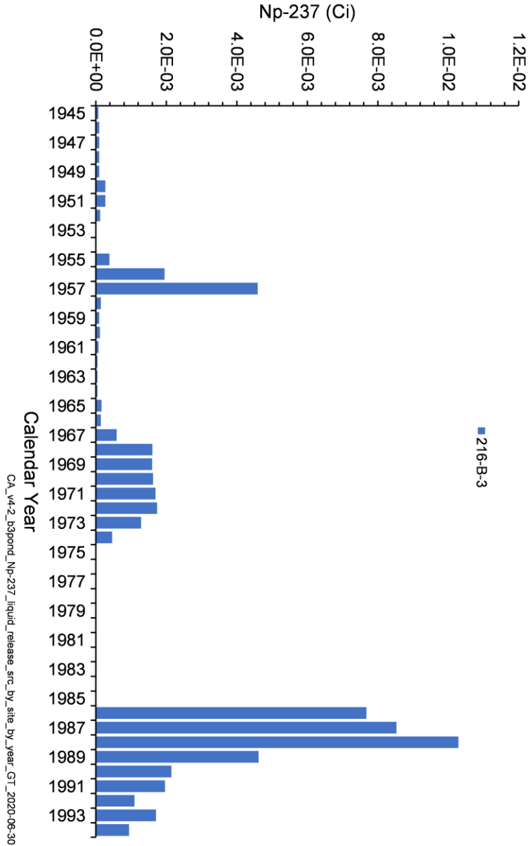
Figure 4-23. Annual Np-237 Activity Released from Liquid Waste Sites in the B-3 Pond Model
