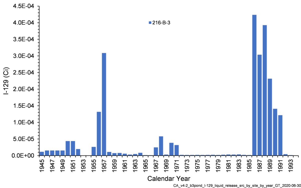
Figure 4-22. Annual I-129 Activity Released from Liquid Waste Sites in the B-3 Pond Model
