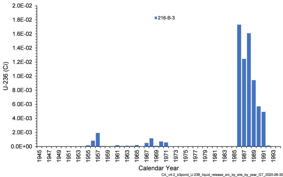
Figure 4-30. Annual U-236 Activity Released from Liquid Waste Sites in the B-3 Pond Model
