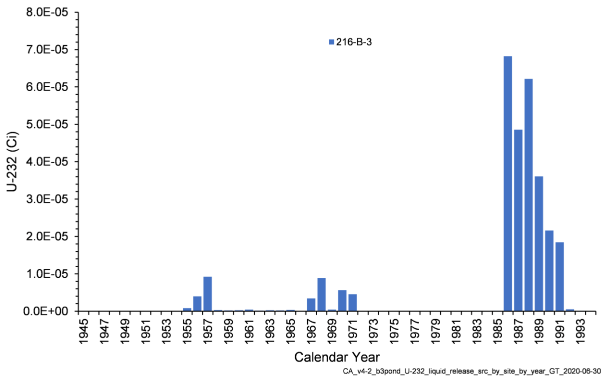
Figure 4-26. Annual U-232 Activity Released from Liquid Waste Sites in the B-3 Pond Model
