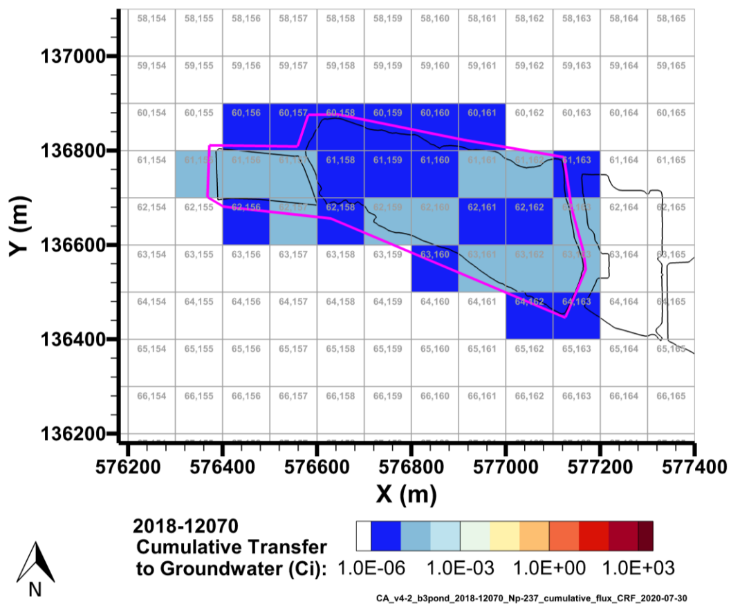
Figure 7-20. Cumulative Np-237 Activity Discharged to Groundwater from the B-3 Pond Model from 2018–12070 per P2R Grid Cell
