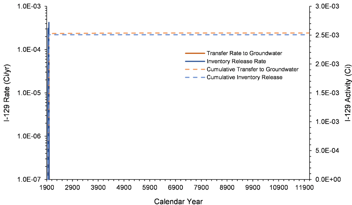
Figure 7-18. I-129 Inventory Release from Waste Sites and Transfer to Groundwater for the B-3 Pond Model from 1943–12070
