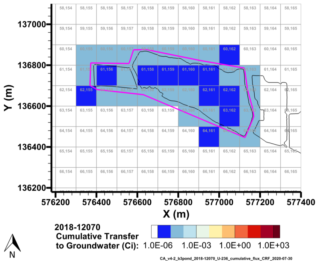
Figure 7-46. Cumulative U-236 Activity Discharged to Groundwater from the B-3 Pond Model from 2018–12070 per P2R Grid Cell
