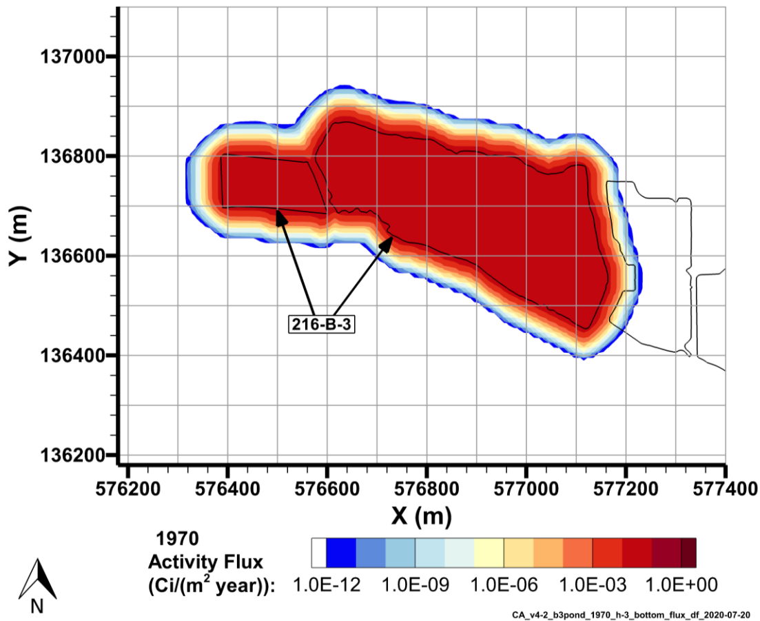
Figure 7-9. H-3 Flux to Groundwater, 1970
