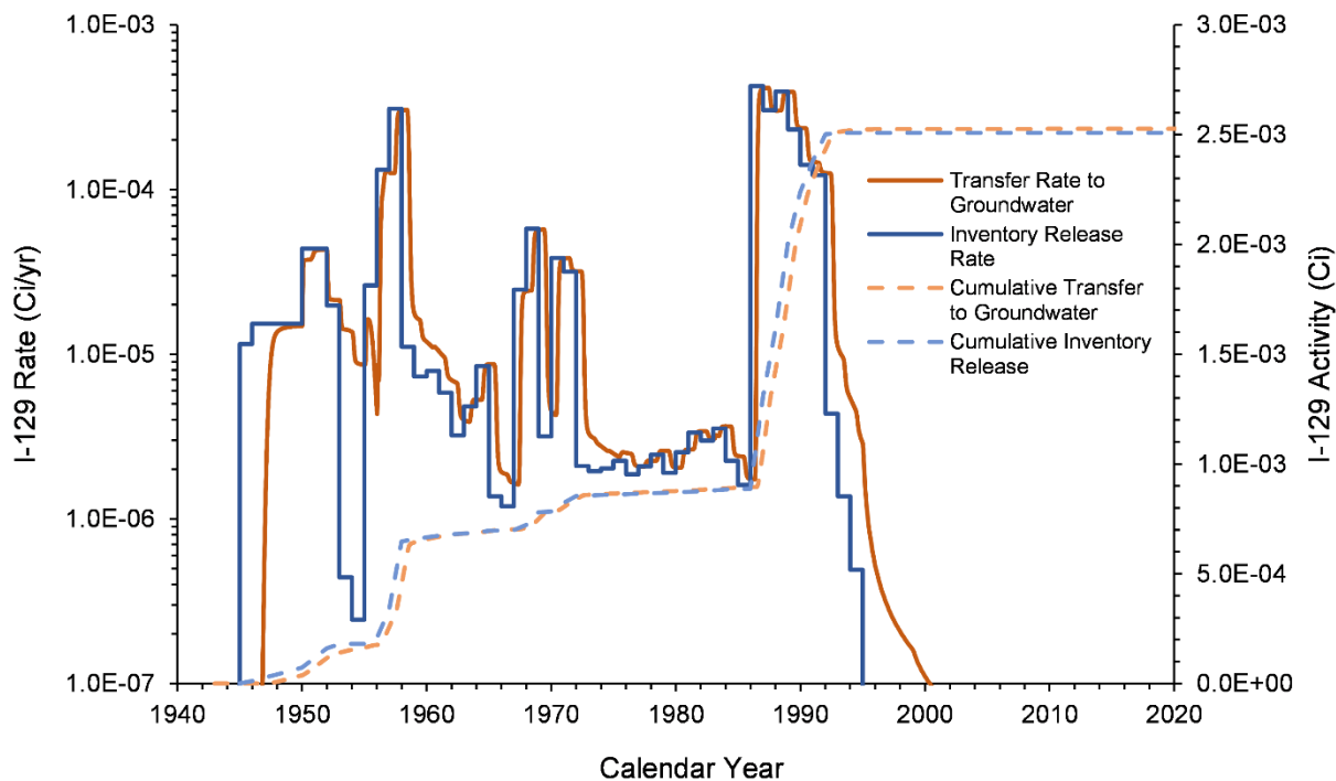
Figure 7-17. I-129 Inventory Release from Waste Sites and Transfer to Groundwater for the B-3 Pond Model from 1943–2018
