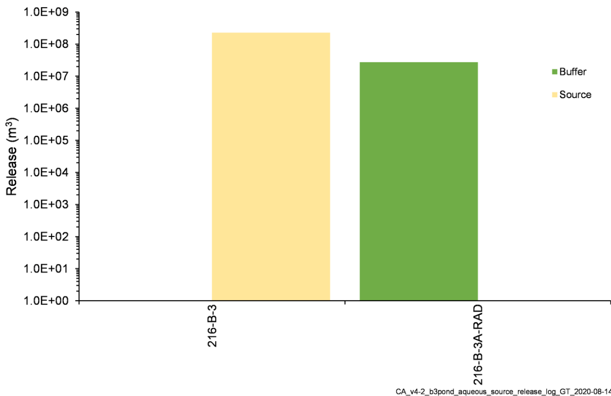
Figure 4-32. Total Volume of Water Released from Liquid Waste Sites in the B-3 Pond Model
