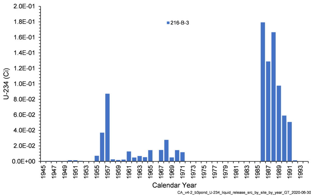
Figure 4-28. Annual U-234 Activity Released from Liquid Waste Sites in the B-3 Pond Model
