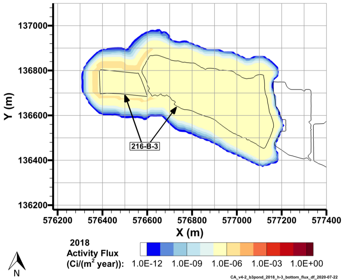
Figure 7-12. H-3 Flux to Groundwater, 2018
