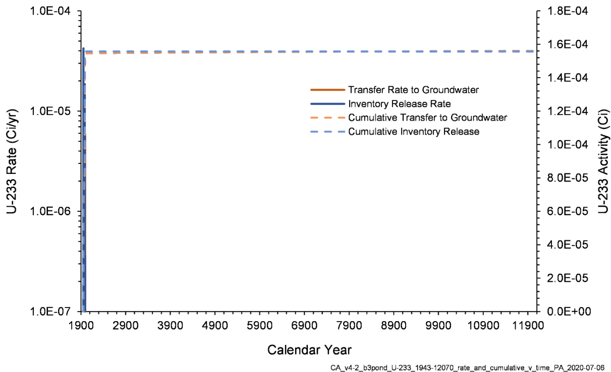
Figure 7-36. U-233 Inventory Release from Waste Sites and Transfer to Groundwater for the B-3 Pond Model from 1943–12070
