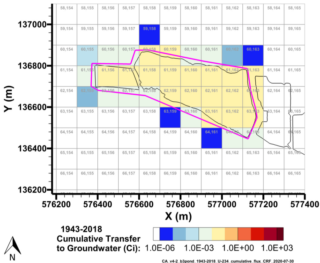
Figure 7-37. Cumulative U-234 Activity Discharged to Groundwater from the B-3 Pond Model from 1943–2018 per P2R Grid Cell
