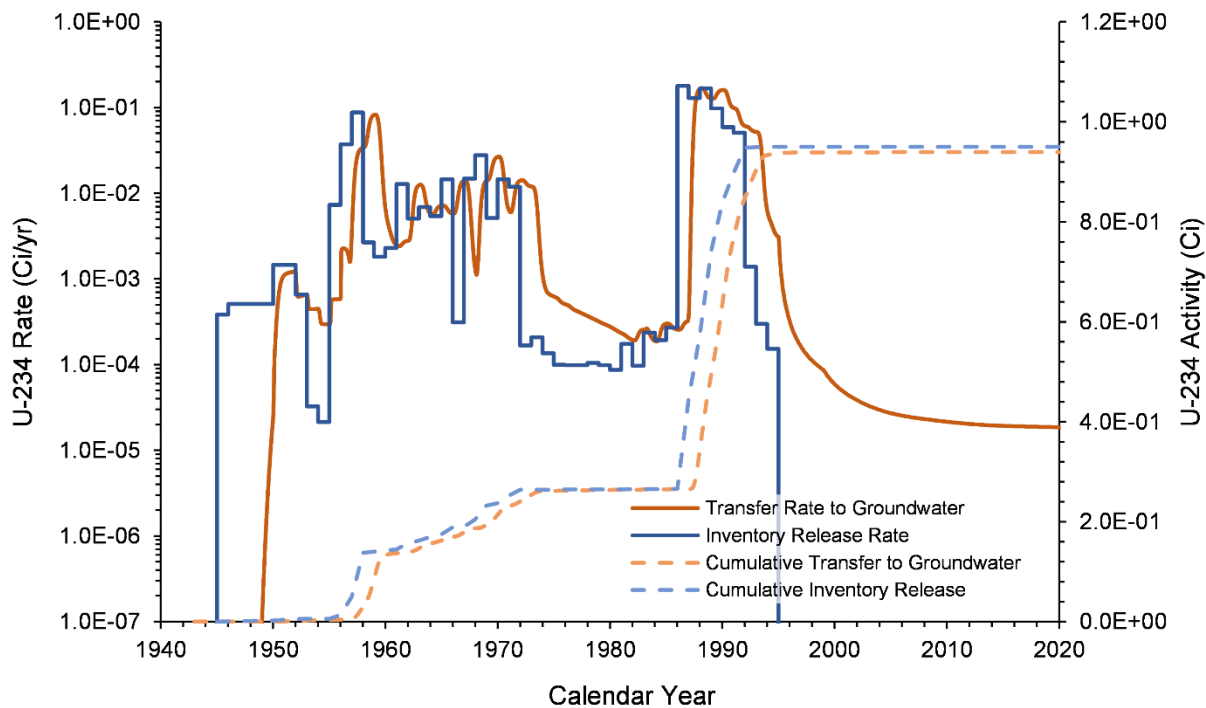
Figure 7-39. U-234 Inventory Release from Waste Sites and Transfer to Groundwater for the B-3 Pond Model from 1943–2018
