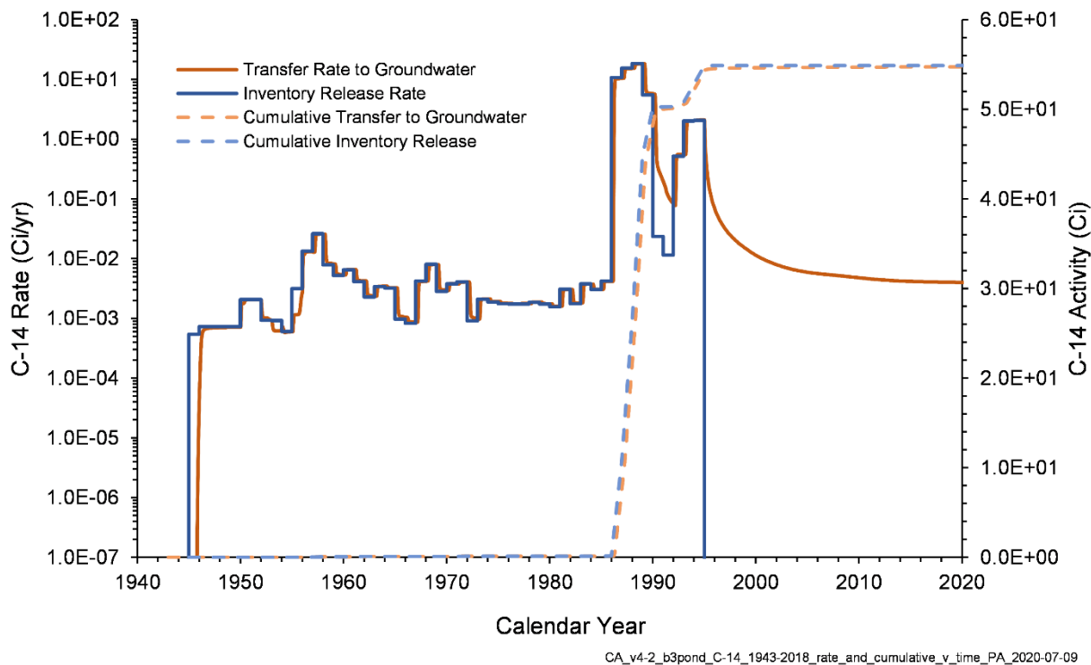
Figure 7-3. C-14 Inventory Release from Waste Sites and Transfer to Groundwater for the B-3 Pond Model from 1943–2018
