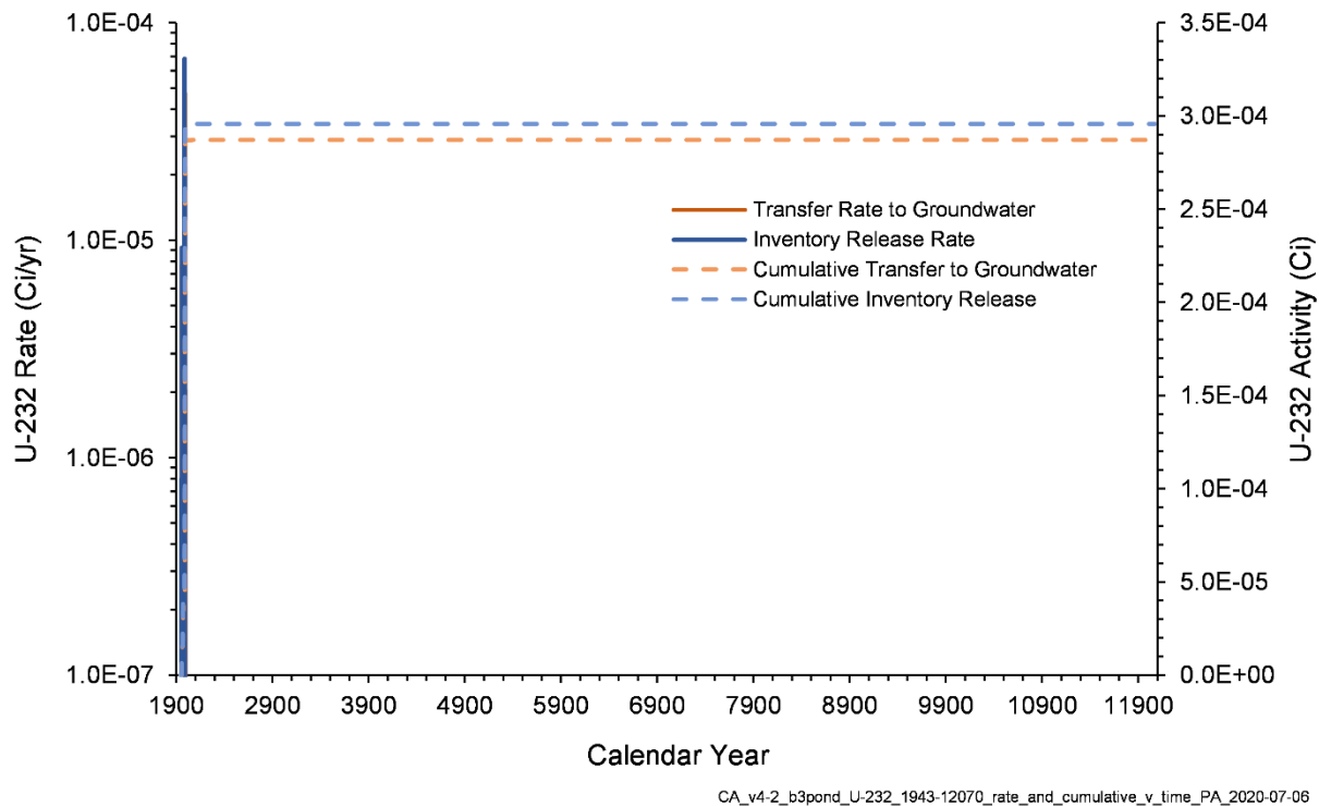
Figure 7-33. U-232 Inventory Release from Waste Sites and Transfer to Groundwater for the B-3 Pond Model from 1943–12070
