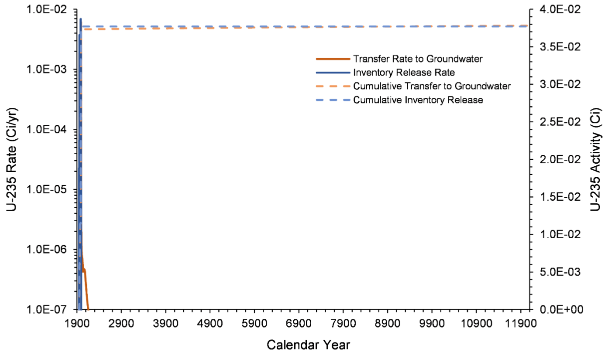
Figure 7-44. U-235 Inventory Release from Waste Sites and Transfer to Groundwater for the B-3 Pond Model from 1943–12070
