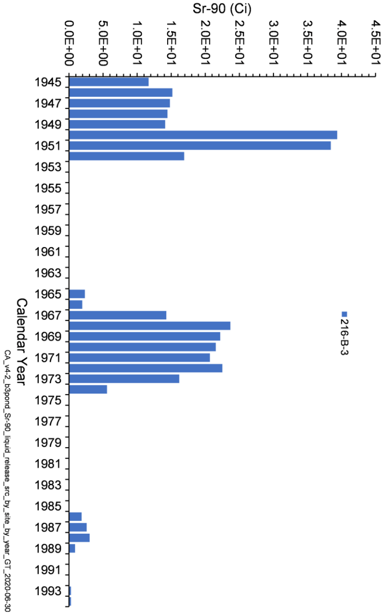
Figure 4-24. Annual Sr-90 Activity Released from Liquid Waste Sites in the B-3 Pond Model
