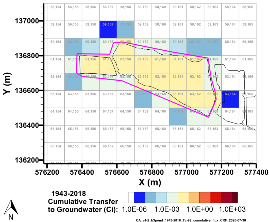
Figure 7-27. Cumulative Tc-99 Activity Discharged to Groundwater from the B-3 Pond Model from 1943–2018 per P2R Grid Cell
