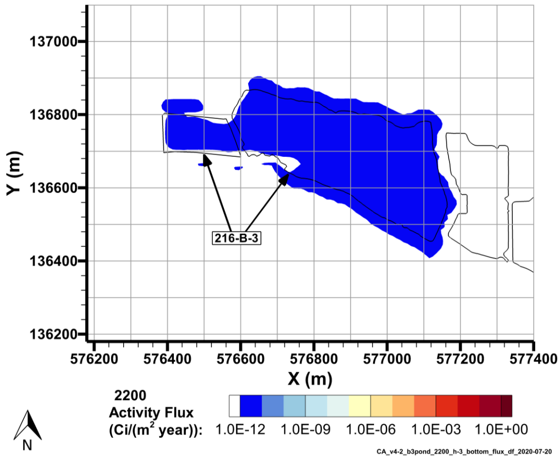
Figure 7-14. H-3 Flux to Groundwater, 2200
