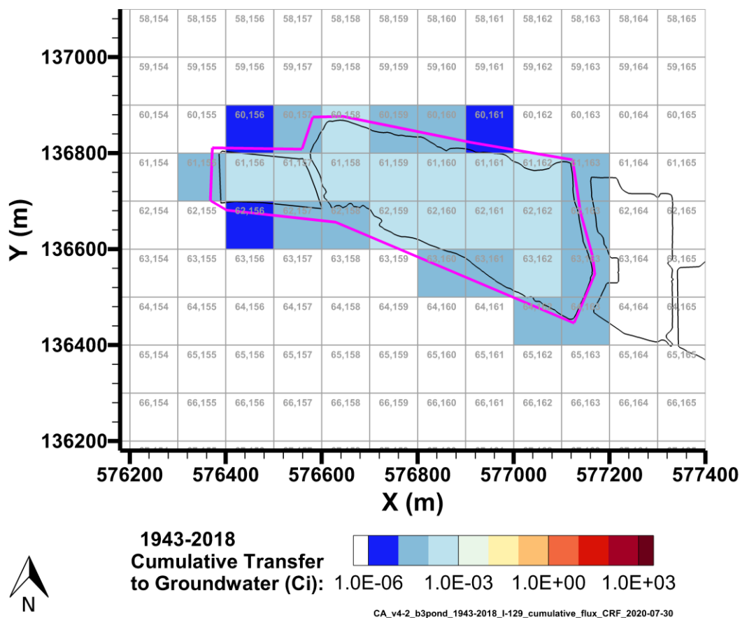
Figure 7-16. Cumulative I-129 Activity Discharged to Groundwater from the B-3 Pond Model from 1943–2018 per P2R Grid Cell
