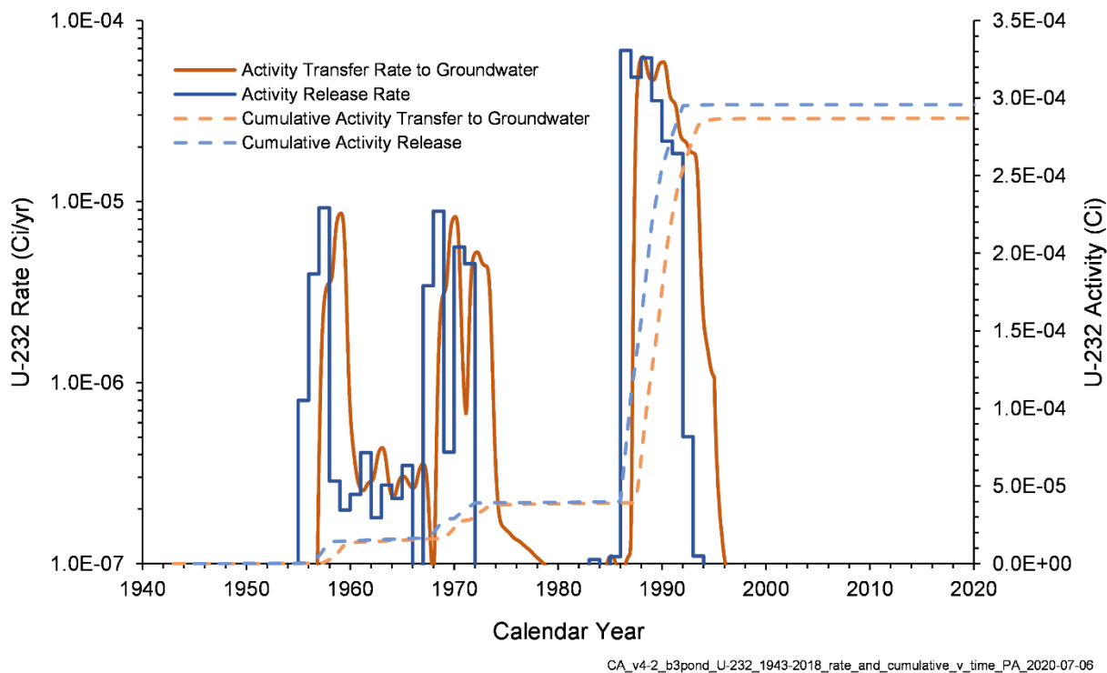
Figure 7-32. U-232 Inventory Release from Waste Sites and Transfer to Groundwater for the B-3 Pond Model from 1943–2018
