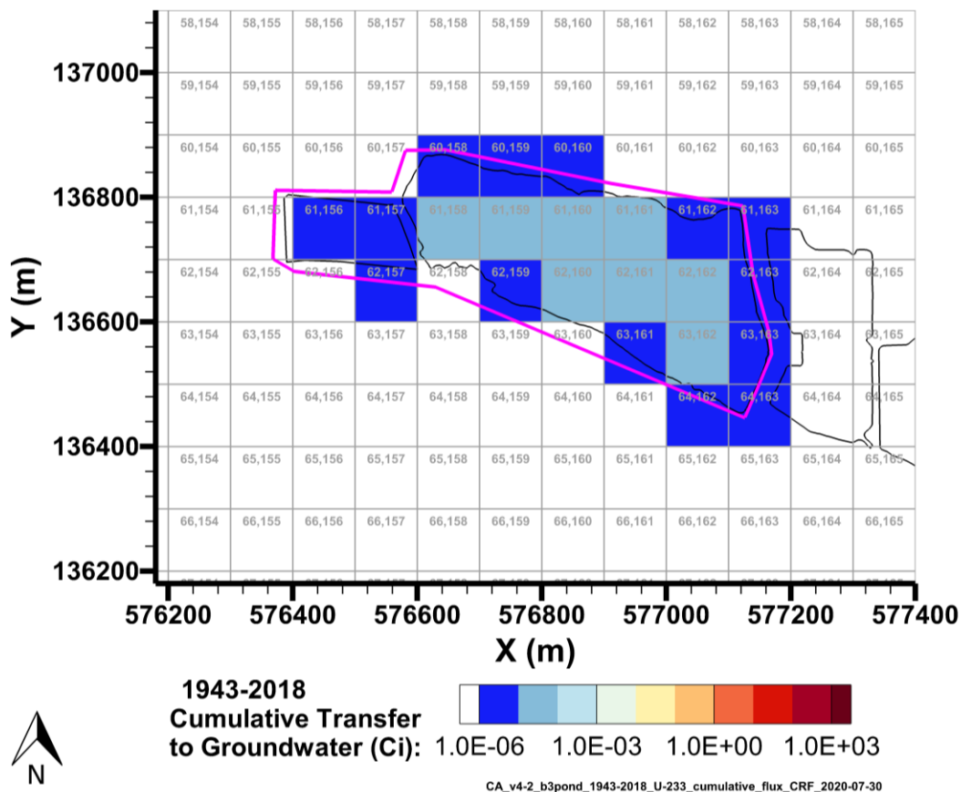
Figure 7-34. Cumulative U-233 Activity Discharged to Groundwater from the B-3 Pond Model from 1943–2018 per P2R Grid Cell
