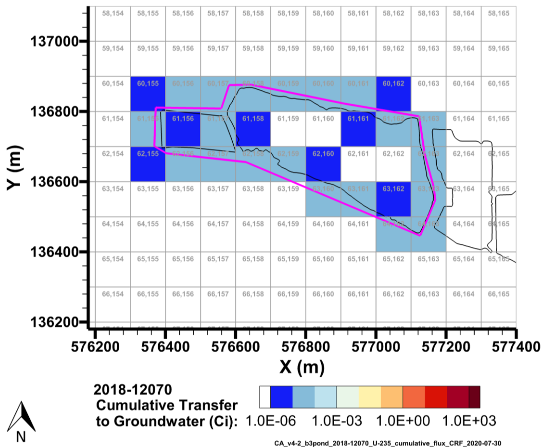
Figure 7-42. Cumulative U-235 Activity Discharged to Groundwater from the B-3 Pond Model from 2018–12070 per P2R Grid Cell
