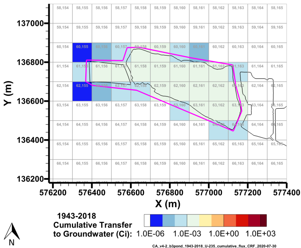
Figure 7-41. Cumulative U-235 Activity Discharged to Groundwater from the B-3 Pond Model from 1943–2018 per P2R Grid Cell
