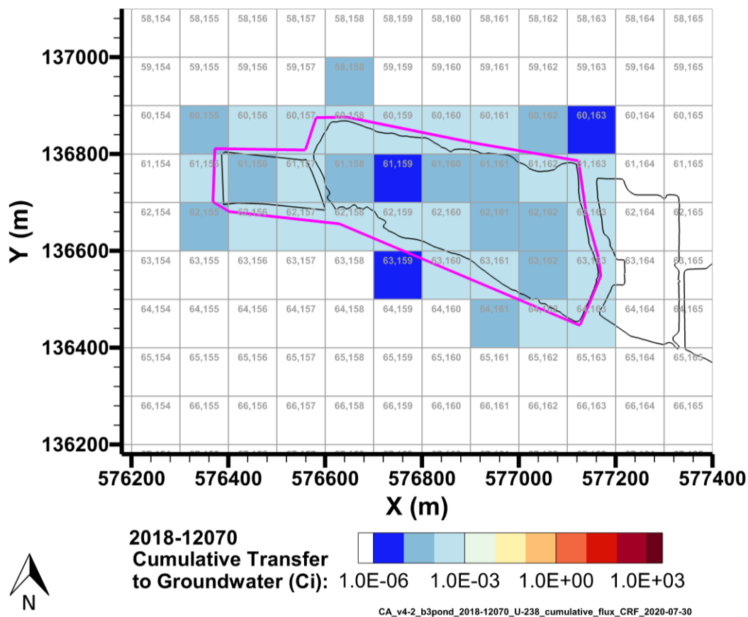
Figure 7-50. Cumulative U-238 Activity Discharged to Groundwater from the B-3 Pond Model from 2018–12070 per P2R Grid Cell
