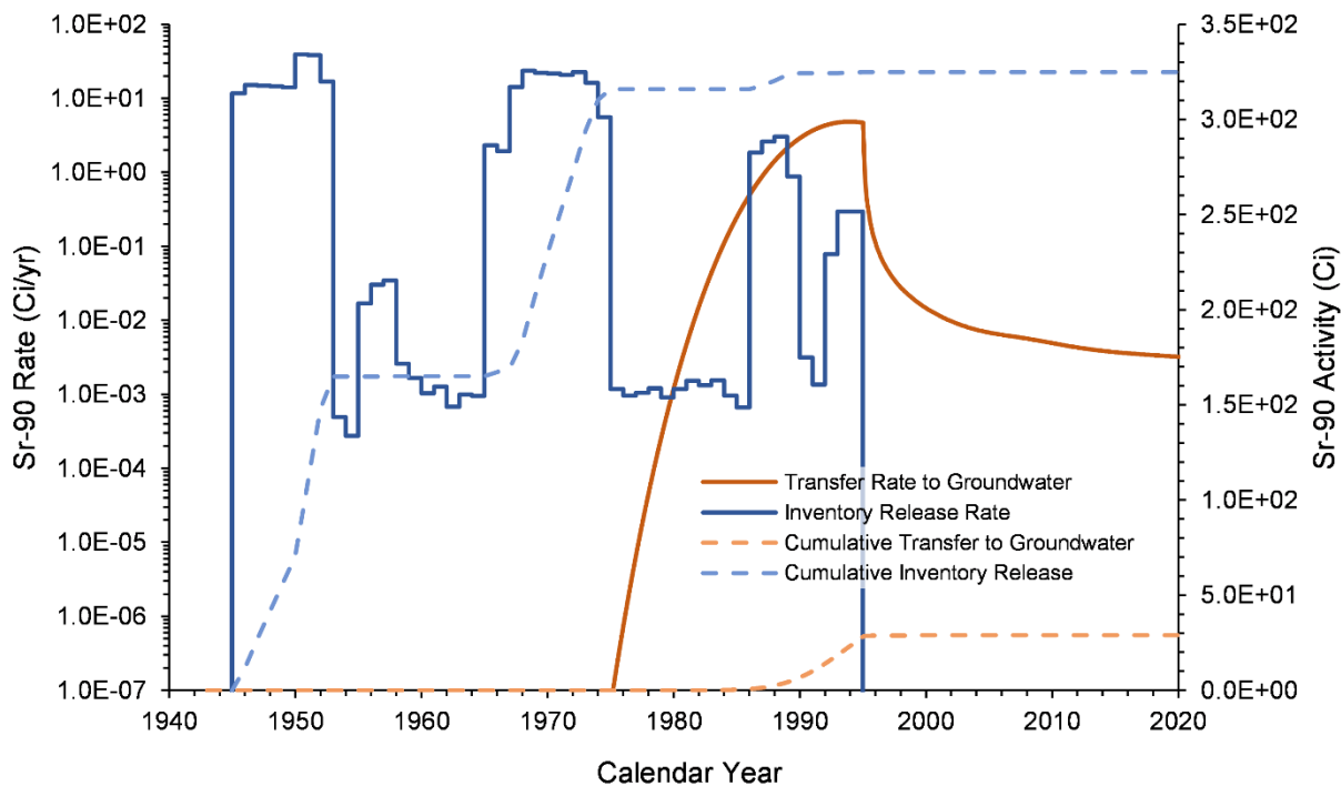
Figure 7-25. Sr-90 Inventory Release from Waste Sites and Transfer to Groundwater for the B-3 Pond Model from 1943–2018
