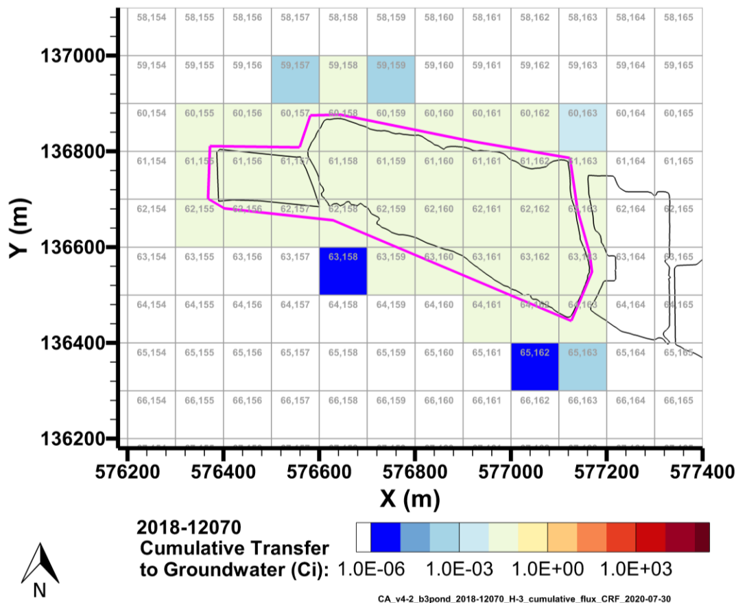
Figure 7-6. Cumulative H-3 Activity Discharged to Groundwater from the B-3 Pond Model from 2018-12070 per P2R Grid Cell
