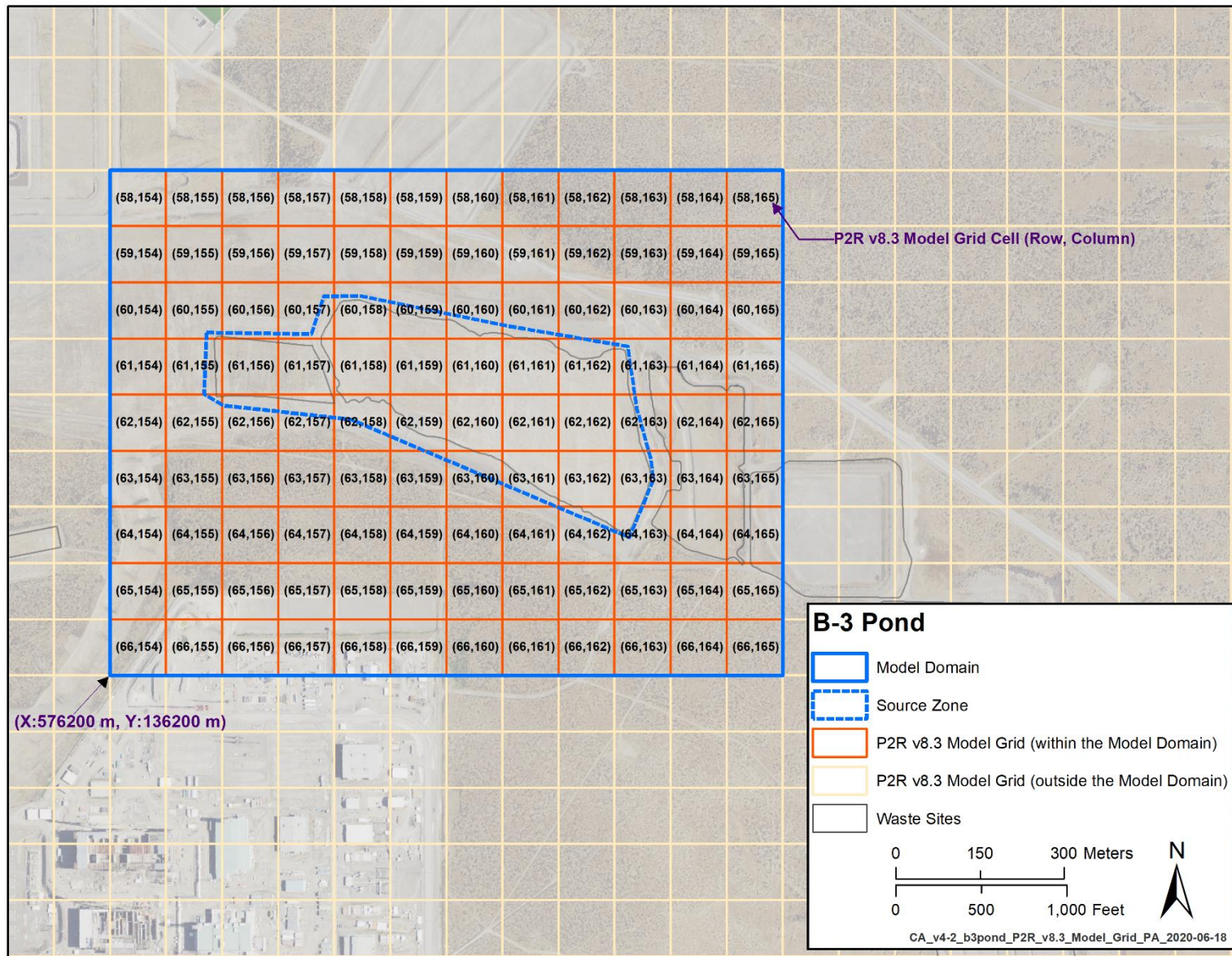
Figure 4-2. Plan View of the P2R Grid Cells in the B-3 Pond Model
