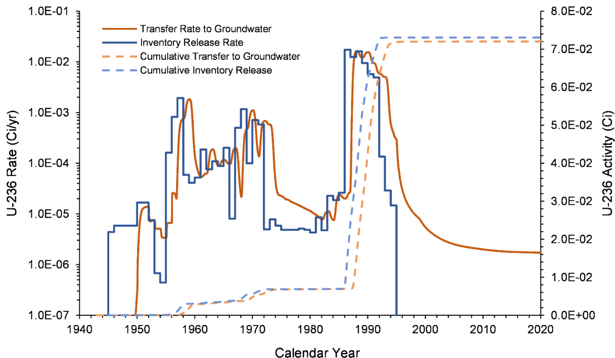
Figure 7-47. U-236 Inventory Release from Waste Sites and Transfer to Groundwater for the B-3 Pond Model from 1943–2018
