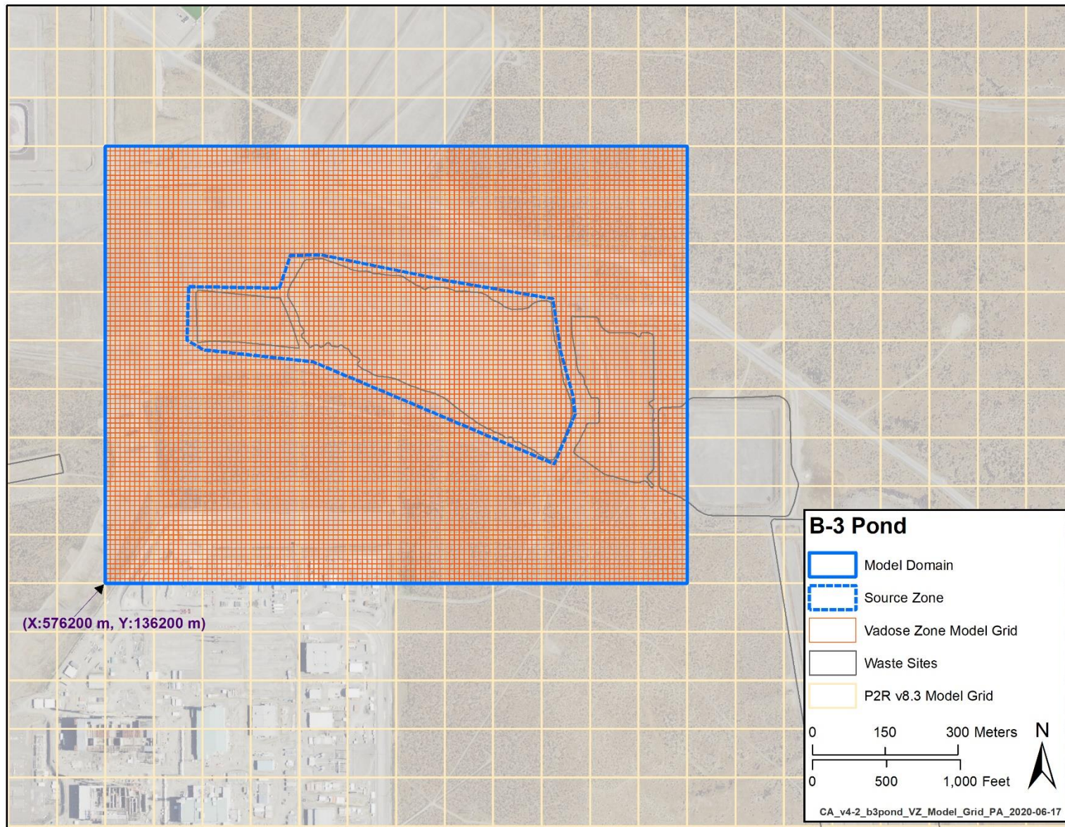
Figure 4-1. Plan View of the B-3 Pond Model Grid Overlain on the P2R Grid Cells
