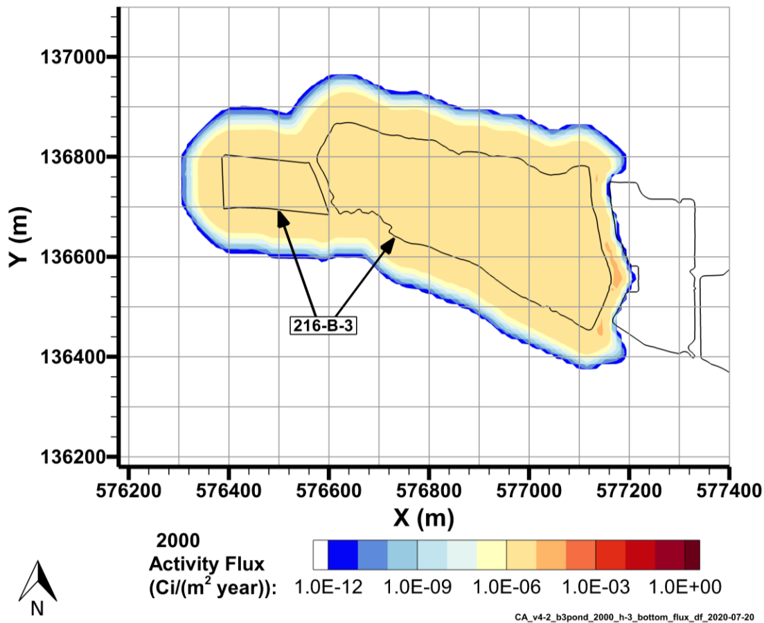
Figure 7-11. H-3 Flux to Groundwater, 2000
