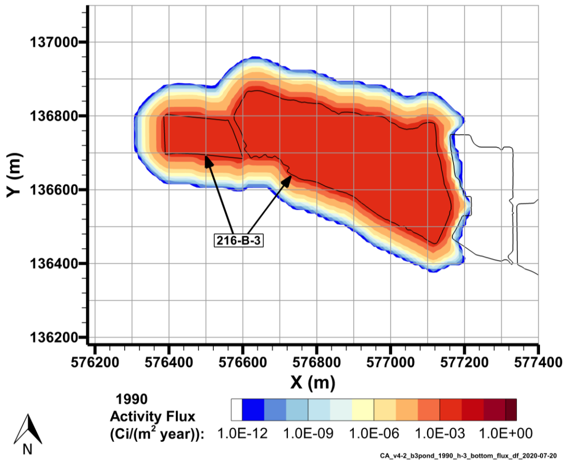
Figure 7-10. H-3 Flux to Groundwater, 1990
