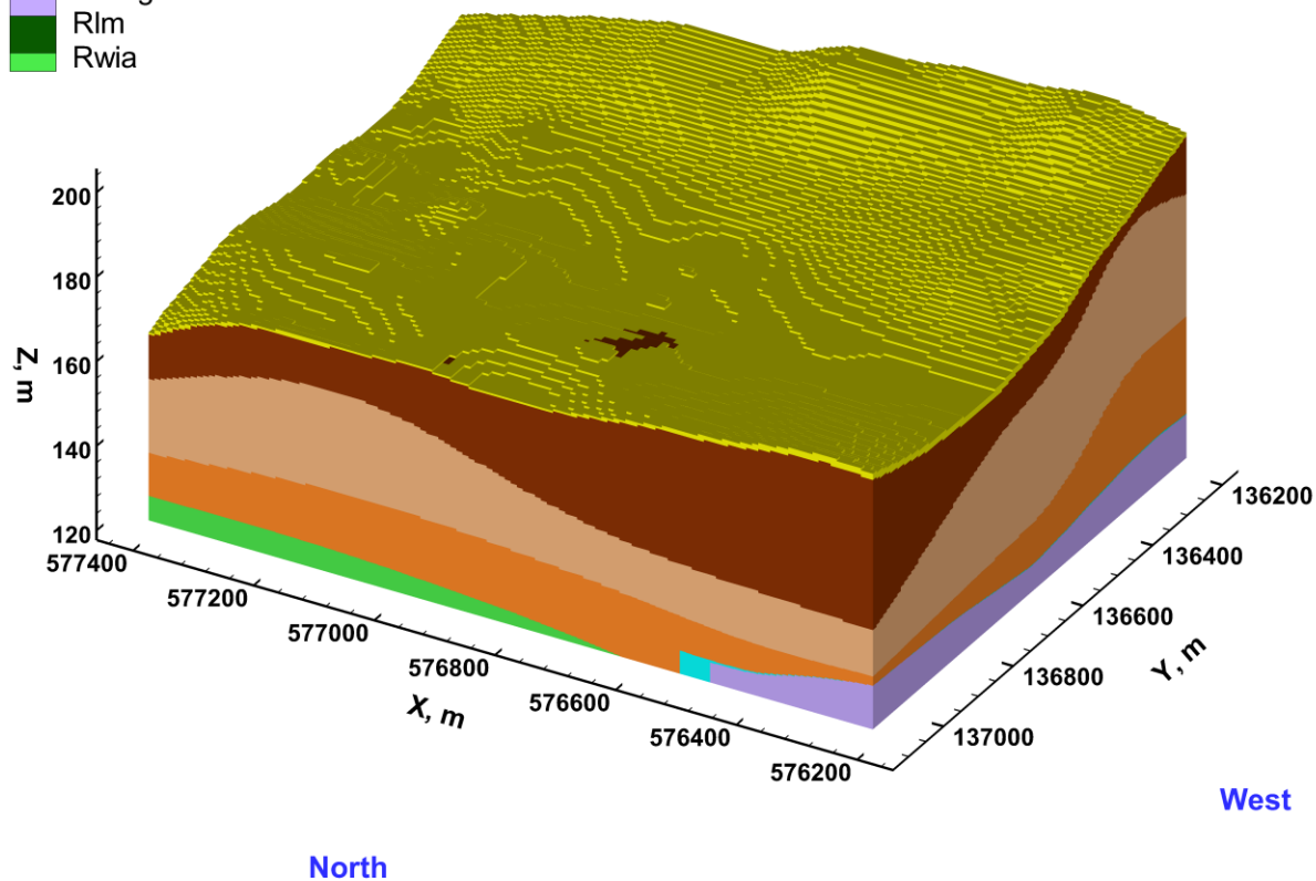
Figure 4-4. Model Hydrostratigraphy Three-Dimensional View Showing the North and West Faces
