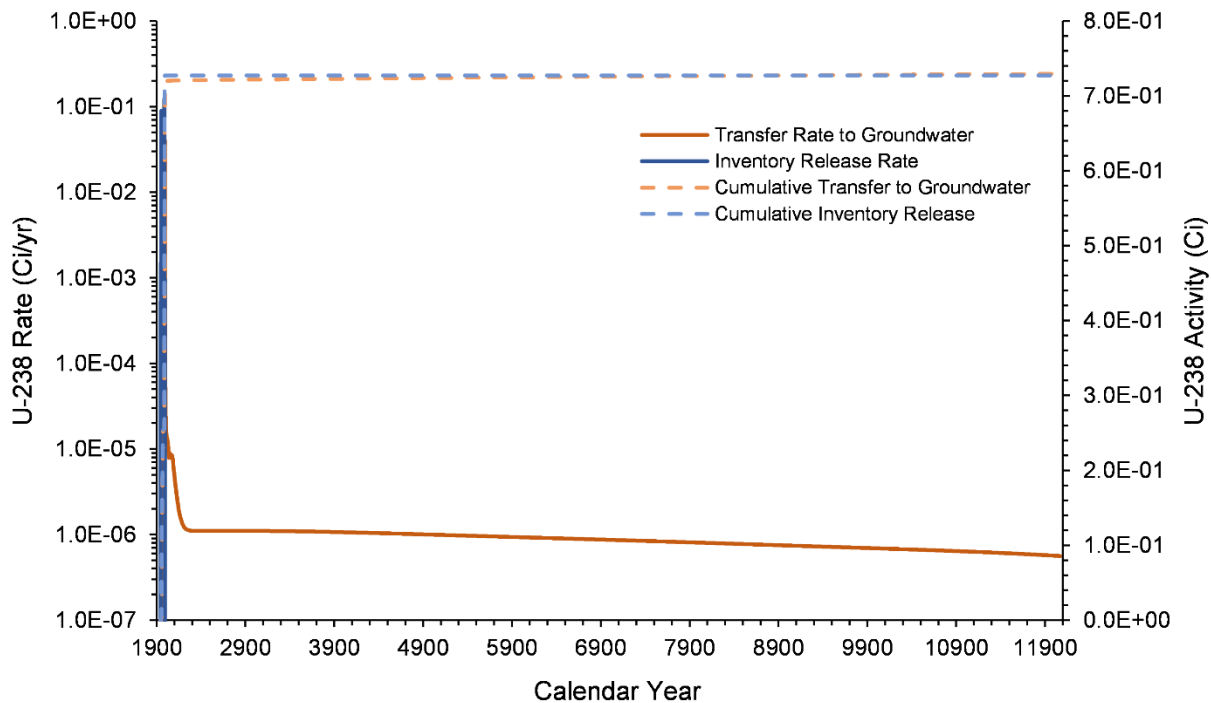
Figure 7-52. U-238 Inventory Release from Waste Sites and Transfer to Groundwater for the B-3 Pond Model from 1943–12070
