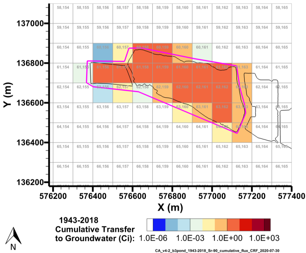
Figure 7-23. Cumulative Sr-90 Activity Discharged to Groundwater from the B-3 Pond Model from 1943–2018 per P2R Grid Cell
