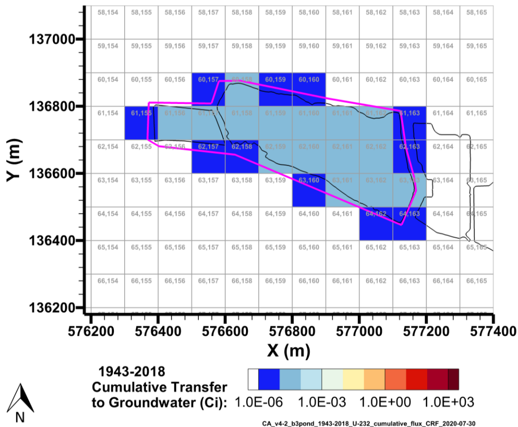
Figure 7-31. Cumulative U-232 Activity Discharged to Groundwater from the B-3 Pond Model from 1943–2018 per P2R Grid Cell
