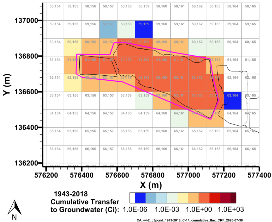
Figure 7-1. Cumulative C-14 Activity Discharged to Groundwater from the B-3 Pond Model from 1943–2018 per P2R Grid Cell
