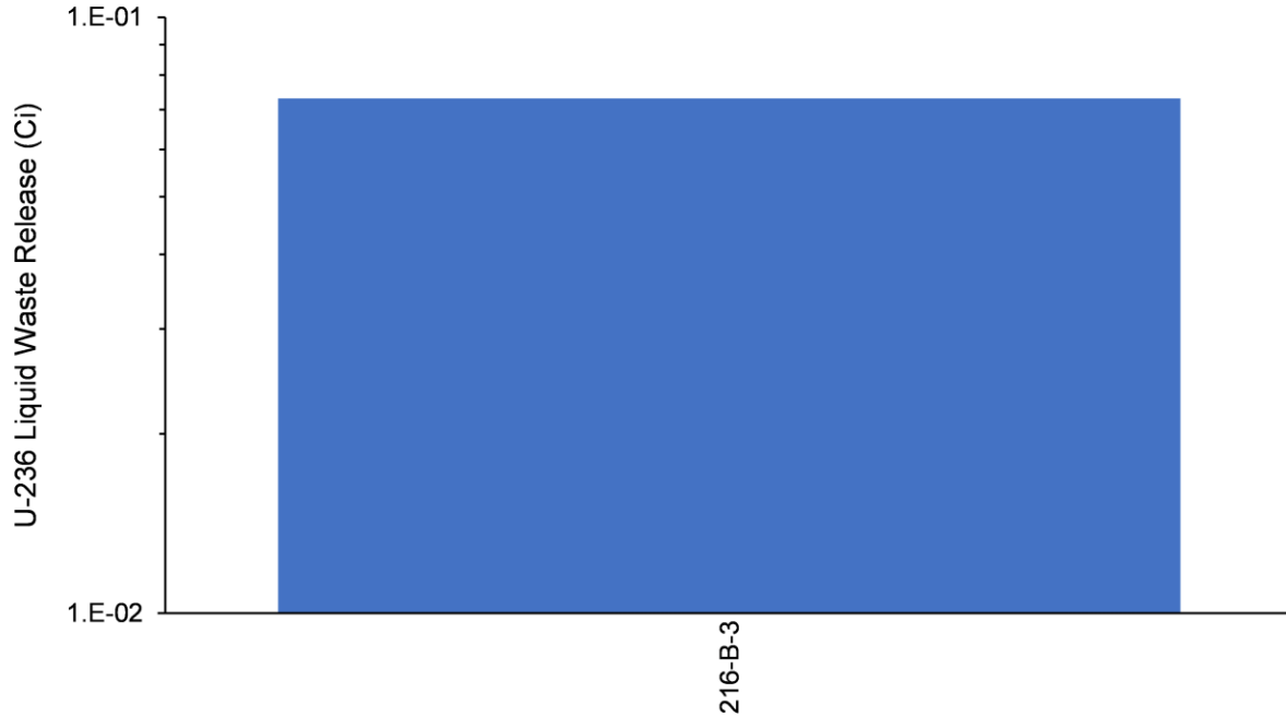
Figure 4-17. Total U-235 Activity Released from Liquid Waste Sites in the B-3 Pond Model
