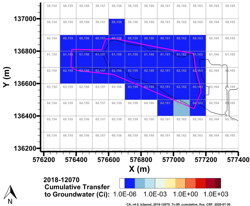
Figure 7-28. Cumulative Tc-99 Activity Discharged to Groundwater from the B-3 Pond Model from 2018–12070 per P2R Grid Cell
