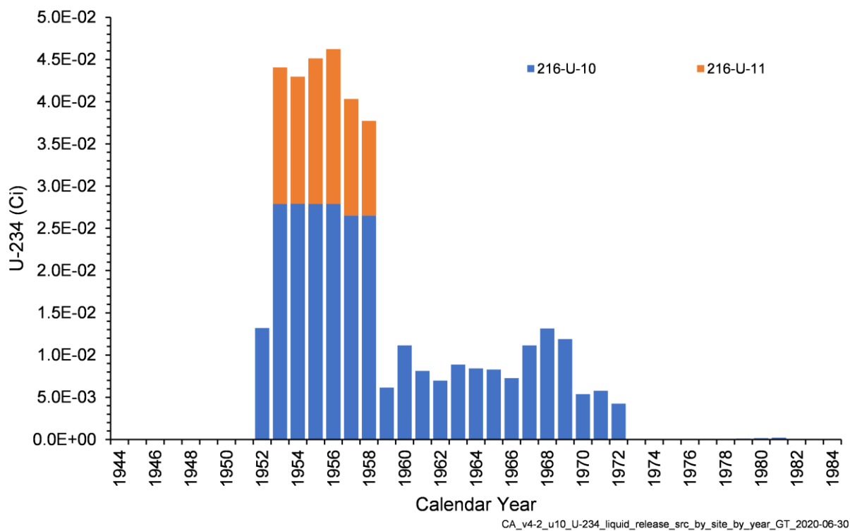
Figure 4-28. Annual U-234 Activity Released from Liquid Waste Sites in the U-10 West Area Model
