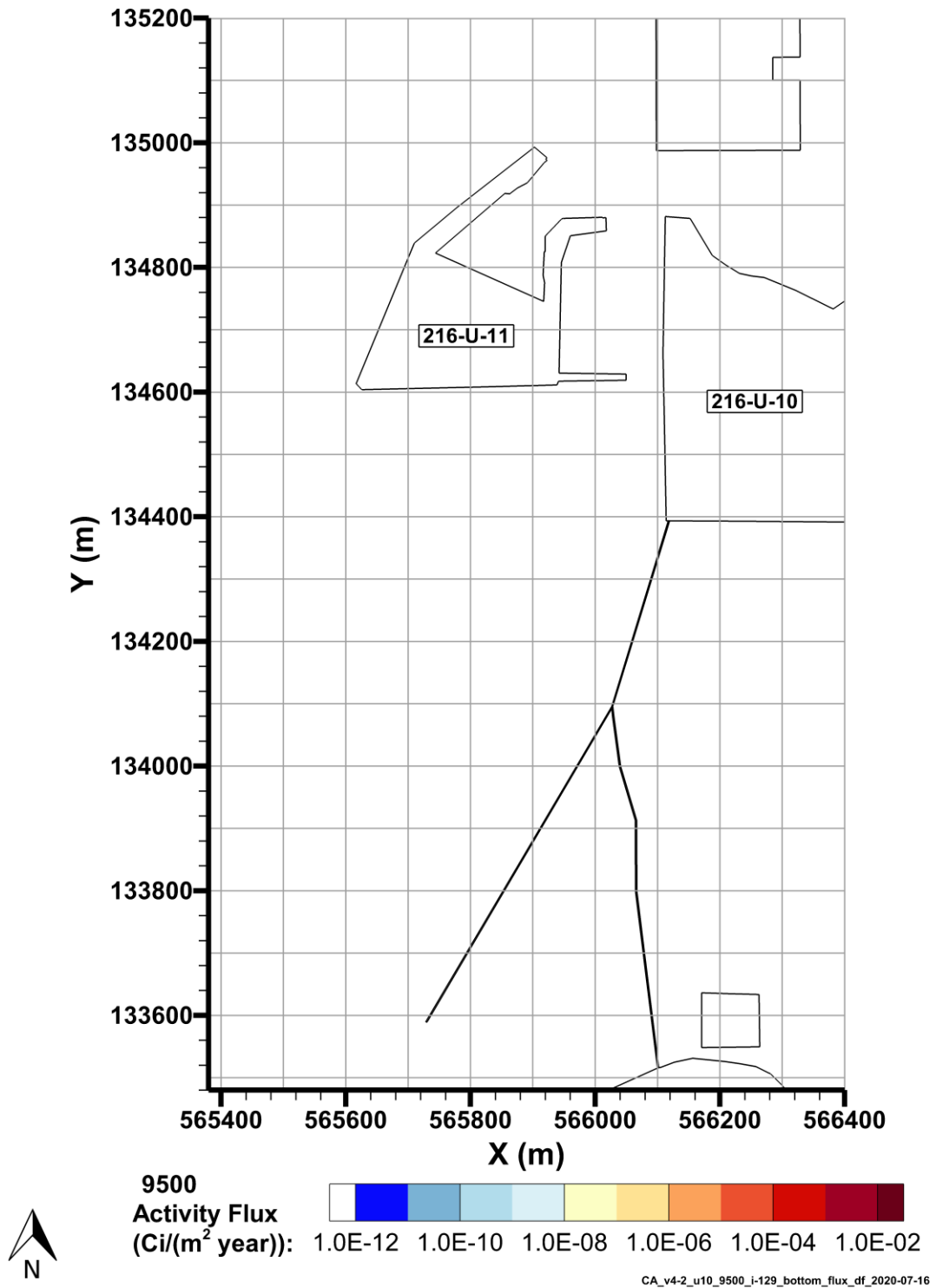
Figure 7-19. I-129 Flux to Groundwater, 9500
