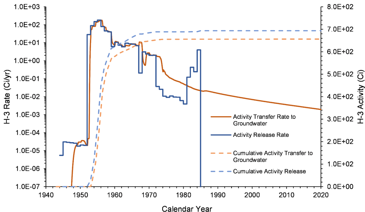
Figure 7-7. H-3 Inventory Release from Waste Sites and Transfer to Groundwater for the U-10 West Area Model from 1943–2018
