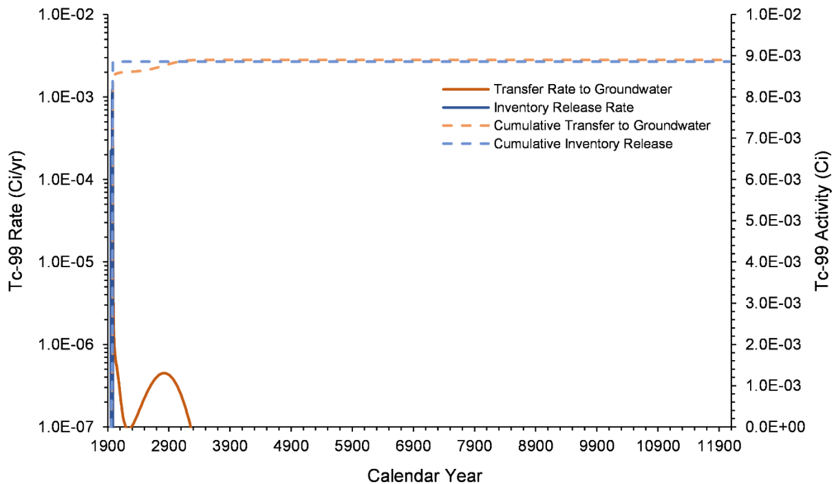
Figure 7-27. Tc-99 Inventory Release from Waste Sites and Transfer to Groundwater for the U-10 West Area Model from 1943–12070
