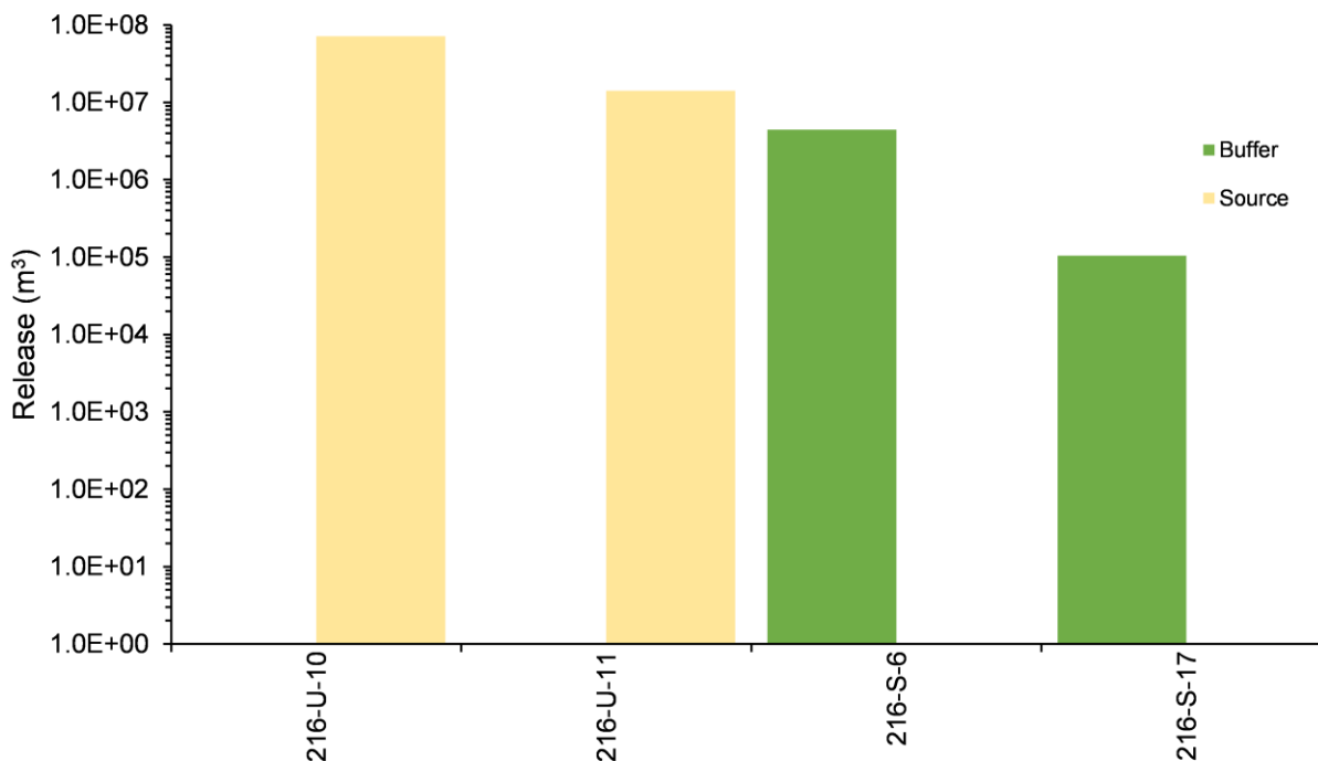
Figure 4-32. Total Volume of Water Released from Liquid Waste Sites in the U-10 West Area Model
