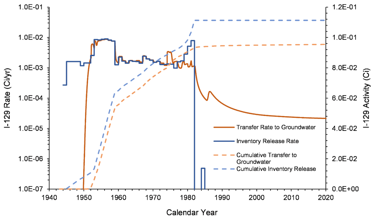
Figure 7-11. I-129 Inventory Release from Waste Sites and Transfer to Groundwater for the U-10 West Area Model from 1943–2018
