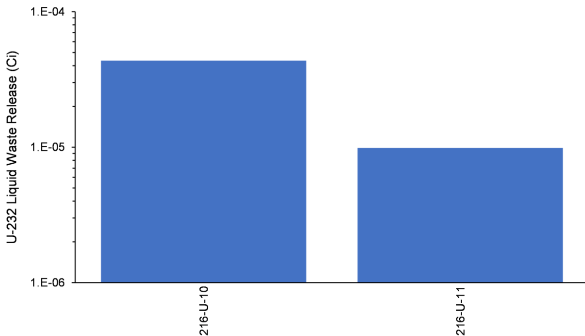
Figure 4-13. Total Tc-99 Activity Released from Liquid Waste Sites in the U-10 West Area Model
