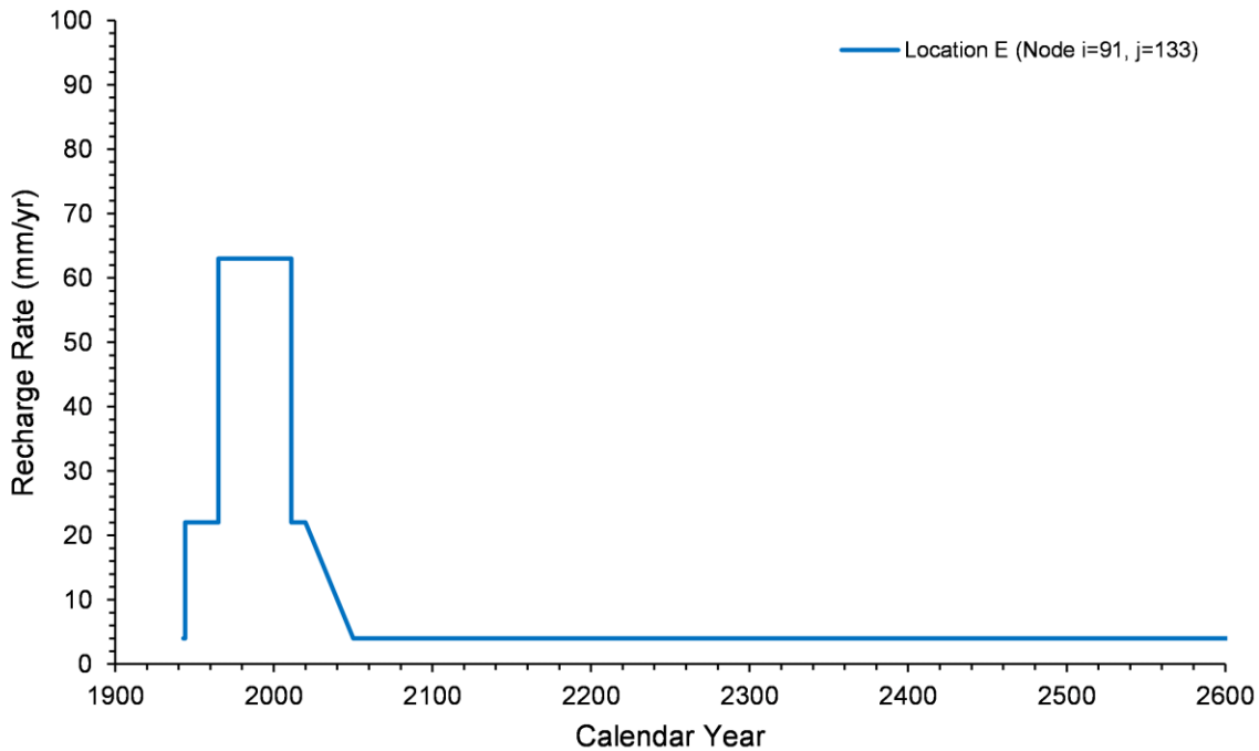
Figure 4-44. Time Series of Natural Recharge Rates, Location E
