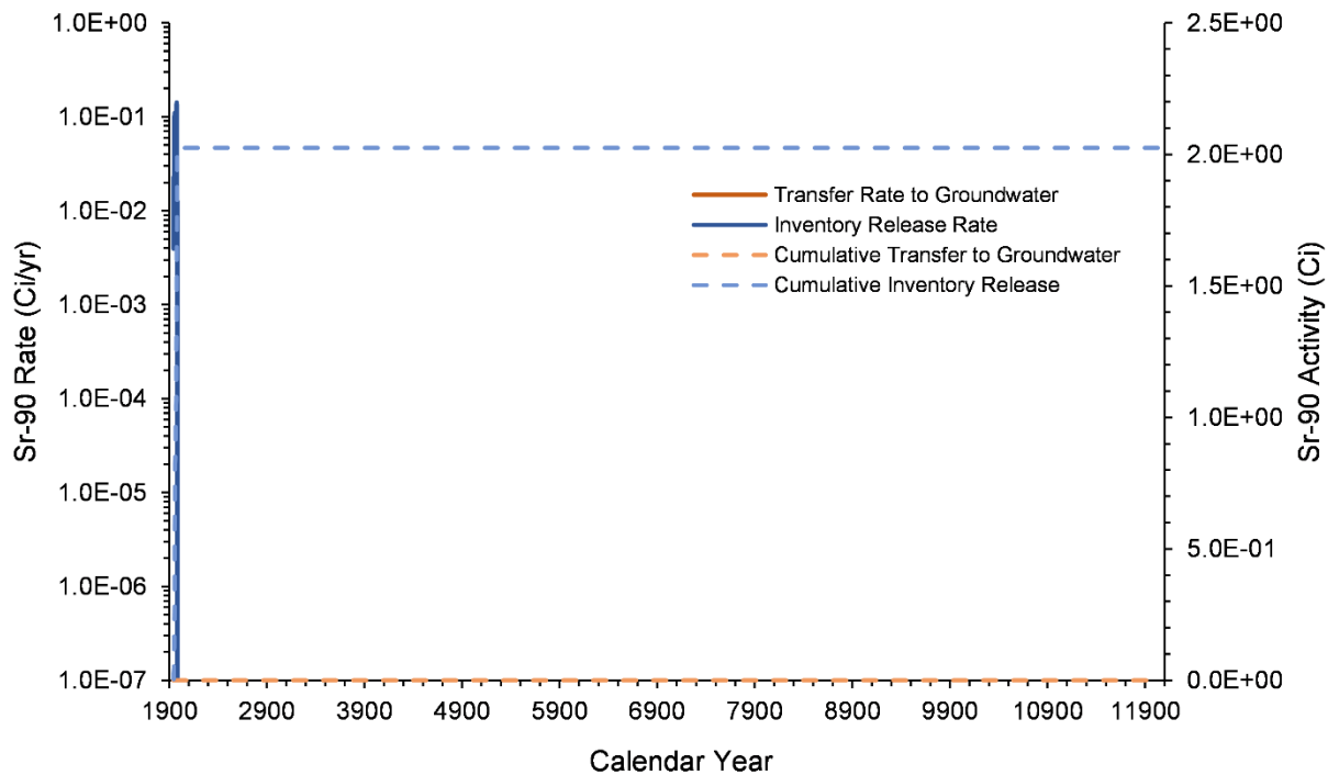
Figure 7-23. Sr-90 Inventory Release from Waste Sites and Transfer to Groundwater for the U-10 West Area Model from 1943–12070
