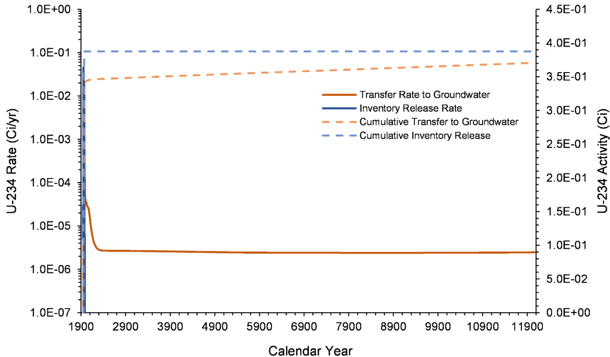
Figure 7-38. U-234 Inventory Release from Waste Sites and Transfer to Groundwater for the U-10 West Area Model from 1943–12070
