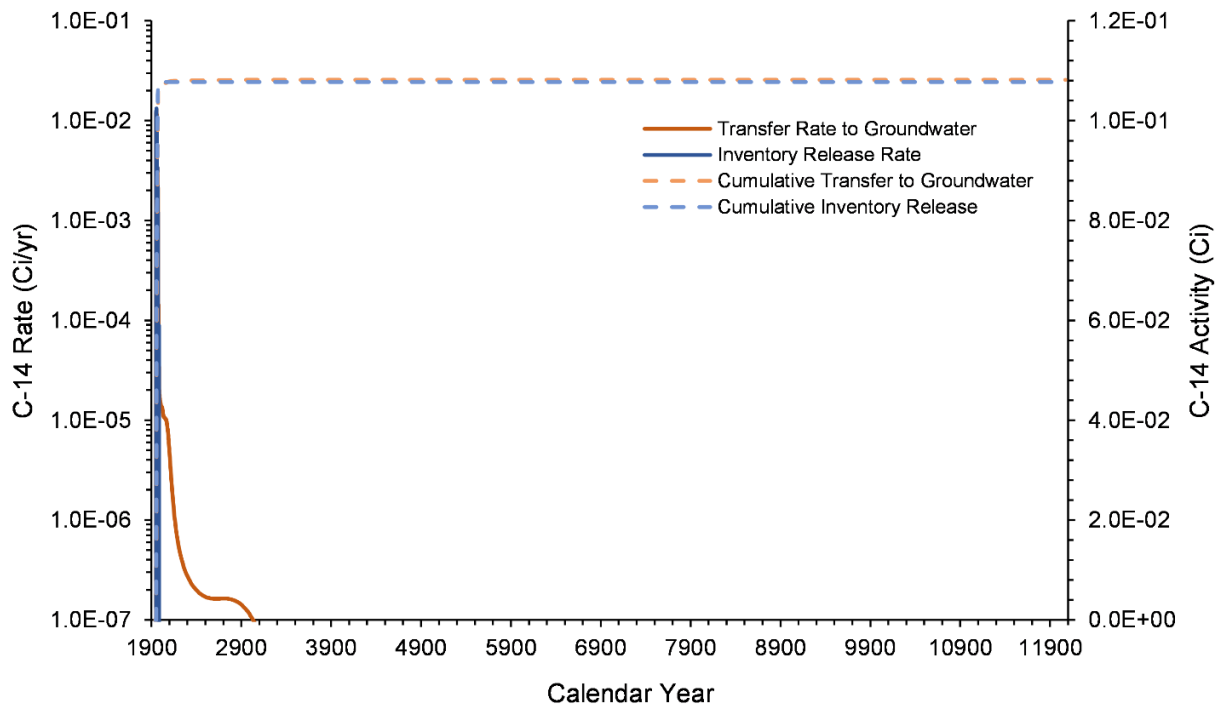
Figure 7-4. C-14 Inventory Release from Waste Sites and Transfer to Groundwater for the U-10 West Area Model from 1943–12070
