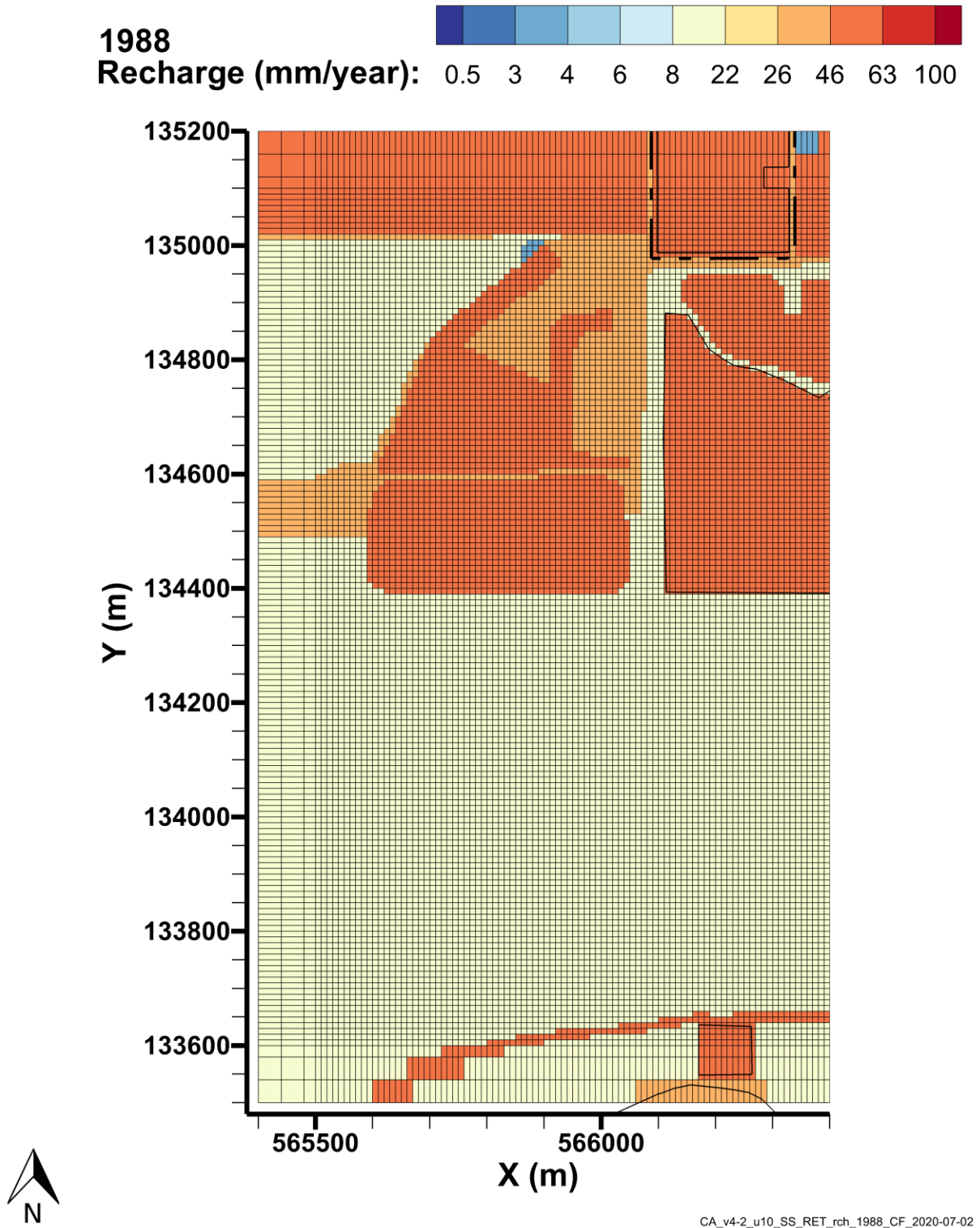
Figure 4-36. Transient Recharge Estimates for the U-10 West Area Model, 1988
