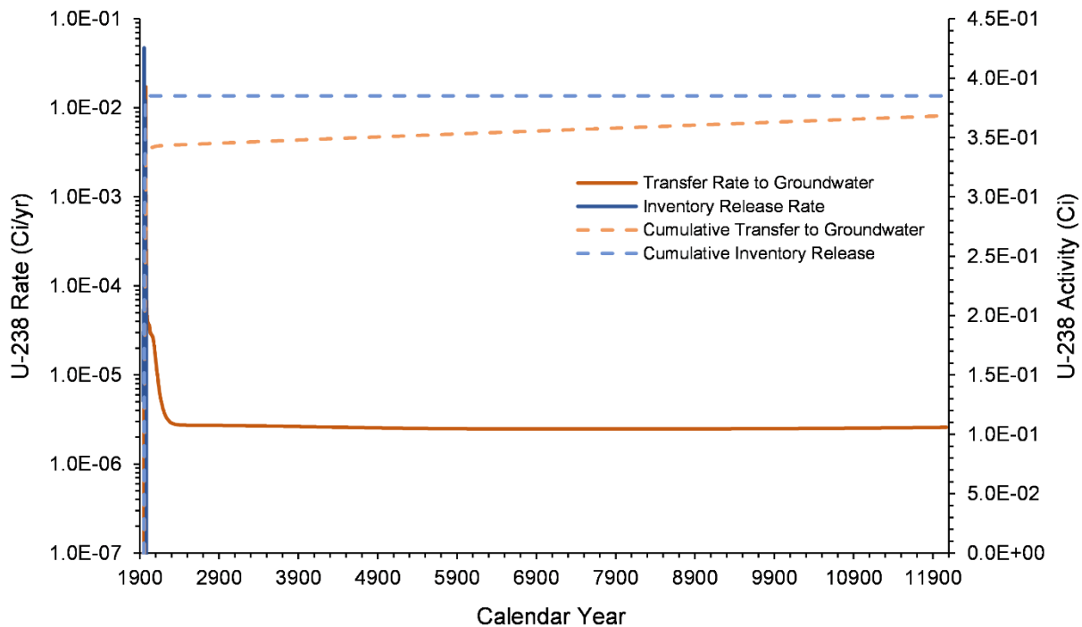
Figure 7-50. U-238 Inventory Release from Waste Sites and Transfer to Groundwater for the U-10 West Area Model from 1943–12070
