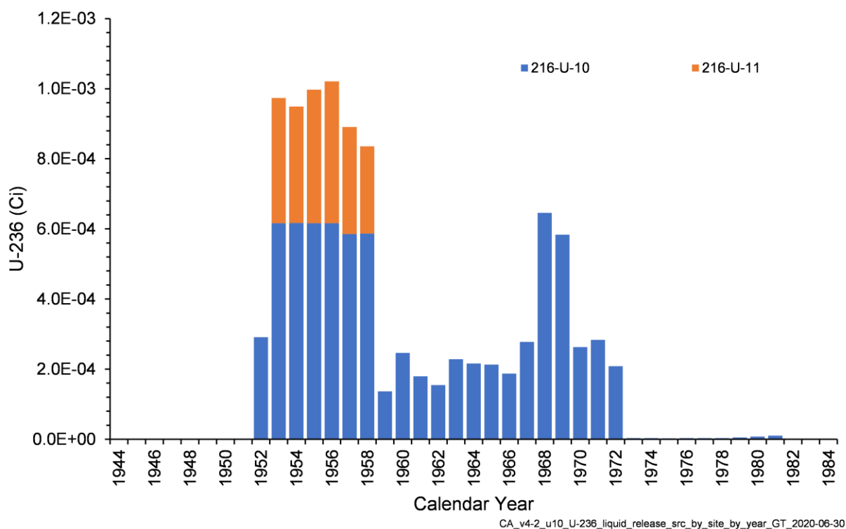
Figure 4-30. Annual U-236 Activity Released from Liquid Waste Sites in the U-10 West Area Model
