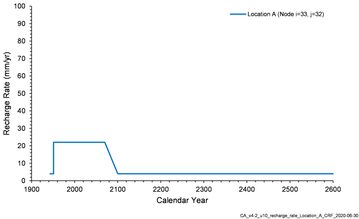
Figure 4-40. Time Series of Natural Recharge Rates, Location A
