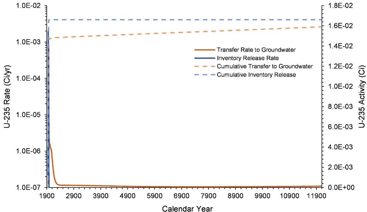
Figure 7-42. U-235 Inventory Release from Waste Sites and Transfer to Groundwater for the U-10 West Area Model from 1943–12070
