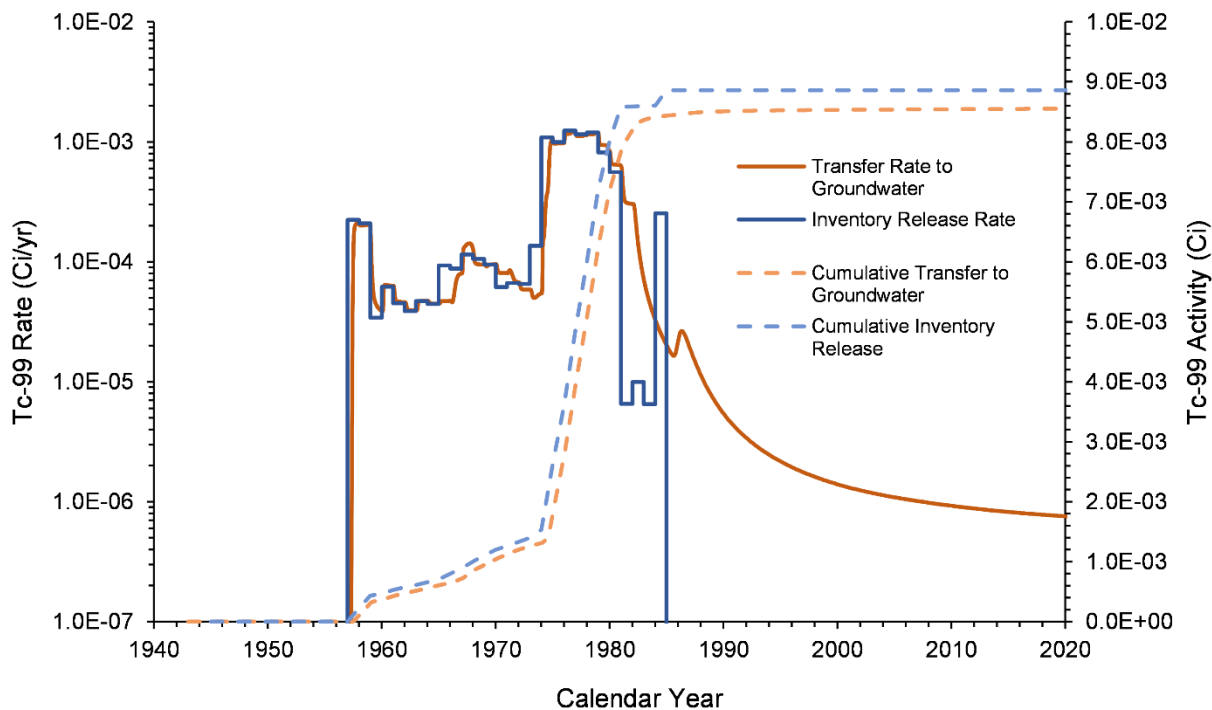
Figure 7-26. Tc-99 Inventory Release from Waste Sites and Transfer to Groundwater for the U-10 West Area Model from 1943–2018
