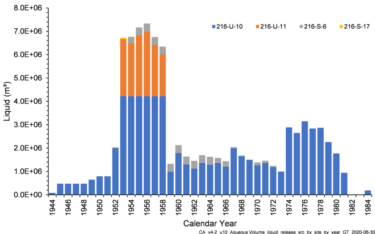
Figure 4-33. Total Volume of Water Released by Year from Liquid Waste Sites in the U-10 West Area Model
