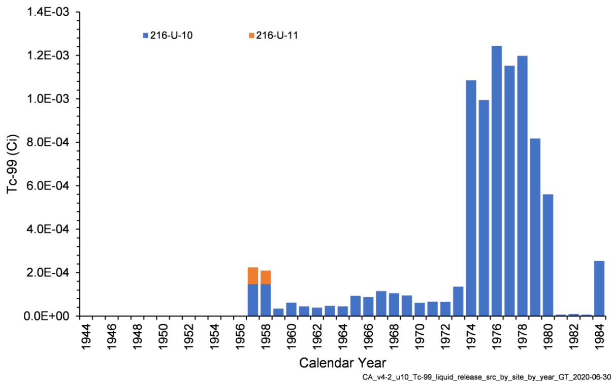
Figure 4-25. Annual Tc-99 Activity Released from Liquid Waste Sites in the U-10 West Area Model
