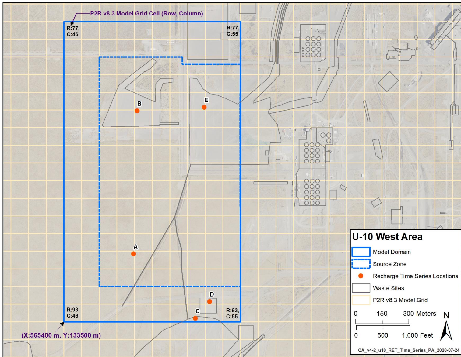
Figure 4-39. Locations of Recharge Rate Time Series Examples
