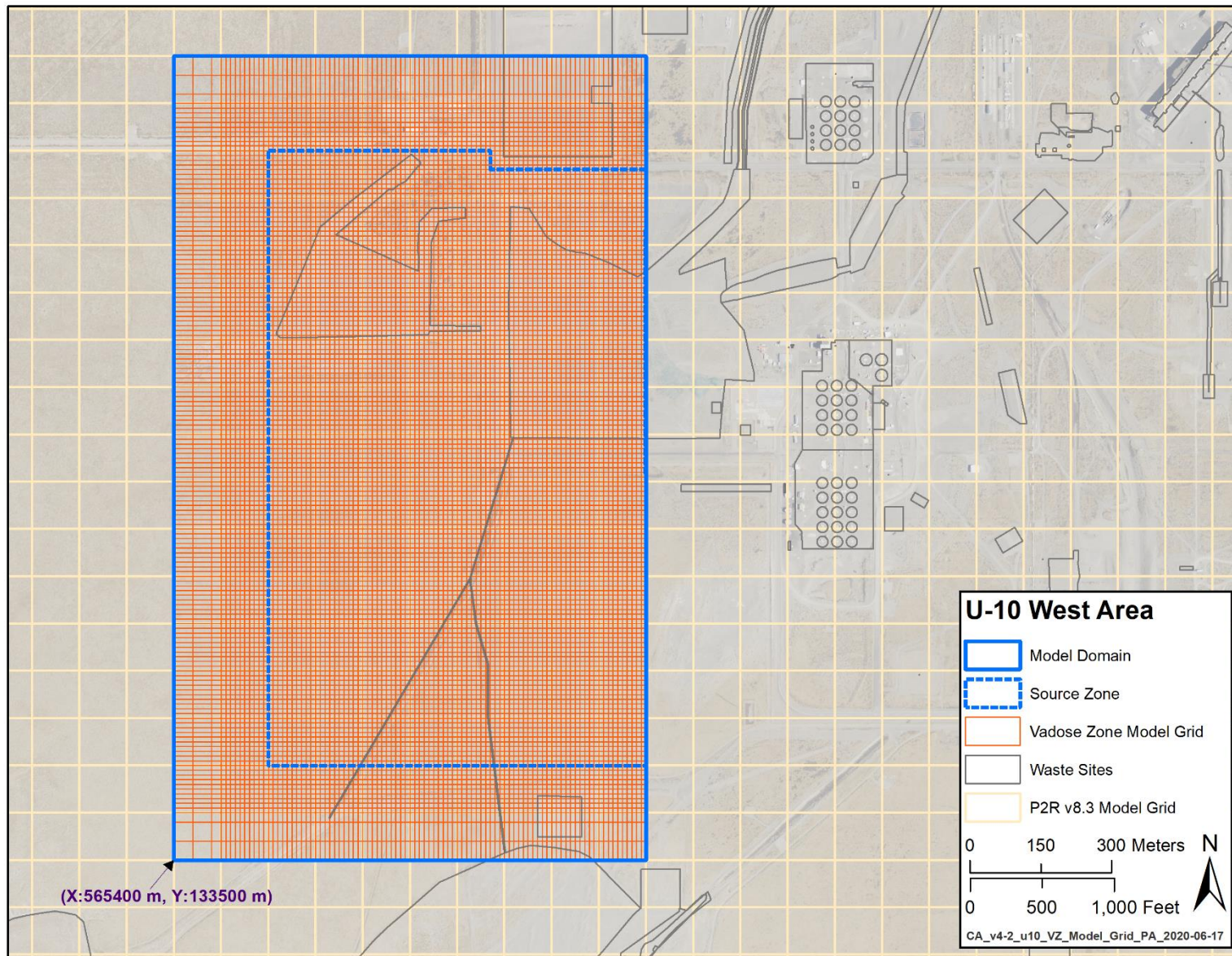
Figure 4-1. Plan View of the U-10 West Area Model Grid Overlain on the P2R Grid Cells
