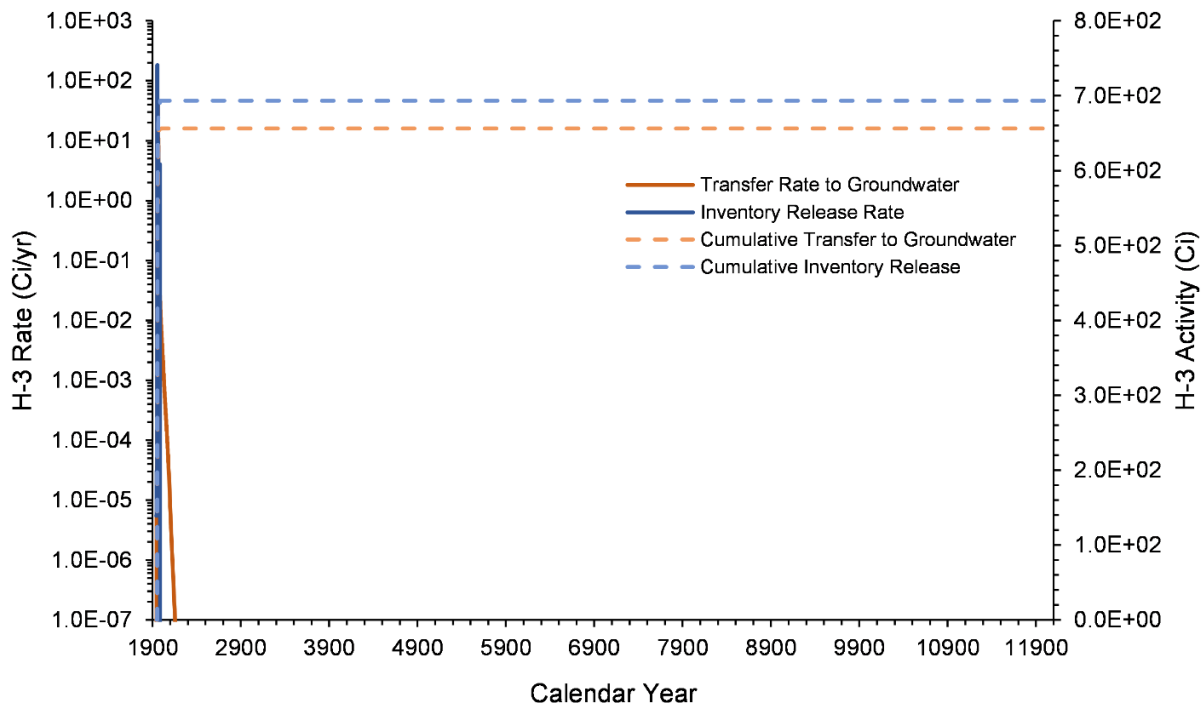
Figure 7-8. H-3 Inventory Release from Waste Sites and Transfer to Groundwater for the U-10 West Area Model from 1943–12070
