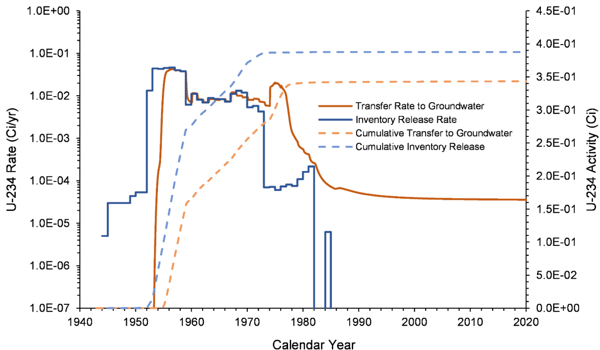
Figure 7-37. U-234 Inventory Release from Waste Sites and Transfer to Groundwater for the U-10 West Area Model from 1943–2018
