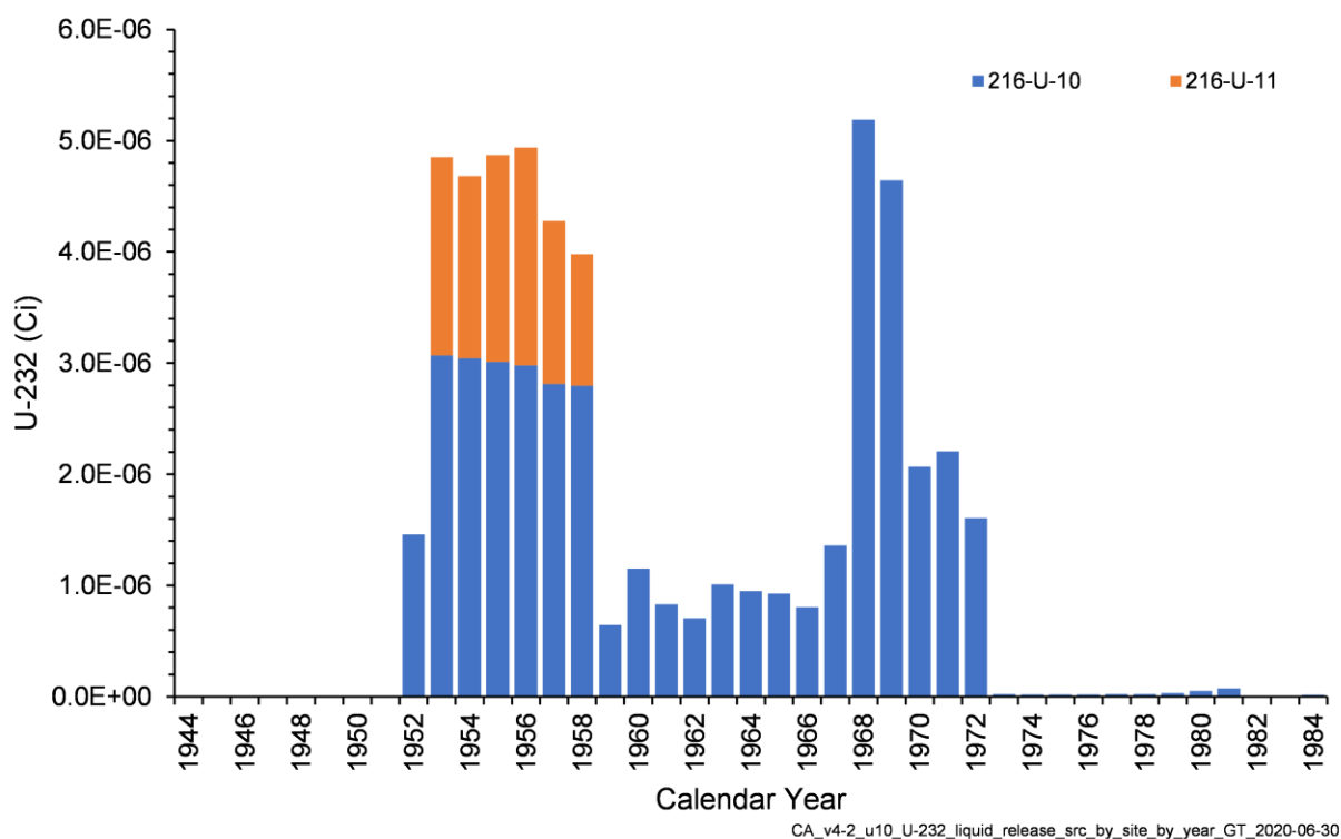
Figure 4-26. Annual U-232 Activity Released from Liquid Waste Sites in the U-10 West Area Model
