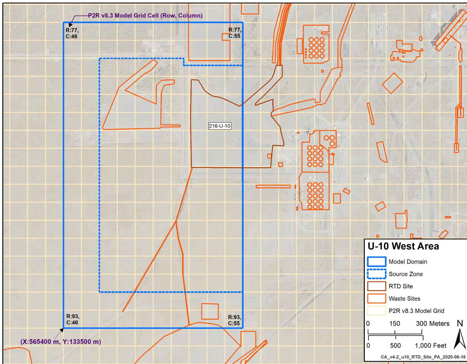
Figure 4-34. Map of the RTD Sites in the U-10 West Area Model
