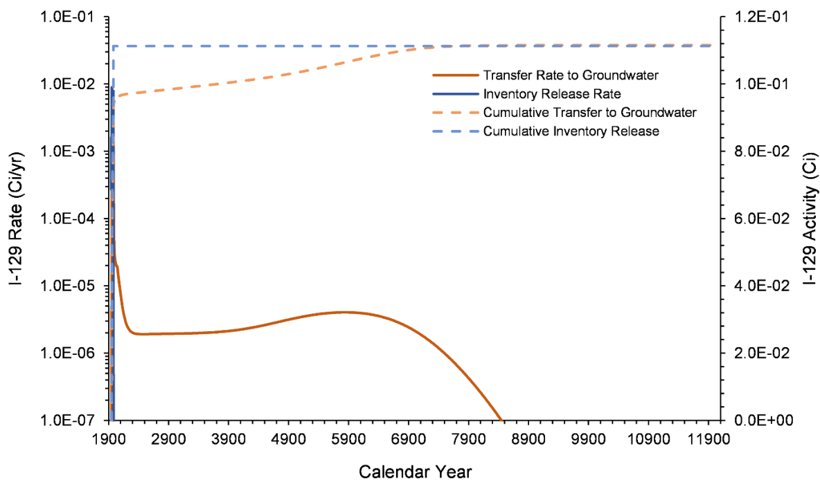
Figure 7-12. I-129 Inventory Release from Waste Sites and Transfer to Groundwater for the U-10 West Area Model from 1943–12070
