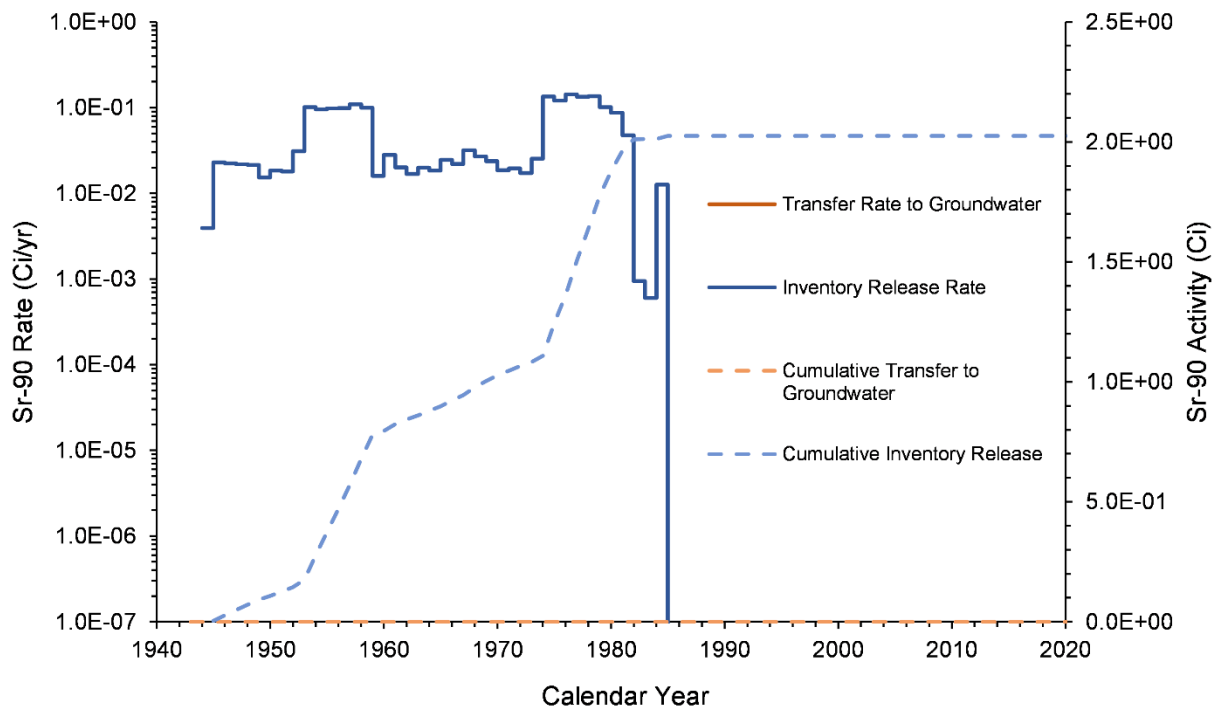
Figure 7-22. Sr-90 Inventory Release from Waste Sites and Transfer to Groundwater for the U-10 West Area Model from 1943–2018
