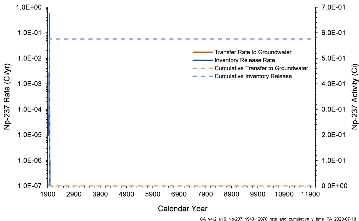
Figure 7-21. Np-237 Inventory Release from Waste Sites and Transfer to Groundwater for the U-10 West Area Model from 1943–12070
