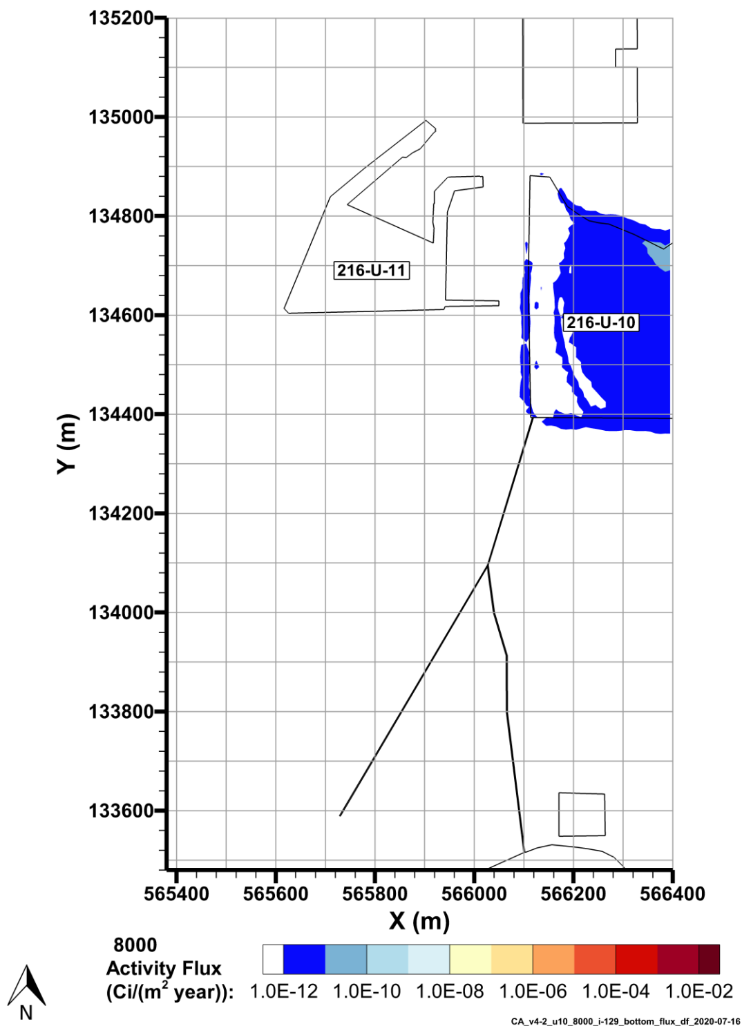
Figure 7-18. I-129 Flux to Groundwater, 8000
