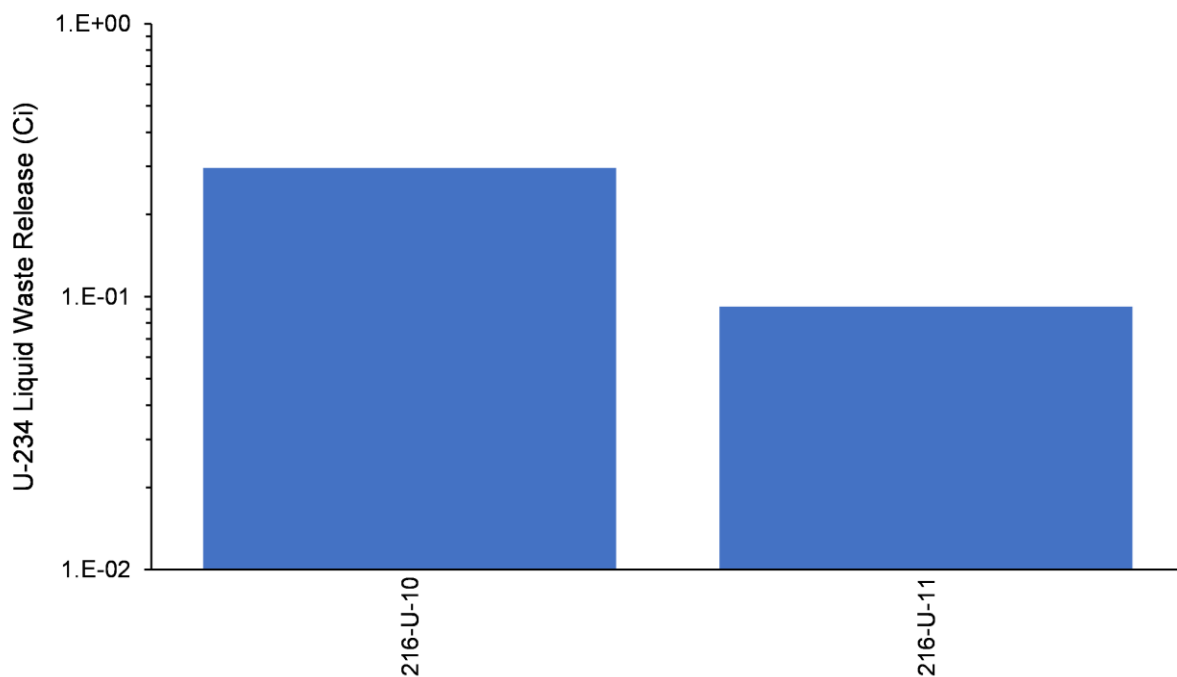
Figure 4-15. Total U-233 Activity Released from Liquid Waste Sites in the U-10 West Area Model
