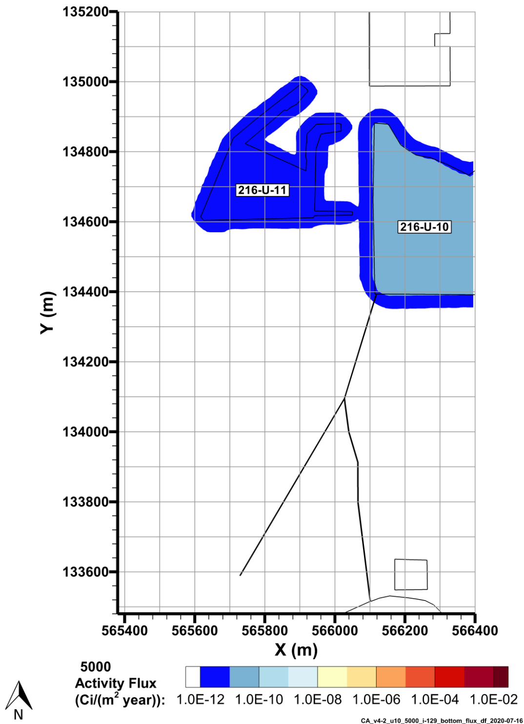
Figure 7-17. I-129 Flux to Groundwater, 5000
