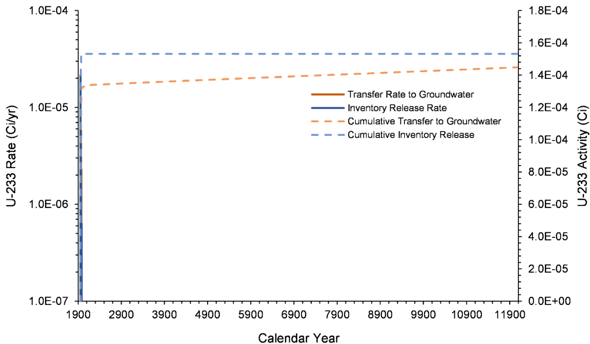
Figure 7-34. U-233 Inventory Release from Waste Sites and Transfer to Groundwater for the U-10 West Area Model from 1943–12070
