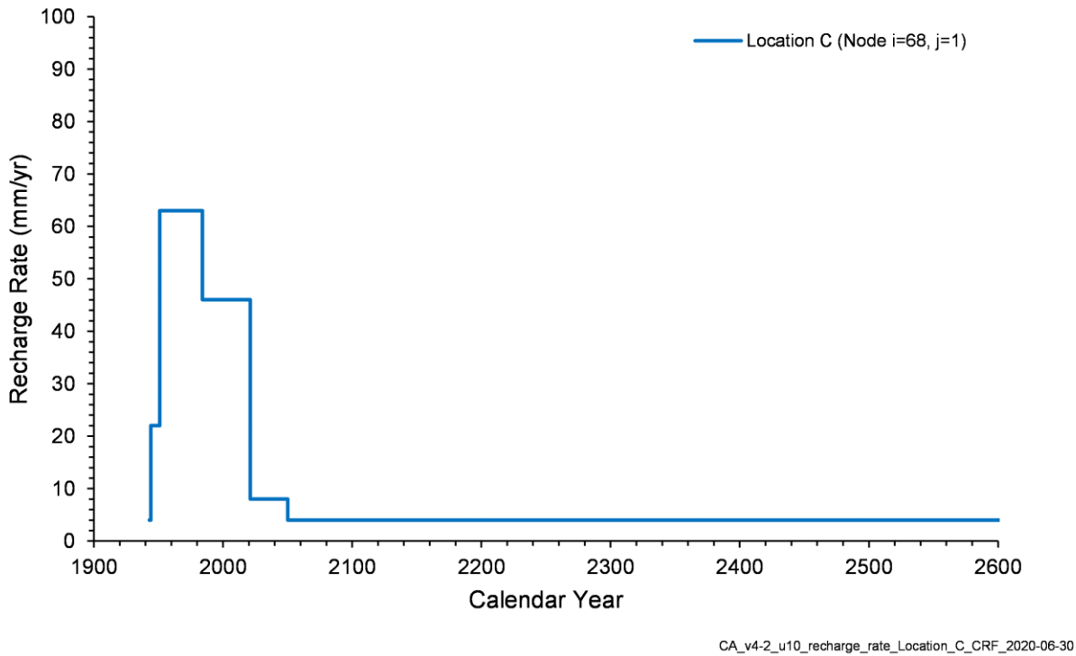
Figure 4-42. Time Series of Natural Recharge Rates, Location C
