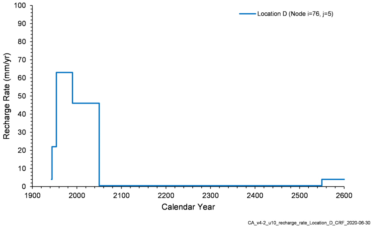
Figure 4-43. Time Series of Natural Recharge Rates, Location D
