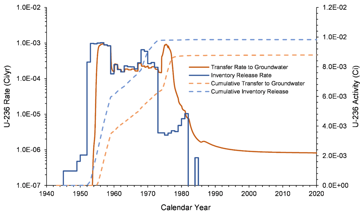
Figure 7-45. U-236 Inventory Release from Waste Sites and Transfer to Groundwater for the U-10 West Area Model from 1943–2018
