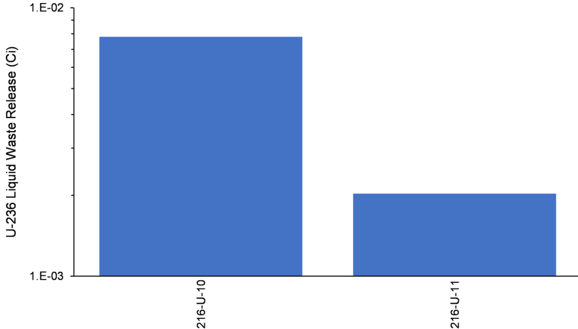
Figure 4-17. Total U-235 Activity Released from Liquid Waste Sites in the U-10 West Area Model
