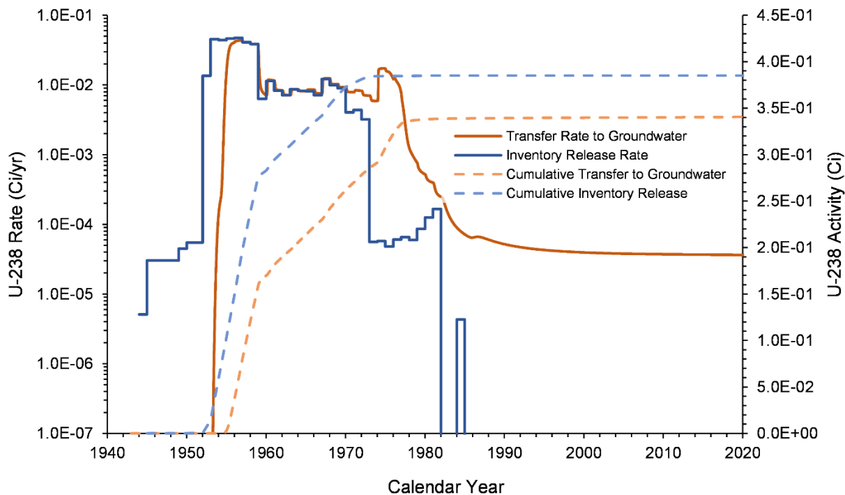
Figure 7-49. U-238 Inventory Release from Waste Sites and Transfer to Groundwater for the U-10 West Area Model from 1943–2018
