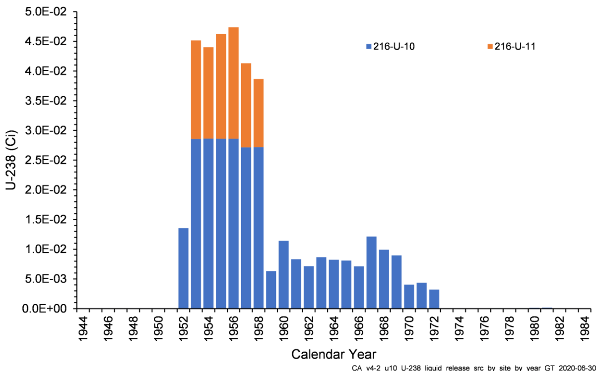
Figure 4-31. Annual U-238 Activity Released from Liquid Waste Sites in the U-10 West Area Model
