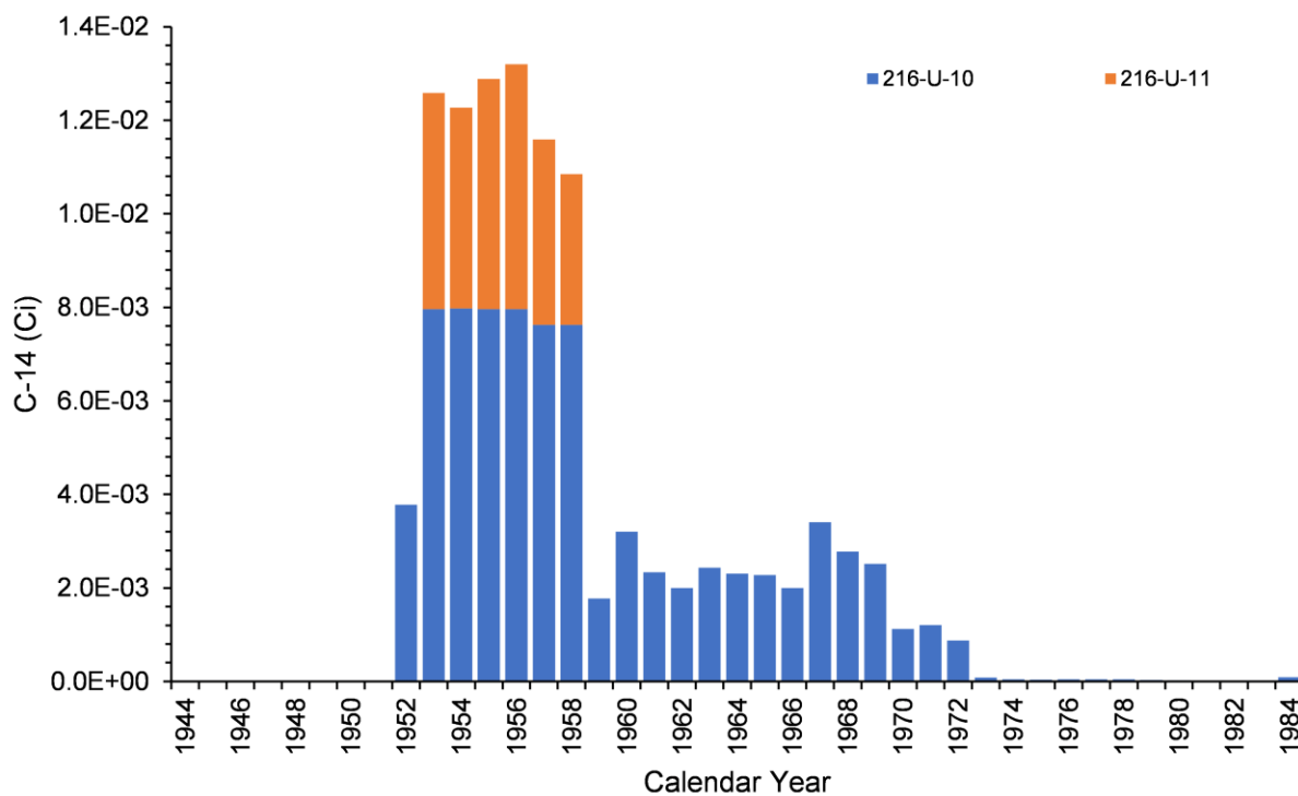
Figure 4-20. Annual C-14 Activity Released from Liquid Waste Sites in the U-10 West Area Model
