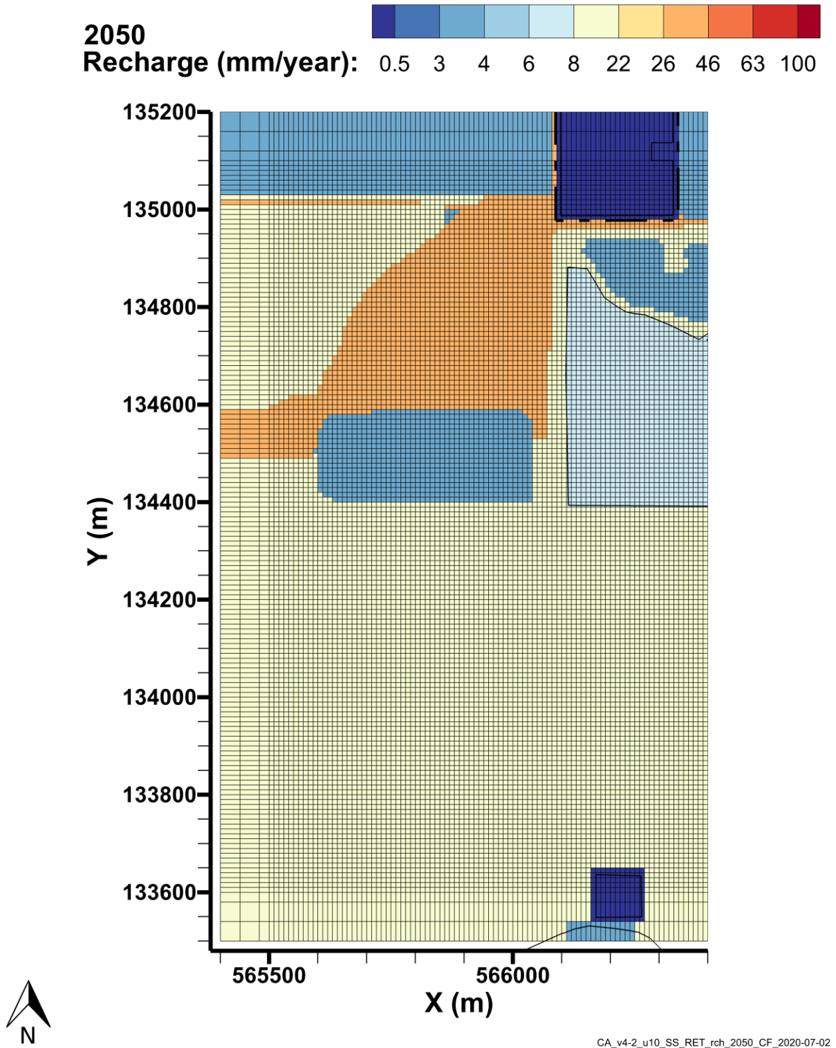
Figure 4-37. Transient Recharge Estimates for the U-10 West Area Model, 2050
