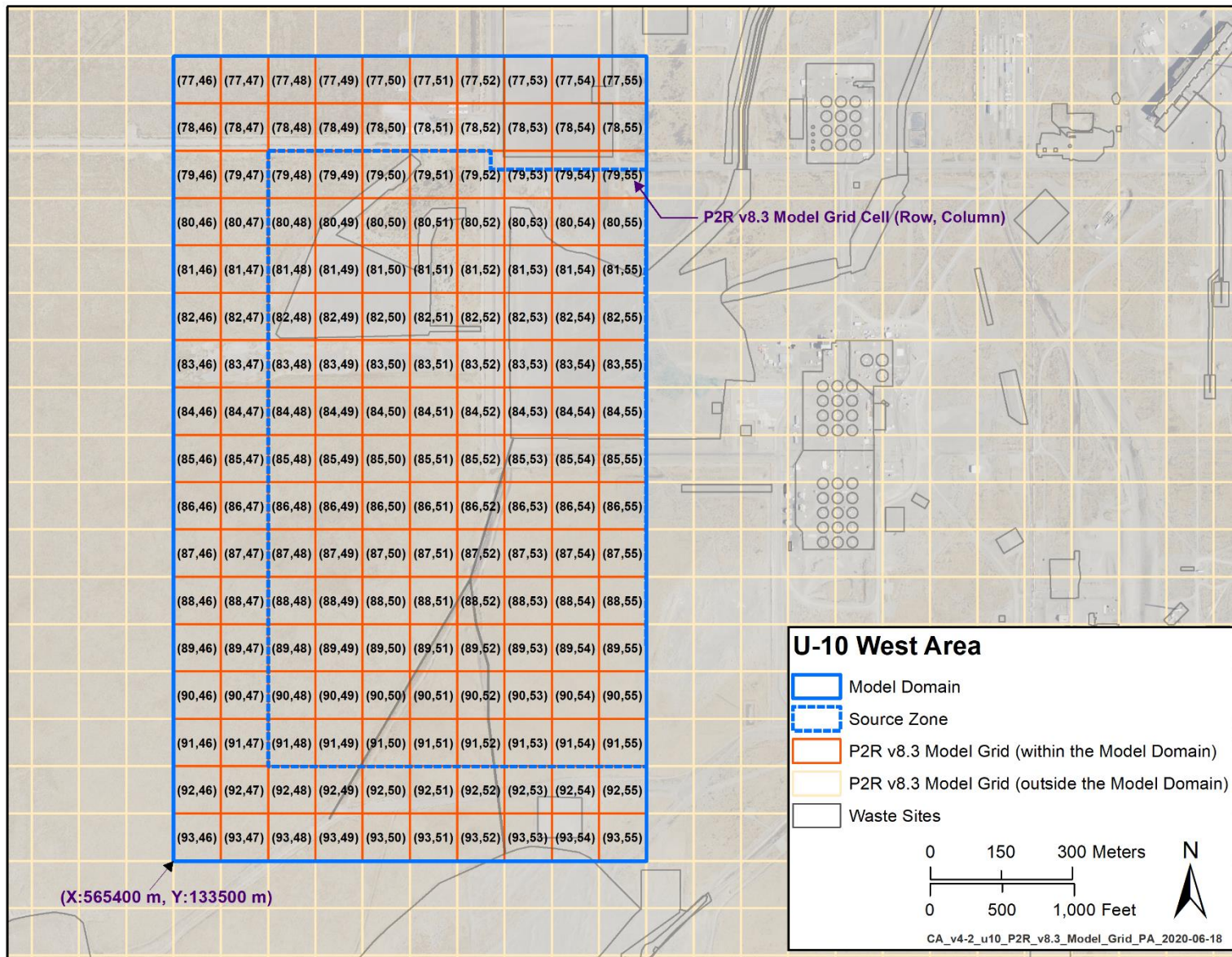
Figure 4-2. Plan View of the P2R Grid Cells in the U-10 West Area Model
