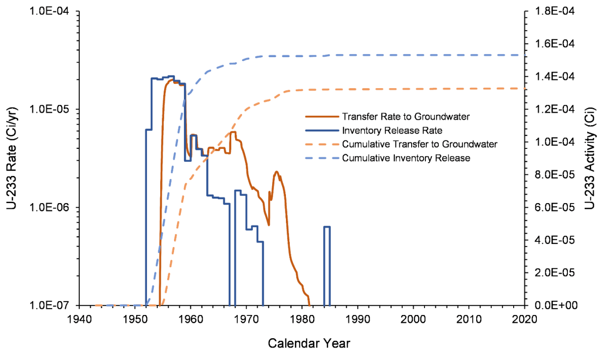
Figure 7-33. U-233 Inventory Release from Waste Sites and Transfer to Groundwater for the U-10 West Area Model from 1943–2018
