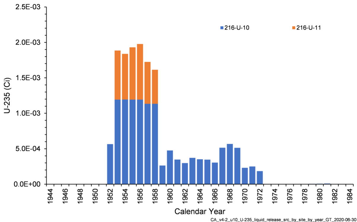
Figure 4-29. Annual U-235 Activity Released from Liquid Waste Sites in the U-10 West Area Model
