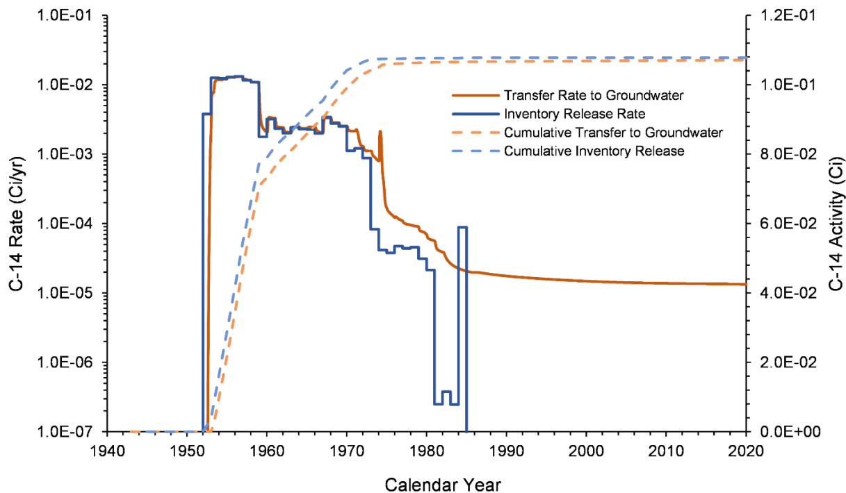
Figure 7-3. C-14 Inventory Release from Waste Sites and Transfer to Groundwater for the U-10 West Area Model from 1943–2018
