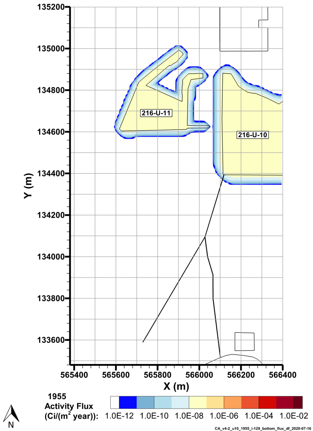
Figure 7-13. I-129 Flux to Groundwater, 1955
