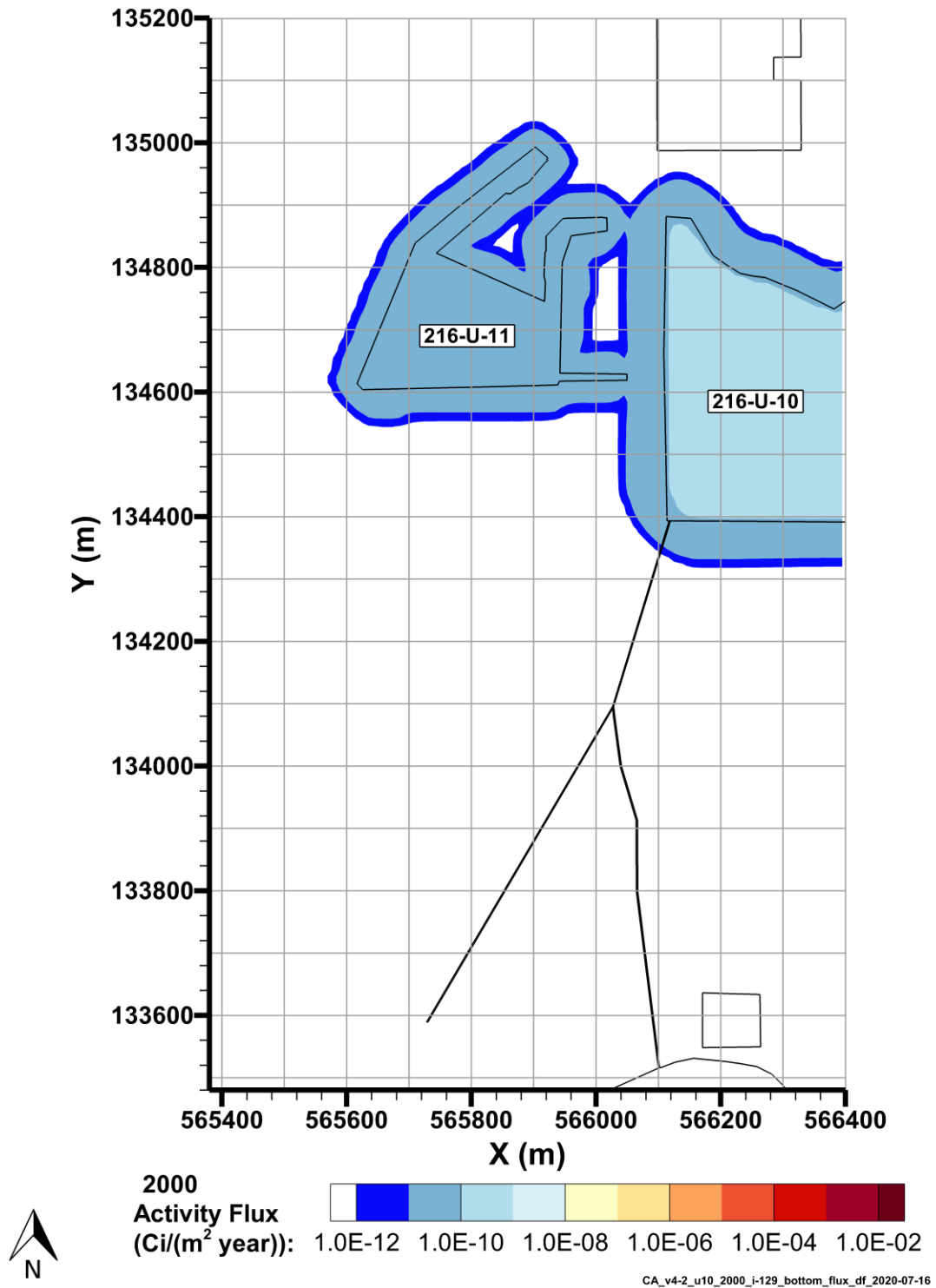
Figure 7-15. I-129 Flux to Groundwater, 2000
