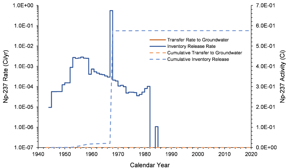
Figure 7-20. Np-237 Inventory Release from Waste Sites and Transfer to Groundwater for the U-10 West Area Model from 1943–2018
