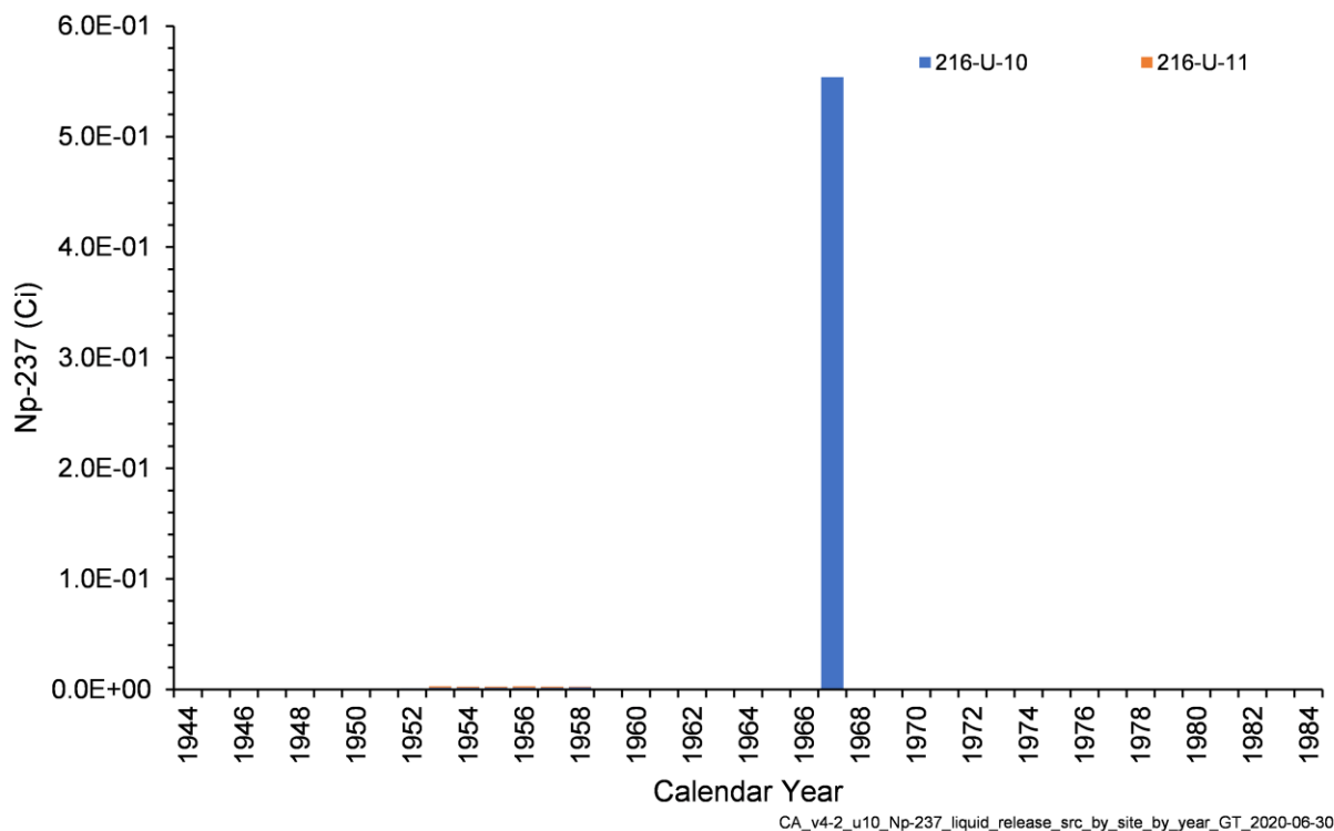
Figure 4-23. Annual Np-237 Activity Released from Liquid Waste Sites in the U-10 West Area Model
