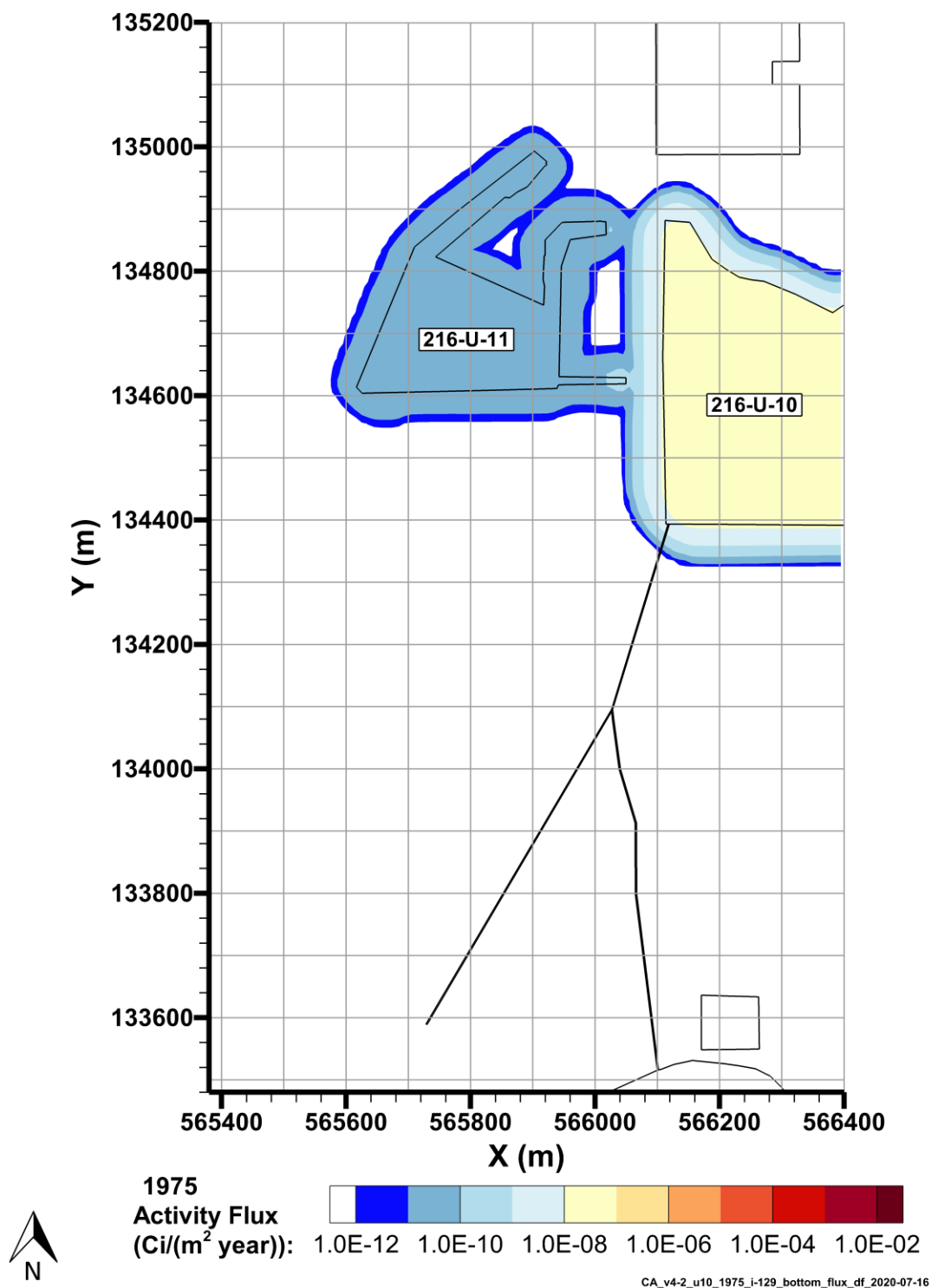
Figure 7-14. I-129 Flux to Groundwater, 1975
