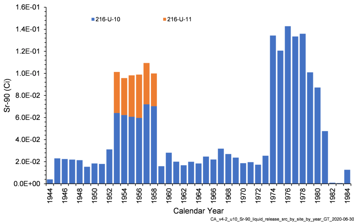
Figure 4-24. Annual Sr-90 Activity Released from Liquid Waste Sites in the U-10 West Area Model
