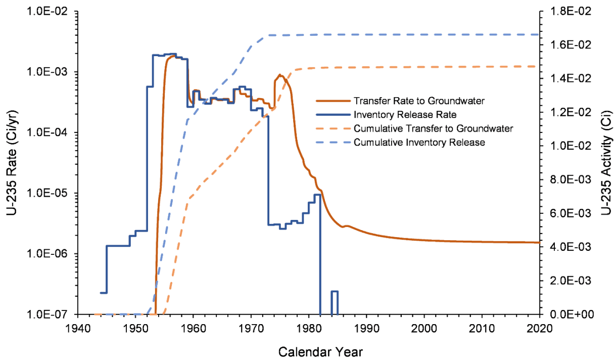
Figure 7-41. U-235 Inventory Release from Waste Sites and Transfer to Groundwater for the U-10 West Area Model from 1943–2018
