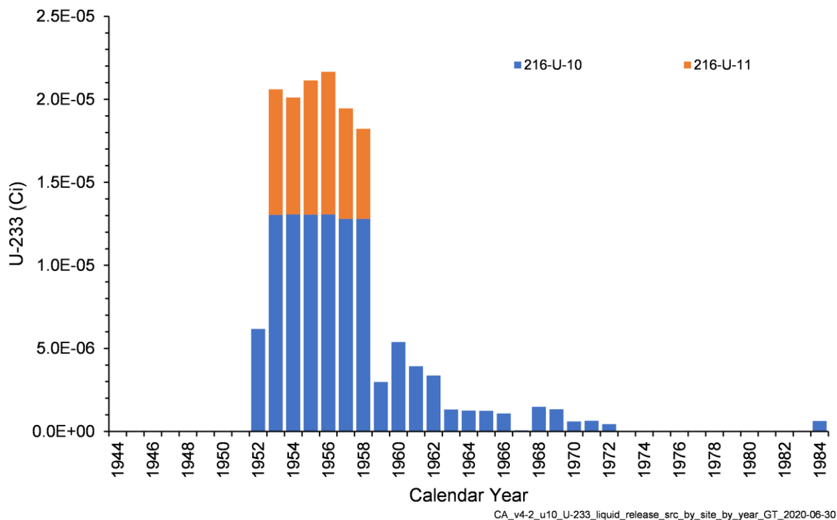
Figure 4-27. Annual U-233 Activity Released from Liquid Waste Sites in the U-10 West Area Model
