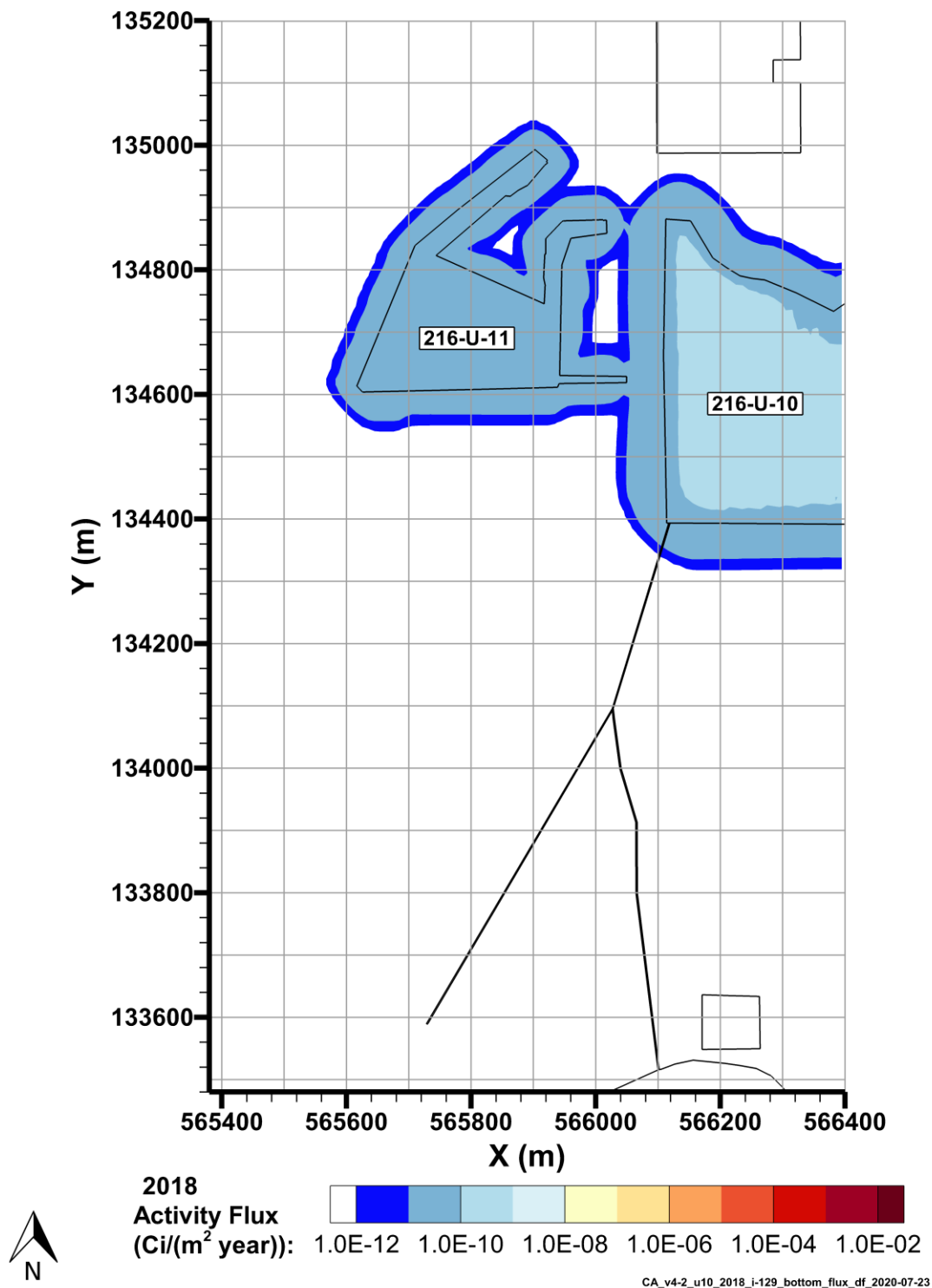
Figure 7-16. I-129 Flux to Groundwater, 2018
