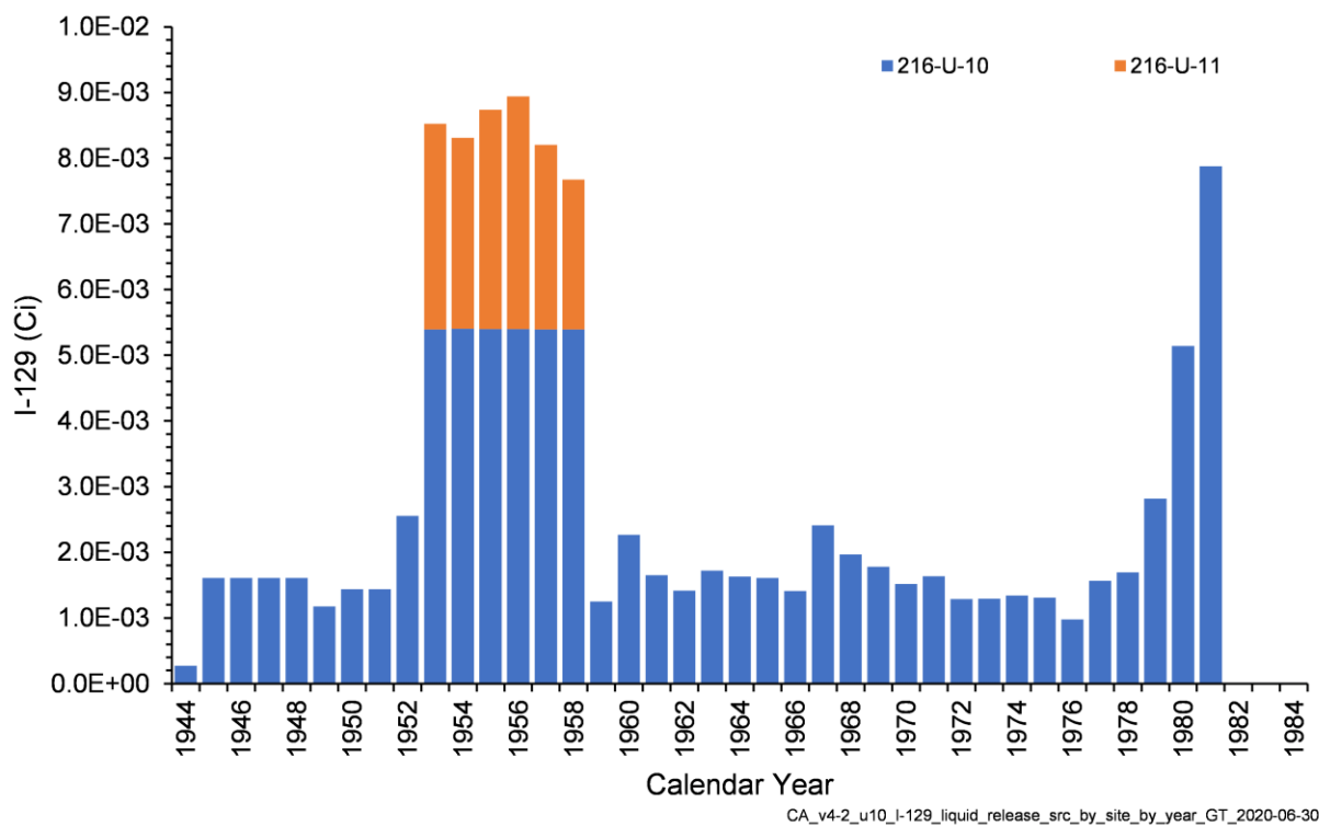
Figure 4-22. Annual I-129 Activity Released from Liquid Waste Sites in the U-10 West Area Model
