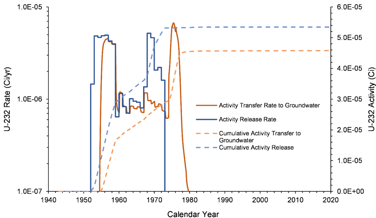
Figure 7-29. U-232 Inventory Release from Waste Sites and Transfer to Groundwater for the U-10 West Area Model from 1943–2018
