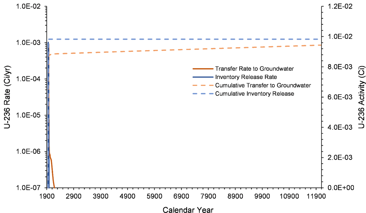
Figure 7-46. U-236 Inventory Release from Waste Sites and Transfer to Groundwater for the U-10 West Area Model from 1943–12070
