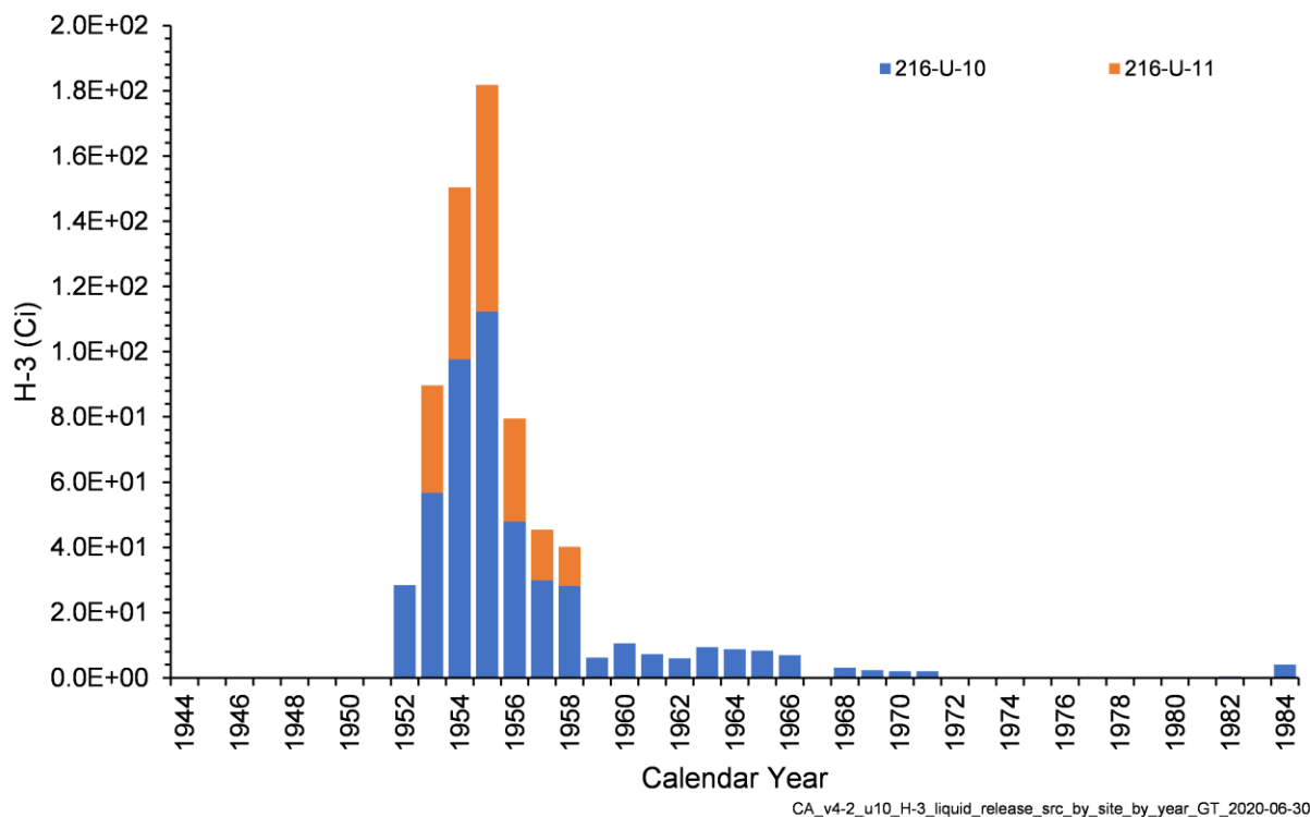
Figure 4-21. Annual H-3 Activity Released from Liquid Waste Sites in the U-10 West Area Model
