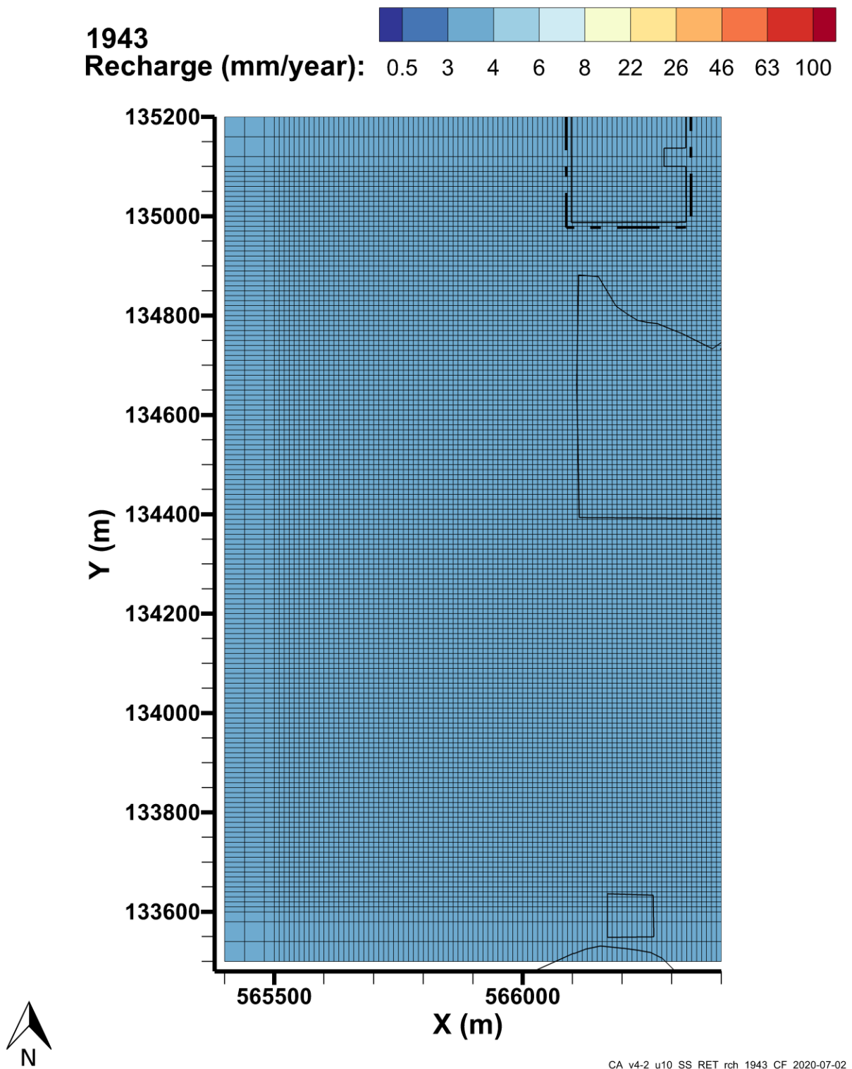
Figure 4-35. Transient Recharge Estimates for the U-10 West Area Model, 1943
