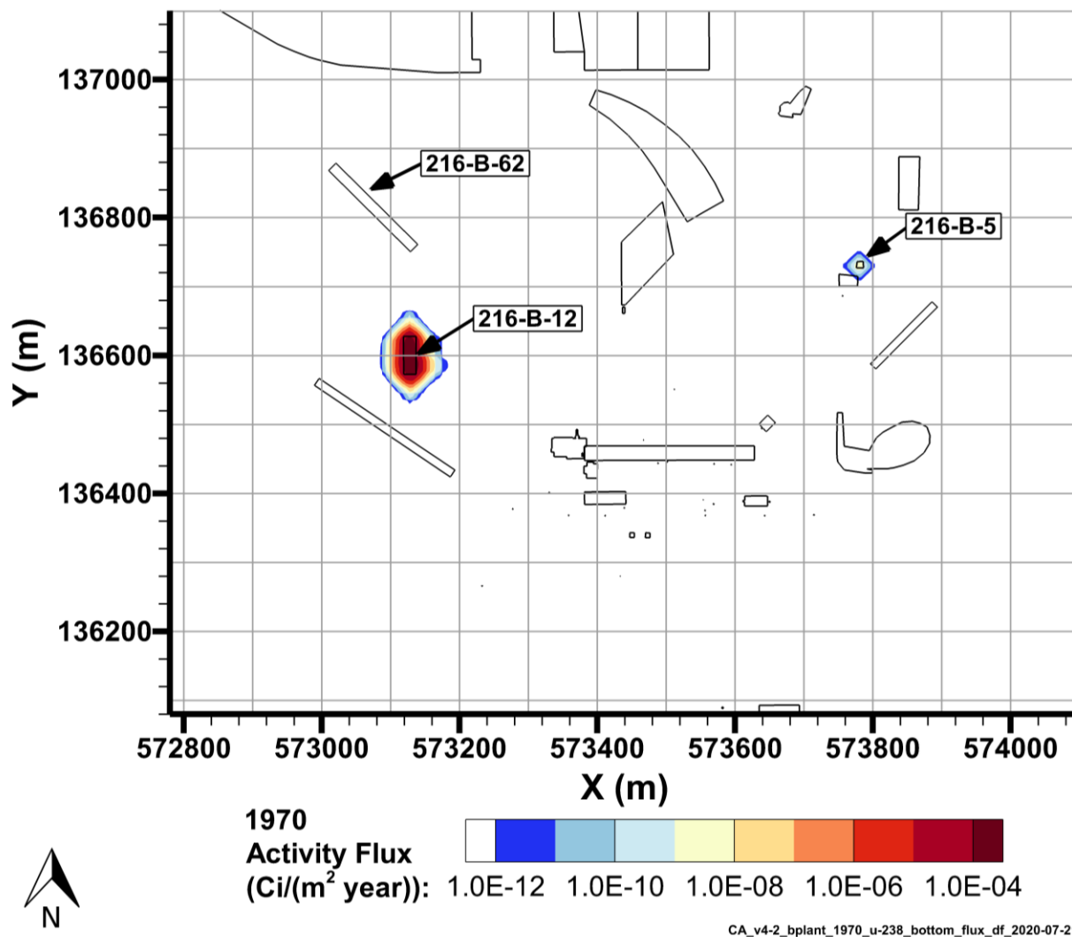
Figure 7-59. U-238 Flux to Groundwater, 1970
