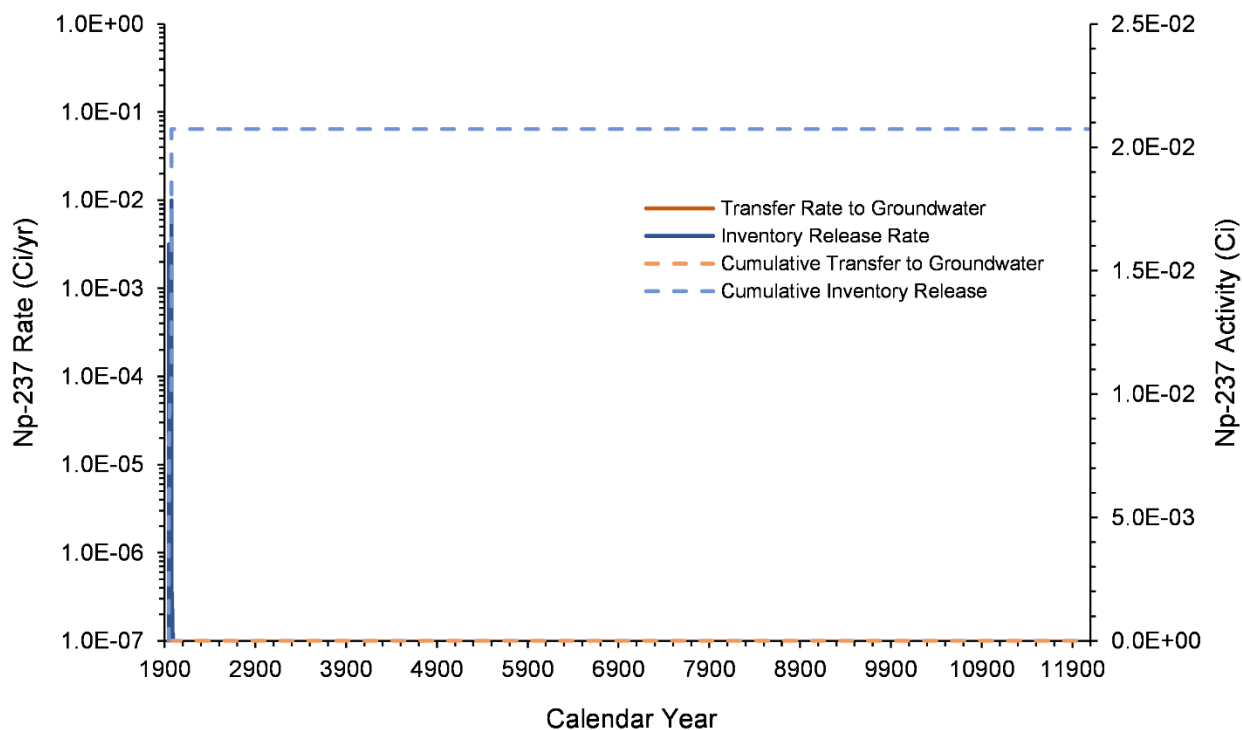
Figure 7-21. Np-237 Inventory Release from Waste Sites and Transfer to Groundwater for the B Plant Area Model from 1943–12070
