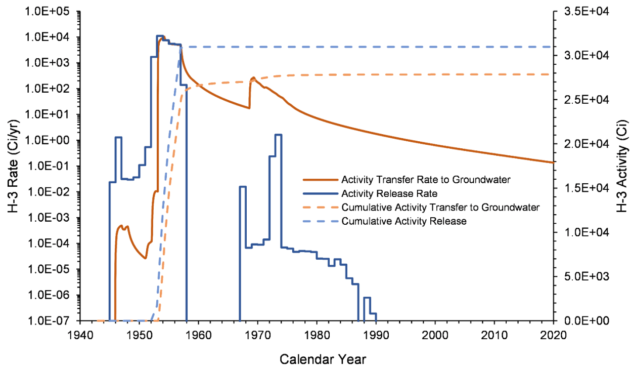
Figure 7-7. Cumulative H-3 Activity Released and Transfer Rate to Groundwater from the B Plant Area Model from 1943–2018
