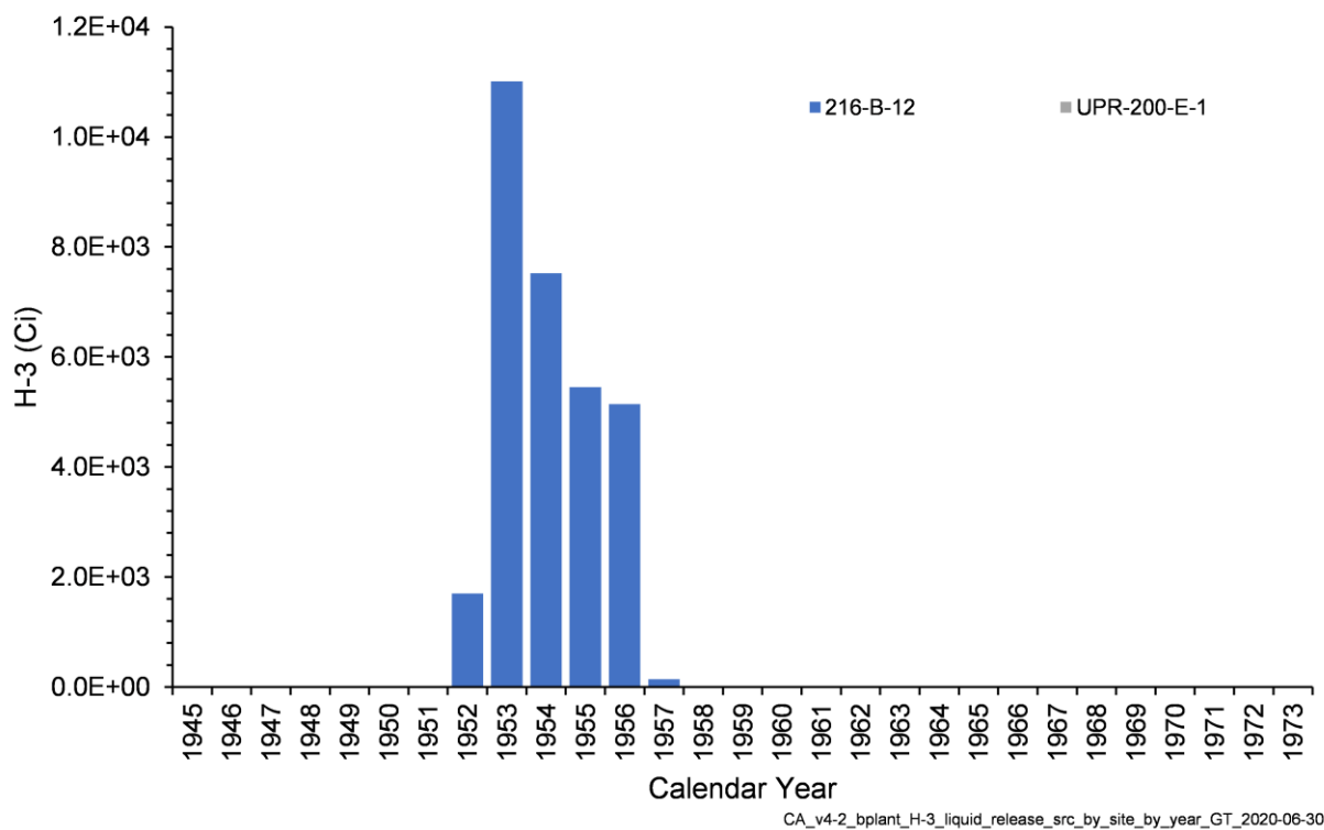
Figure 4-21. Annual H-3 Activity Released from Liquid Waste Sites in the B Plant Area Model
