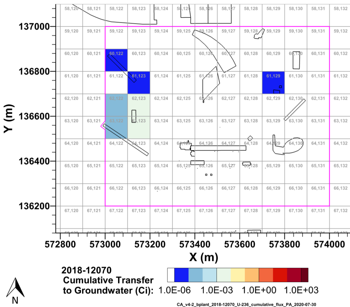
Figure 7-50. Cumulative U-236 Activity Discharged to Groundwater from the B Plant Area Model from 2018–12070 per P2R Grid Cell
