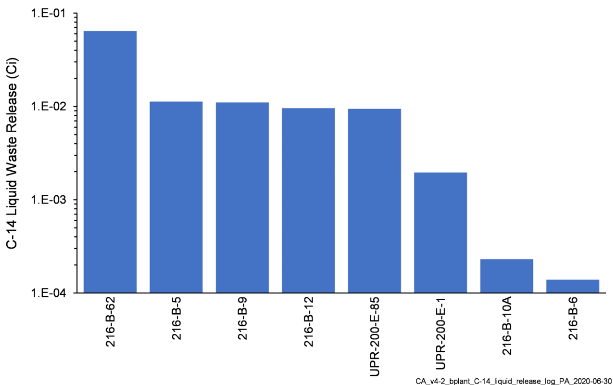
Figure 4-9. Total C-14 Activity Released from Liquid Waste Sites in the B Plant Area Model
