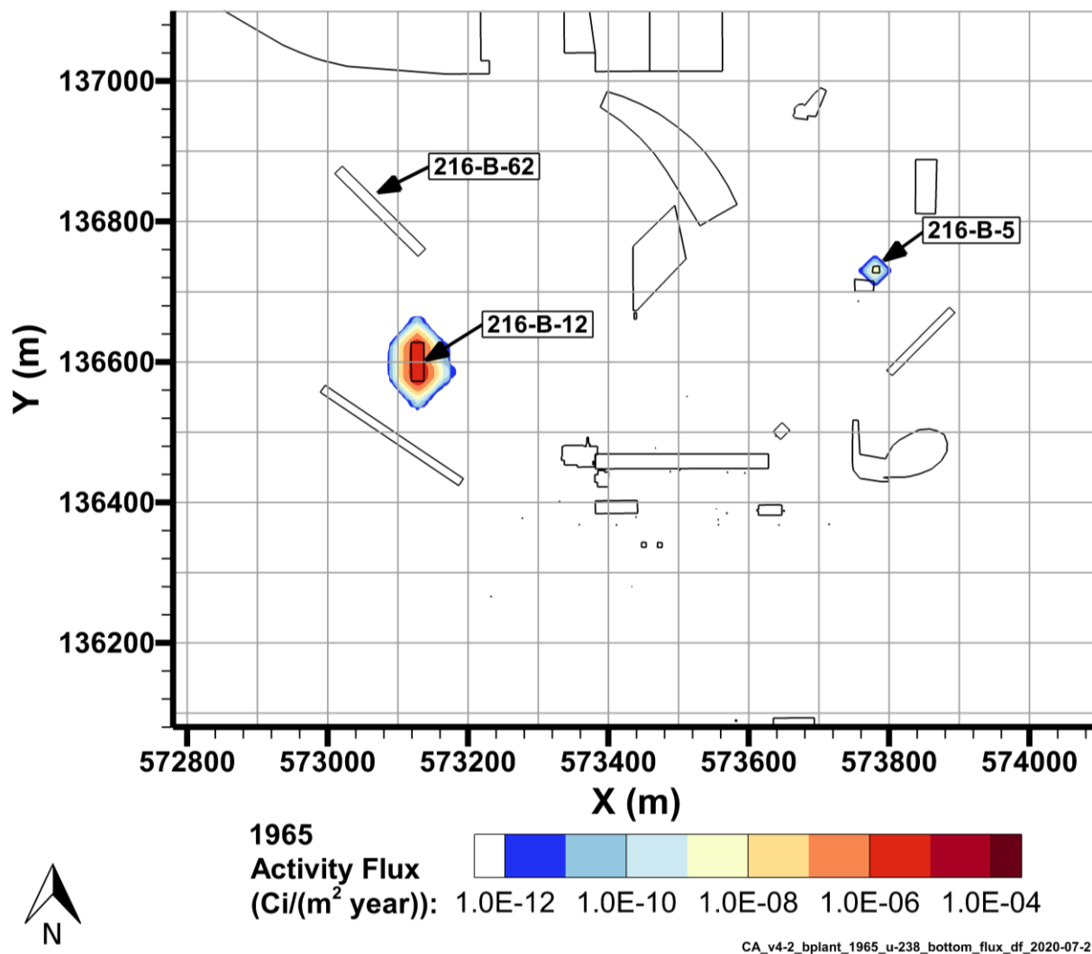
Figure 7-58. U-238 Flux to Groundwater, 1965
