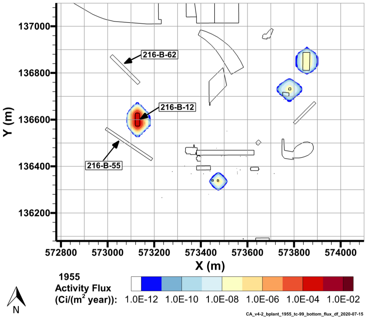
Figure 7-28. Tc-99 Flux to Groundwater, 1955
