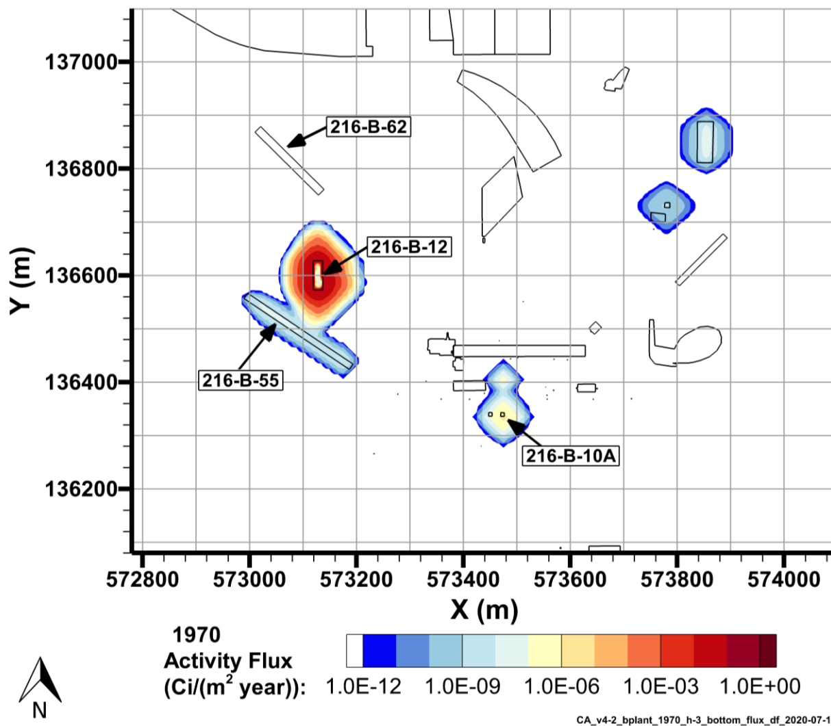
Figure 7-10. H-3 Flux to Groundwater, 1970
