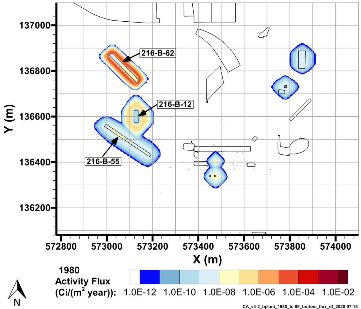
Figure 7-30. Tc-99 Flux to Groundwater, 1980
