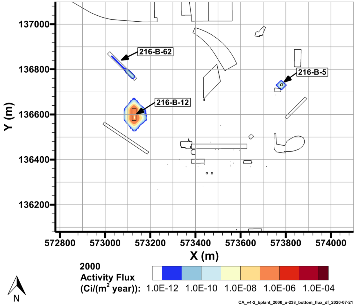
Figure 7-60. U-238 Flux to Groundwater, 2000
