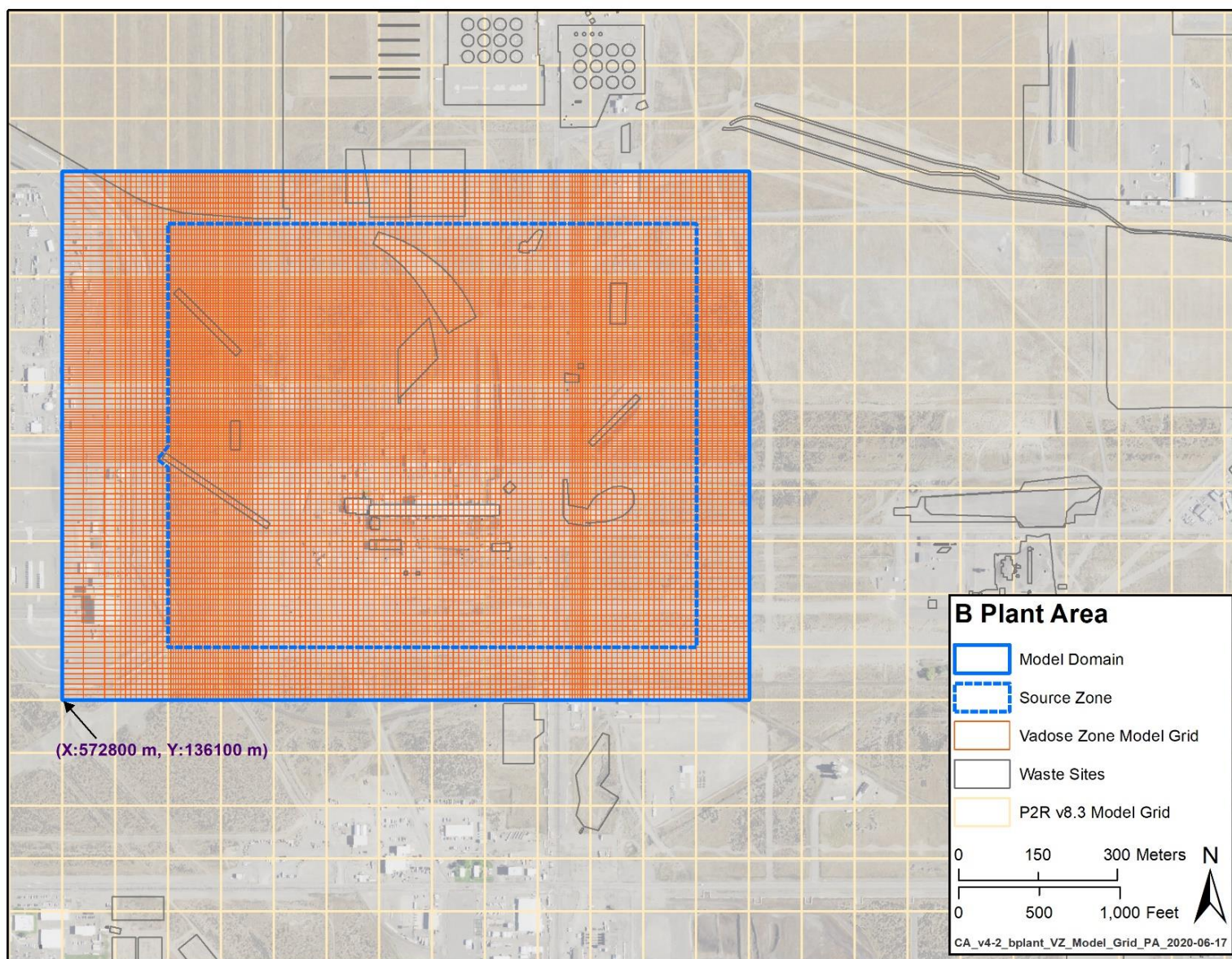
Figure 4-1. Plan View of the B Plant Area Model Grid Overlain on the P2R Grid Cells
