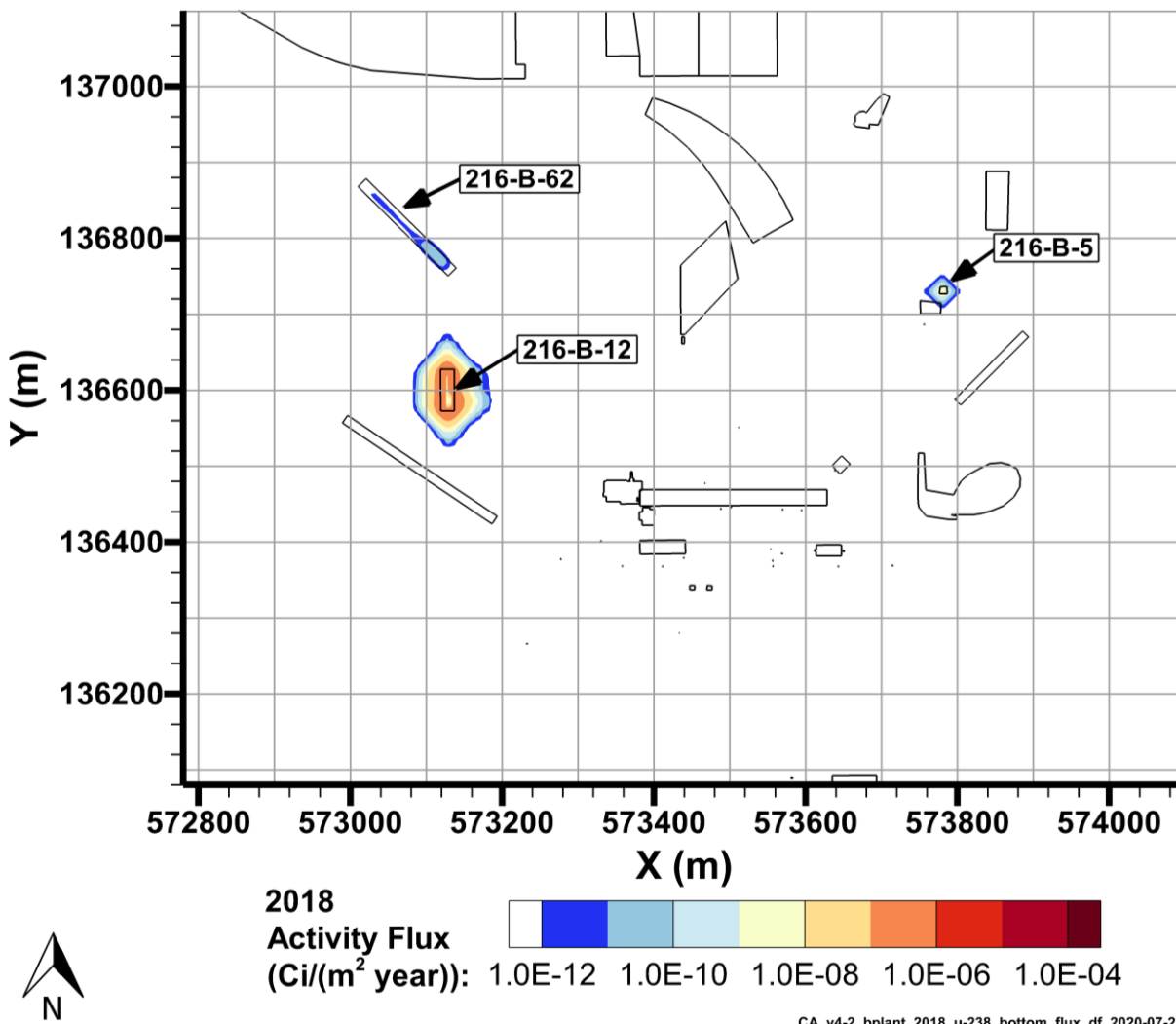
Figure 7-61. U-238 Flux to Groundwater, 2018
