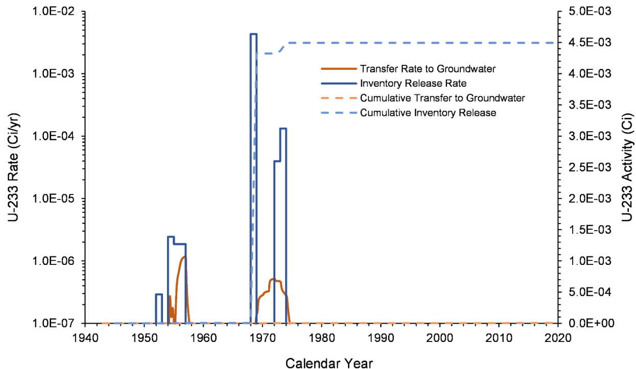
Figure 7-39. U-233 Inventory Release from Waste Sites and Transfer to Groundwater for the B Plant Area Model from 1943–2018
