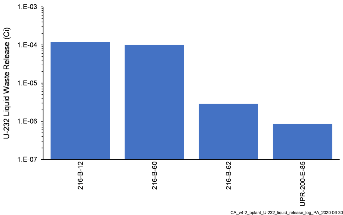
Figure 4-15. Total U-232 Activity Released from Liquid Waste Sites in the B Plant Area Model
