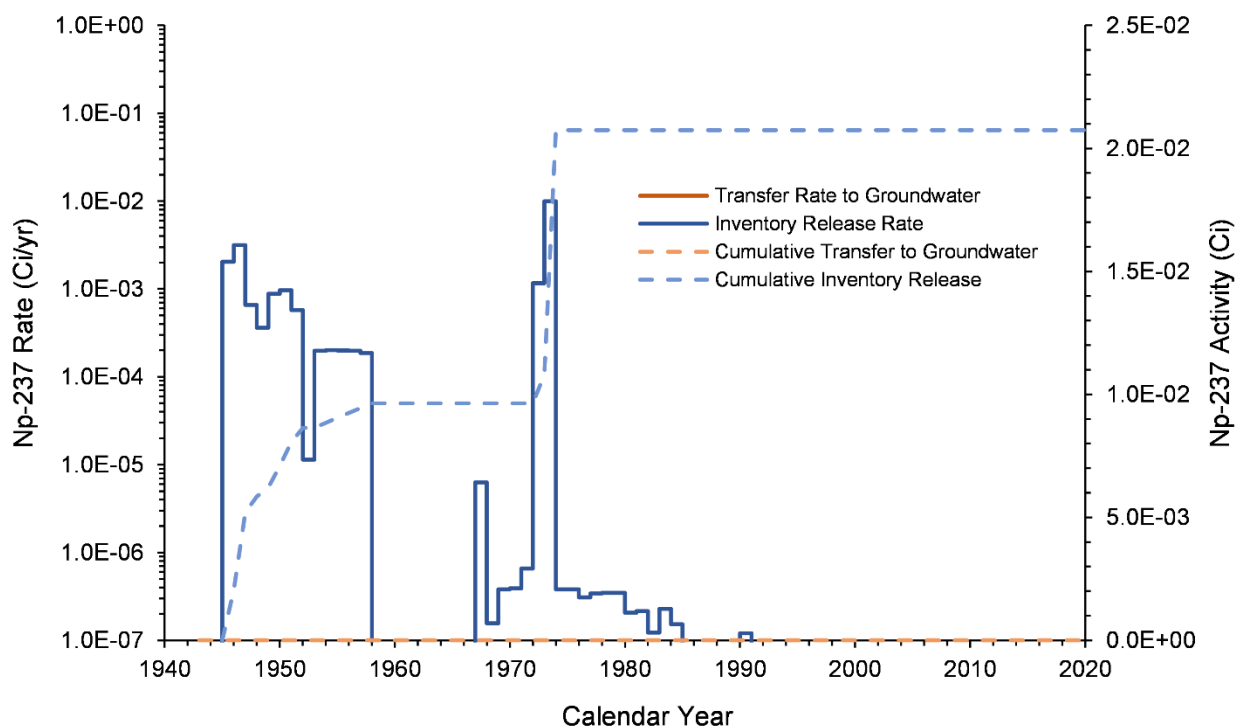
Figure 7-20. Np-237 Inventory Release from Waste Sites and Transfer to Groundwater for the B Plant Area Model from 1943–2018
