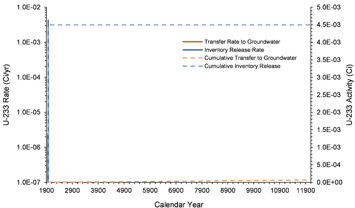
Figure 7-40. U-233 Inventory Release from Waste Sites and Transfer to Groundwater for the B Plant Area Model from 1943–12070
