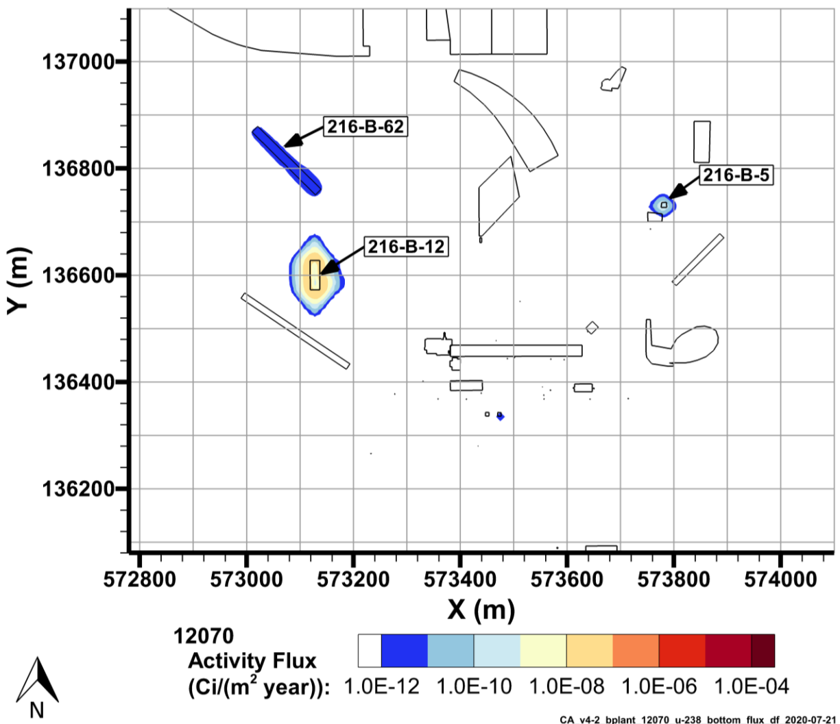
Figure 7-63. U-238 Flux to Groundwater, 12070
