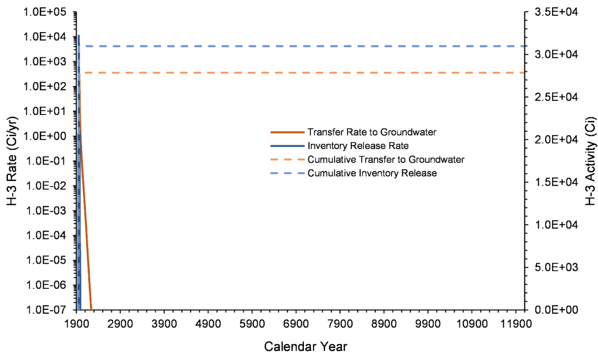
Figure 7-8. Cumulative H-3 Activity Released and Transfer Rate to Groundwater from the B Plant Area Model from 1943–12070
