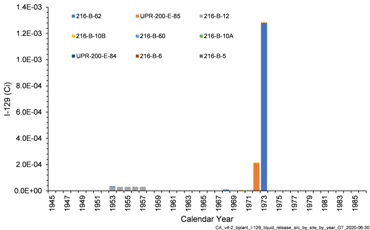
Figure 4-22. Annual I-129 Activity Released from Liquid Waste Sites in the B Plant Area Model
