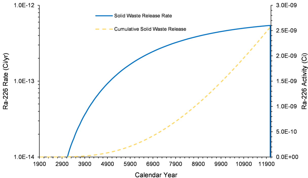
Figure 4-44. Ra-226 Release Rate and Cumulative Activity from Solid Waste in the B Plant Area Model, 1943–12070
