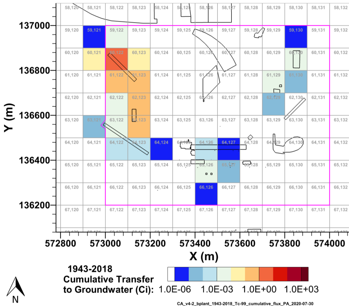
Figure 7-24. Cumulative Tc-99 Activity Discharged to Groundwater from the B Plant Area Model from 1943–2018 per P2R Grid Cell
