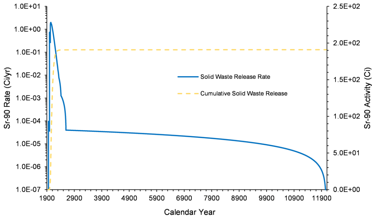
Figure 4-42. Sr-90 Release Rate and Cumulative Activity from Solid Waste in the B Plant Area Model, 1943–12070
