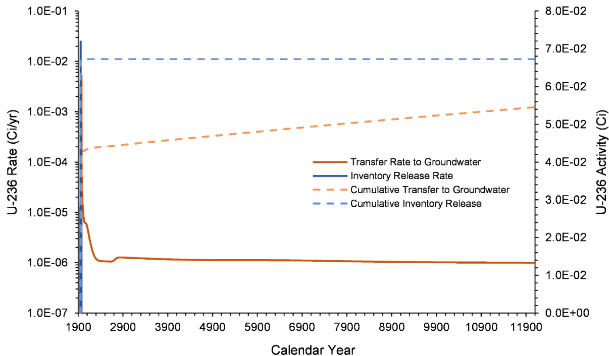
Figure 7-52. U-236 Inventory Release from Waste Sites and Transfer to Groundwater for the B Plant Area Model from 1943–12070
