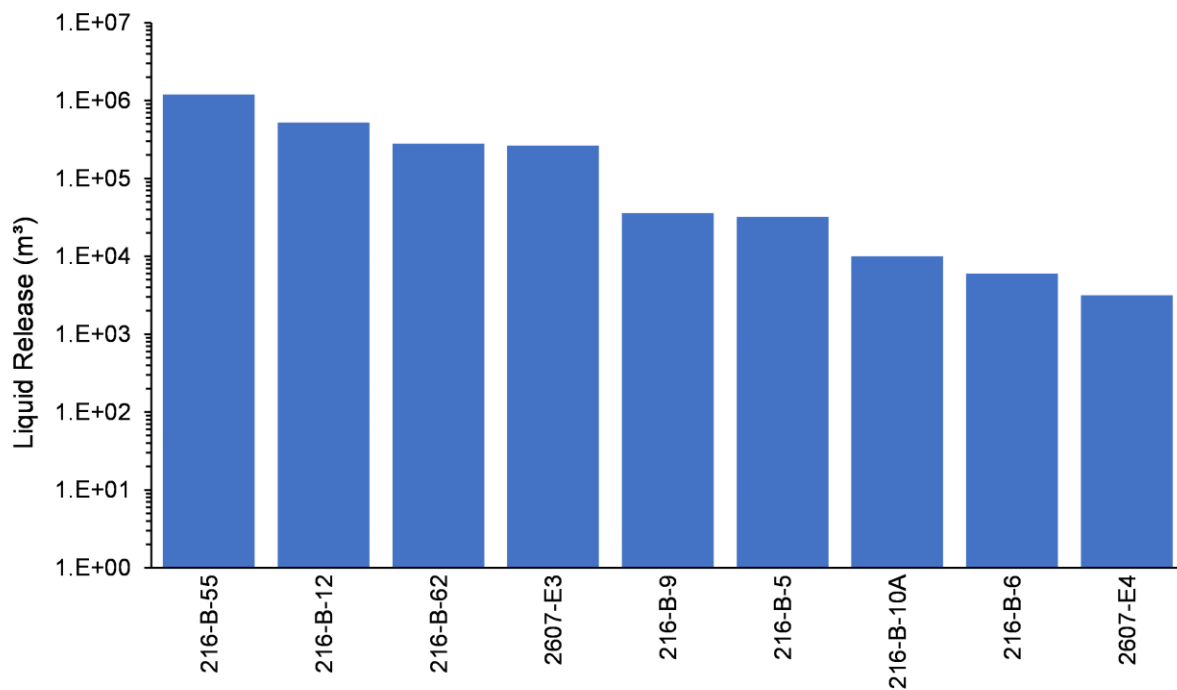
Figure 4-56. Total Volume of Water Released from Liquid Waste Sites in the B Plant Area Model
