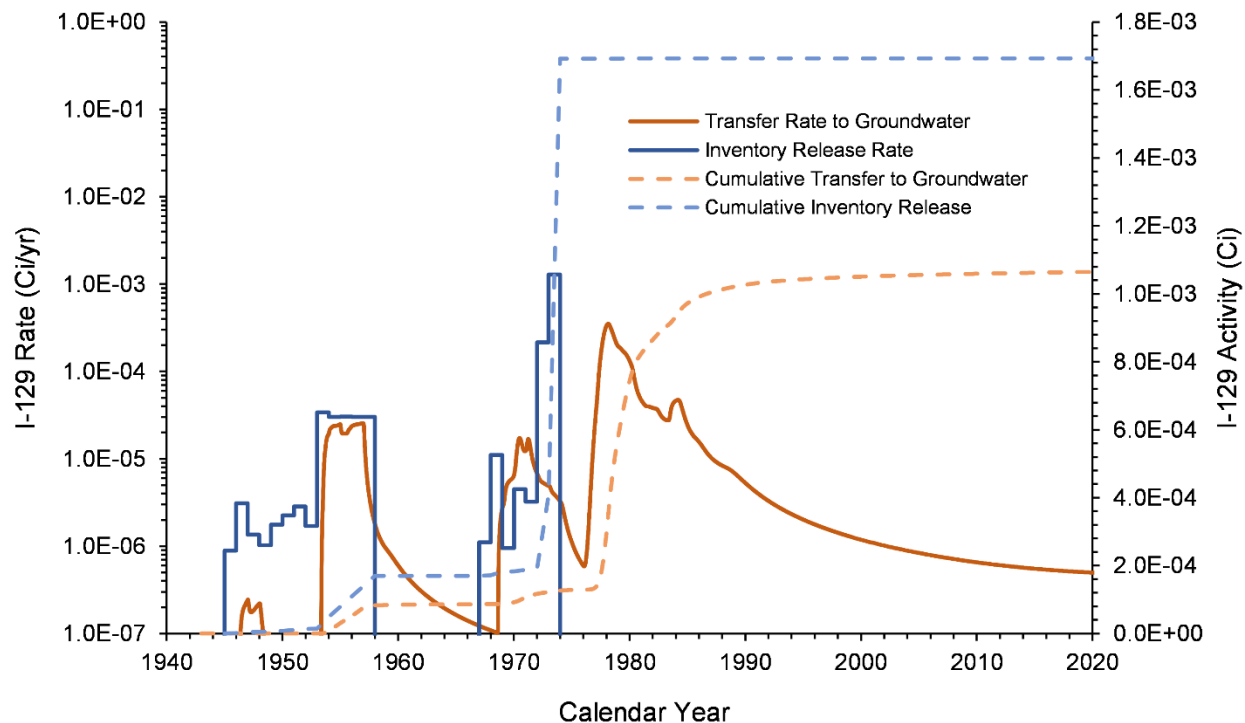
Figure 7-18. Cumulative I-129 Activity Released and Transfer Rate to Groundwater from the B Plant Area Model from 1943–2018
