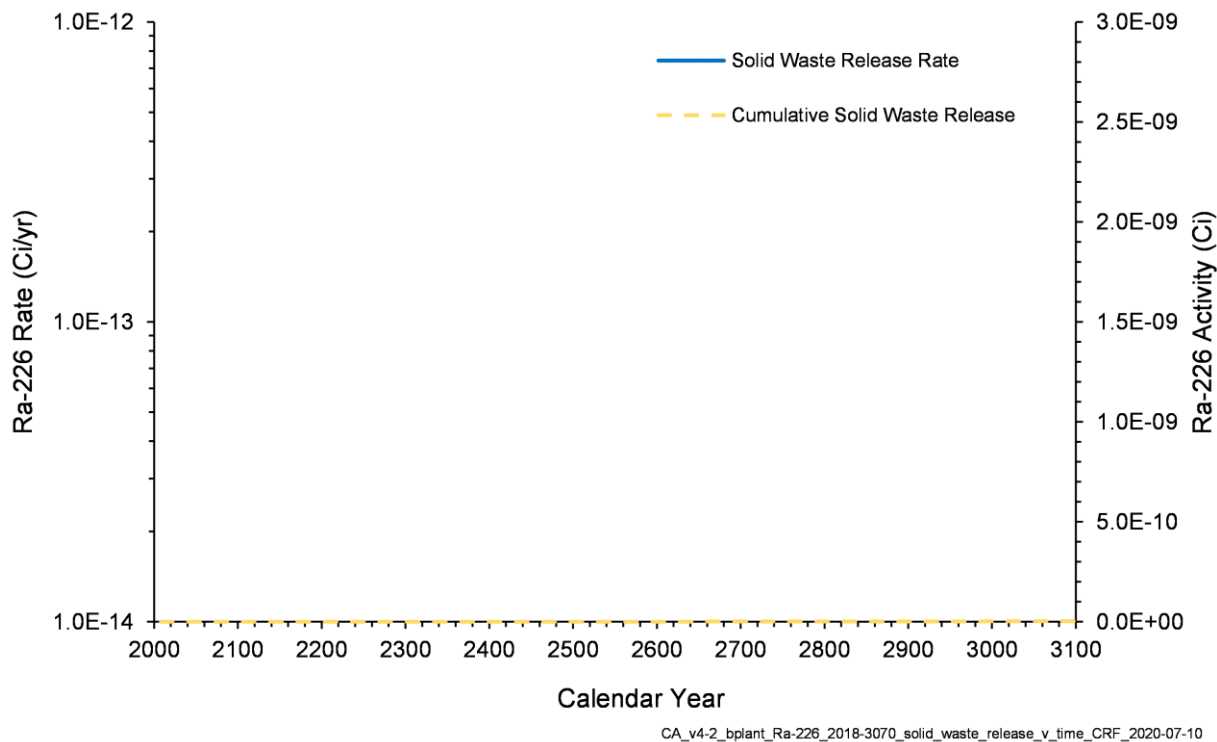
Figure 4-45. Ra-226 Release Rate and Cumulative Activity from Solid Waste in the B Plant Area Model, 2018–3070
