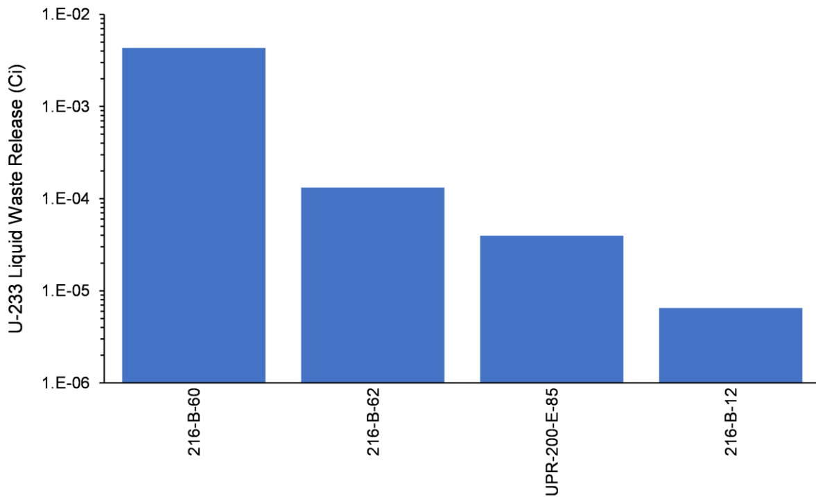
Figure 4-16. Total U-233 Activity Released from Liquid Waste Sites in the B Plant Area Model
