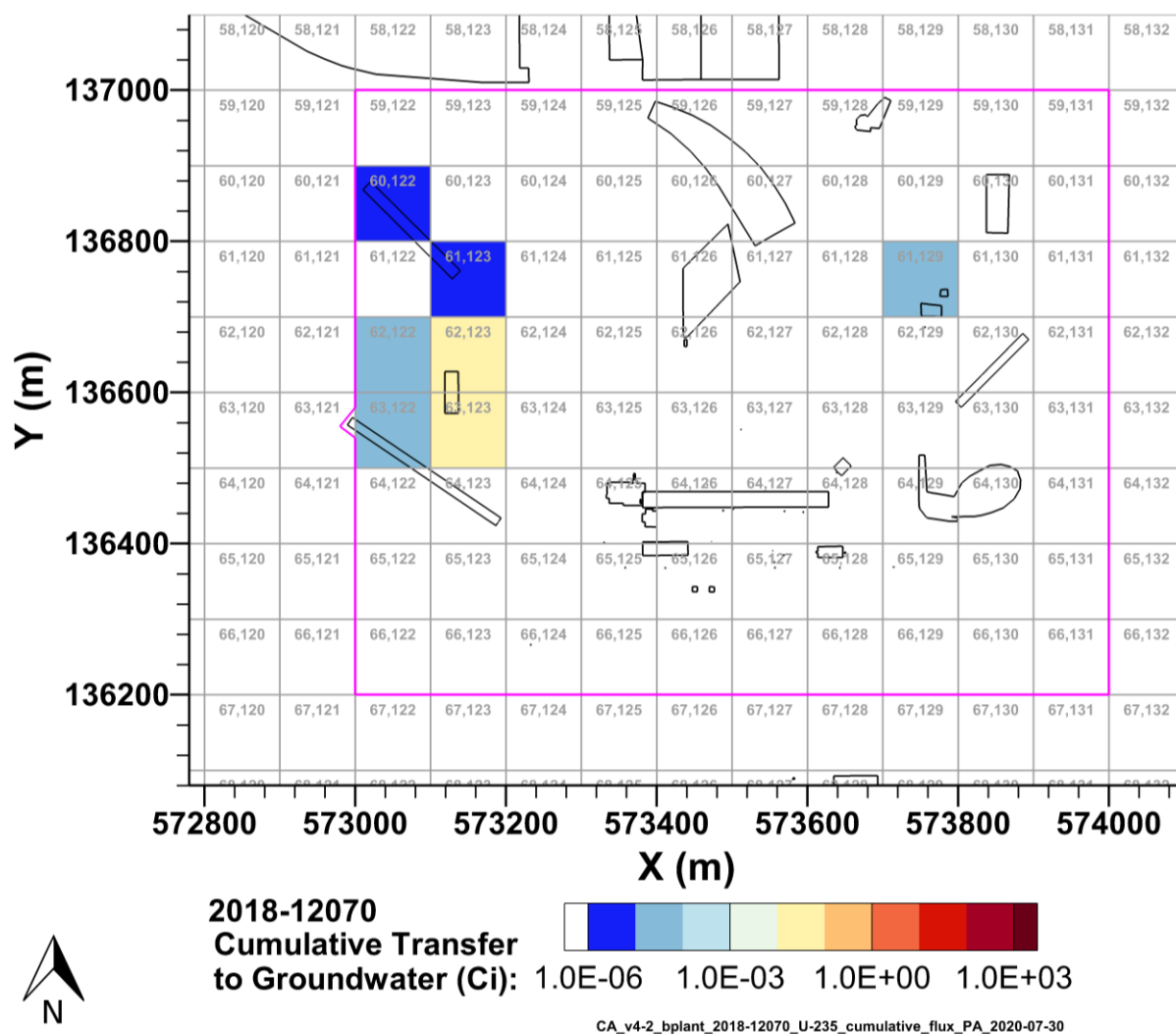
Figure 7-46. Cumulative U-235 Activity Discharged to Groundwater from the B Plant Area Model from 2018–12070 per P2R Grid Cell
