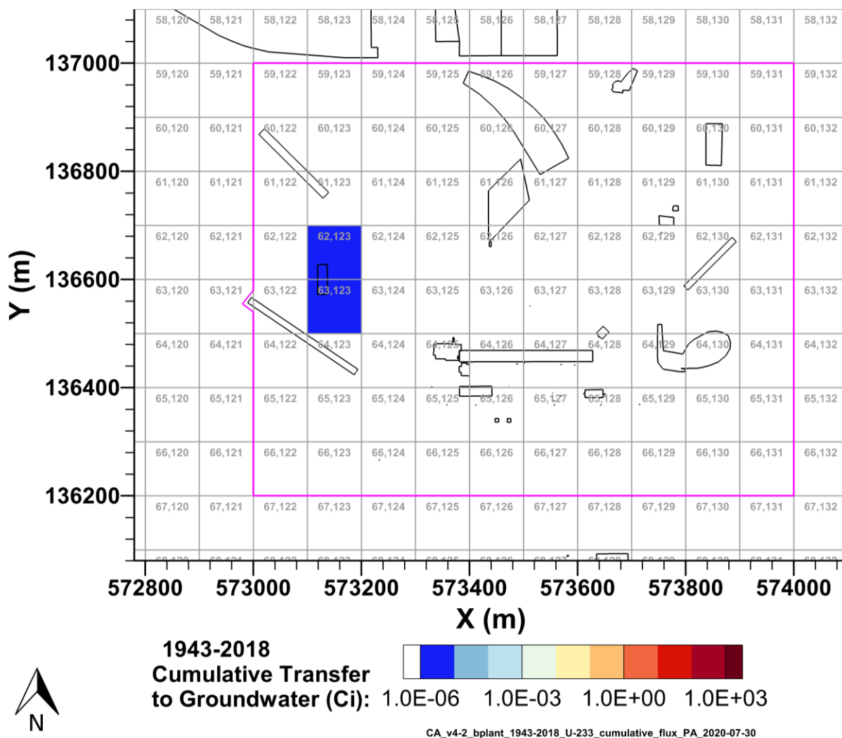
Figure 7-37. Cumulative U-233 Activity Discharged to Groundwater from the B Plant Area Model from 1943–2018 per P2R Grid Cell
