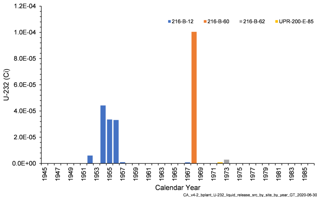
Figure 4-26. Annual U-232 Activity Released from Liquid Waste Sites in the B Plant Area Model
