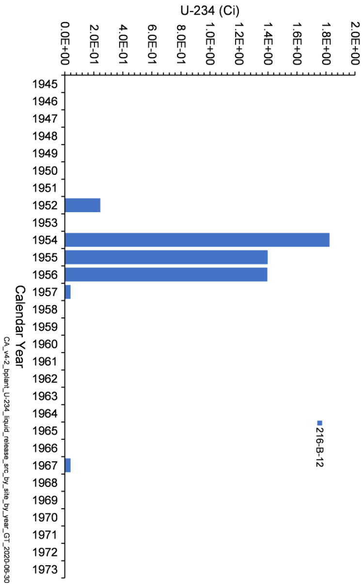
Figure 4-28. Annual U-234 Activity Released from Liquid Waste Sites in the B Plant Area Model
