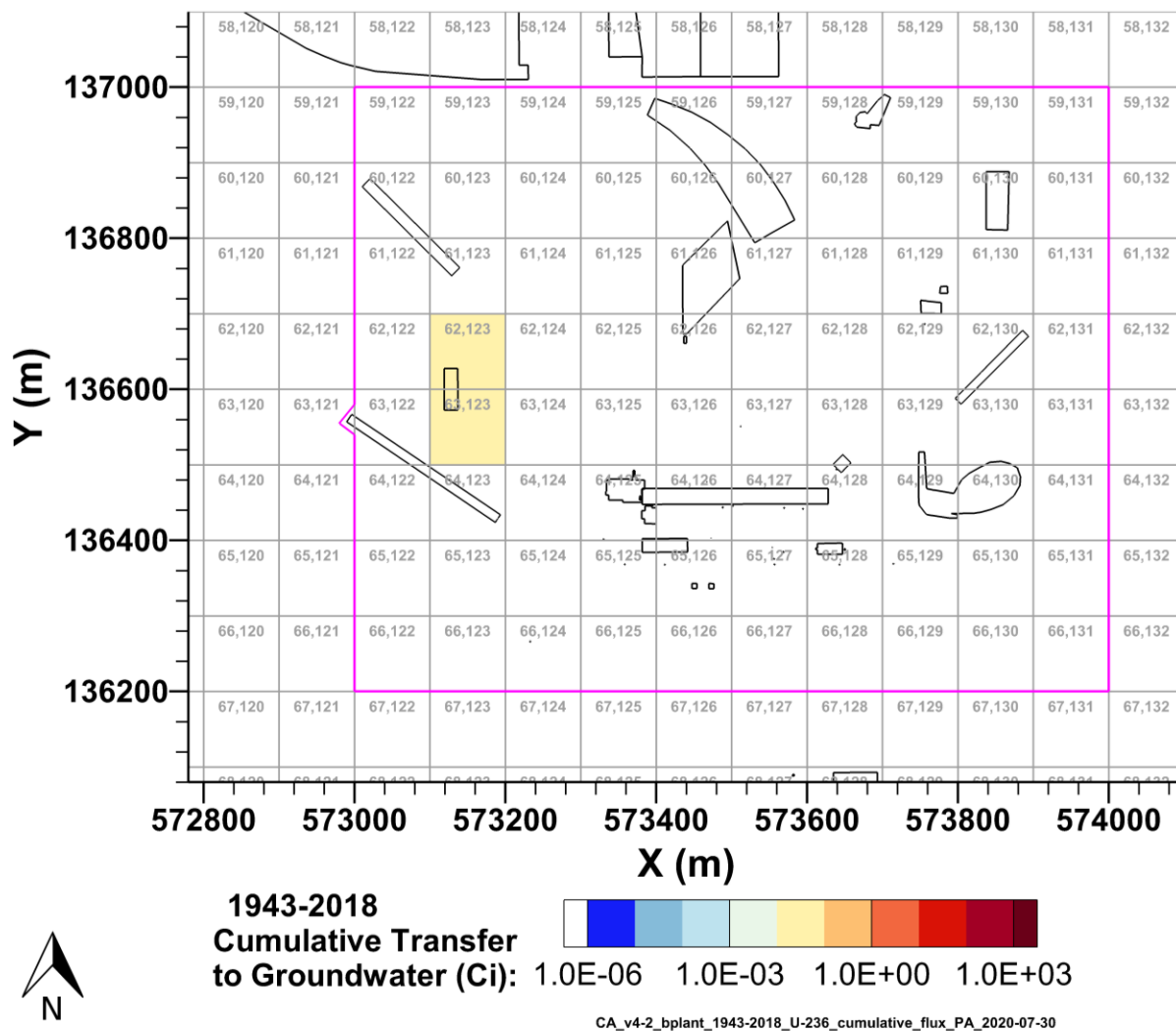
Figure 7-49. Cumulative U-236 Activity Discharged to Groundwater from the B Plant Area Model from 1943–2018 per P2R Grid Cell
