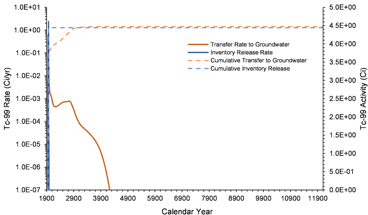
Figure 7-27. Cumulative Tc-99 Activity Released and Transfer Rate to Groundwater from the B Plant Area Model from 1943–12070
