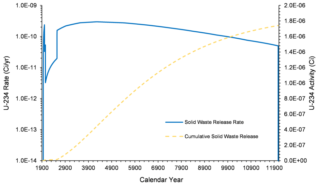
Figure 4-50. U-234 Release Rate and Cumulative Activity from Solid Waste in the B Plant Area Model, 1943–12070
