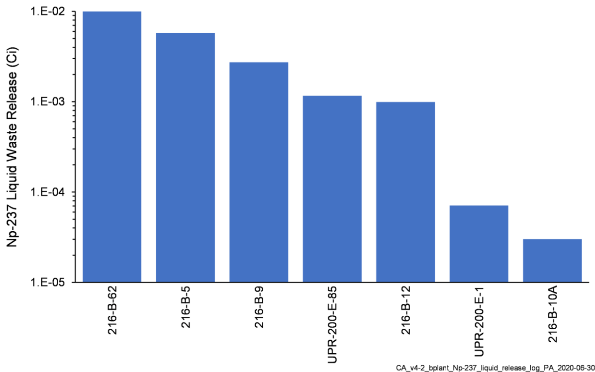
Figure 4-12. Total Np-237 Activity Released from Liquid Waste Sites in the B Plant Area Model
