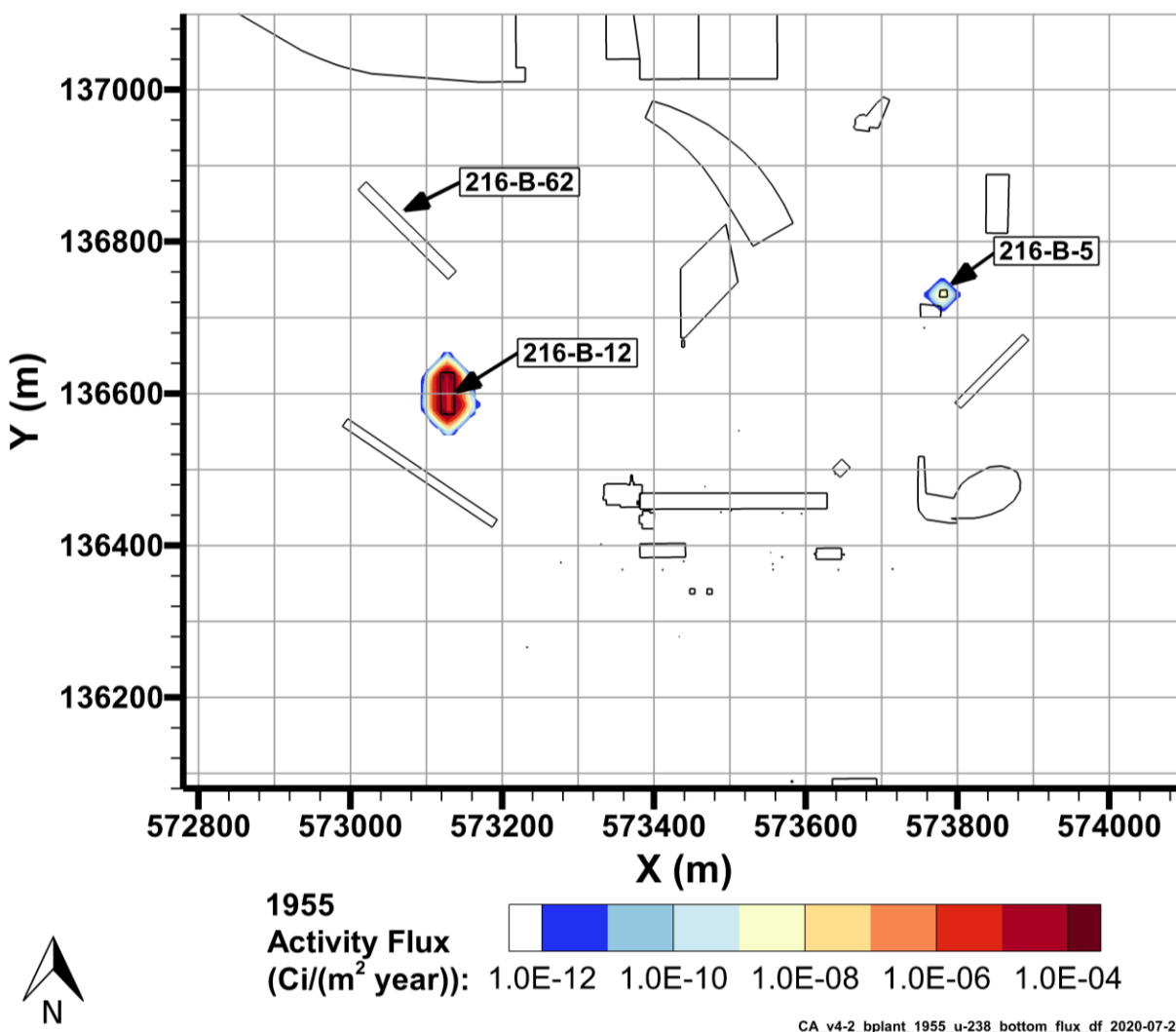
Figure 7-57. U-238 Flux to Groundwater, 1955
