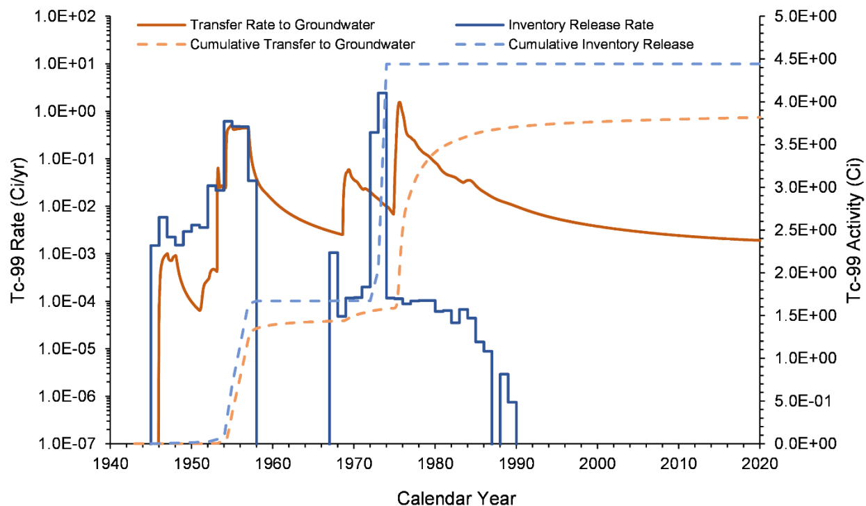
Figure 7-26. Cumulative Tc-99 Activity Released and Transfer Rate to Groundwater from the B Plant Area Model from 1943–2018
