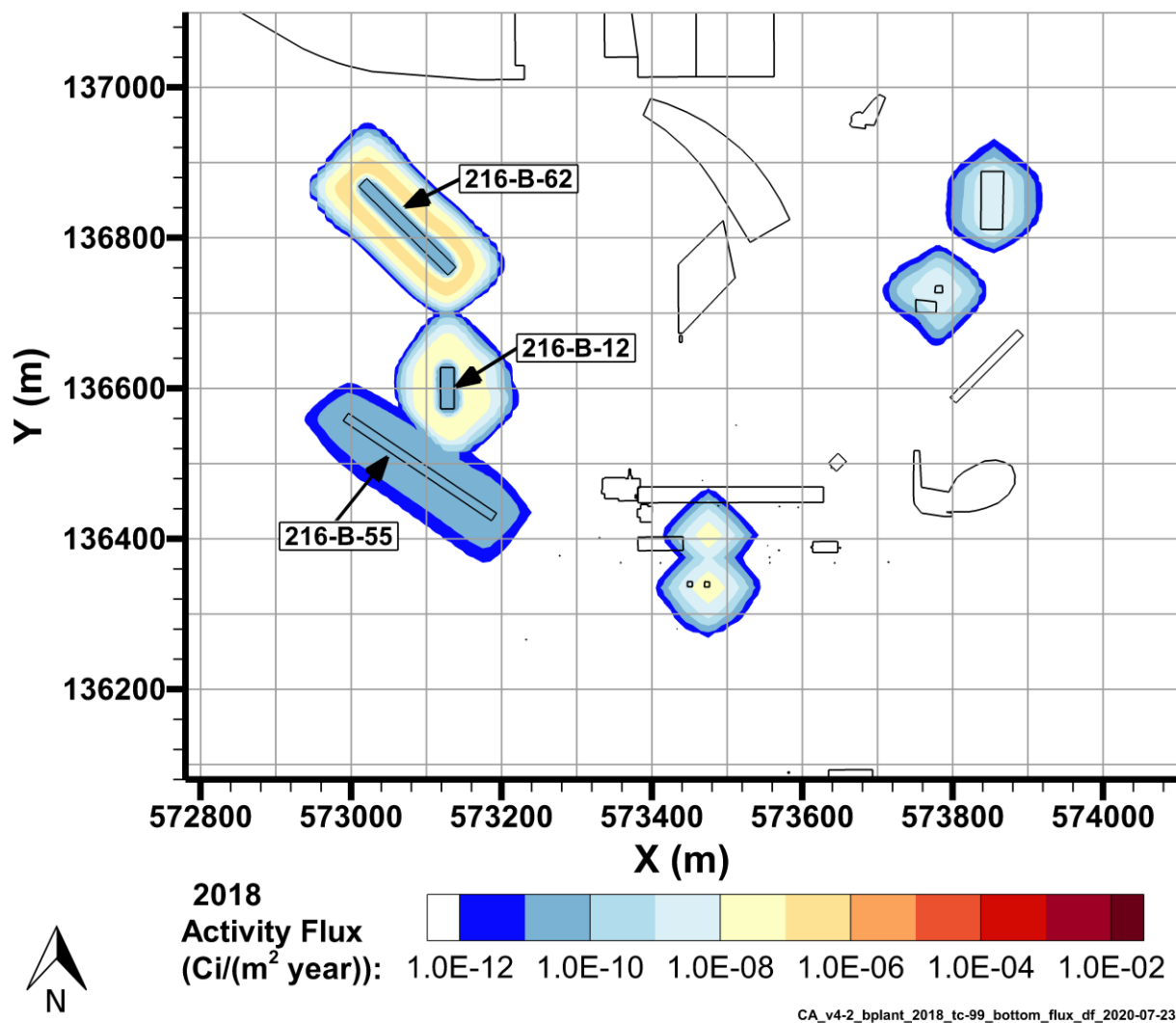
Figure 7-31. Tc-99 Flux to Groundwater, 2018
