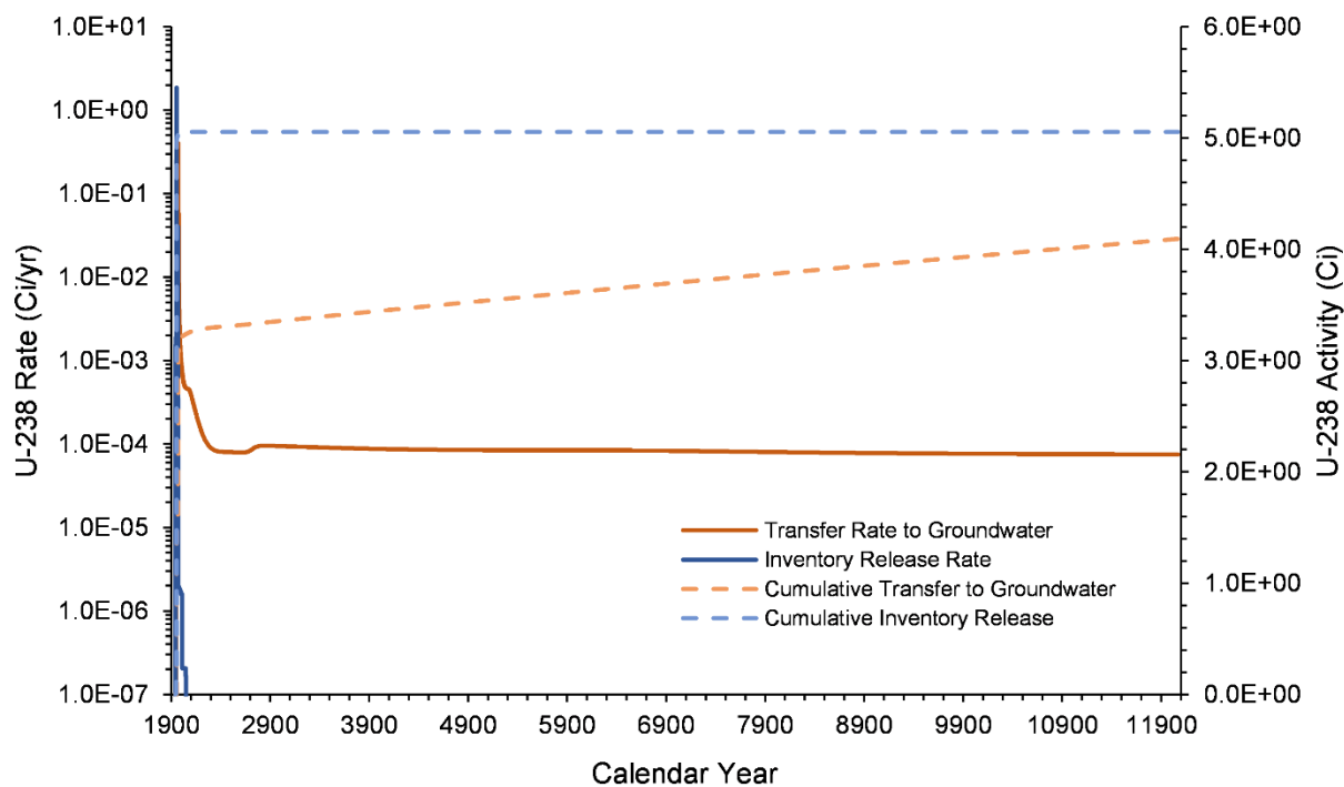
Figure 7-56. Cumulative U-238 Activity Released and Transfer Rate to Groundwater from the B Plant Area Model from 1943–12070
