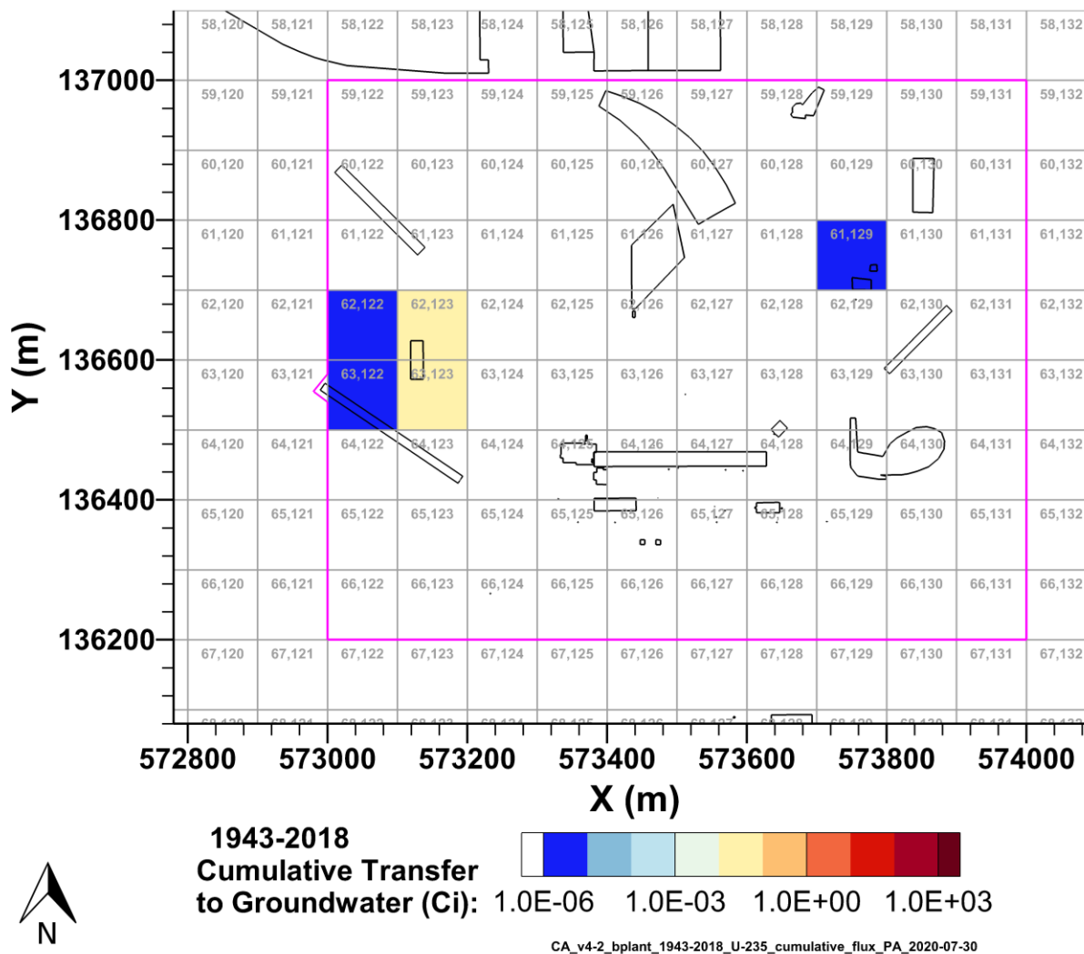
Figure 7-45. Cumulative U-235 Activity Discharged to Groundwater from the B Plant Area Model from 1943–2018 per P2R Grid Cell
