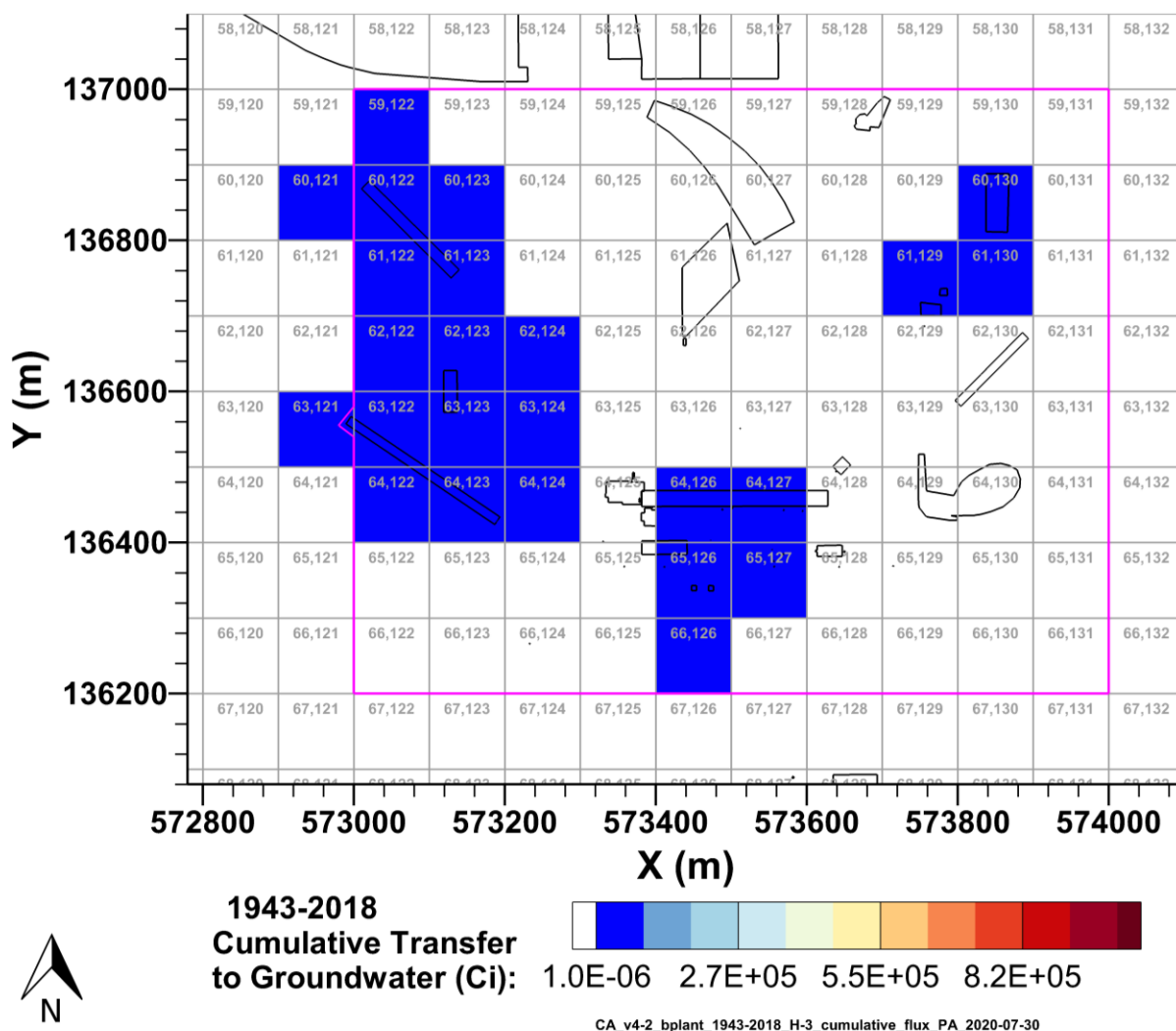
Figure 7-5. Cumulative H-3 Activity Discharged to Groundwater from the B Plant Area Model from 1943–2018 per P2R Grid Cell
