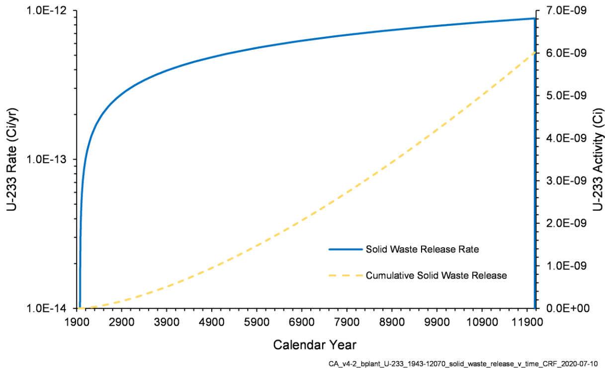
Figure 4-48. U-233 Release Rate and Cumulative Activity from Solid Waste in the B Plant Area Model, 1943–12070
