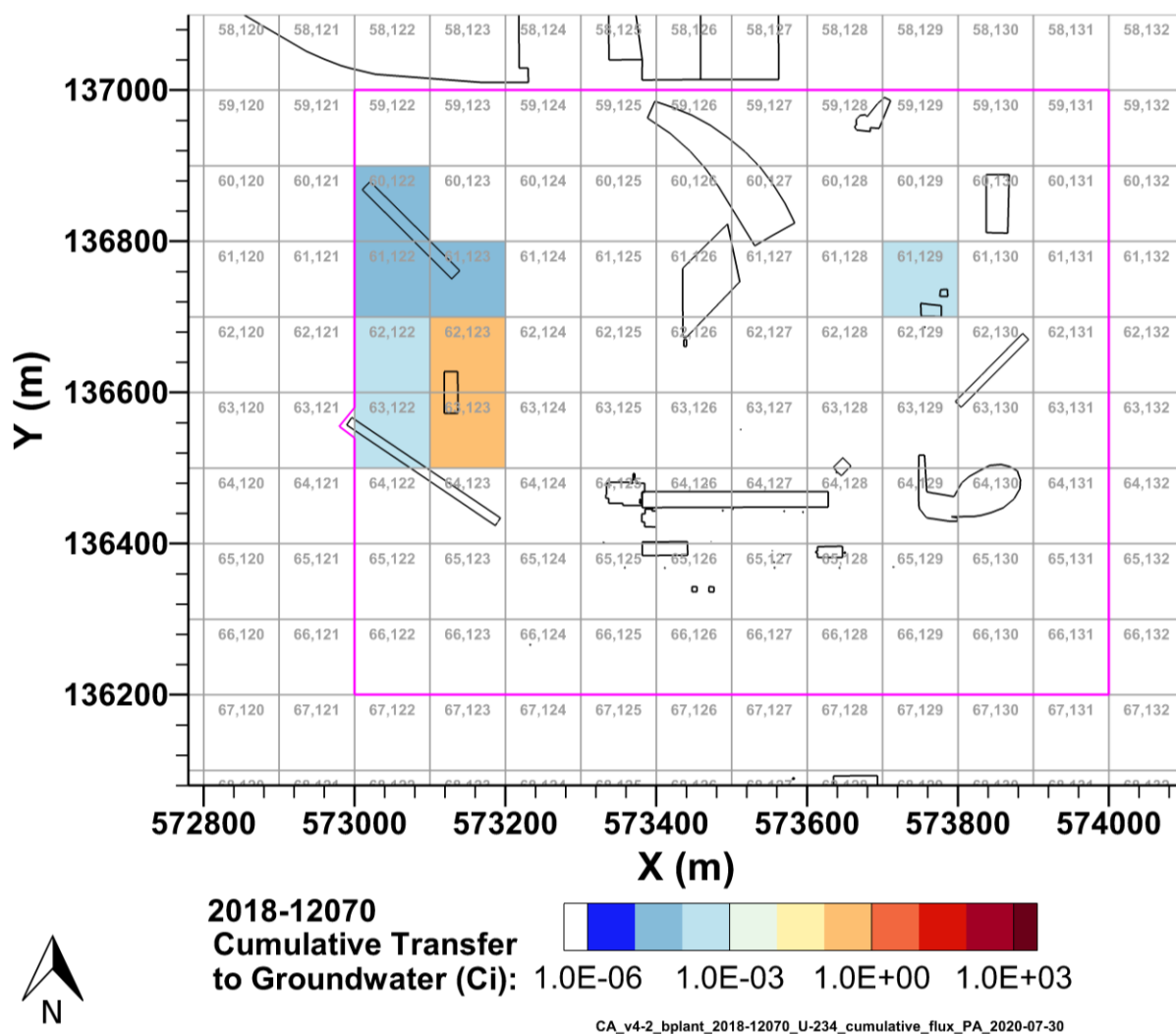
Figure 7-42. Cumulative U-234 Activity Discharged to Groundwater from the B Plant Area Model from 2018–12070 per P2R Grid Cell
