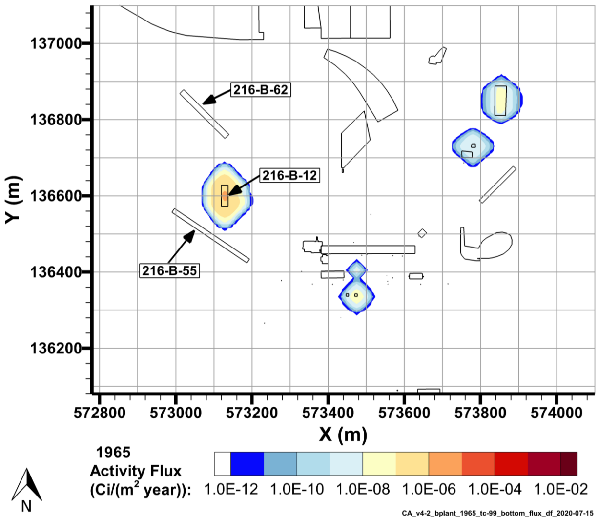
Figure 7-29. Tc-99 Flux to Groundwater, 1965
