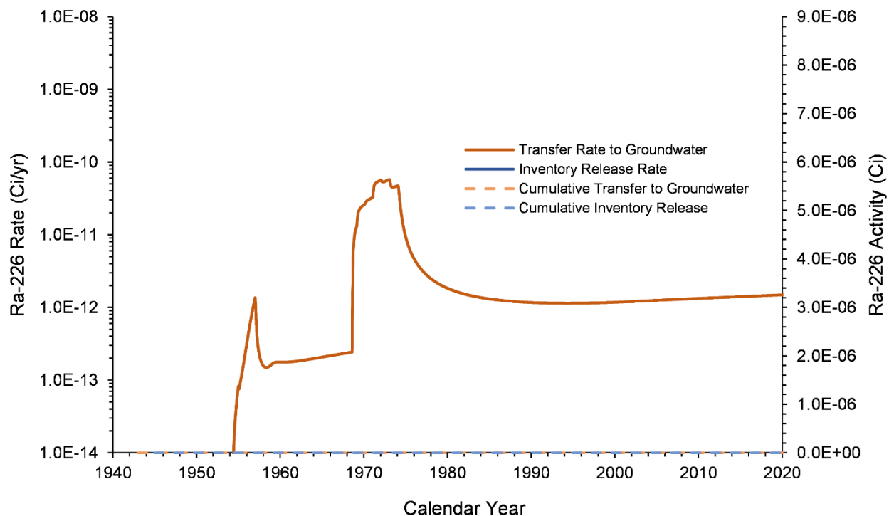
Figure 7-65. Ra-226 Inventory Release from Waste Sites and Transfer to Groundwater for the B Plant Area Model from 1943–2018
