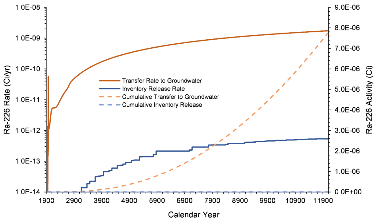
Figure 7-66. Ra-226 Inventory Release from Waste Sites and Transfer to Groundwater for the B Plant Area Model from 1943–12070
