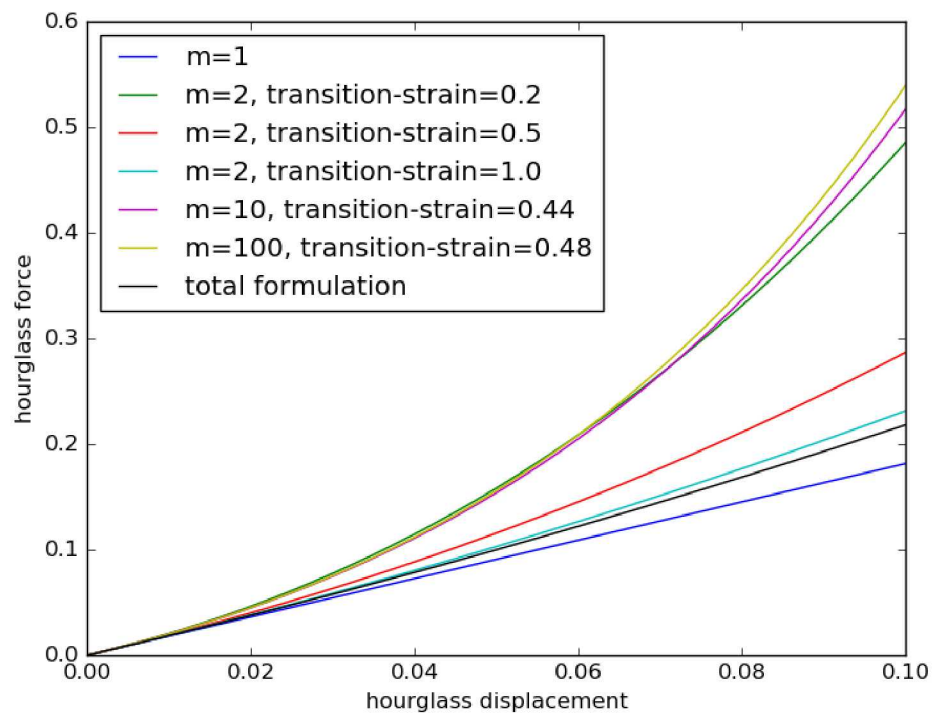
Figure 15-3. Nonlinear hourglass force versus displacement
