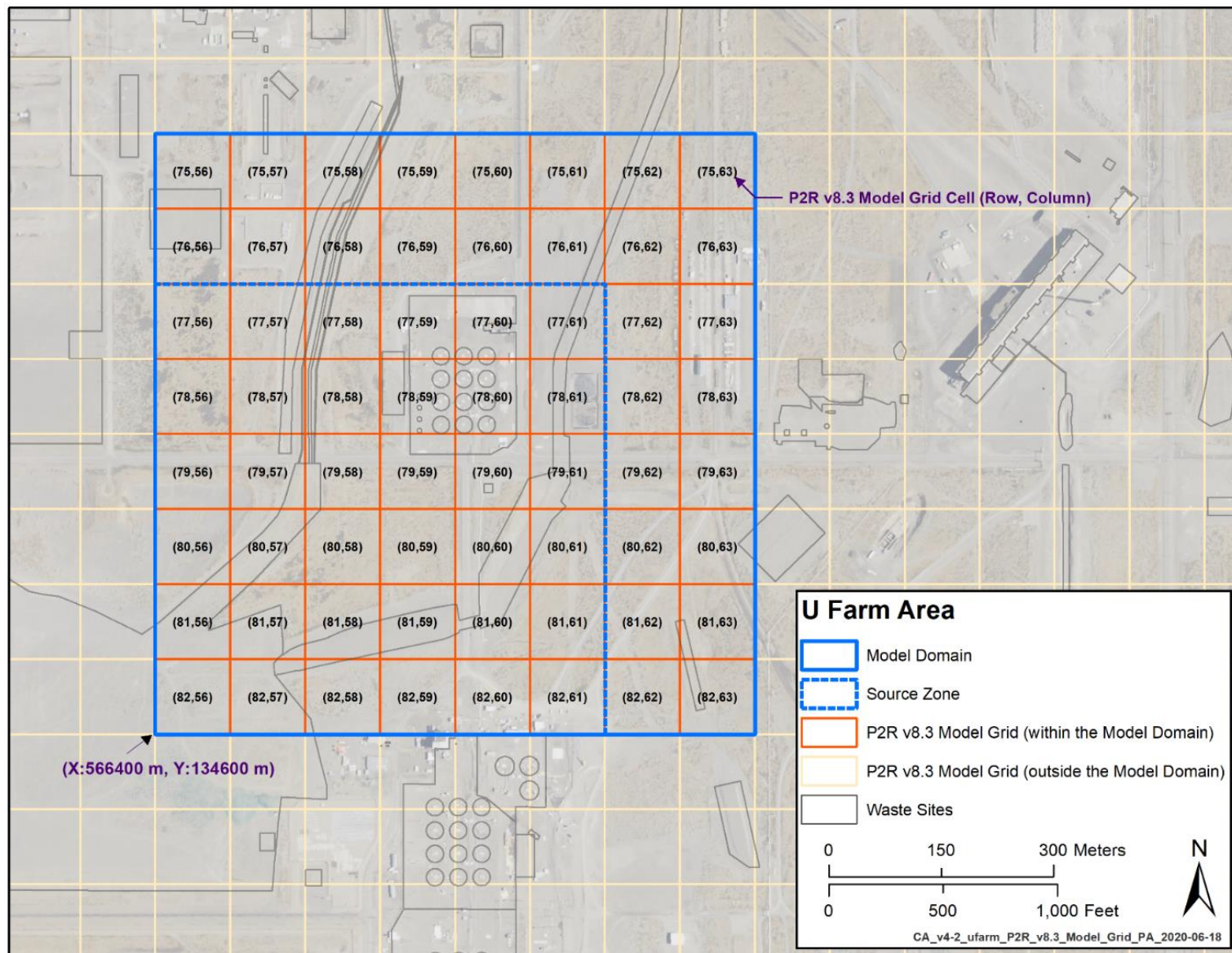
Figure 4-2. Plan View of the P2R Grid Cells in the U Farm Area Model
