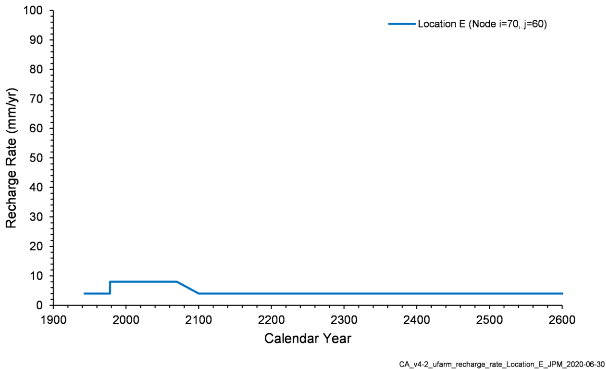
Figure 4-89. Time Series of Natural Recharge Rates, Location E
