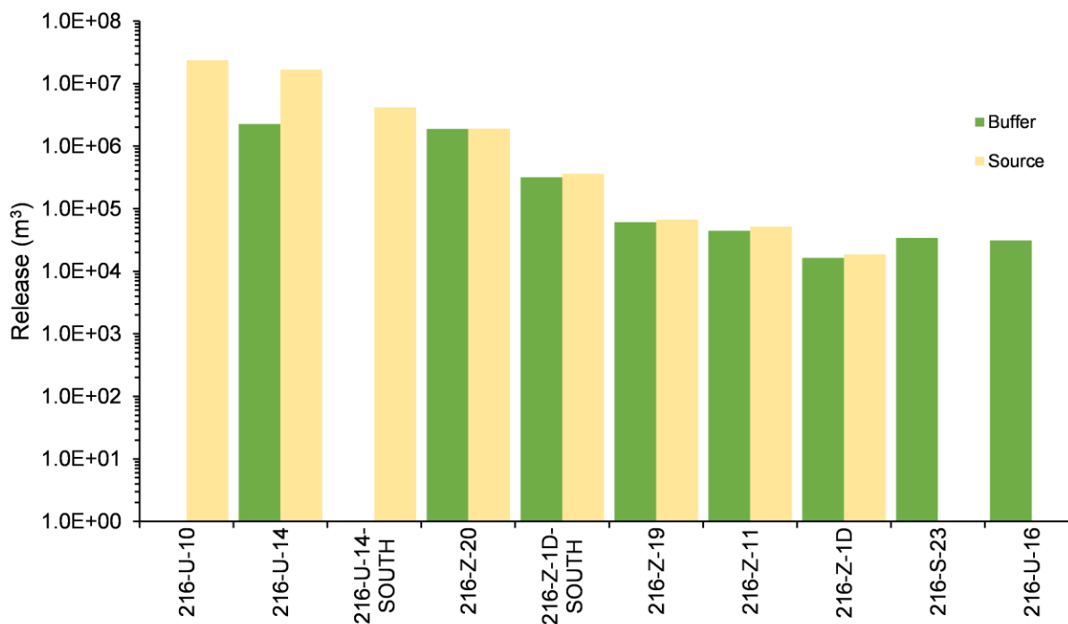
Figure 4-75. Total Volume of Water Released from Liquid Waste Sites in the U Farm Area Model
