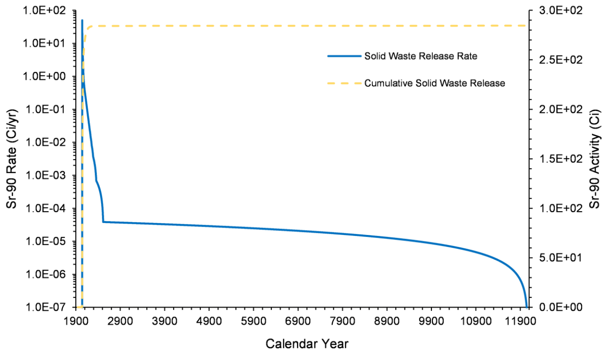
Figure 4-55. Sr-90 Release Rate and Cumulative Activity from Solid Waste in the U Farm Area Model, 1943–12070
