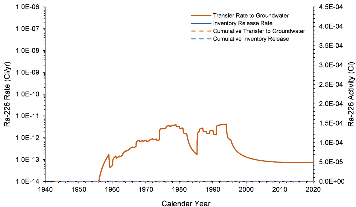
Figure 7-57. Ra-226 Inventory Release from Waste Sites and Transfer to Groundwater for the U Farm Area Model from 1943–2018
