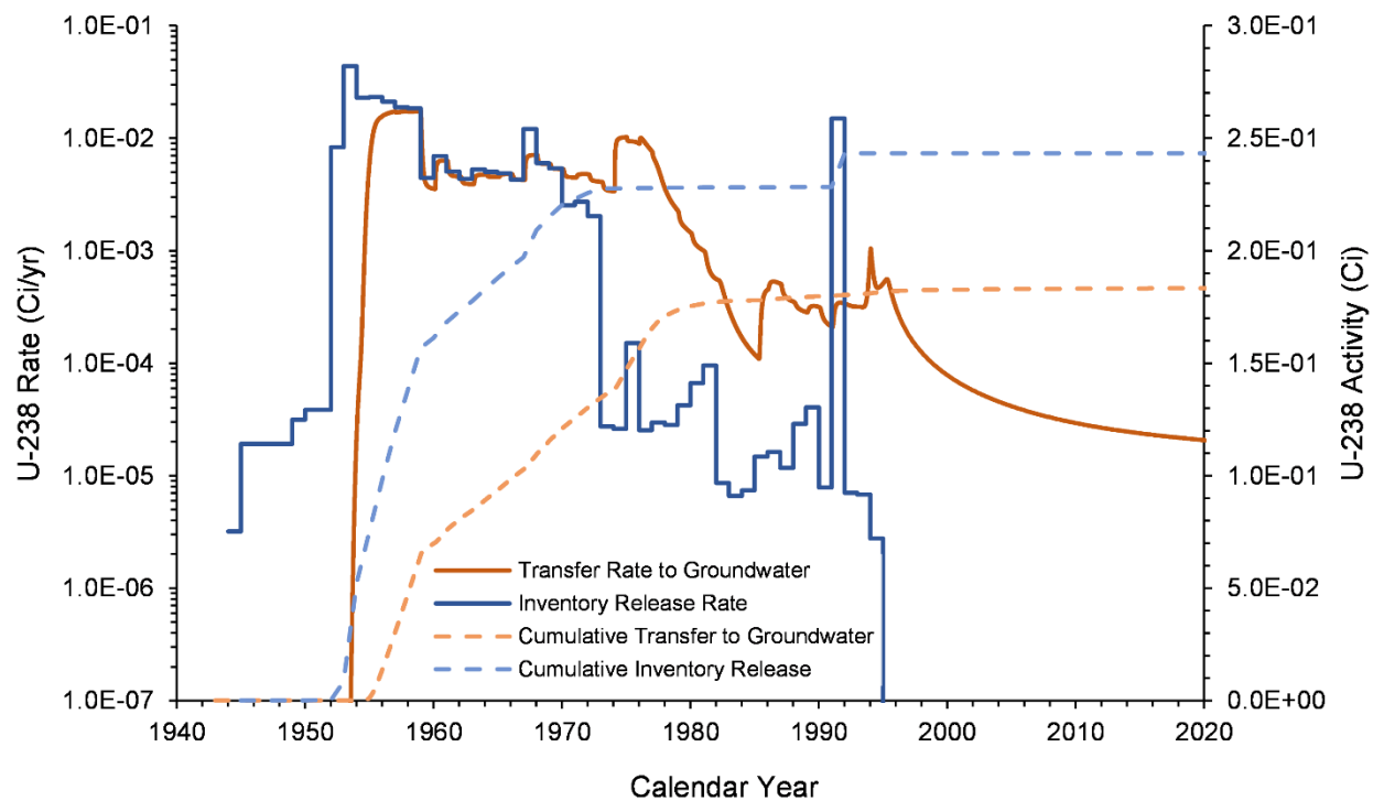
Figure 7-55. U-238 Inventory Release from Waste Sites and Transfer to Groundwater for the U Farm Area Model from 1943–2018
