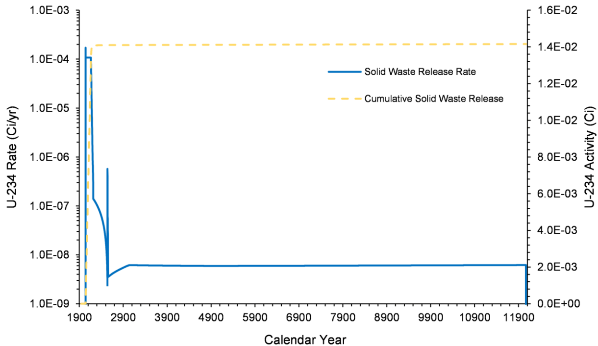
Figure 4-67. U-234 Release Rate and Cumulative Activity from Solid Waste in the U Farm Area Model, 1943–12070
