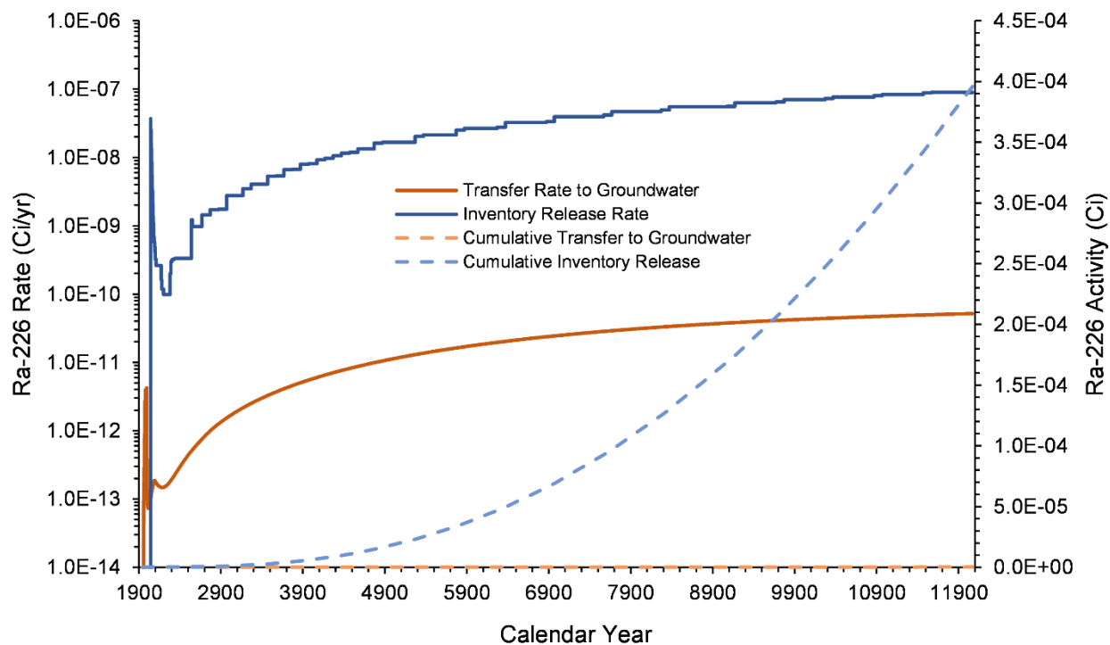
Figure 7-58. Ra-226 Inventory Release from Waste Sites and Transfer to Groundwater for the U Farm Area Model from 1943–12070
