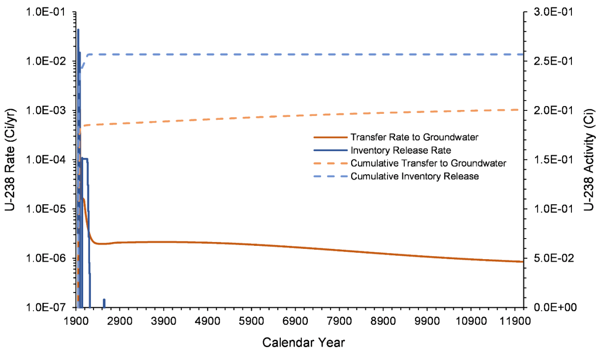
Figure 7-56. U-238 Inventory Release from Waste Sites and Transfer to Groundwater for the U Farm Area Model from 1943–12070
