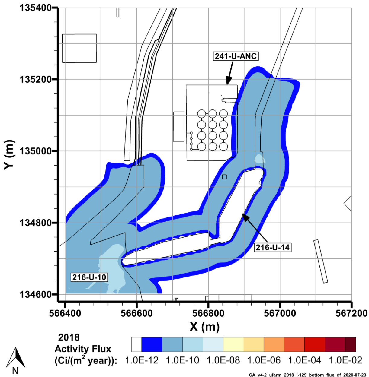
Figure 7-16. I-129 Flux to Groundwater, 2018
