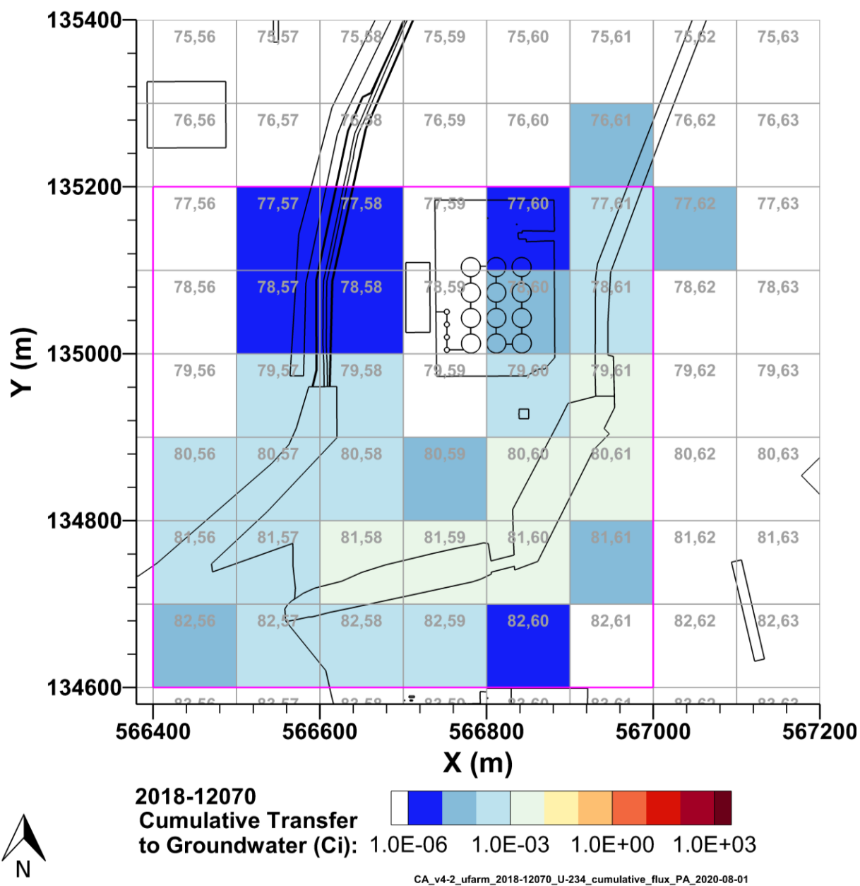
Figure 7-42. Cumulative U-234 Activity Discharged to Groundwater from the U Farm Area Model from 2018–12070 per P2R Grid Cell
