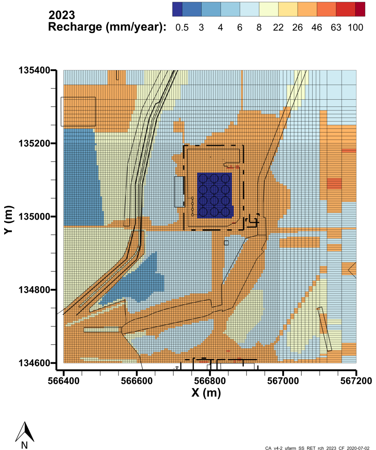
Figure 4-81. Transient Recharge Estimates for the U Farm Area Model, 2023
