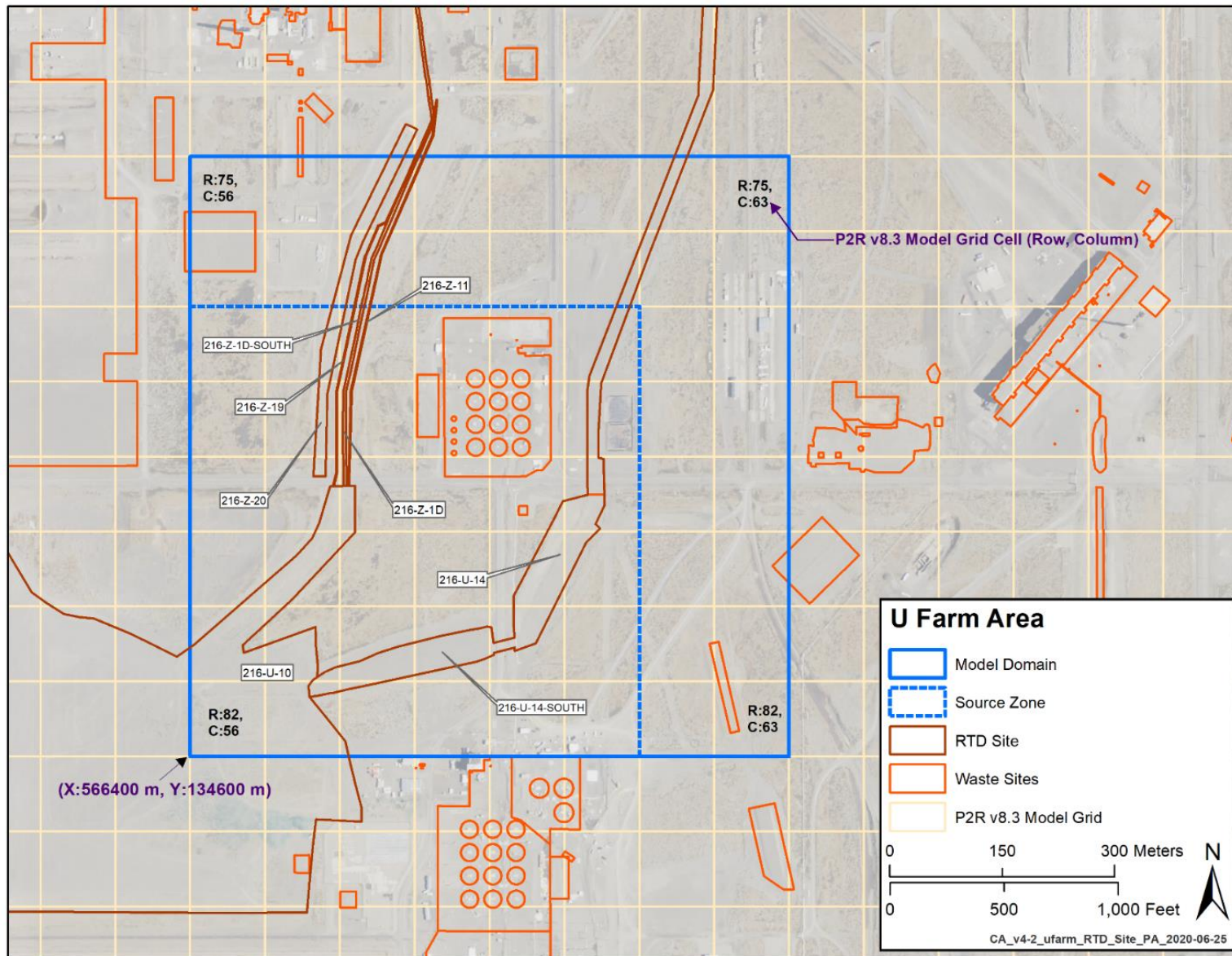
Figure 4-77. Map of the RTD Sites in the U Farm Area Model
