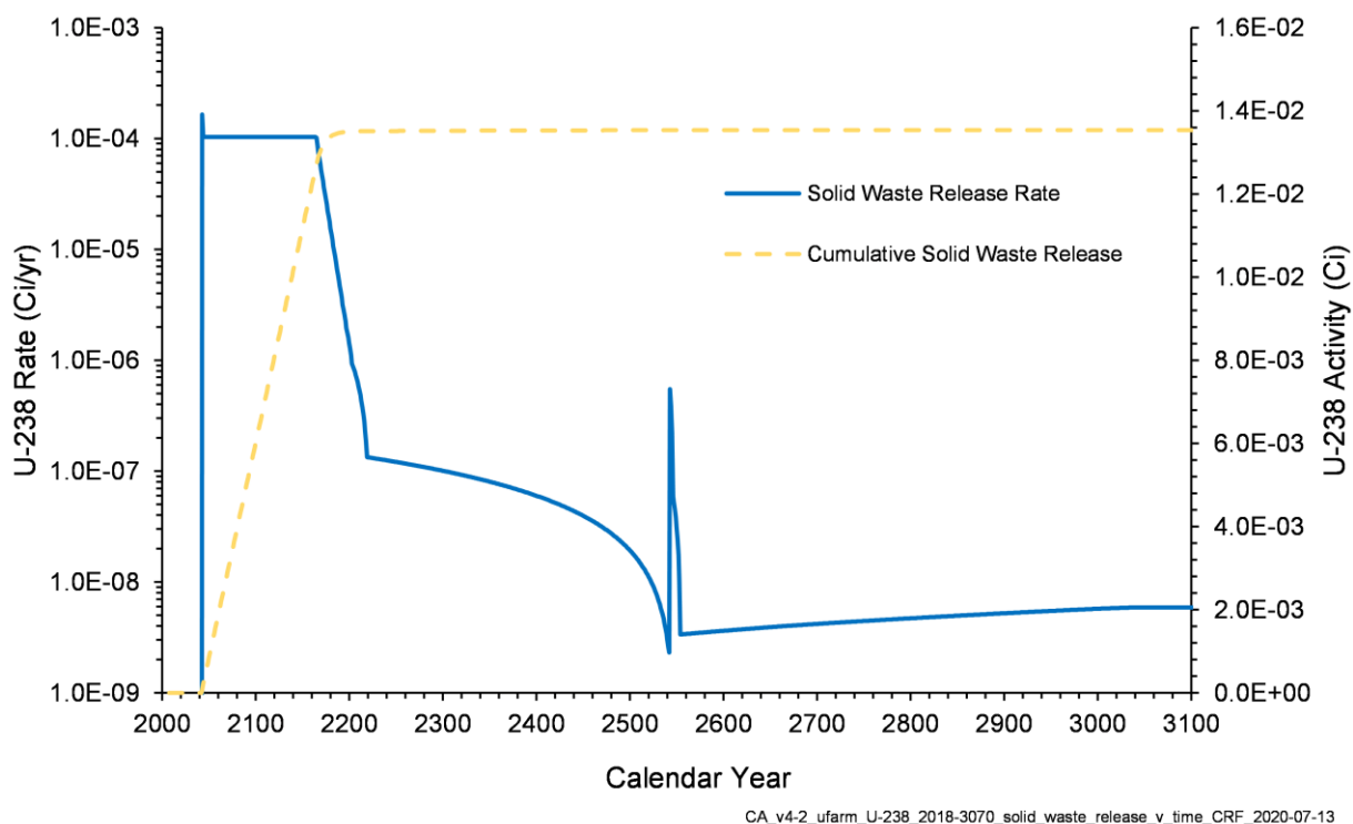
Figure 4-74. U-238 Release Rate and Cumulative Activity from Solid Waste in the U Farm Area Model, 2018–3070
