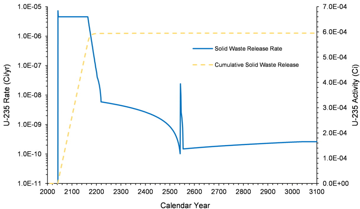
Figure 4-70. U-235 Release Rate and Cumulative Activity from Solid Waste in the U Farm Area Model, 2018–3070
