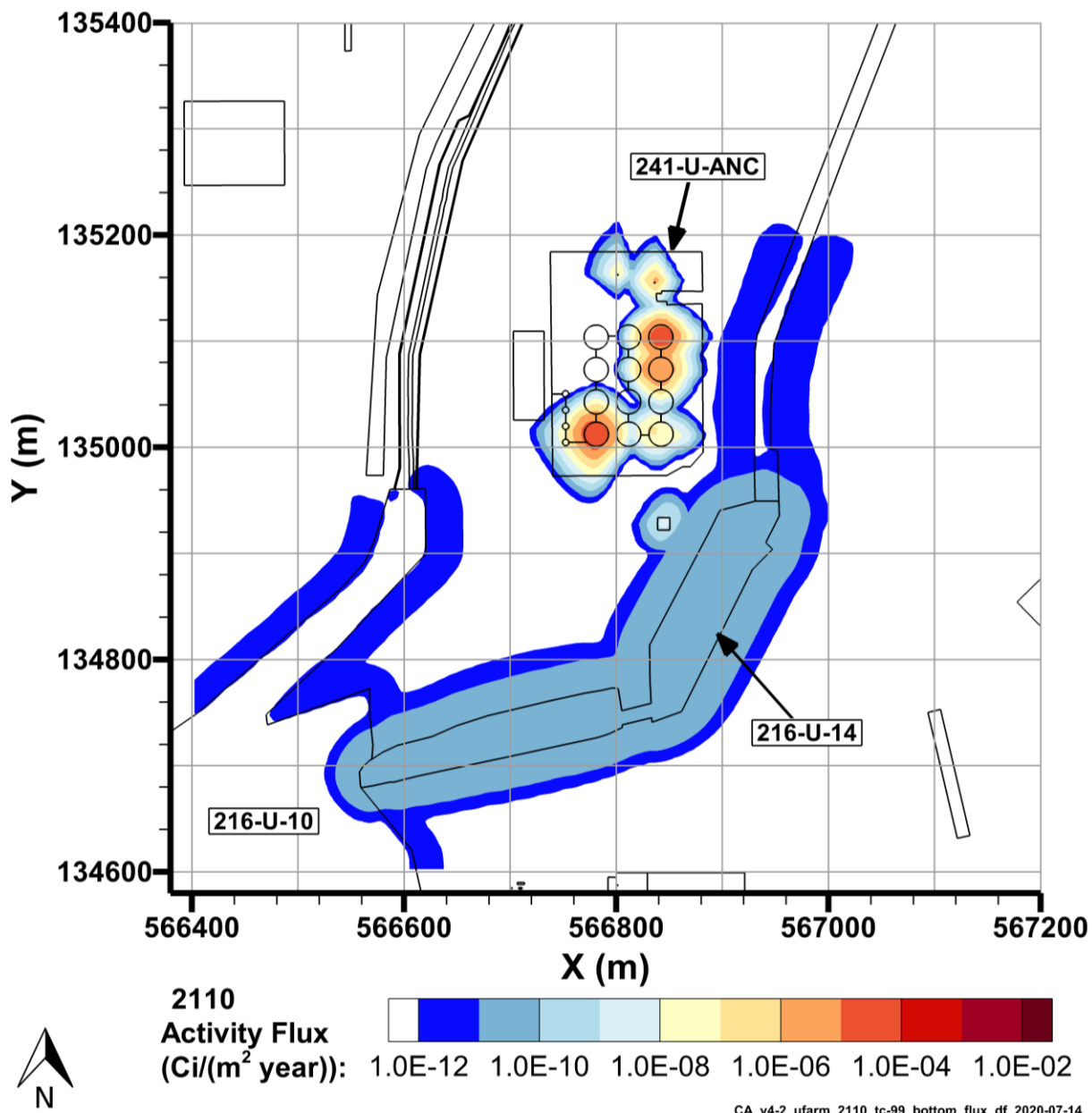
Figure 7-30. Tc-99 Flux to Groundwater, 2110
