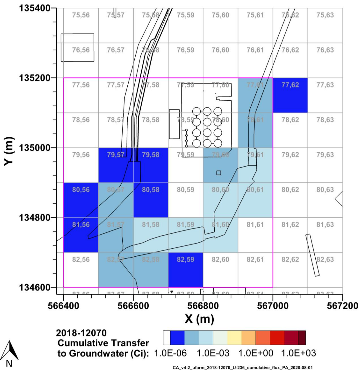
Figure 7-50. Cumulative U-236 Activity Discharged to Groundwater from the U Farm Area Model from 2018–12070 per P2R Grid Cell
