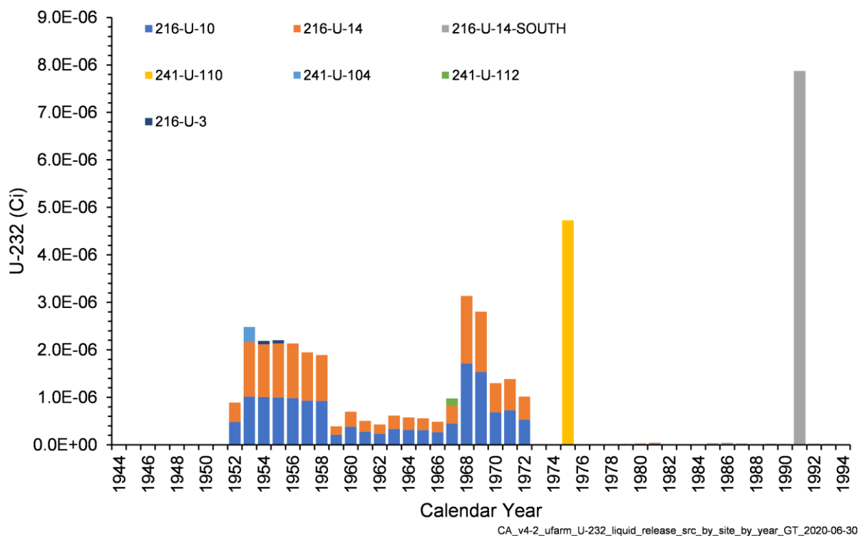
Figure 4-27. Annual U-232 Activity Released from Liquid Waste Sites in the U Farm Area Model
