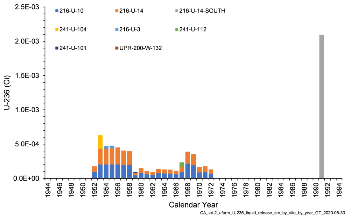
Figure 4-31. Annual U-236 Activity Released from Liquid Waste Sites in the U Farm Area Model
