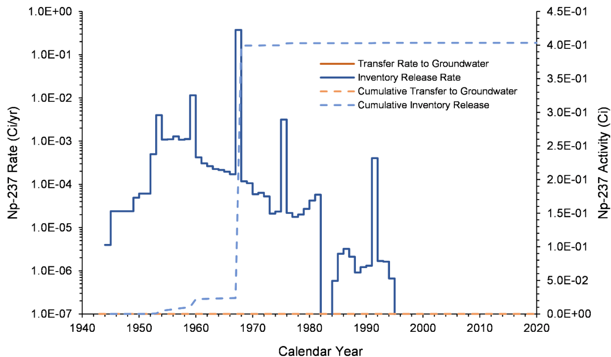
Figure 7-20. Np-237 Inventory Release from Waste Sites and Transfer to Groundwater for the U Farm Area Model from 1943–2018
