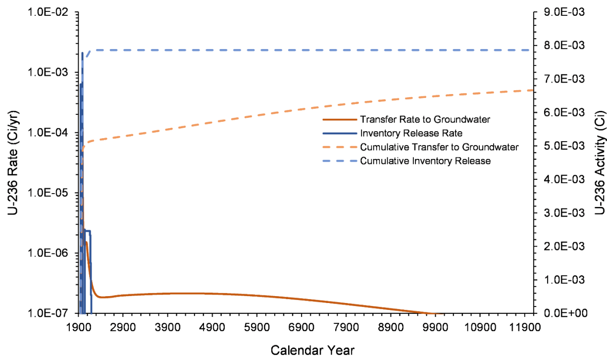
Figure 7-52. U-236 Inventory Release from Waste Sites and Transfer to Groundwater for the U Farm Area Model from 1943–12070
