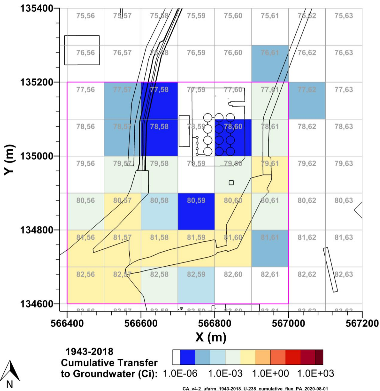
Figure 7-53. Cumulative U-238 Activity Discharged to Groundwater from the U Farm Area Model from 1943–2018 per P2R Grid Cell
