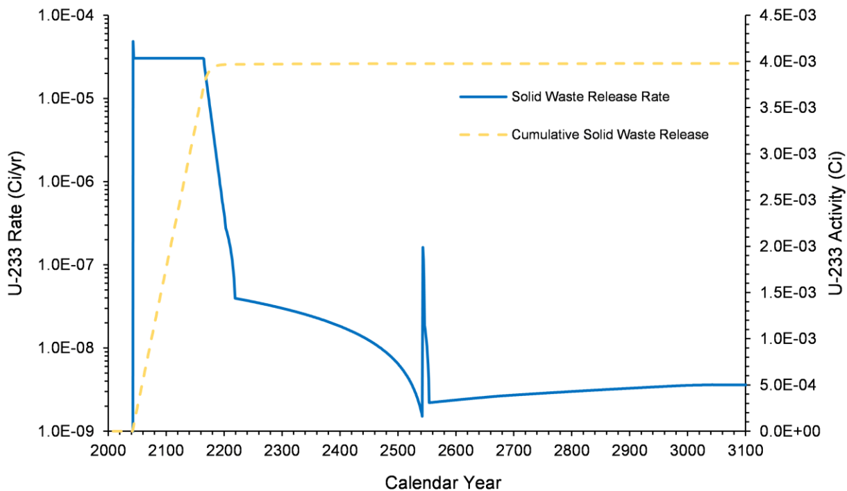
Figure 4-66. U-233 Release Rate and Cumulative Activity from Solid Waste in the U Farm Area Model, 2018–3070
