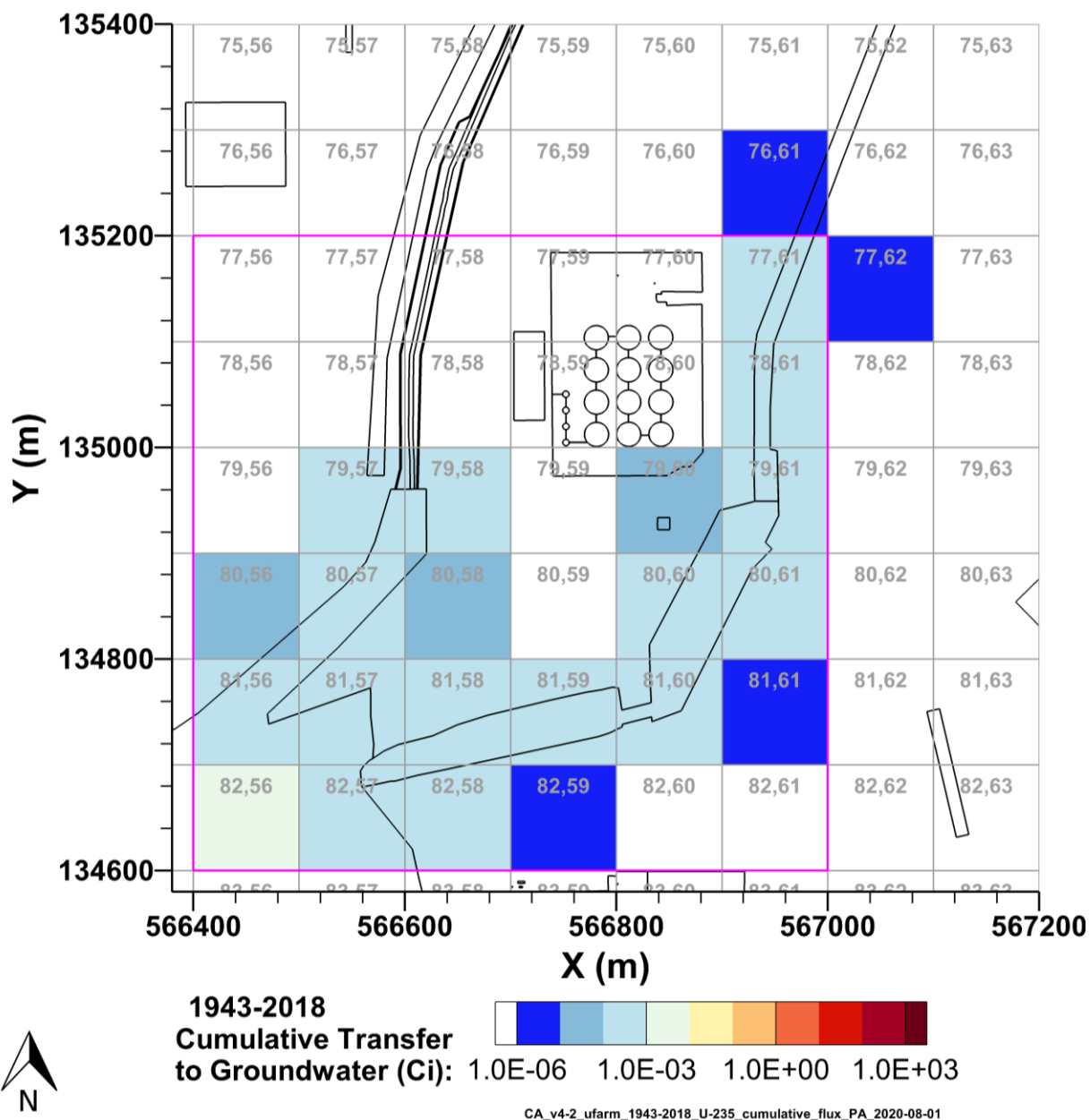
Figure 7-45. Cumulative U-235 Activity Discharged to Groundwater from the U Farm Area Model from 1943–2018 per P2R Grid Cell
