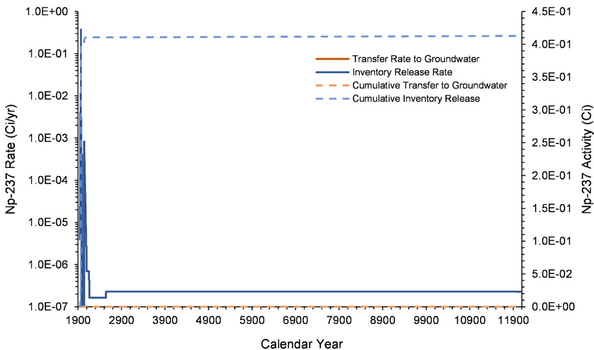
Figure 7-21. Np-237 Inventory Release from Waste Sites and Transfer to Groundwater for the U Farm Area Model from 1943–12070
