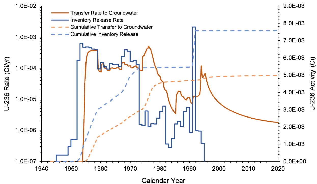
Figure 7-51. U-236 Inventory Release from Waste Sites and Transfer to Groundwater for the U Farm Area Model from 1943–2018
