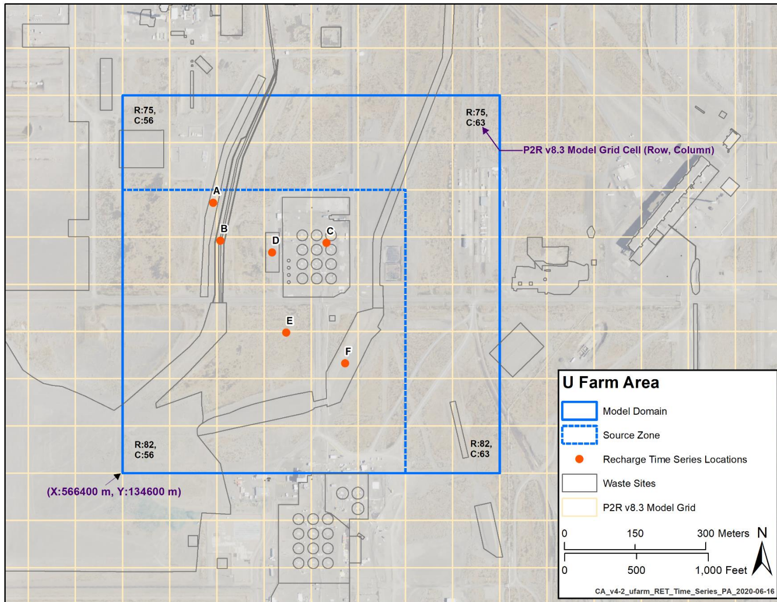
Figure 4-84. Locations of Recharge Rate Time Series Examples
