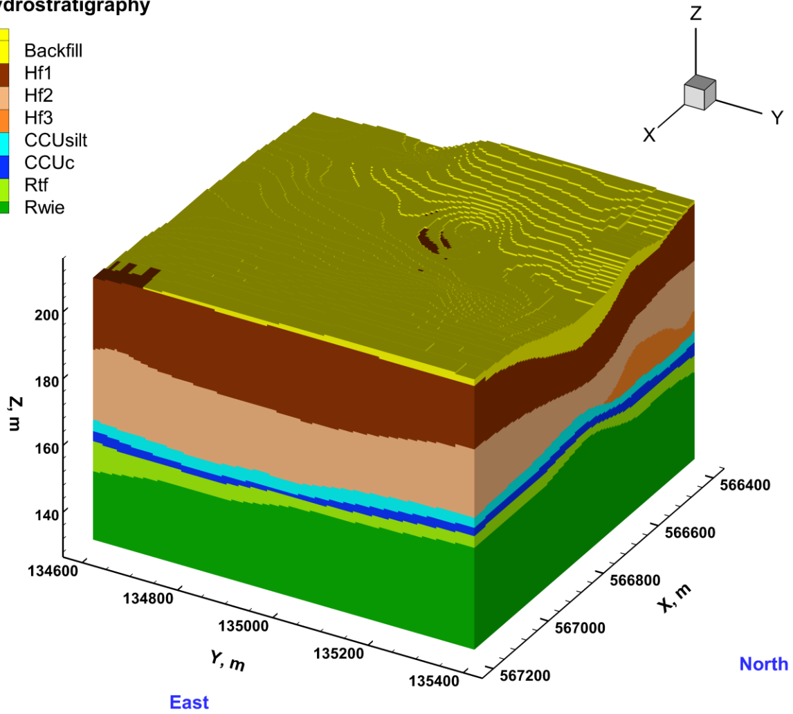
Figure 4-3. Model Hydrostratigraphy Three-Dimensional View Showing the North and East Faces
