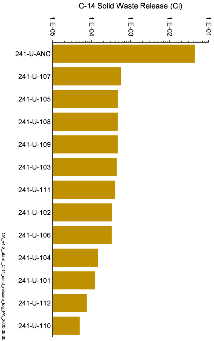
Figure 4-33. Total C-14 Activity Released from Solid Waste Sites in the U Farm Area Model
