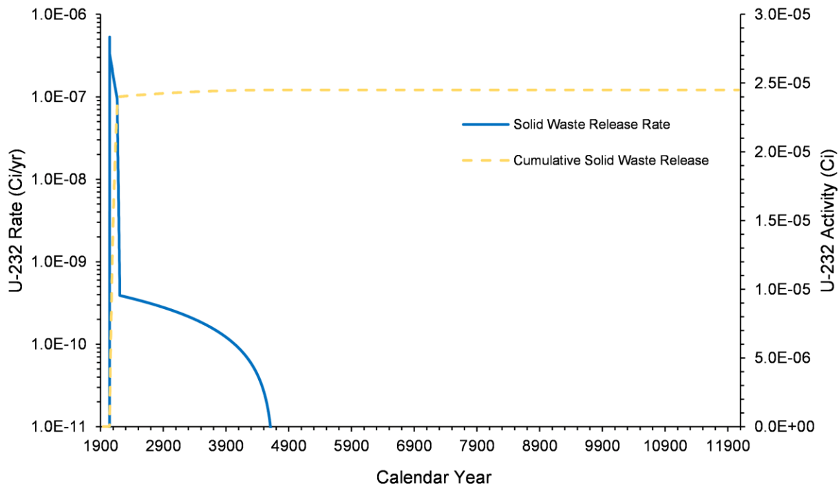
Figure 4-63. U-232 Release Rate and Cumulative Activity from Solid Waste in the U Farm Area Model, 1943–12070
