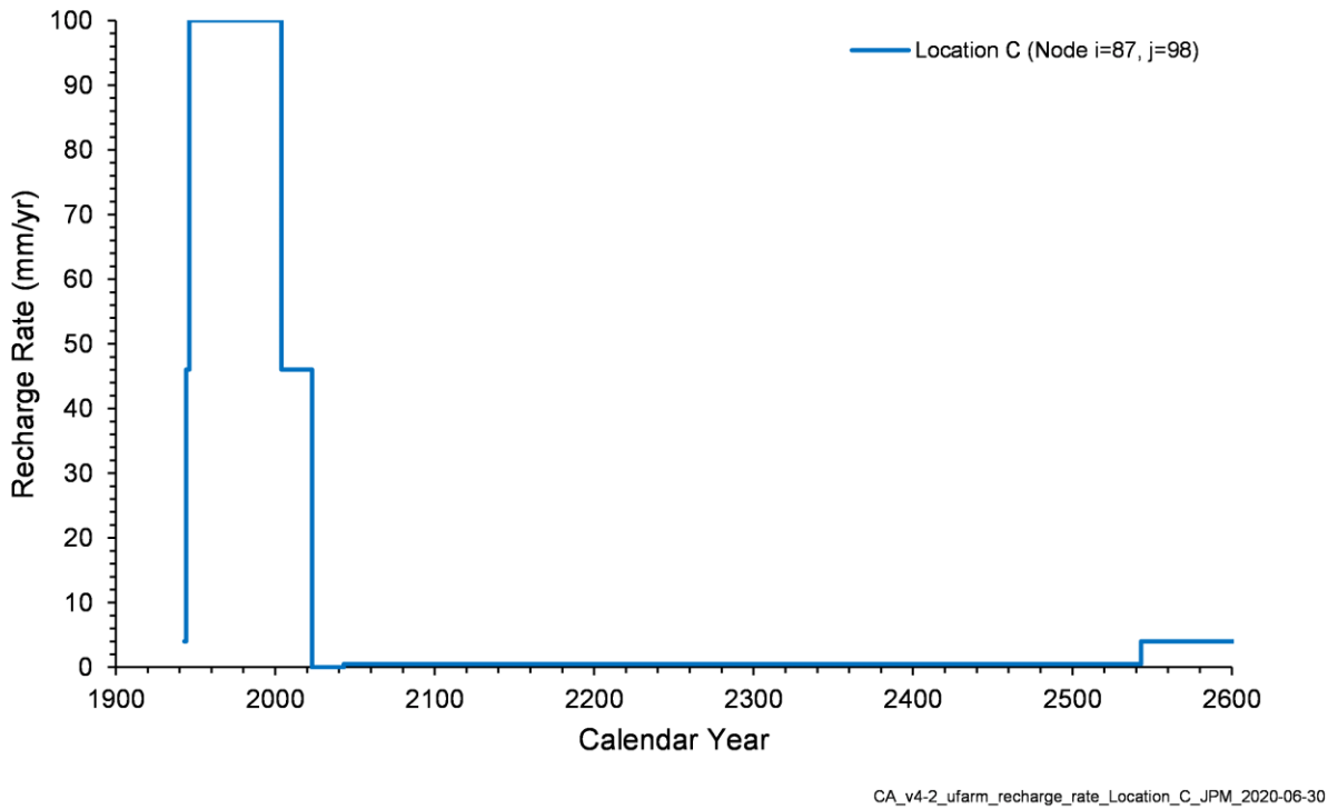
Figure 4-87. Time Series of Natural Recharge Rates, Location C
