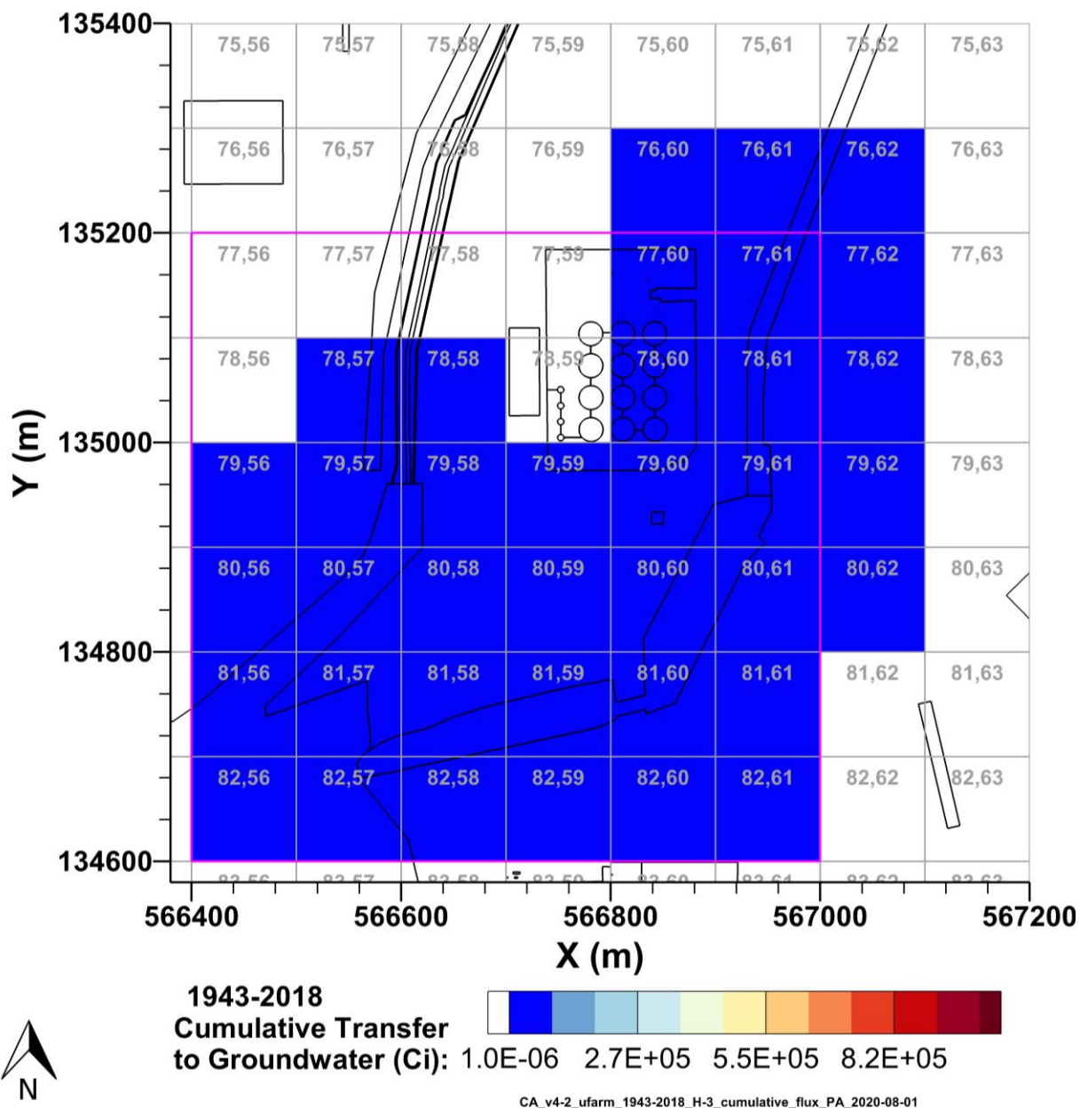
Figure 7-5. Cumulative H-3 Activity Discharged to Groundwater from the U Farm Area Model from 1943-2018 per P2R Grid Cell
