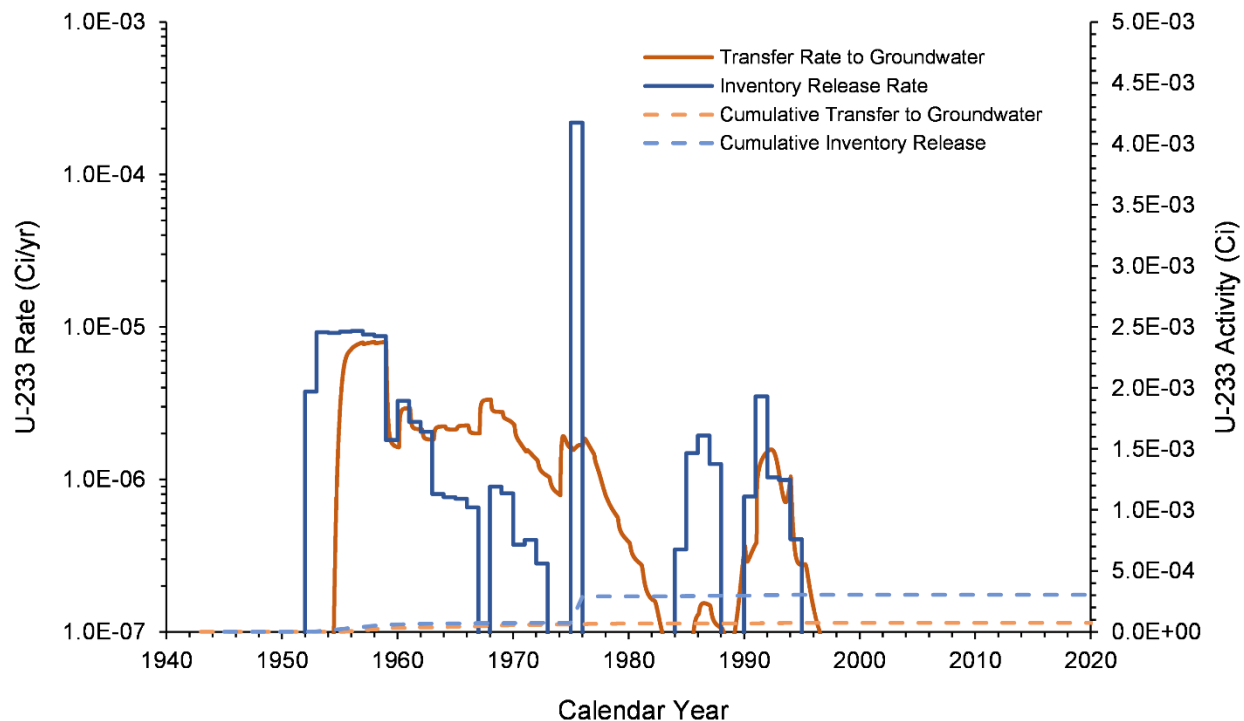
Figure 7-39. U-233 Inventory Release from Waste Sites and Transfer to Groundwater for the U Farm Area Model from 1943–2018
