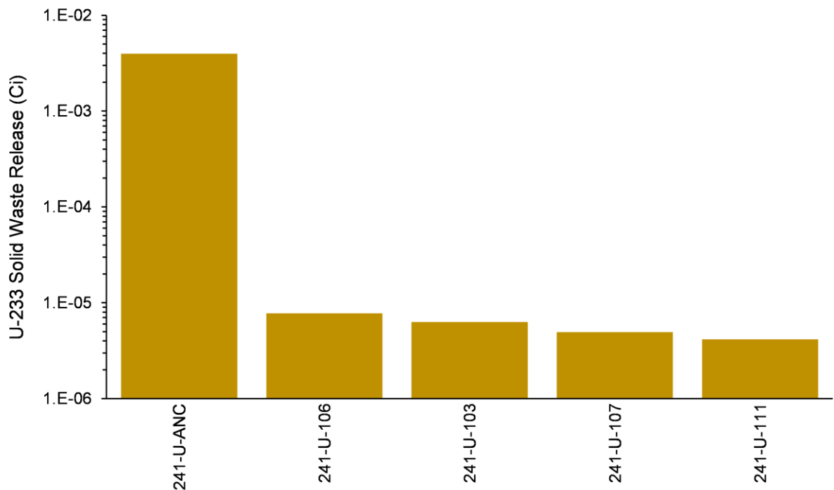
Figure 4-42. Total U-233 Activity Released from Solid Waste Sites in the U Farm Area Model
