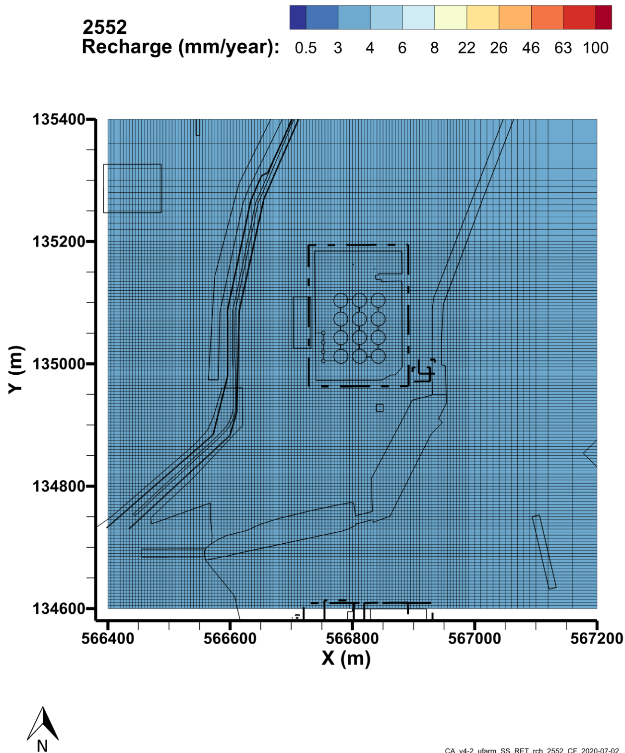
Figure 4-83. Transient Recharge Estimates for the U Farm Area Model, 2552
