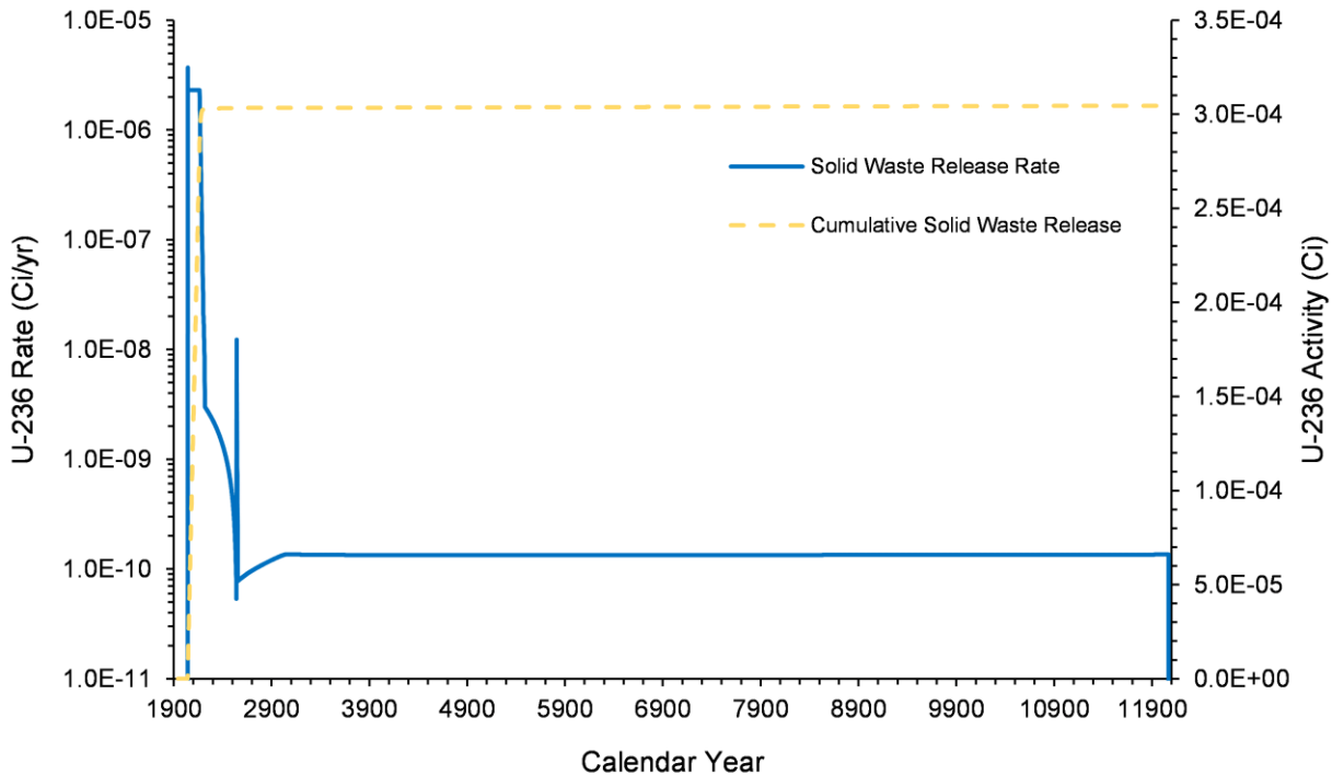
Figure 4-71. U-236 Release Rate and Cumulative Activity from Solid Waste in the U Farm Area Model, 1943–12070
