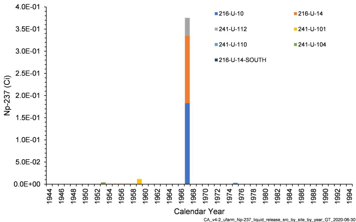
Figure 4-24. Annual Np-237 Activity Released from Liquid Waste Sites in the U Farm Area Model
