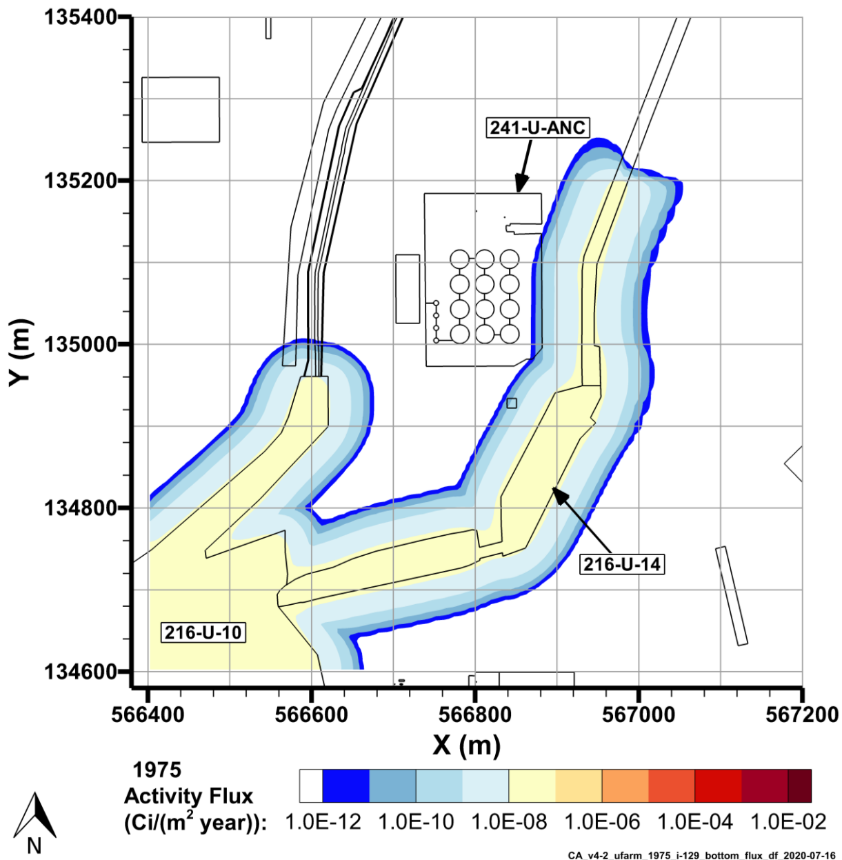
Figure 7-14. I-129 Flux to Groundwater, 1975
