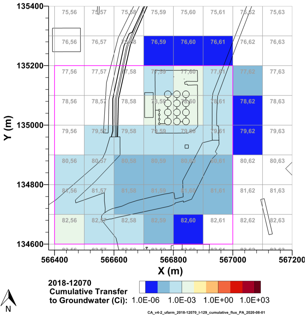
Figure 7-10. Cumulative I-129 Activity Discharged to Groundwater from the U Farm Area Model from 2018–12070 per P2R Grid Cell
