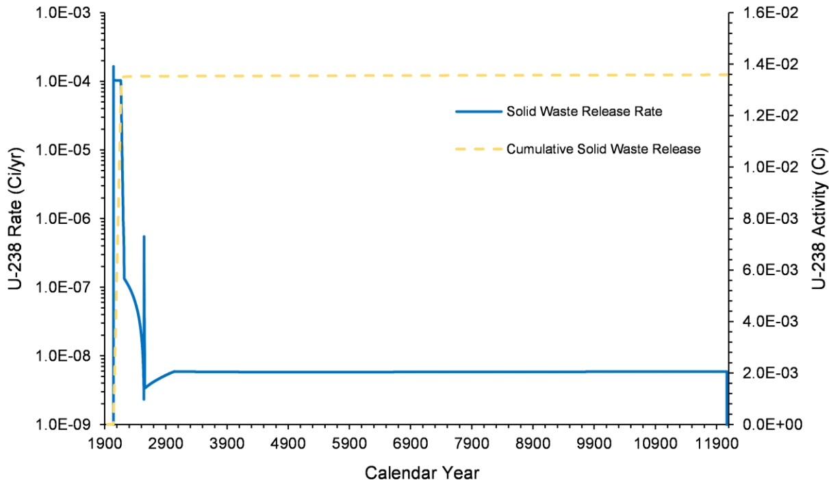
Figure 4-73. U-238 Release Rate and Cumulative Activity from Solid Waste in the U Farm Area Model, 1943–12070
