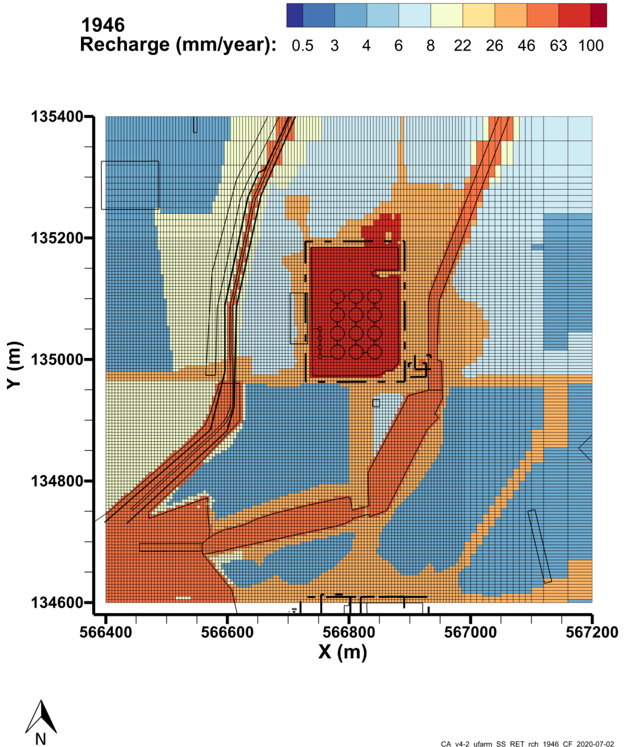
Figure 4-79. Transient Recharge Estimates for the U Farm Area Model, 1946
