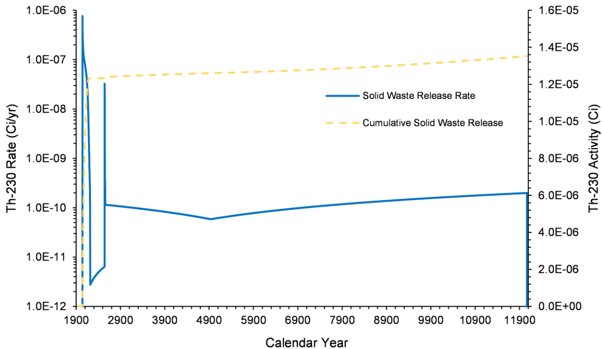
Figure 4-61. Th-230 Release Rate and Cumulative Activity from Solid Waste in the U Farm Area Model, 1943–12070
