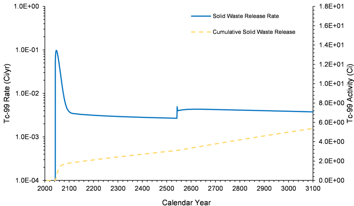
Figure 4-58. Tc-99 Release Rate and Cumulative Activity from Solid Waste in the U Farm Area Model, 2018–3070
