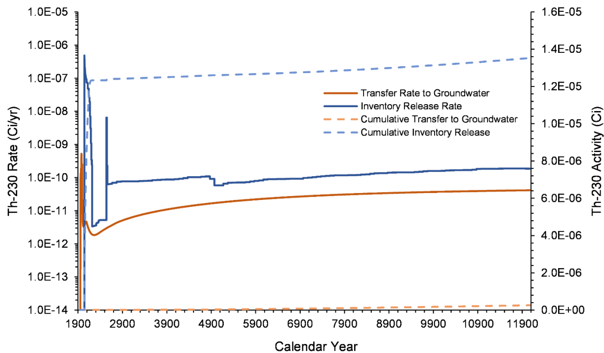
Figure 7-60. Th-230 Inventory Release from Waste Sites and Transfer to Groundwater for the U Farm Area Model from 1943–12070
