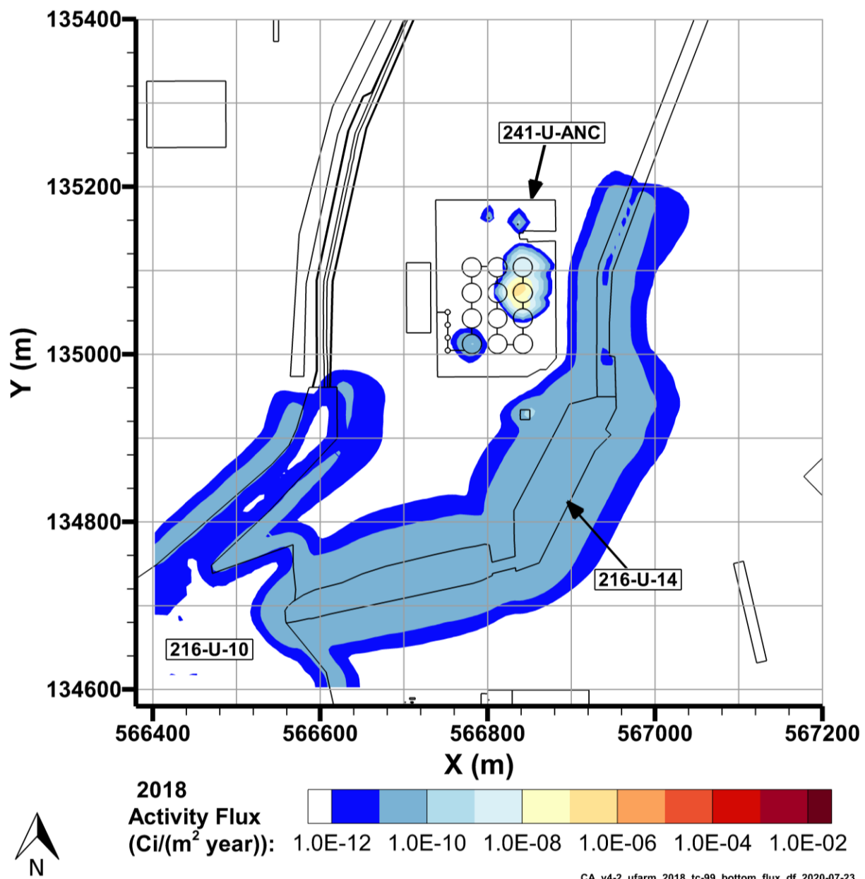
Figure 7-29. Tc-99 Flux to Groundwater, 2018
