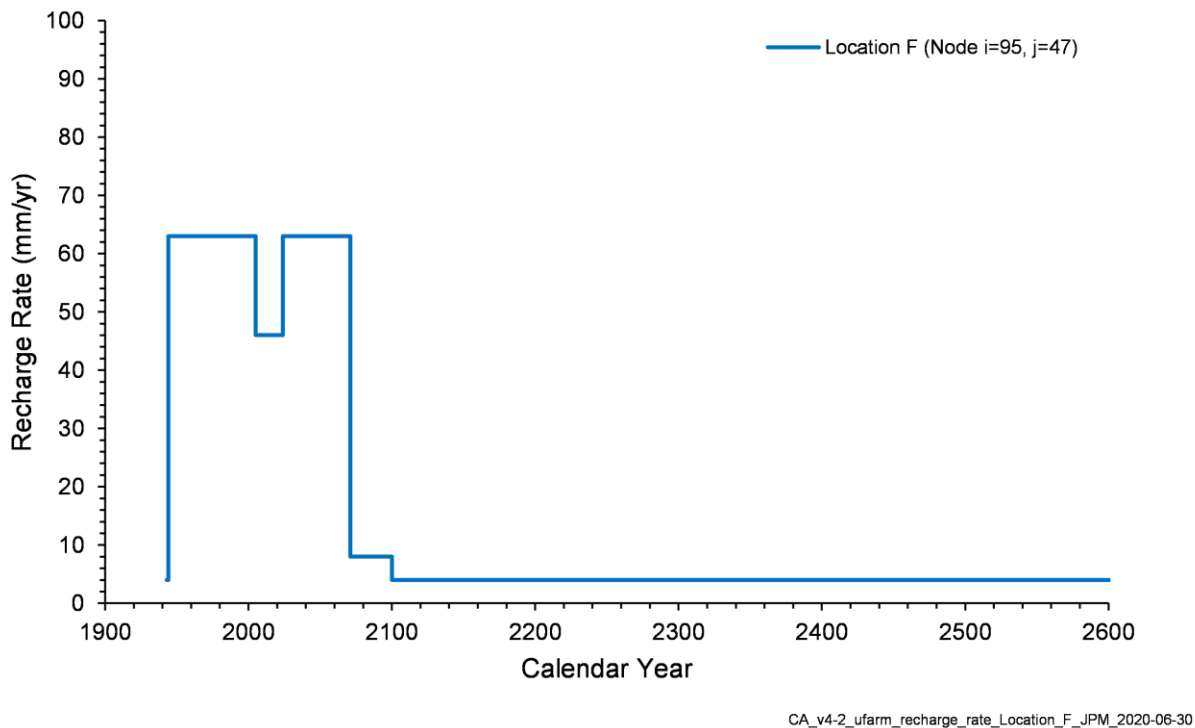
Figure 4-90. Time Series of Natural Recharge Rates, Location F
