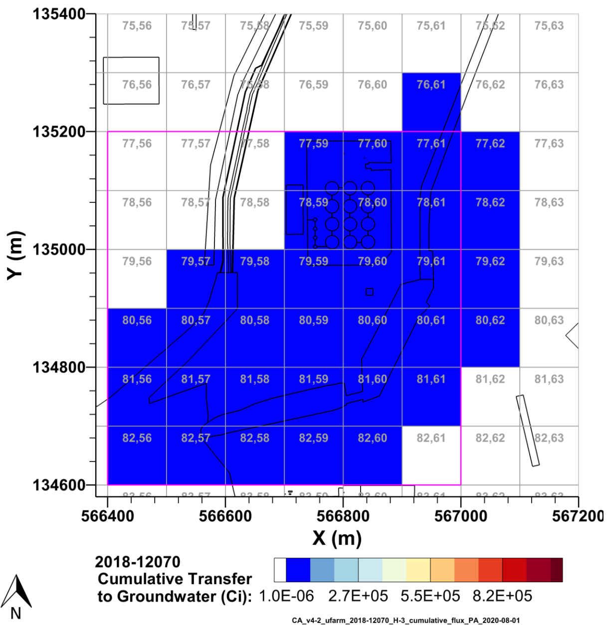
Figure 7-6. Cumulative H-3 Activity Discharged to Groundwater from the U Farm Area Model from 2018–12070 per P2R Grid Cell
