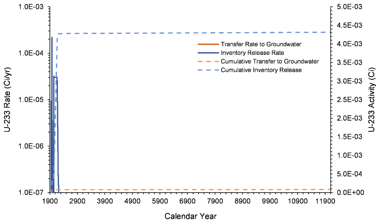
Figure 7-40. U-233 Inventory Release from Waste Sites and Transfer to Groundwater for the U Farm Area Model from 1943–12070
