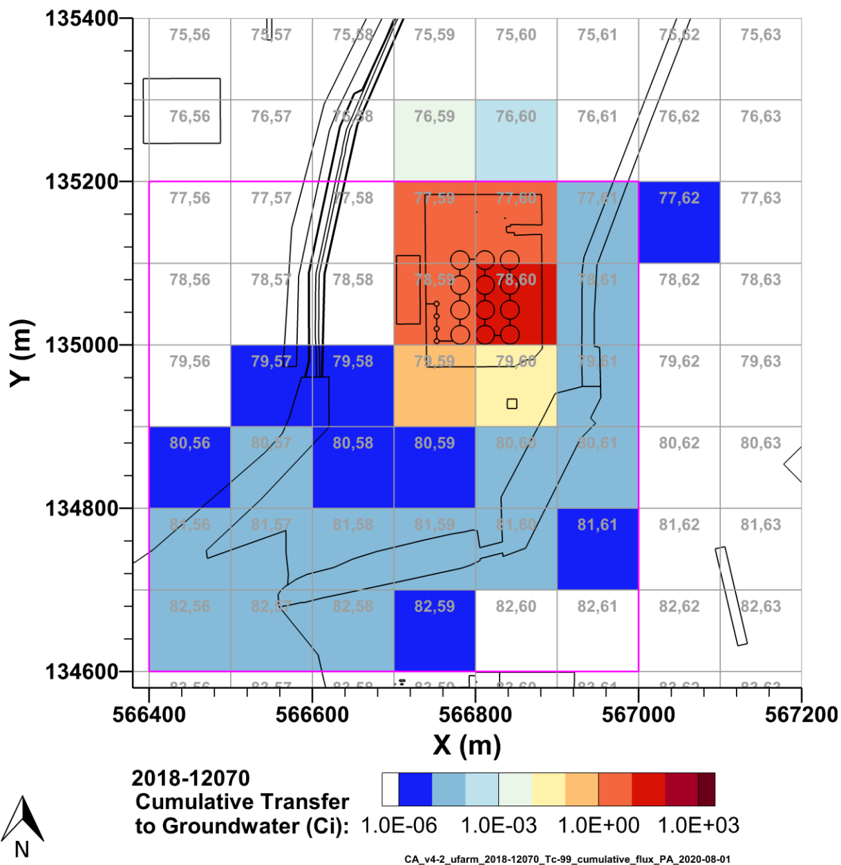
Figure 7-25. Cumulative Tc-99 Activity Discharged to Groundwater from the U Farm Area Model from 2018–12070 per P2R Grid Cell
