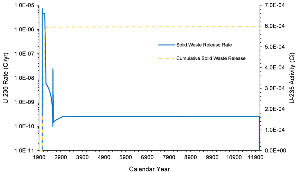
Figure 4-69. U-235 Release Rate and Cumulative Activity from Solid Waste in the U Farm Area Model, 1943–12070
