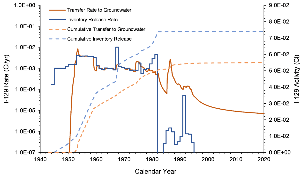
Figure 7-11. I-129 Inventory Release from Waste Sites and Transfer to Groundwater for the U Farm Area Model from 1943–2018
