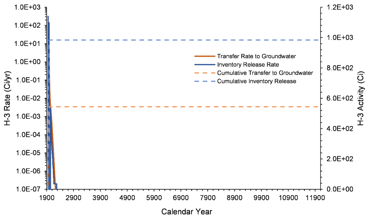
Figure 7-8. H-3 Inventory Release from Waste Sites and Transfer to Groundwater for the U Farm Area Model from 1943–12070
