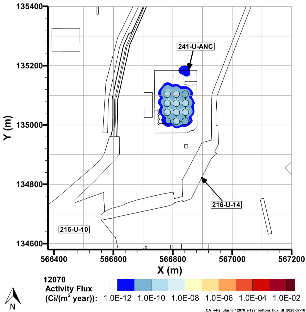
Figure 7-19. I-129 Flux to Groundwater, 12070
