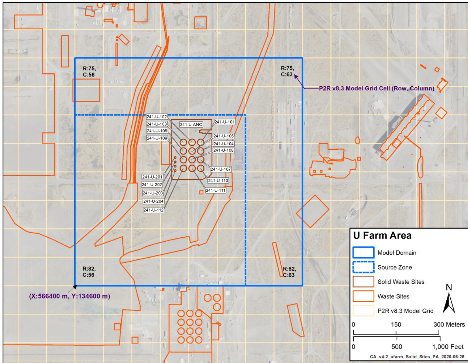
Figure 4-8. Waste Sites in the U Farm Area Model with Solid Source Inventory
