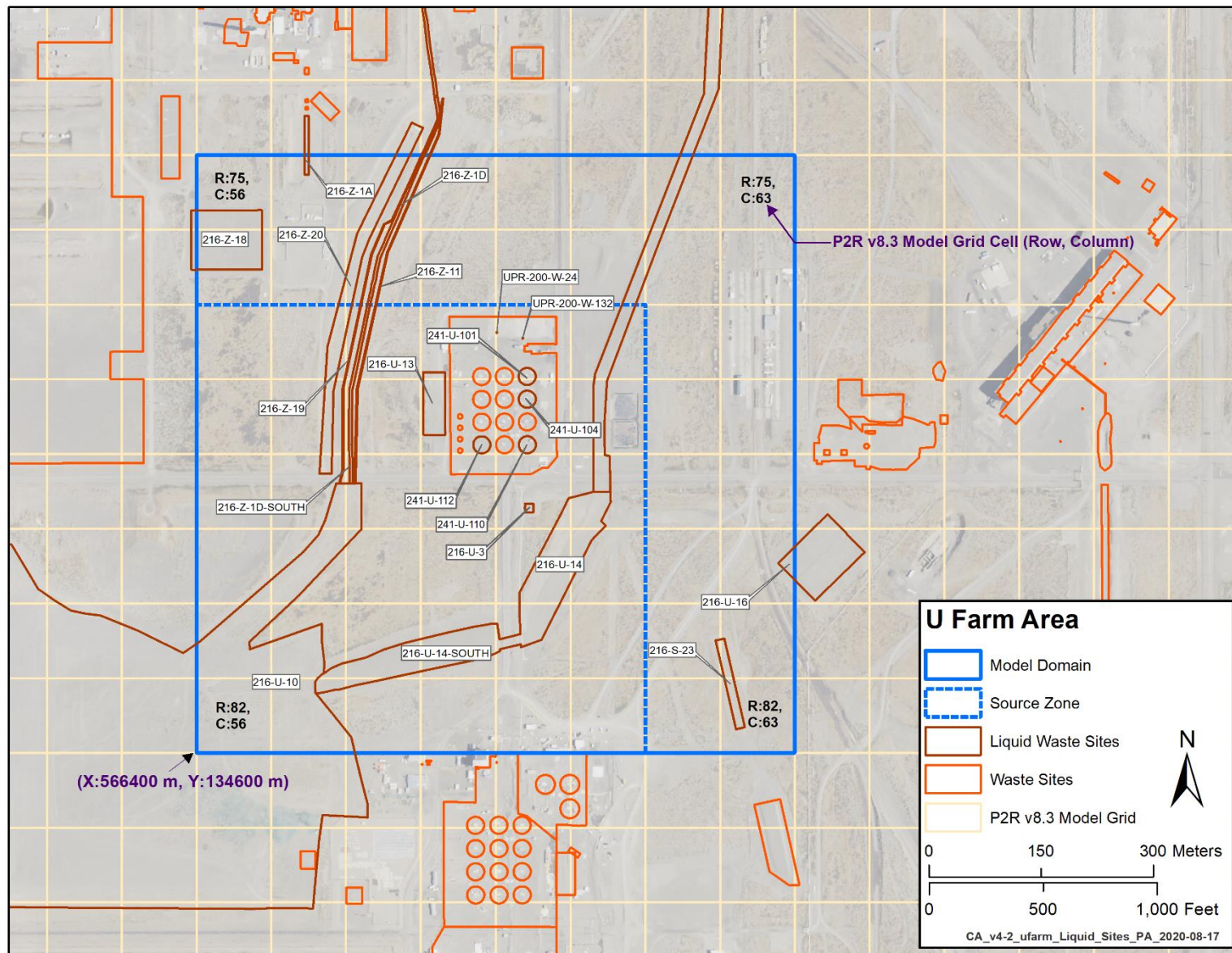
Figure 4-7. Waste Sites in the U Farm Area Model with Liquid Source Inventory
