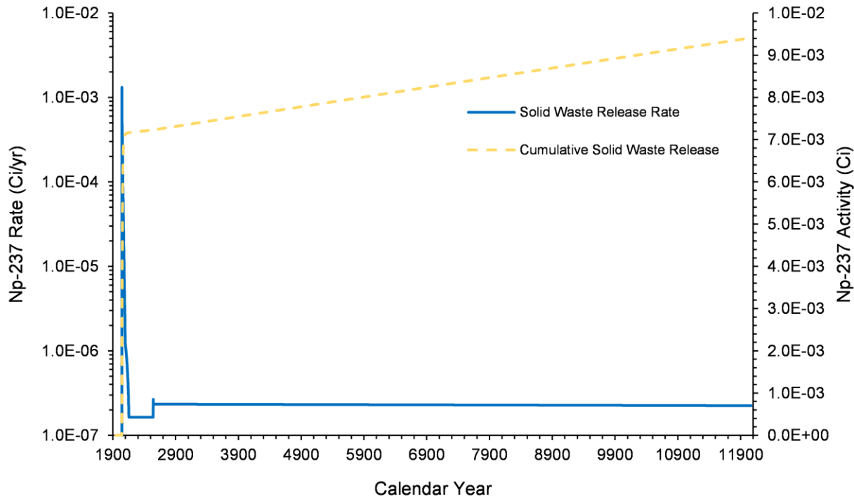
Figure 4-53. Np-237 Release Rate and Cumulative Activity from Solid Waste in the U Farm Area Model, 1943–12070
