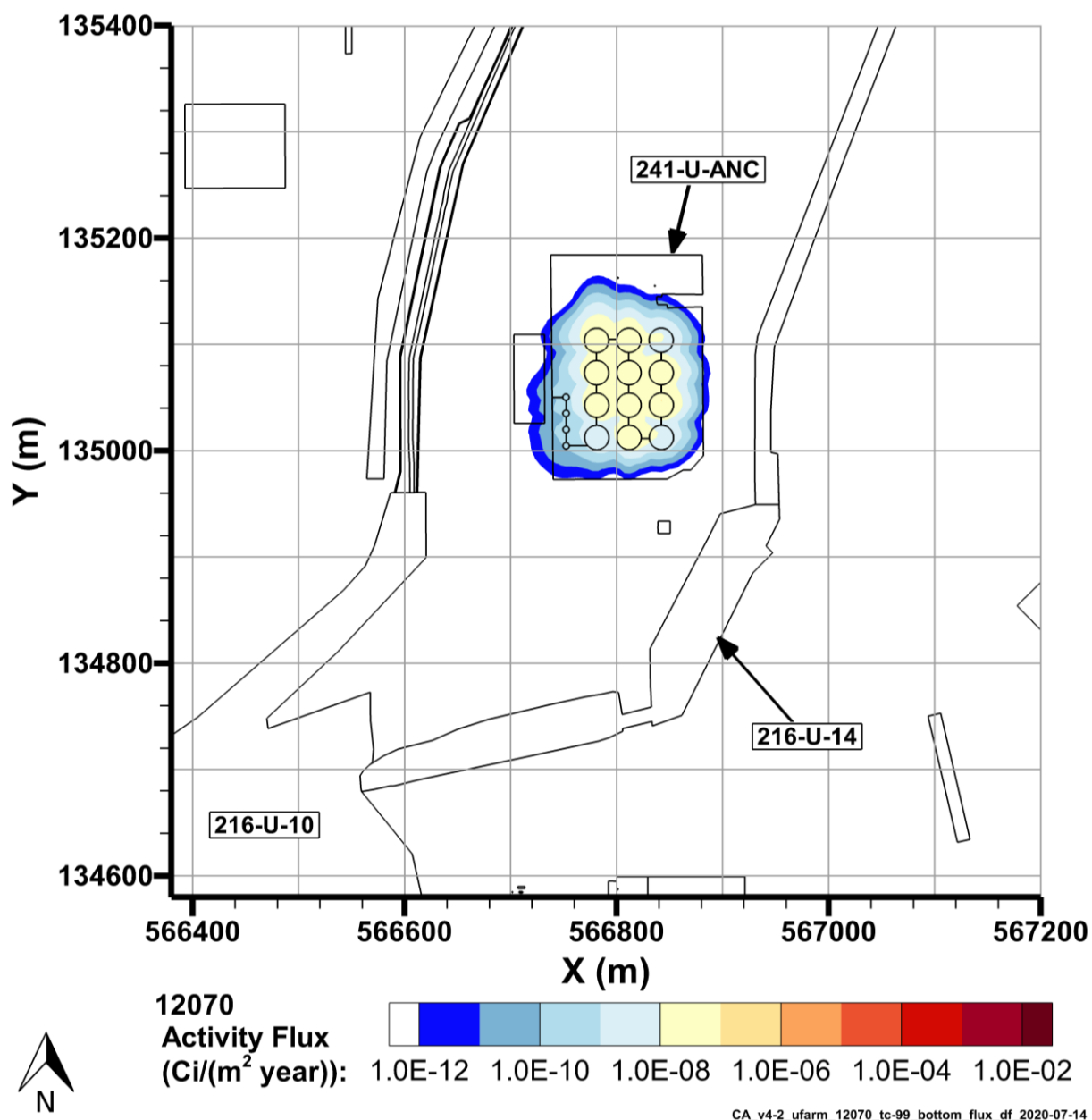
Figure 7-34. Tc-99 Flux to Groundwater, 12070
