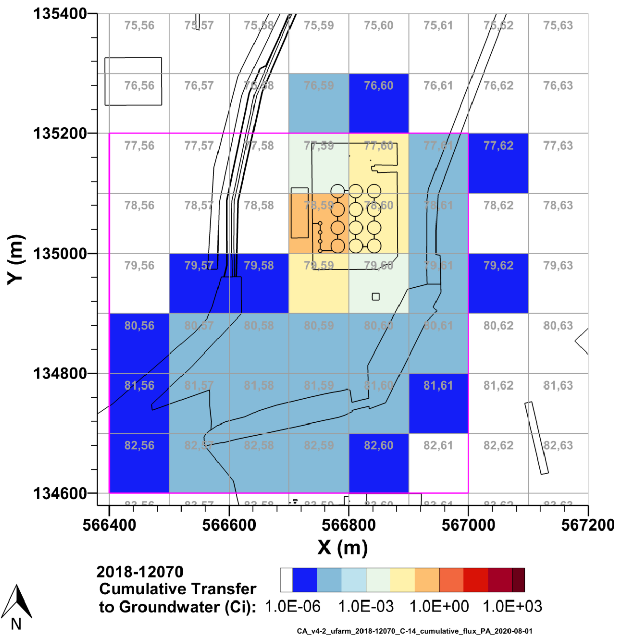
Figure 7-2. Cumulative C-14 Activity Discharged to Groundwater from the U Farm Area Model from 2018–12070 per P2R Grid Cell
