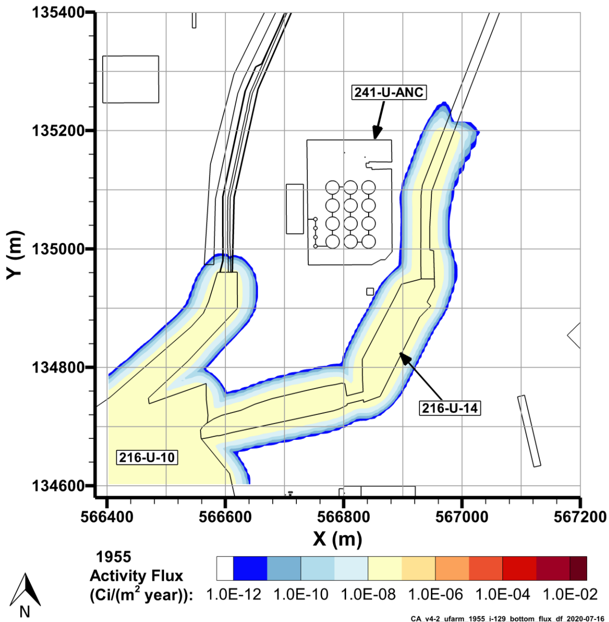
Figure 7-13. I-129 Flux to Groundwater, 1955
