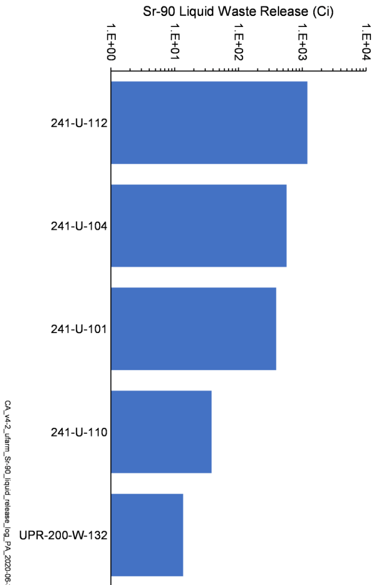
Figure 4-13. Total Sr-90 Activity Released from Liquid Waste Sites in the U Farm Area Model
