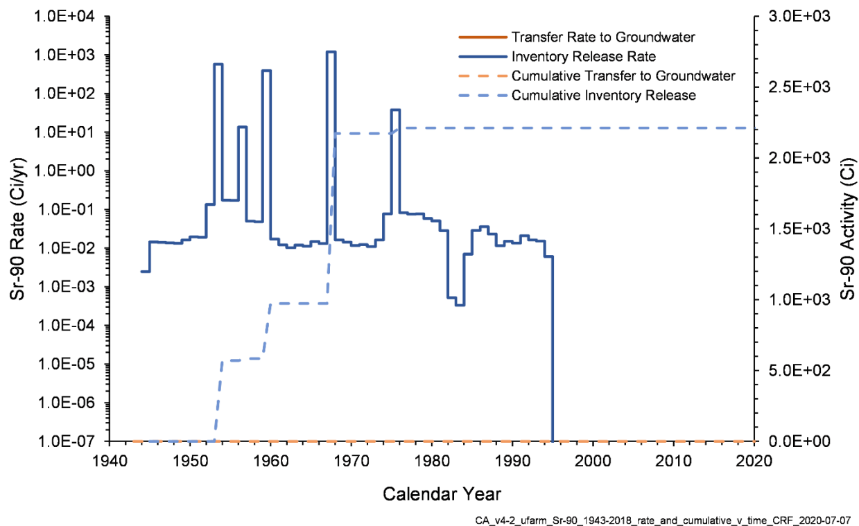
Figure 7-22. Sr-90 Inventory Release from Waste Sites and Transfer to Groundwater for the U Farm Area Model from 1943–2018
