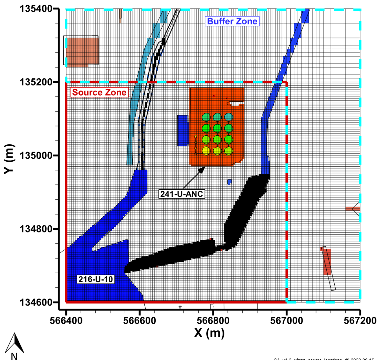
Figure 4-91. Distribution of Source Nodes in the U Farm Area Model
