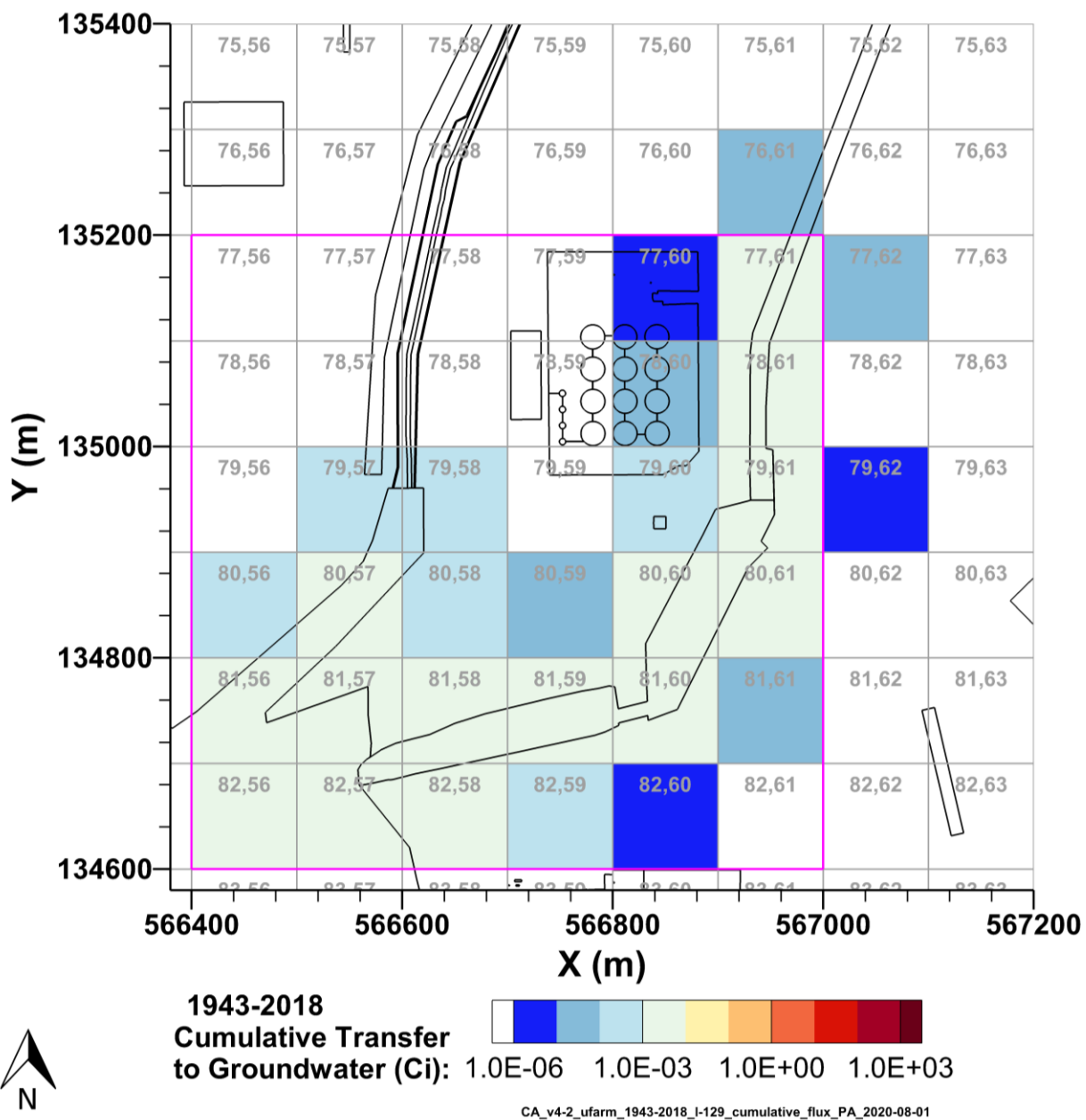
Figure 7-9. Cumulative I-129 Activity Discharged to Groundwater from the U Farm Area Model from 1943–2018 per P2R Grid Cell
