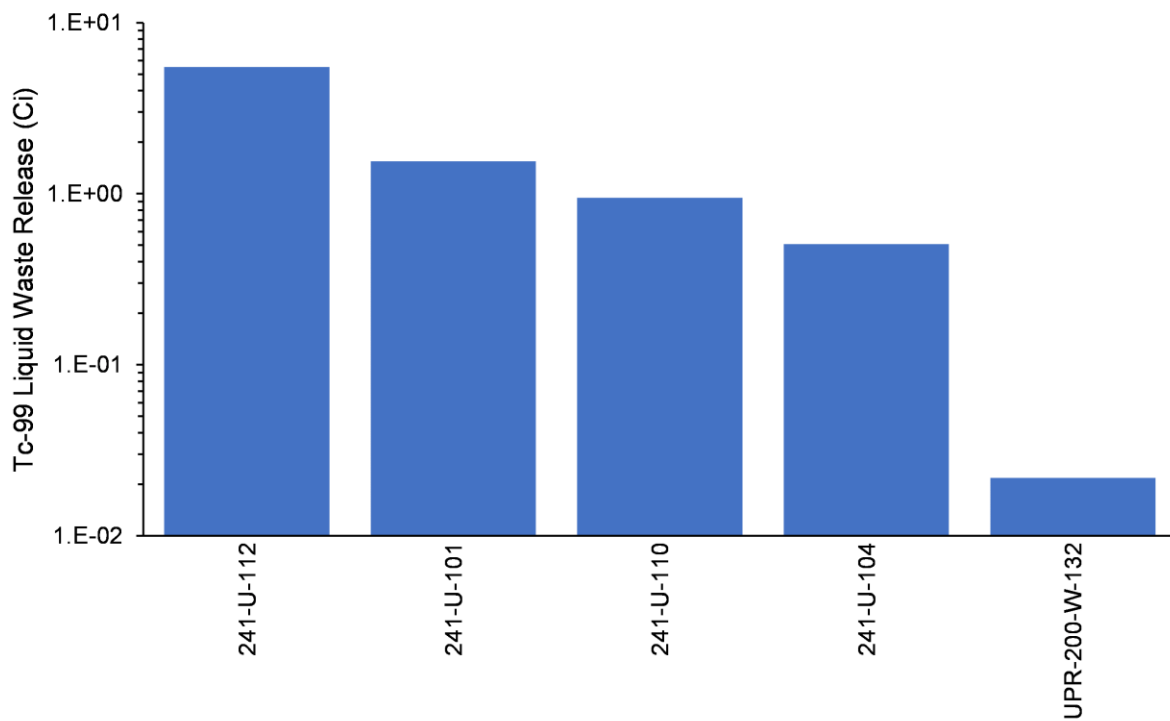
Figure 4-14. Total Tc-99 Activity Released from Liquid Waste Sites in the U Farm Area Model
