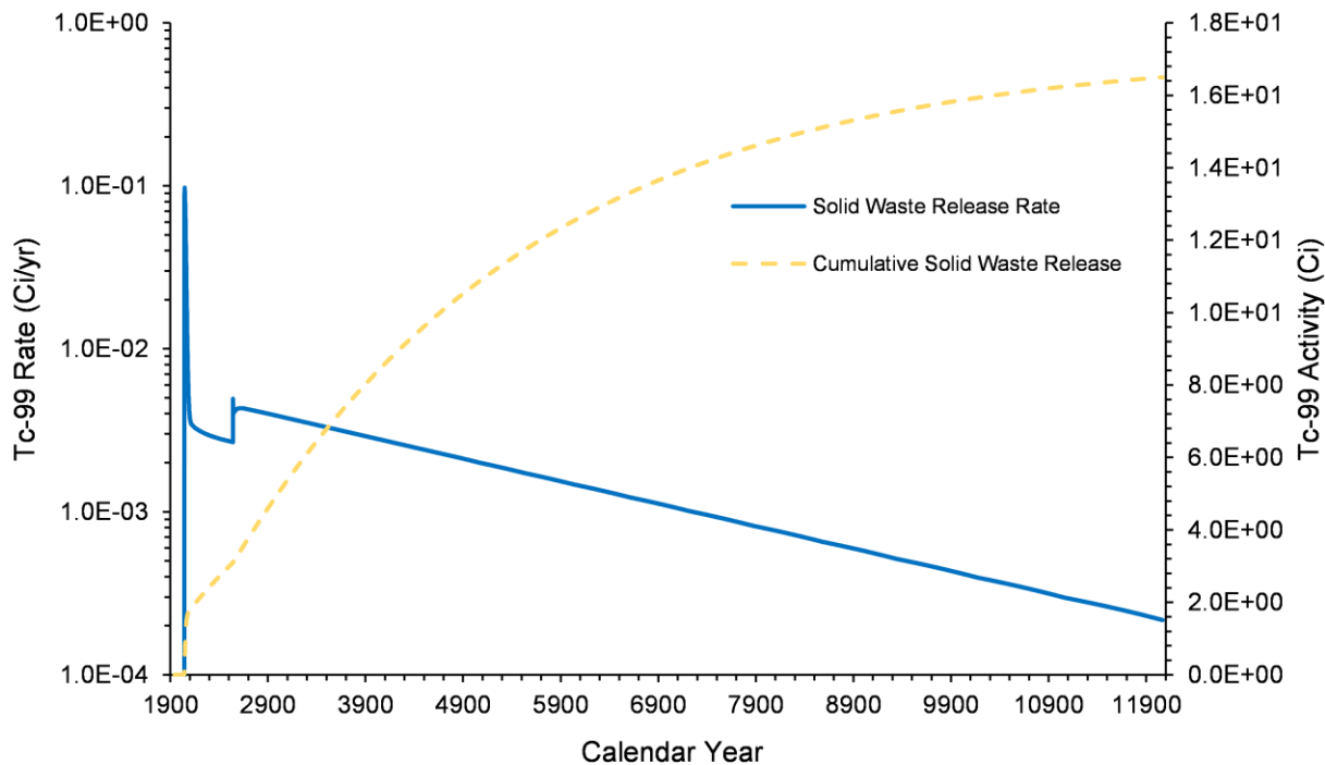
Figure 4-57. Tc-99 Release Rate and Cumulative Activity from Solid Waste in the U Farm Area Model, 1943–12070
