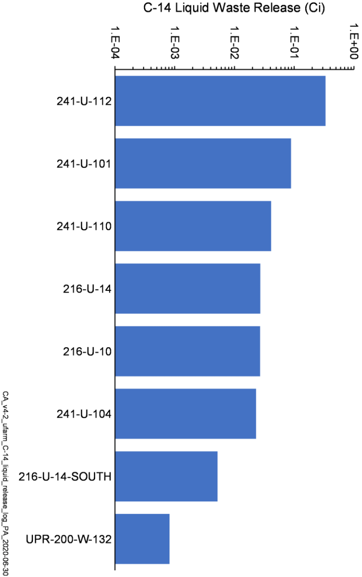
Figure 4-9. Total C-14 Activity Released from Liquid Waste Sites in the U Farm Area Model
