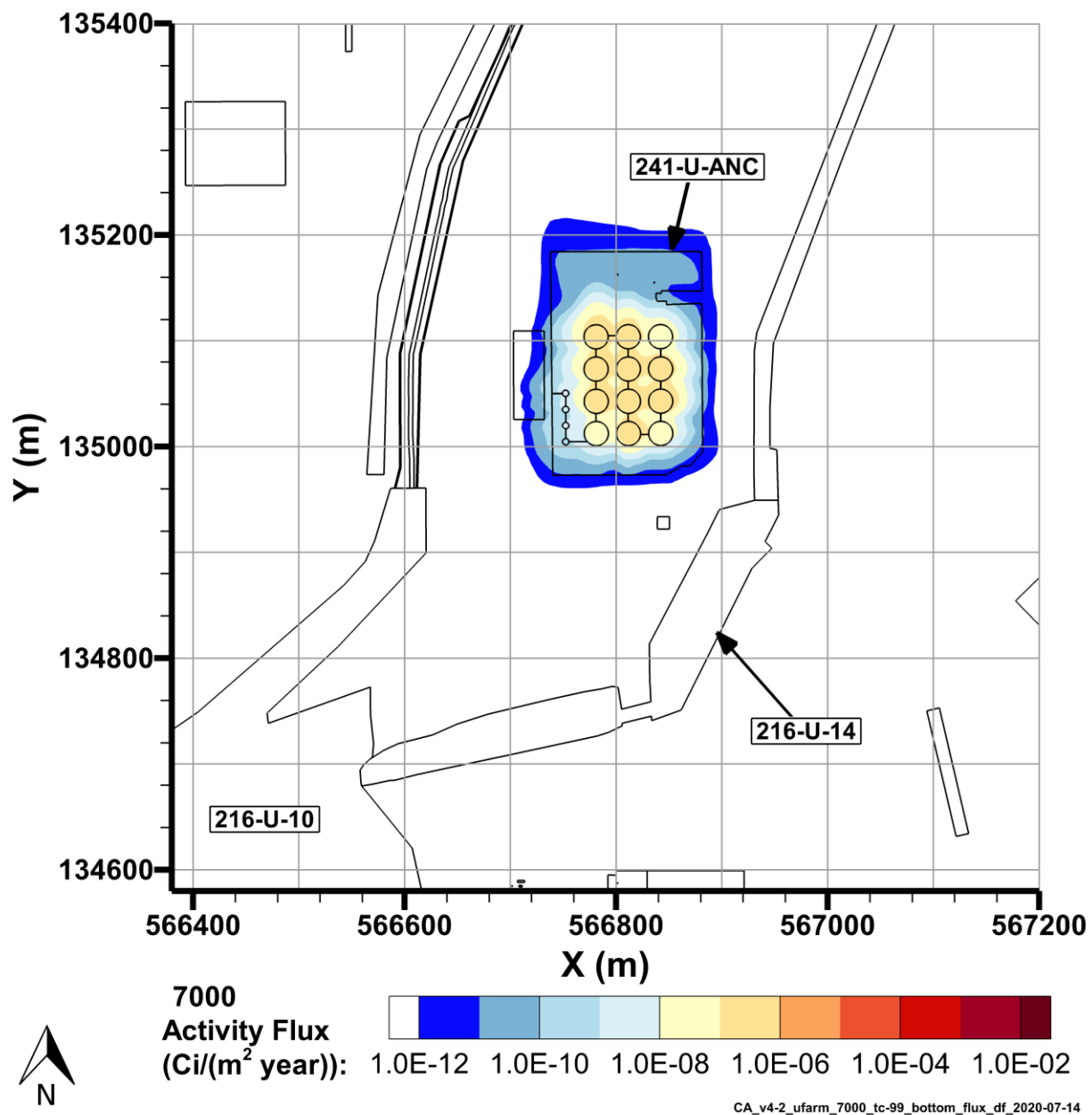
Figure 7-33. Tc-99 Flux to Groundwater, 7000
