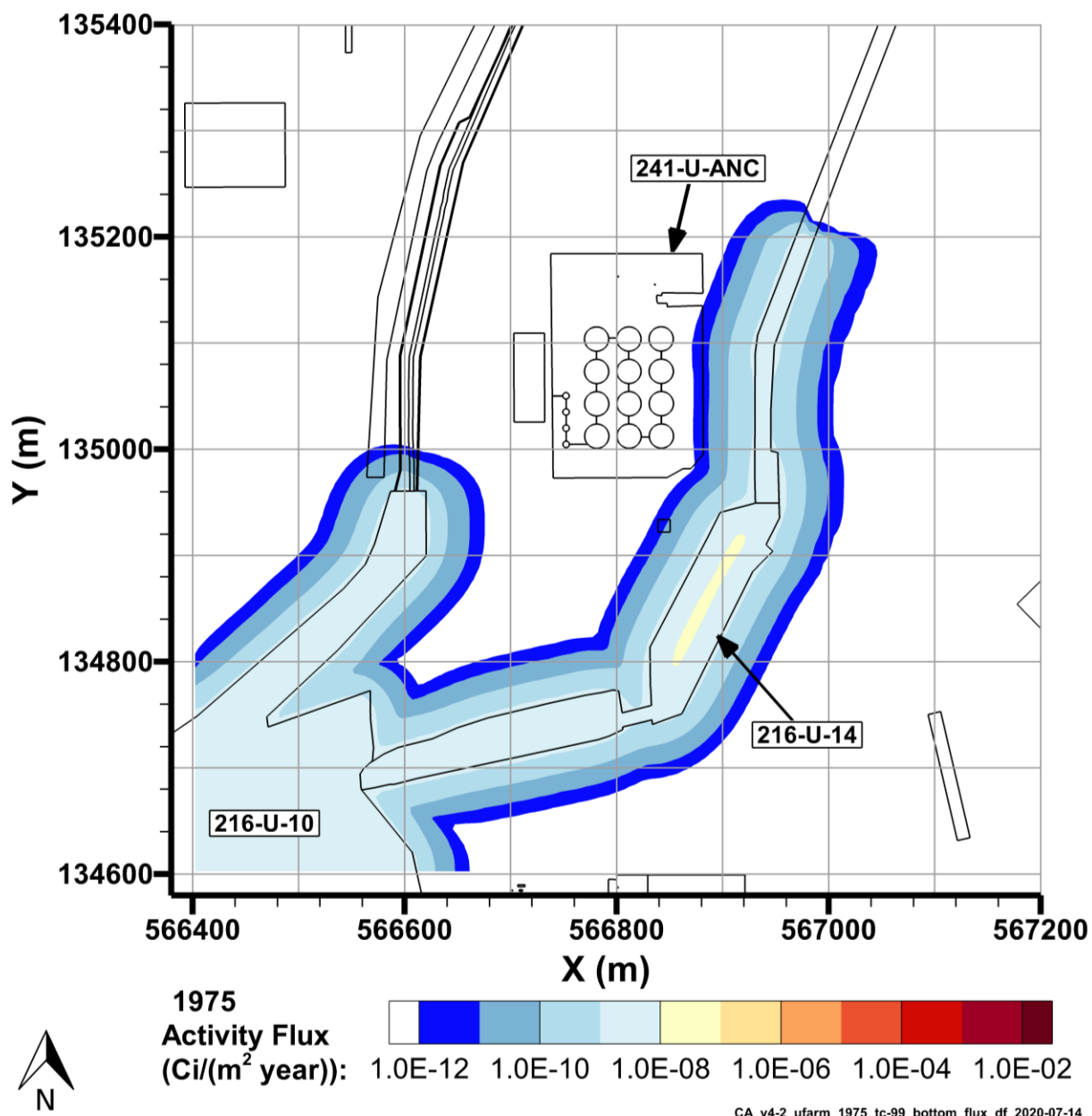
Figure 7-28. Tc-99 Flux to Groundwater, 1975
