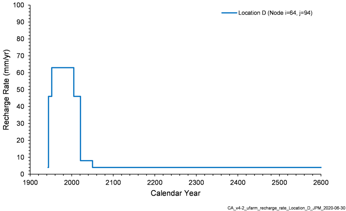
Figure 4-88. Time Series of Natural Recharge Rates, Location D
