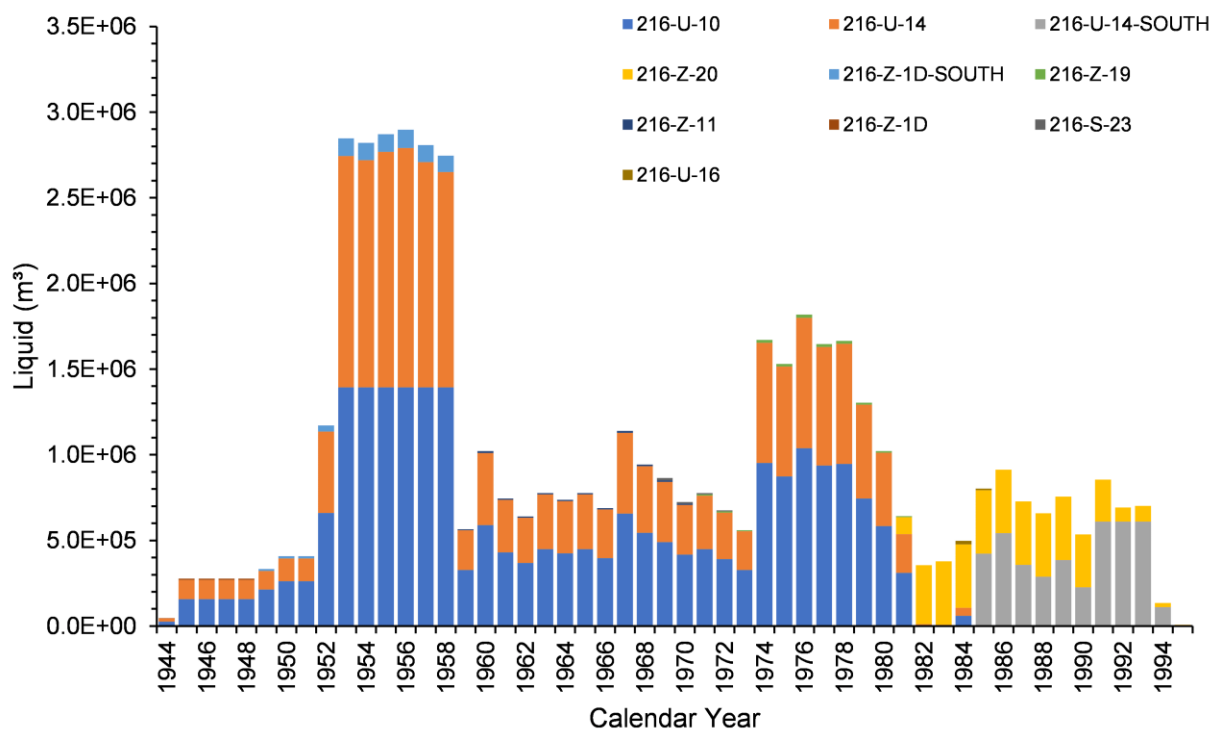
Figure 4-76. Total Volume of Water Released by Year from Liquid Waste Sites in the U Farm Area Model
