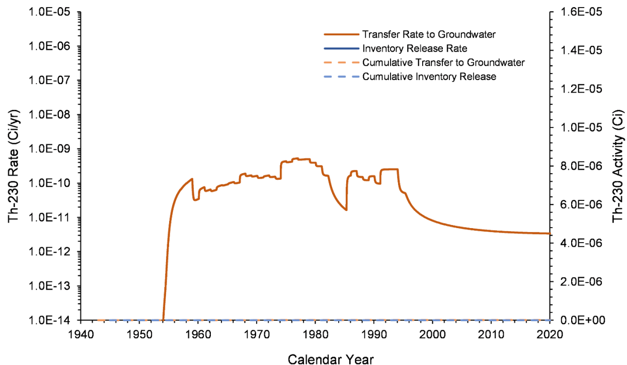
Figure 7-59. Th-230 Inventory Release from Waste Sites and Transfer to Groundwater for the U Farm Area Model from 1943–2018
