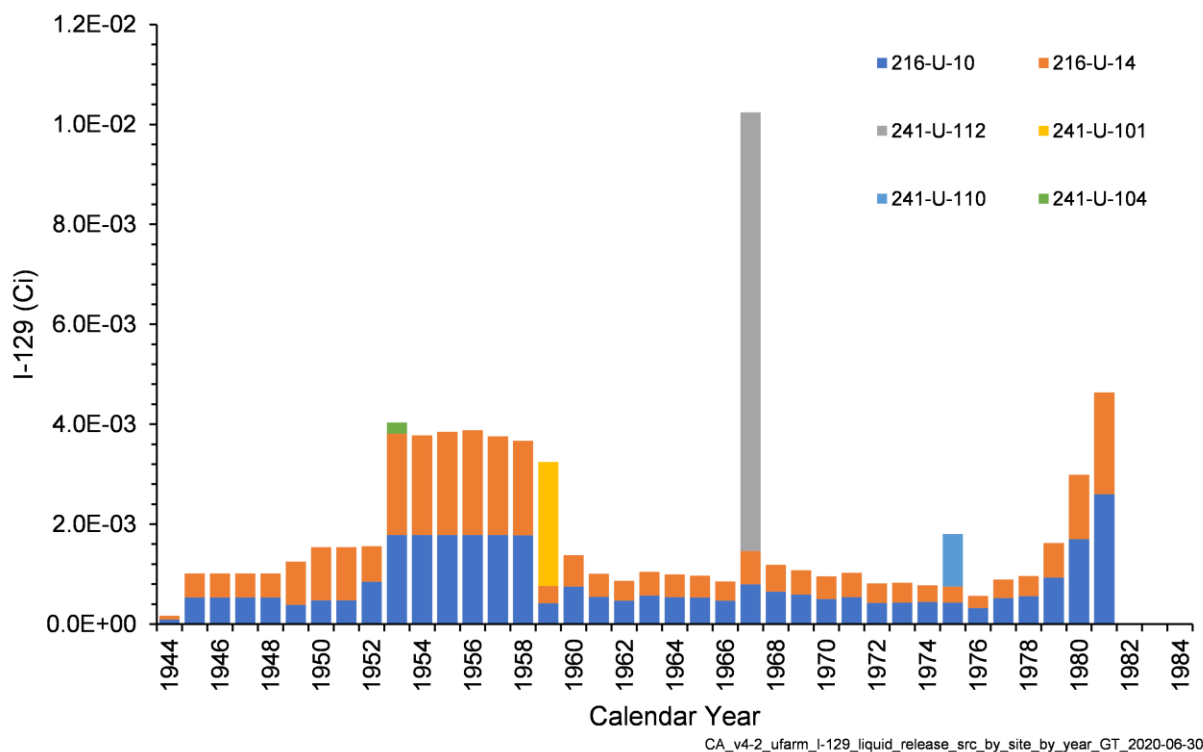
Figure 4-23. Annual I-129 Activity Released from Liquid Waste Sites in the U Farm Area Model
