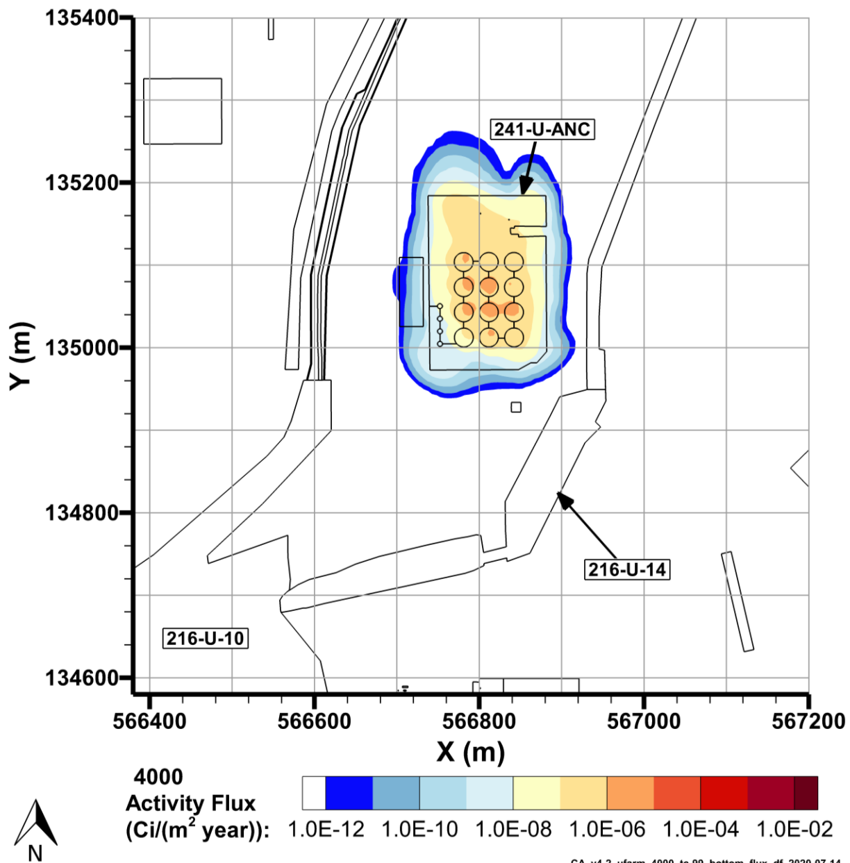
Figure 7-32. Tc-99 Flux to Groundwater, 4000
