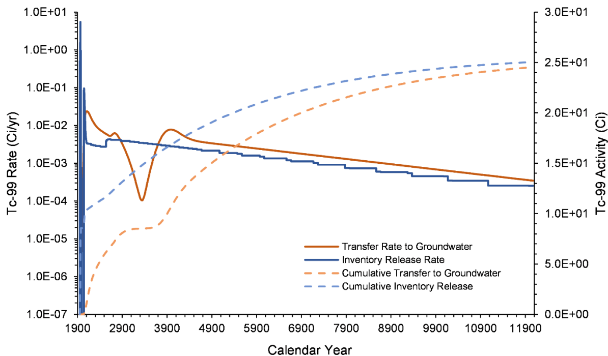
Figure 7-27. Tc-99 Inventory Release from Waste Sites and Transfer to Groundwater for the U Farm Area Model from 1943–12070
