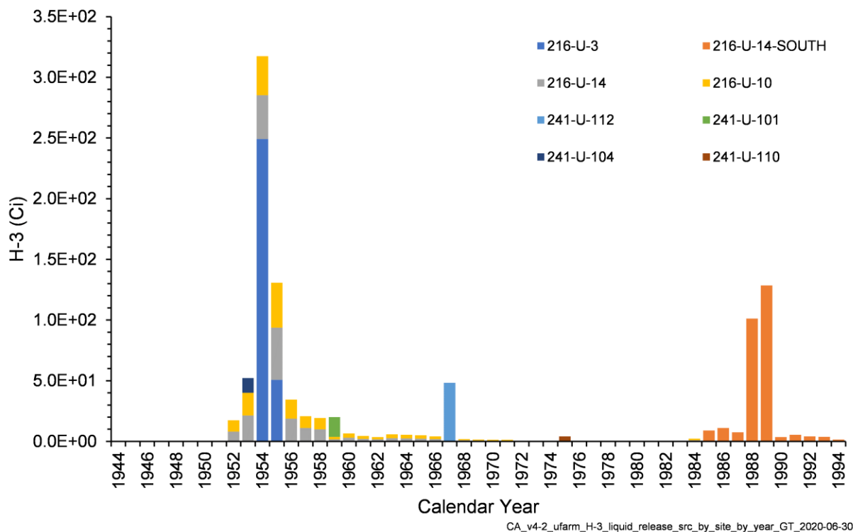
Figure 4-22. Annual H-3 Activity Released from Liquid Waste Sites in the U Farm Area Model
