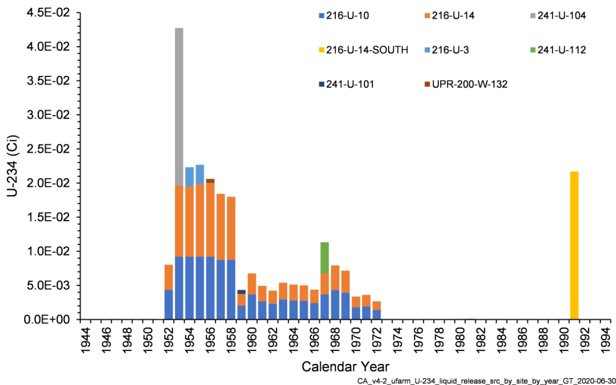
Figure 4-29. Annual U-234 Activity Released from Liquid Waste Sites in the U Farm Area Model
