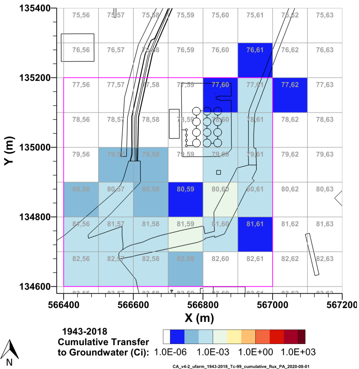
Figure 7-24. Cumulative Tc-99 Activity Discharged to Groundwater from the U Farm Area Model from 1943–2018 per P2R Grid Cell
