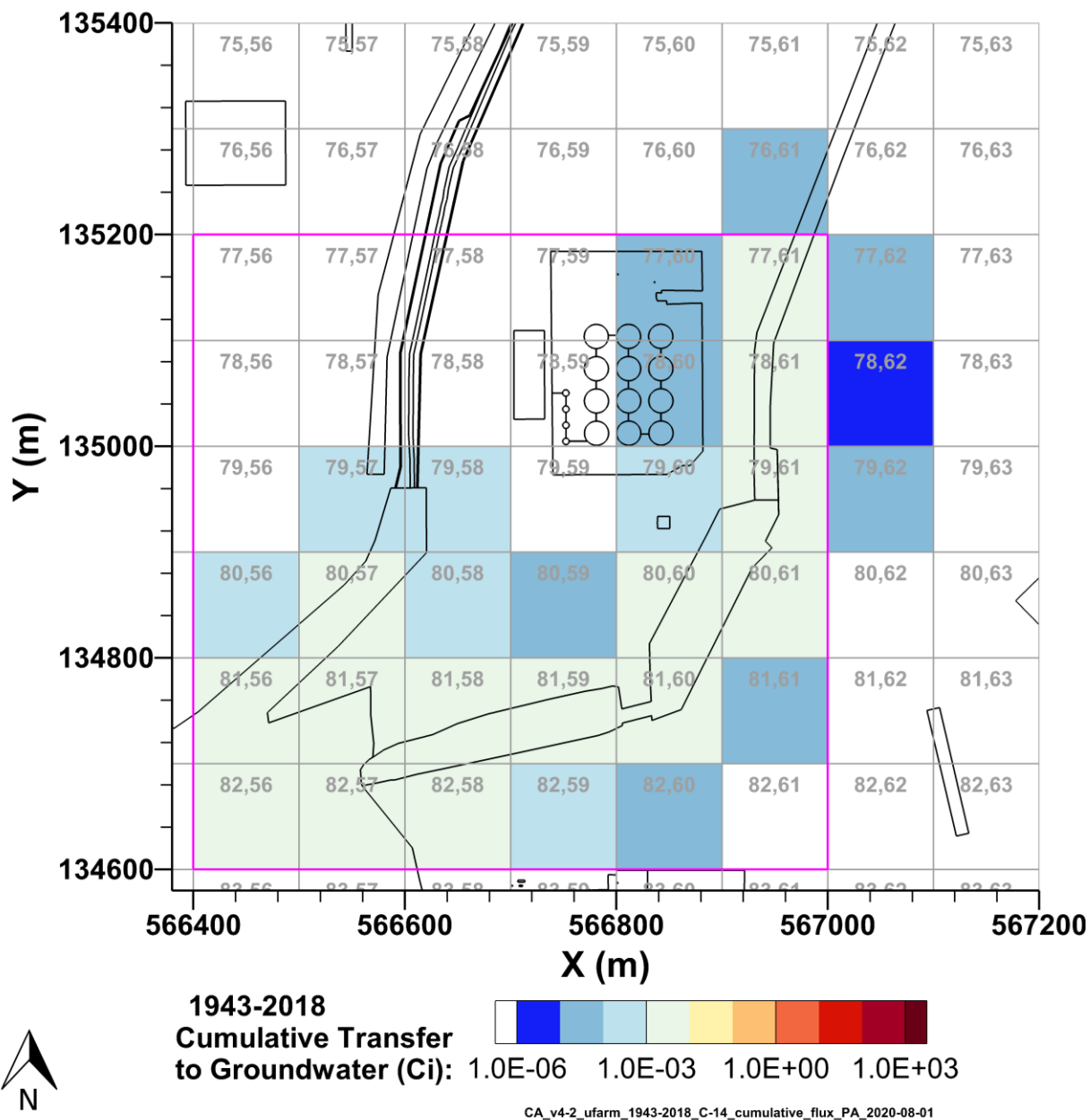
Figure 7-1. Cumulative C-14 Activity Discharged to Groundwater from the U Farm Area Model from 1943–2018 per P2R Grid Cell
