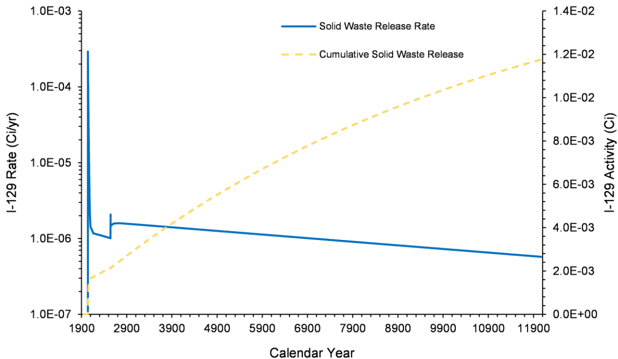
Figure 4-51. I-129 Release Rate and Cumulative Activity from Solid Waste in the U Farm Area Model, 1943–12070
