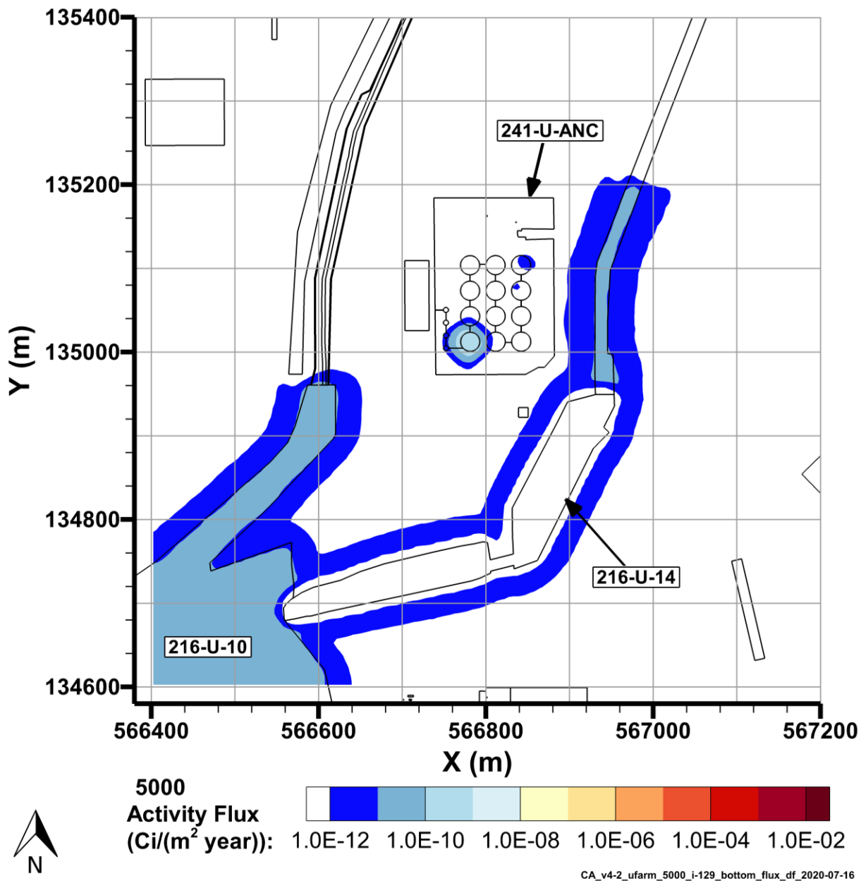
Figure 7-17. I-129 Flux to Groundwater, 5000
