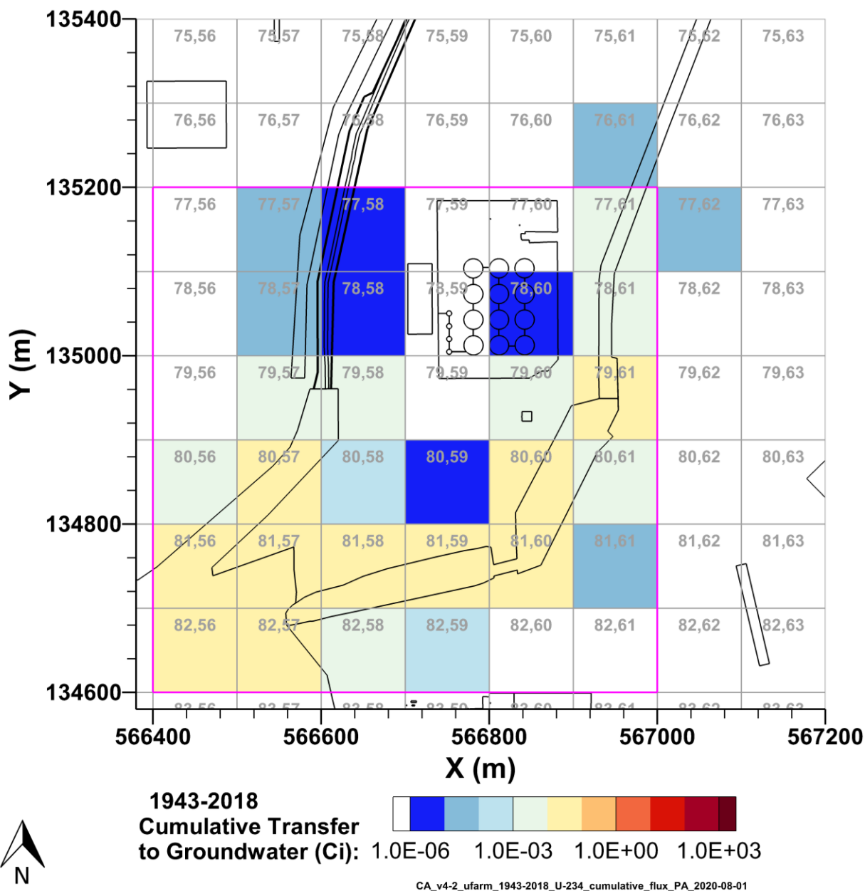
Figure 7-41. Cumulative U-234 Activity Discharged to Groundwater from the U Farm Area Model from 1943–2018 per P2R Grid Cell
