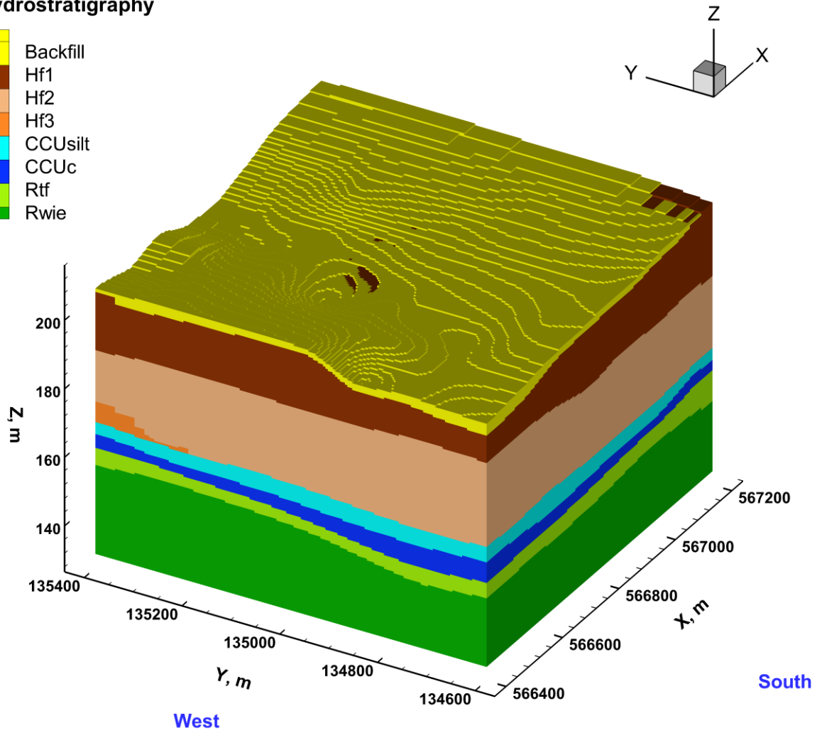
Figure 4-5. Model Hydrostratigraphy Three-Dimensional View Showing the South and West Faces
