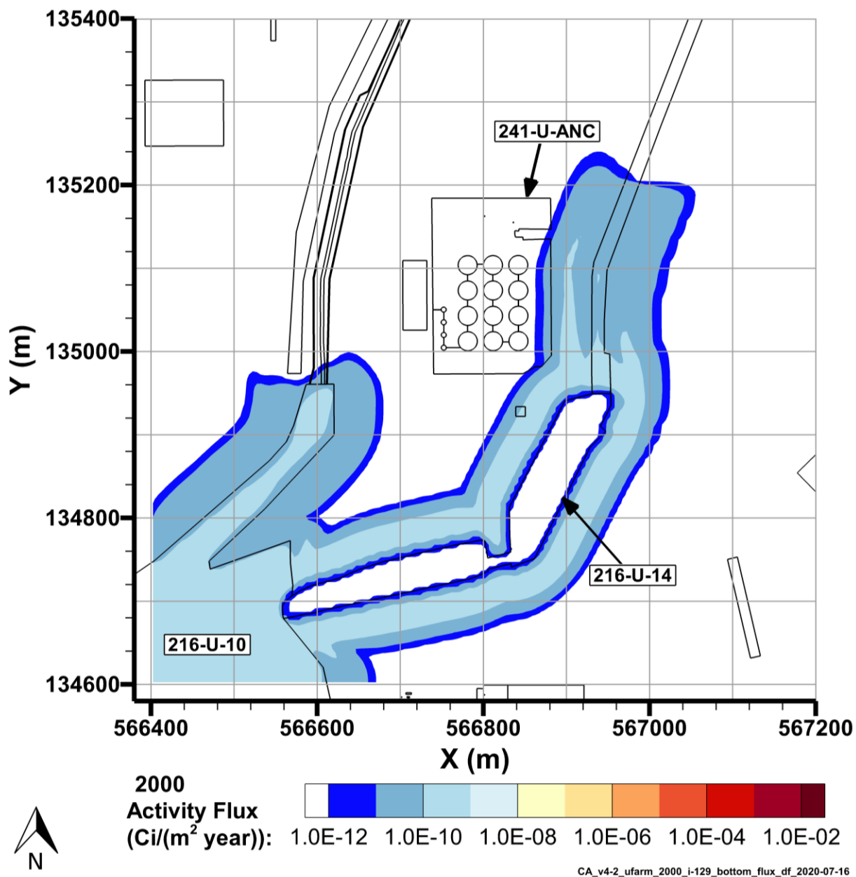
Figure 7-15. I-129 Flux to Groundwater, 2000
