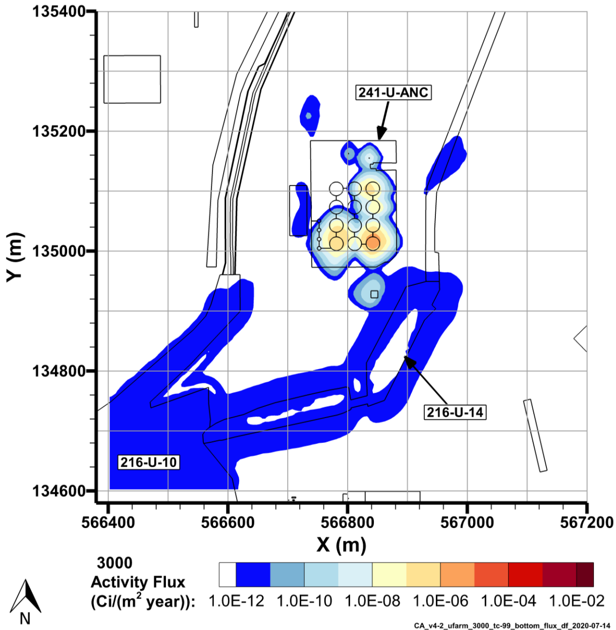
Figure 7-31. Tc-99 Flux to Groundwater, 3000
