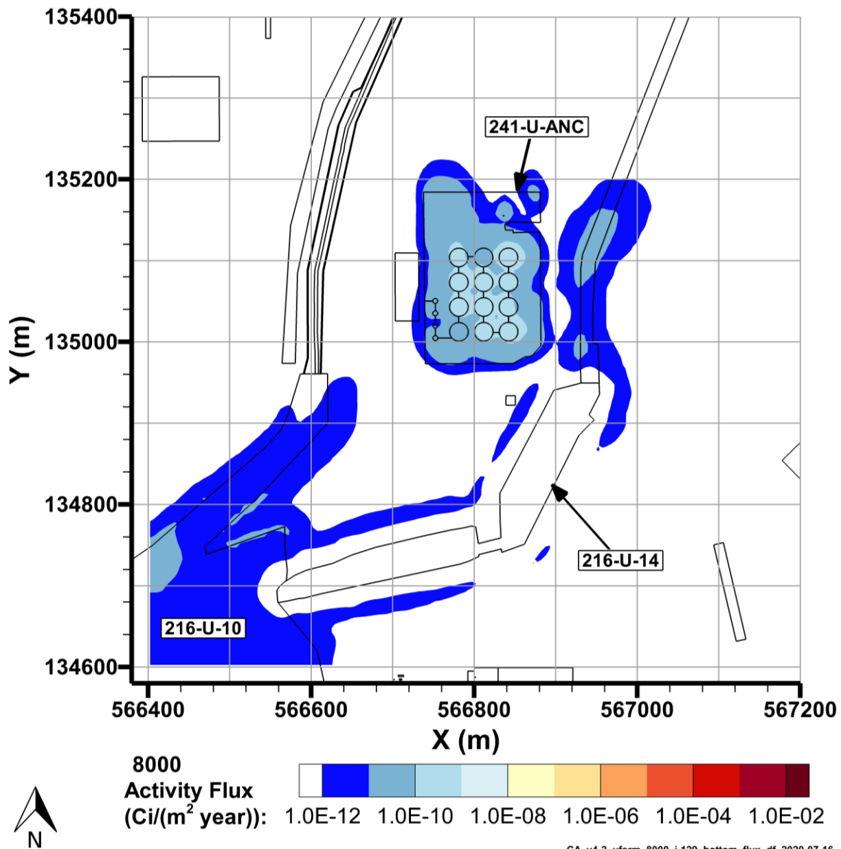
Figure 7-18. I-129 Flux to Groundwater, 8000
