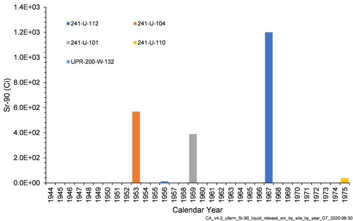
Figure 4-25. Annual Sr-90 Activity Released from Liquid Waste Sites in the U Farm Area Model
