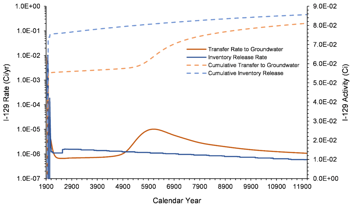
Figure 7-12. I-129 Inventory Release from Waste Sites and Transfer to Groundwater for the U Farm Area Model from 1943–12070
