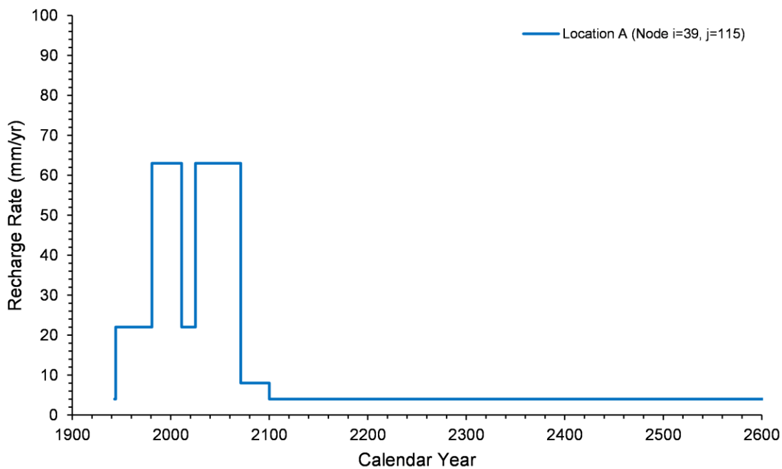
Figure 4-85. Time Series of Natural Recharge Rates, Location A
