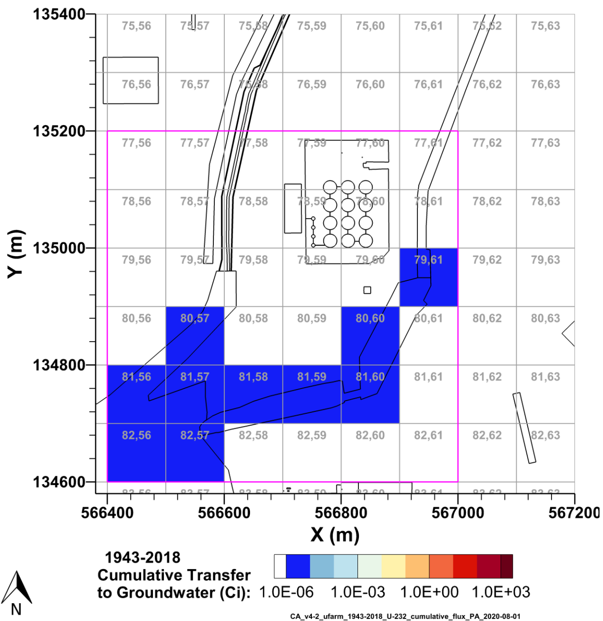
Figure 7-35. Cumulative U-232 Activity Discharged to Groundwater from the U Farm Area Model from 1943-2018 per P2R Grid Cell
