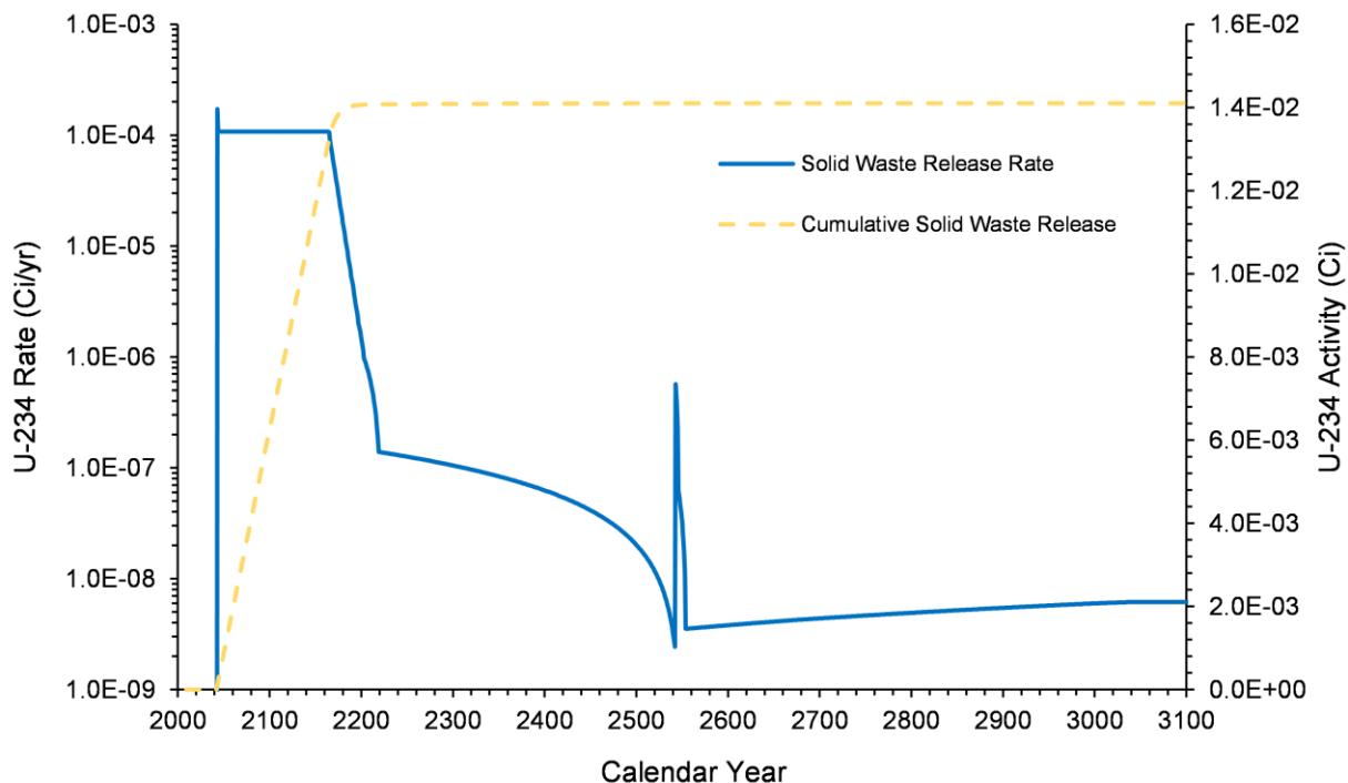
Figure 4-68. U-234 Release Rate and Cumulative Activity from Solid Waste in the U Farm Area Model, 2018–3070
