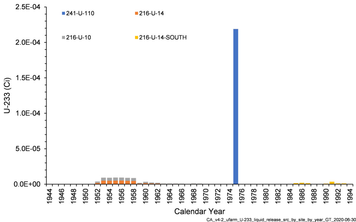
Figure 4-28. Annual U-233 Activity Released from Liquid Waste Sites in the U Farm Area Model
