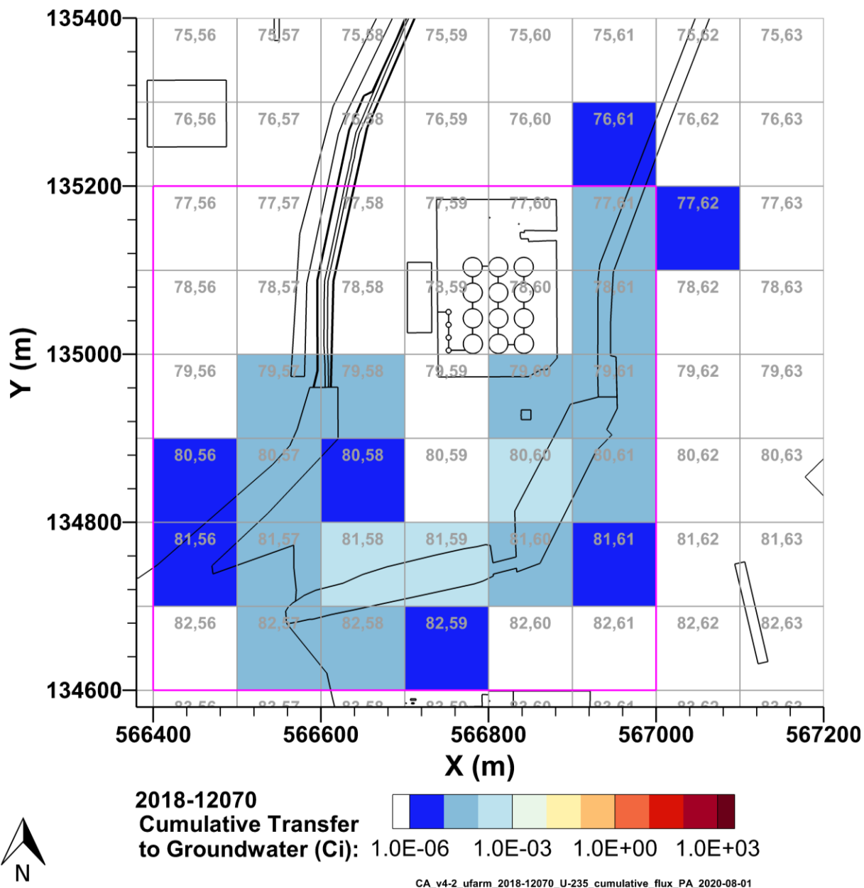
Figure 7-46. Cumulative U-235 Activity Discharged to Groundwater from the U Farm Area Model from 2018–12070 per P2R Grid Cell
