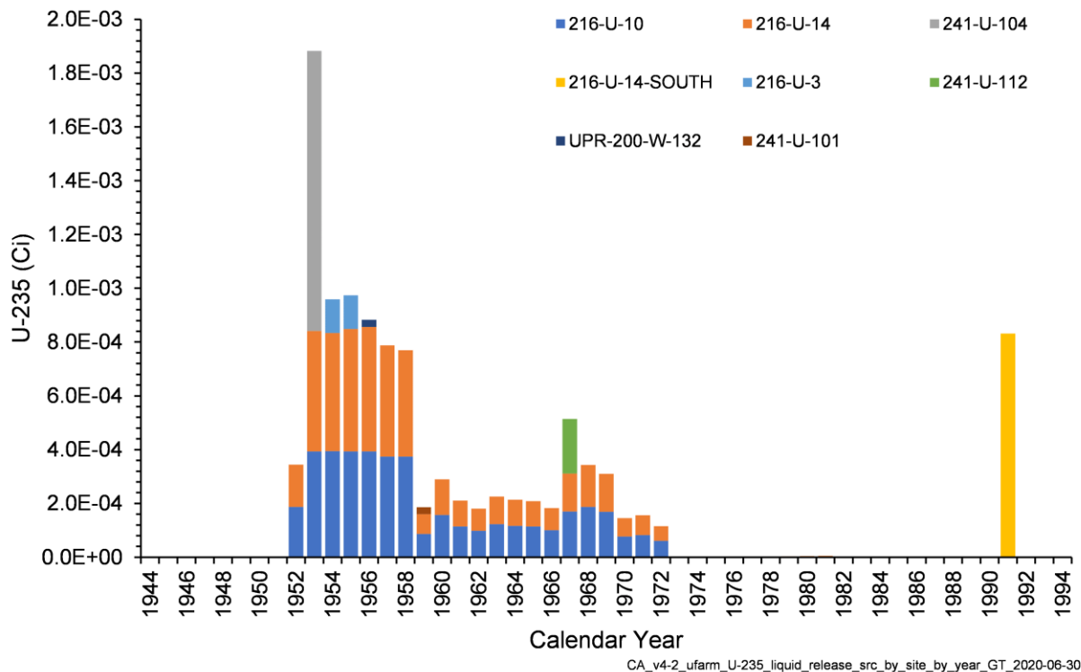
Figure 4-30. Annual U-235 Activity Released from Liquid Waste Sites in the U Farm Area Model
