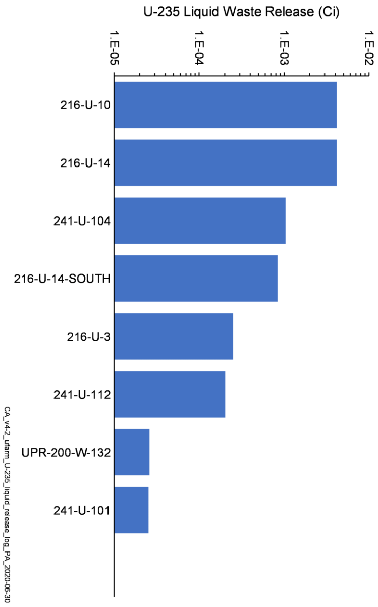
Figure 4-18. Total U-235 Activity Released from Liquid Waste Sites in the U Farm Area Model
