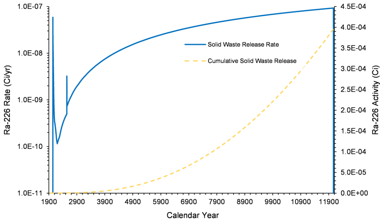
Figure 4-59. Ra-226 Release Rate and Cumulative Activity from Solid Waste in the U Farm Area Model, 1943–12070
