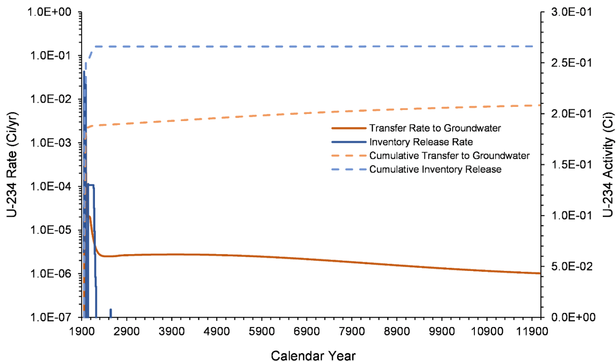
Figure 7-44. U-234 Inventory Release from Waste Sites and Transfer to Groundwater for the U Farm Area Model from 1943–12070
