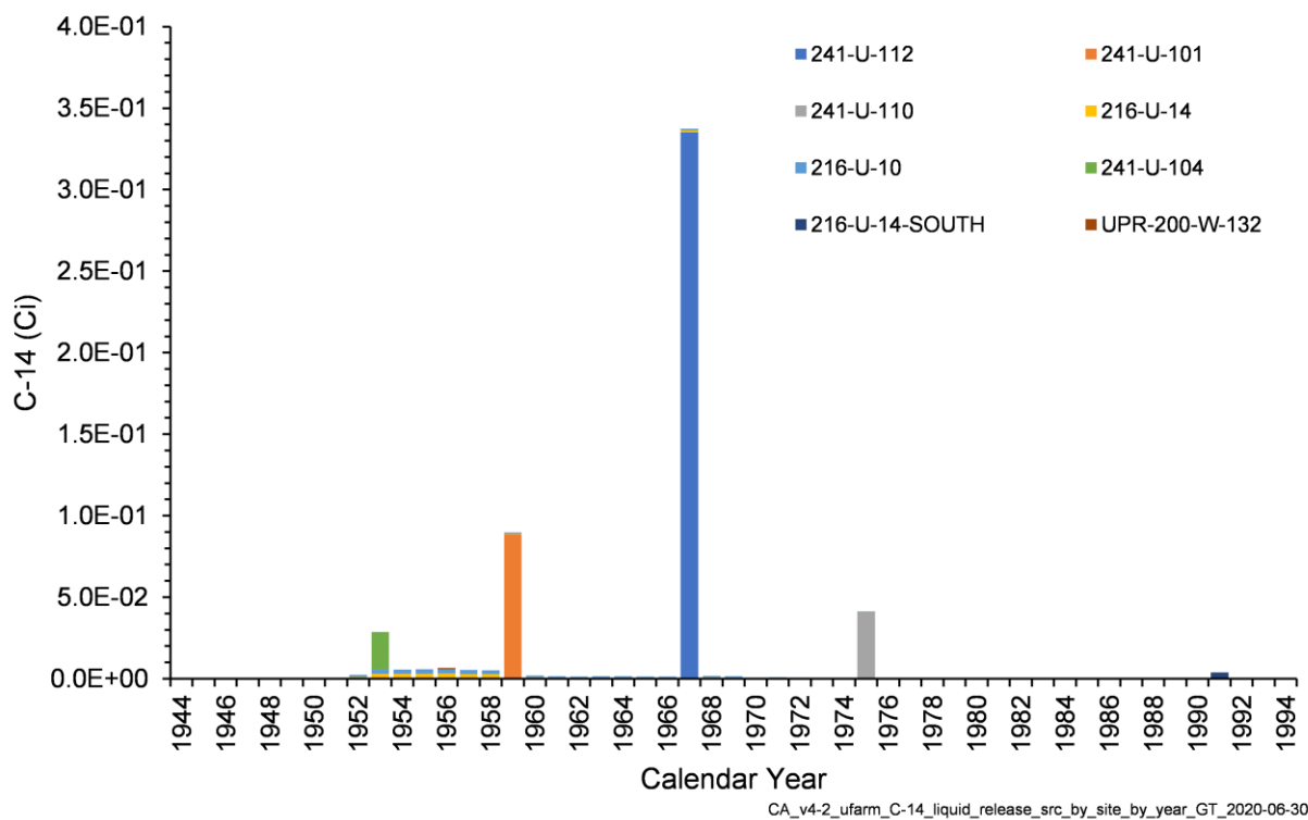
Figure 4-21. Annual C-14 Activity Released from Liquid Waste Sites in the U Farm Area Model
