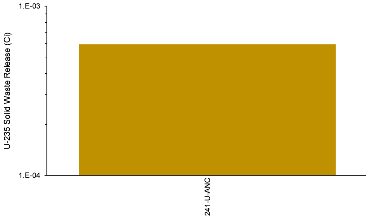
Figure 4-44. Total U-235 Activity Released from Solid Waste Sites in the U Farm Area Model
