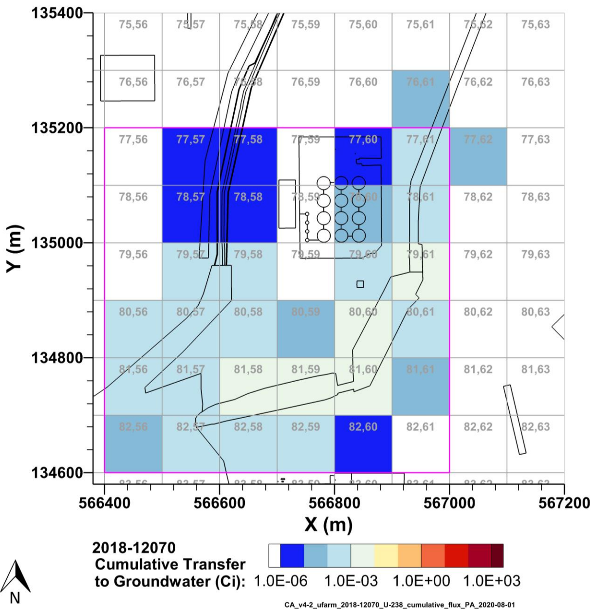
Figure 7-54. Cumulative U-238 Activity Discharged to Groundwater from the U Farm Area Model from 2018–12070 per P2R Grid Cell
