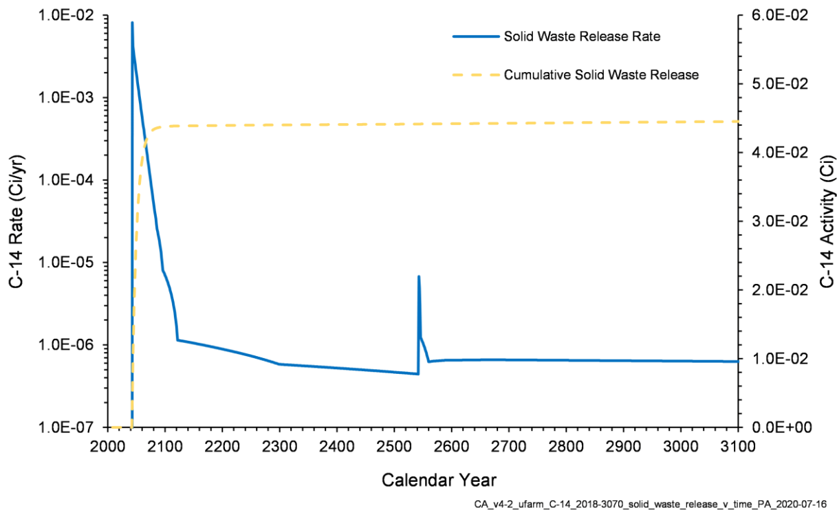
Figure 4-48. C-14 Release Rate and Cumulative Activity from Solid Waste in the U Farm Area Model, 2018–3070
