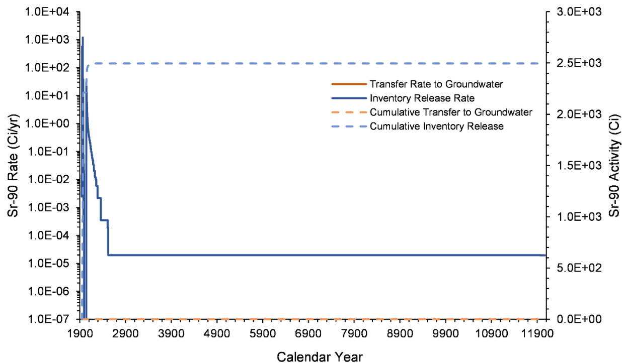
Figure 7-23. Sr-90 Inventory Release from Waste Sites and Transfer to Groundwater for the U Farm Area Model from 1943–12070
