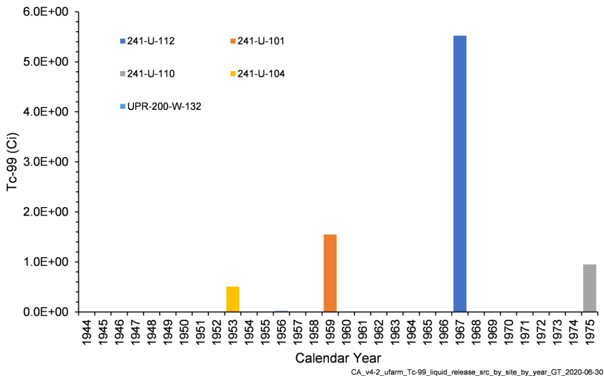
Figure 4-26. Annual Tc-99 Activity Released from Liquid Waste Sites in the U Farm Area Model
