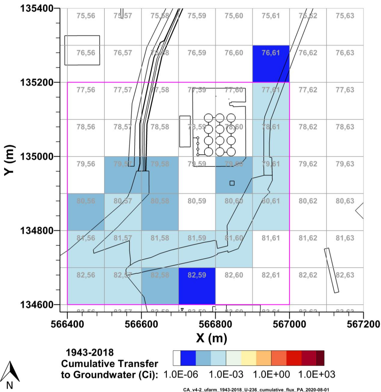
Figure 7-49. Cumulative U-236 Activity Discharged to Groundwater from the U Farm Area Model from 1943–2018 per P2R Grid Cell
