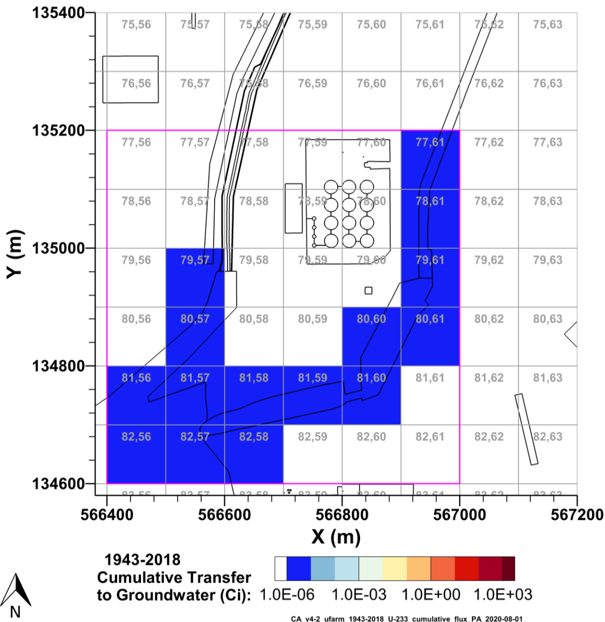
Figure 7-38. Cumulative U-233 Activity Discharged to Groundwater from the U Farm Area Model from 1943–2018 per P2R Grid Cell
