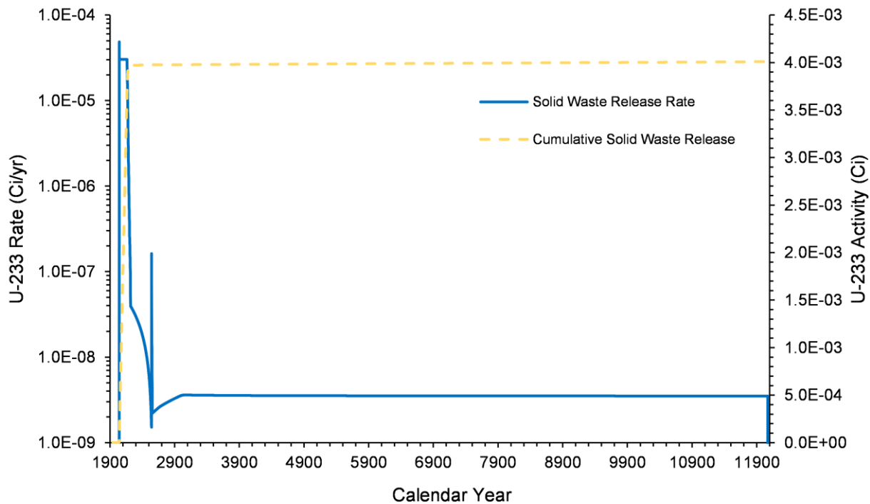
Figure 4-65. U-233 Release Rate and Cumulative Activity from Solid Waste in the U Farm Area Model, 1943–12070
