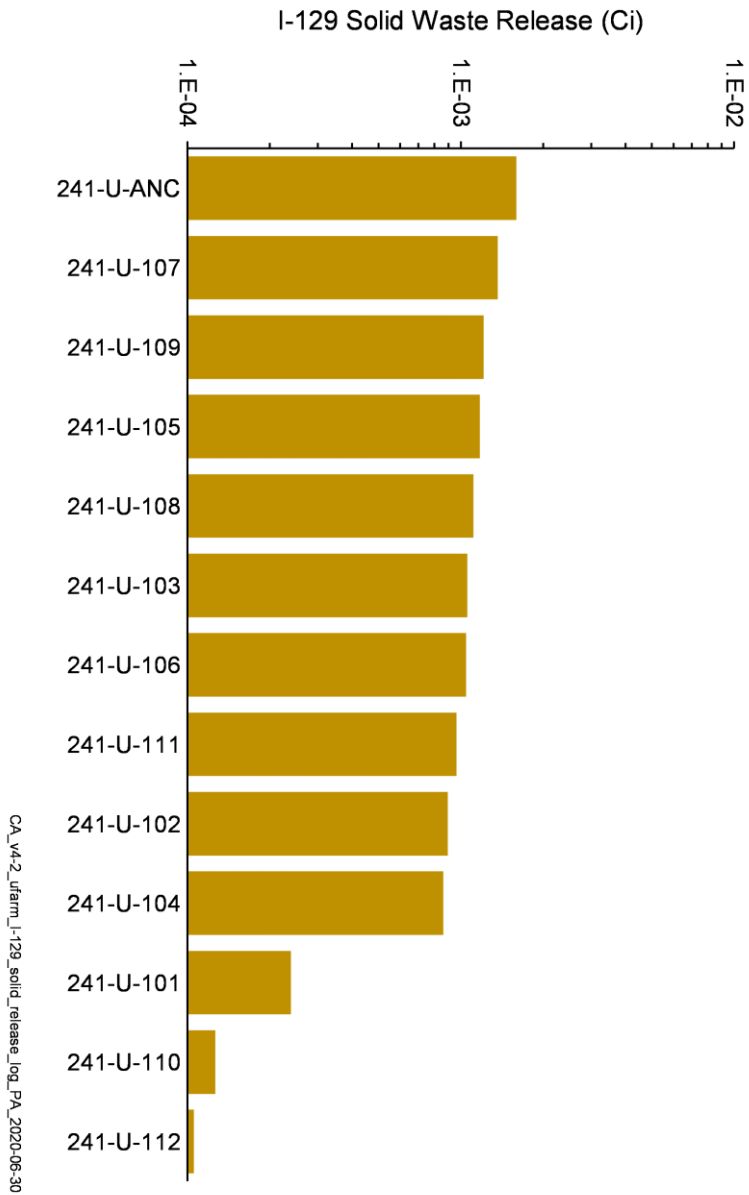
Figure 4-35. Total I-129 Activity Released from Solid Waste Sites in the U Farm Area Model
