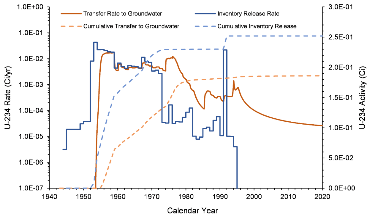
Figure 7-43. U-234 Inventory Release from Waste Sites and Transfer to Groundwater for the U Farm Area Model from 1943–2018
