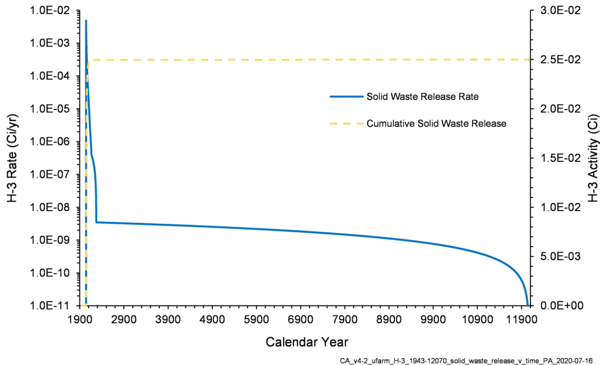
Figure 4-49. H-3 Release Rate and Cumulative Activity from Solid Waste in the U Farm Area Model, 1943–12070
