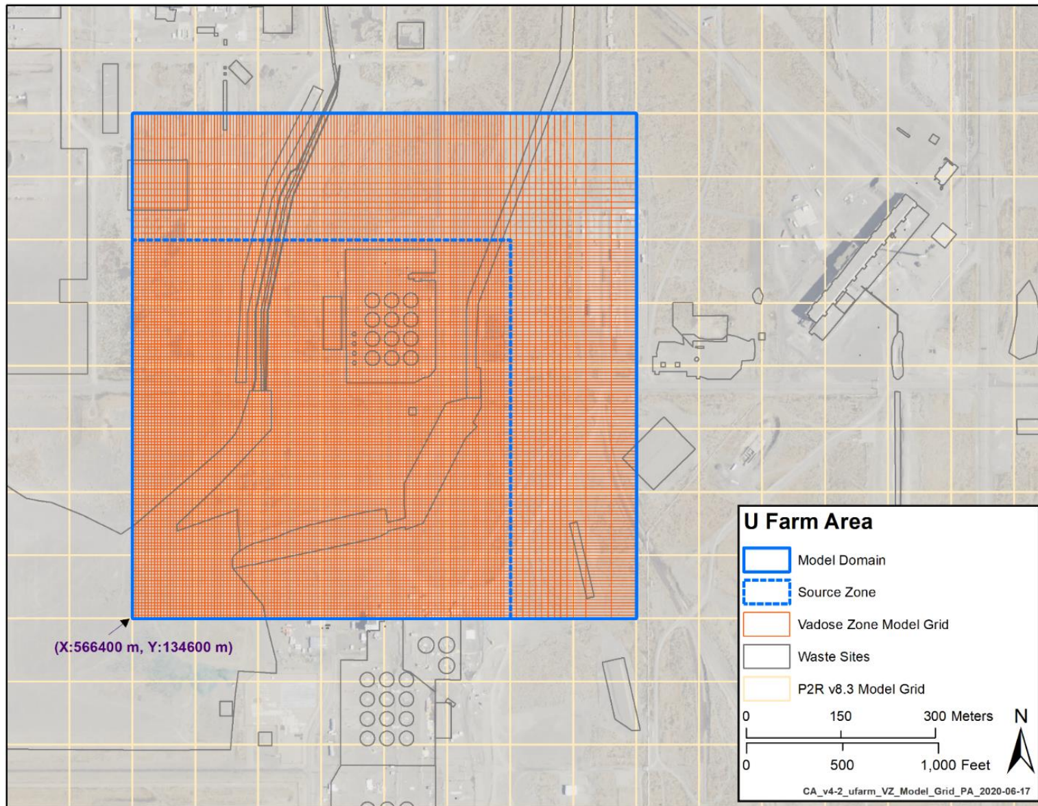
Figure 4-1. Plan View of the U Farm Area Model Grid Overlain on the P2R Grid Cells
