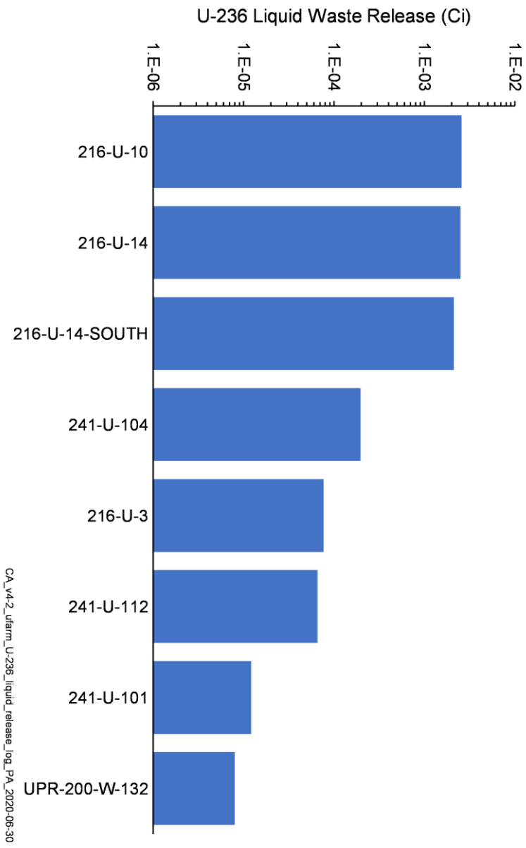
Figure 4-19. Total U-236 Activity Released from Liquid Waste Sites in the U Farm Area Model
