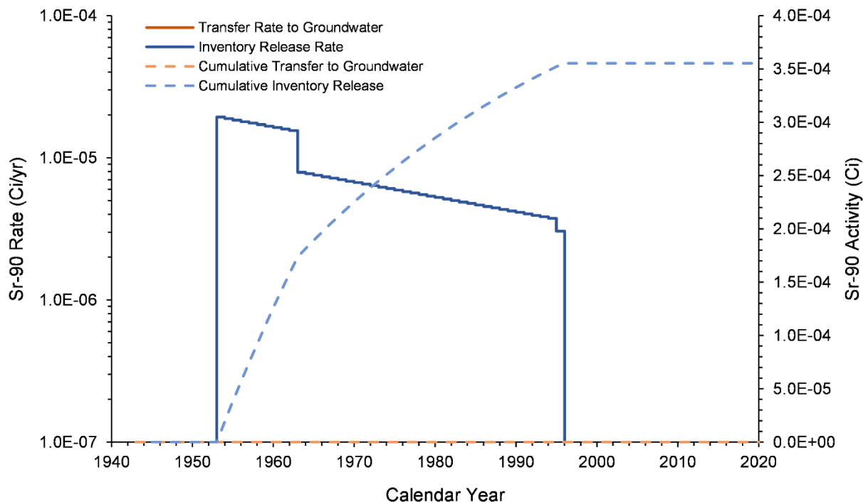
Figure 7-14. Sr-90 Inventory Release from Waste Sites and Transfer to Groundwater for the M Pond Area Model from 1943–2018
