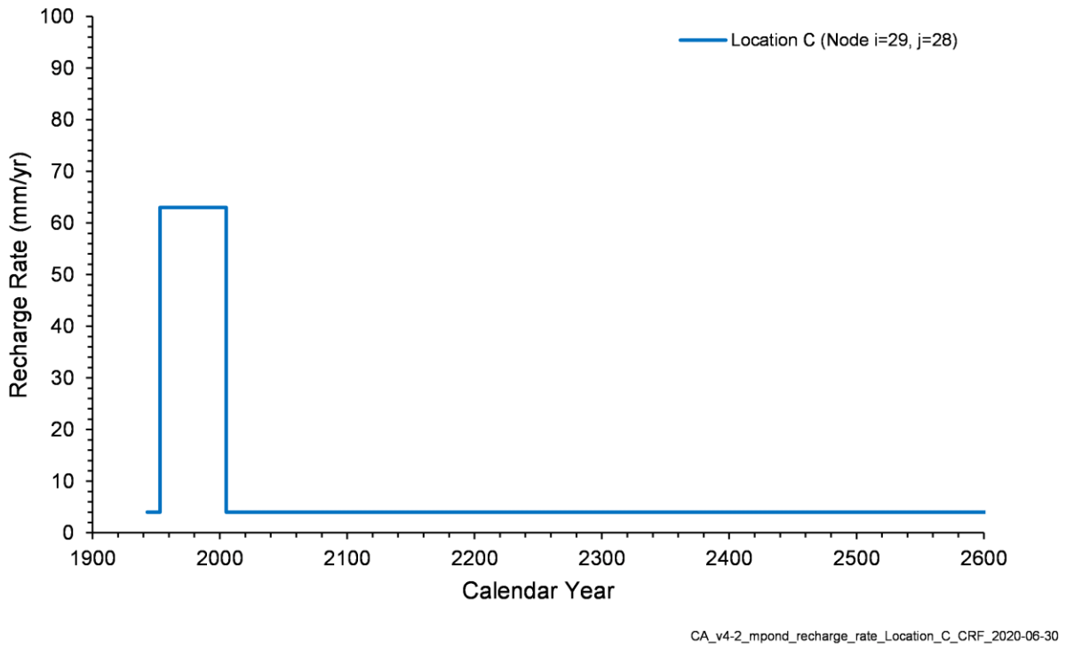
Figure 4-38. Time Series of Natural Recharge Rates, Location C
