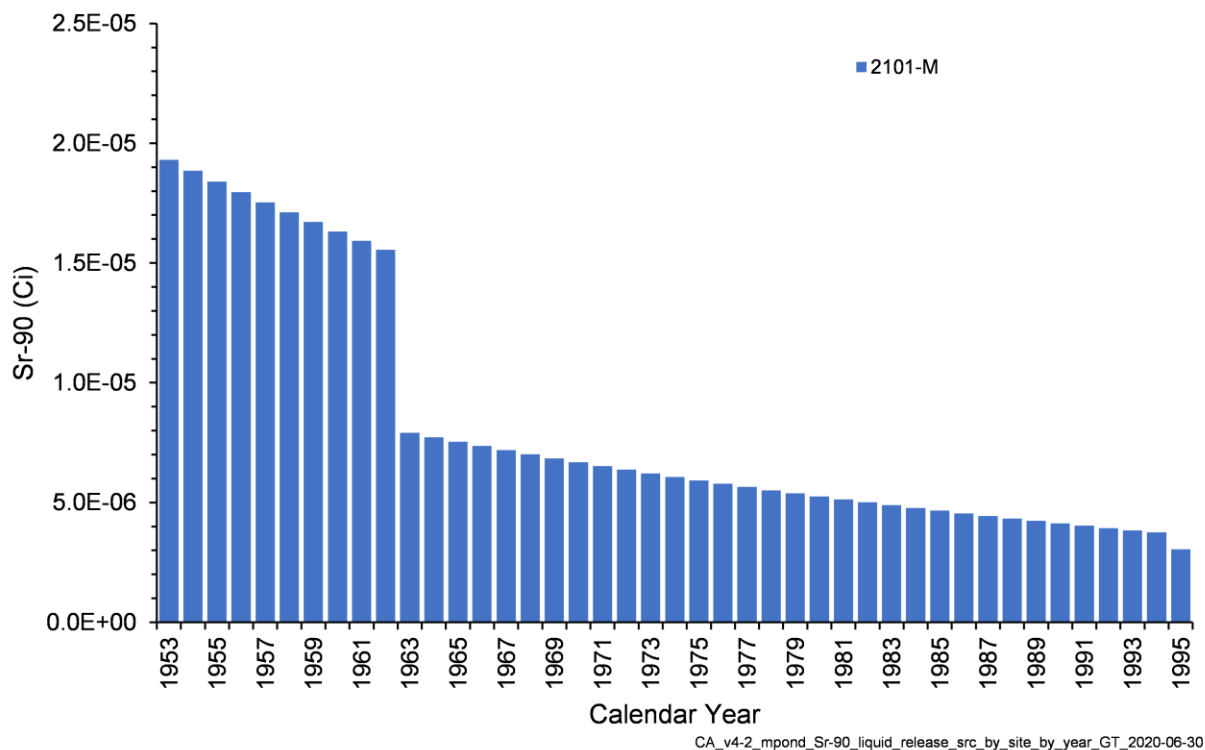
Figure 4-23. Annual Sr-90 Activity Released from Liquid Waste Sites in the M Pond Area Model
