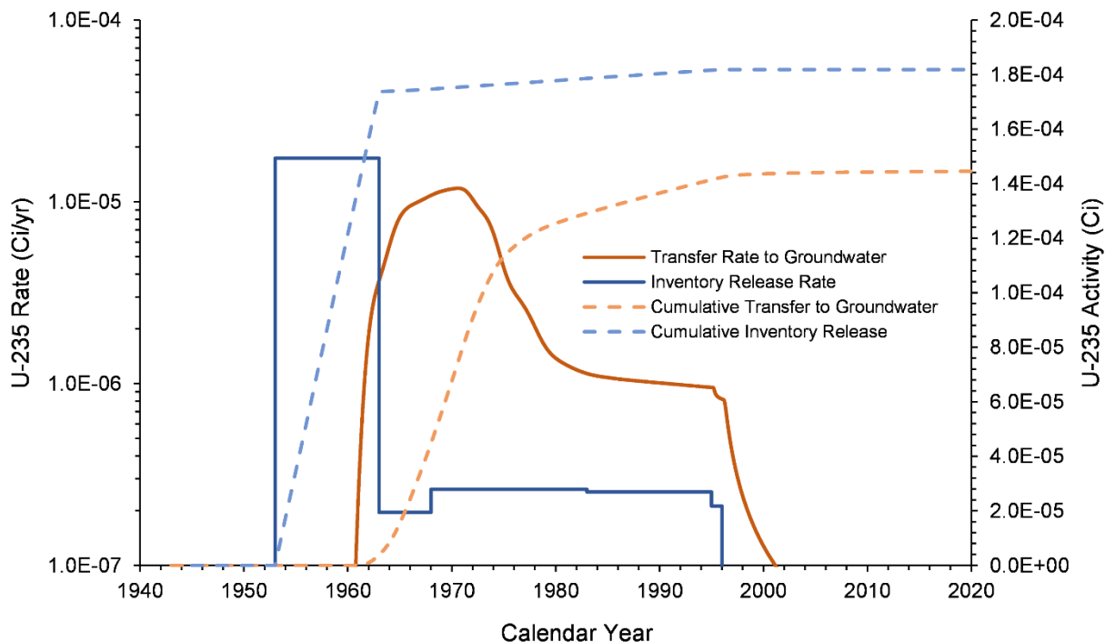
Figure 7-27. U-235 Inventory Release from Waste Sites and Transfer to Groundwater for the M Pond Area Model from 1943–2018
