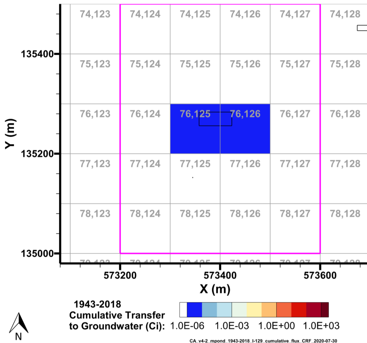
Figure 7-9. Cumulative I-129 Activity Discharged to Groundwater from the M Pond Area Model from 1943–2018 per P2R Grid Cell
