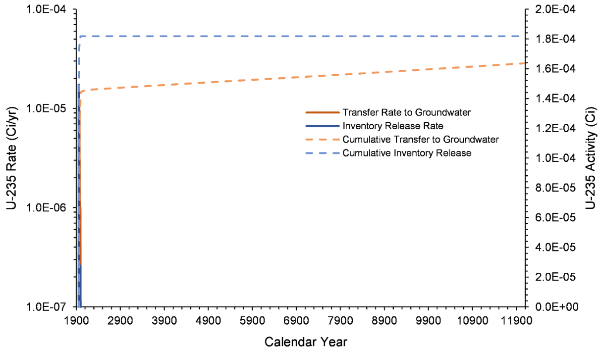
Figure 7-28. U-235 Inventory Release from Waste Sites and Transfer to Groundwater for the M Pond Area Model from 1943–12070
