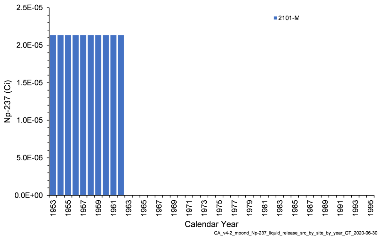
Figure 4-22. Annual Np-237 Activity Released from Liquid Waste Sites in the M Pond Area Model
