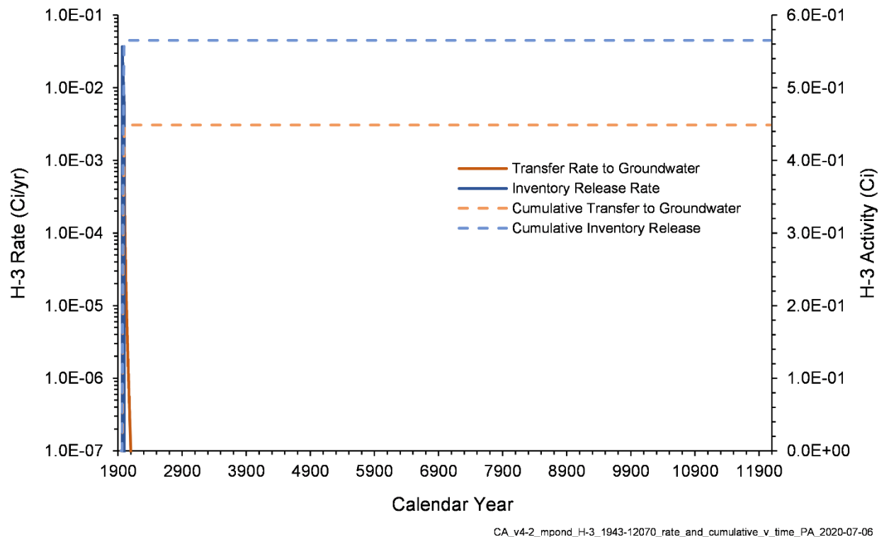
Figure 7-8. H-3 Inventory Release from Waste Sites and Transfer to Groundwater for the M Pond Area Model from 1943–12070
