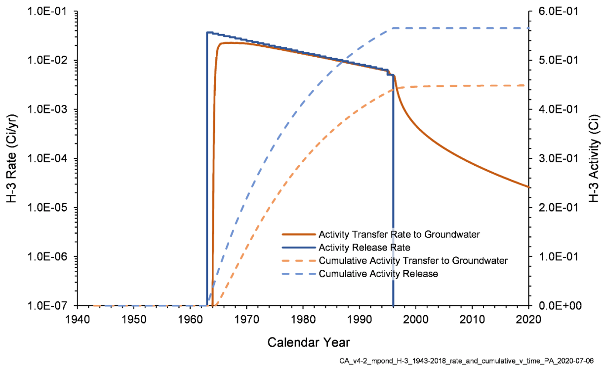
Figure 7-7. H-3 Inventory Release from Waste Sites and Transfer to Groundwater for the M Pond Area Model from 1943–2018
