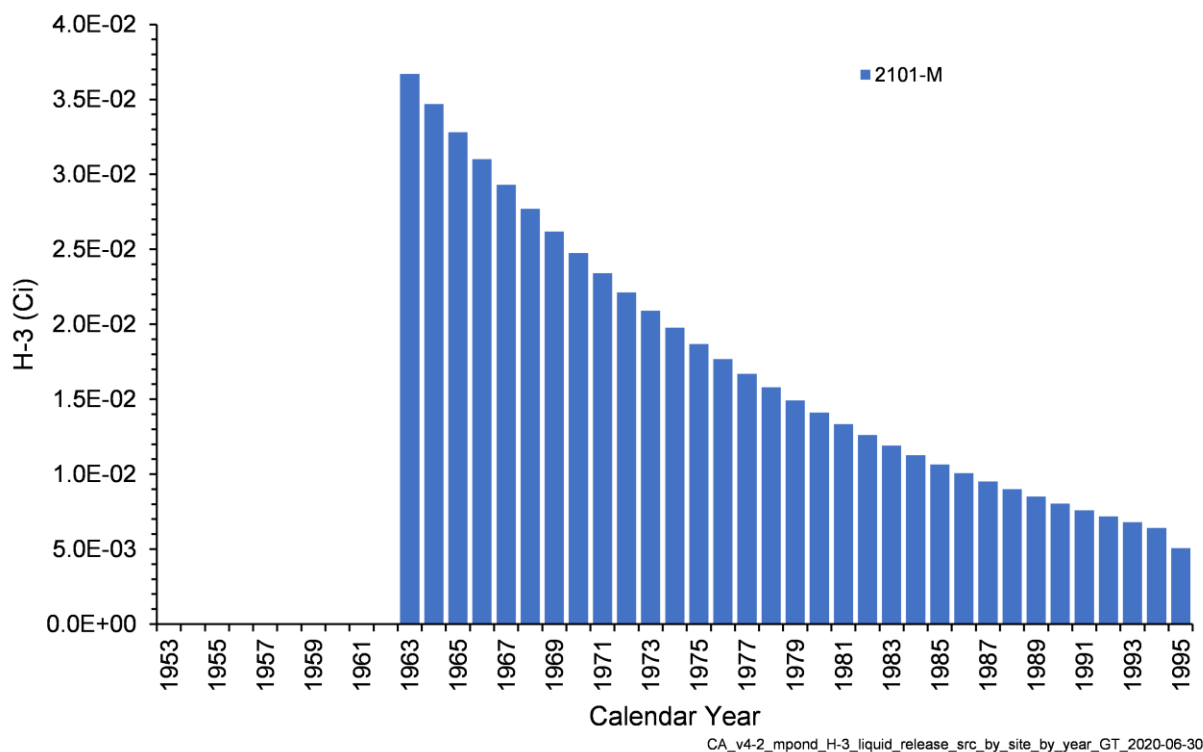
Figure 4-20. Annual H-3 Activity Released from Liquid Waste Sites in the M Pond Area Model
