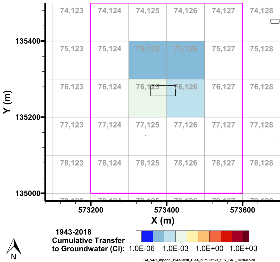
Figure 7-1. Cumulative C-14 Activity Discharged to Groundwater from the M Pond Area Model from 1943–2018 per P2R Grid Cell
