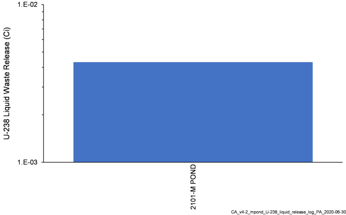
Figure 4-18. Total U-238 Activity Released from Liquid Waste Sites in the M Pond Area Model
