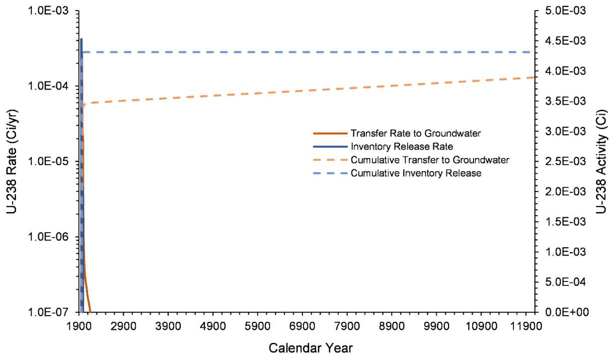
Figure 7-36. U-238 Inventory Release from Waste Sites and Transfer to Groundwater for the M Pond Area Model from 1943–12070
