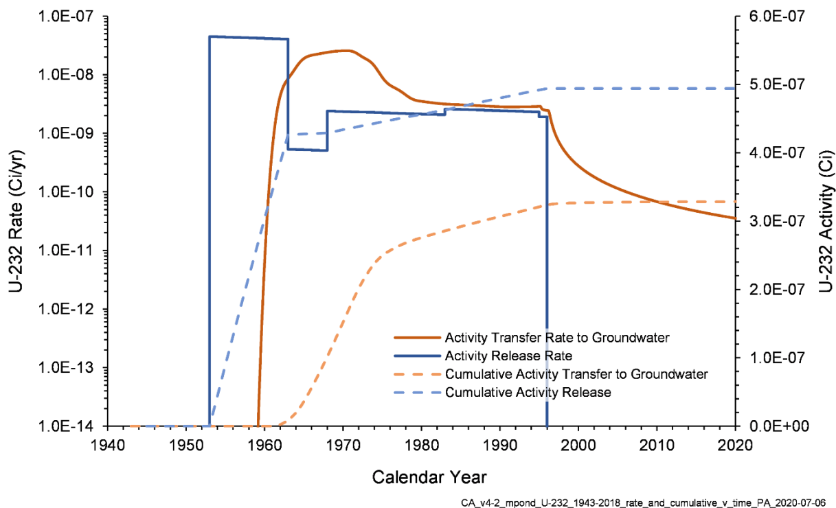
Figure 7-16. U-232 Inventory Release from Waste Sites and Transfer to Groundwater for the M Pond Area Model from 1943–2018
