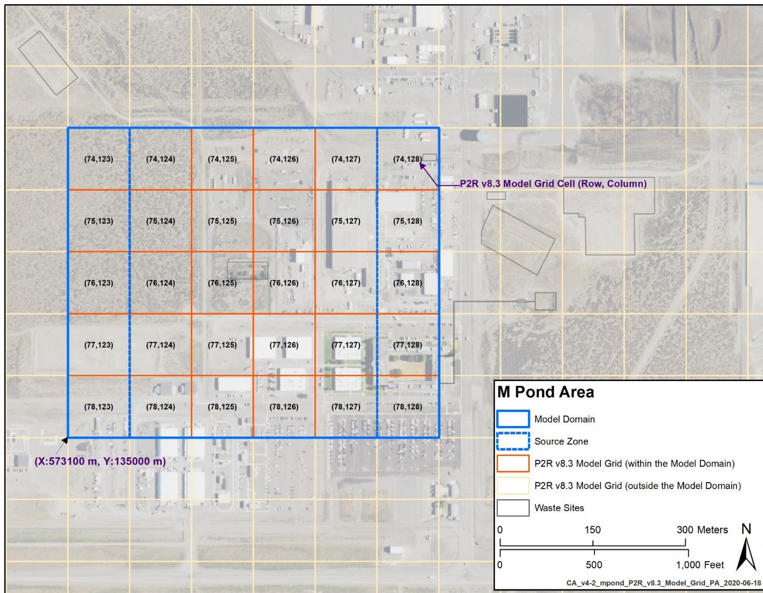
Figure 4-2. Plan View of the P2R Grid Cells in the M Pond Area Model
