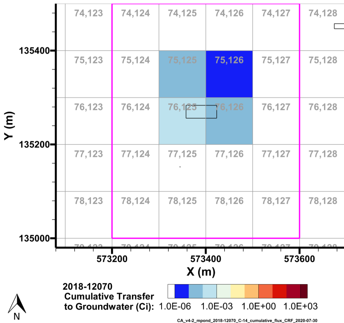
Figure 7-2. Cumulative C-14 Activity Discharged to Groundwater from the M Pond Area Model from 2018–12070 per P2R Grid Cell
