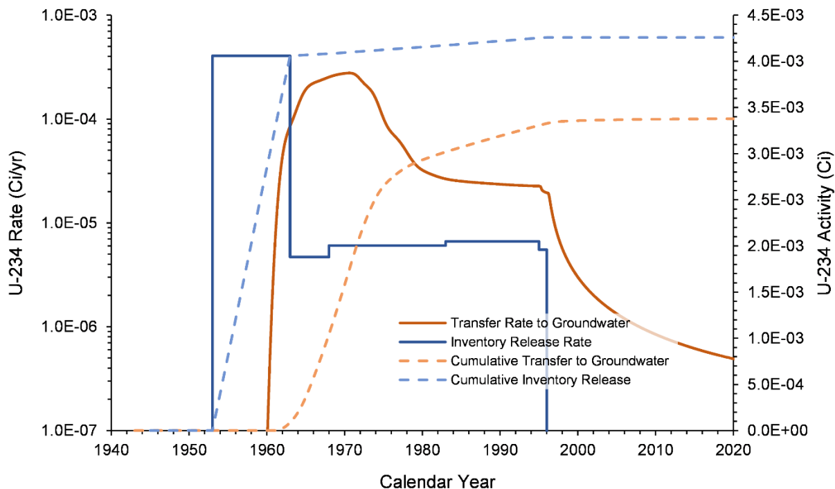
Figure 7-23. U-234 Inventory Release from Waste Sites and Transfer to Groundwater for the M Pond Area Model from 1943–2018
