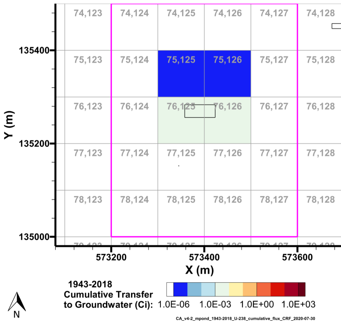
Figure 7-33. Cumulative U-238 Activity Discharged to Groundwater from the M Pond Area Model from 1943–2018 per P2R Grid Cell
