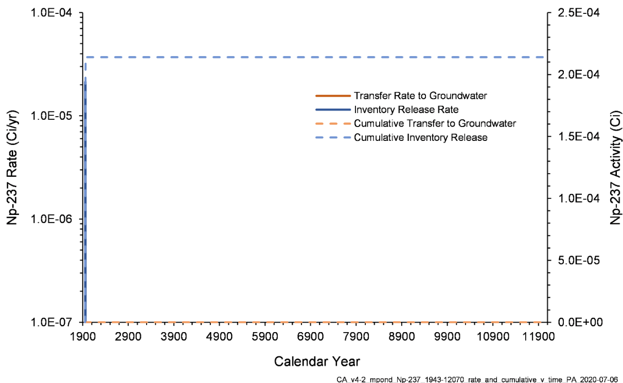
Figure 7-13. Np-237 Inventory Release from Waste Sites and Transfer to Groundwater for the M Pond Area Model from 1943–12070
