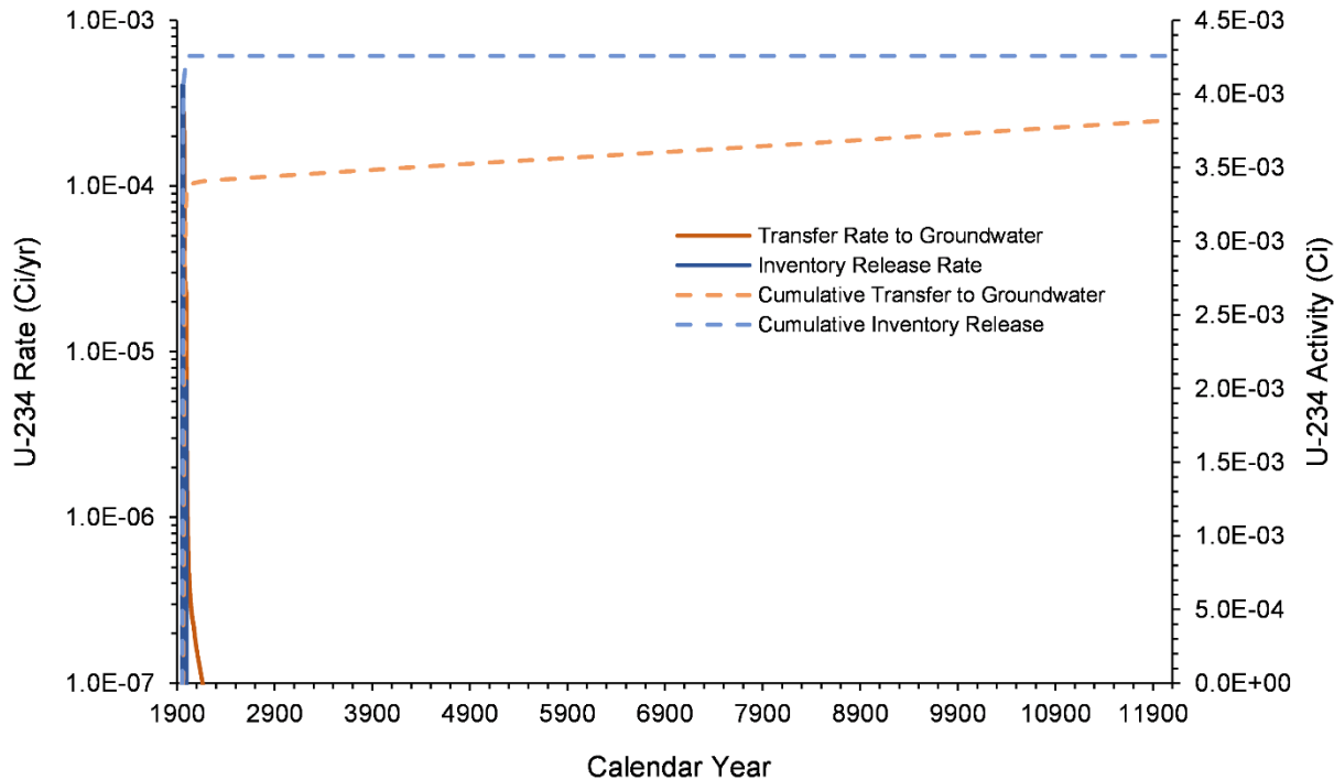
Figure 7-24. U-234 Inventory Release from Waste Sites and Transfer to Groundwater for the M Pond Area Model from 1943–12070
