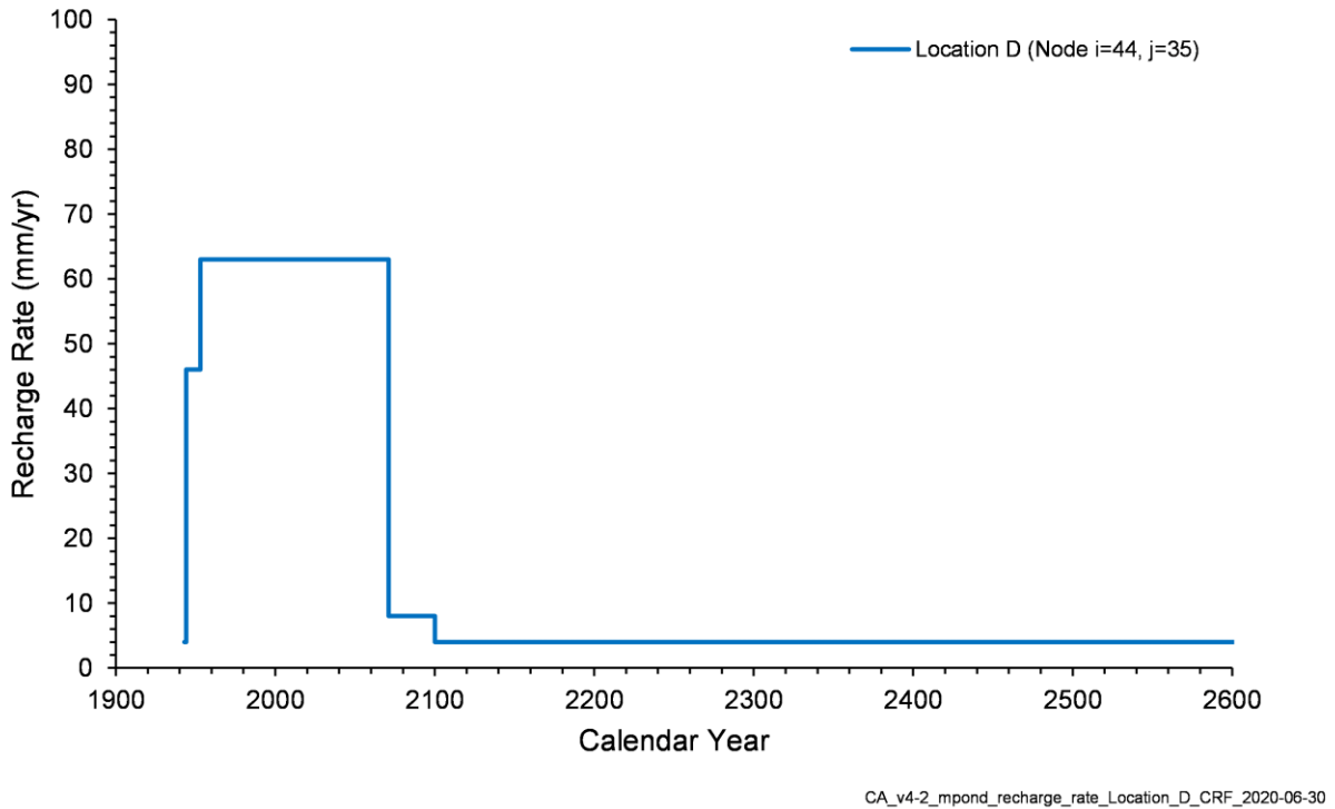
Figure 4-39. Time Series of Natural Recharge Rates, Location D
