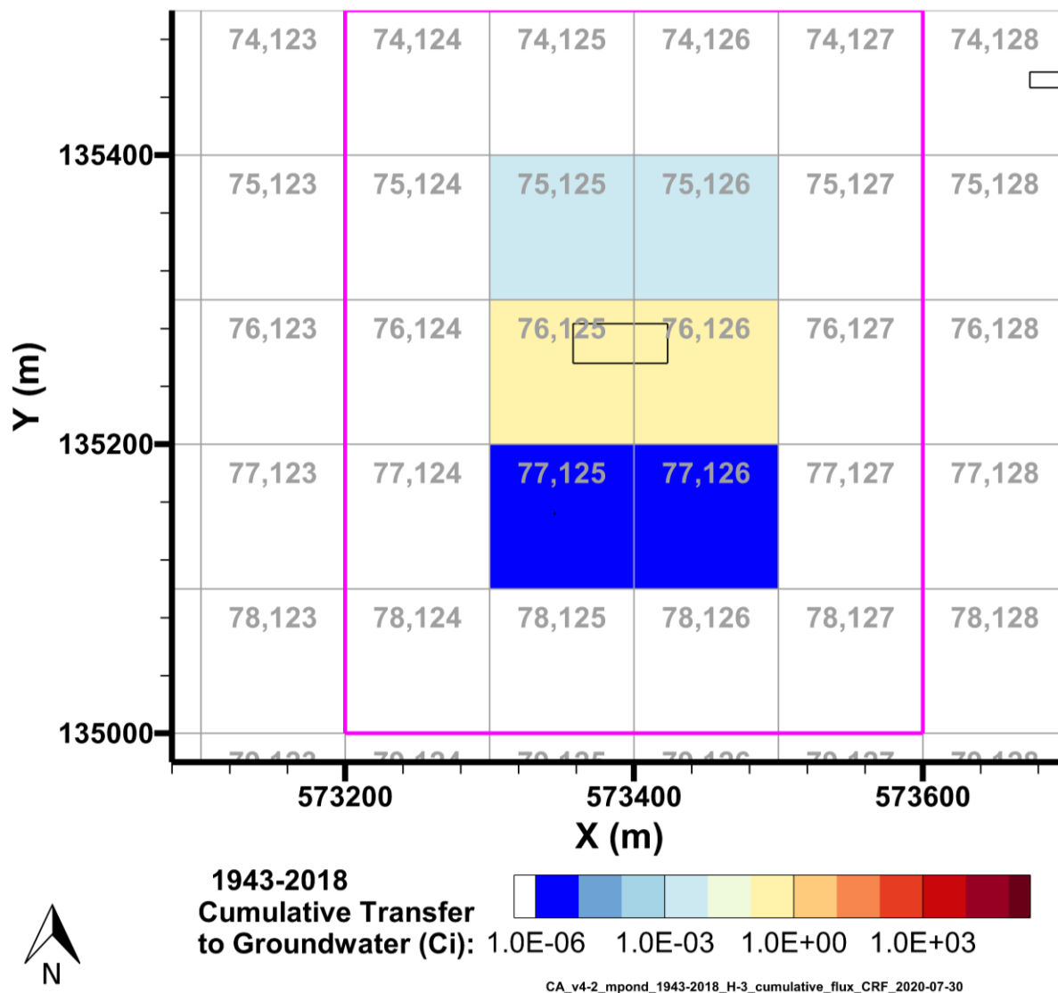
Figure 7-5. Cumulative H-3 Activity Discharged to Groundwater from the M Pond Area Model from 1943–2018 per P2R Grid Cell
