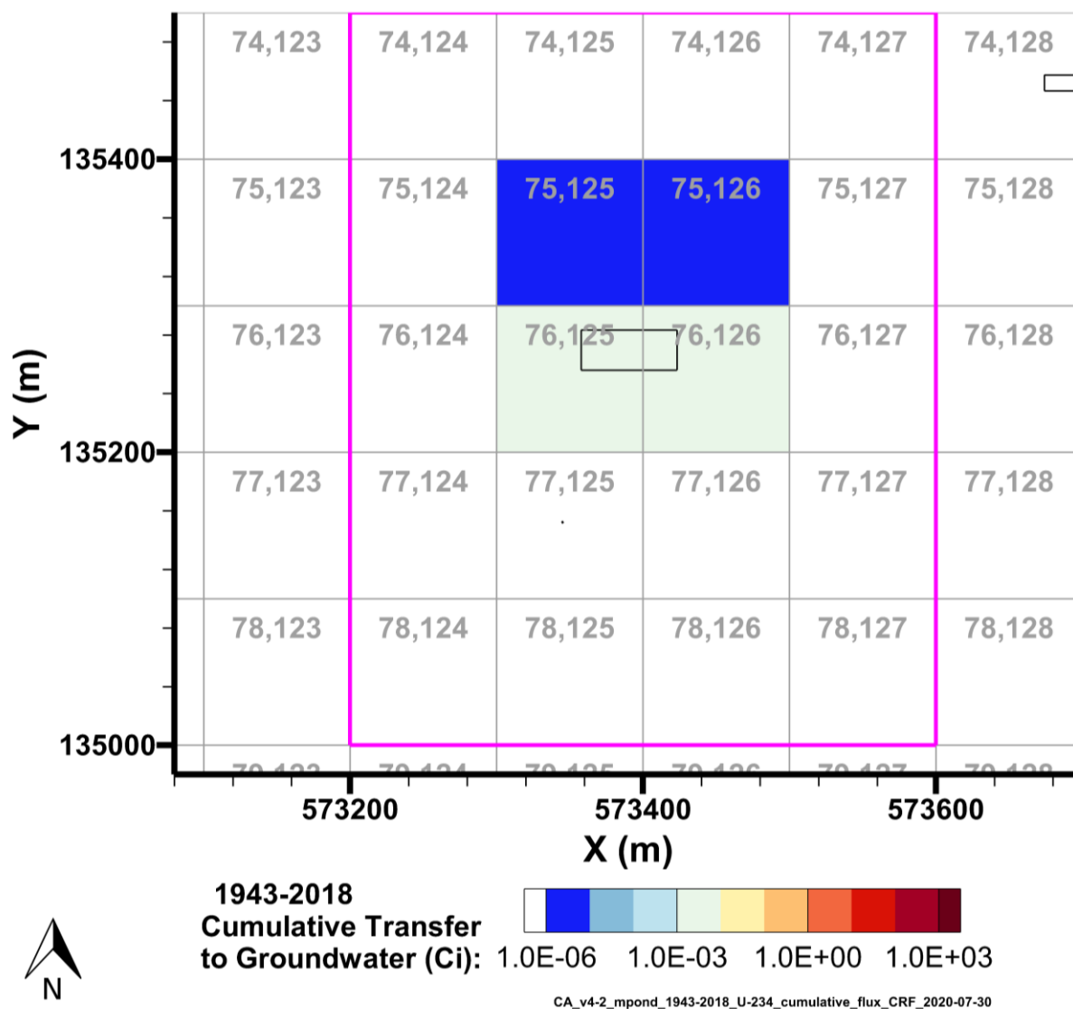
Figure 7-21. Cumulative U-234 Activity Discharged to Groundwater from the M Pond Area Model from 1943–2018 per P2R Grid Cell
