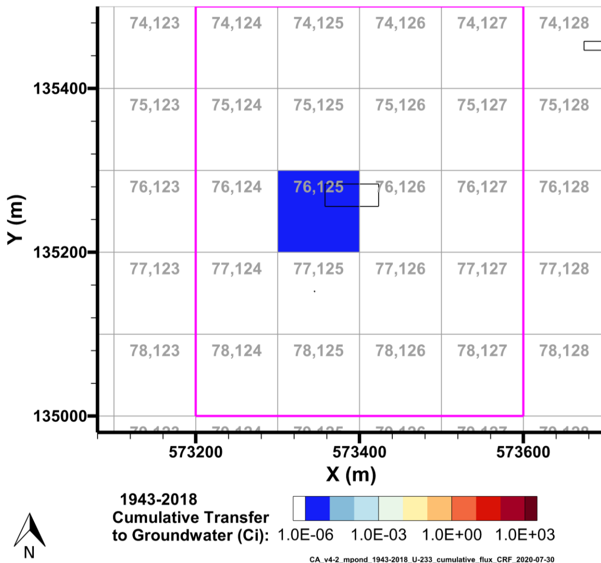
Figure 7-18. Cumulative U-233 Activity Discharged to Groundwater from the M Pond Area Model from 1943–2018 per P2R Grid Cell
