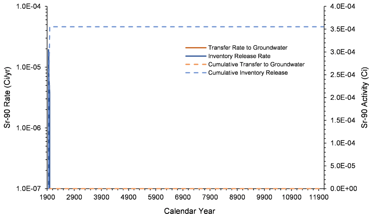
Figure 7-15. Sr-90 Inventory Release from Waste Sites and Transfer to Groundwater for the M Pond Area Model from 1943–12070
