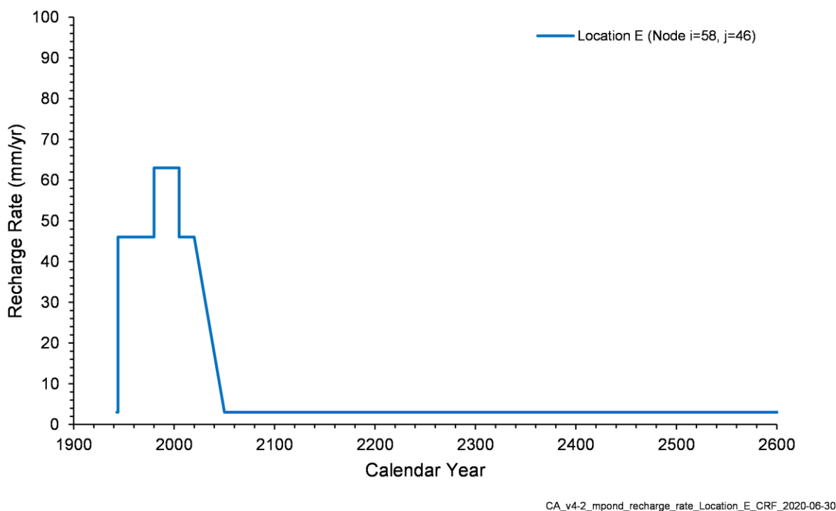
Figure 4-40. Time Series of Natural Recharge Rates, Location E
