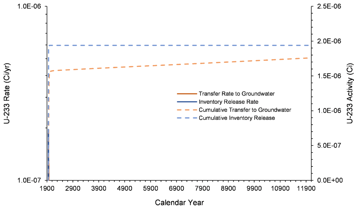
Figure 7-20. U-233 Inventory Release from Waste Sites and Transfer to Groundwater for the M Pond Area Model from 1943–12070
