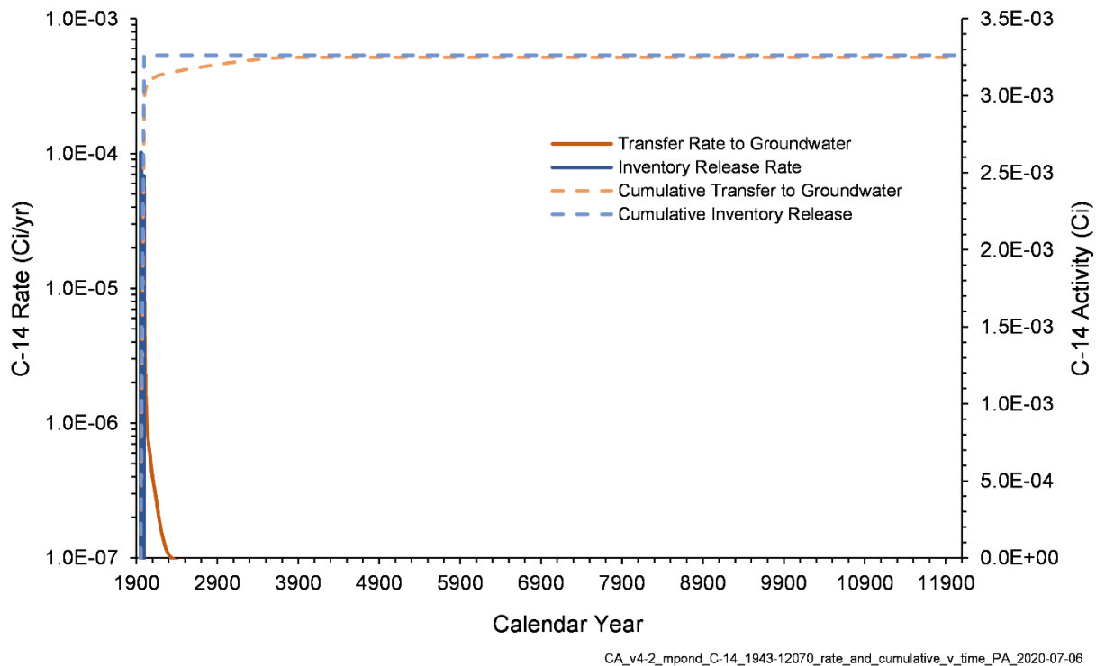
Figure 7-4. C-14 Inventory Release from Waste Sites and Transfer to Groundwater for the M Pond Area Model from 1943–12070
