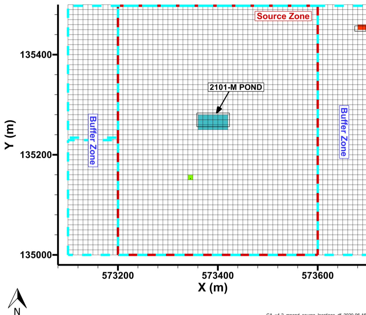
Figure 4-41. Distribution of Source Nodes in the M Pond Area Model
