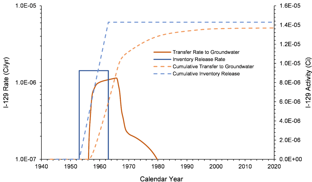
Figure 7-10. I-129 Inventory Release from Waste Sites and Transfer to Groundwater for the M Pond Area Model from 1943–2018
