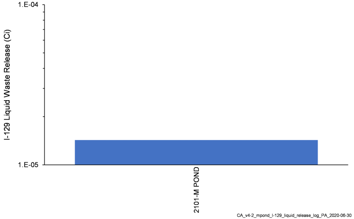
Figure 4-10. Total I-129 Activity Released from Liquid Waste Sites in the M Pond Area Model
