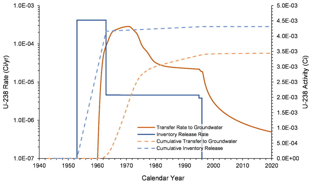
Figure 7-35. U-238 Inventory Release from Waste Sites and Transfer to Groundwater for the M Pond Area Model from 1943–2018
