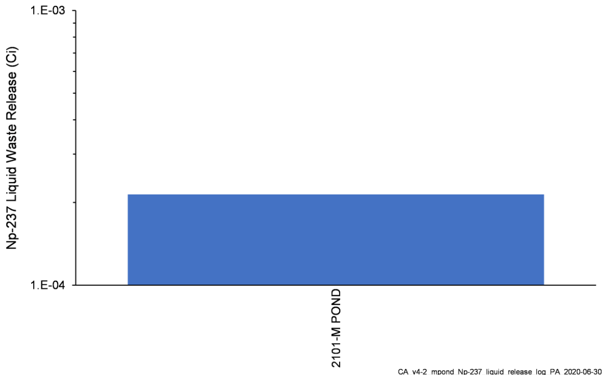
Figure 4-11. Total Np-237 Activity Released from Liquid Waste Sites in the M Pond Area Model
