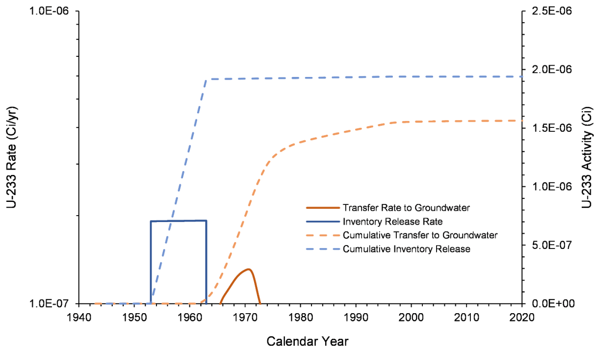
Figure 7-19. U-233 Inventory Release from Waste Sites and Transfer to Groundwater for the M Pond Area Model from 1943–2018
