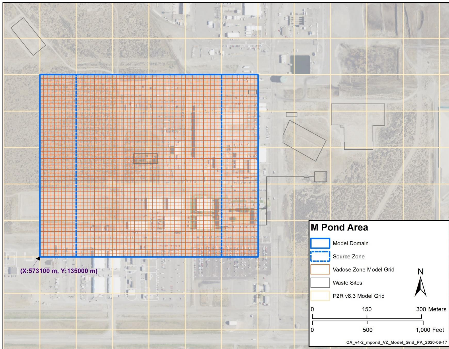
Figure 4-1. Plan View of the M Pond Area Model Grid Overlain on the P2R Grid Cells
