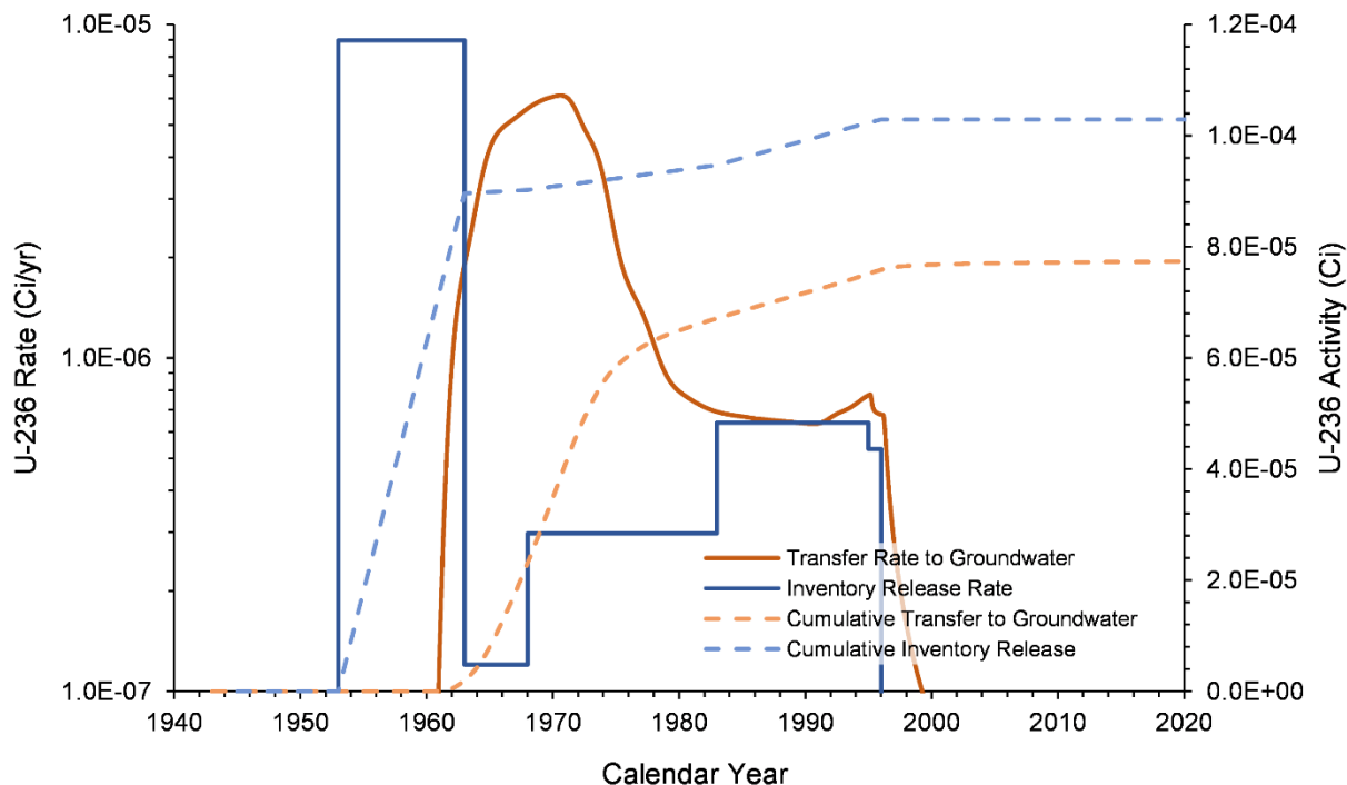
Figure 7-31. U-236 Inventory Release from Waste Sites and Transfer to Groundwater for the M Pond Area Model from 1943–2018
