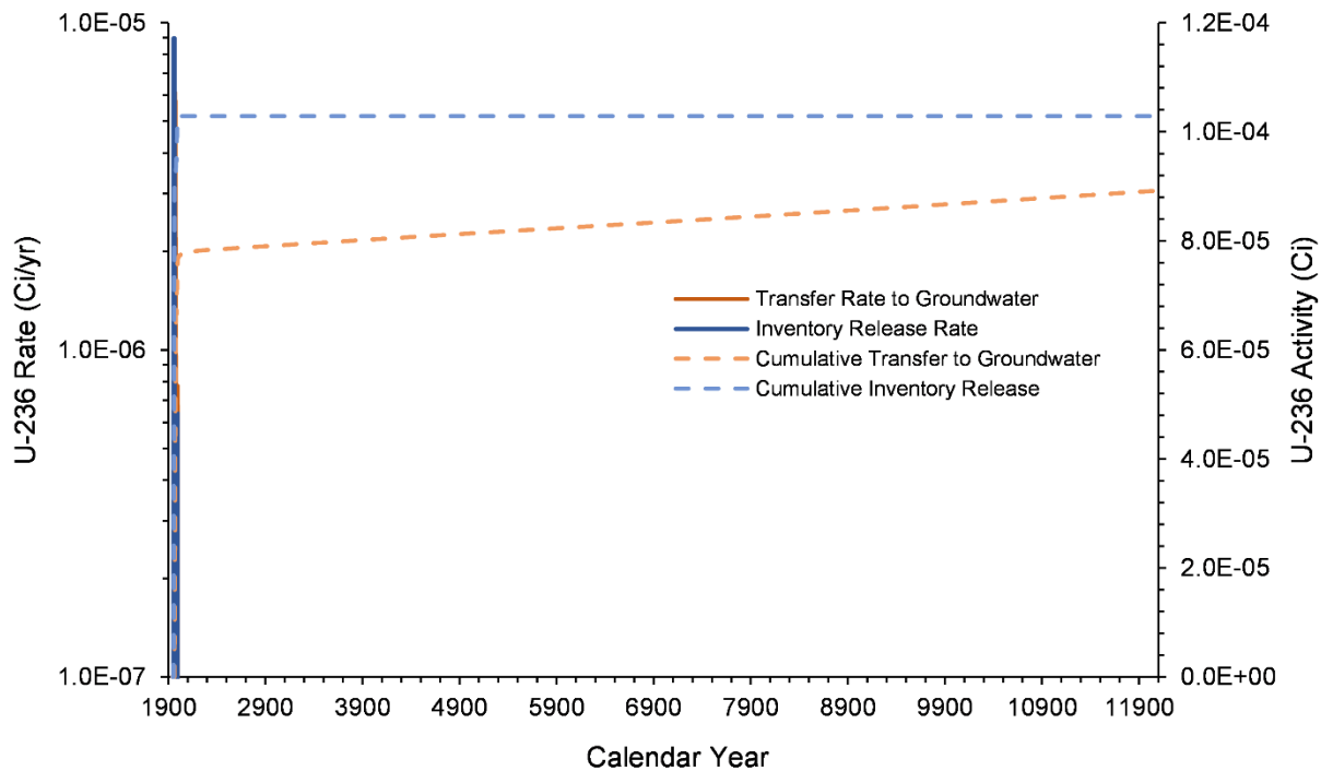
Figure 7-32. U-236 Inventory Release from Waste Sites and Transfer to Groundwater for the M Pond Area Model from 1943–12070
