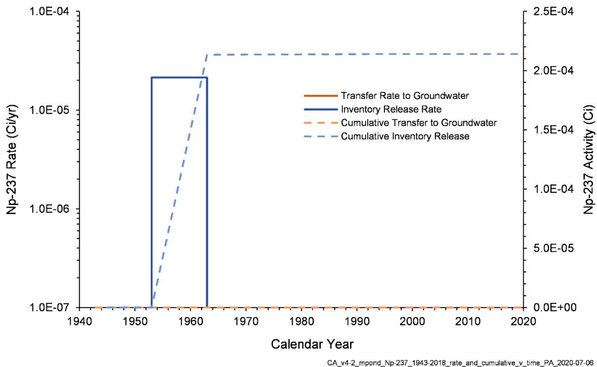
Figure 7-12. Np-237 Inventory Release from Waste Sites and Transfer to Groundwater for the M Pond Area Model from 1943–2018
