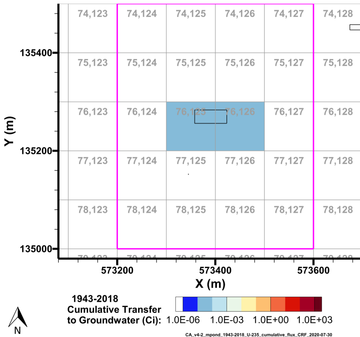
Figure 7-25. Cumulative U-235 Activity Discharged to Groundwater from the M Pond Area Model from 1943–2018 per P2R Grid Cell
