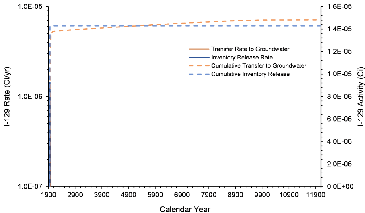
Figure 7-11. I-129 Inventory Release from Waste Sites and Transfer to Groundwater for the M Pond Area Model from 1943–12070
