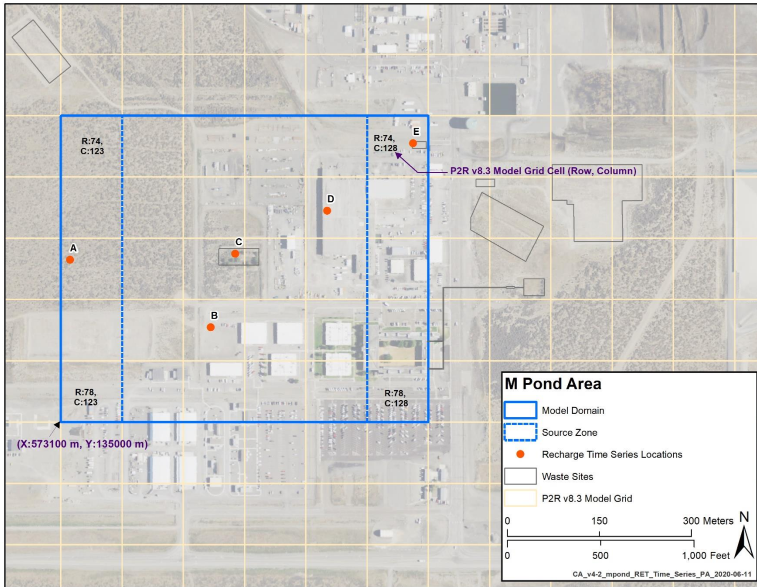
Figure 4-35. Locations of Recharge Rate Time Series Examples
