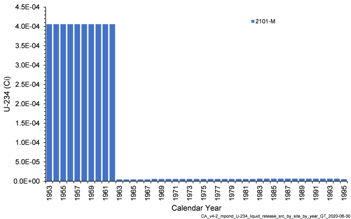
Figure 4-26. Annual U-234 Activity Released from Liquid Waste Sites in the M Pond Area Model
