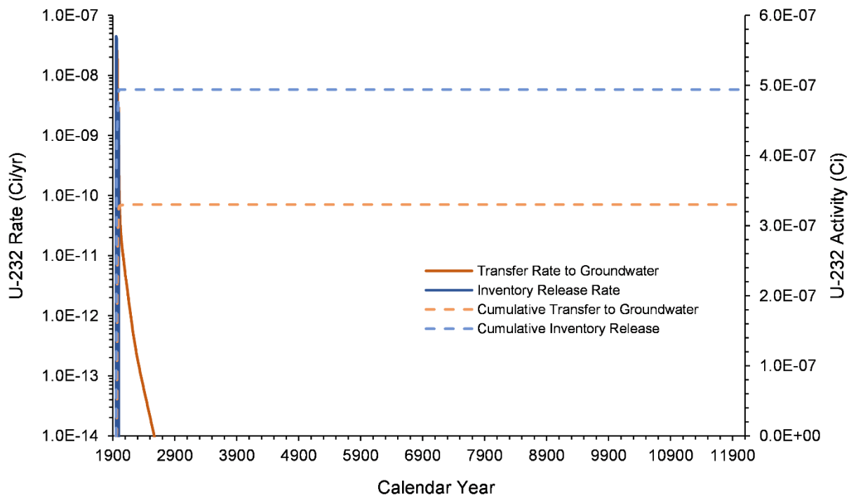
Figure 7-17. U-232 Inventory Release from Waste Sites and Transfer to Groundwater for the M Pond Area Model from 1943–12070
