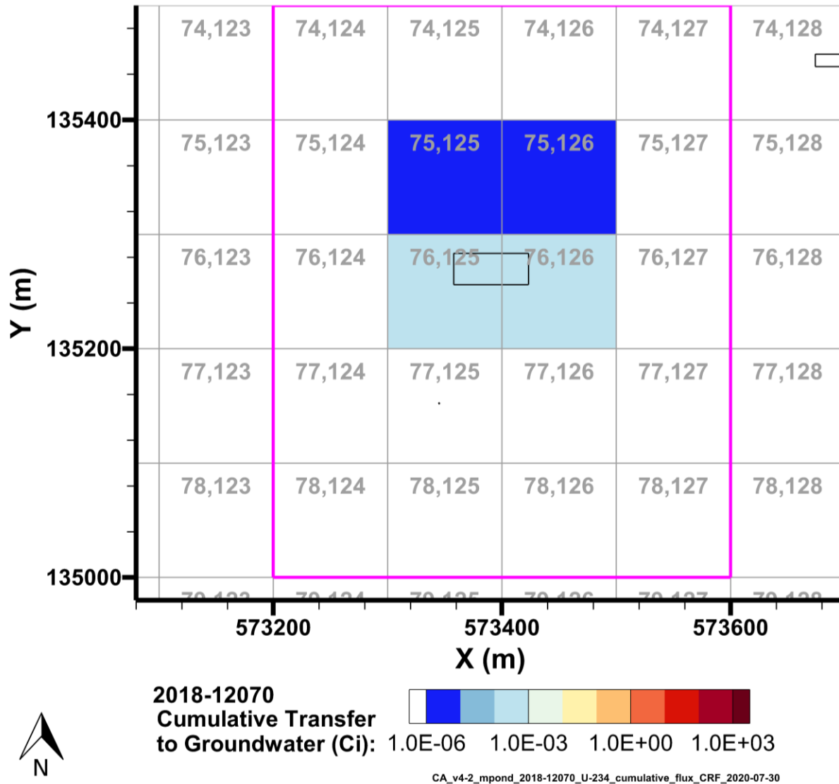
Figure 7-22. Cumulative U-234 Activity Discharged to Groundwater from the M Pond Area Model from 2018–12070 per P2R Grid Cell
