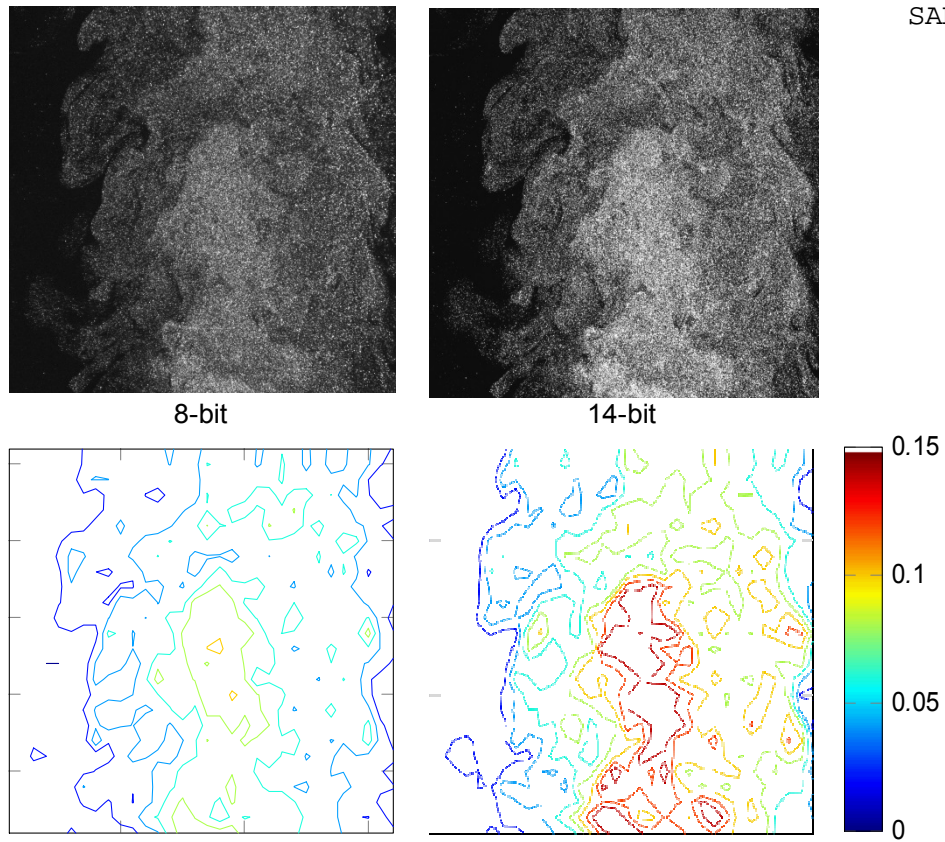
A PIV image (above) and the corresponding seeding density based on the ABD method (below) for images acquired simultaneously from two cameras with differing bit depth. The color bar shows the particle image density in particles/pixel. Images are used with permission from Sandia National Laboratories.
