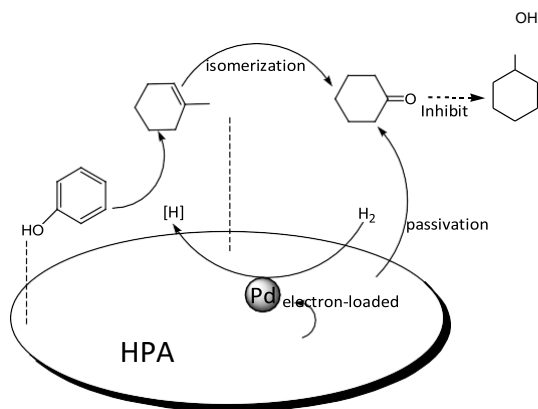
Scheme 1 Reaction mechanism of phenol over Pd/C-Heteropoly acid
