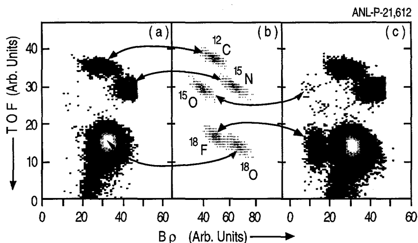
Fig. I-33. (a) Two-dimensional plot of time-of-flight (TOF) vs. magnetic rigidity (Bp) measured with the gas-filled magnet for 13.4-MeV ^{18}\text{O} ions bombarding a polypropylene target. (b) Raytrace calculation for various ions in a gas-filled magnet. See text for details. (c) Same as (a) but with a mixed ^{18}\text{F} - ^{18}\text{O} sample in the ion source.
