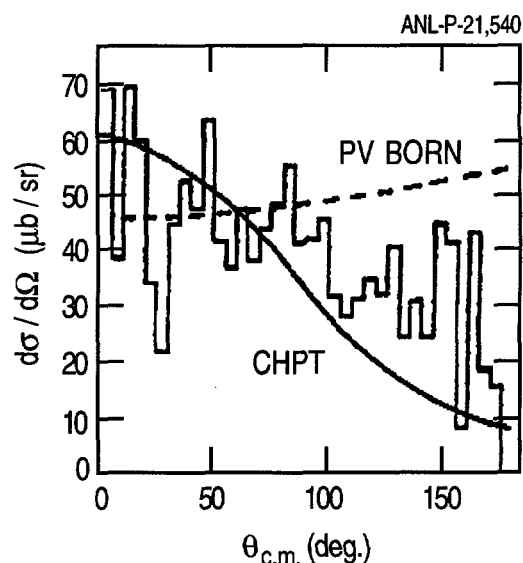
Fig. IV-1. Transverse differential cross sections of p(ee'\pi^0) reaction calculated from CHPT (solid) and PV coupling (dashed).
