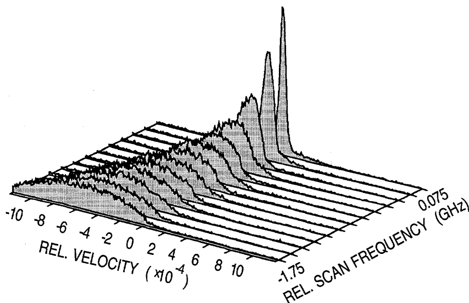
Fig. I-45. Velocity distributions measured by laser-induced fluorescence at various times during bunched-beam laser cooling. The center of each distribution is offset for clarity.
