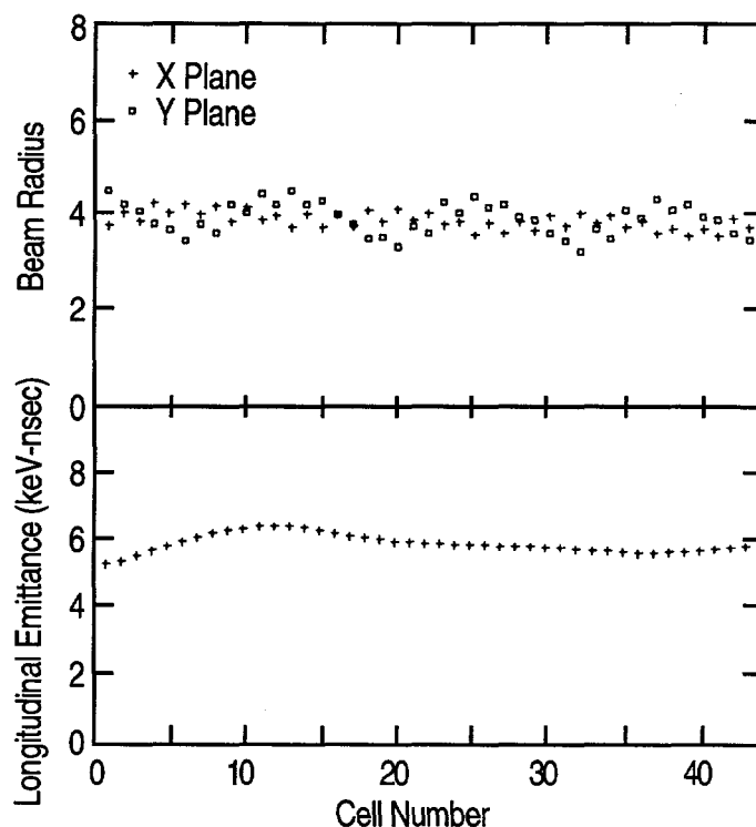
Fig. II-10. Beam dynamics calculation for a 12 MHz normally conducting RFQ appropriate for use to preaccelerate radioactive ions with q/m = 1/132 and normalized emittance of 0.25 \pi \text{ mm-mr} .
