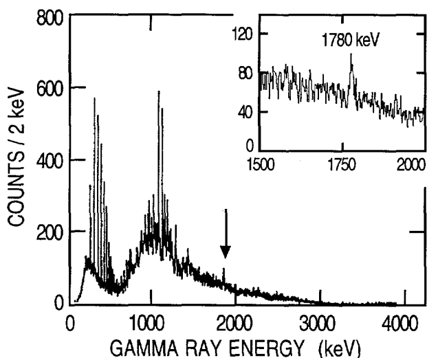
Fig. I-41. Doppler-corrected gamma-ray spectrum from ^{238}\text{U} + ^{208}\text{Pb} at 5.8 MeV/u.
