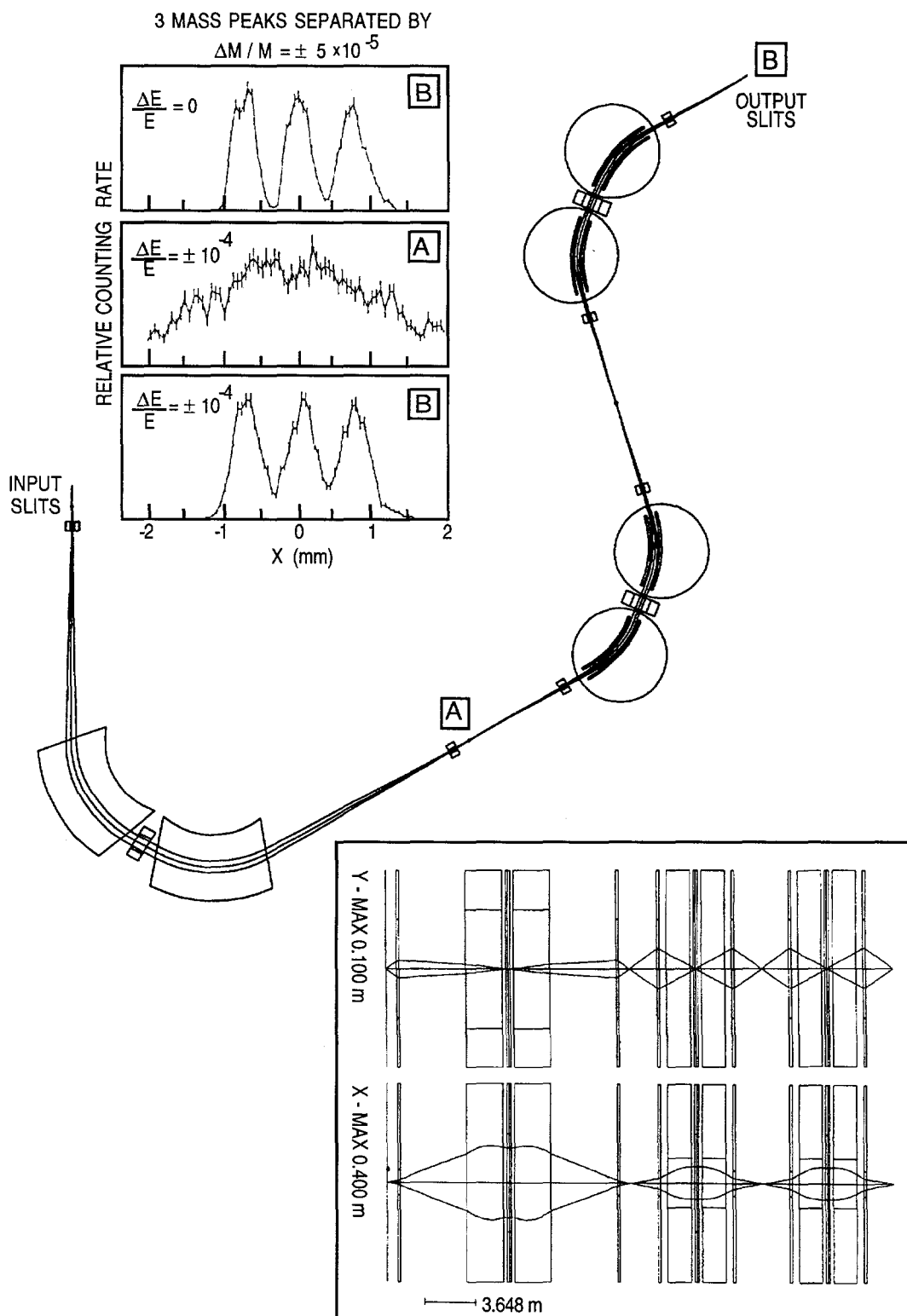
Fig. I-38. Schematic of the high-resolution mass separator. The location of the ion-optical elements (two magnetic and four electric dipoles) are indicated in the center part. Mass spectra for three masses with \Delta M/M = \pm 5 \times 10^{-5} calculated under different assumptions about the incident energy uncertainty are shown at points A and B along the beam path. The beam profile expected along the mass separator is shown in the lower panel.
