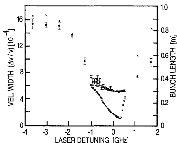
Fig. I-46. Longitudinal velocity spread (X's, left ordinate) and bunch length (dots, right ordinate) versus laser detuning, measured during a cooling scan. The laser is scanned past the optimum detuning, leading to the rise in temperature and bunch length at the right of the figure.
