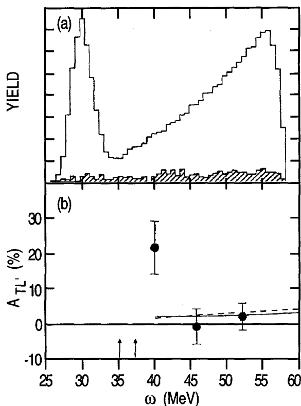
Fig. III-4. (a) Relative yield as a function of energy transfer for the target full vs. empty. The elastic peak is seen at \omega = 30 MeV. (b) Measured inelastic asymmetry as a function of \omega on the low-energy transfer side of the quasielastic peak. The error bars indicate the statistical uncertainty. The arrows point to the two- and three-body breakup thresholds. The curves correspond to the PWIA calculations of Schulze and Sauer (solid) and Salmé, Pace, and Ciofi degli Atti (dashed).
