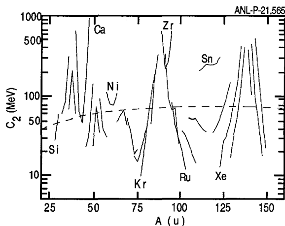
Fig. I-4. Restoring force parameter C_2 for stable even-even nuclei with masses between A = 28 and A = 150 . C_2 values for isotopes of a given element are connected by solid lines. The dashed line is the prediction from the liquid-drop model.
