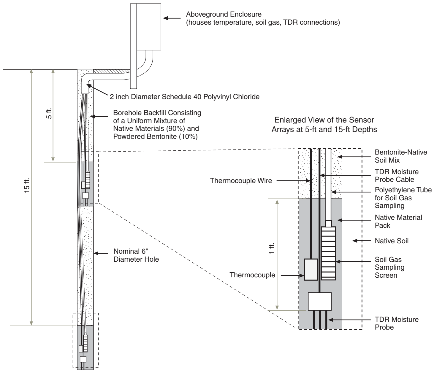
Figure 2.2-1 Configuration of Vertical Sensor Array Monitoring Subsystem
