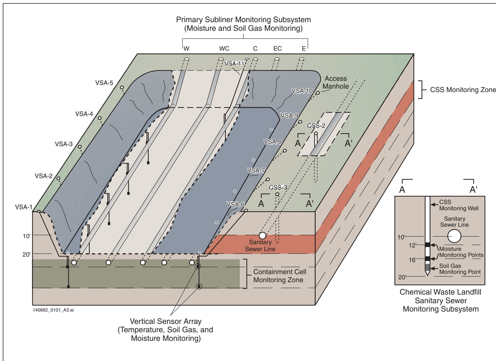
Figure 2-3 Block Diagram of CAMU Containment Cell and Vadose Zone Monitoring System
