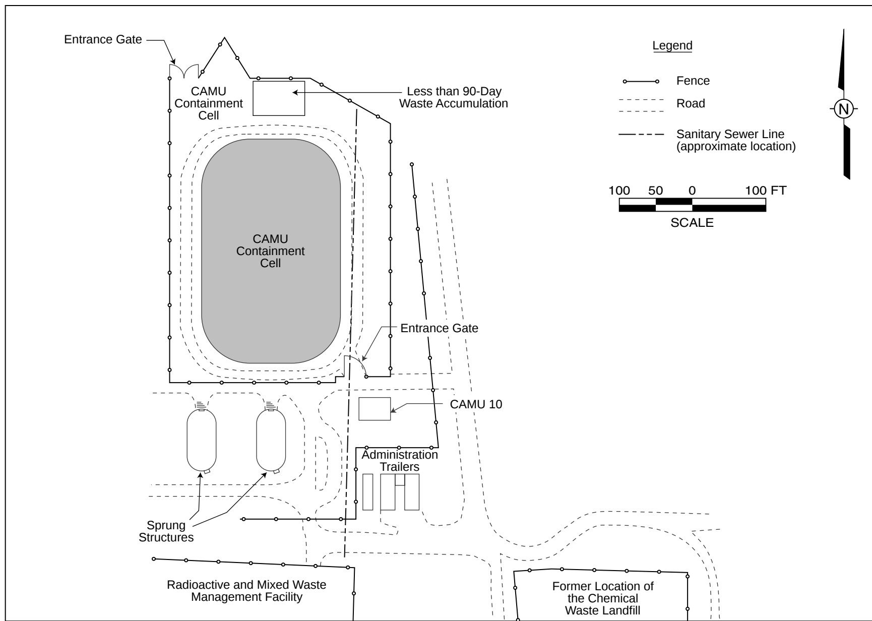
Figure 2-1 Local Area Map of CAMU Containment Cell
