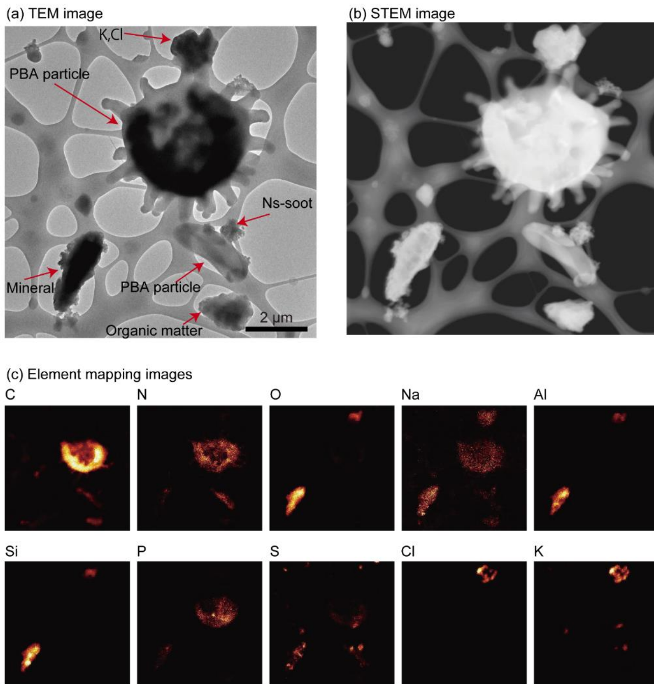
Supporting Figure 5. Shapes and compositions of PBA, mineral, and KCl particles. (a) TEM and (b) STEM and (c) element mapping images of these particles. The sample was collected from 0:00-0:30, 27 February, 2014.
