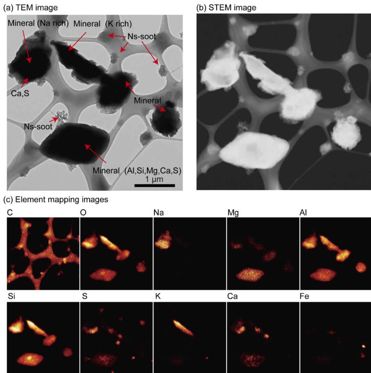
30 Supporting Figure 2. Shapes and compositions of mineral particles. (a) TEM and (b) STEM and (c) element mapping images of mineral particles. These mineral particles contain Al-Si-Mg-O-, Al-Si-Na-O-, or Al-Si-K-O-rich grains. There are Ca- or Fe-rich grains within the mineral particles. Ns-soot and sulfate particles also occur. The sample was collected from 12:00-12:30, 29 March, 2014.
