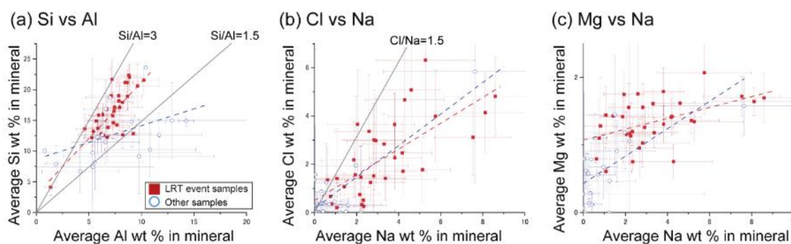
Figure 7. Relations (a) between average Si and Al weight % in mineral particles, (b) between average Cl and Na weight % in mineral particles, and (c) between average Mg and Na weight % in mineral particles. Red squares indicate sample averaged values for LRT period samples. Blue open circles indicate sample average values for other (non-LRT period) samples. The sample from 9:00 on 6 February had only one mineral particle and is not shown in the plots because it has a large Al fraction and no Na (0, 30, and 1 weight % for Na, Al, and Si, respectively). Coefficients R^2 of determination for (a), (b), and (c) were 0.60, 0.47, and 0.24 for the LRT period samples and 0.18, 0.66, and 0.40 for other samples, respectively. Trend lines are shown in red and blue broken lines for LRT period and other samples, respectively. The correlation between Si and Al for other samples (a) is relatively low because of possible contributions from two sources (LRT and local dusts). Error bars indicate the 95% confidence intervals.
