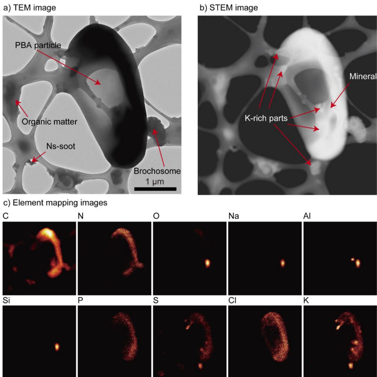
Supporting Figure 3. Shape and composition of PBA particle with K-rich grains. (a) TEM and (b) STEM and (c) element mapping images of the PBA particle. A mineral particle attaches to the PBA particle. The sample was collected from 3:00-3:30, 15 March, 2014.
