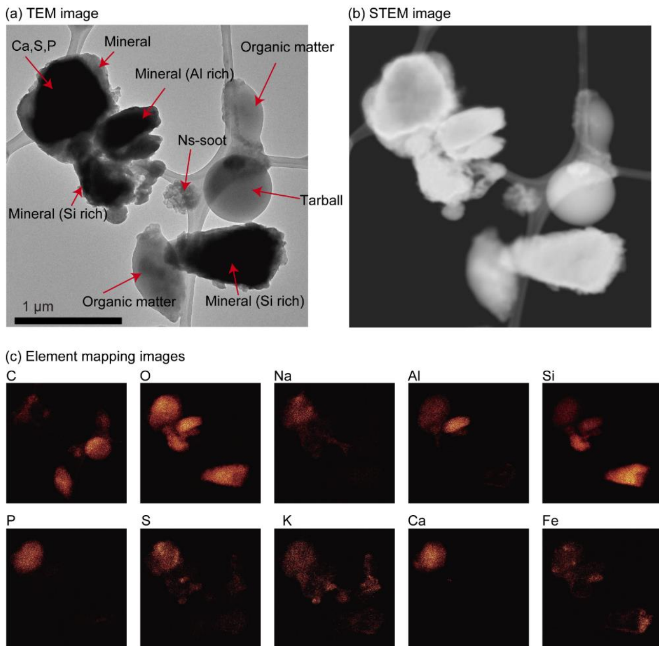
70 Supporting Figure 9. Shapes and compositions of mineral and carbonaceous particles, including tarball, ns-soot, and organic matters (primary organic aerosol (POA) particles). (a) TEM and (b) STEM and (c) element mapping images of these particles. The mineral particles include those with Al- and Si-rich particles. The sample was collected from 12:00-12:30, 14 February, 2014.
