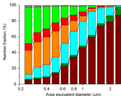
(c) Number fractions for other periods
