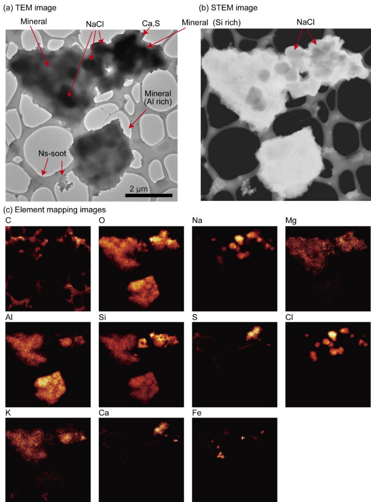
Supporting Figure 6. Shapes and compositions of mineral particles that attach sea-salt (NaCl) particles. (a) TEM and (b) STEM images and (c) element mapping images of these particles. The sample was collected from 18:00-18:30, 2 February, 2014. Mg distributes over the upper particle, suggesting that hydrate Mg salt coated the particles.
