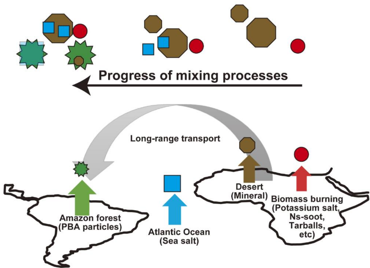
Figure 12. Schematic image of possible particle sources and transport pathways. Top images show the progress of individual-particle mixings during LRT. The bottom image shows possible major sources for each particle (Martin et al., 2010b).
