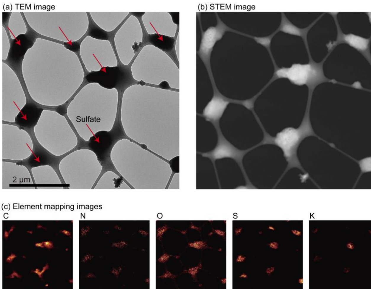
Supporting Figure 8. Shapes and compositions of sulfate particles. (a) TEM and (b) STEM and (c) element mapping images of these particles. These sulfate particles include N, O, S, and K, implying that they are ammonium or potassium sulfate. Carbon occurs around the sulfate, showing that the sulfates are coated by secondary organic matters and have ns-soot inclusions. Sulfate particles deform over the substrates and decompose after intense electron beam irradiation. The sample was collected during 12:55-13:25, 26 March, 2014.
