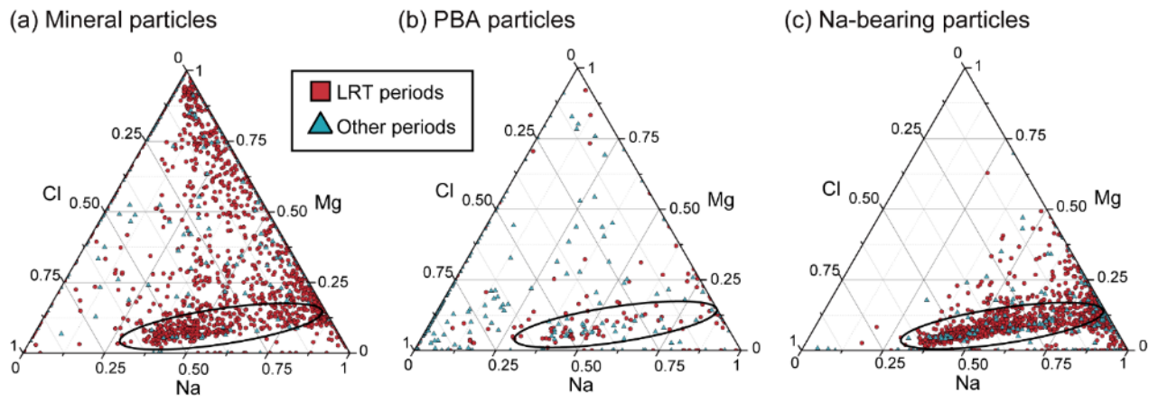
Figure 10. Weight % ratios among Na, Mg, and Cl within (a) mineral particles, (b) PBA particles, and (c) Na-bearing particles. The black ellipse areas indicate typical sea-salt compositions from a marine source.
