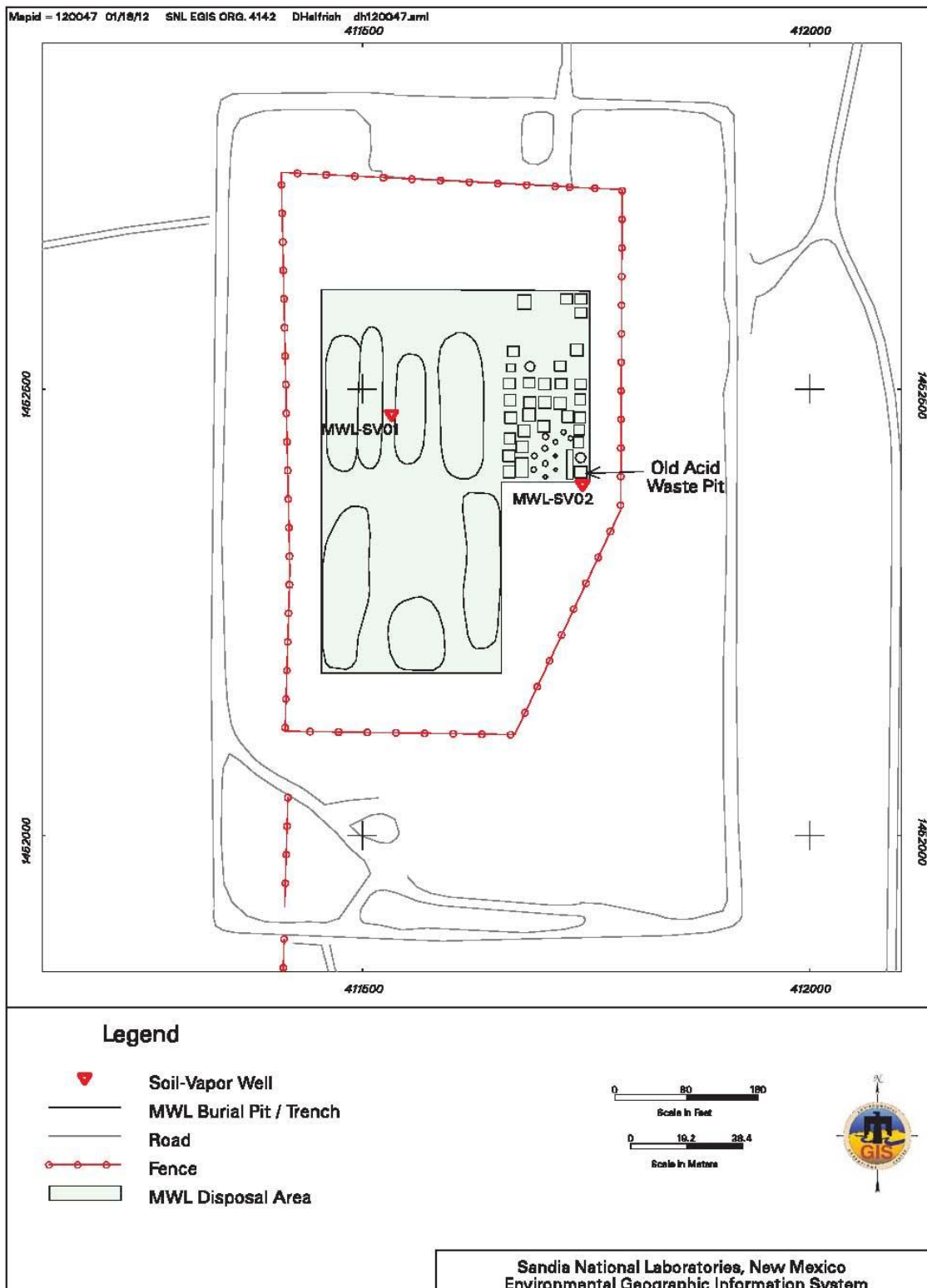
Figure 1-2 Mixed Waste Landfill Location of Soil-Vapor Wells MWL-SV01 and MWL-SV02
