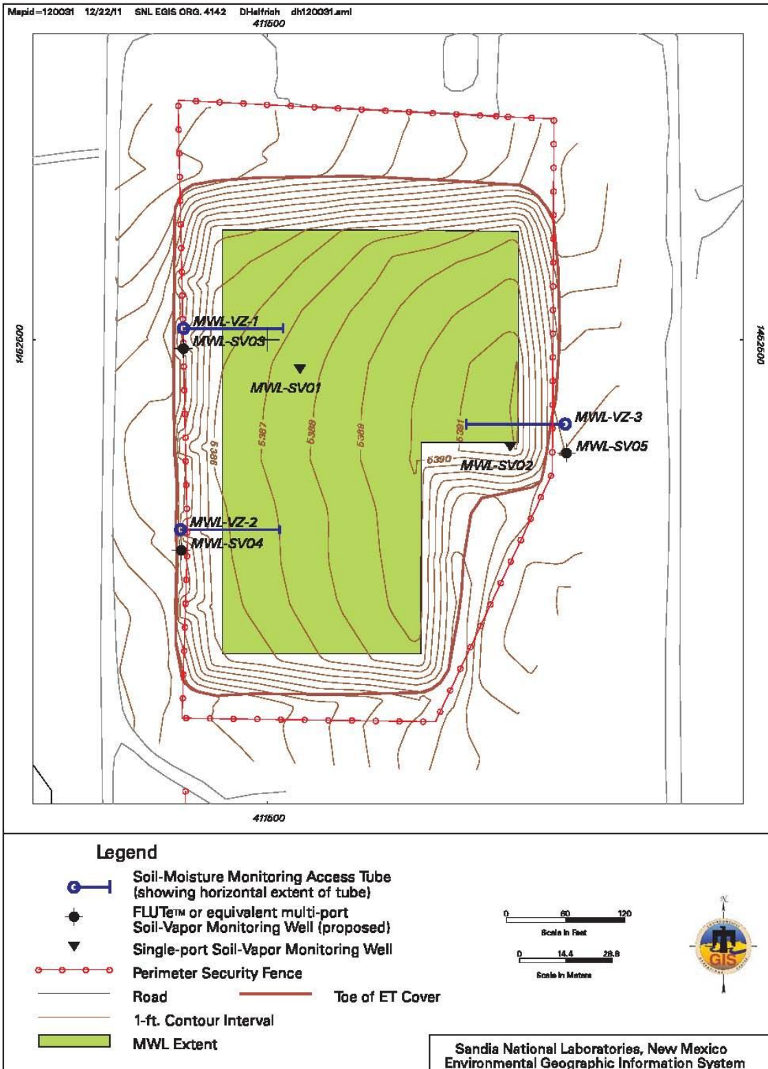
Figure 3.4.1-1 Soil-Vapor Monitoring Well and Soil-Moisture Monitoring Access Tube Locations at the Mixed Waste Landfill
