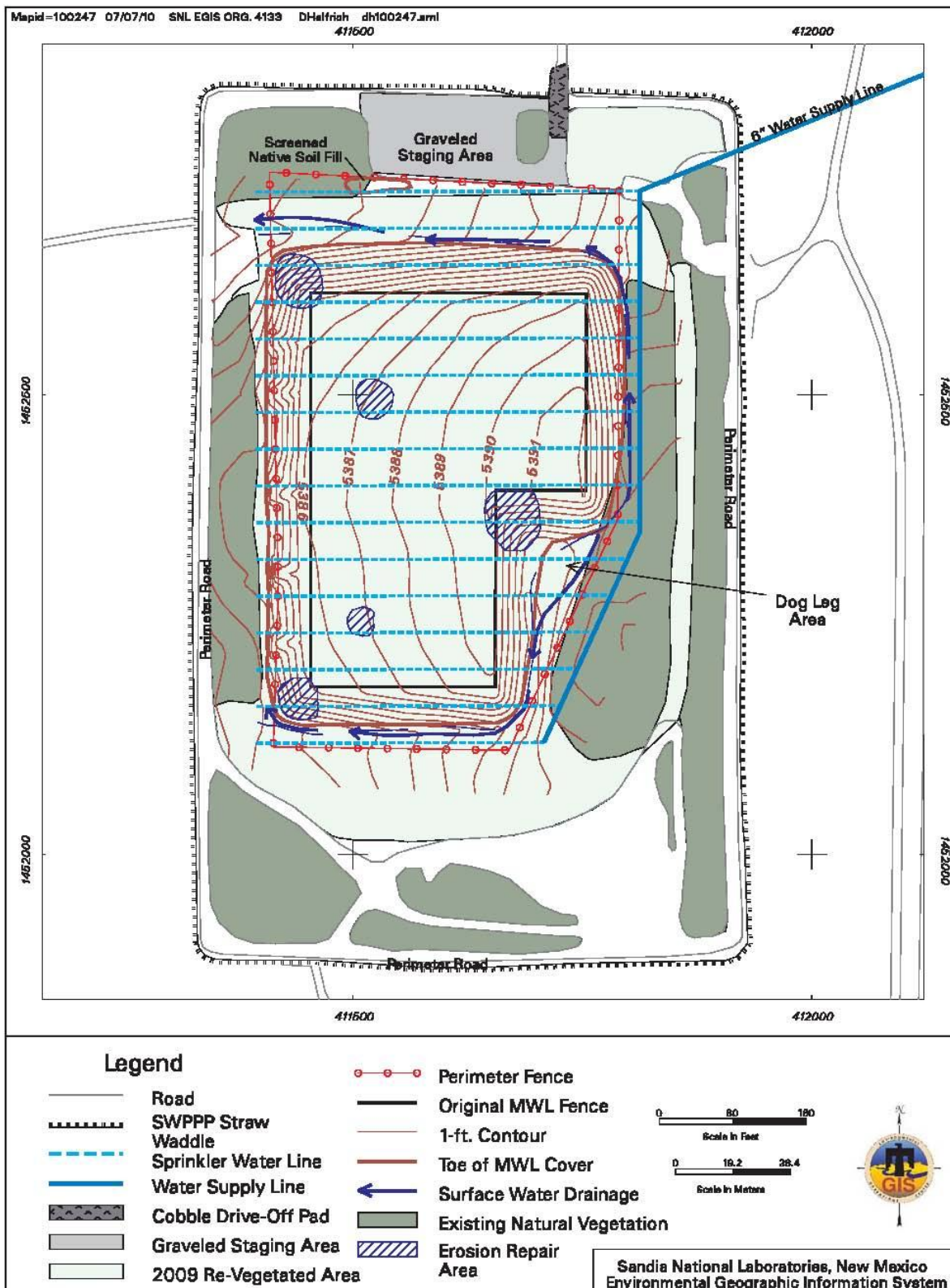
Figure B-1 MWL Temporary Irrigation System, 2009
