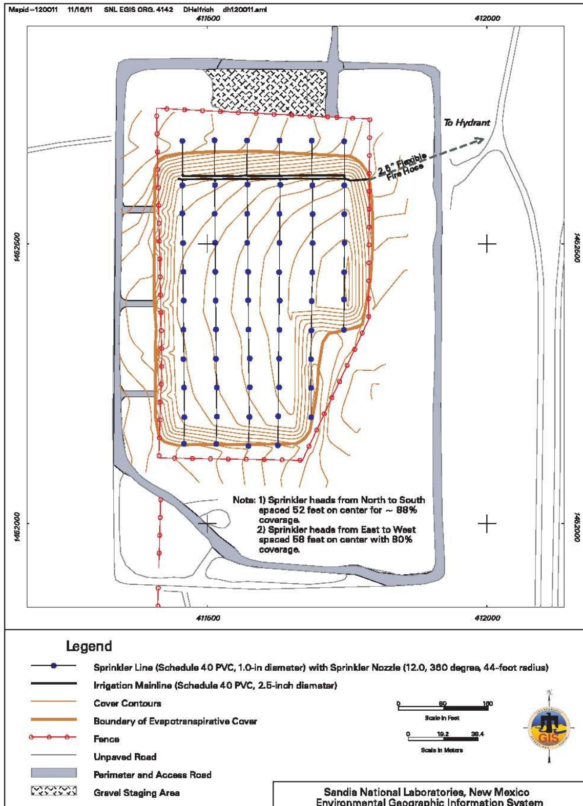
Figure B-3 Temporary Supplemental Watering System at the Mixed Waste Landfill
