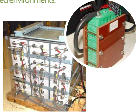
The Energy Storage Analysis Laboratory tests from cell to module systems, ranging from 1 V to 50 V and from the mA to 1000 A range.
