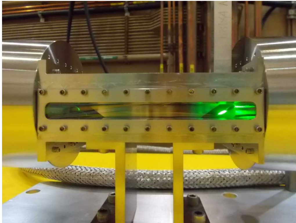
The White Dwarf Gas Cell with green alignment laser
