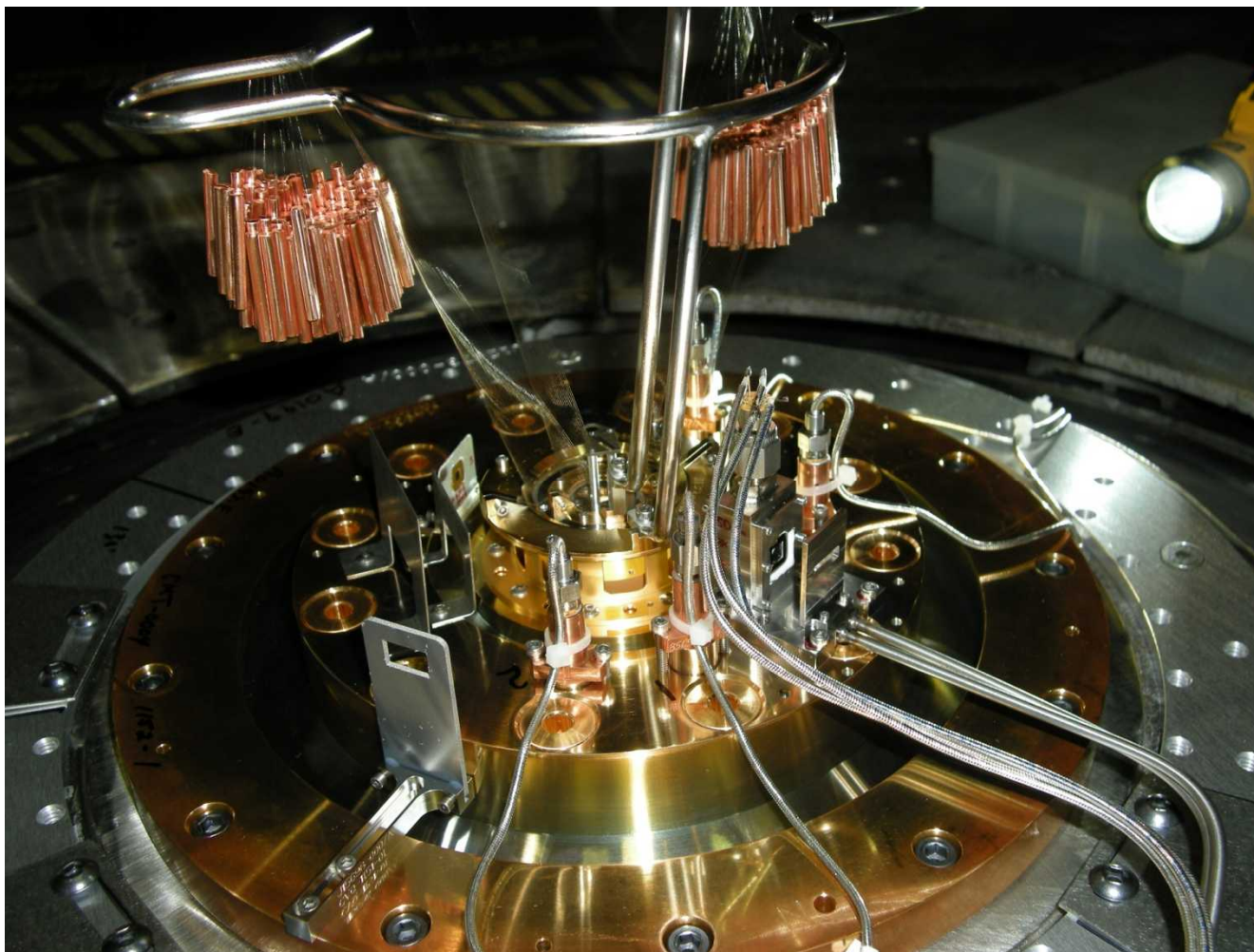
The Z-pinch radiation source used to heat the gas cell
