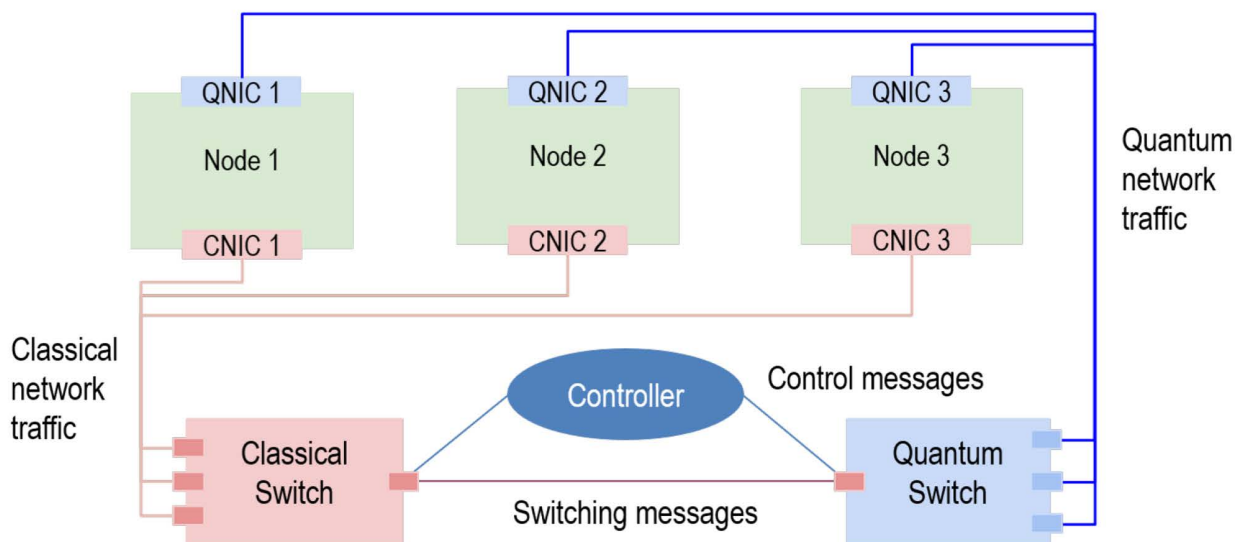
Figure 3:I. Design schematic for a three-node quantum network with SDN controller connected to both the classical and quantum switch. Reproduced from "Proc. SPIE 9873, Quantum Information and Computation IX," 98730B (2016).
