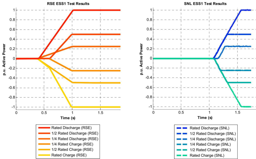
Figure 10: RSE and SANDIA test results for ESS1 function
