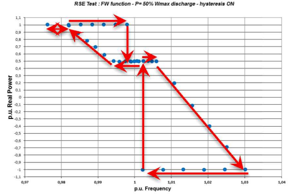
Figure 8: RSE test results for the Italian grid code FW curves without hysteresis.
