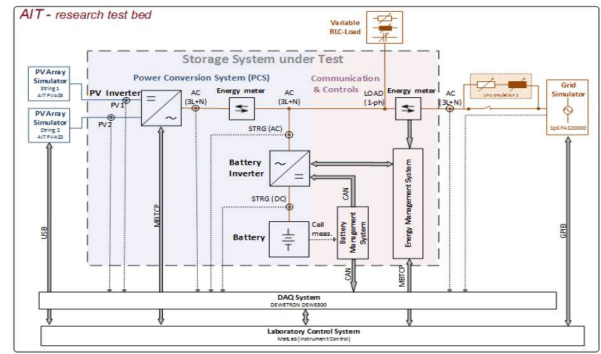
Figure 4: AIT Smart Electricity Systems and Technologies (SmartEST) PV inverter test laboratory.
