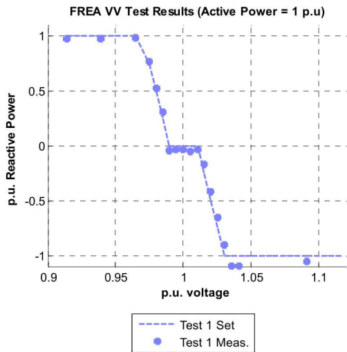
Figure 13: Example of FREA test results for VV function (one test case at rated active power).
