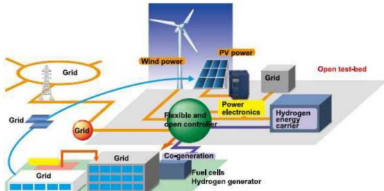
Figure 7: FREA Open test bed for testing of grid-connected inverters and energy storage systems.
