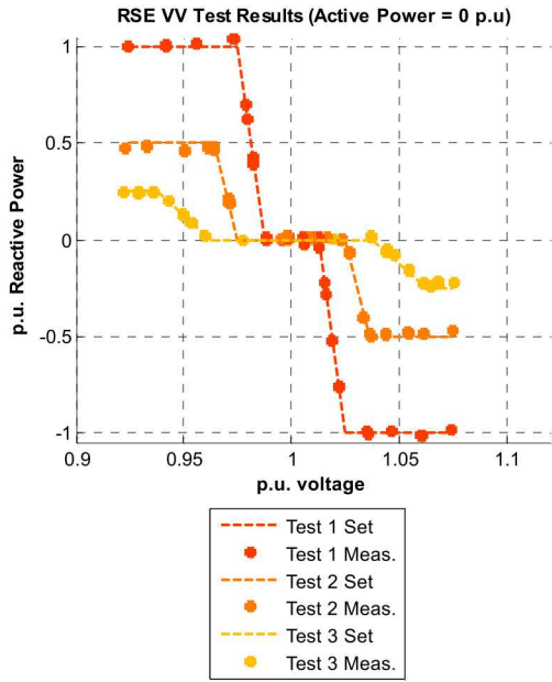
Figure 12: Example of RSE test results for VV function (three test cases with no active power).
