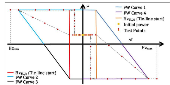
Figure 2: Frequency test points required for FW Domain tests. The points are traced with the grid simulator to reach the hysteresis values.
