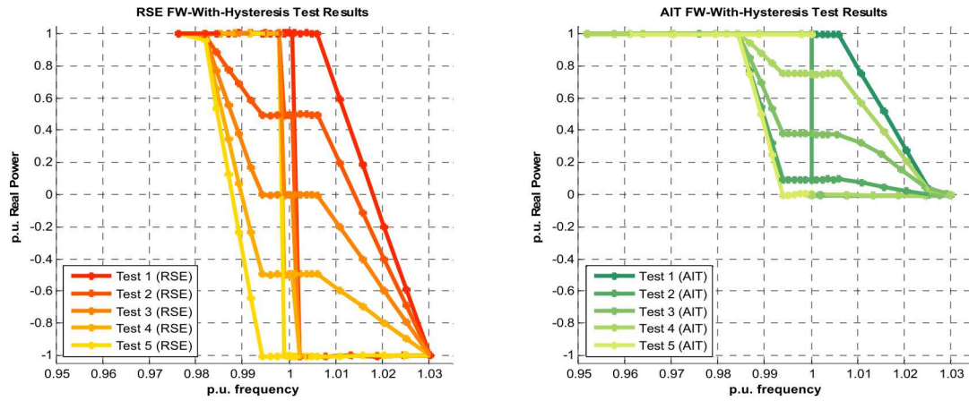
Figure 9: RSE and AIT Test Results for FW with hysteresis.
