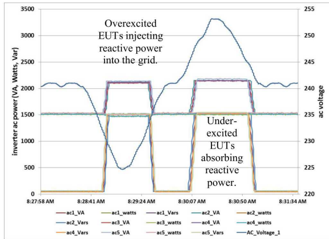
Fig. 5. Volt-VAR evaluations conducted on five inverters.
