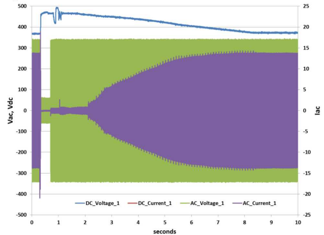
Fig. 3. Voltage < 50% of nominal ride through.
