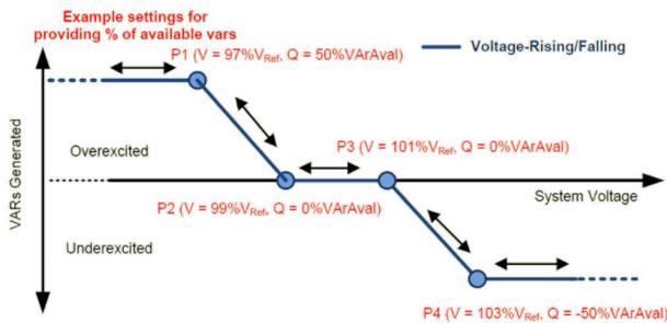
Fig. 1. Typical volt-VAr curve.
