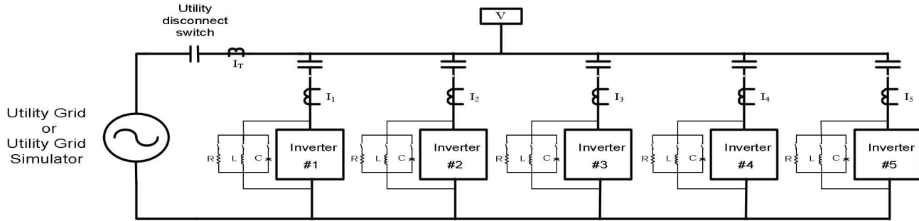
Fig. 2. Single or multi-inverter test configuration.
