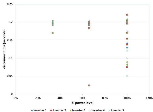
Fig. 11. Unintentional islanding test results with five inverters.
