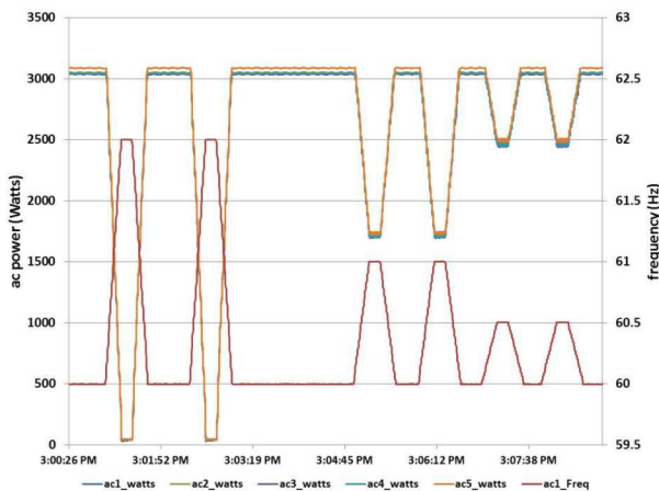
Fig. 9. Frequency-watt results with high-frequency deviation.
