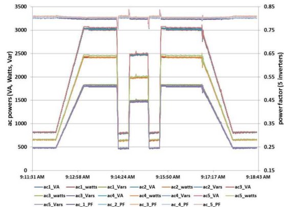
Fig. 7. PF evaluation with varying dc/ac power.
