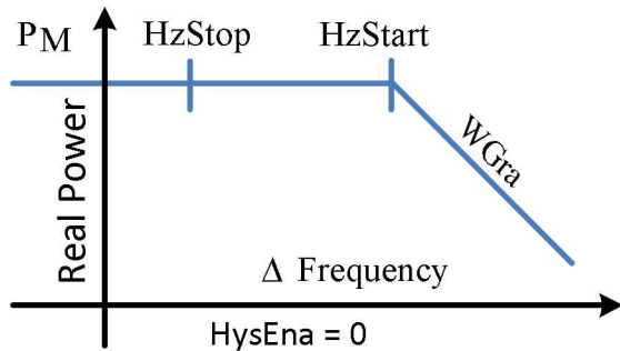
Fig. 8. Single frequency-watt curve.
