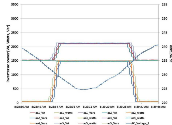
Fig. 6. Detailed five-inverter volt-VAR test results.
