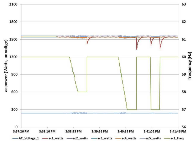
Fig. 10. Frequency-watt results with low-frequency deviation.
