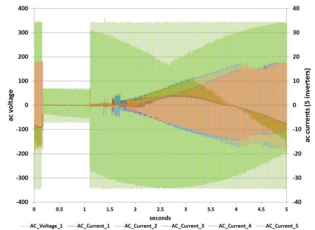
Fig. 4. Voltage < 50% of nominal ride through (5-inverter configuration).
