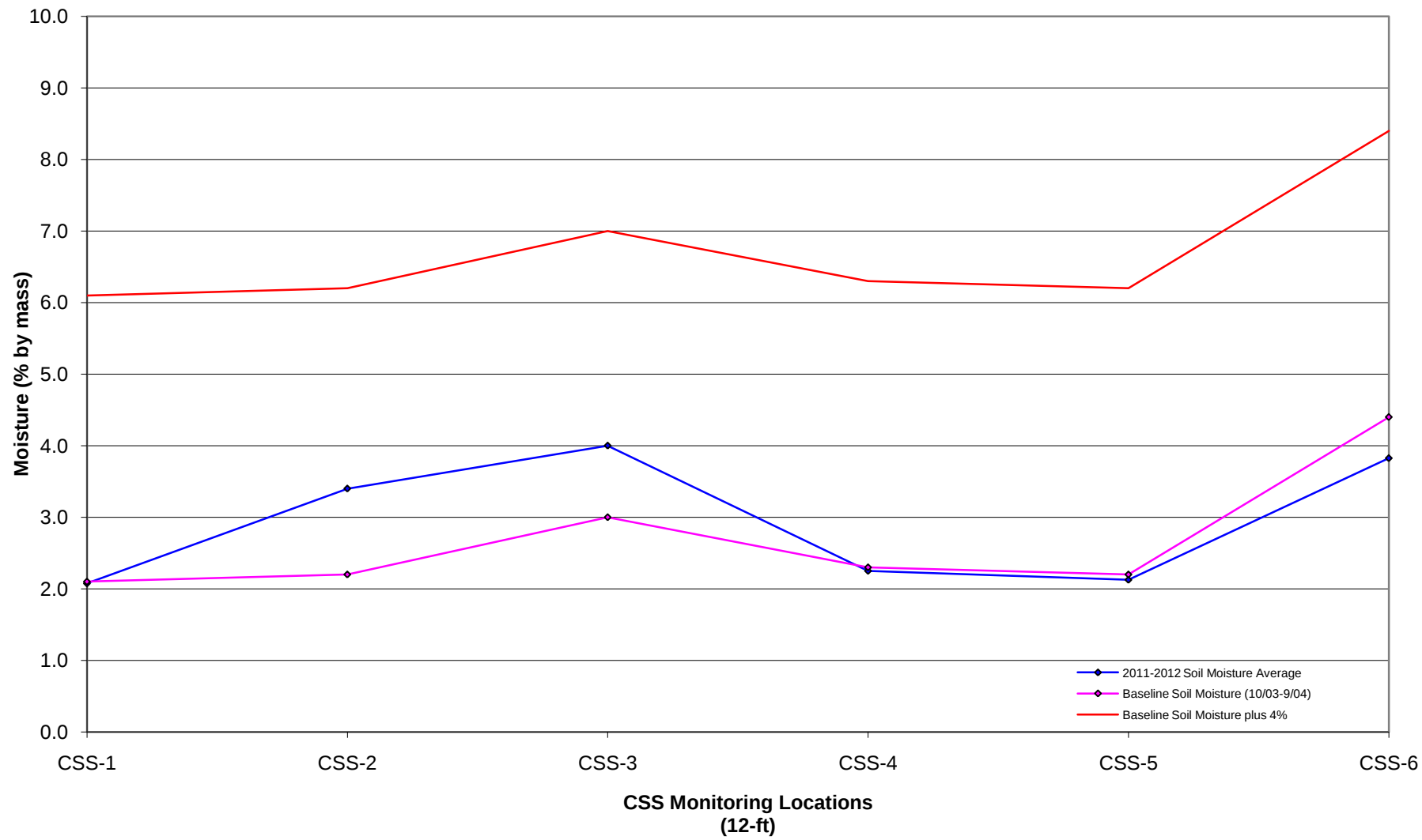
Figure C-1 Graph of CSS Soil Moisture Monitoring Results (12-Foot Monitoring Depth) July 2011–June 2012
