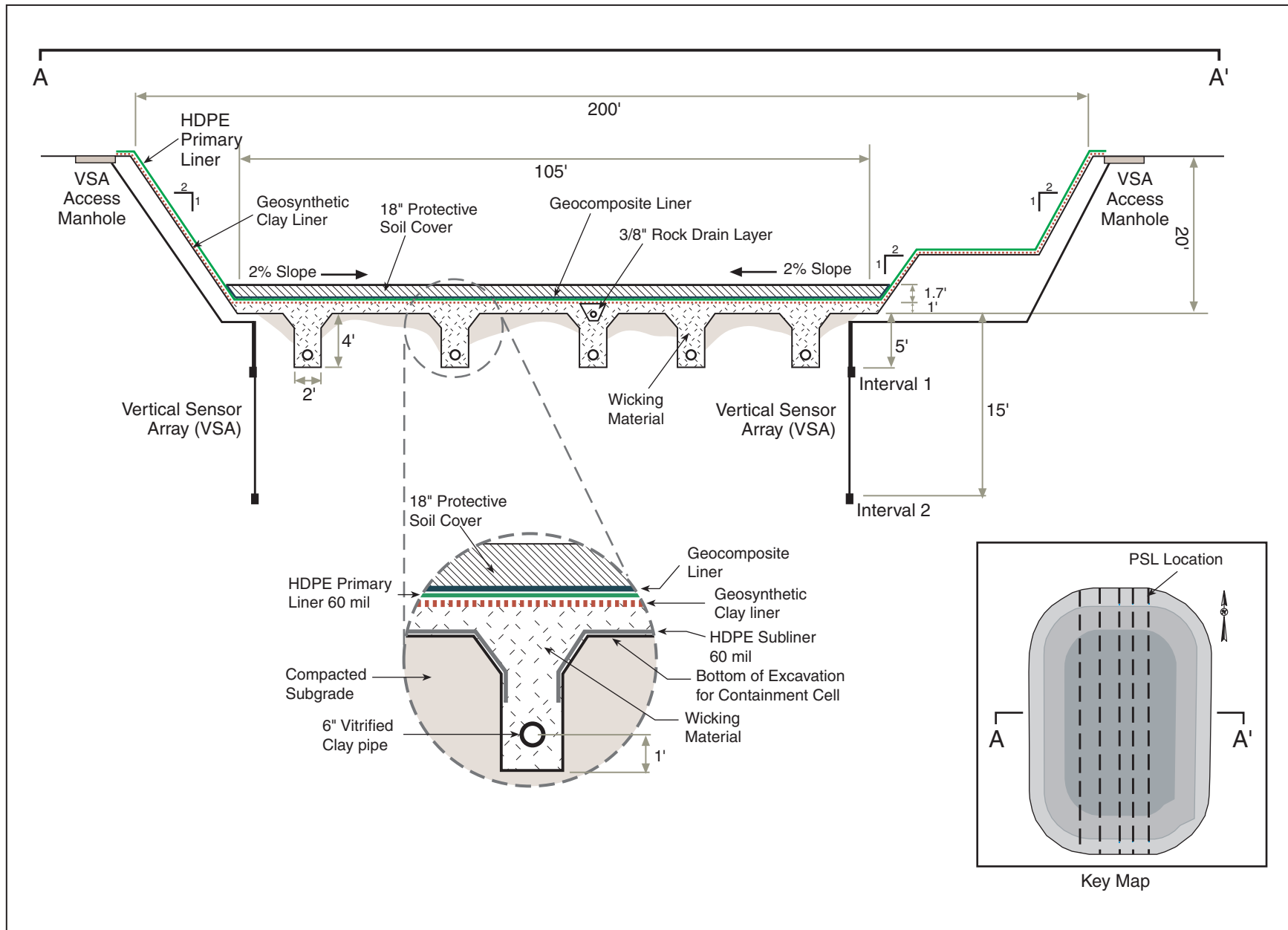
Figure 2.1-1 Cross-Sectional View of CAMU Containment Cell and Primary Subliner Monitoring Subsystem
