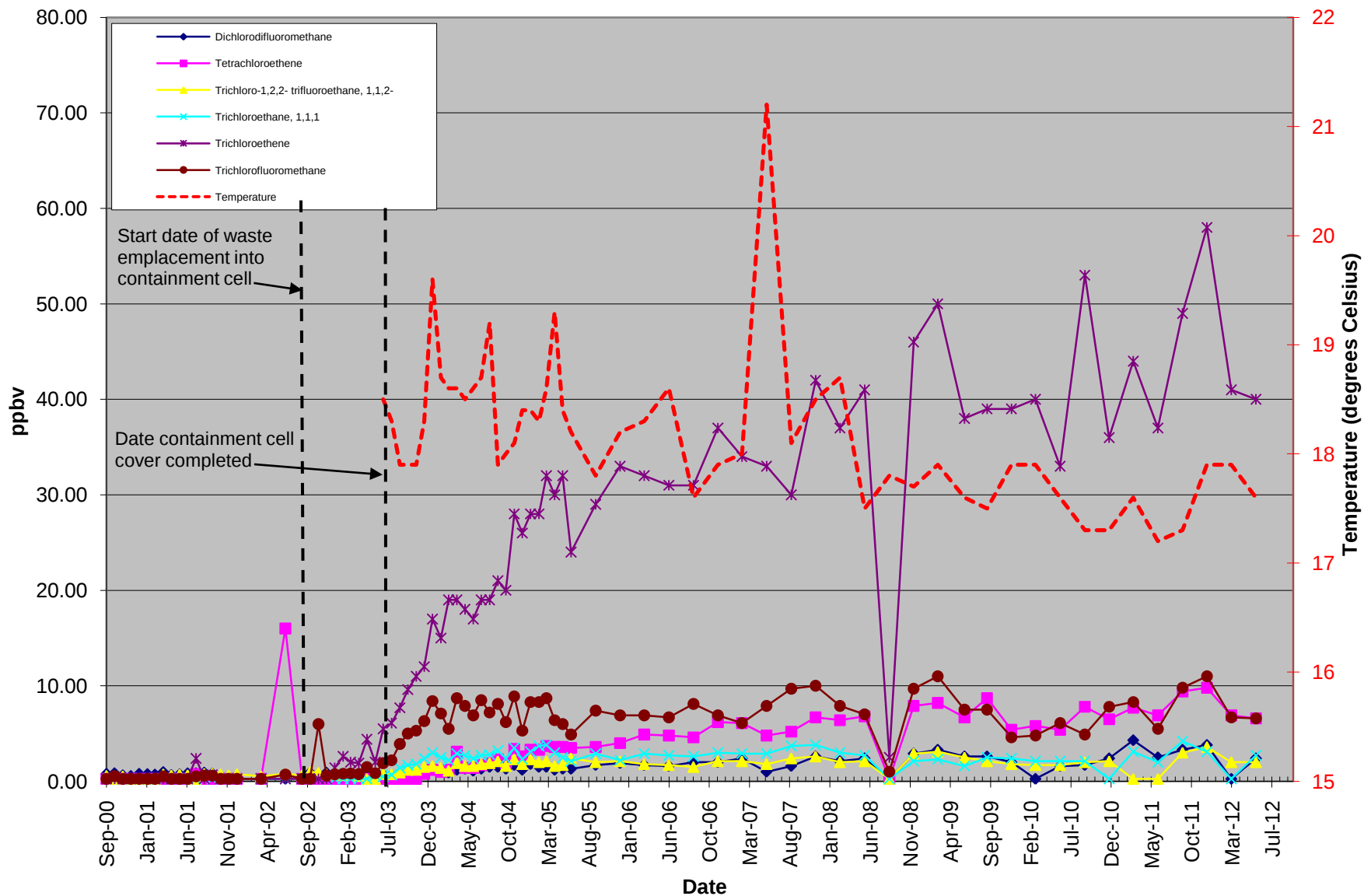
Figure D-16 Graph of VOC Concentrations at VSA5-15
