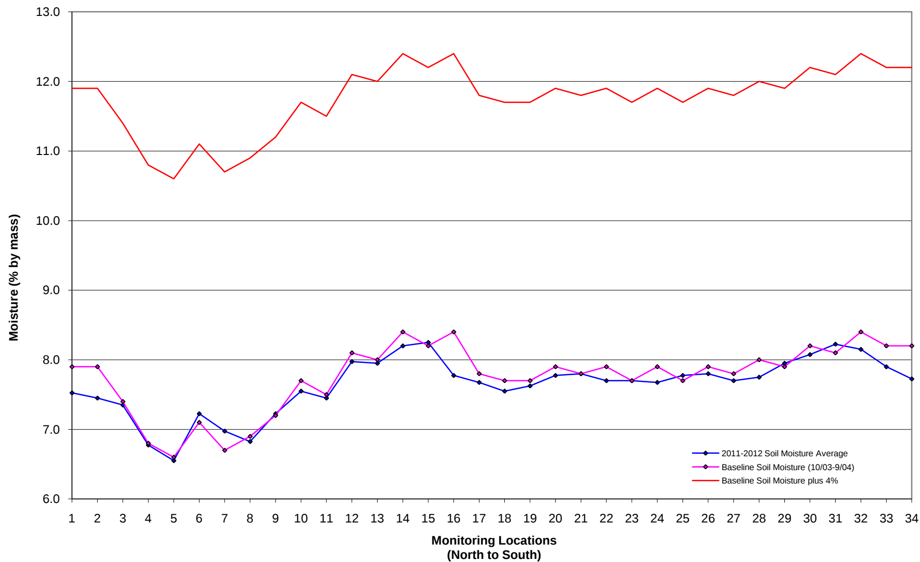
Figure A-5 Graph of PSL Soil Moisture Monitoring Results for the East Access Tube July 2011–June 2012
