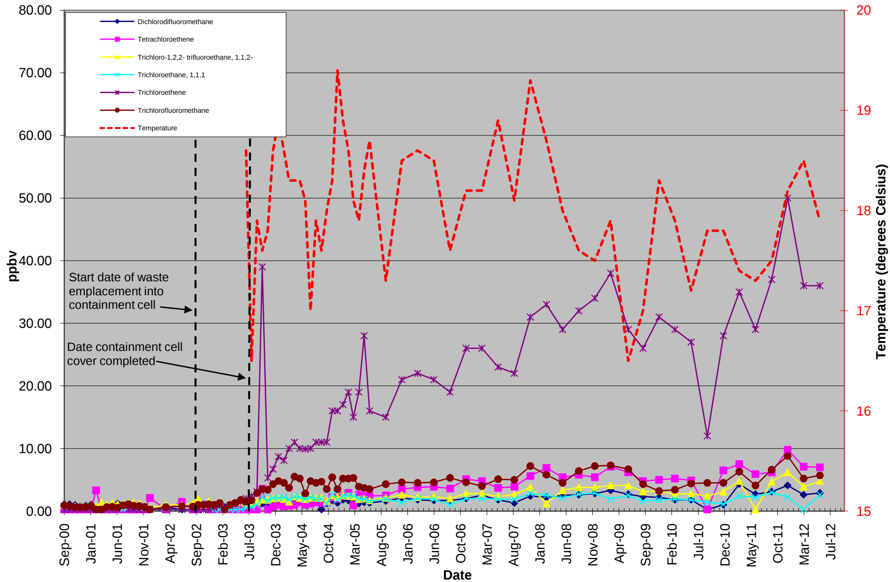
Figure D-8 Graph of VOC Concentrations at VSA1-15
