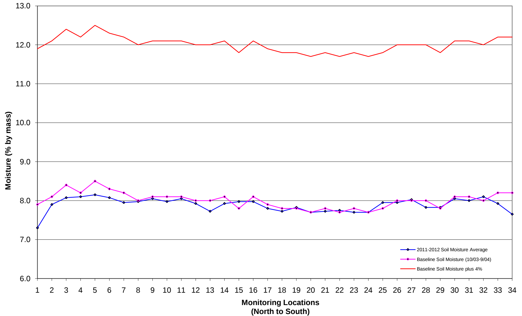
Figure A-1 Graph of PSL Soil Moisture Monitoring Results for the West Access Tube July 2011–June 2012
