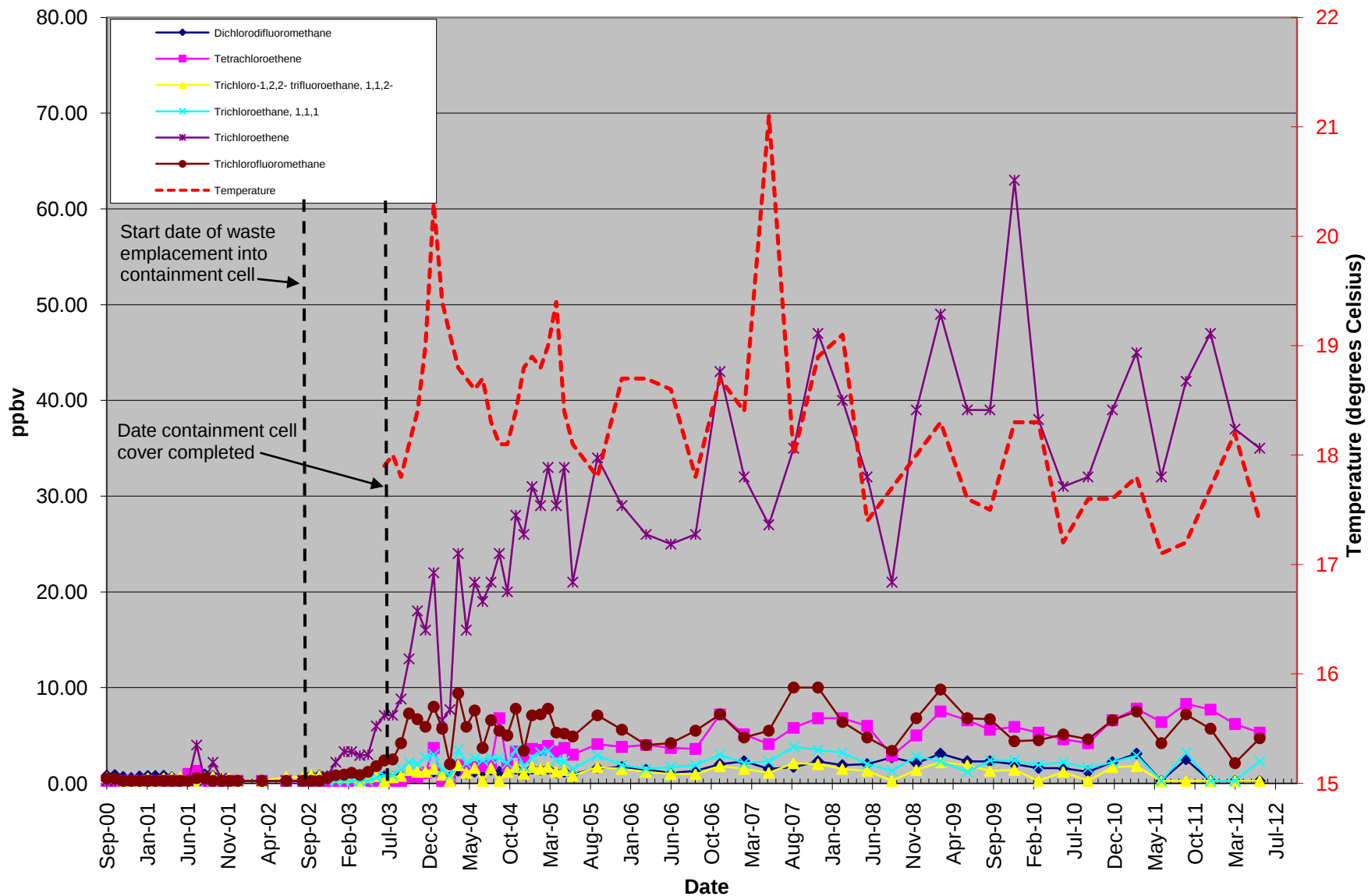
Figure D-15 Graph of VOC Concentrations at VSA5-5
