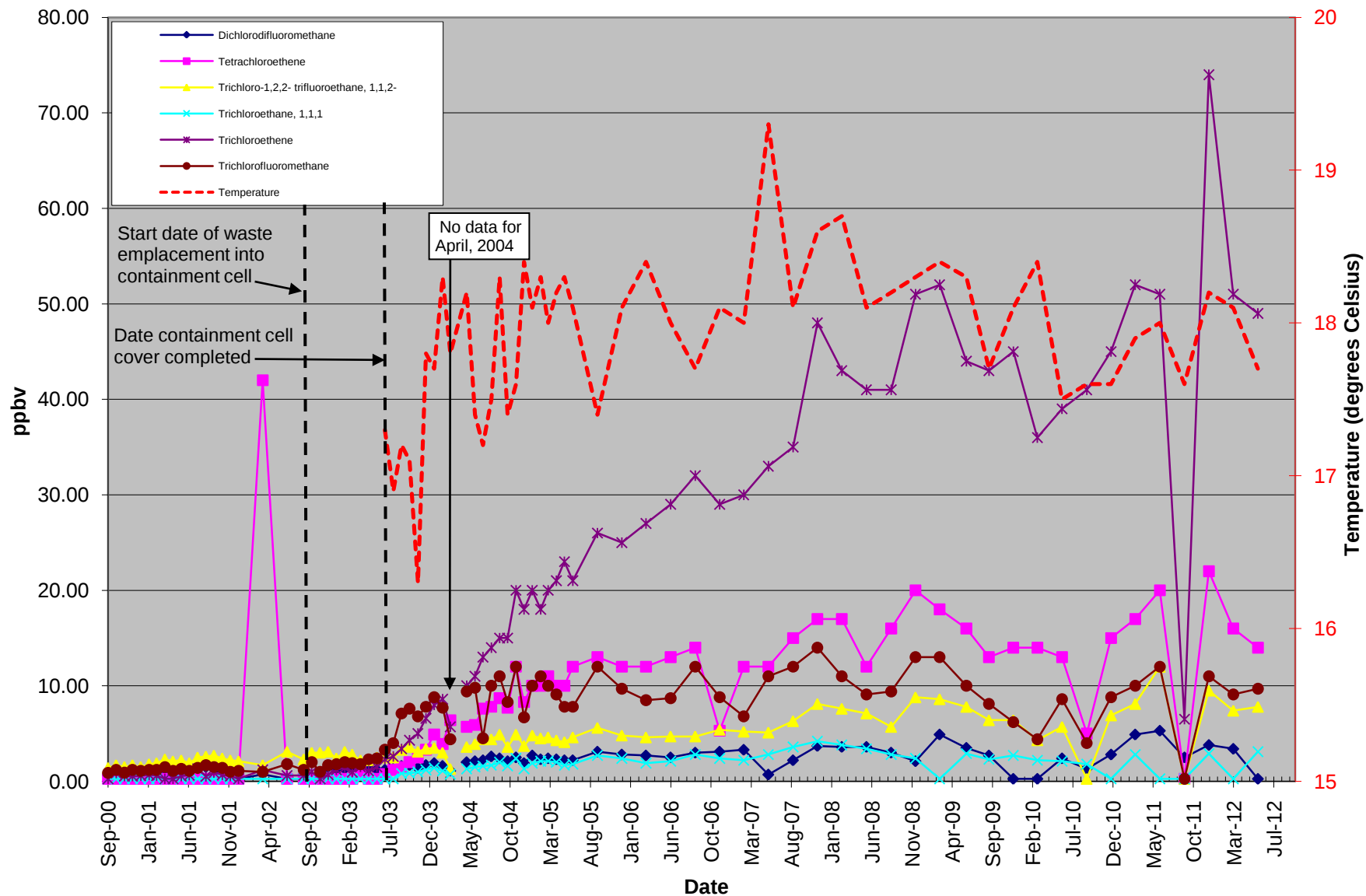
Figure D-18 Graph of VOC Concentrations at VSA6-15
