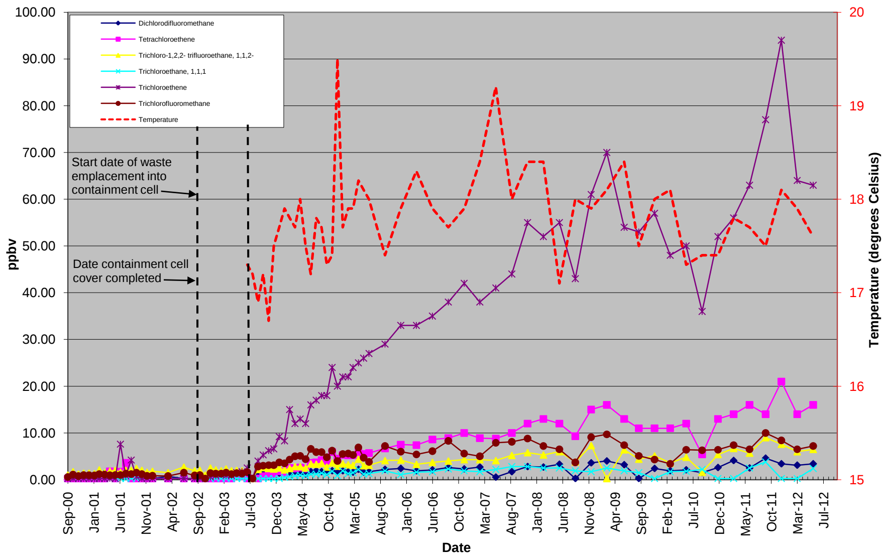
Figure D-20 Graph of VOC Concentrations at VSA7-15
