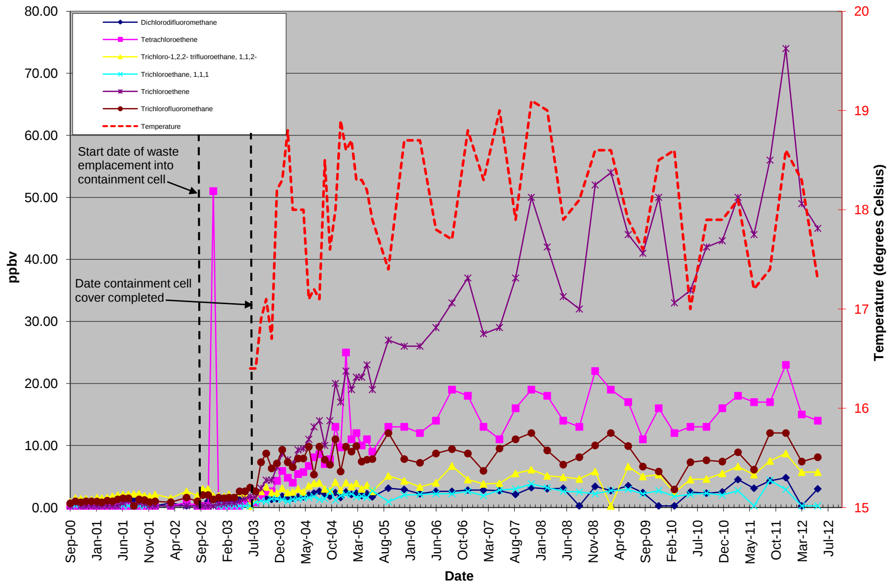
Figure D-17 Graph of VOC Concentrations at VSA6-5
