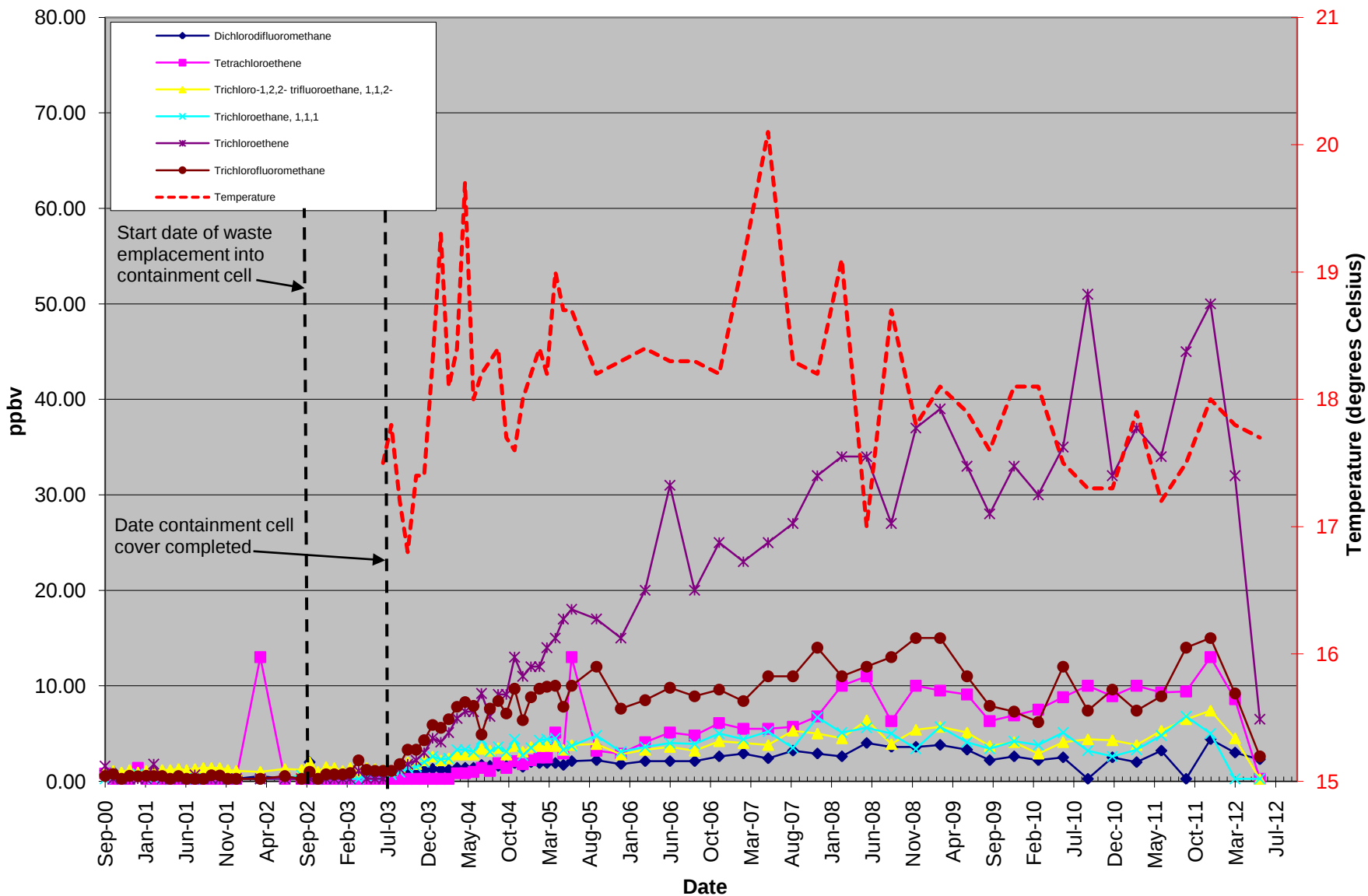
Figure D-26 Graph of VOC Concentrations at VSA10-15
