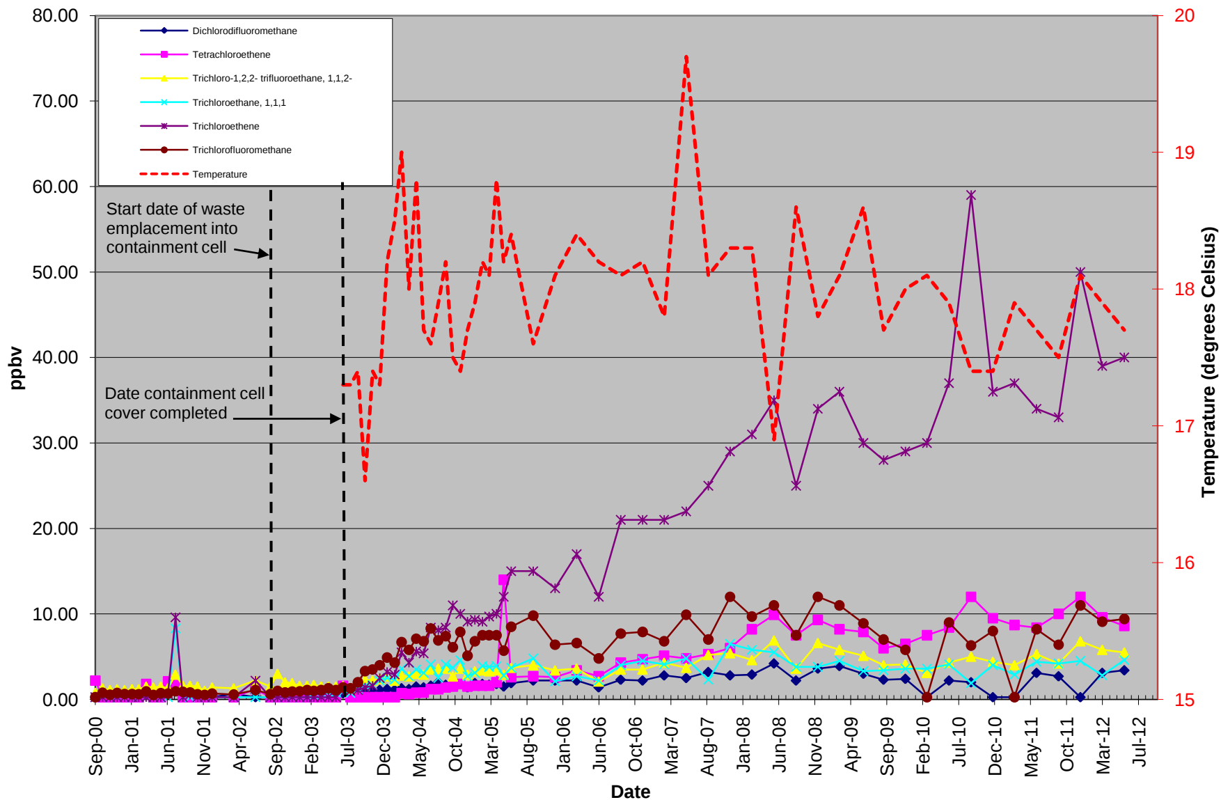
Figure D-24 Graph of VOC Concentrations at VSA9-15
