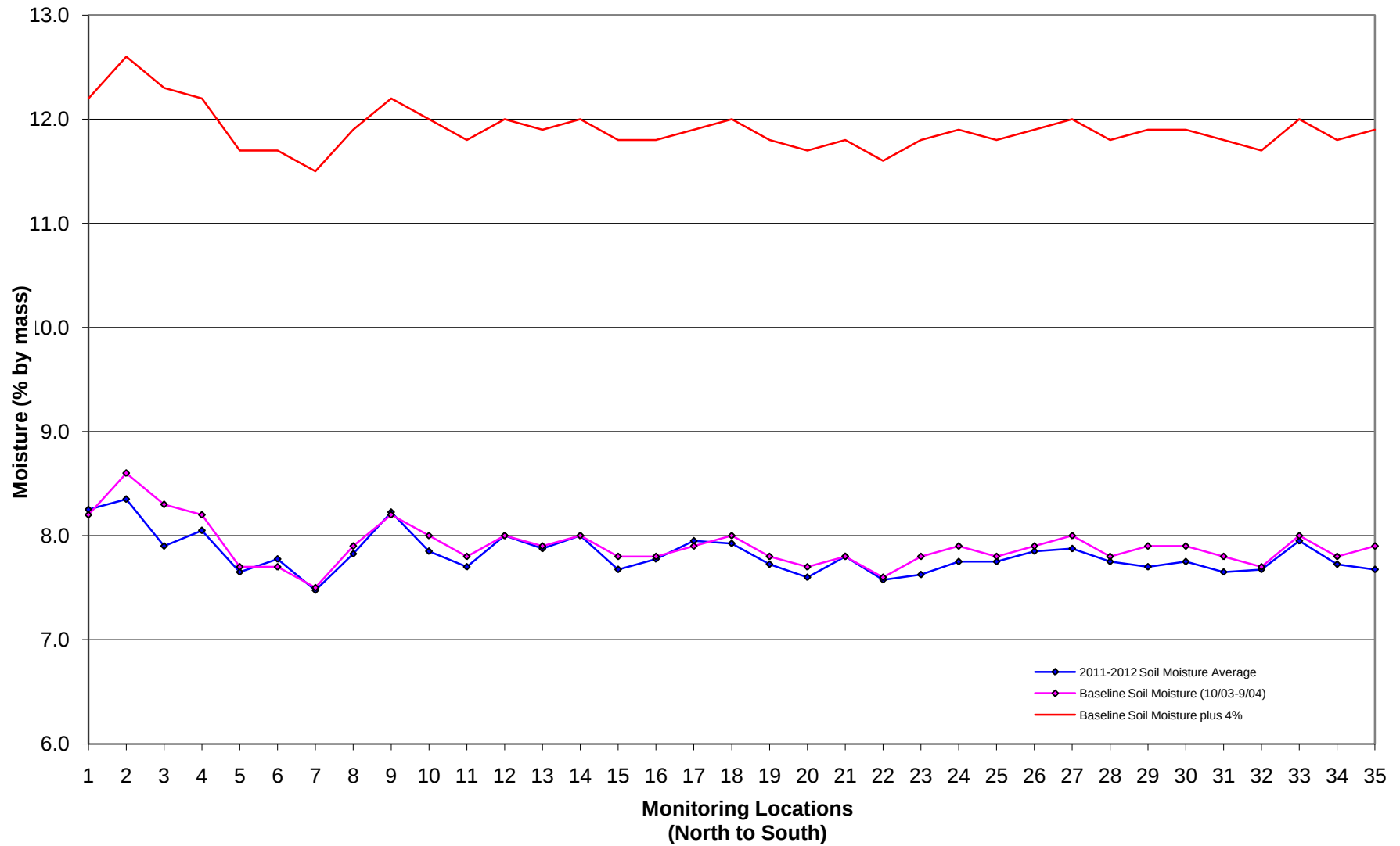
Figure A-3 Graph of PSL Soil Moisture Monitoring Results for the Central Access Tube July 2011–June 2012
