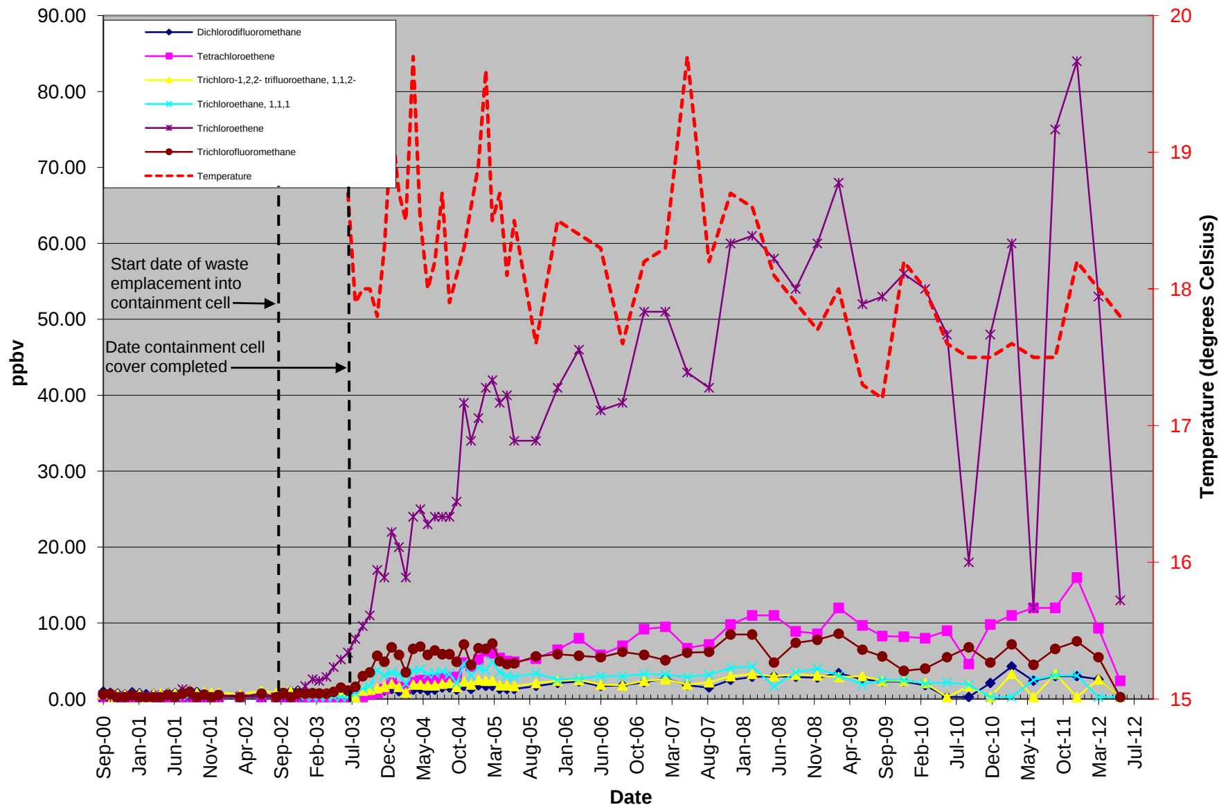
Figure D-12 Graph of VOC Concentrations at VSA3-15
