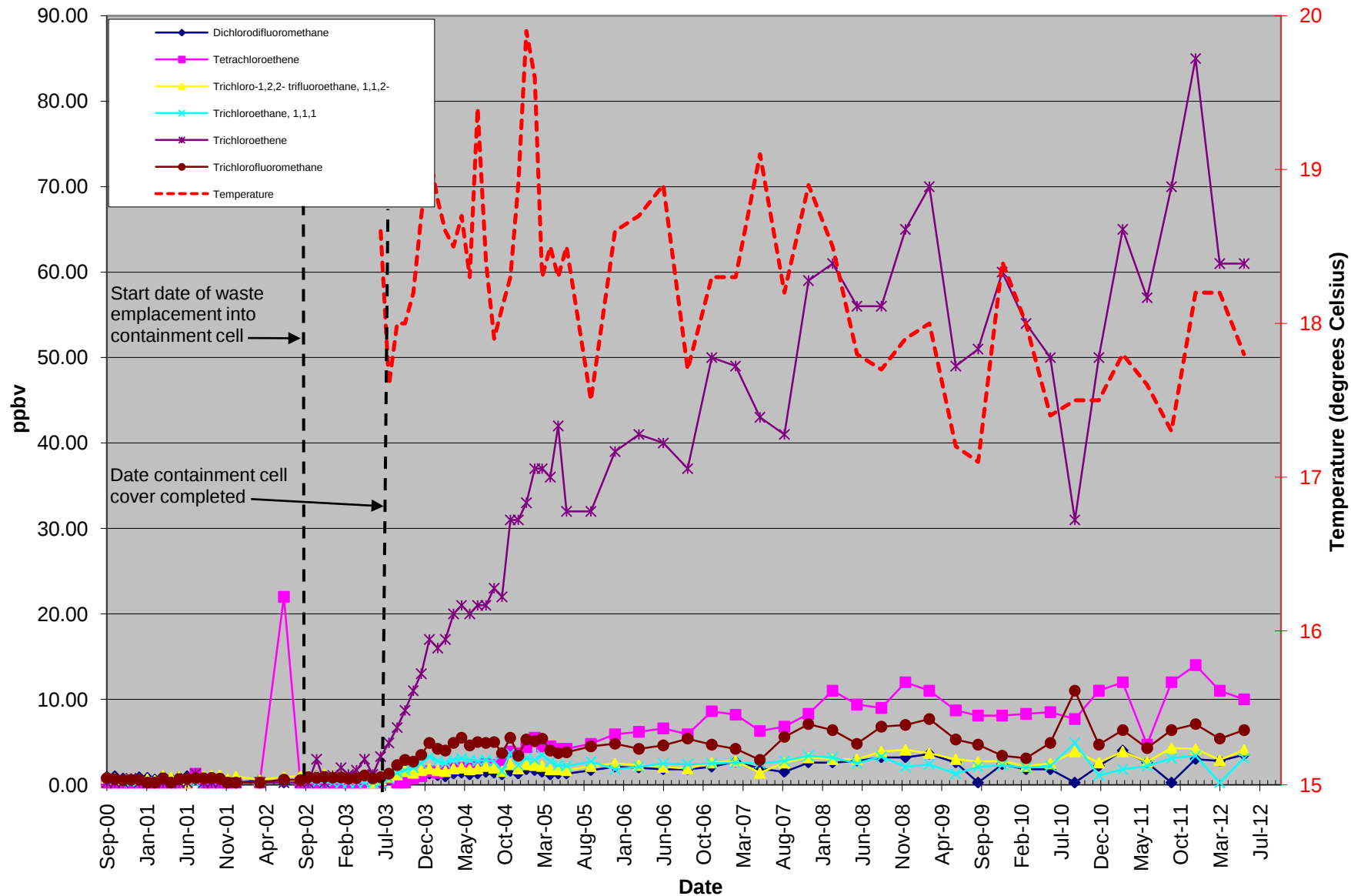
Figure D-10 Graph of VOC Concentrations at VSA2-15
