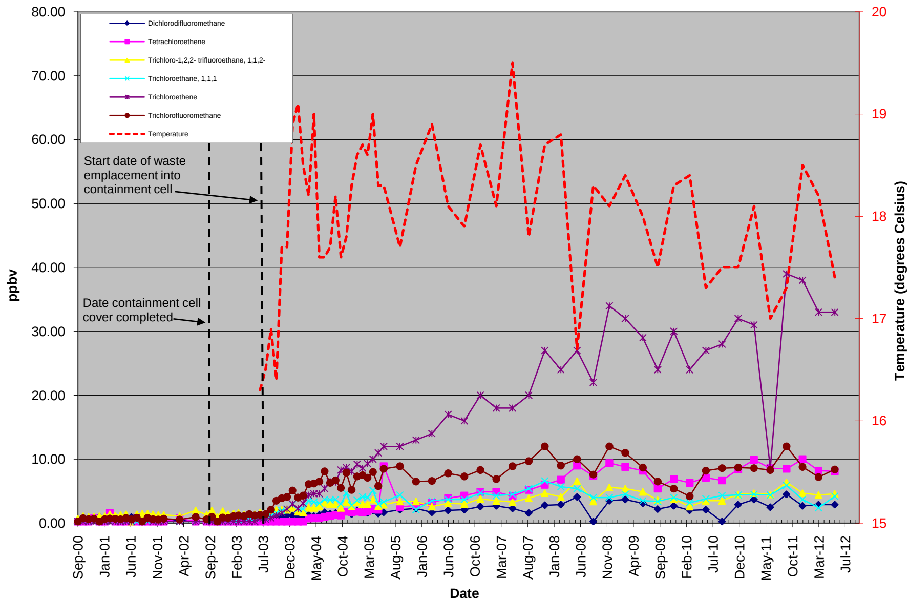
Figure D-23 Graph of VOC Concentrations at VSA9-5
