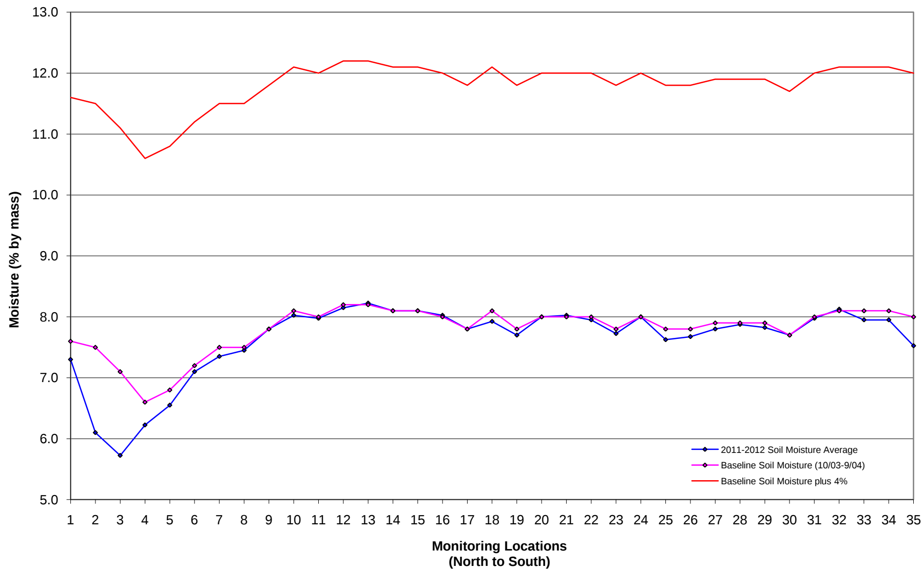
Figure A-2 Graph of PSL Soil Moisture Monitoring Results for the West-Central Access Tube July 2011–June 2012
