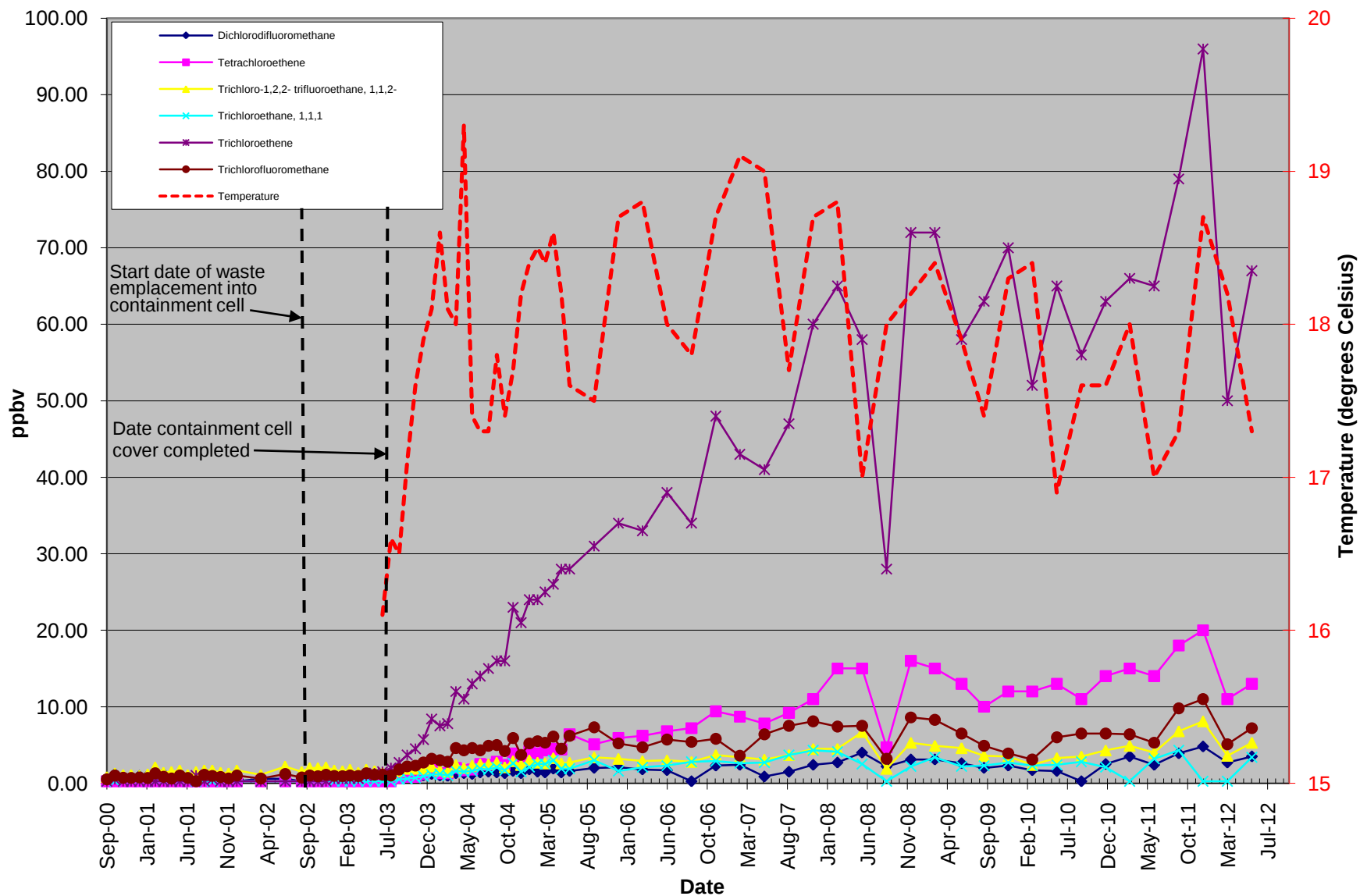
Figure D-21 Graph of VOC Concentrations at VSA8-5
