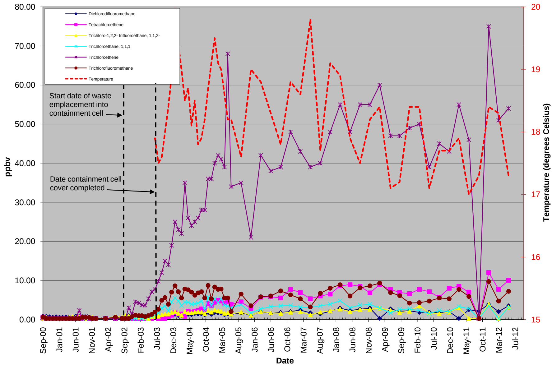
Figure D-13 Graph of VOC Concentrations at VSA4-5
