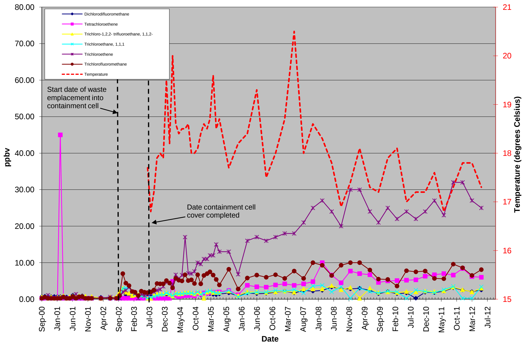
Figure D-27 Graph of VOC Concentrations at VSA11-5
