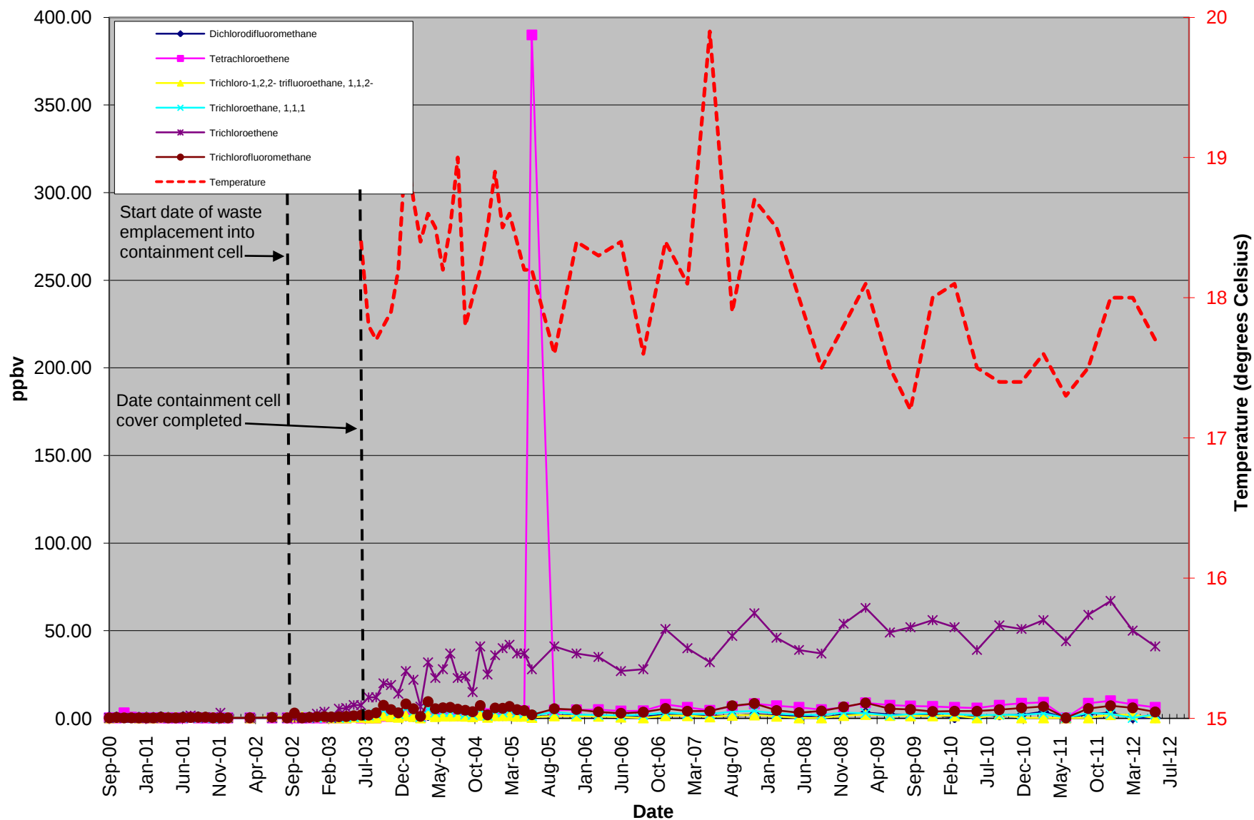
Figure D-14 Graph of VOC Concentrations at VSA4-15
