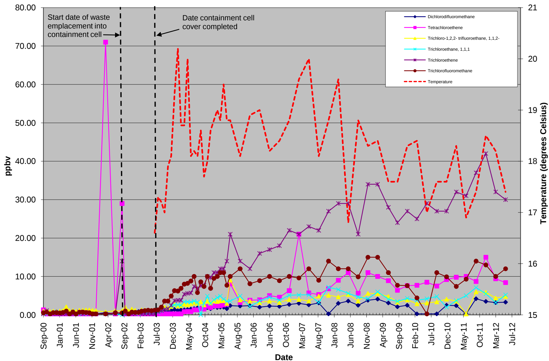
Figure D-25 Graph of VOC Concentrations at VSA10-5
