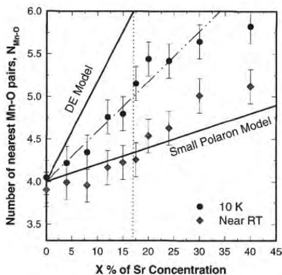
FIGURE 1a.9. The composition dependence of the Jahn-Teller polarons in CMR material, \text{La}_{1-x}\text{Sr}_x\text{MnO}_3 determined from pulsed neutron diffraction and the pair density function analysis from data collected at IPNS.
