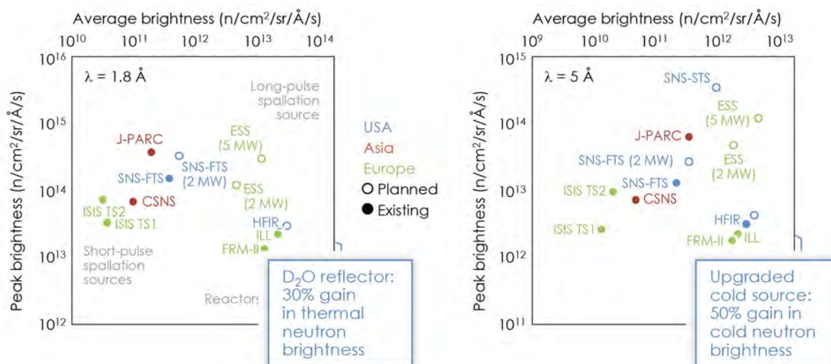
FIGURE A1.6. The Upgraded HFIR Will Provide World-leading Time-averaged Brightness for Both Cold and Thermal Neutrons
