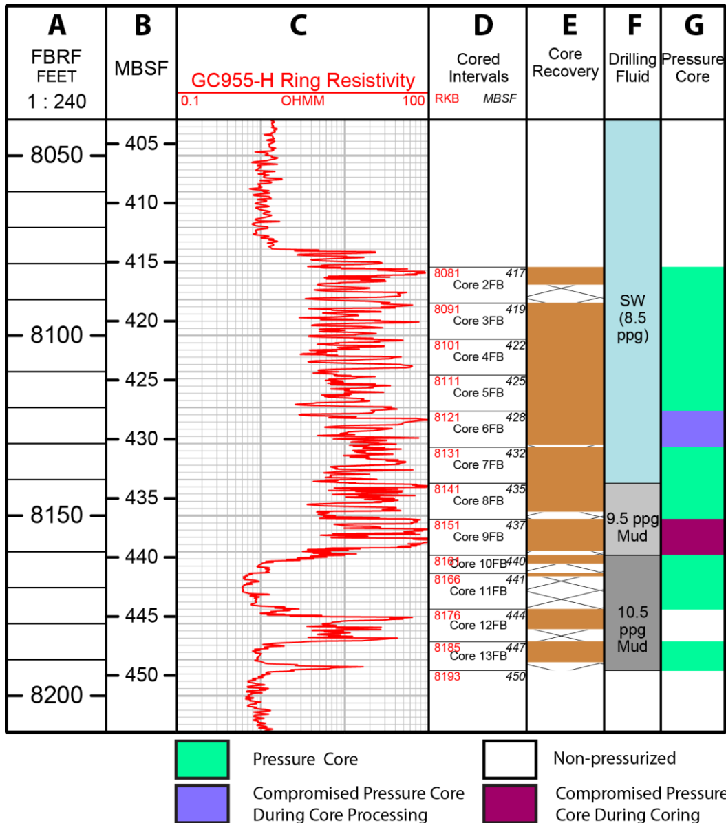
Figure 1.3.5 Cored intervals and core recovery from H005 compared to H001 resistivity log. The recovery is indicated by the brown box. Cores 2-7 were drilled with seawater, cores 8-9 were drilled with 9.5 ppg mud, and cores 10-13 were drilled with 10.5 ppg mud.
