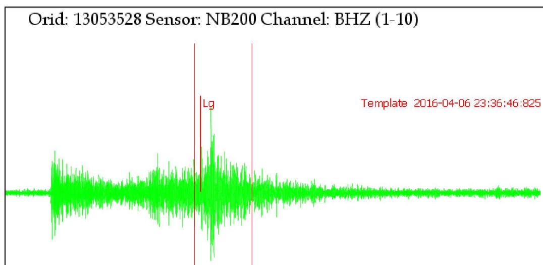
Figure 2-19. An example 60s NOA Lg template waveform for the NB200 element from an REB event located at (67.855°N, 20.197°E) on 2016-04-06 23:36 UTC.
