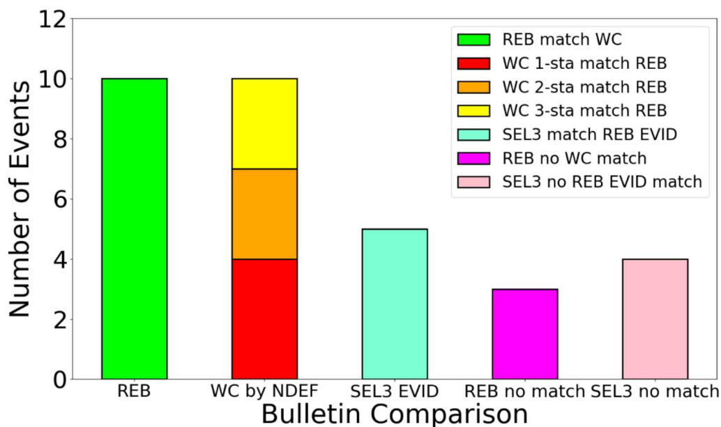
Figure 3-5. Number of Wyoming Week 1 events that are categorized in Figure 3-4 (same colors used on map). The first green column represents 10 REB events that matched WC events within tolerances of ( 1^\circ , \pm 15 s). The second column represents 10 WC events that matched the REB events, color-coded by number of detecting stations (PDAR, NVAR, TXAR). The third column represents 5 SEL3 events that were modified to become REB events (same EVID). The magenta column represents 3 REB events that did not match WC events within the tolerances. The pink column represents 4 SEL3 events that were discarded.
