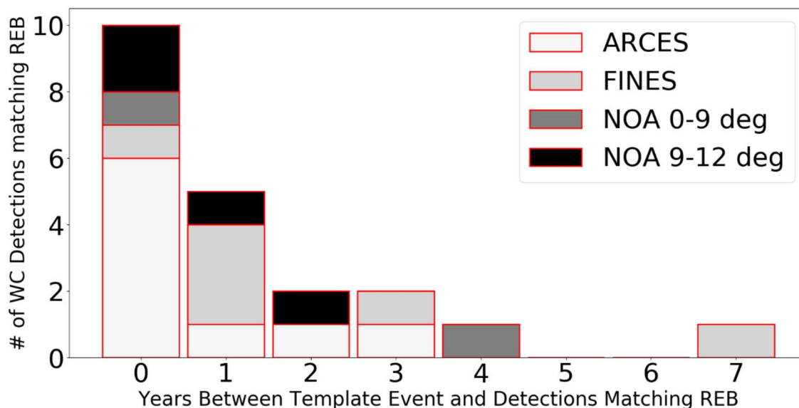
Figure 2-61. Number of Scandinavia Week 2 waveform detections matching the REB events, by age and by station.
