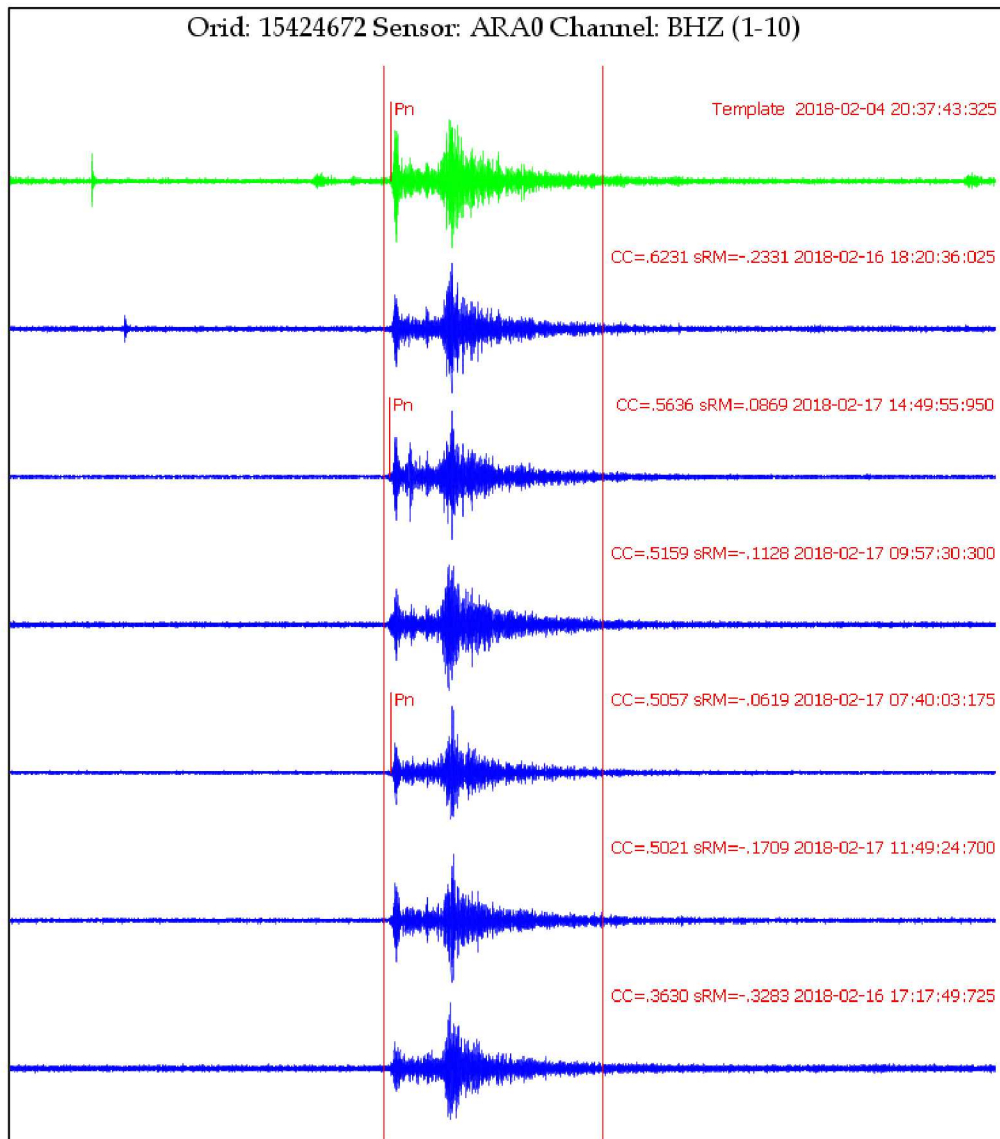
Figure 2-30. ARCES Pn template with a series of detections ordered by cross-correlation score. Two of the six detections were picked arrivals for the REB (the ones with labelled Pn picks).
