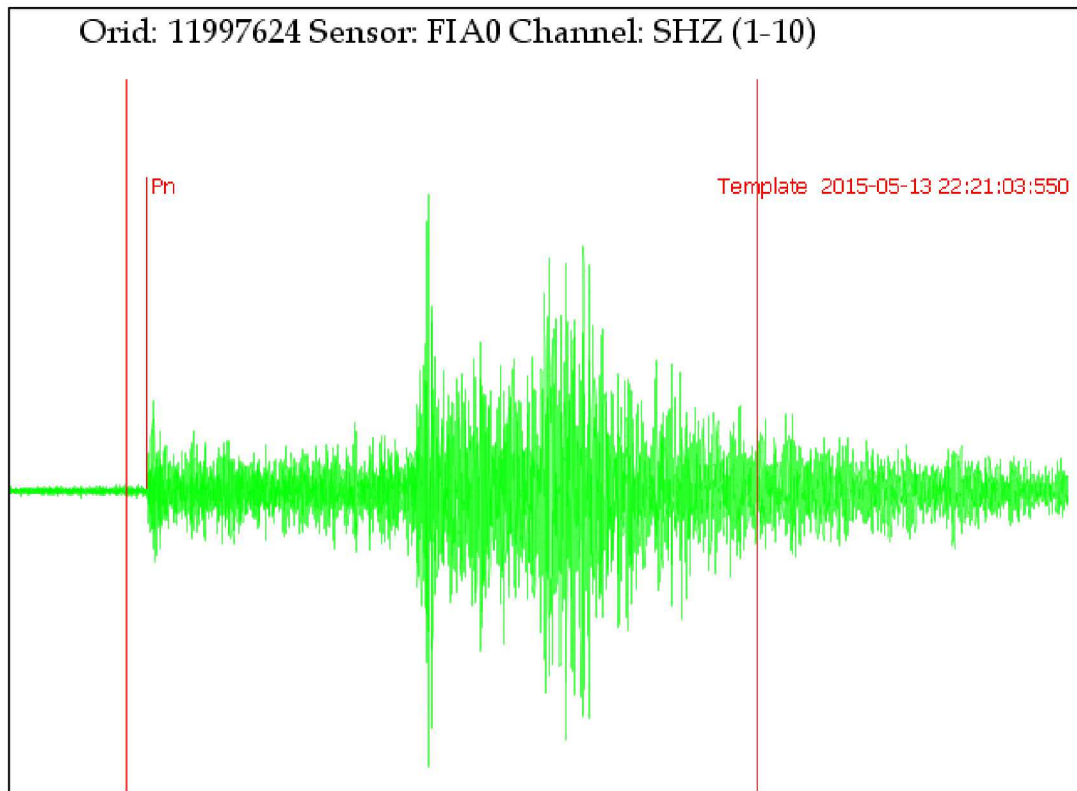
Figure 2-23. An example 160s FINES Pn template waveform for the FIA0 element from an REB event located at (67.209°N, 20.939°E) on 2015-05-13 22:21 UTC. The portion of the waveform between the two vertical red lines indicates the portion of the arrival waveform that is used as the template waveform for cross-correlation with continuous data.
