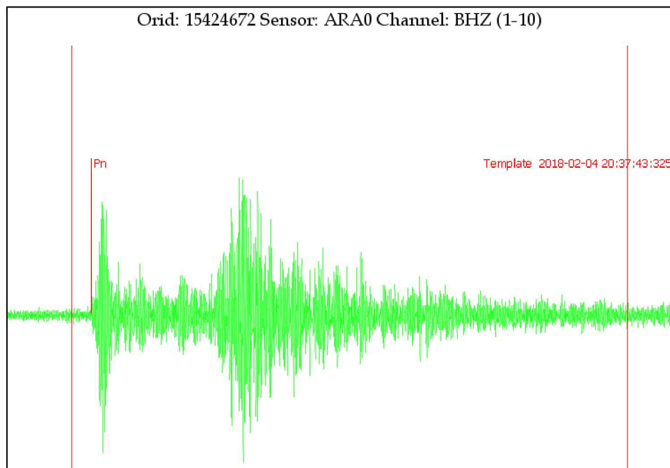
Figure 2-16. An example 140s ARCYES Pn template waveform for the ARA0 element. The portion of the waveform between the two vertical red lines indicates the portion of the arrival waveform that is used as the template waveform for cross-correlation with continuous data.
