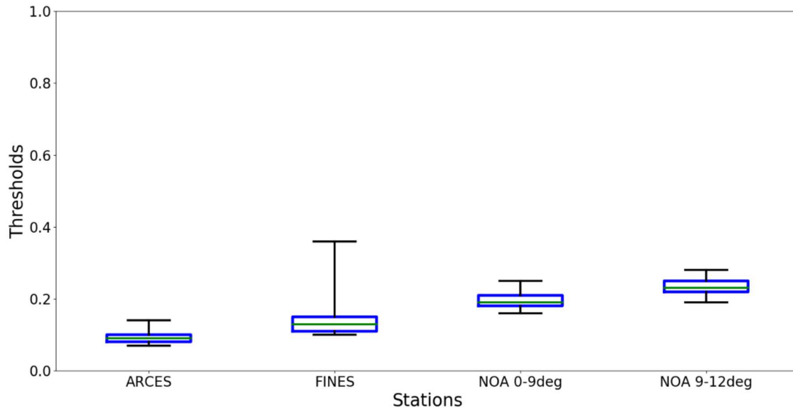
Figure 2-28. Statistics for Scandinavia Week 2 template threshold values. The box extends from the lower to upper quartile of the threshold values with a line representing the median threshold value. The minimum (maximum) threshold value is the bottom (top) line of the distribution.
