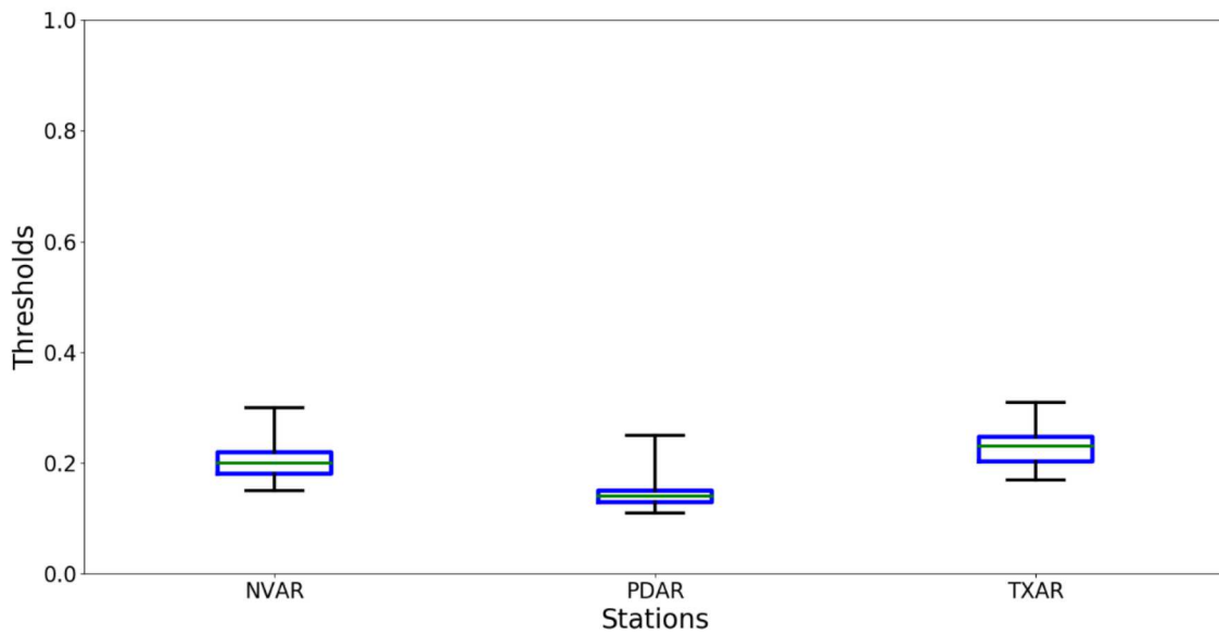
Figure 2-15. Statistics for Wyoming Week 2 template threshold values. The box extends from the lower to upper quartile of the threshold values with a line representing the median threshold value. The minimum (maximum) threshold value is the bottom (top) line of the distribution.
