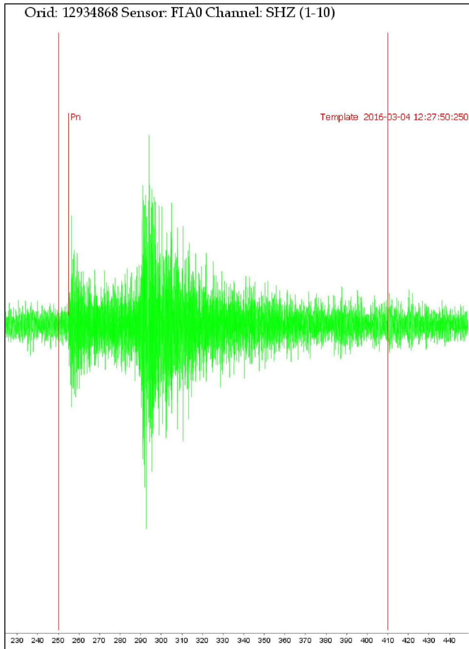
Figure 2-51. Example FINES template from REB ORID 12934868 (63.962, 28.036, 04-Mar-16 12:27:50) shown for comparison with missed REB event in Figure 2-50.
