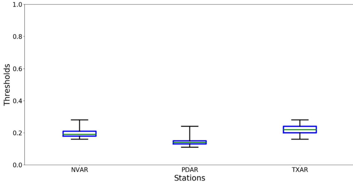
Figure 2-9. Statistics for Wyoming Week 1 template threshold values. The box extends from the lower to upper quartile of the threshold values with a line representing the median threshold value. The minimum (maximum) threshold value is the bottom (top) line of the distribution.
