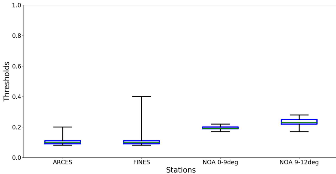
Figure 2-22. Statistics for Scandinavia Week 1 template threshold values. The box extends from the lower to upper quartile of the threshold values with a line representing the median threshold value. The minimum (maximum) threshold value is the bottom (top) line of the distribution.
