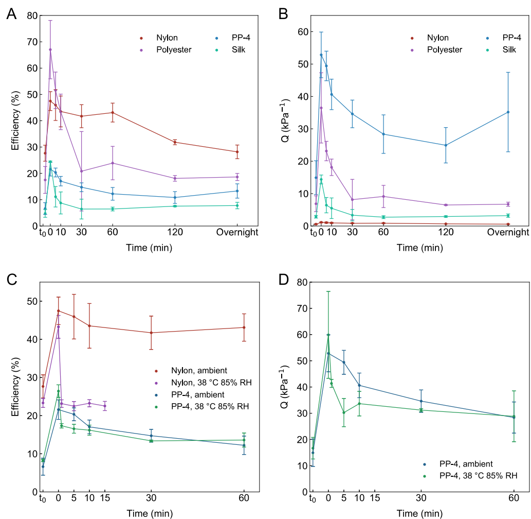
Figure 3. Time evolution of filtration properties of common materials. Each uncertainty represents the standard deviation of three samples. (a) Filtration efficiency decay in ambient conditions (listed in the main text), up to overnight. (b) Evolution of Q as a function of time, up to overnight. (c) Evolution of filtration efficiency in a humid and warmer environment, up to an hour. (d) Evolution of the PP-4 Q as a function of the time, up to an hour.
