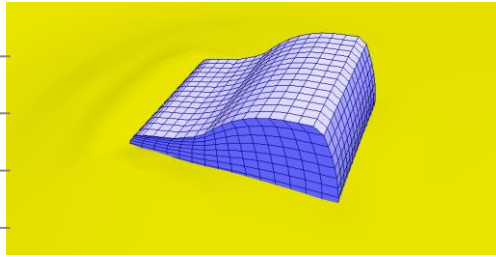
Azura Heave Oscillation Tests from OpenFOAM
