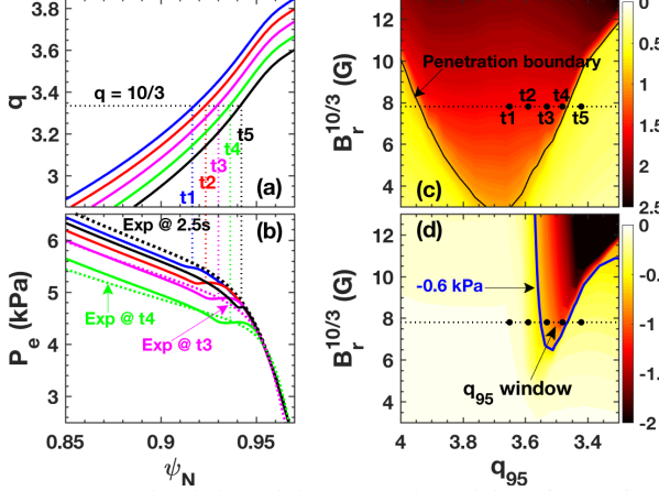
Fig. 2. TM1 simulation of the penetration of the m/n = 10/3 RMP and its effect on the electron pressure at different q_{95} for #145380: (a) q profiles at different times from Fig. 1d, (b) electron pressure profile from TM1 (solid) vs measurement (dashed) for each q -profile from t_1 - t_5 , (c) island width W_{10/3} from TM1 and (d) change in pedestal pressure \Delta P_{e,ped} from TM1 versus RMP strength and q_{95} , showing the five different times as black dots. The experimental pressure profiles before ELM suppression (black dashed) is shown in Fig. 2b.
