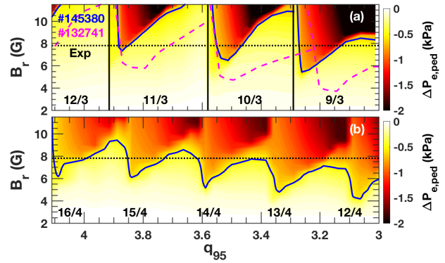
Fig. 5. TM1 simulation of the pedestal pressure change \Delta P_{e,ped} versus resonant field strength B_r (G) and q_{95} for (a) n = 3 RMP and (b) n = 4 RMP at high plasma density for discharge #145380 (Fig. 1a). The blue solid line corresponds to a 15% reduction in P_{e,ped} , and the purple dashed line in Fig. 5a corresponds to a 15% reduction in the pedestal pressure for the intermediate density discharge #132741 (Fig. 1b).
