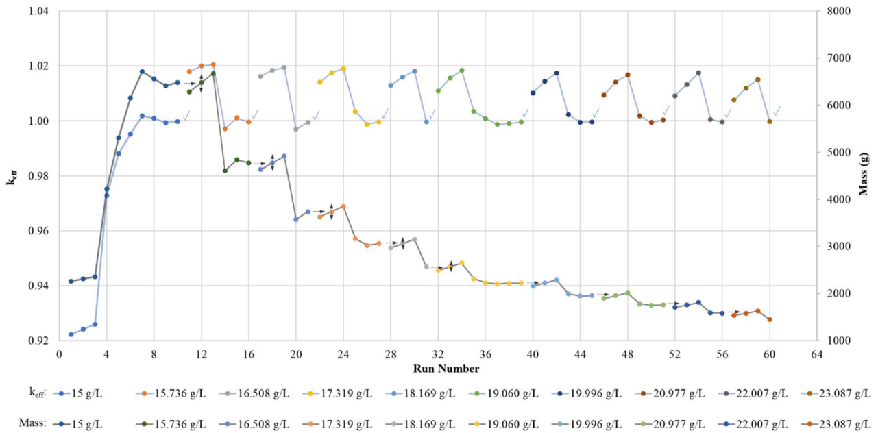
Figure 2. Convergence of k_{\text{eff}} and corresponding fissile mass for first 10 concentrations of ^{235}\text{U}
