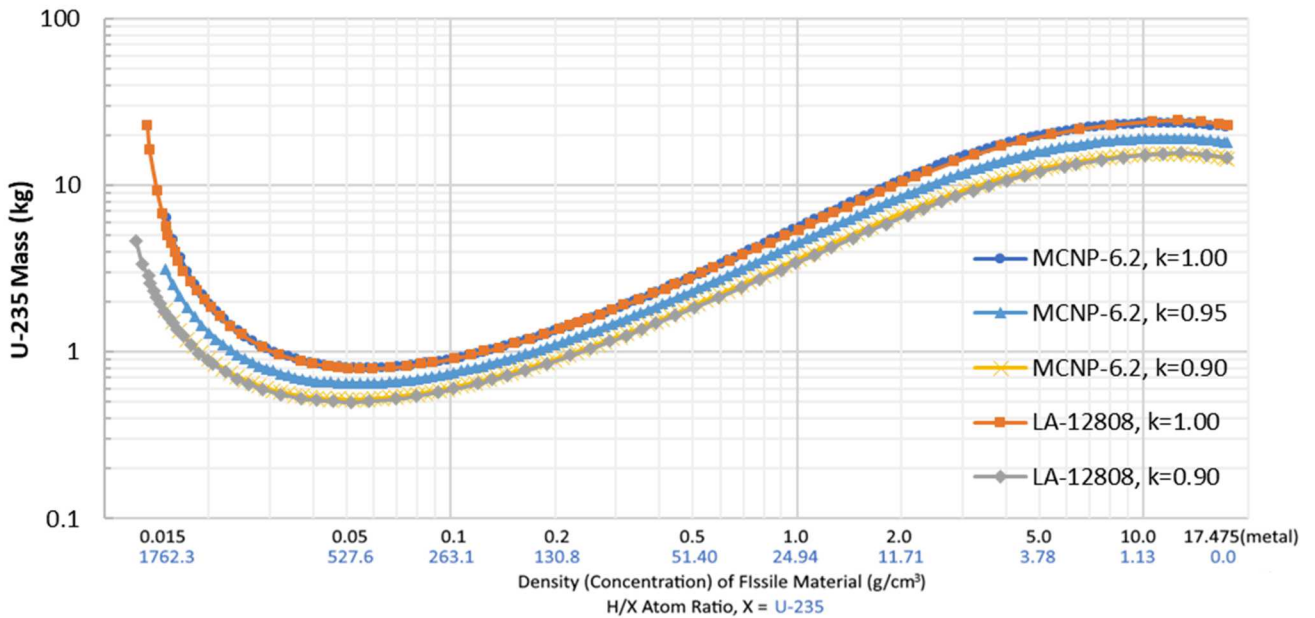
Figure 6. Critical and subcritical mass curves for ^{235}\text{U} as a function of ^{235}\text{U} concentration
