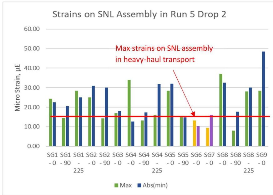
Figure 13. Strain on the SNL assembly in the most severe dry storage handling test.
