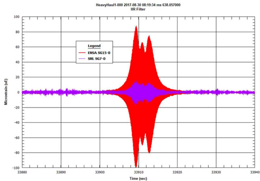
Figure 11. Example of characteristic shape of powerline interference.
