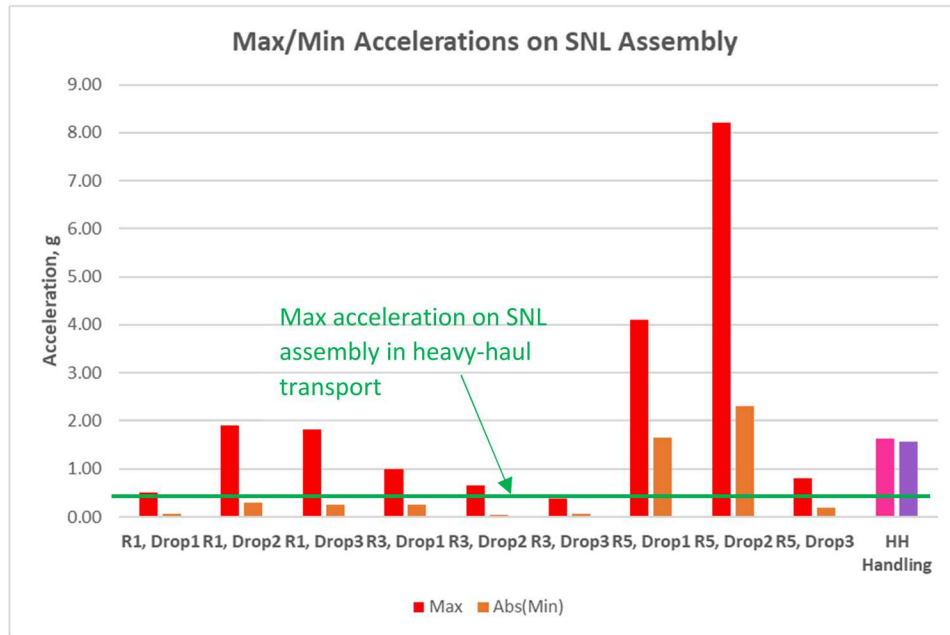
Figure 122. Maximum accelerations in dry storage and heavy-haul cask handling tests compared with maximum acceleration during heavy-haul transportation.
