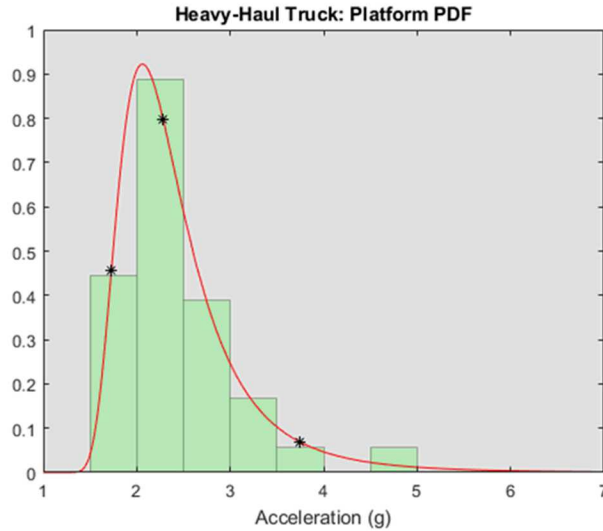
Figure 8. Truck platform acceleration histogram and Fréchet PDF for heavy-haul transport.
