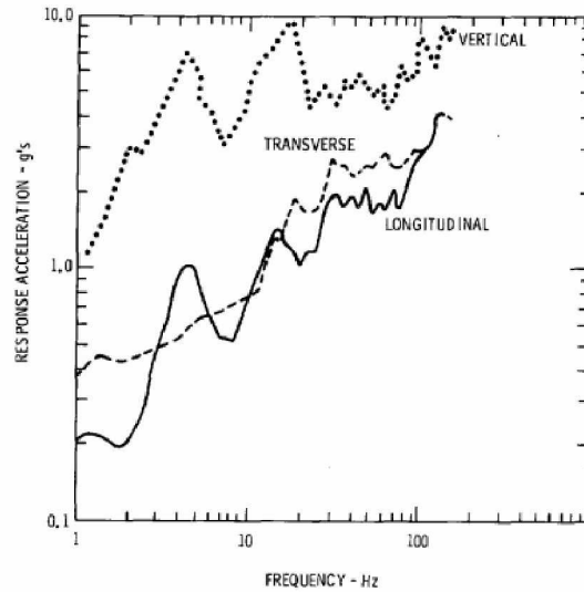
Figure 3. Shock response for truck transport from NUREG 766510 (SAND76-0427).
