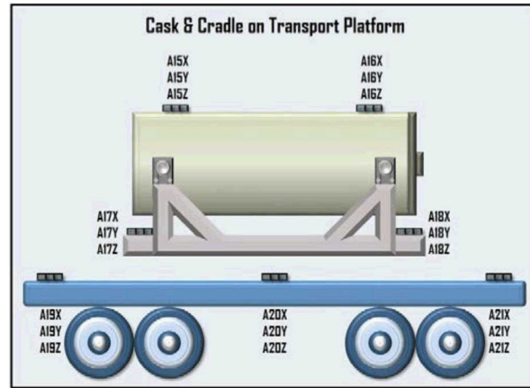
Figure 1. Truck platform, cask, and cradle accelerometer configuration.
