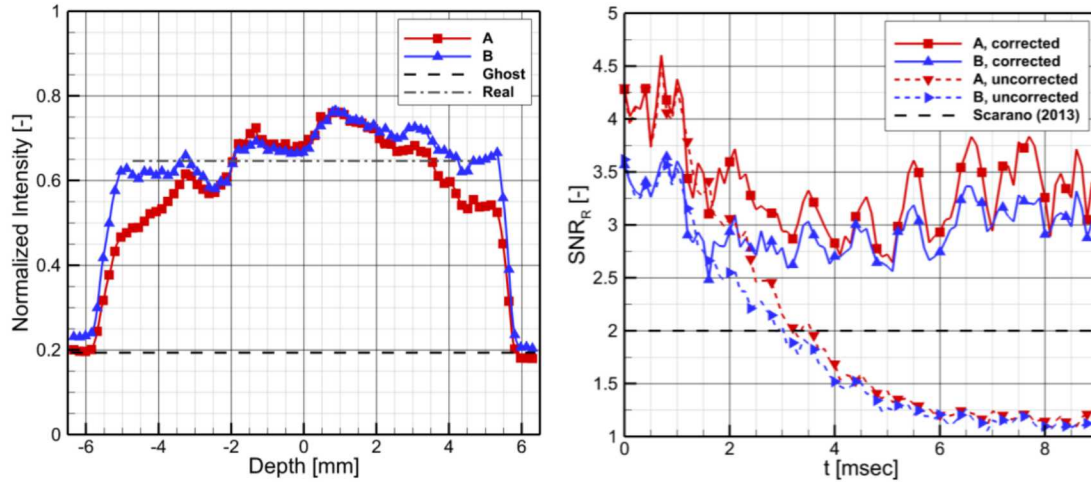
Figure 6. Left, Average reconstructed z-intensity profile for frames A and B with single-image self-calibration applied. Dashed regions indicate example intensities for calculation of the SNR. Right, SNR throughout the sequence with and without the single-image self-calibration. Data from run 1693, a 10 psi run.
