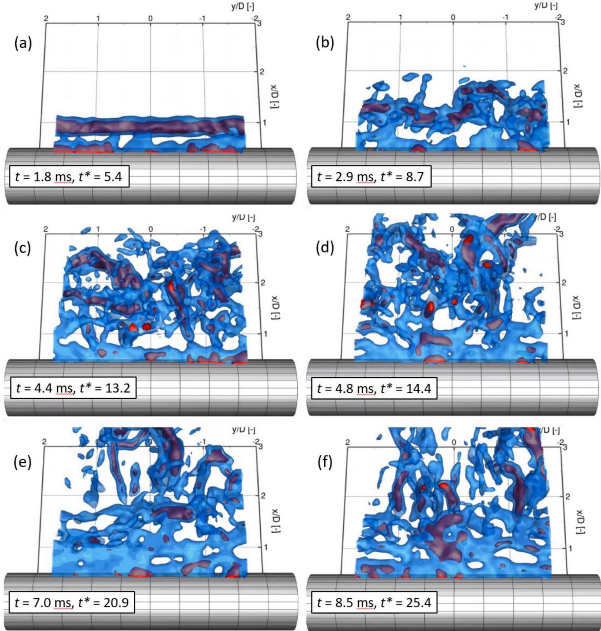
Figure 7. Vortex organization for Re_D = 31,000 . Isosurfaces of \omega^* = \omega D / u_\infty magnitude, values 6 (blue) and 10 (red).
