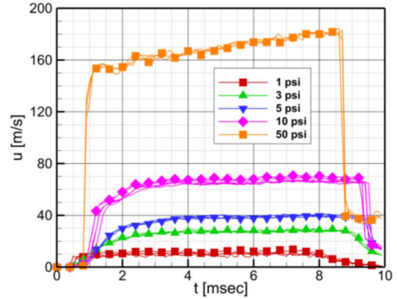
Figure 1: Freestream velocity for the empty shock tube at the test section location. Data from pulse-burst planar PIV acquired along a centerline plane. Overlays at each condition correspond to multiple runs.
