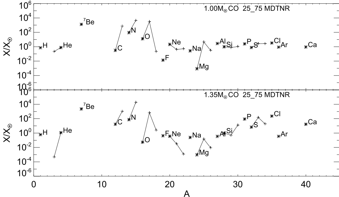
Figure 11. Top panel: the abundances of the stable isotopes from hydrogen to calcium in the ejecta for the 1.0 M_{\odot} CO WD sequence. The x -axis is the atomic mass and the y -axis is the logarithmic ratio of the abundance divided by the solar abundance (Lodders 2003). We also include {}^7\text{Be} in this plot, even though it is radioactive, because of its large overproduction. Both the initial {}^7\text{Li} and {}^6\text{Li} are depleted during the evolution. As in Timmes et al. (1995), the most abundant isotope of a given element is designated by an “*” and all isotopes of a given element are connected by solid lines. Any isotope above 1.0 is overproduced in the ejecta and a number of light, odd isotopes are significantly enriched in the ejecta as is {}^7\text{Be} . Bottom panel: the same plot as the top panel but for the 1.35 M_{\odot} simulation with 25% WD matter and 75% solar matter. Because of the higher peak temperature in this simulation, in addition to the light, odd isotopes of carbon, nitrogen, and oxygen, phosphorus, and chlorine are also enriched.
