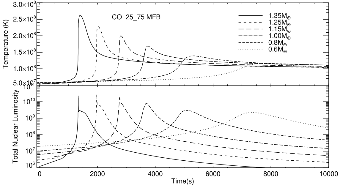
Figure 1. Top panel: the variation with time of the temperature in those mass zones near the interface between the outer layers of the CO WD and the accreted plus WD matter for the simulations with 25% WD material and 75% solar material. In these simulations we accreted the mixed composition from the beginning (MFB). The results for all six simulations are shown (the WD mass is identified in the legend). The curve for each sequence has been shifted in time to improve its visibility. As expected, the peak temperature achieved in each simulation is an increasing function of WD mass. Bottom panel: The variation with time of the total nuclear luminosity ( \text{erg s}^{-1} ) in solar units ( L_{\odot} ) around the time of peak temperature during the TNR. We integrated over all zones with ongoing nuclear fusion to obtain the plotted numbers. The identification with each WD mass is given on the plot and the evolution time has again been shifted to improve visibility. The cause of the sharp spike at the peak of the curve is discussed in the text.
