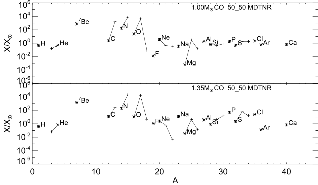
Figure 12. Top panel: the same plot as in Figure 11 but for the 1.0 M_{\odot} simulation with 50% WD matter and 50% solar matter. The most enriched species are ^{13}\text{C} , ^{15}\text{N} , ^{17}\text{O} , and ^7\text{Be} . Bottom panel: the same plot as the bottom panel in Figure 11 but for the simulation with a mass of 1.35 M_{\odot} and the 50% WD and 50% solar composition.
