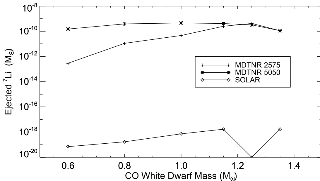
Figure 10. The predicted {}^7\text{Li} abundance in the ejecta as a function of WD mass in units of solar masses. The TNRs on CO WDs reach sufficiently high temperatures to deplete the initial {}^7\text{Li} present in the accreted material. The TNR then produces {}^7\text{Be} which is mixed to the surface by strong convection during the TNR and we actually plot that nucleus. {}^7\text{Be} decays ( \sim 53 day half-life) after the end of the simulations. The simulations where we mix from the beginning (MFB) eject far less {}^7\text{Li} and are not plotted here. The simulation with solar abundances on a 1.25 M_{\odot} WD did not eject any material.
