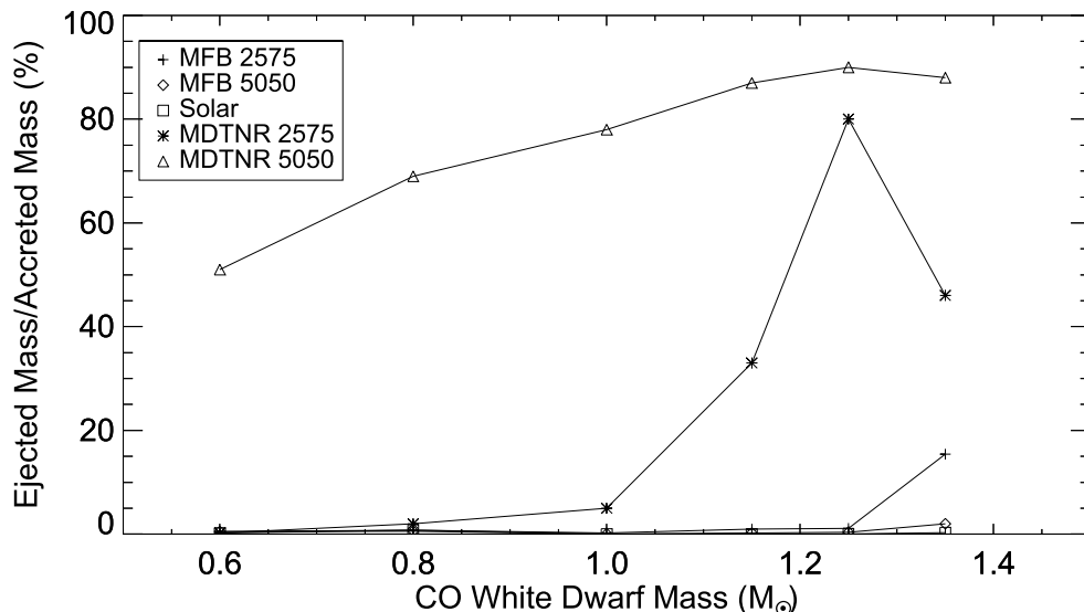
Figure 8. The ratio of ejected to accreted mass (in percent) as a function of CO WD mass. Neither the MFB nor the solar simulations eject much material and, thereby, the WD is growing in mass toward the Chandrasekhar Limit. While the 25% WD - 75% solar on the 1.25 M_{\odot} and 1.35 M_{\odot} simulations eject 81% and 46% of the accreted mass, respectively; only 25% of the ejecta is WD material and we predict that the WD is gaining in mass as a result of the CN outburst. The other sequences that eject a significant amount of material are the 50% WD and 50% MDTNR simulations on the massive WDs but only half of the ejecta is WD material.
