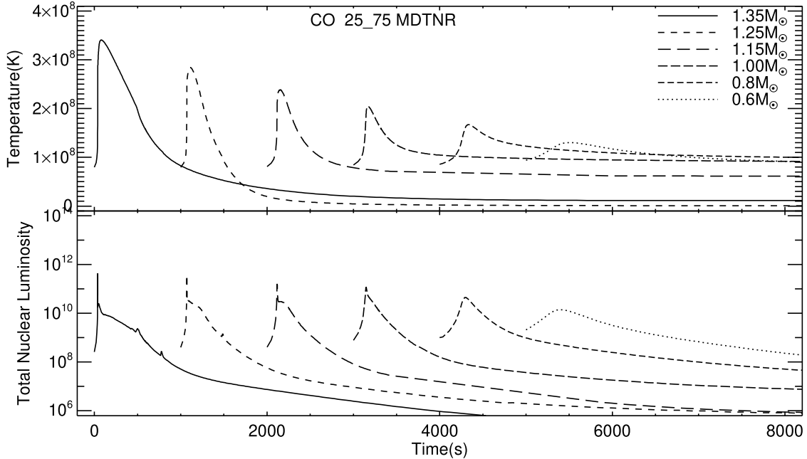
Figure 6. Top panel: the variation with time of the temperature in those mass zones near the interface between the outer layers of the WD and the accreted plus WD matter for the simulations with 25% WD material and 75% solar. This plot is the analog of the top panel of Figure 1. The results for all six simulations are shown (the WD mass is identified in the inset). The curve for each sequence has been shifted in time to improve its visibility. As expected, the peak temperature achieved in each simulation is an increasing function of CO WD mass. Bottom panel: same as the bottom panel of Figure 1 but for the simulation with 25% WD-75% solar. The small “glitches” that appear on the decline are caused by convection moving in and out and bringing in small amounts of fresh nuclei to the nuclear burning regime.
