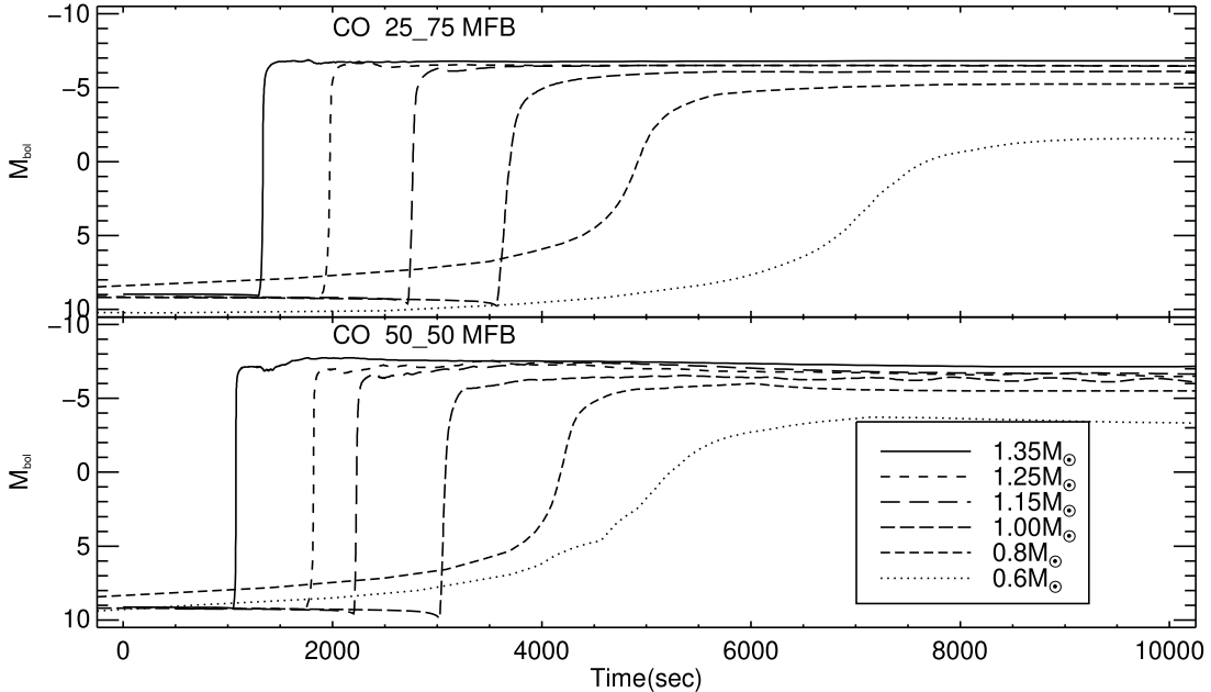
Figure 3. Top panel: the variation with time of the absolute bolometric magnitude for the simulations where we mixed a composition of 25% WD matter and 75% solar from the beginning (MFB). While the simulations on the more massive CO WDs reach values that agree with observations, those on the lower mass WDs are too faint to agree with the observations. Bottom panel: The same plot as in the top panel but for a mixed composition of 50% WD matter and 50% solar matter. Again the simulations on lower mass CO WDs do not reach to values that agree with typical CN observations where M_{\text{Bol}} is around -7 or higher. The small variations are real and suggest oscillatory behavior in the light curves but these times are normally before the nova is discovered.
