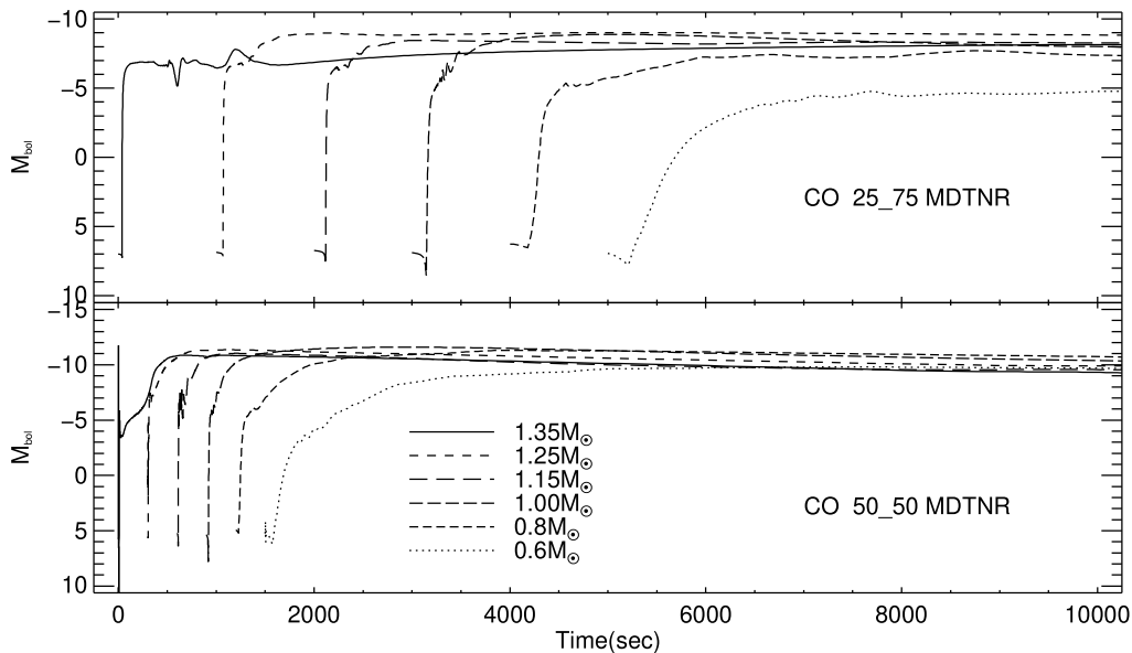
Figure 9. Top panel: the variation with time of the absolute bolometric magnitude for the simulations where we used a composition of 25% WD matter and 75% solar after the TNR was well underway (MDTNR). After the initial few hundred seconds they show a range in peak bolometric magnitude but there is no correlation with CO WD mass. Bottom panel: The same plot as in the top panel but for a composition of 50% WD and 50% solar. The large amount of ^{12}\text{C} in these simulations drives an initial shock in the most massive WD and the other simulations all reach a peak M_{\text{bol}} around -10 which is extremely bright for the typical CN outburst. We, therefore, claim that this choice of composition does not agree with observations.
