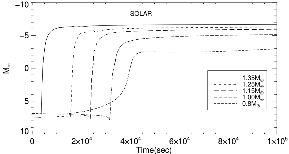
Figure 5. The same plot as shown in Figure 3 but for the solar composition simulations. Note that only the simulations on the most massive CO WDs reach peak values close to those that are observed. They also evolve extremely slowly compared to the mixed compositions (both MFB and MDTNR) as can be seen on the time axis. We do not plot the evolution of the 0.6 M_{\odot} simulation since it is still rising after 10^5 s.
