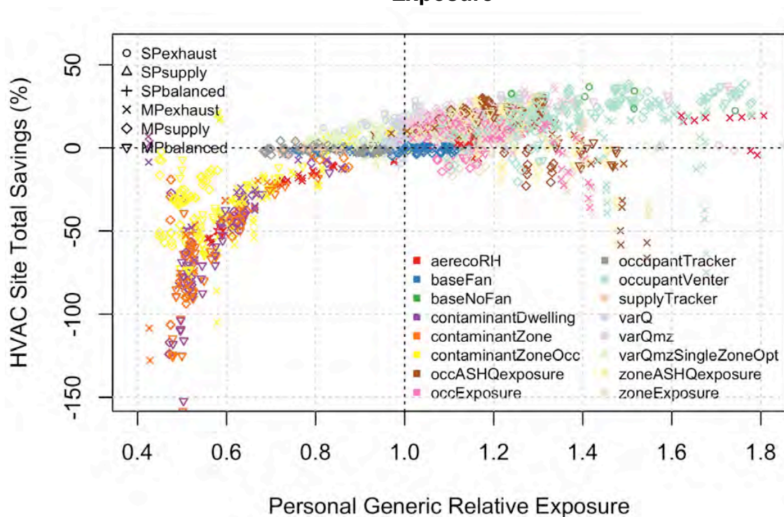
Figure 5: Site Energy Total HVAC Savings (%) and Personal Generic Relative Exposure
