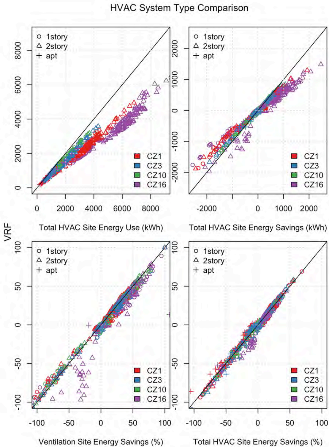
Figure 16 Comparison of Site Energy Performance by HVAC System Type. All Prototypes.
