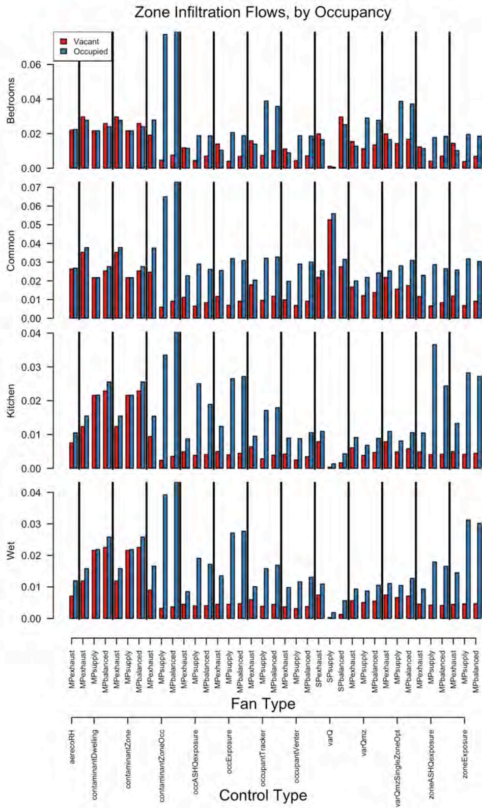
Figure 18: Infiltration ( \text{m}^3/\text{s} ) For Each Zone When Vacant vs. Occupied, by Control Type. 1-story dwellings, HPfau.
