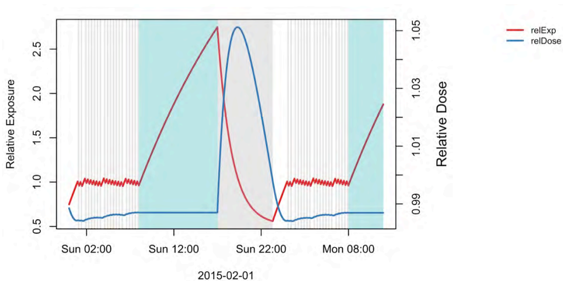
Figure 69 Illustration of Occupancy control operation with 1st shift occupancy schedule. IAQ fan periods highlighted in light grey, unoccupied period in aqua.
