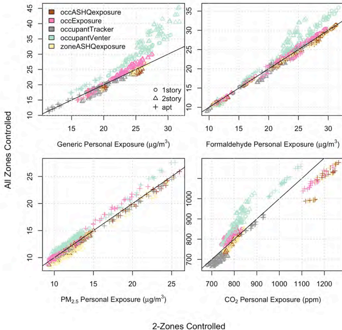
Figure 26: Comparison Of Personal Pollutant Exposure By Number of Control Zones.
