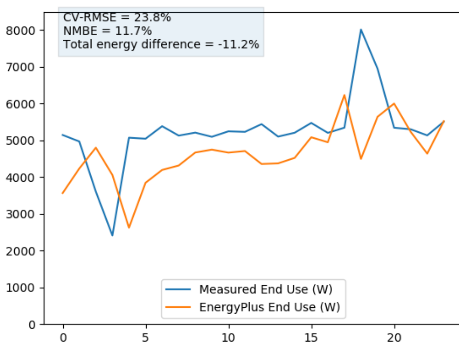
Figure 6. Comparison of measured and simulated power consumption for central heating baseline (sensor in master bedroom)
