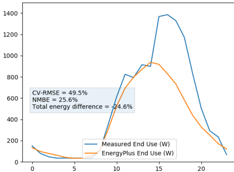
Figure 12. Comparison of measured and simulated power consumption for zonal cooling baseline (doors closed)
