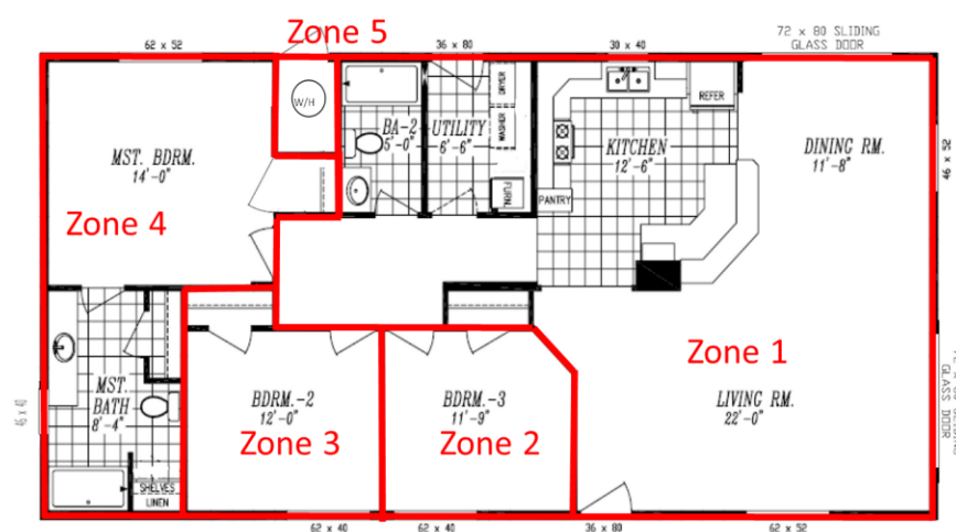
Figure 1. Lab Home floor plan and thermal zoning in the EnergyPlus model.
