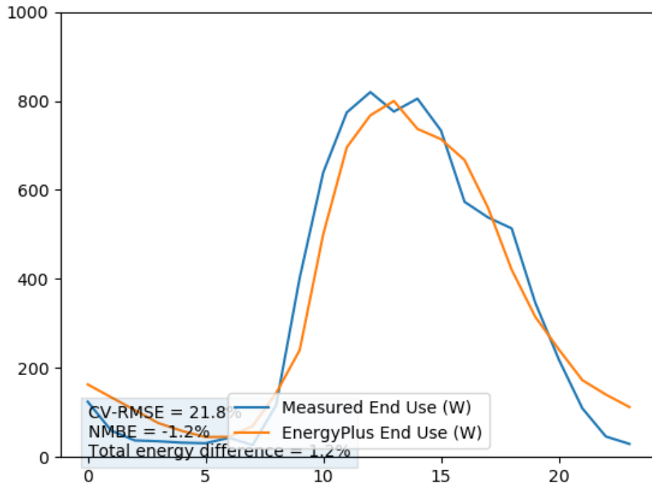
Figure 11. Comparison of measured and simulated power consumption for Zonal cooling baseline (doors open)
