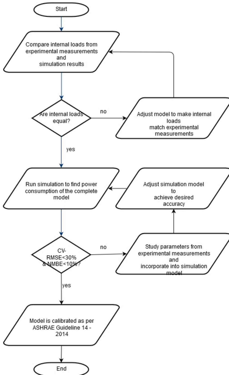
Figure 4. Flowchart indicating the process for model calibration
