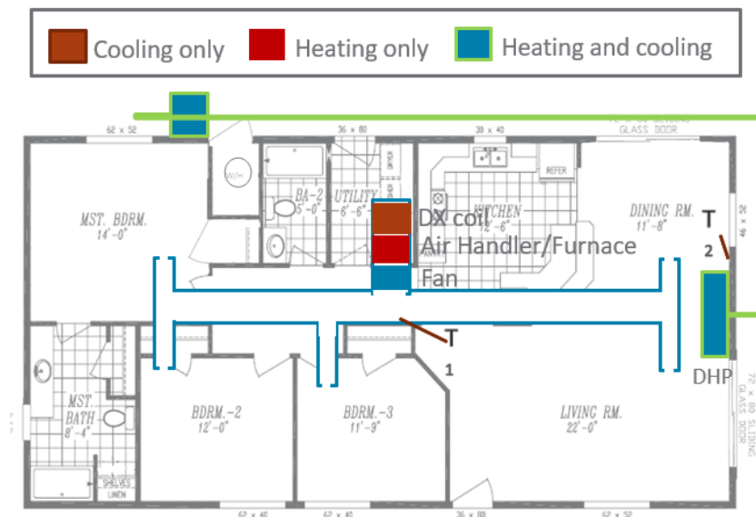
Figure 2. HVAC system configuration diagram for Central System with DHP
