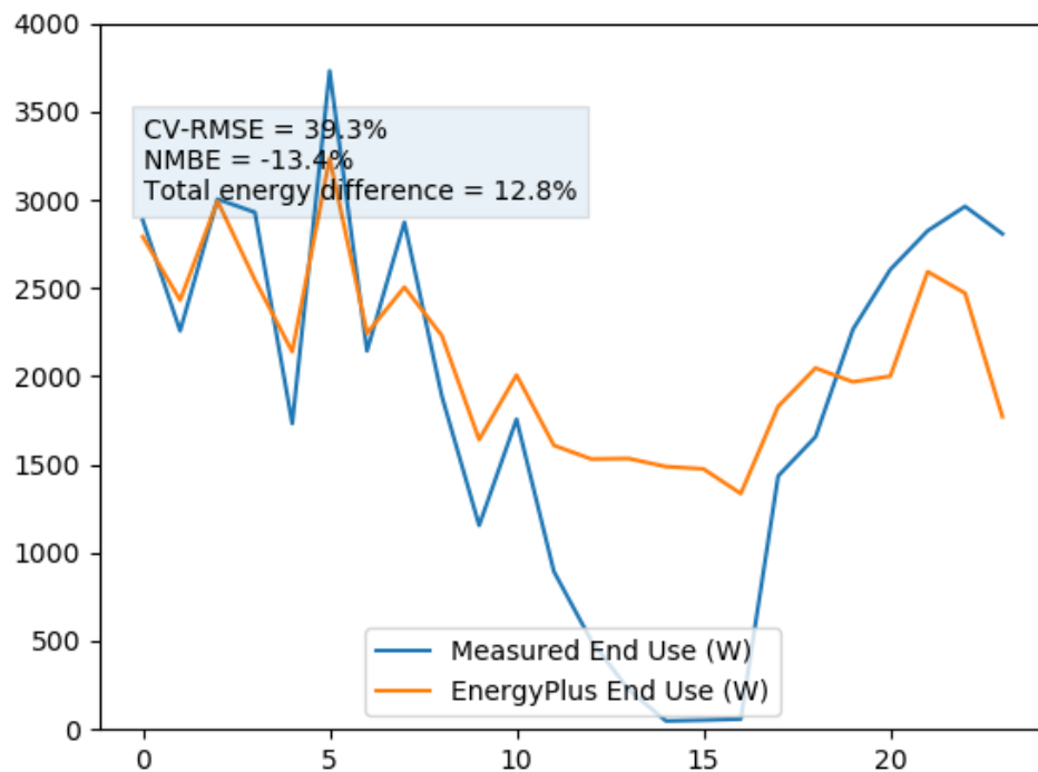
Figure 9. Comparison of measured and simulated power consumption for zonal heating baseline (doors open)
