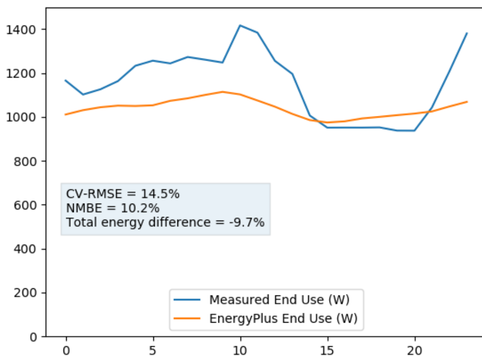
Figure 8. Comparison of measured and simulated power consumption for DHP only heating baseline.
