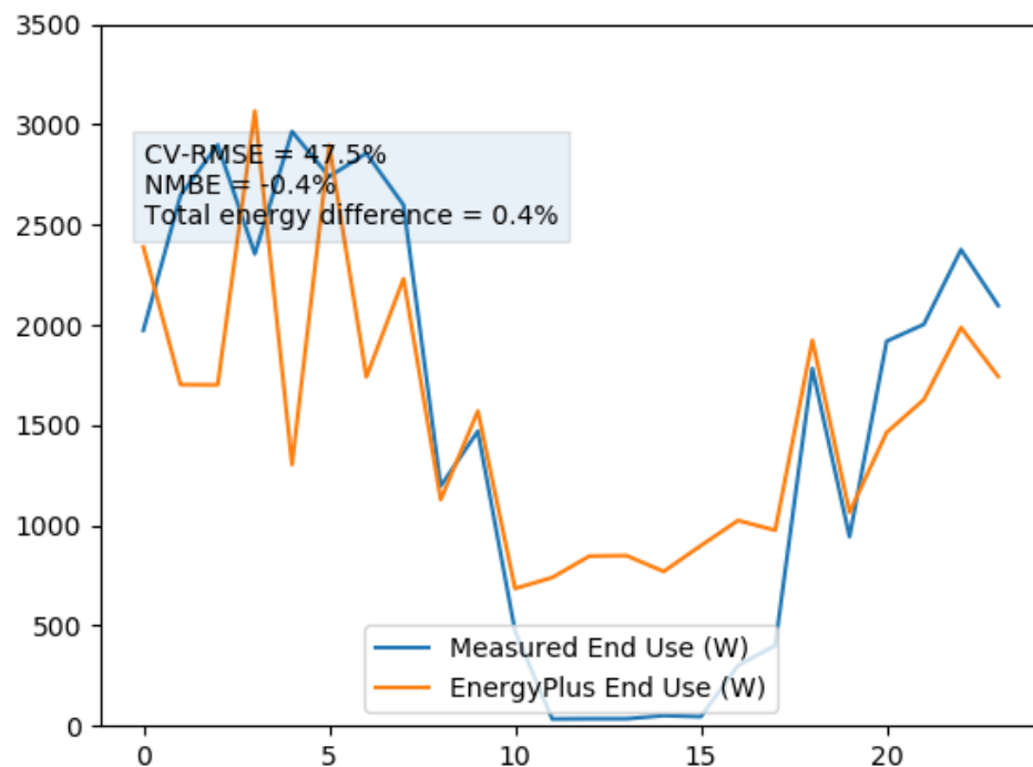
Figure 10. Comparison of measured and simulated power consumption for zonal heating baseline (doors closed)
