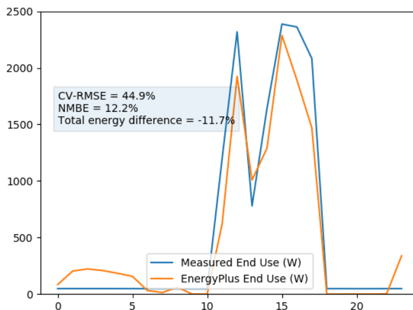
Figure 7. Comparison of measured and simulated power consumption for baseline model with central system in cooling mode (DHP disabled).
