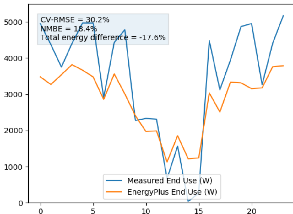
Figure 5. Comparison of measured and simulated power consumption for heating baseline – central system only
