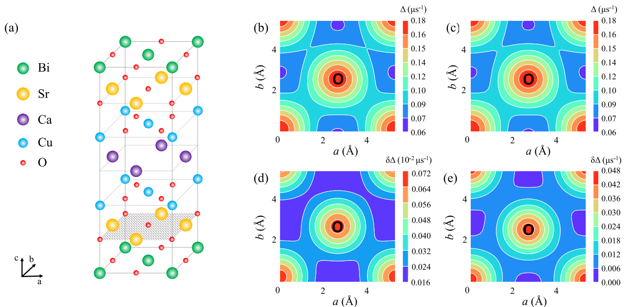
FIG. 6. (a) The orthonormal crystal structure of Bi2212 (only half of the crystal structure is illustrated for clarity). Contour plots of \Delta in the SrO layer (shaded plane) are calculated for (b) T = 150 K and (c) T = 5 K. (d) The difference between the \Delta values in (b) and (c) at 100 \times magnification. (e) The difference between the \Delta values within the SrO layer for T = 150 K and within a parallel plane 0.15 Å toward the nearest BiO layer for T = 5 K. Note that the large values for \Delta near the apical oxygen atoms are due to the Cu and Bi nuclei located directly below or above in the adjacent \text{CuO}_2 and BiO layers.
