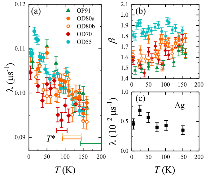
FIG. 4. Temperature dependence of (a) the ZF relaxation rate \lambda and (b) the stretching exponent \beta resulting from fits of the ZF- \mu SR asymmetry spectra assuming Eq. (3). The two data sets for the OD80 sample in (a) correspond to data collected during two separate experiments, demonstrating the reproducibility of the results. The range of T^* values shown at the bottom of panel (a) are compiled values from angle-resolved photoemission spectroscopy and tunneling experiments. 34 (c) Temperature dependence of the ZF relaxation rate in high purity Ag measured in the same experimental setup. Note that \lambda in this case comes from fits to Eq. (3) with \beta=1 .
