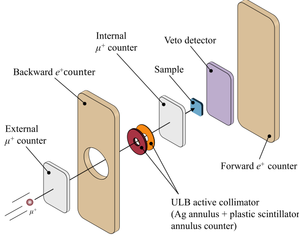
FIG. 2. Schematic of the arrangement of the external muon, external positron, internal muon and internal veto counters, where external and internal refer to outside and inside the helium-gas flow cryostat, respectively. Muons passing through the internal \mu^+ counter that trigger the veto counter are rejected. Also shown are internal Ag and plastic scintillator counter annuli with equivalent 3 mm-diameter holes. These serve as a second type of veto (“active collimator”) in the “ultra-low background” (ULB) setup. Muons stopping in the Ag annulus do not pass through the internal muon counter and are rejected. The Ag annulus protects the scintillator counter annulus from muons, so that it can be used to detect and reject positrons from decay muons in the Ag annulus.
