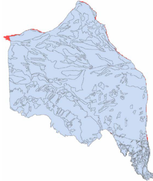
Figure 28. Missing Soil Type (in Red)
