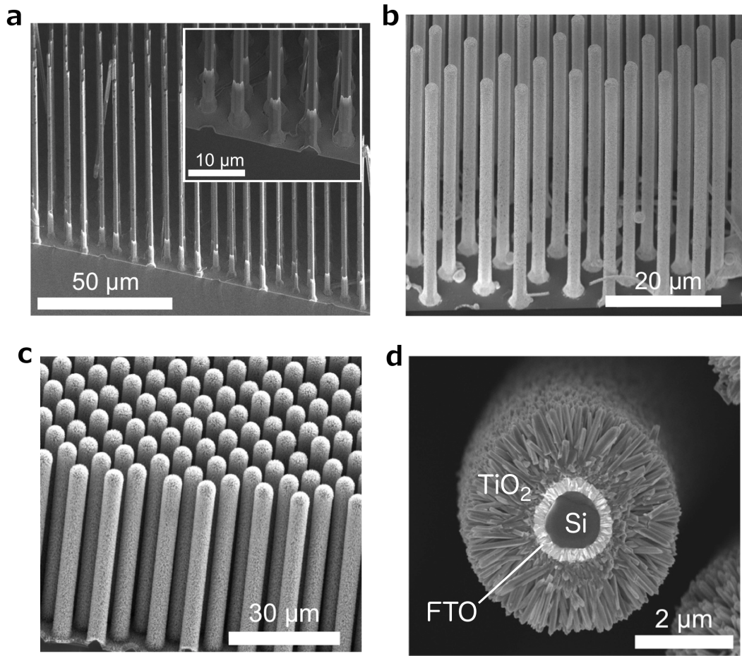
Figure 2: Scanning-electron microscopy (SEM) images showing samples at various stages in the fabrication process. a) A radial junction np + -Si microwire array ( Figure 1d ). Inset shows a zoomed-in image of the SiO 2 diffusion barrier at the bases of the microwires. b) FTO-coated np + -Si microwire array ( Figure 1e ). c) TiO 2 -coated np + -Si/FTO microwire array ( Figure 1f ). d) Cross section of a single np + -Si/FTO/TiO 2 microwire with each layer labeled.
