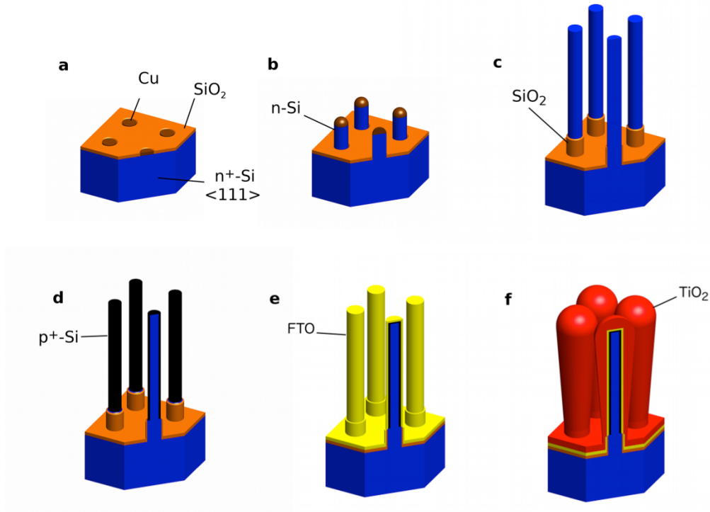
Figure 1: Schematic of the fabrication process. a) 3 \mu\text{m} diameter circular Cu growth catalysts photolithographically patterned in a 7 \mu\text{m} x 7 \mu\text{m} matrix in a 500 nm thick \text{SiO}_2 layer on an \text{n}^+\text{-Si} (111)-oriented wafer. b) \text{n-Si} microwire array growth at 1000 ^\circ\text{C} in a flowing gas consisting of \text{SiCl}_4 and \text{PH}_3 in \text{H}_2 . c) Metal and organic cleaned \text{Si} microwire array that has a \text{SiO}_2 diffusion barrier around each wire's base, formed by a dry oxidation of the entire wire array followed by a polymetyldisiloxane mask infill and subsequent etch in \text{HF(aq)} to remove the exposed \text{SiO}_2 . d) \text{p}^+\text{-Si} emitter formation by gas phase doping with \text{BCl}_3 . e) Conformal deposition of FTO by spray pyrolysis at 500 ^\circ\text{C} in air. f) \text{TiO}_2 deposition by an aqueous hydrothermal process followed by a 2 h anneal at 500 ^\circ\text{C} in air.
