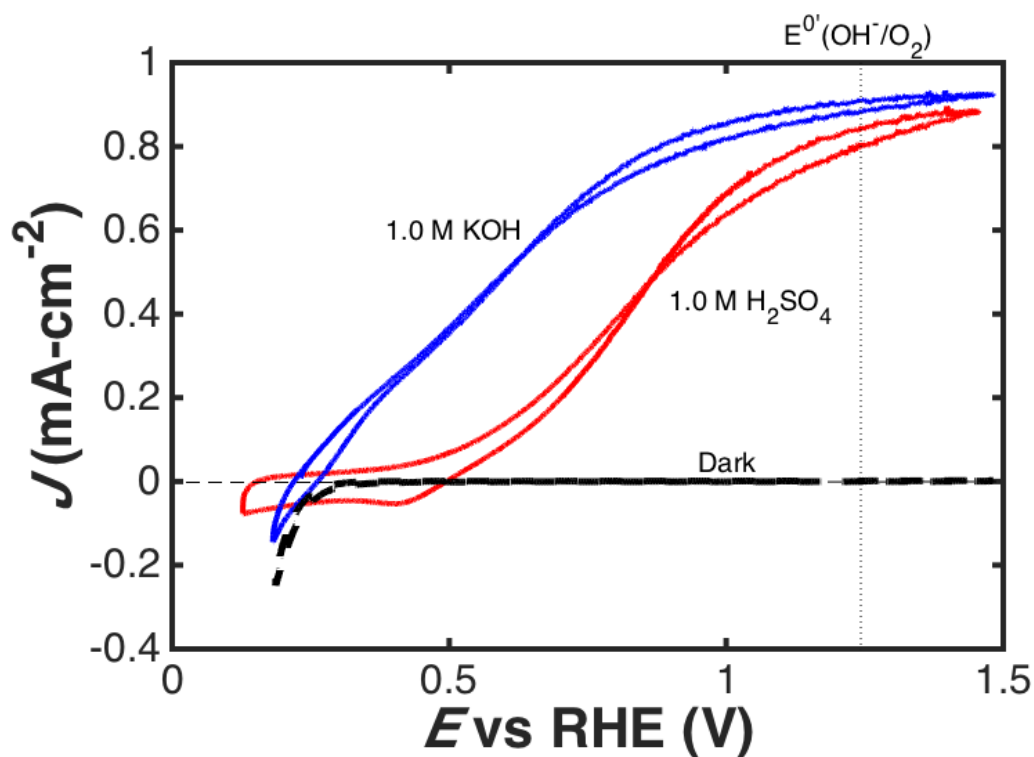
Figure 3: Current density versus potential behavior of p + -Si/FTO/TiO 2 microwire array photoelectrodes under dark (1.0 M KOH) and simulated 1 Sun conditions in 1.0 M KOH(aq) and in 1.0 M H 2 SO 4 (aq). This behavior demonstrates the superior photoanode performance in 1.0 M KOH, consistent with higher catalytic activity for oxygen evolution on the TiO 2 surface in alkaline media relative to under acidic conditions.
