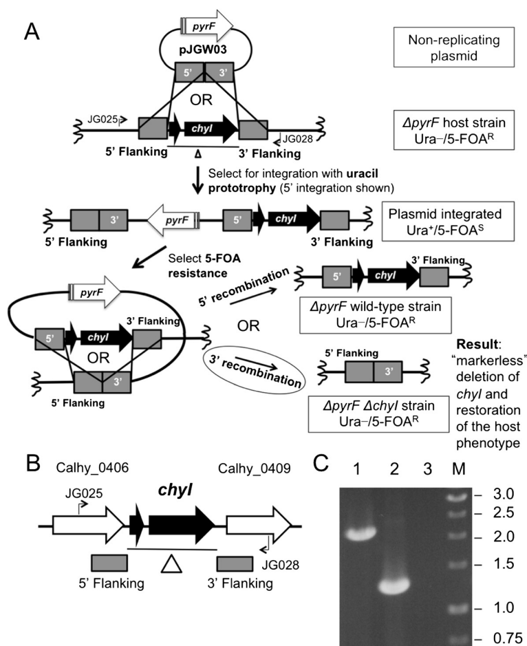
Figure 4 Deletion of the gene encoding putative restriction enzyme Chyl. A) Scheme for targeted gene deletion. The pJGW03 chyl knockout vector is transformed into JWCH006 ( \Delta pyrF), and uracil prototrophy selects for integration at one of the 500-bp flanking regions, denoted by the gray boxes. 5' integration is shown. The uracil prototroph is then plated on 5-FOA to select for loop-out of the pyrF cassette via homologous recombination between flanking region sequences. The two possible results are a return to the wild-type sequence or a clean chyl deletion. (B) Chromosomal map of the locus containing the ORF for chyl . The deleted region is indicated by the line below the diagram. Bent arrows depict primers used to verify deletion of chyl in the JWCH008 strain. (C) Gel depicting PCR products of the chyl region in the JWCH006 \Delta pyrF strain (2.3 kb) compared to the JWCH008 \Delta pyrF \Delta chyl strain (1.25 kb) amplified by the indicated primers (JG025 and JG028). 1: C. hydrothermalis JWCH006 genomic DNA; 2: C. hydrothermalis JWCH008 genomic DNA; 3: negative control; M: 1 kb DNA ladder (NEB).
